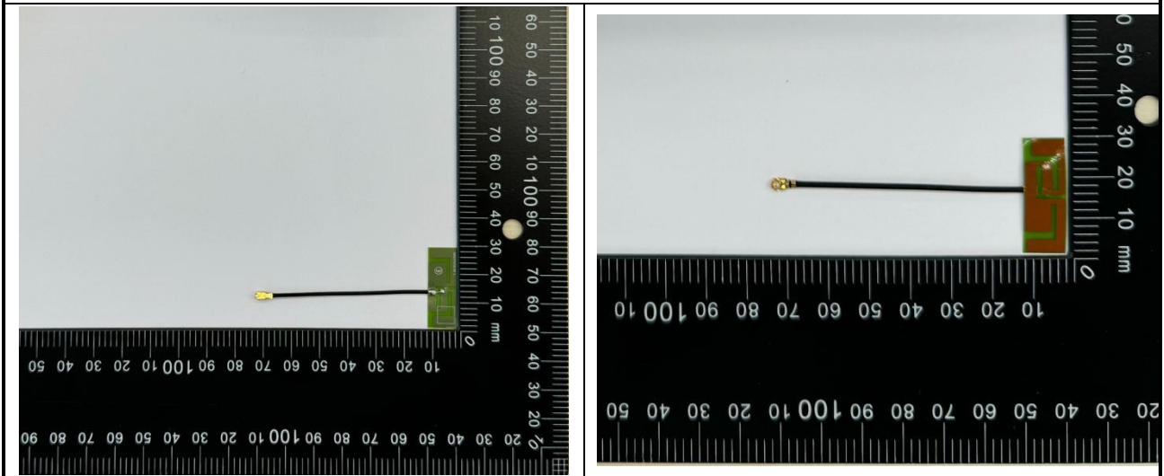
Fig.2 Antenna #3 (WLAN 2.4GHz/5GHz)
