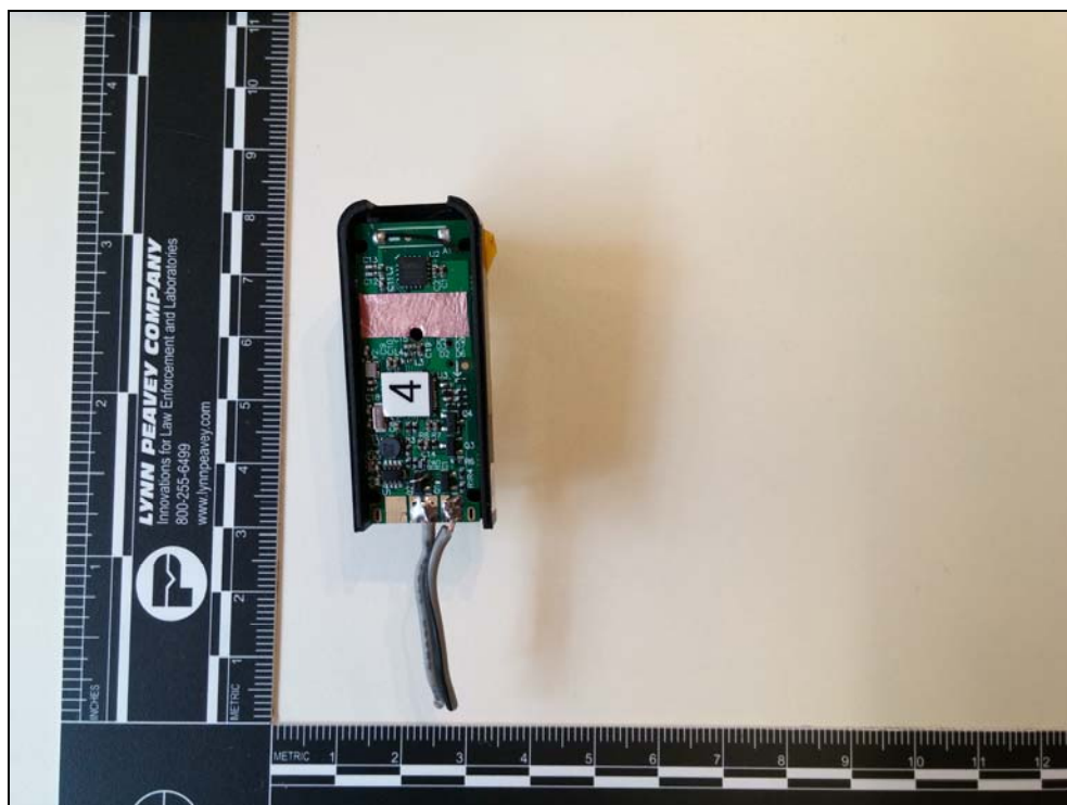
Figure 1: Mainboard Back – With Copper Foil – In Plastic
