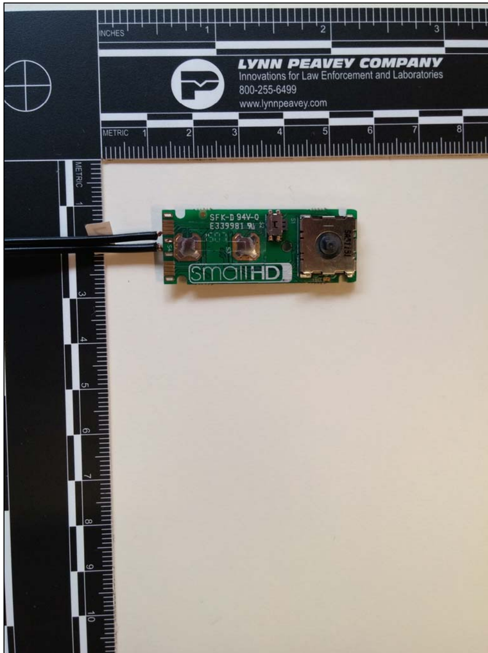
Figure 3: Mainboard - Front
