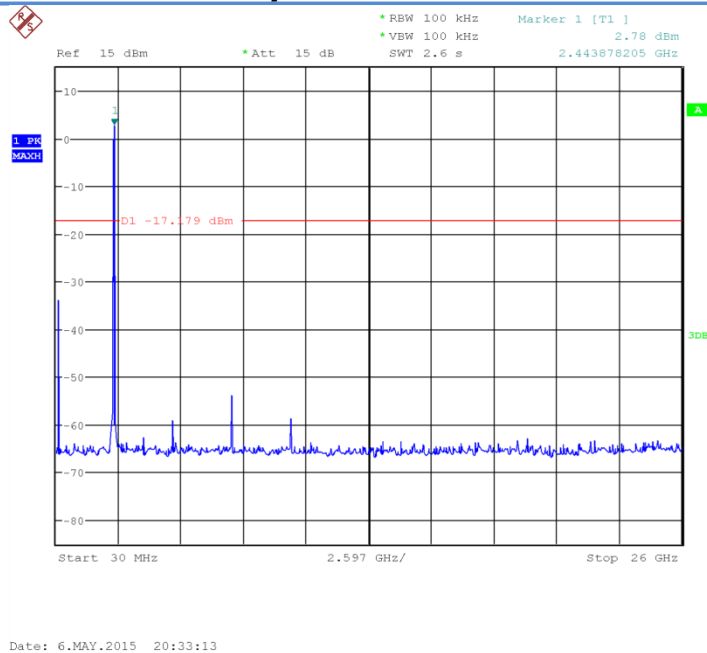
Fig.28 Conducted Spurious Emission (802.11b, Ch6, 30MHz~26GHz)
