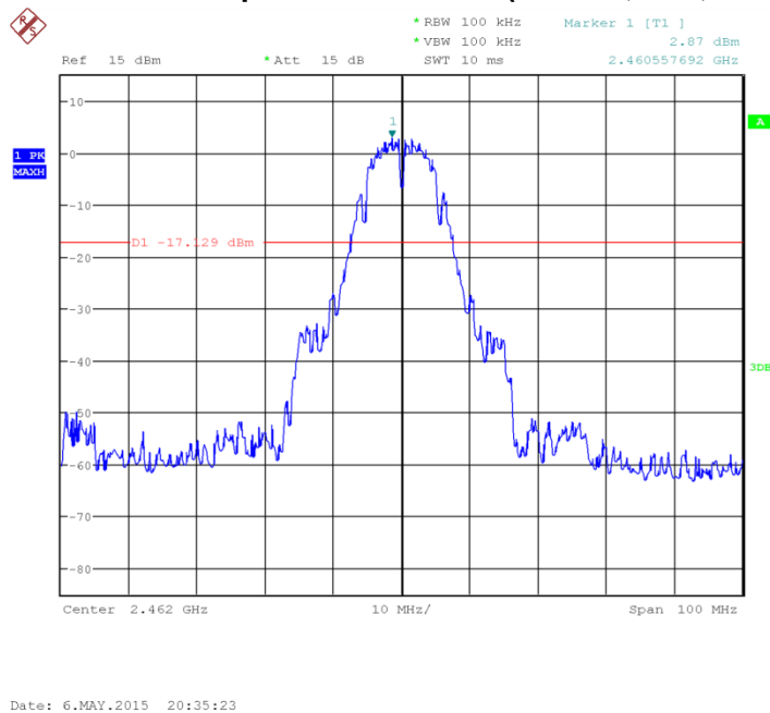
Fig.29 Conducted Spurious Emission (802.11b, Ch11)
