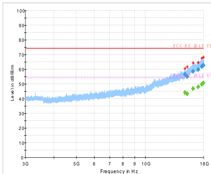
Fig.48 Radiated Spurious Emission (802.11b,Ch1,3GHz~18GHz)
