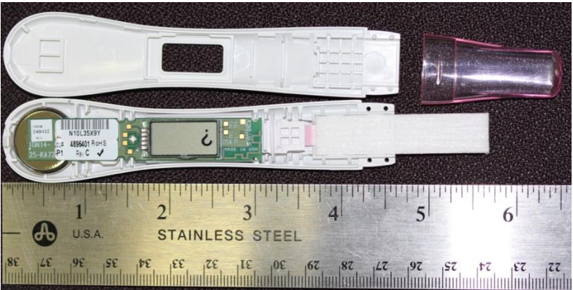
INTERNAL Assembled
