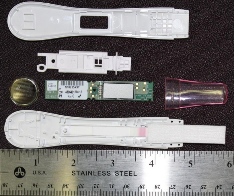
Disassembled
