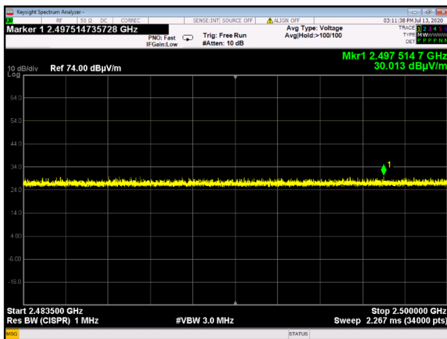
Plot 4.5.6: Spurious Emissions in Restricted Bands, Single mode, F_c = 2402\text{MHz} , Vertical Polarization 2483.5-2500MHz
