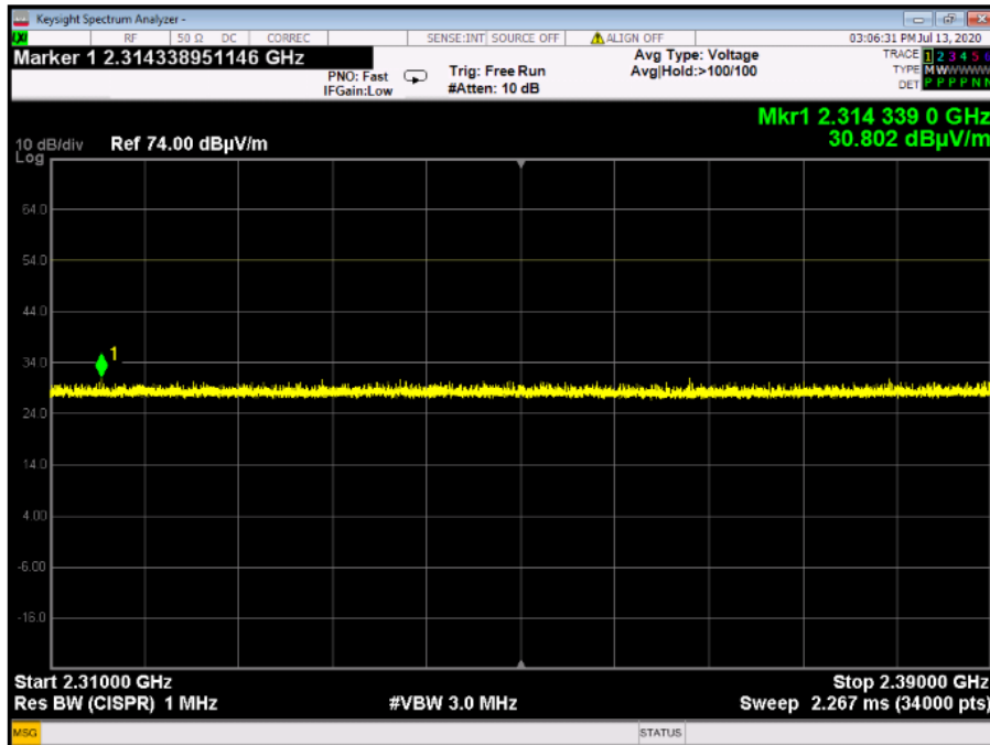
Plot 4.5.4: Spurious Emissions in Restricted Bands, Single mode, F_c = 2402\text{MHz} , Vertical Polarization 2310-2390MHz
