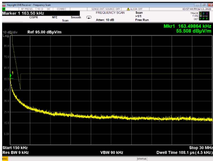
Plot 4.5.2: Spurious Emissions in Restricted Bands, Single mode, F_c = 2402\text{MHz} , Horizontal Polarization, 150K-30MHz
