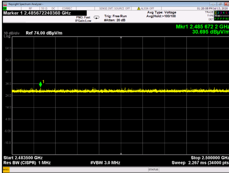
Plot 4.5.9: Spurious Emissions in Restricted Bands, Single mode, F_c = 2440\text{MHz} , Horizontal Polarization, 2483.5-2500MHz
