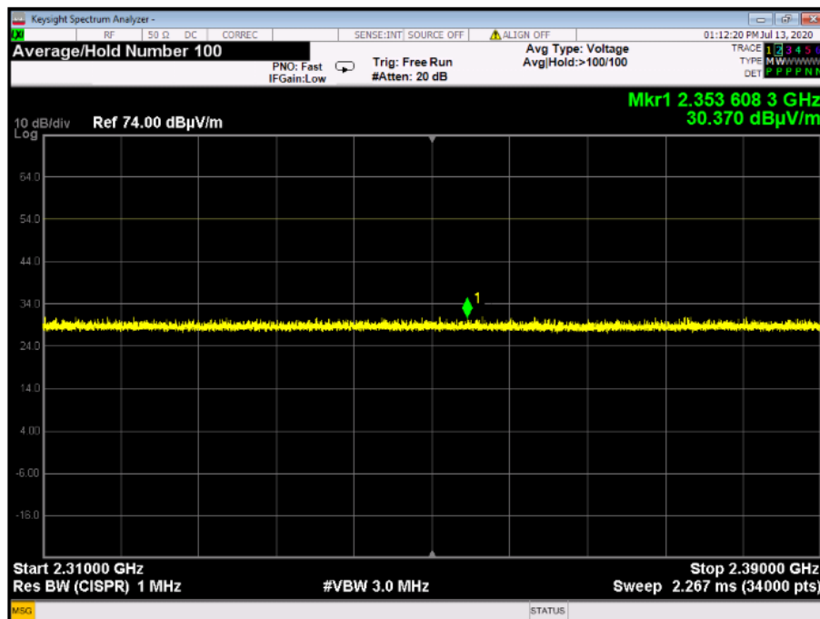
Plot 4.5.8: Spurious Emissions in Restricted Bands, Single mode, F_c = 2440\text{MHz} , Vertical Polarization 2310-2390MHz
