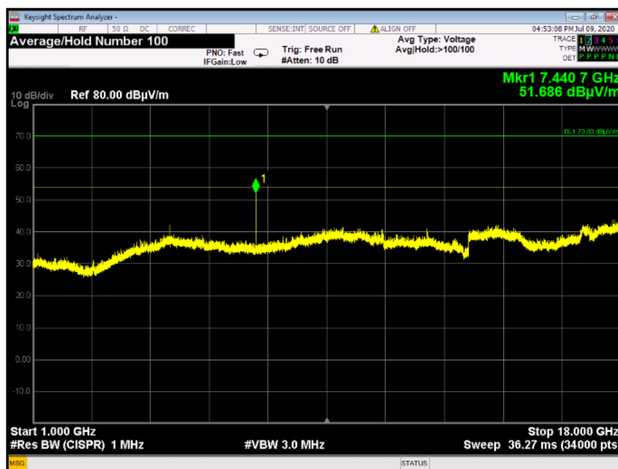
Plot 4.4.16: Radiated Spurious Emission in 1 – 18 GHz range, F_c = 2480 MHz, Horizontal Polarization Peak
