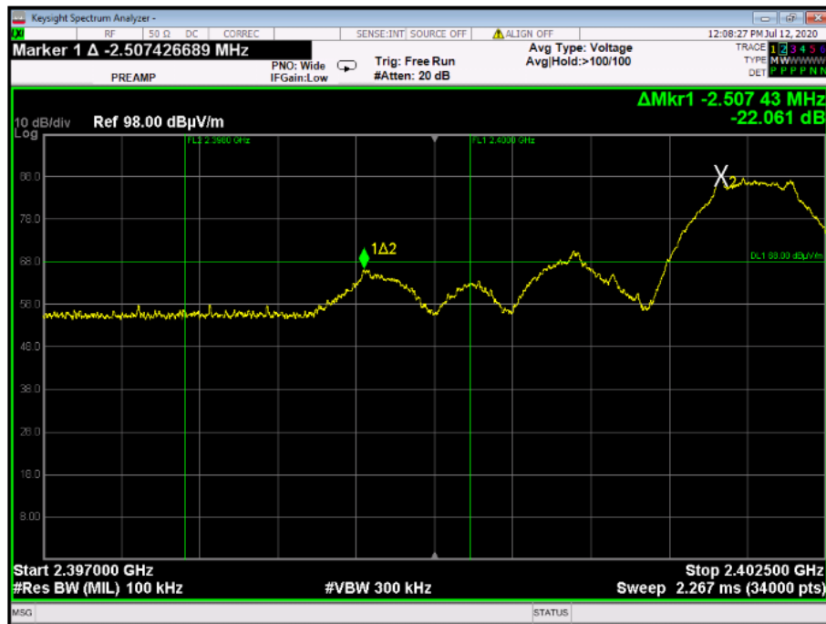
Plot 4.6.1: Band-edge test results, GFSK, channel 0, Horizontal Polarization
