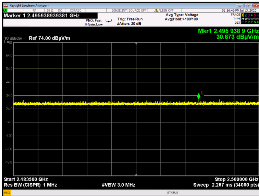
Plot 4.5.10: Spurious Emissions in Restricted Bands, Single mode, F_c = 2440\text{MHz} , Vertical Polarization 2483.5-2500MHz
