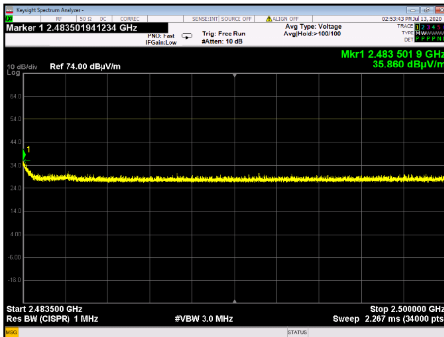
Plot 4.5.14: Spurious Emissions in Restricted Bands, Single mode, F_c = 2480\text{MHz} , Vertical Polarization 2483.5-2500MHz
