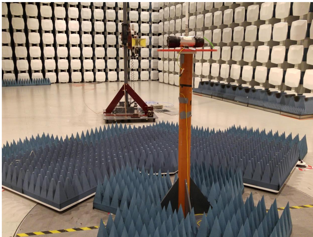
Radiated emissions, 1 – 8.5 GHz
