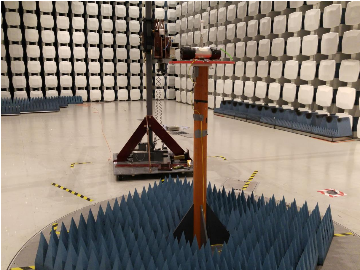
Radiated emissions, 12 – 18 GHz
