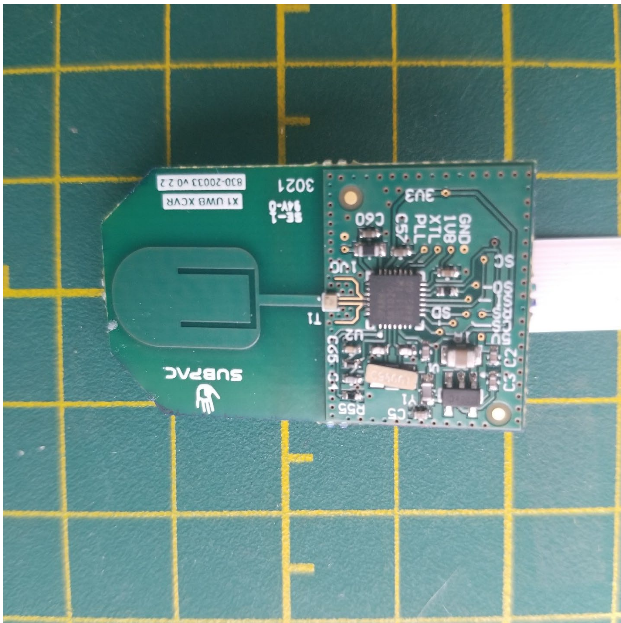
UWB Board
