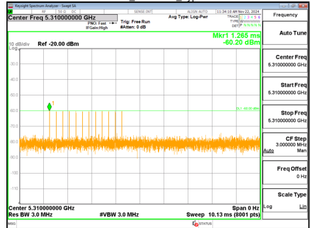
HE40_5310MHz_Type 5
