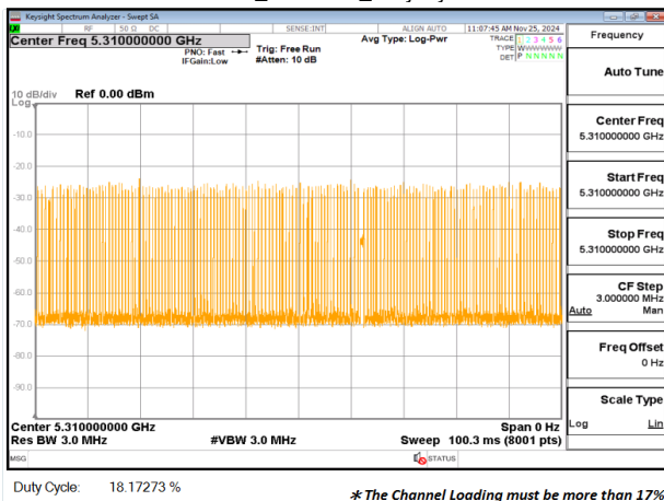
HE40_5310MHz_Duty Cycle
