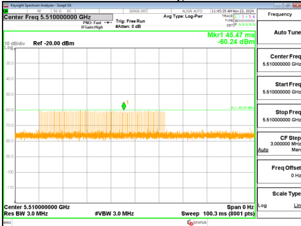
HE40_5510MHz_Type 1-B
