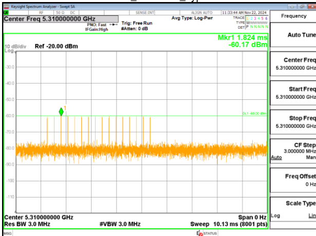
HE40_5310MHz_Type 3
