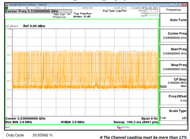
HE80_5530MHz_Duty Cycle
