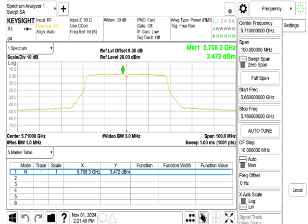
802.11n_40MHz_Chain0_5710MHz_UNII 3
