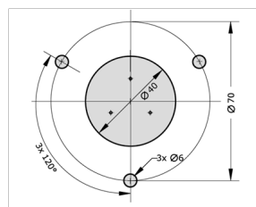
Drilling pattern
