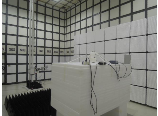
FCC_15_247_WLAN_Radiated_HUBER+SUHNER_Setup
