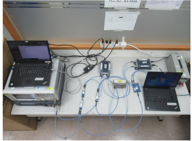
WLAN_Normal_DFS_Slave_Setup
