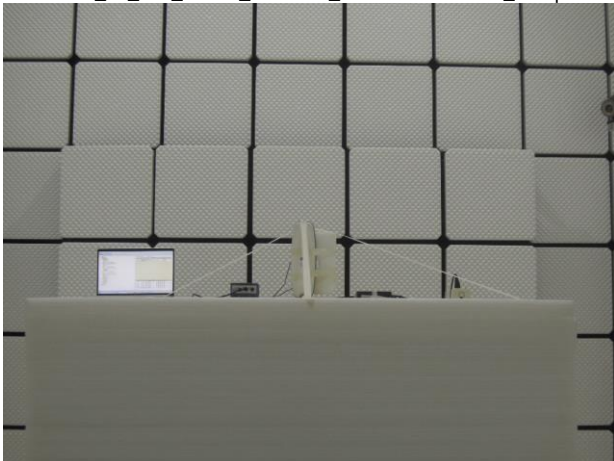
FCC_15_247_WLAN_Radiated_HUBER+SUHNER_Setup
