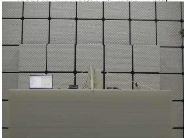
FCC_15_407_WLAN_Radiated_HUBER+SUHNER_Setup
