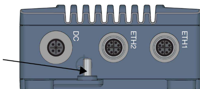
Figure 9 Earth connection
