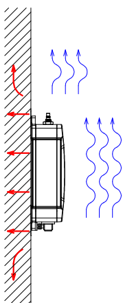
Figure 12 Improved heat transfer based on fixing plate
