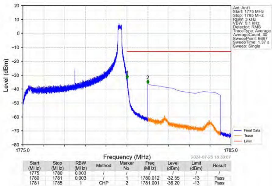
Band66 5MHz 16QAM HCH 1777.5MHz RB 1 24 NTNV
