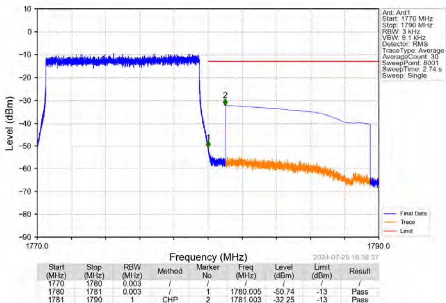
Band66 10MHz 16QAM HCH 1775MHz RB 1 49 NTNV
