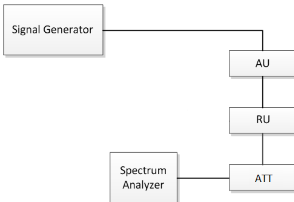
Fig.6 RF Output Power test configuration
