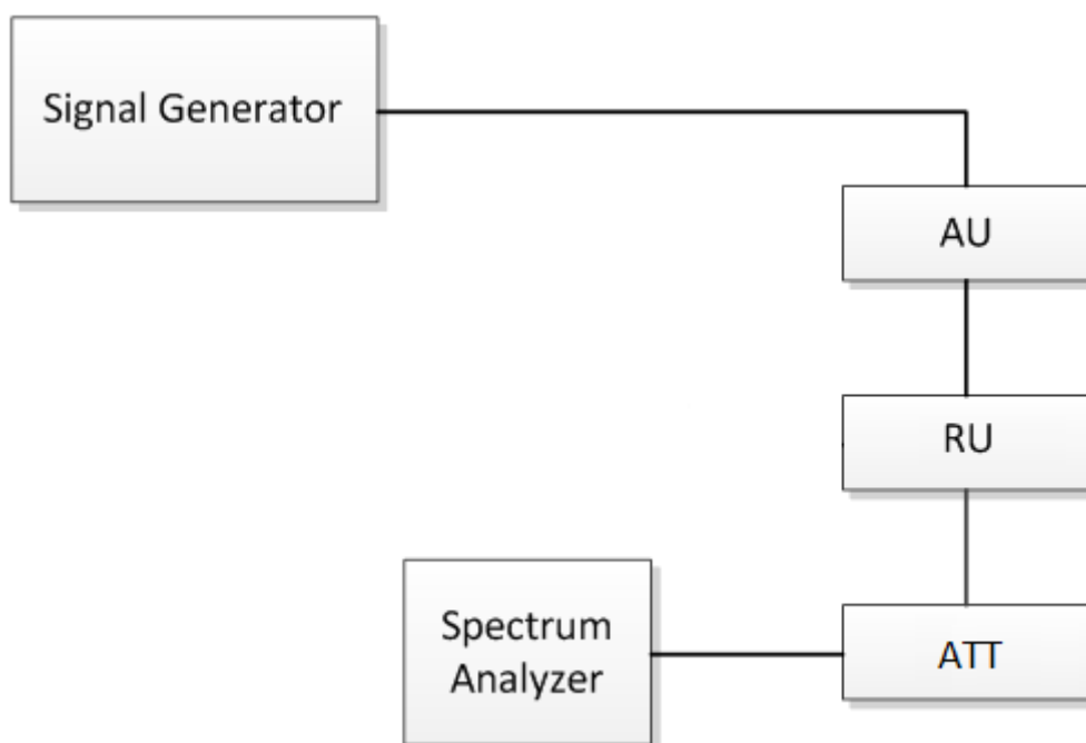
Fig.10. Out of Band rejection test configuration
