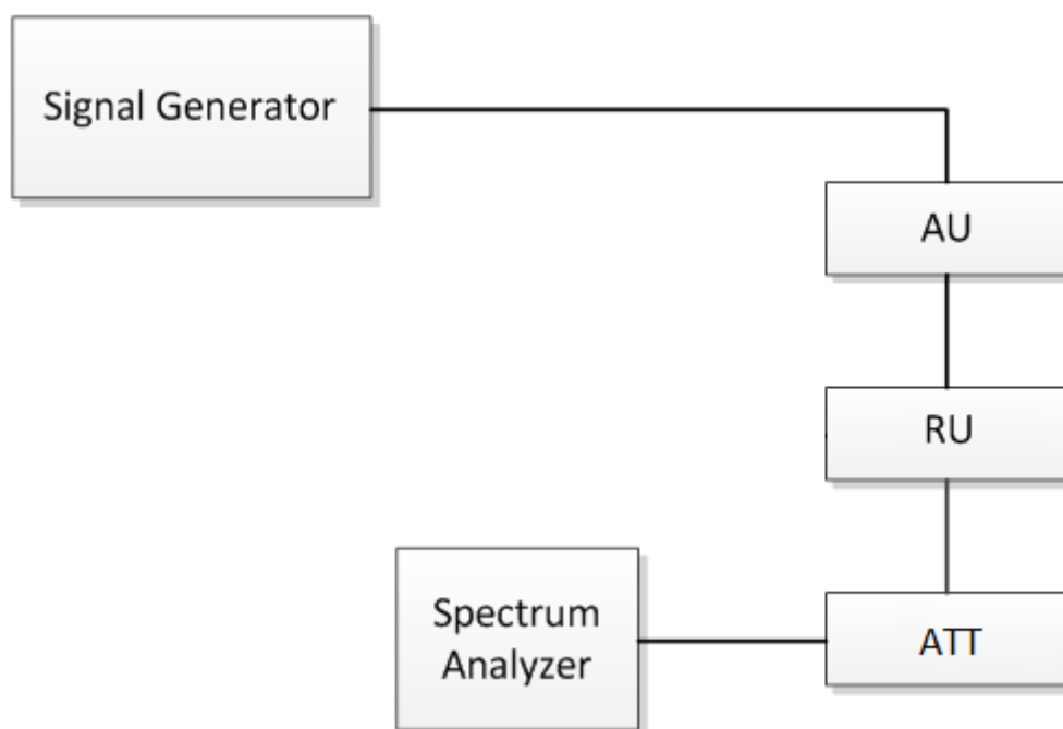
Fig.7. Conducted Spurious Emissions test configuration
