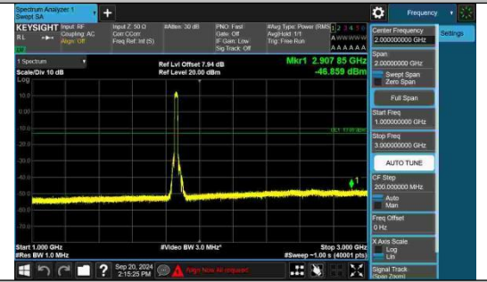
Band2-20MHz-QPSK-18700-100RB#0-1000~3000-PASS
