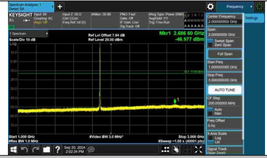
Band2-3MHz-QPSK-18900-1RB#14-1000~3000-PASS
