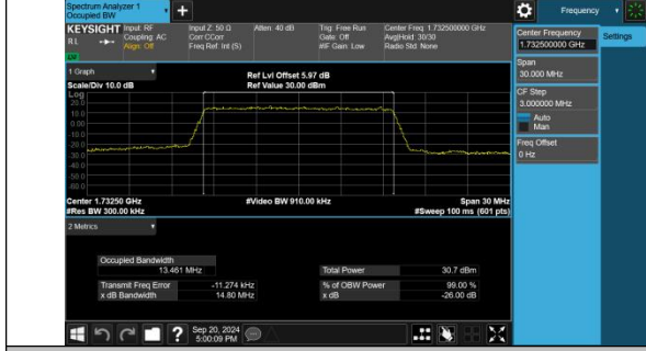
Band4-15MHz-QPSK-20175-75RB#0-PASS
