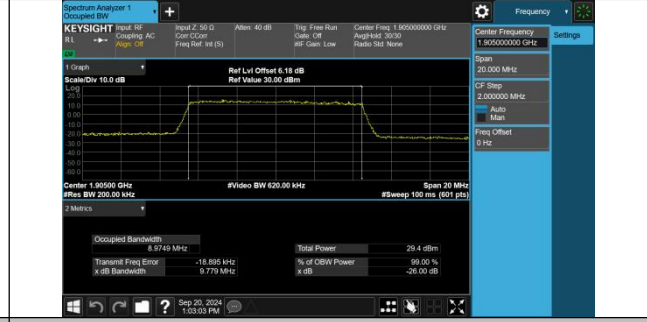
Band2-10MHz-16QAM-19150-50RB#0-PASS
