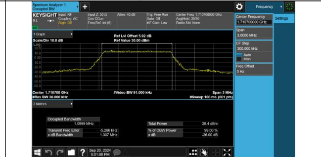
Band4-1.4MHz-16QAM-19957-6RB#0-PASS
