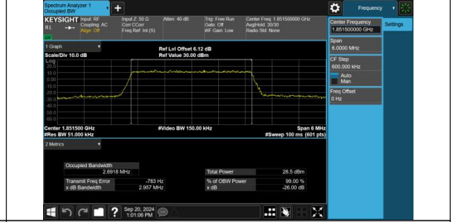
Band2-3MHz-16QAM-18615-15RB#0-PASS
