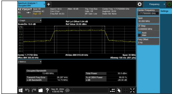
Band4-15MHz-QPSK-20025-75RB#0-PASS
