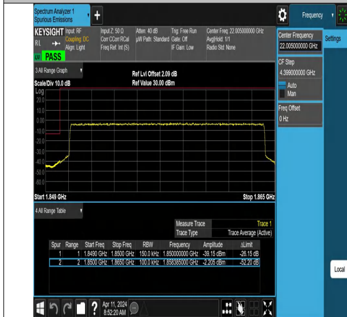
Band25_15MHz_QPSK_26115_75RB#0
