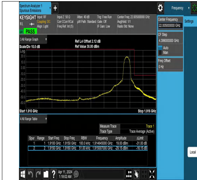
Band25_5MHz_QPSK_26665_1RB#24
