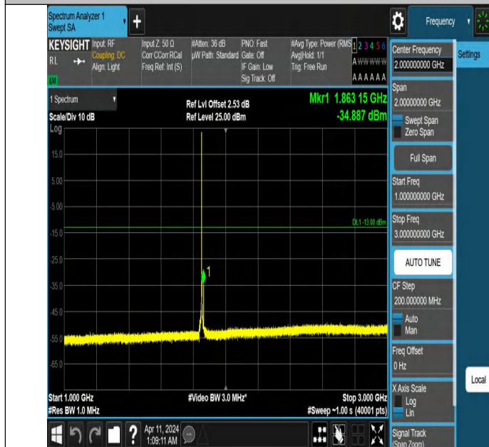
Band25_3MHz_QPSK_26055_1RB#0_1000~3000_1000~3000
