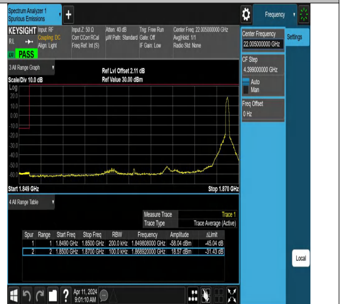
Band25_20MHz_QPSK_26140_1RB#99
