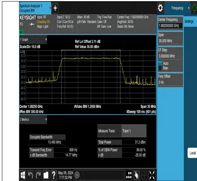
Band25-15MHz-QPSK-26365-75RB#0-PASS
