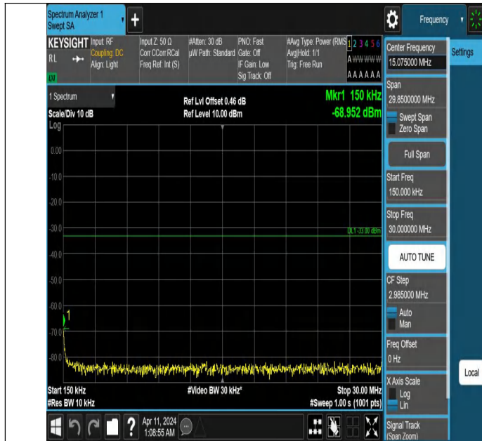
Band25_3MHz_QPSK_26055_1RB#0_0.15~30_0.15~30
