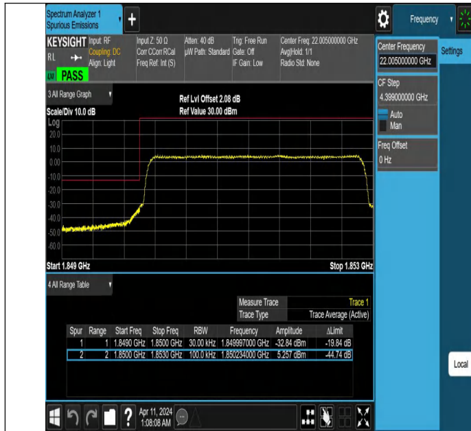
Band25_3MHz_QPSK_26055_15RB#0
