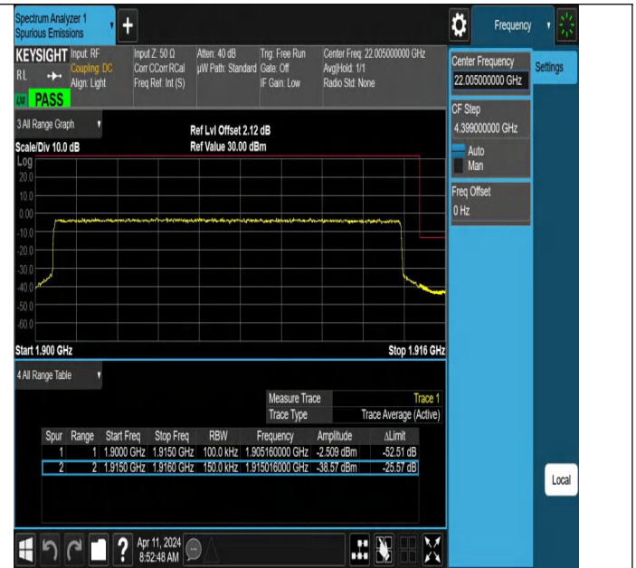
Band25_15MHz_QPSK_26615_75RB#0
