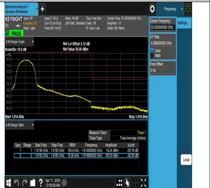
Band25_1.4MHz_QPSK_26683_1RB#0
