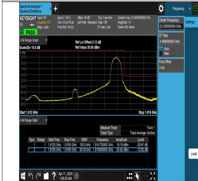
Band25_3MHz_QPSK_26675_1RB#14
