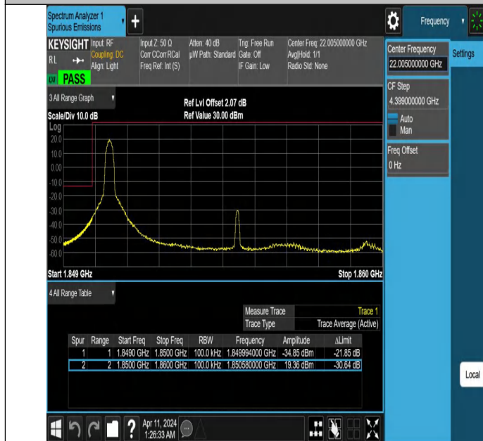
Band25_10MHz_QPSK_26090_1RB#0
