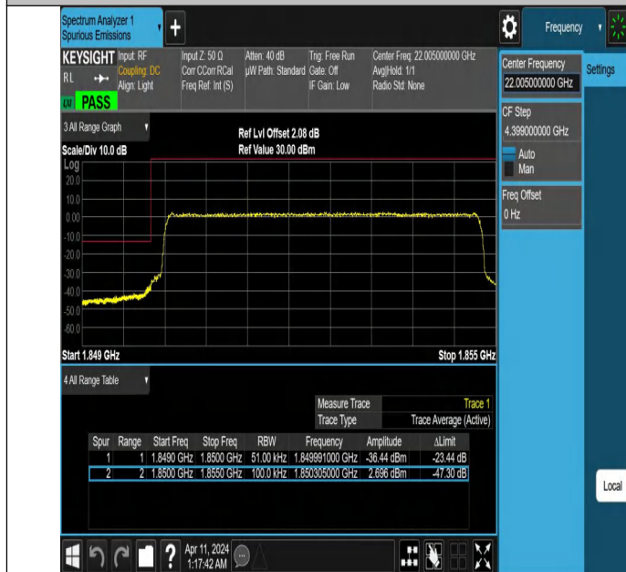
Band25_5MHz_QPSK_26065_25RB#0
