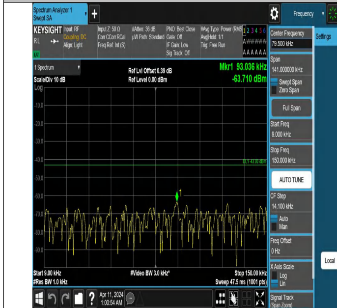
Band25_1.4MHz_QPSK_26683_1RB#0_0.009~0.15_0.009~0.15
