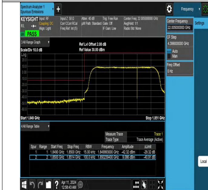
Band25_1.4MHz_QPSK_26047_6RB#0
