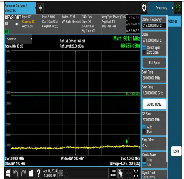
Band25_3MHz_QPSK_26055_1RB#0_30~1000_30~1000
