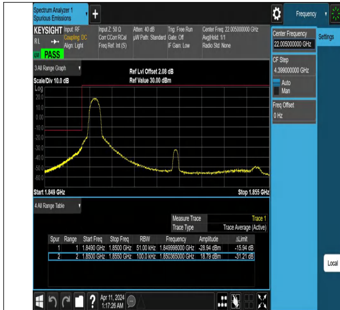
Band25_5MHz_QPSK_26065_1RB#0
