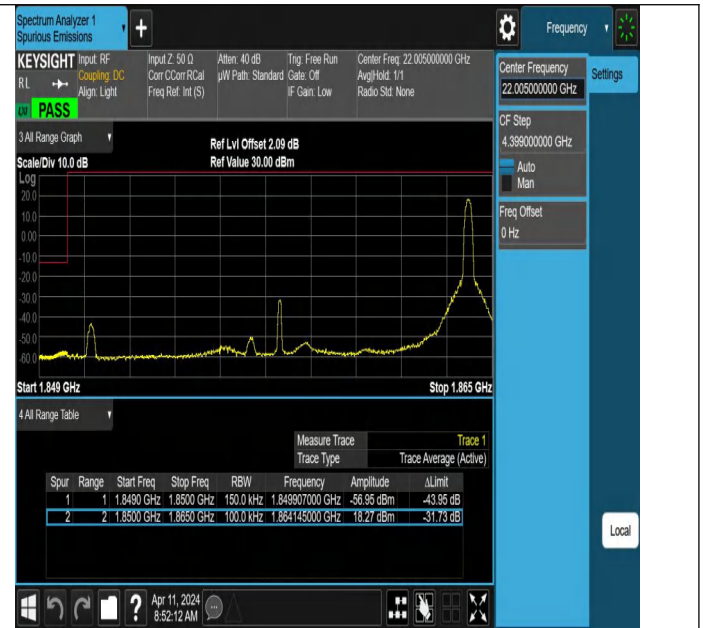
Band25_15MHz_QPSK_26115_1RB#74
