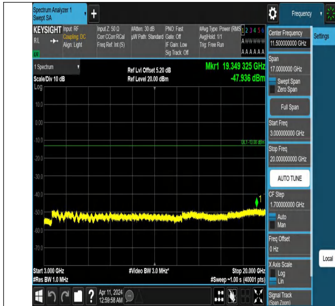
Band25_1.4MHz_QPSK_26047_1RB#0_3000~20000_3000~2000
