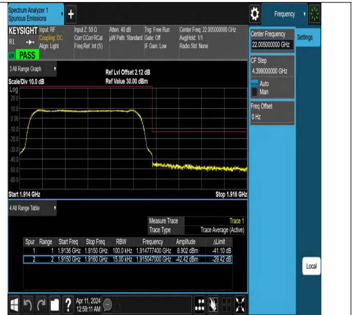
Band25_1.4MHz_QPSK_26683_6RB#0
