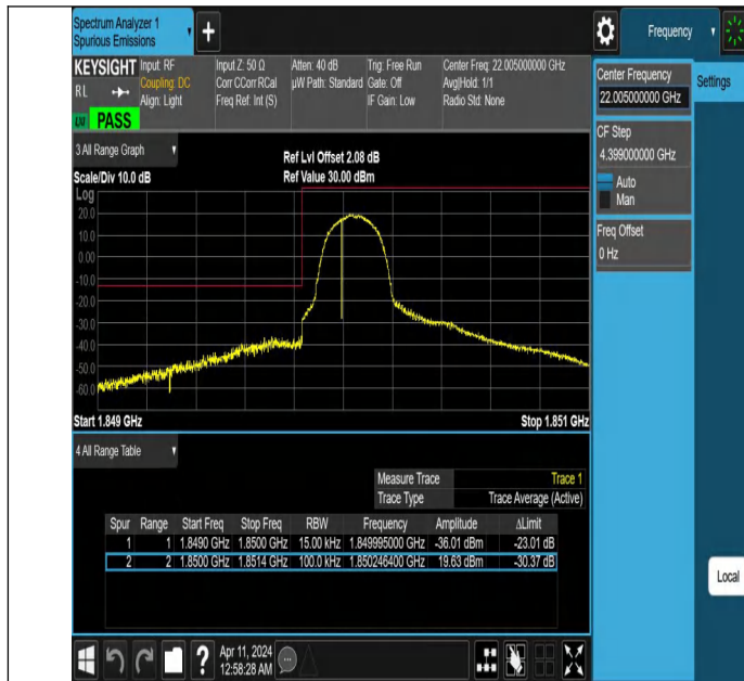
Band25_1.4MHz_QPSK_26047_1RB#0
