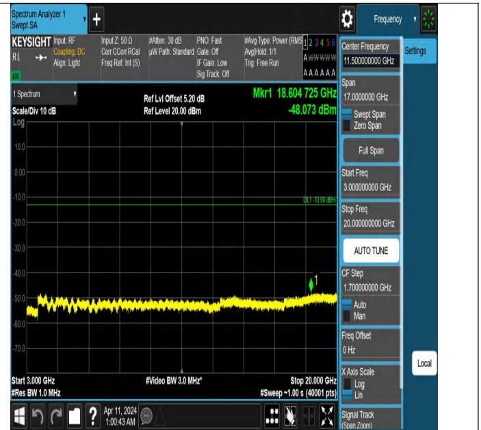
Band25_1.4MHz_QPSK_26365_1RB#0_3000~20000_3000~2000
