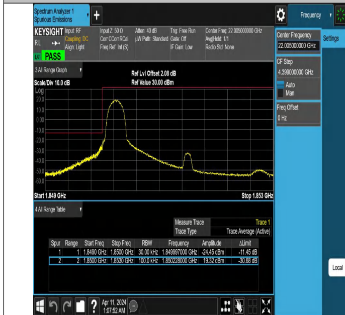
Band25_3MHz_QPSK_26055_1RB#0
