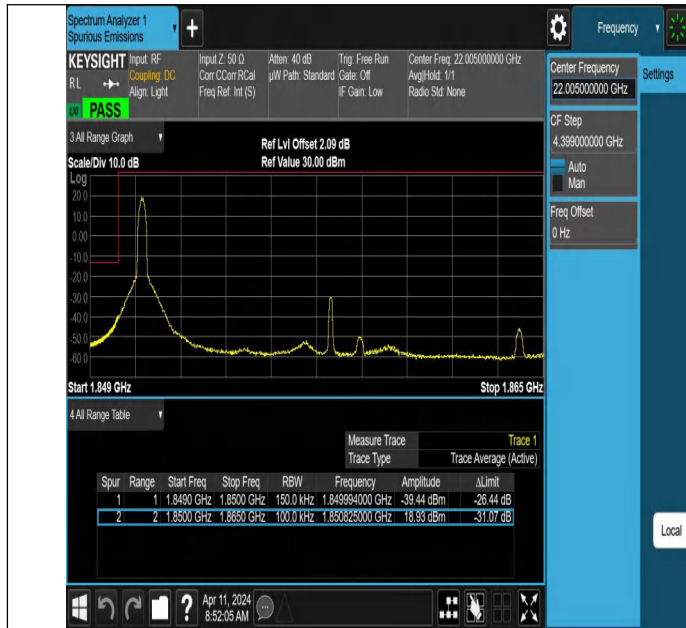
Band25_15MHz_QPSK_26115_1RB#0
