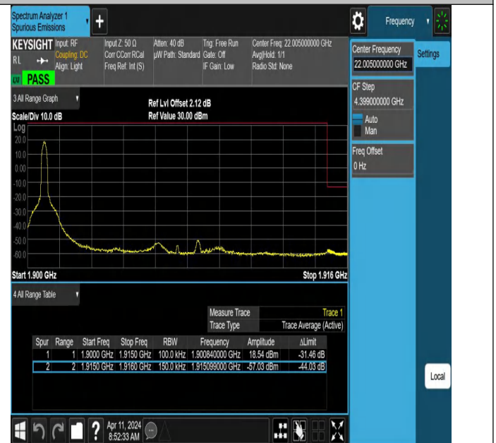
Band25_15MHz_QPSK_26615_1RB#0
