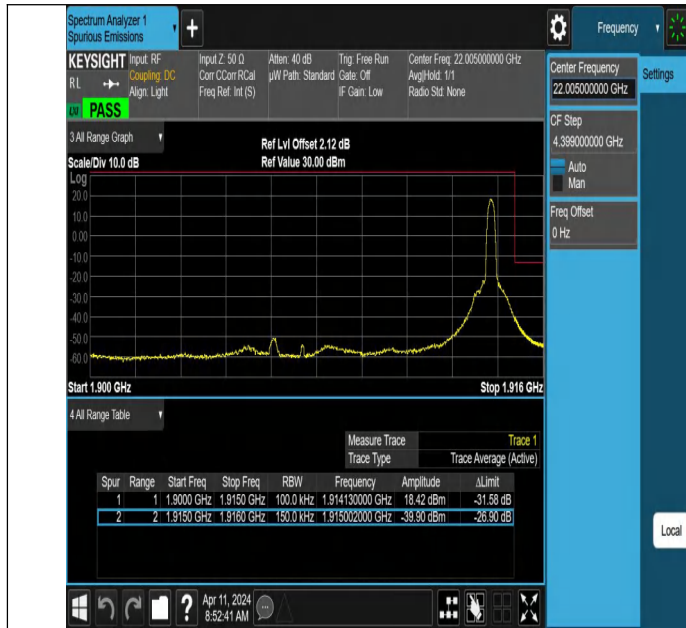
Band25_15MHz_QPSK_26615_1RB#74
