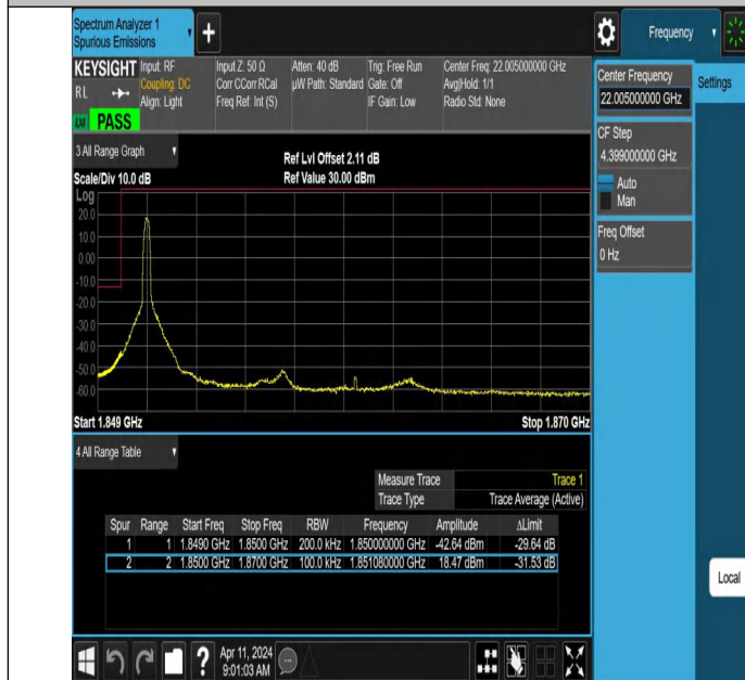
Band25_20MHz_QPSK_26140_1RB#0
