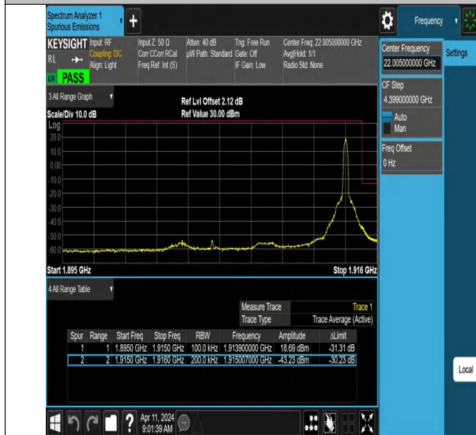
Band25_20MHz_QPSK_26590_1RB#99
