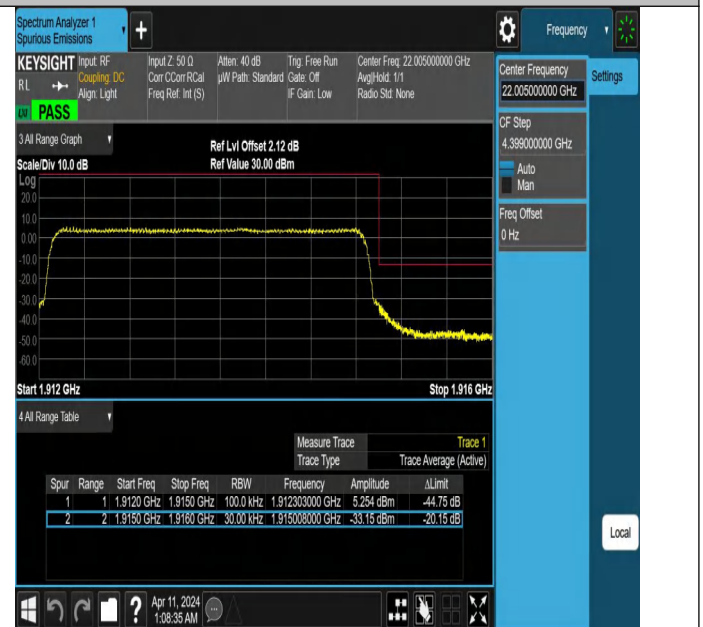
Band25_3MHz_QPSK_26675_15RB#0
