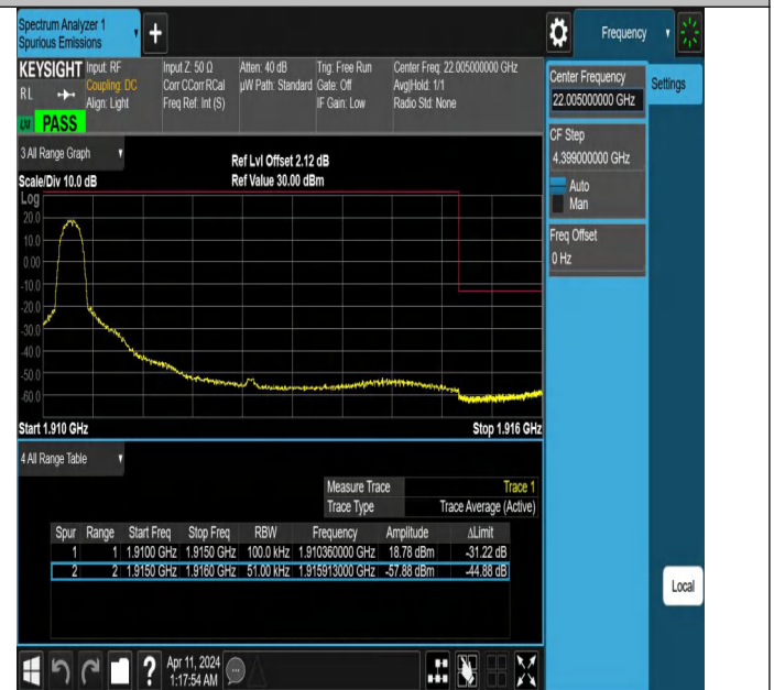
Band25_5MHz_QPSK_26665_1RB#0
