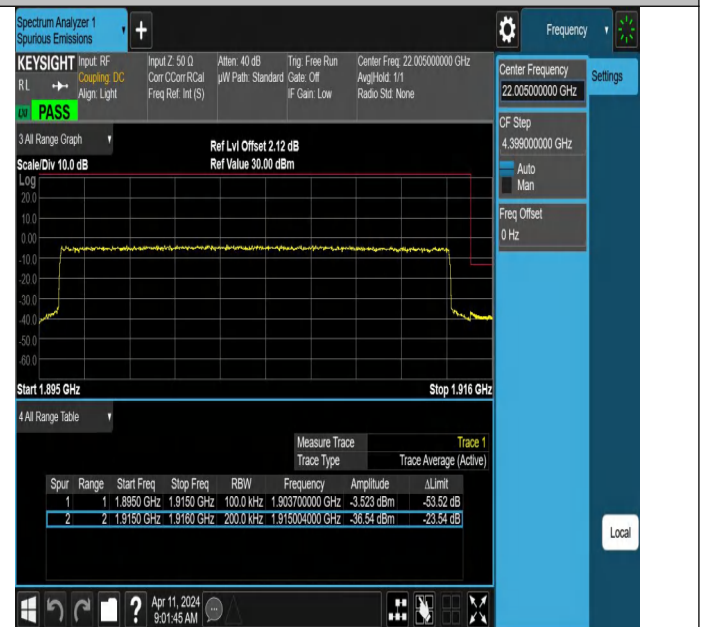
Band25_20MHz_QPSK_26590_100RB#0
