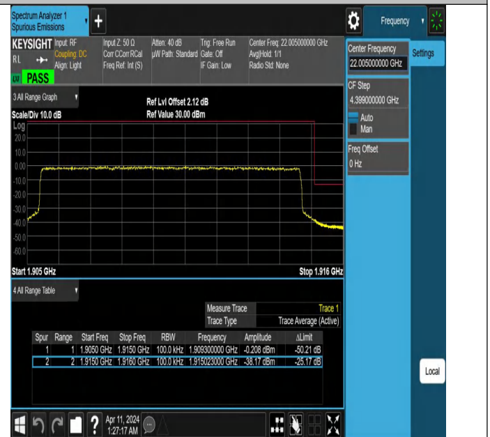
Band25_10MHz_QPSK_26640_50RB#0
