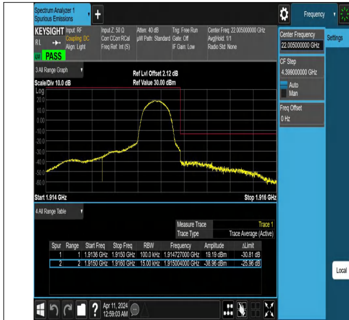
Band25_1.4MHz_QPSK_26683_1RB#5
