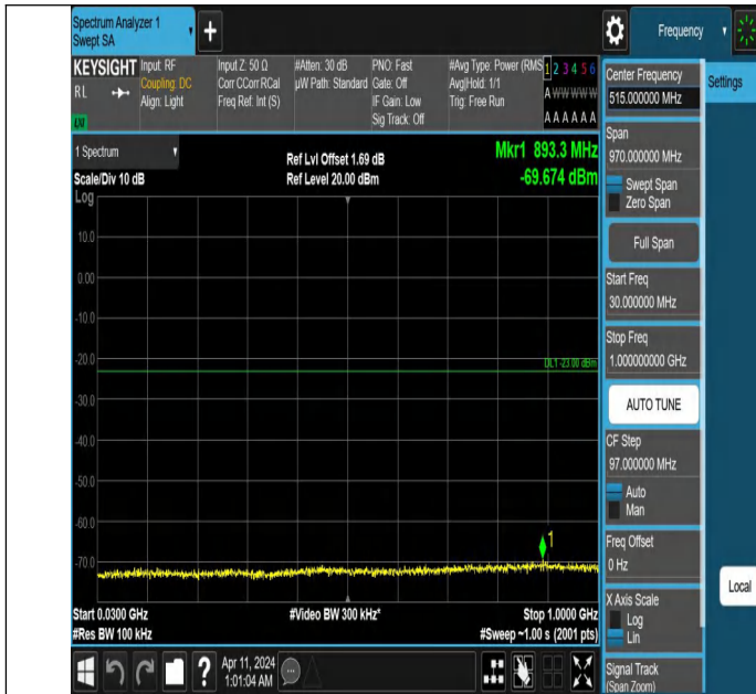
Band25_1.4MHz_QPSK_26683_1RB#0_30~1000_30~1000
