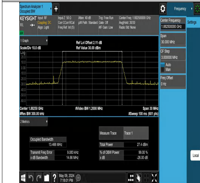
Band25-15MHz-256QAM-26365-75RB#0-PASS
