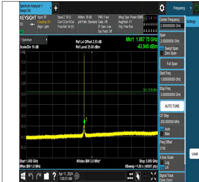
Band25_1.4MHz_QPSK_26365_1RB#0_1000~3000_1000~3000
