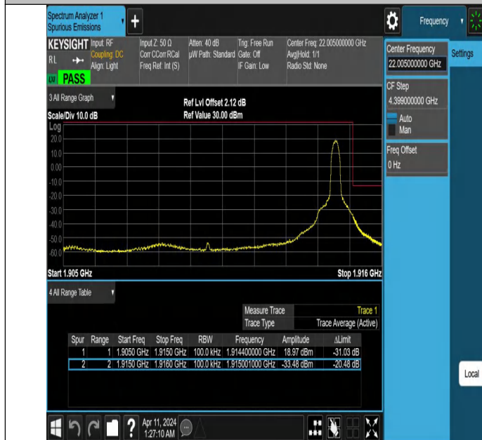
Band25_10MHz_QPSK_26640_1RB#49
