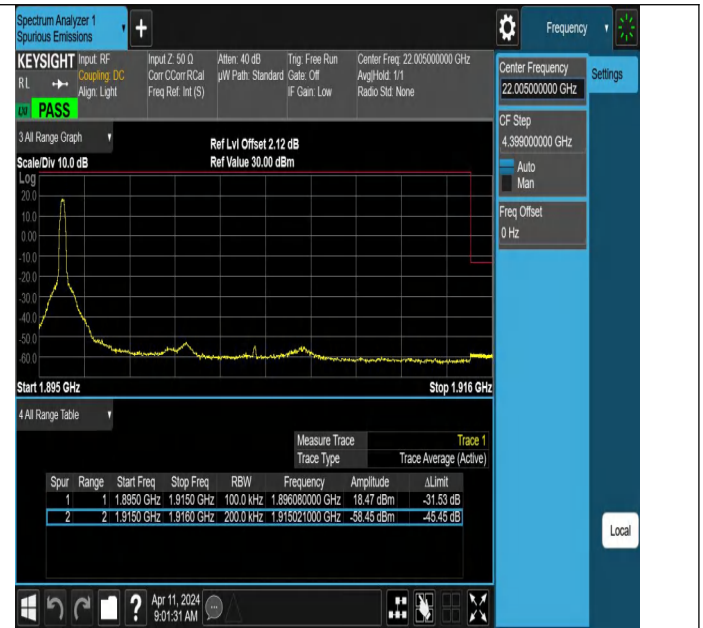
Band25_20MHz_QPSK_26590_1RB#0
