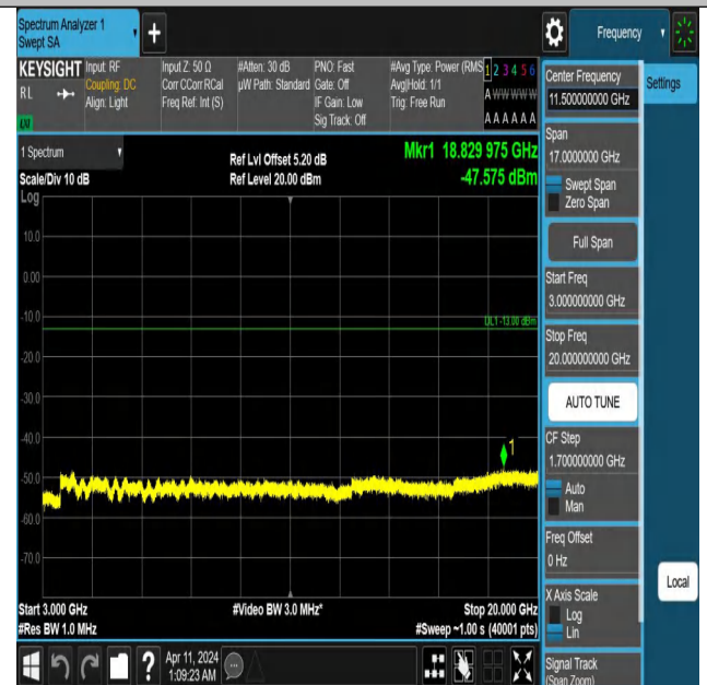
Band25_3MHz_QPSK_26055_1RB#0_3000~20000_3000~20000
