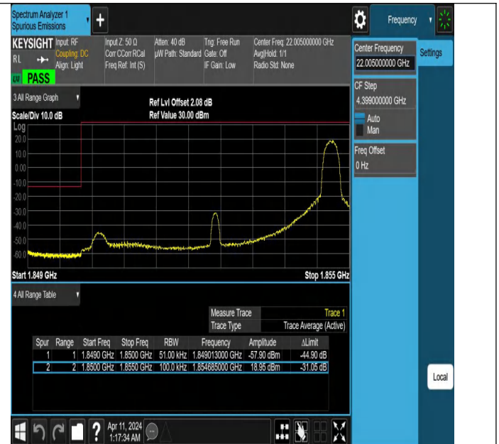
Band25_5MHz_QPSK_26065_1RB#24
