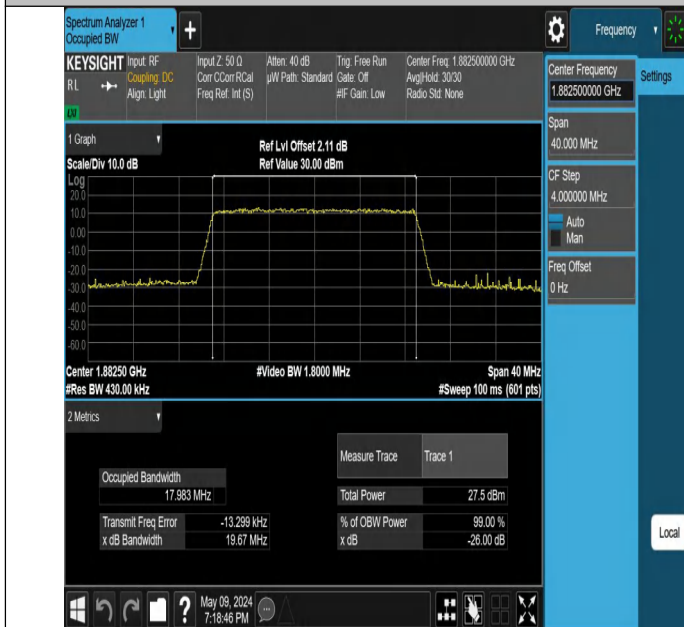
Band25-20MHz-256QAM-26365-100RB#0-PASS
