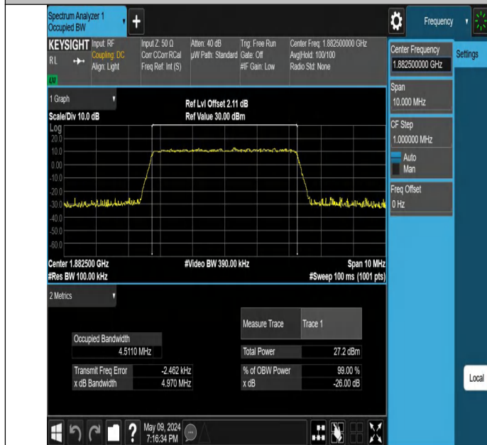
Band25-5MHz-256QAM-26365-25RB#0-PASS
