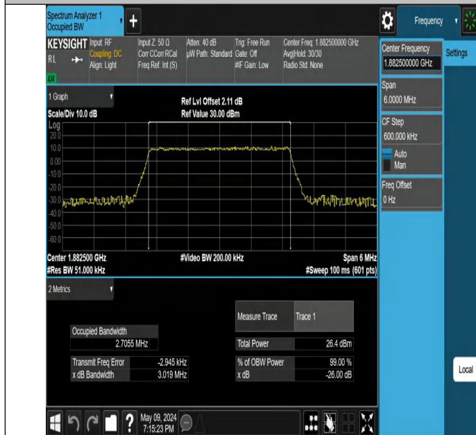
Band25-3MHz-256QAM-26365-15RB#0-PASS
