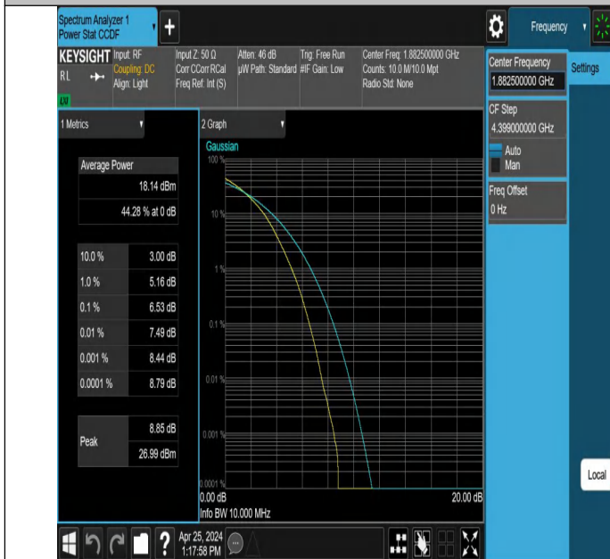
Band25-10MHz-256QAM-26365-50RB#0-PASS
