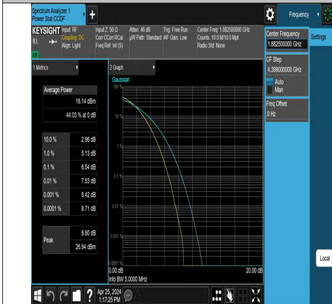
Band25-5MHz-256QAM-26365-25RB#0-PASS
