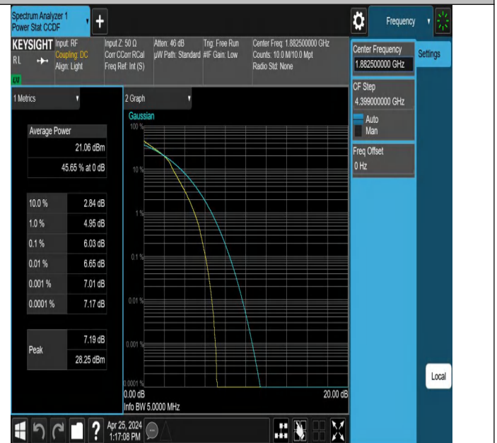
Band25-5MHz-16QAM-26365-25RB#0-PASS
