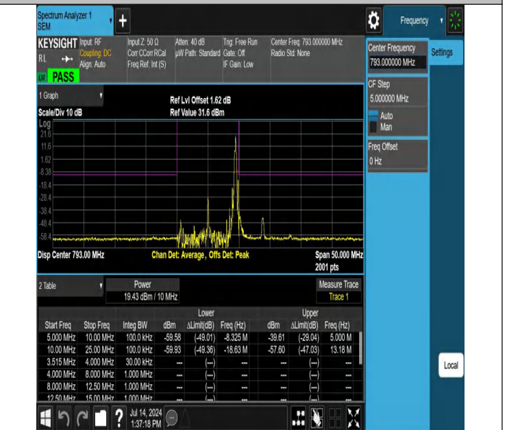
NTNV-Band14-10MHz-256QAM-23330-1RB#49-10.00-25.00-PAS
