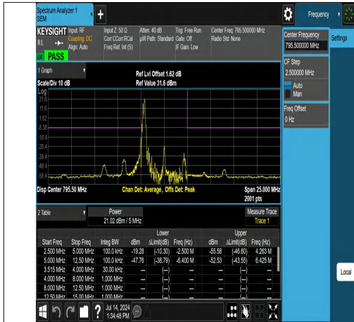
NTNV-Band14-5MHz-64QAM-23355-1RB#0--5.00--2.50-PASS
