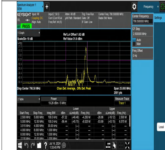
NTNV-Band14-5MHz-256QAM-23305-1RB#24--12.50--5.00-PASS
