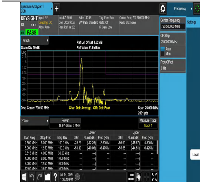
NTNV-Band14-5MHz-256QAM-23305-1RB#0--12.50--5.00-PASS
