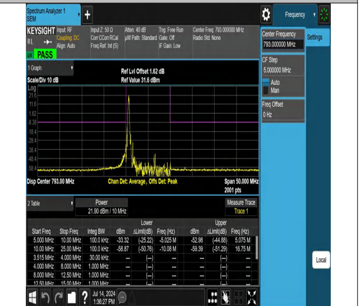
NTNV-Band14-10MHz-16QAM-23330-1RB#0-10.00-25.00-PASS
