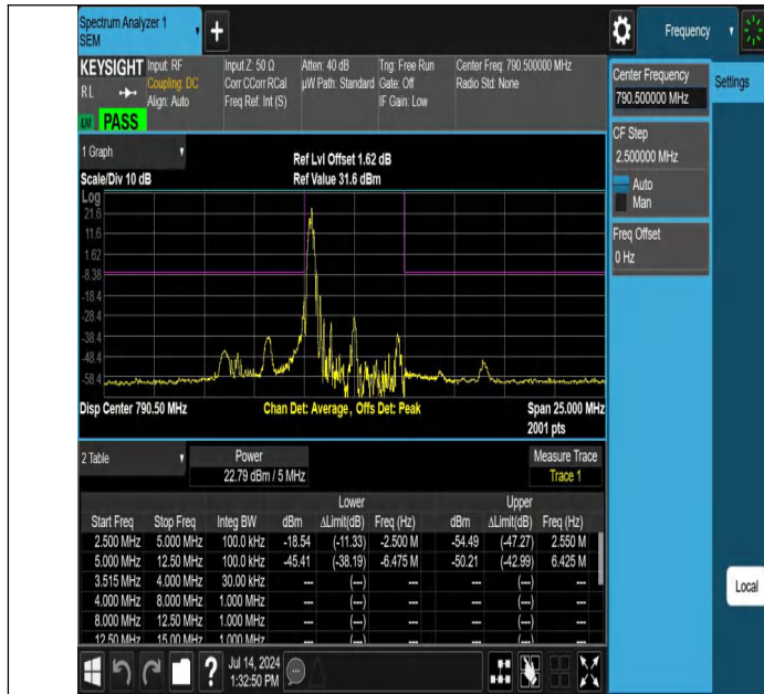
NTNV-Band14-5MHz-16QAM-23305-1RB#0--5.00--2.50-PASS
