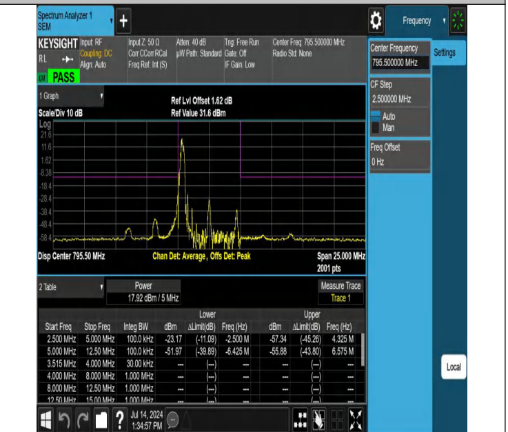
NTNV-Band14-5MHz-256QAM-23355-1RB#0-5.00-12.50-PASS
