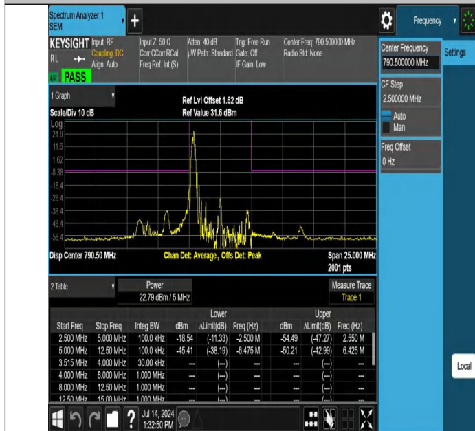
NTNV-Band14-5MHz-16QAM-23305-1RB#0--12.50--5.00-PASS
