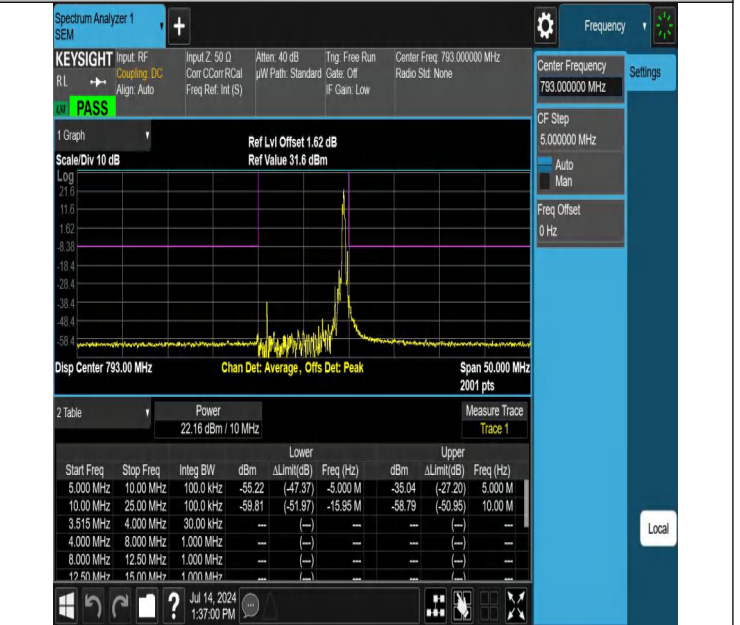
NTNV-Band14-10MHz-16QAM-23330-1RB#49-5.00-10.00-PASS
