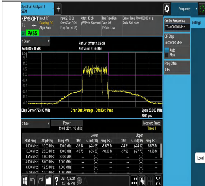
NTNV-Band14-10MHz-64QAM-23330-50RB#0--25.00--10.00-PASS
