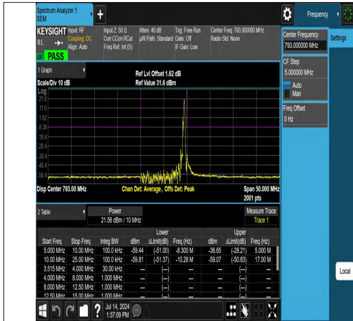
NTNV-Band14-10MHz-64QAM-23330-1RB#49--10.00--5.00-PASS
