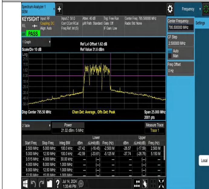
NTNV-Band14-5MHz-16QAM-23355-25RB#0--12.50--5.00-PASS
