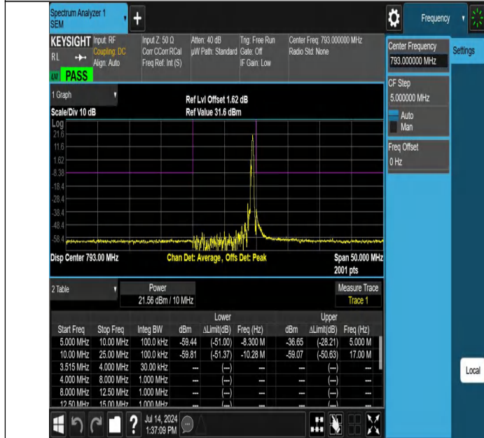
NTNV-Band14-10MHz-64QAM-23330-1RB#49--25.00--10.00-PASS
