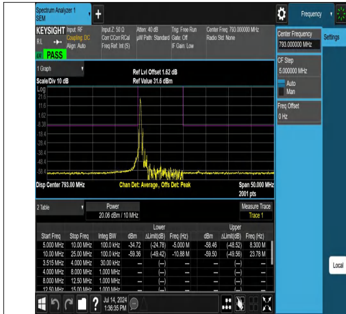
NTNV-Band14-10MHz-64QAM-23330-1RB#0--10.00--5.00-PASS
