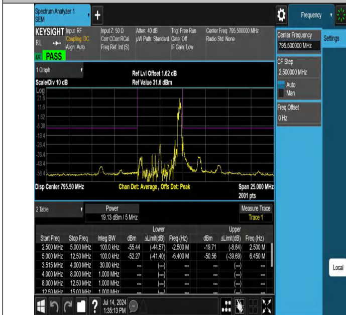
NTNV-Band14-5MHz-16QAM-23355-1RB#24--12.50--5.00-PASS
