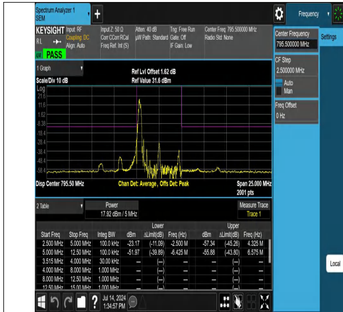
NTNV-Band14-5MHz-256QAM-23355-1RB#0--5.00--2.50-PASS
