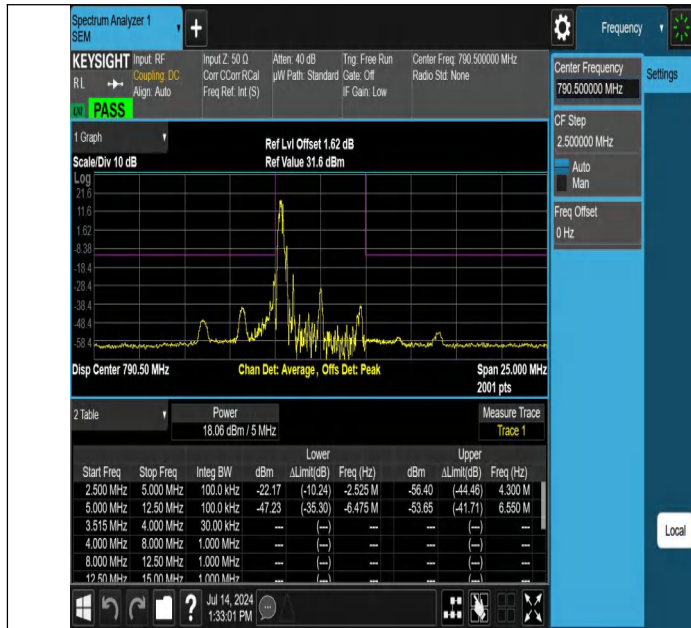
NTNV-Band14-5MHz-64QAM-23305-1RB#0--5.00--2.50-PASS
