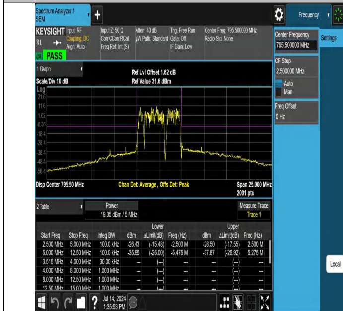
NTNV-Band14-5MHz-64QAM-23355-25RB#0--12.50--5.00-PASS
