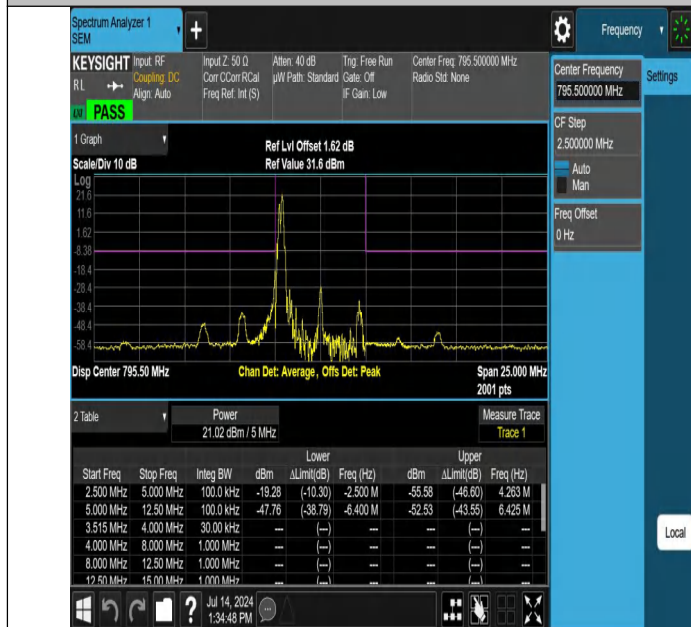
NTNV-Band14-5MHz-64QAM-23355-1RB#0--12.50--5.00-PASS
