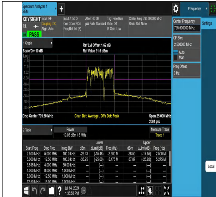
NTNV-Band14-5MHz-64QAM-23355-25RB#0--5.00--2.50-PASS
