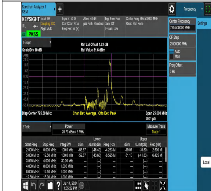
NTNV-Band14-5MHz-64QAM-23355-1RB#24--12.50--5.00-PASS
