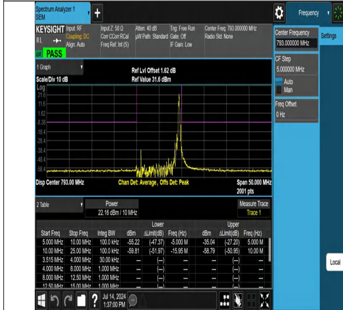
NTNV-Band14-10MHz-16QAM-23330-1RB#49--25.00--10.00-PASS
