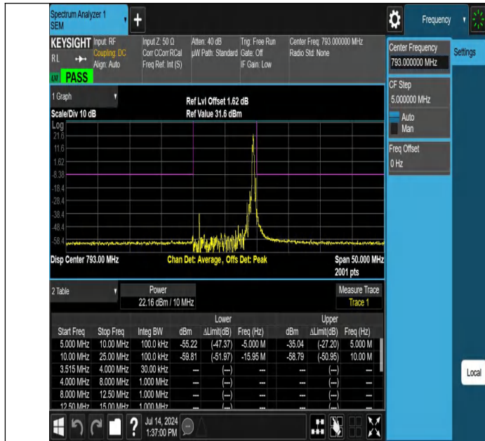
NTNV-Band14-10MHz-16QAM-23330-1RB#49--10.00--5.00-PASS
