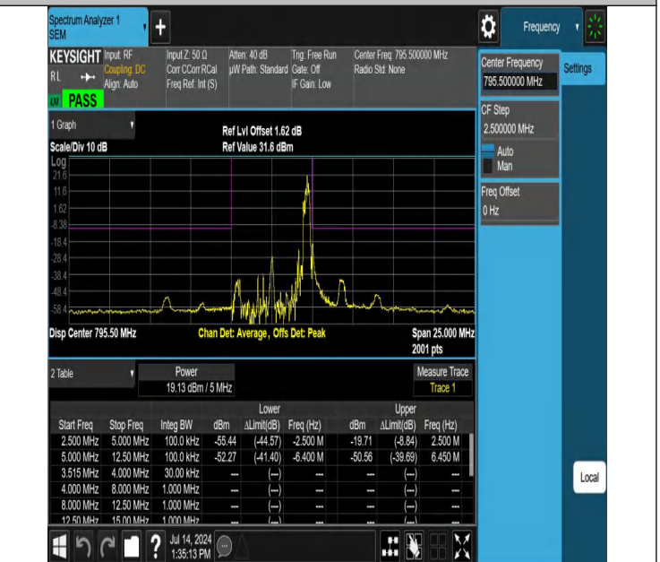
NTNV-Band14-5MHz-16QAM-23355-1RB#24-5.00-12.50-PASS
