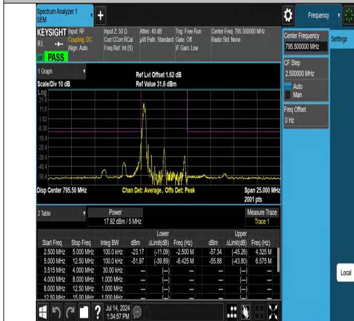
NTNV-Band14-5MHz-256QAM-23355-1RB#0--12.50--5.00-PASS
