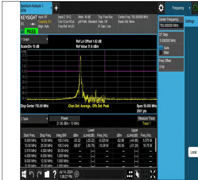
NTNV-Band14-10MHz-16QAM-23330-1RB#0--10.00--5.00-PASS
