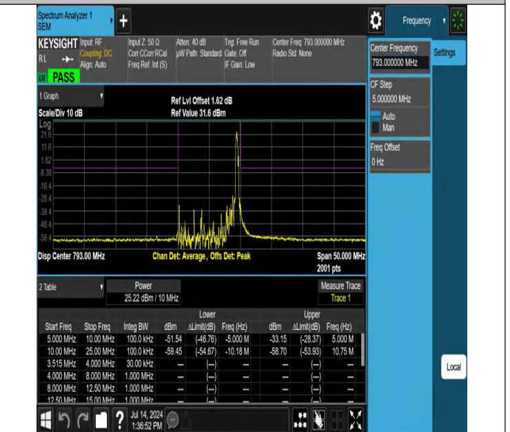
NTNV-Band14-10MHz-QPSK-23330-1RB#49-10.00-25.00-PASS
