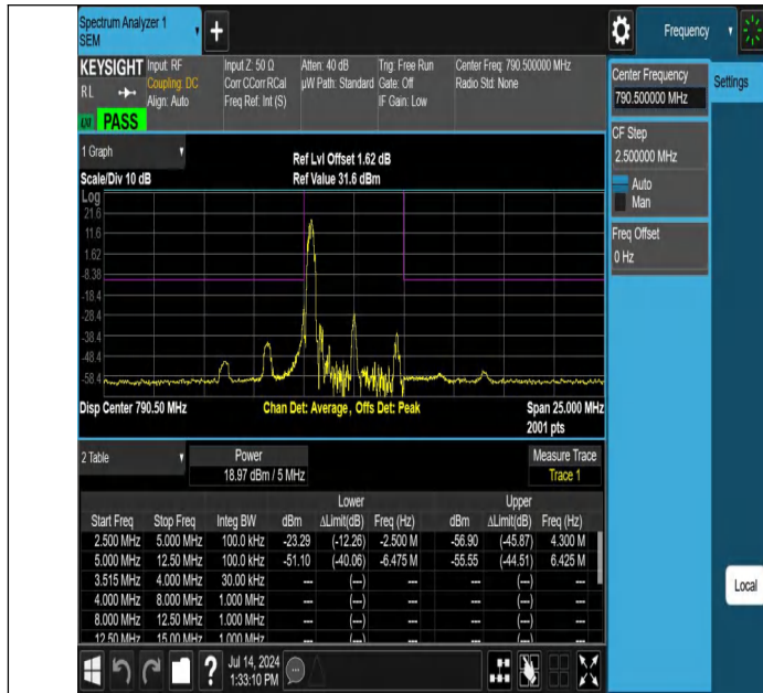
NTNV-Band14-5MHz-256QAM-23305-1RB#0--5.00--2.50-PASS
