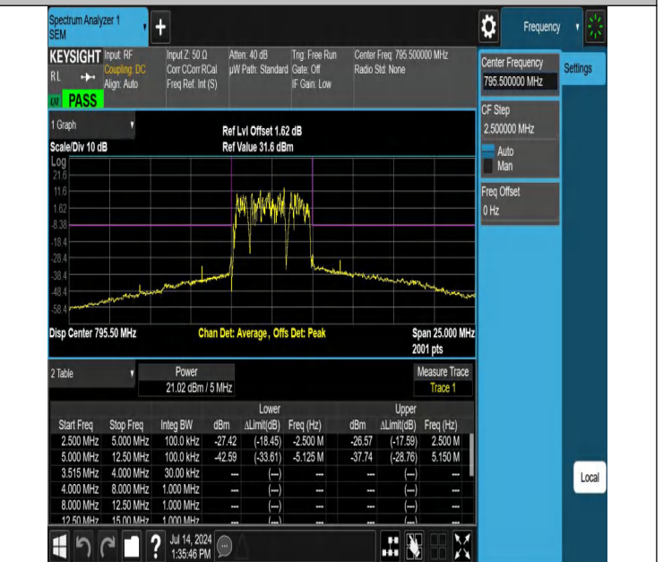
NTNV-Band14-5MHz-16QAM-23355-25RB#0-5.00-12.50-PASS
