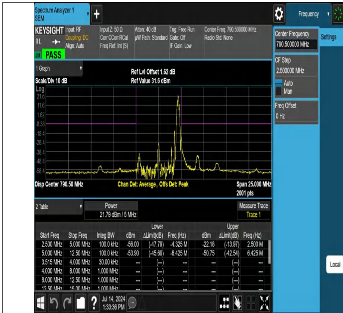
NTNV-Band14-5MHz-64QAM-23305-1RB#24--5.00--2.50-PASS
