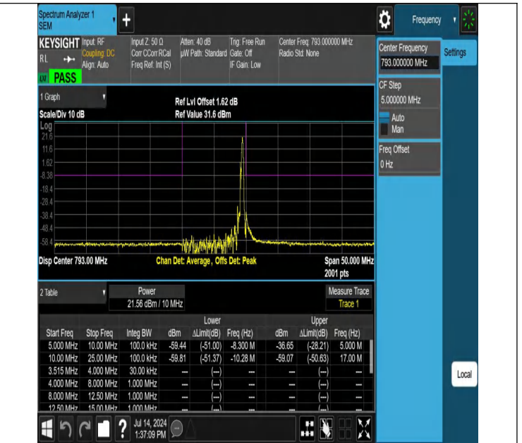
NTNV-Band14-10MHz-64QAM-23330-1RB#49--5.00-5.00-PASS
