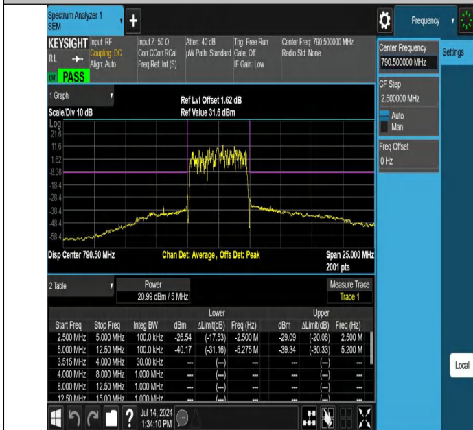
NTNV-Band14-5MHz-64QAM-23305-25RB#0--12.50--5.00-PASS
