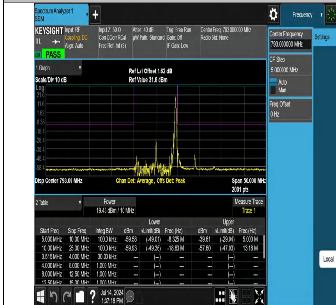
NTNV-Band14-10MHz-256QAM-23330-1RB#49--25.00--10.00-PAS
