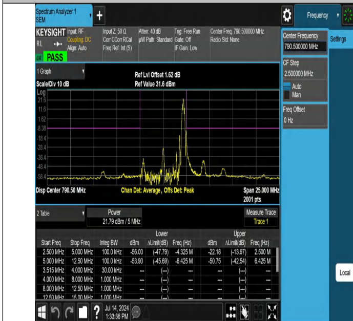
NTNV-Band14-5MHz-64QAM-23305-1RB#24--12.50--5.00-PASS
