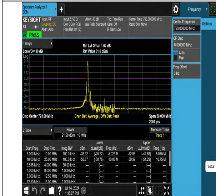
NTNV-Band14-10MHz-16QAM-23330-1RB#0--25.00--10.00-PASS
