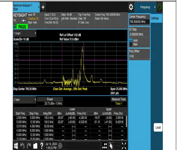
NTNV-Band14-5MHz-64QAM-23355-1RB#24-5.00-12.50-PASS
