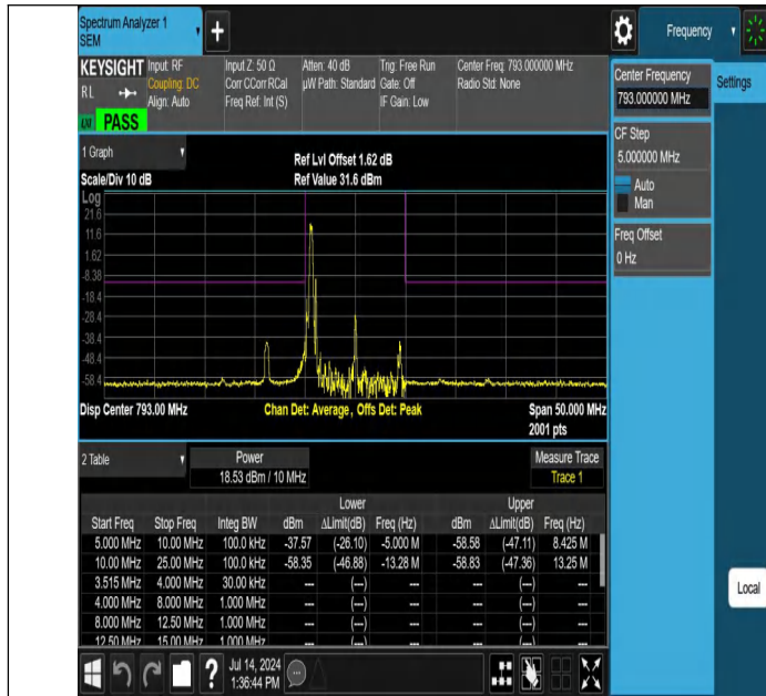
NTNV-Band14-10MHz-256QAM-23330-1RB#0--10.00--5.00-PASS
