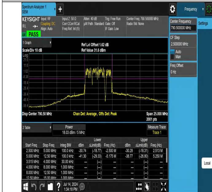
NTNV-Band14-5MHz-256QAM-23305-25RB#0--12.50--5.00-PASS
