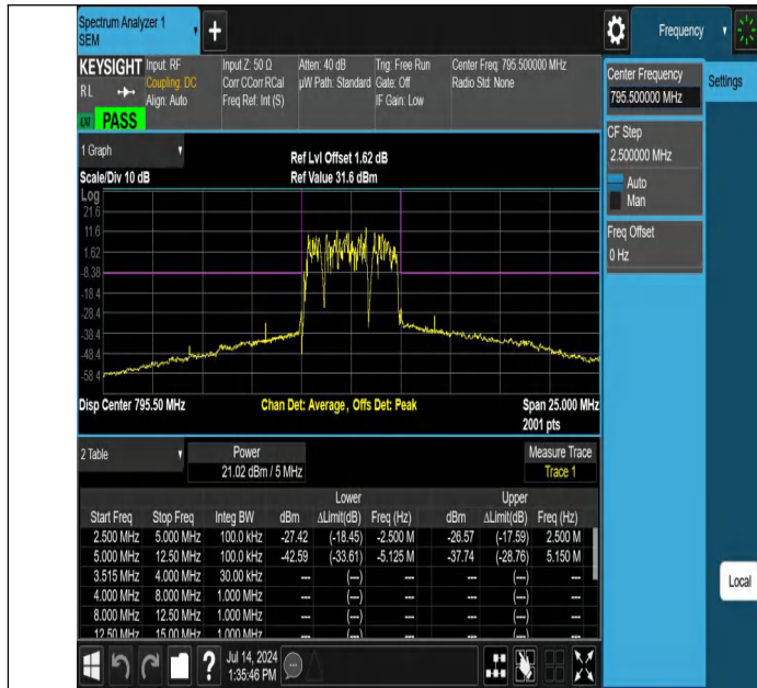
NTNV-Band14-5MHz-16QAM-23355-25RB#0--5.00--2.50-PASS
