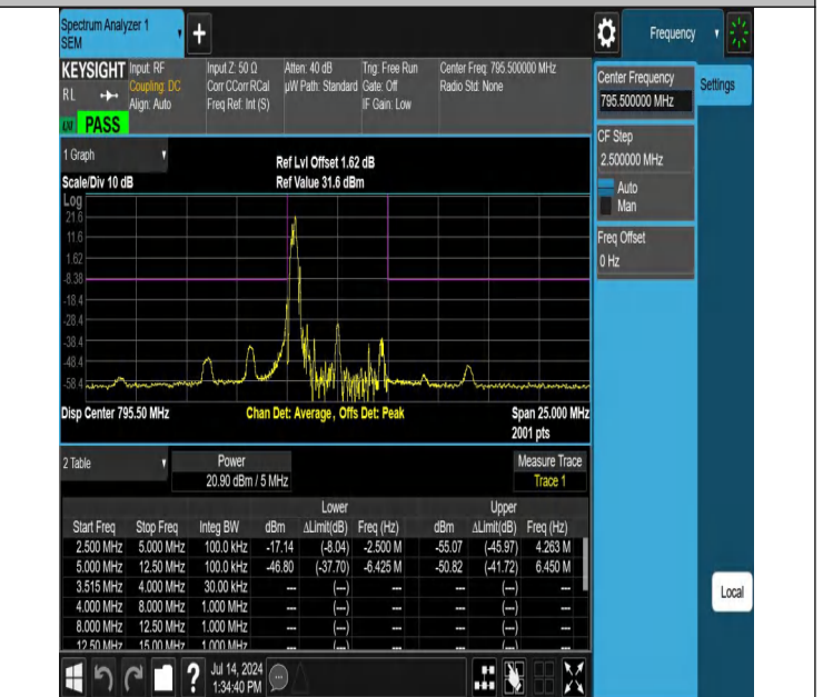
NTNV-Band14-5MHz-16QAM-23355-1RB#0-5.00-12.50-PASS
