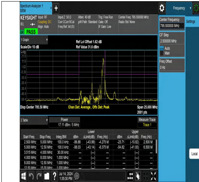
NTNV-Band14-5MHz-256QAM-23355-1RB#24--5.00--2.50-PASS
