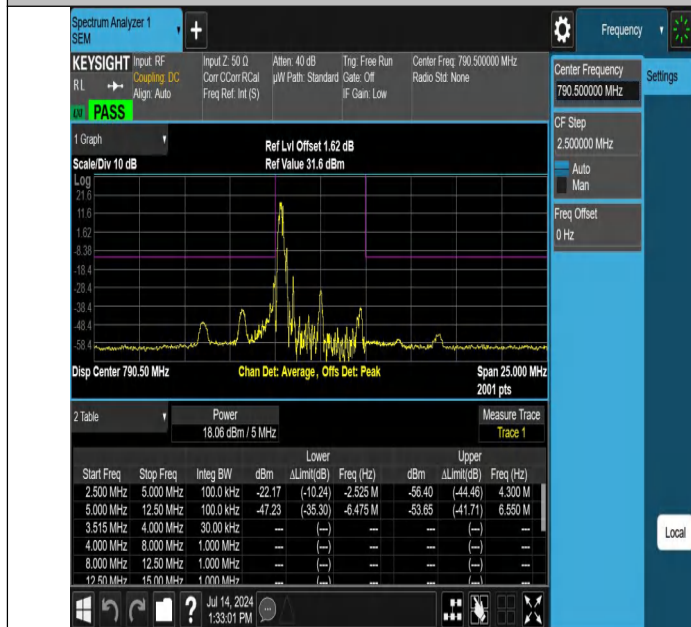
NTNV-Band14-5MHz-64QAM-23305-1RB#0--12.50--5.00-PASS
