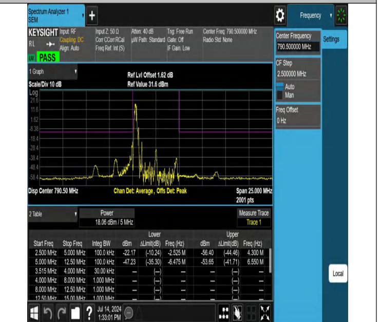
NTNV-Band14-5MHz-64QAM-23305-1RB#0-5.00-12.50-PASS
