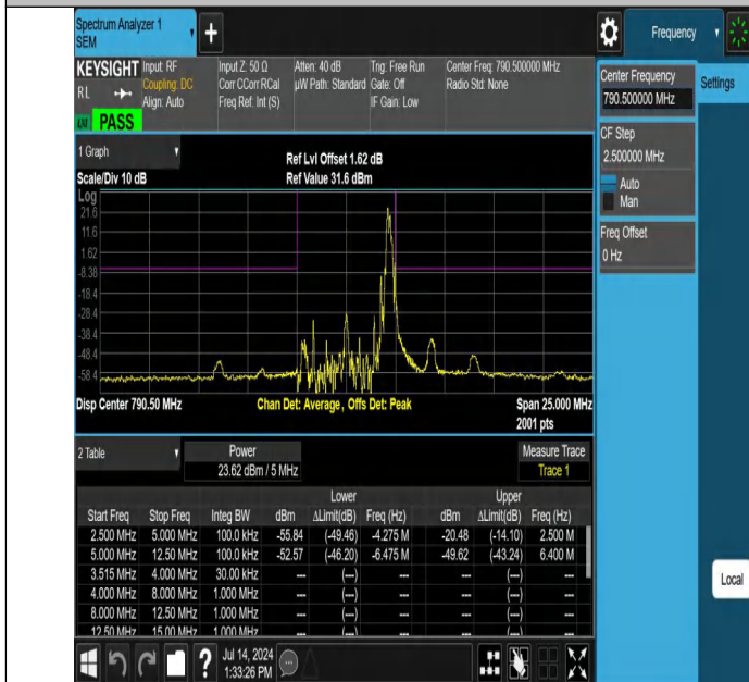
NTNV-Band14-5MHz-16QAM-23305-1RB#24--12.50--5.00-PASS
