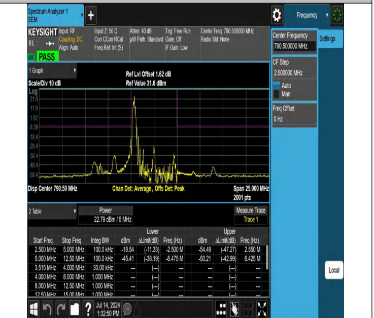
NTNV-Band14-5MHz-16QAM-23305-1RB#0-5.00-12.50-PASS
