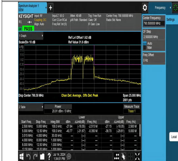
NTNV-Band14-5MHz-16QAM-23305-25RB#0--12.50--5.00-PASS
