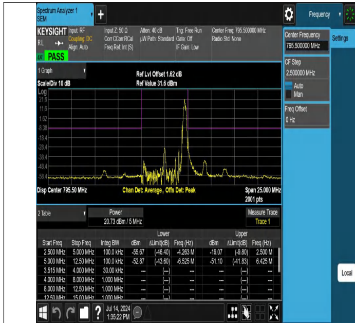
NTNV-Band14-5MHz-64QAM-23355-1RB#24--5.00--2.50-PASS
