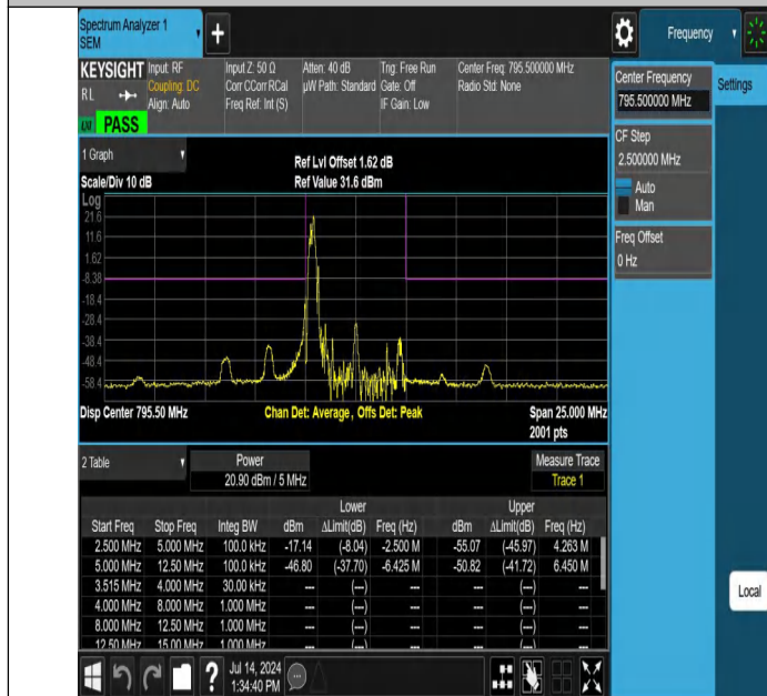
NTNV-Band14-5MHz-16QAM-23355-1RB#0--12.50--5.00-PASS
