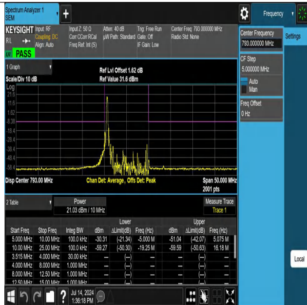
NTNV-Band14-10MHz-QPSK-23330-1RB#0--10.00--5.00-PASS
