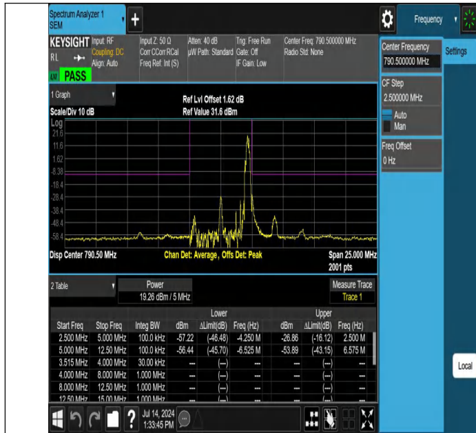
NTNV-Band14-5MHz-256QAM-23305-1RB#24--5.00--2.50-PASS
