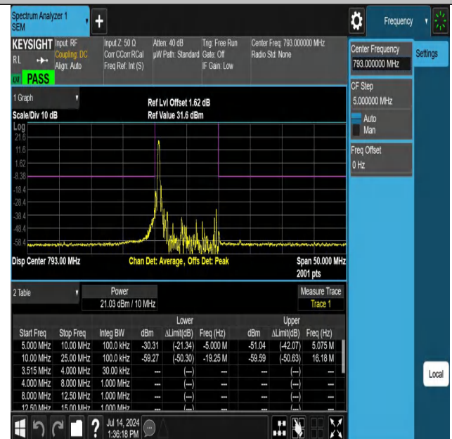
NTNV-Band14-10MHz-QPSK-23330-1RB#0-10.00-25.00-PASS
