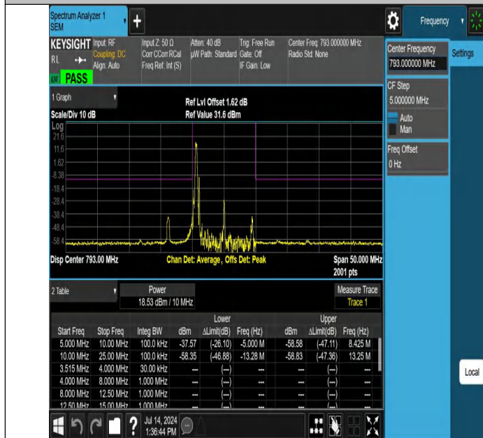
NTNV-Band14-10MHz-256QAM-23330-1RB#0--25.00--10.00-PASS
