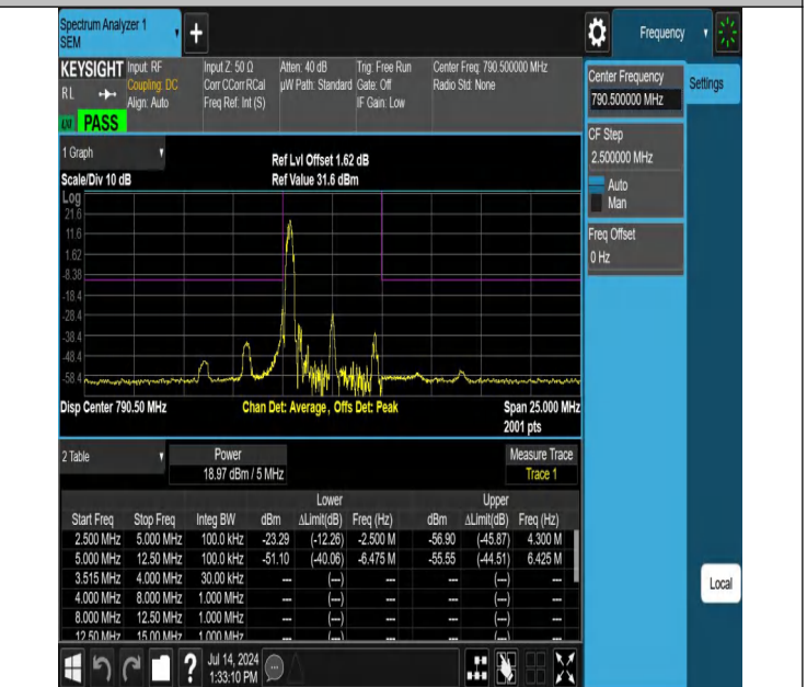
NTNV-Band14-5MHz-256QAM-23305-1RB#0-5.00-12.50-PASS
