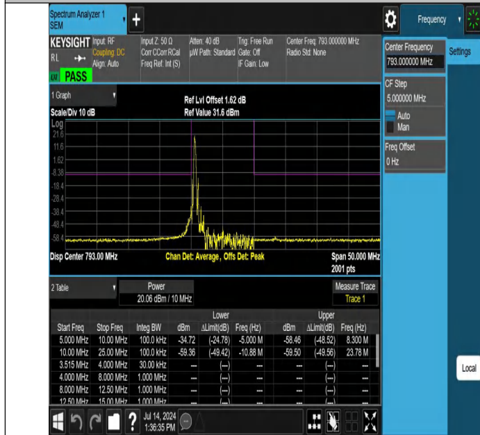
NTNV-Band14-10MHz-64QAM-23330-1RB#0--25.00--10.00-PASS
