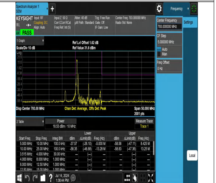
NTNV-Band14-10MHz-256QAM-23330-1RB#0-10.00-25.00-PASS
