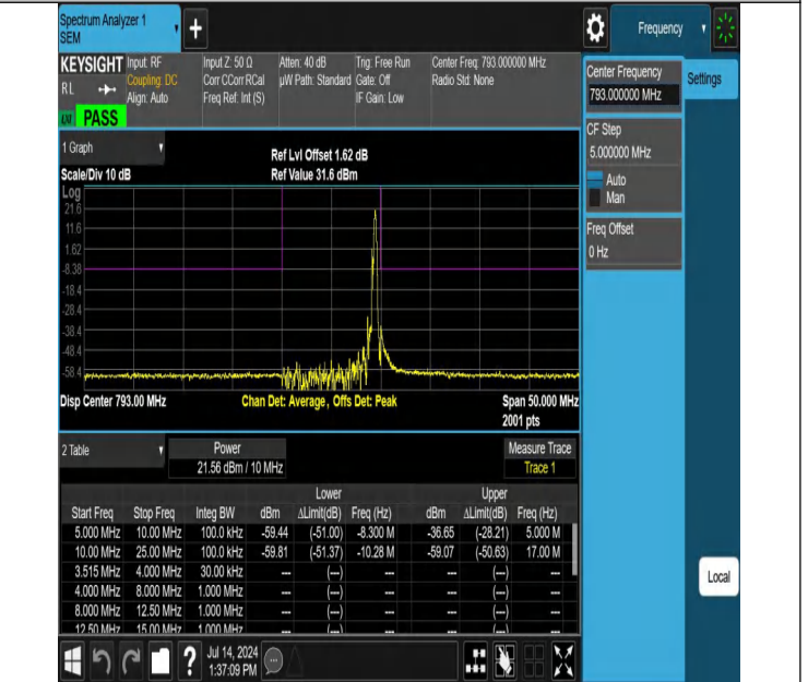
NTNV-Band14-10MHz-64QAM-23330-1RB#49-10.00-25.00-PASS
