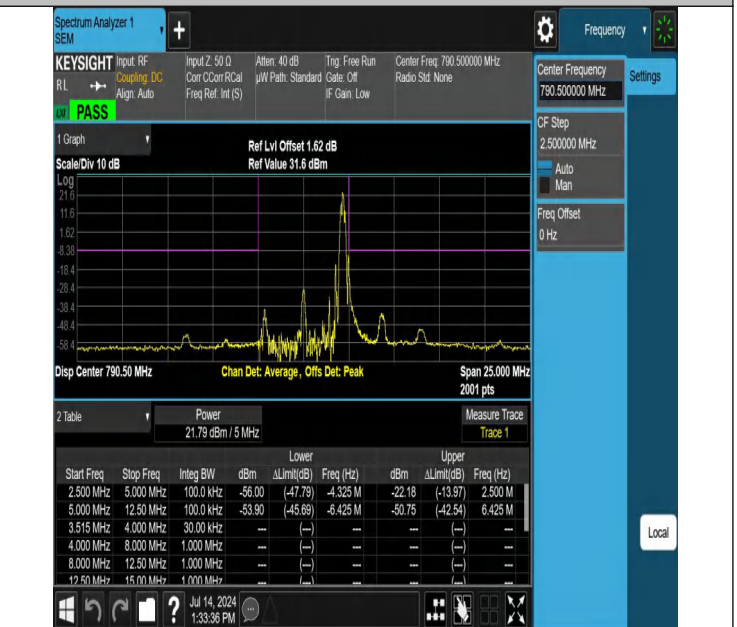
NTNV-Band14-5MHz-64QAM-23305-1RB#24-5.00-12.50-PASS
