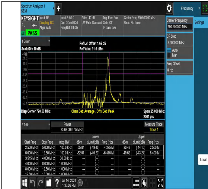
NTNV-Band14-5MHz-16QAM-23305-1RB#24--5.00--2.50-PASS
