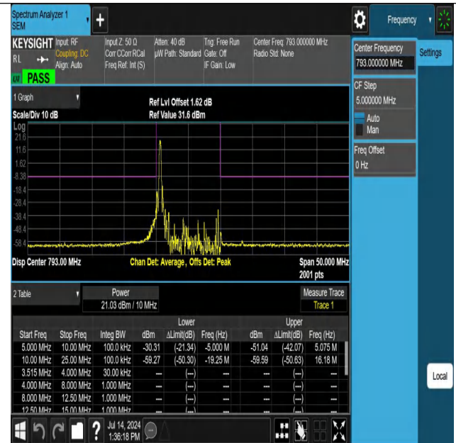
NTNV-Band14-10MHz-QPSK-23330-1RB#0-5.00-10.00-PASS
