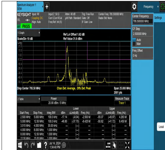
NTNV-Band14-5MHz-16QAM-23355-1RB#0--5.00--2.50-PASS
