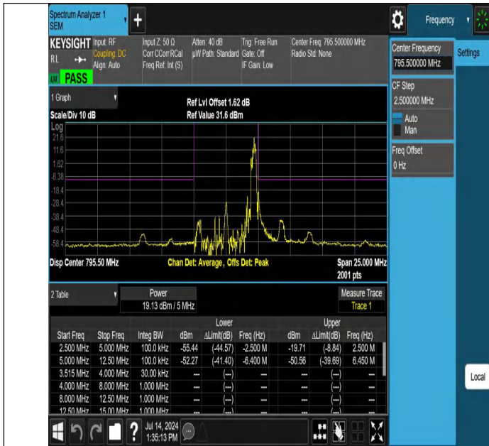
NTNV-Band14-5MHz-16QAM-23355-1RB#24--5.00--2.50-PASS
