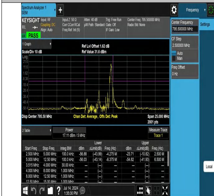
NTNV-Band14-5MHz-256QAM-23355-1RB#24--12.50--5.00-PASS
