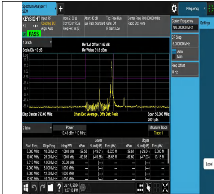
NTNV-Band14-10MHz-256QAM-23330-1RB#49--10.00--5.00-PASS
