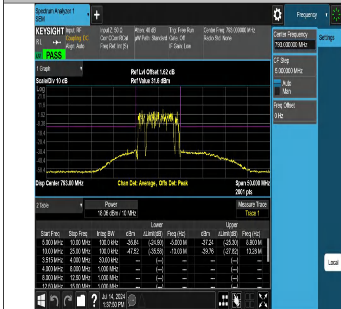
NTNV-Band14-10MHz-256QAM-23330-50RB#0--25.00--10.00-PAS
