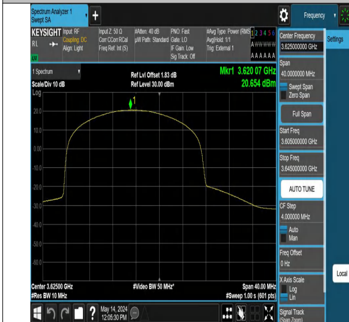
Band48-20MHz-QPSK-55990-50RB#25-PASS
