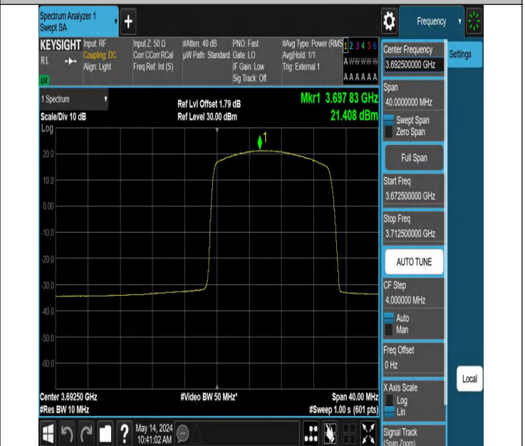
Band48-15MHz-16QAM-56665-1RB#74-PASS
