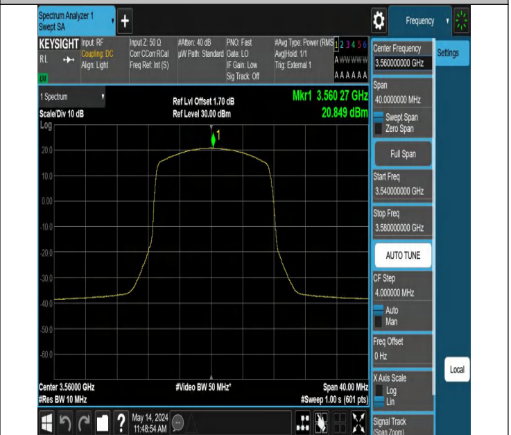
Band48-20MHz-16QAM-55340-1RB#49-PASS
