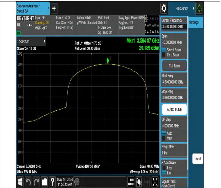
Band48-20MHz-QPSK-55340-50RB#50-PASS
