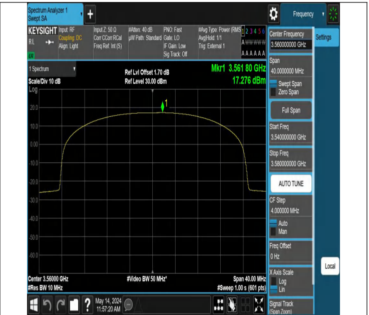
Band48-20MHz-16QAM-55340-100RB#0-PASS
