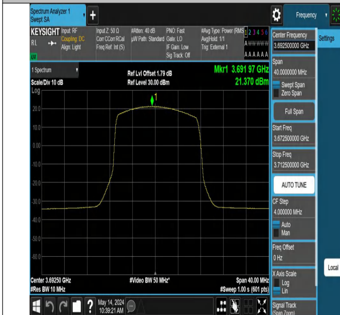
Band48-15MHz-16QAM-56665-1RB#38-PASS
