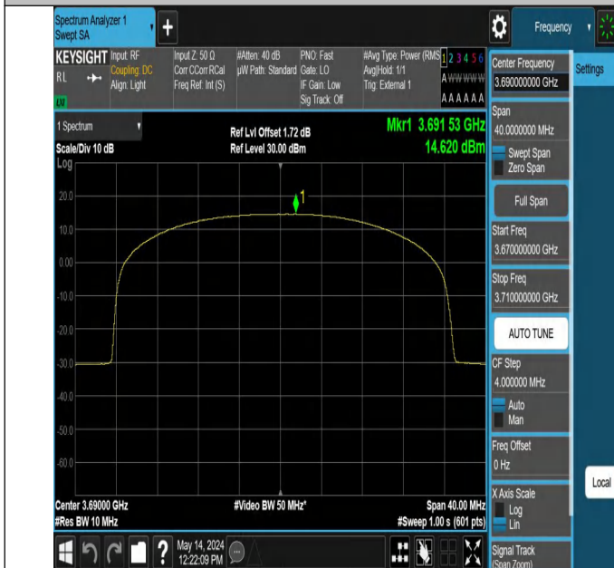
Band48-20MHz-256QAM-56640-100RB#0-PASS
