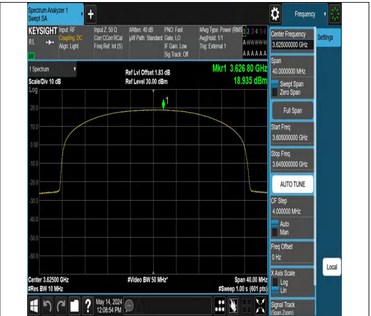
Band48-20MHz-QPSK-55990-100RB#0-PASS
