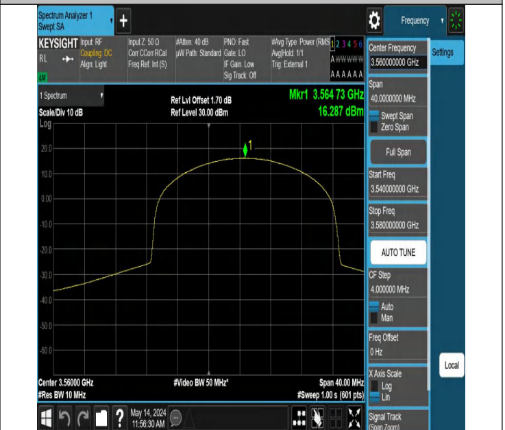
Band48-20MHz-256QAM-55340-50RB#50-PASS
