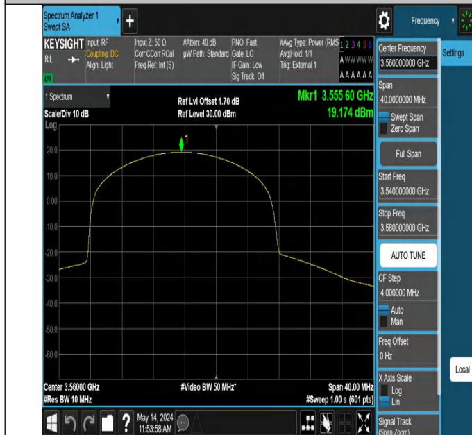
Band48-20MHz-16QAM-55340-50RB#25-PASS
