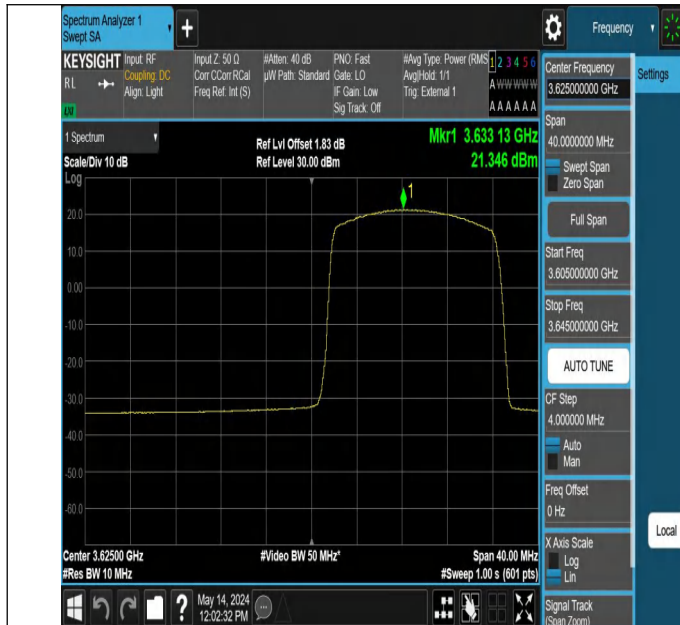
Band48-20MHz-16QAM-55990-1RB#99-PASS
