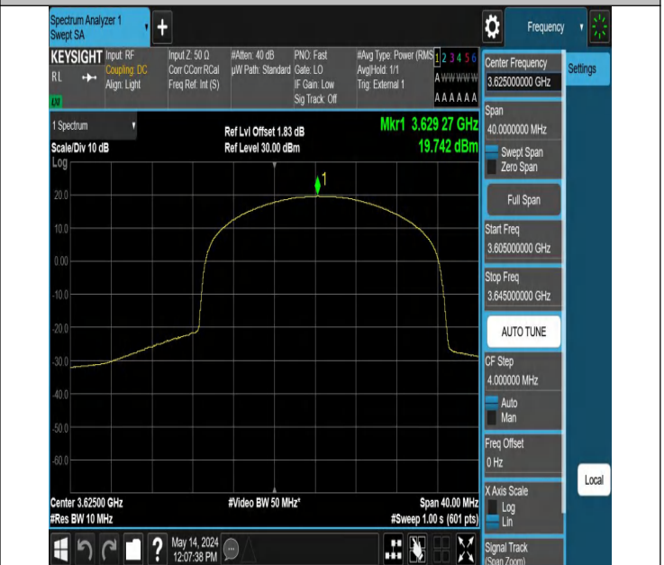
Band48-20MHz-16QAM-55990-50RB#50-PASS
