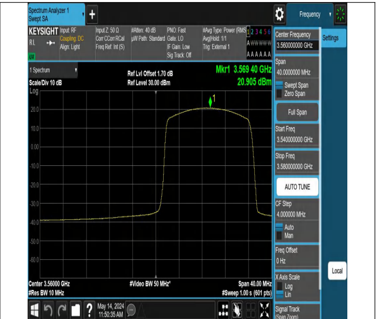
Band48-20MHz-16QAM-55340-1RB#99-PASS
