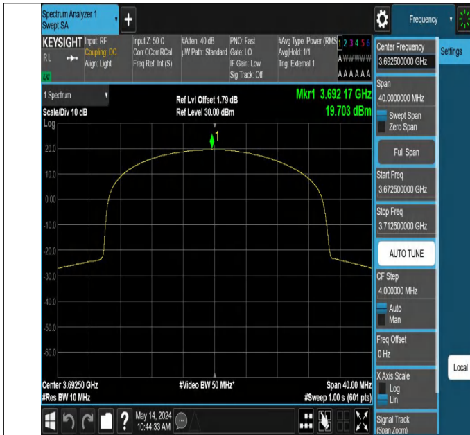
Band48-15MHz-16QAM-56665-38RB#18-PASS
