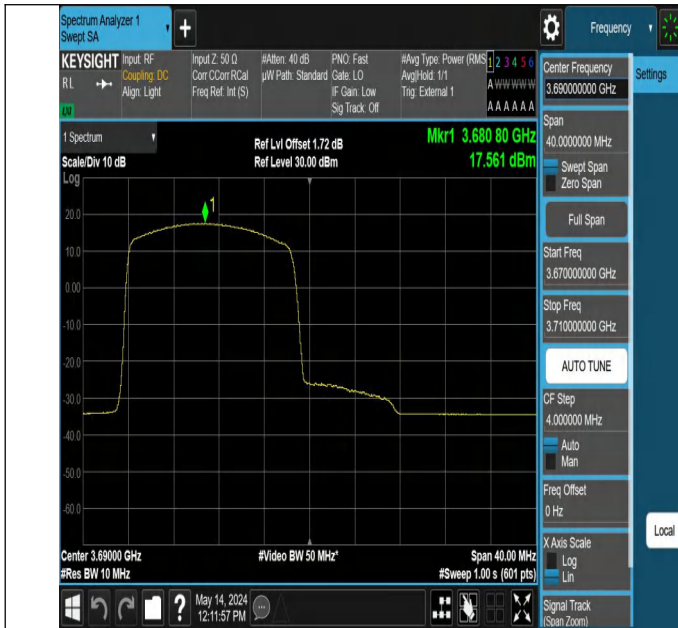
Band48-20MHz-256QAM-56640-1RB#0-PASS
