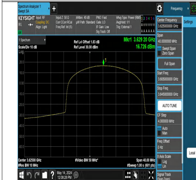
Band48-20MHz-256QAM-55990-50RB#50-PASS
