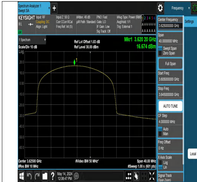
Band48-20MHz-256QAM-55990-50RB#25-PASS
