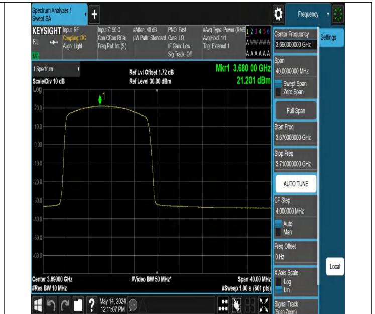
Band48-20MHz-16QAM-56640-1RB#0-PASS
