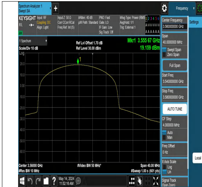
Band48-20MHz-16QAM-55340-50RB#0-PASS
