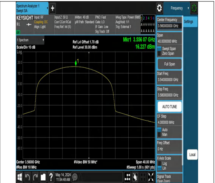
Band48-20MHz-256QAM-55340-50RB#25-PASS
