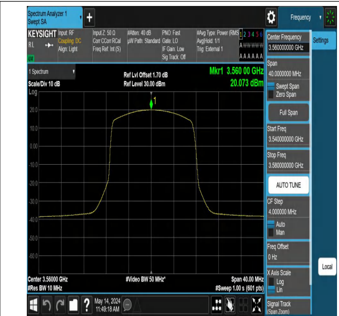
Band48-20MHz-64QAM-55340-1RB#49-PASS
