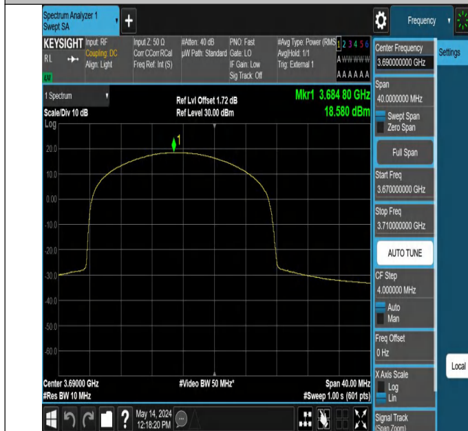
Band48-20MHz-64QAM-56640-50RB#25-PASS
