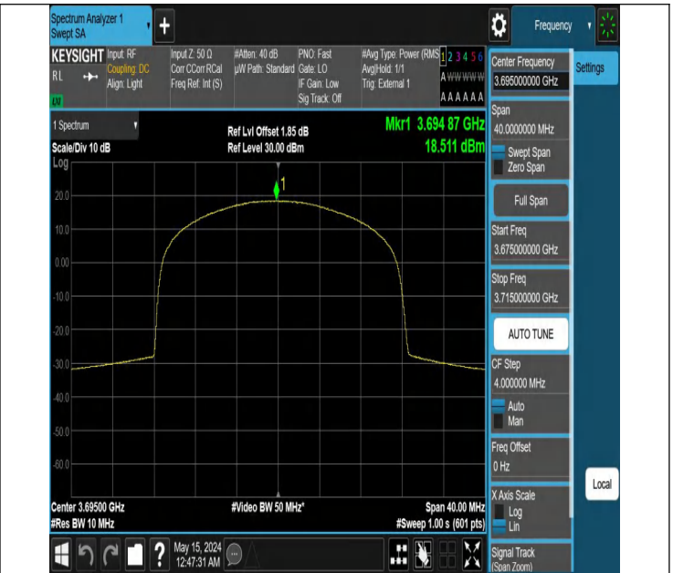
Band48-10MHz-64QAM-56690-50RB#0-PASS
