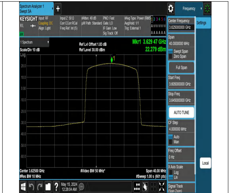
Band48-10MHz-QPSK-55990-1RB#49-PASS
