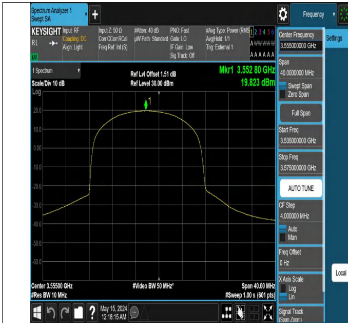
Band48-10MHz-16QAM-55290-25RB#0-PASS
