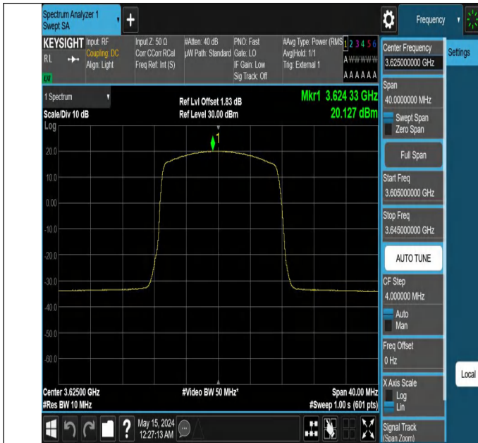
Band48-10MHz-64QAM-55990-1RB#24-PASS
