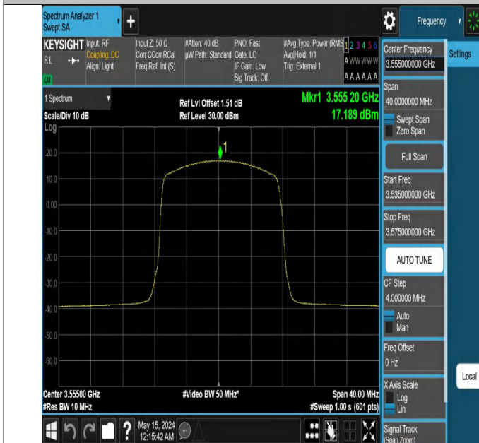
Band48-10MHz-256QAM-55290-1RB#24-PASS
