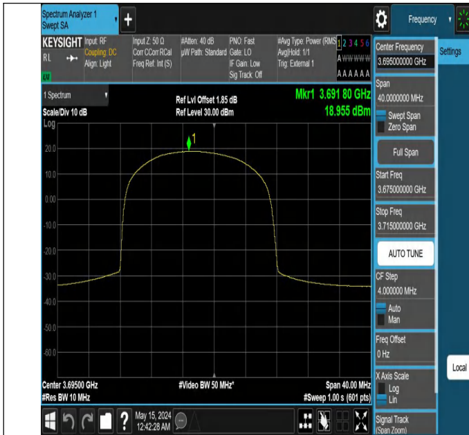
Band48-10MHz-64QAM-56690-25RB#0-PASS
