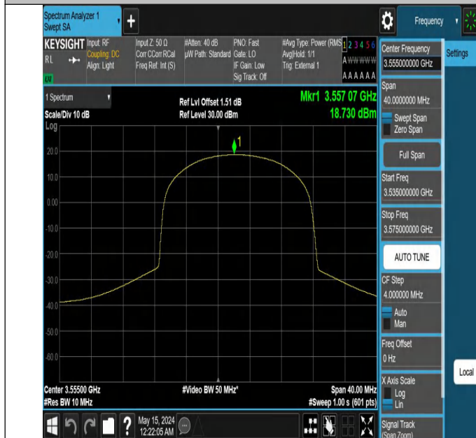
Band48-10MHz-64QAM-55290-25RB#25-PASS
