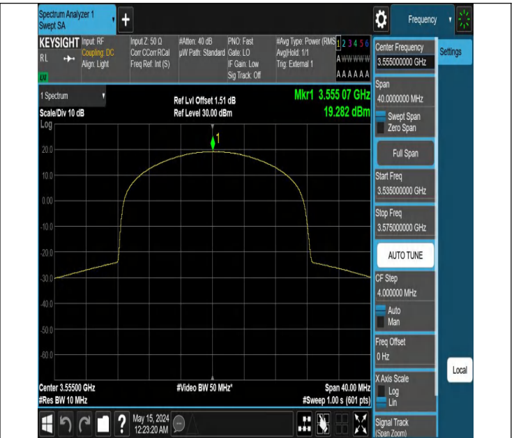
Band48-10MHz-16QAM-55290-50RB#0-PASS
