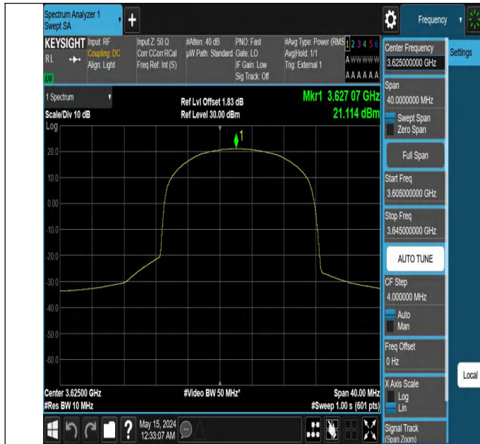
Band48-10MHz-QPSK-55990-25RB#25-PASS
