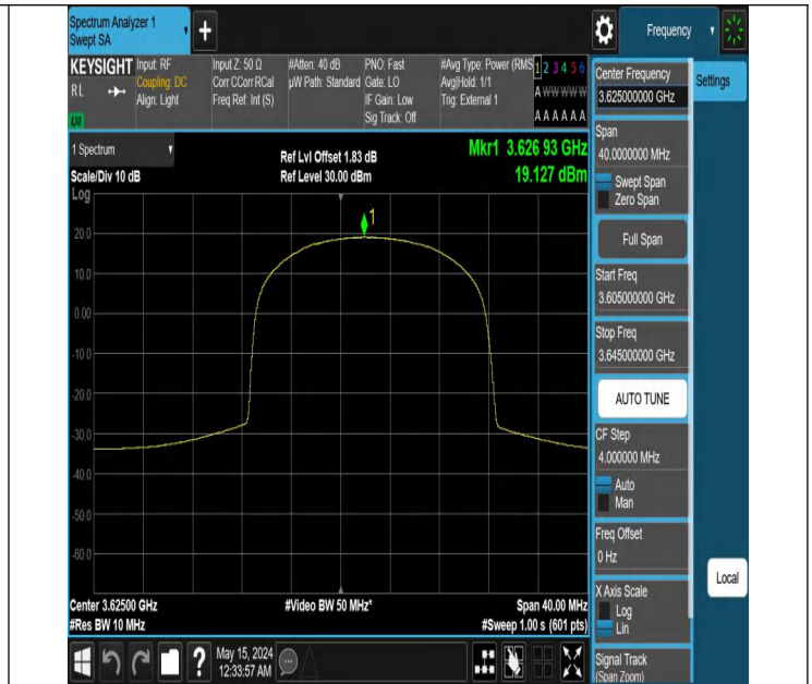
Band48-10MHz-64QAM-55990-25RB#25-PASS
