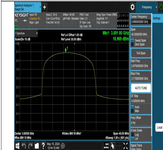
Band48-10MHz-64QAM-56690-25RB#12-PASS
