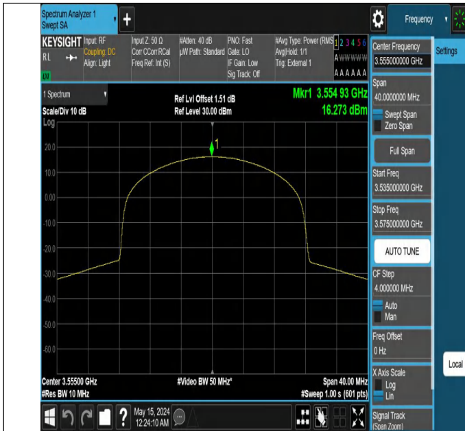
Band48-10MHz-256QAM-55290-50RB#0-PASS
