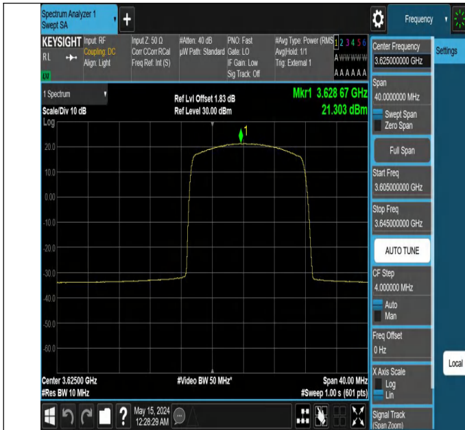
Band48-10MHz-16QAM-55990-1RB#49-PASS
