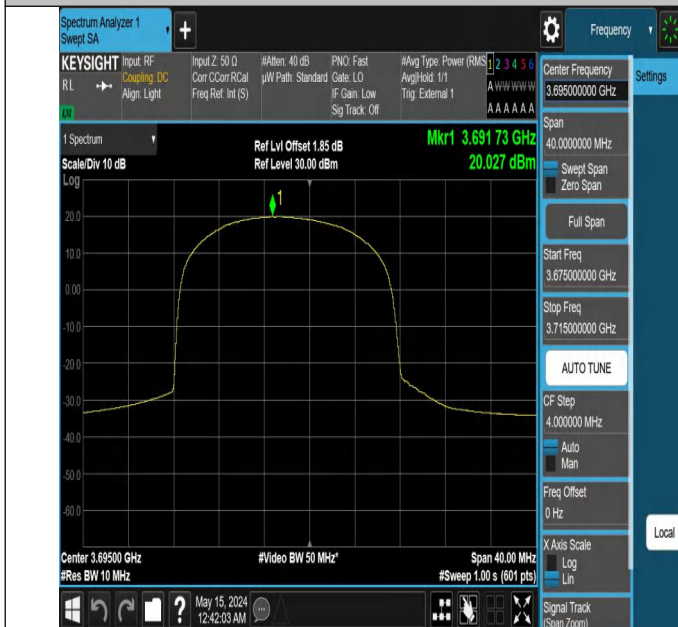
Band48-10MHz-16QAM-56690-25RB#0-PASS
