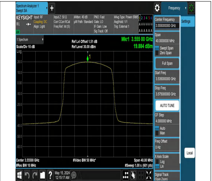
Band48-10MHz-64QAM-55290-1RB#24-PASS
