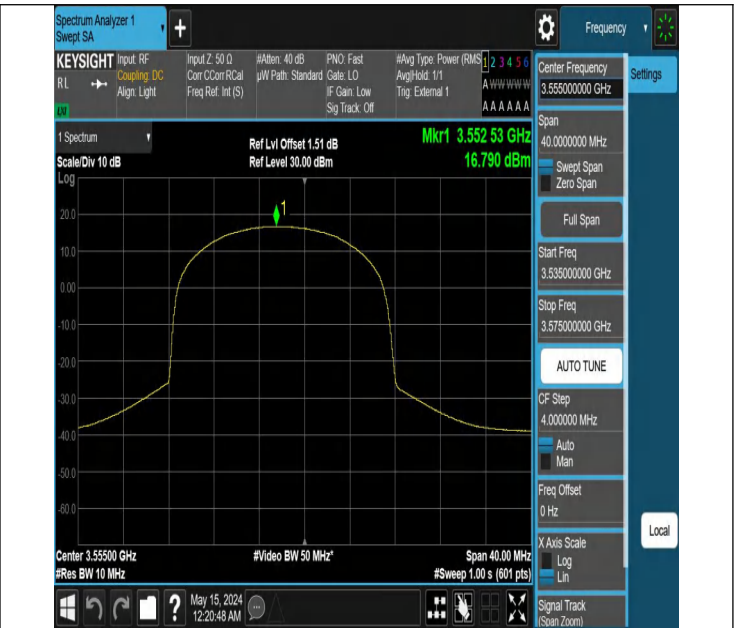
Band48-10MHz-256QAM-55290-25RB#12-PASS
