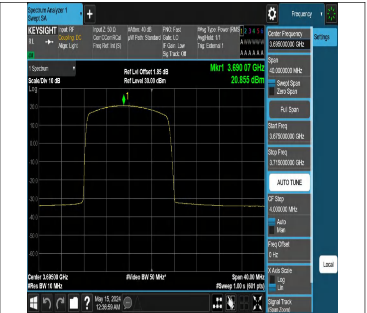
Band48-10MHz-16QAM-56690-1RB#0-PASS
