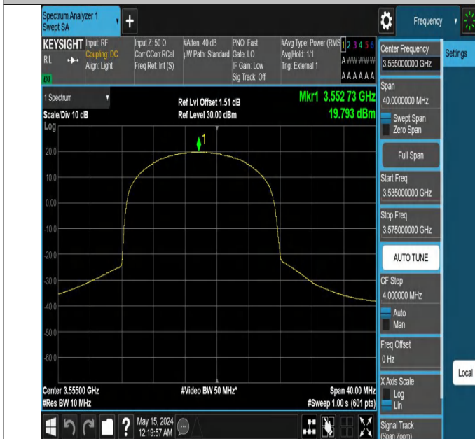
Band48-10MHz-16QAM-55290-25RB#12-PASS
