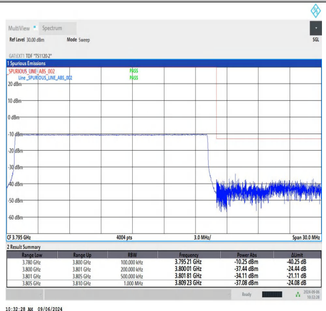
NTNV-n78(3700-3800)-PC2-30-20-H-CP-QPSK-Outer_Full-PA
