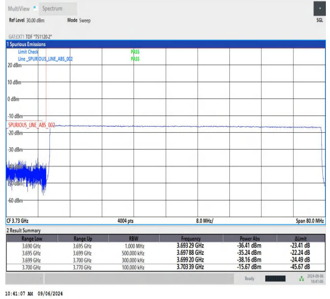
NTNV-n78(3700-3800)-PC2-30-70-L-CP-QPSK-Outer_Full-PA
