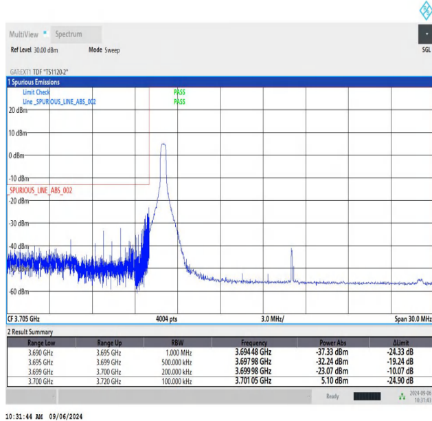
NTNV-n78(3700-3800)-PC2-30-20-L-CP-QPSK-Edge_1RB_Left-PAS
