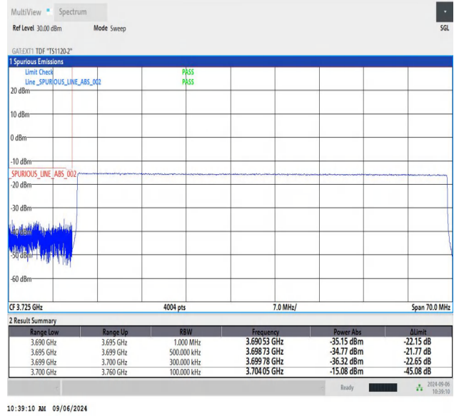
NTNV-n78(3700-3800)-PC2-30-60-L-CP-QPSK-Outer_Full-PA
