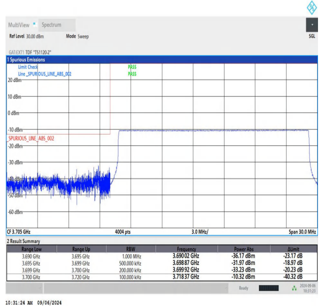
NTNV-n78(3700-3800)-PC2-30-20-L-CP-QPSK-Outer_Full-PA
