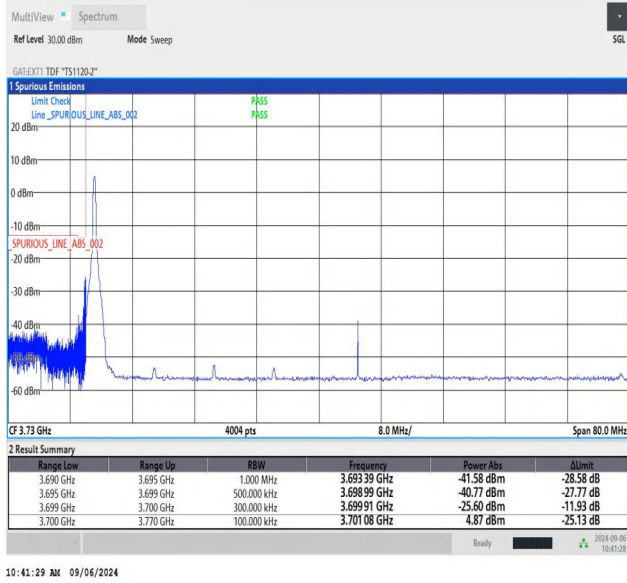
NTNV-n78(3700-3800)-PC2-30-70-L-CP-QPSK-Edge_1RB_Left-PAS
