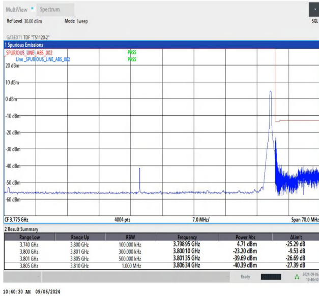
NTNV-n78(3700-3800)-PC2-30-60-H-CP-QPSK-Edge_1RB_Right-PA
