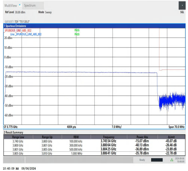
NTNV-n78(3700-3800)-PC2-30-60-H-CP-QPSK-Outer_Full-PA
