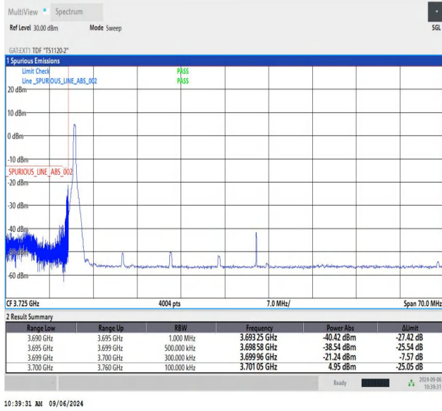
NTNV-n78(3700-3800)-PC2-30-60-L-CP-QPSK-Edge_1RB_Left-PAS
