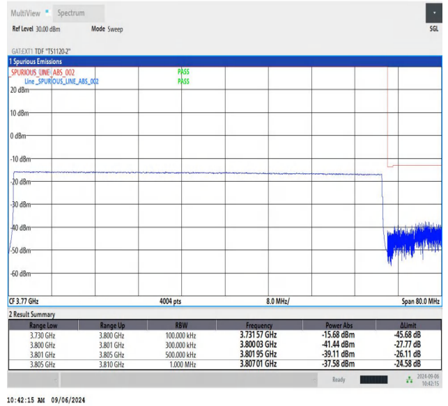
NTNV-n78(3700-3800)-PC2-30-70-H-CP-QPSK-Outer_Full-PA
