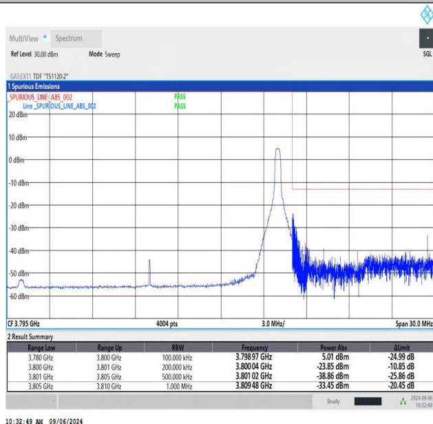
NTNV-n78(3700-3800)-PC2-30-20-H-CP-QPSK-Edge_1RB_Right-PA
