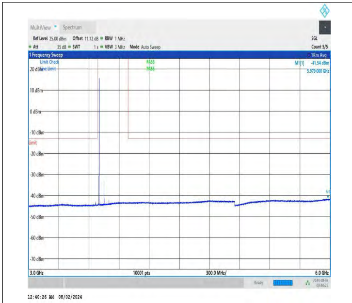
NTNV-DC_26A-n78A(3700-3800)-PC3-30-5+100-M+M-QPSK-ID LE-DFT-BPSK-Edge_1RB_Left-3000-6000-PASS
