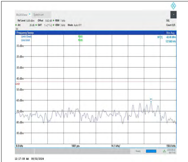
NTNV-DC_26A-n78A(3700-3800)-PC3-30-5+90-M+L-QPSK-IDL E-DFT-BPSK-Edge_1RB_Left-0.009-0.15-PASS
