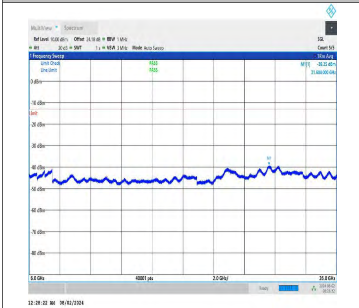
NTNV-DC_26A-n78A(3700-3800)-PC3-30-5+90-M+M-QPSK-IDL E-DFT-QPSK-Edge_1RB_Right-6000-26000-PASS
