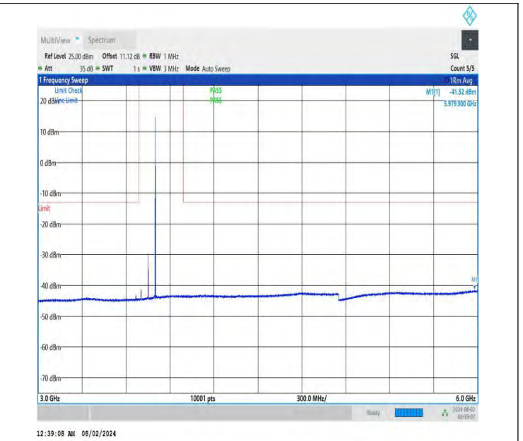
NTNV-DC_26A-n78A(3700-3800)-PC3-30-5+100-M+L-QPSK-IDL E-DFT-QPSK-Edge_1RB_Right-3000-6000-PASS
