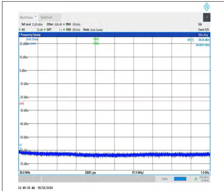
NTNV-DC_26A-n78A(3700-3800)-PC3-30-5+100-M+H-QPSK-ID LE-DFT-QPSK-Edge_1RB_Left-30-1000-PASS
