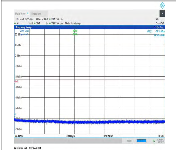
NTNV-DC_26A-n78A(3700-3800)-PC3-30-5+100-M+L-QPSK-IDL E-DFT-BPSK-Edge_1RB_Left-30-1000-PASS
