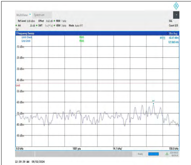
NTNV-DC_26A-n78A(3700-3800)-PC3-30-5+100-M+M-QPSK-ID LE-DFT-BPSK-Edge_1RB_Left-0.009-0.15-PASS
