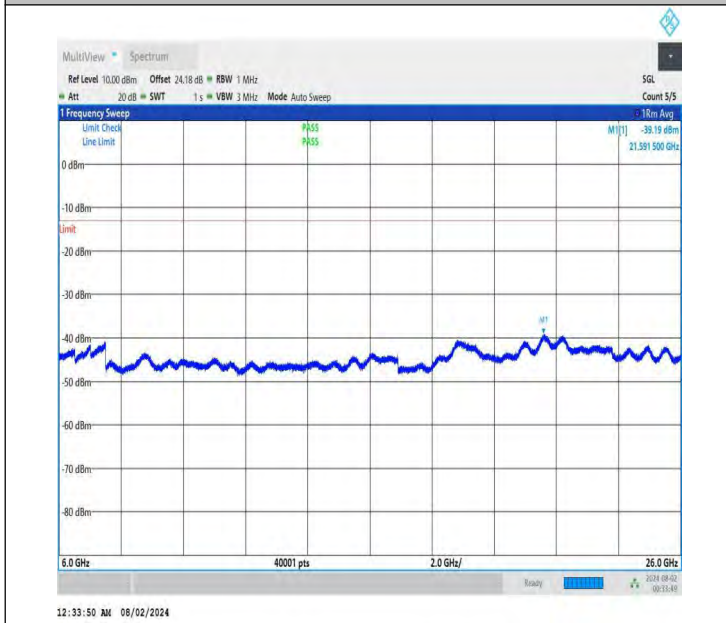
NTNV-DC_26A-n78A(3700-3800)-PC3-30-5+90-M+H-QPSK-IDL E-DFT-QPSK-Edge_1RB_Right-6000-26000-PASS
