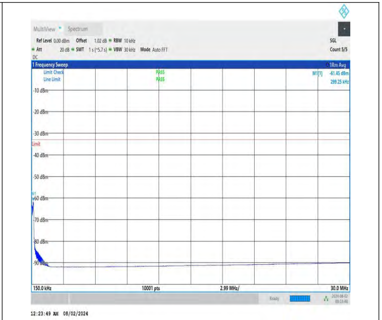
NTNV-DC_26A-n78A(3700-3800)-PC3-30-5+90-M+M-QPSK-IDLE -DFT-BPSK-Edge_1RB_Left-0.15-30-PASS
