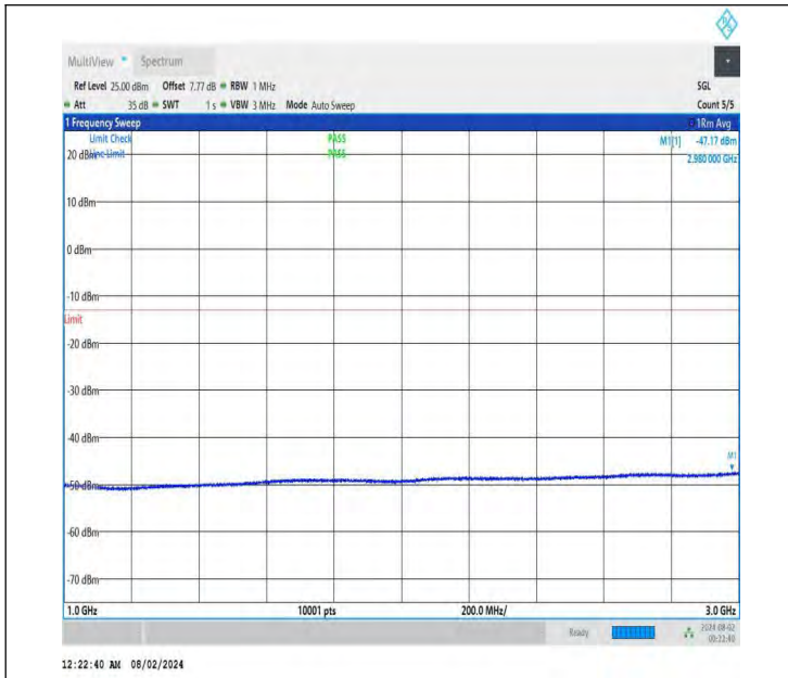
NTNV-DC_26A-n78A(3700-3800)-PC3-30-5+90-M+L-QPSK-IDL E-DFT-QPSK-Edge_1RB_Right-1000-3000-PASS
