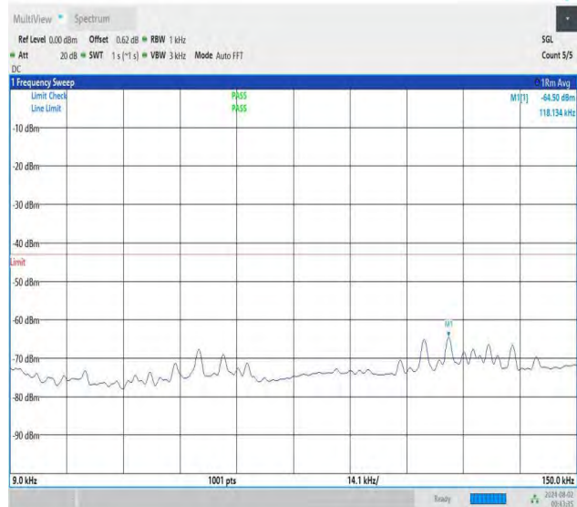
NTNV-DC_26A-n78A(3700-3800)-PC3-30-5+100-M+M-QPSK-IDL E-DFT-QPSK-Edge 1RB Right-0.009-0.15-PASS
