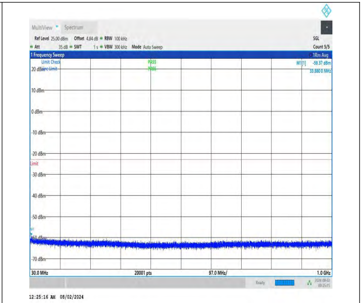
NTNV-DC_26A-n78A(3700-3800)-PC3-30-5+90-M+M-QPSK-IDLE -DFT-BPSK-Edge_1RB_Right-30-1000-PASS
