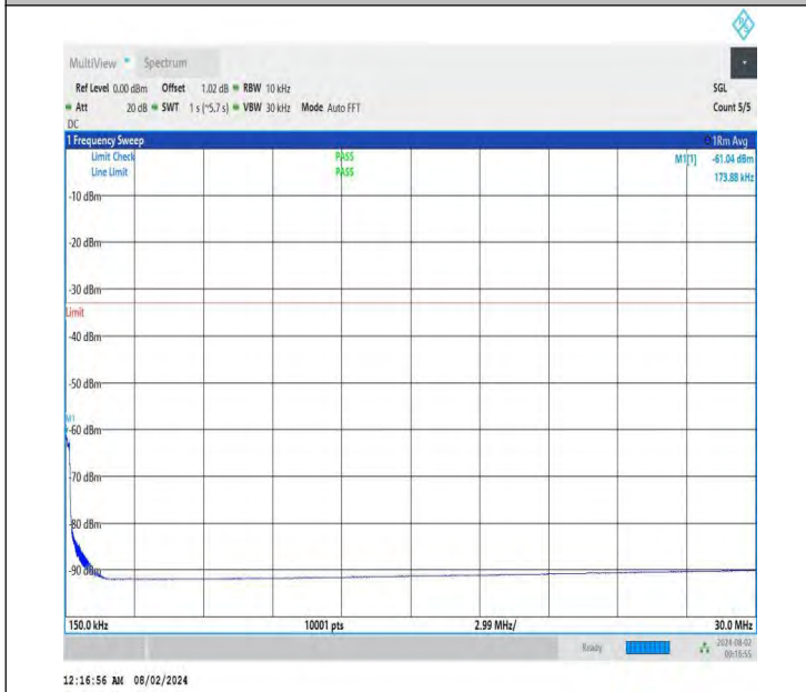
NTNV-DC_26A-n78A(3700-3800)-PC3-30-5+80-M+H-QPSK-IDL E-DFT-QPSK-Edge_1RB_Right-0.15-30-PASS
