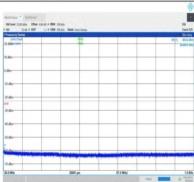
NTNV-DC_26A-n78A(3700-3800)-PC3-30-5+100-M+M-QPSK-IDL E-DFT-QPSK-Edge 1RB Right-0.009-0.15-PASS
