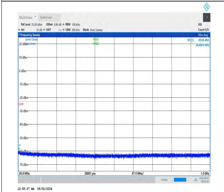
NTNV-DC_26A-n78A(3700-3800)-PC3-30-5+100-M+H-QPSK-ID LE-DFT-BPSK-Edge_1RB_Left-30-1000-PASS
