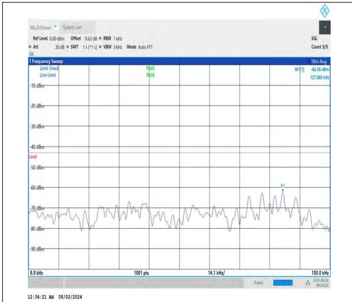
NTNV-DC_26A-n78A(3700-3800)-PC3-30-5+100-M+L-QPSK-IDL E-DFT-BPSK-Edge_1RB_Left-0.009-0.15-PASS
