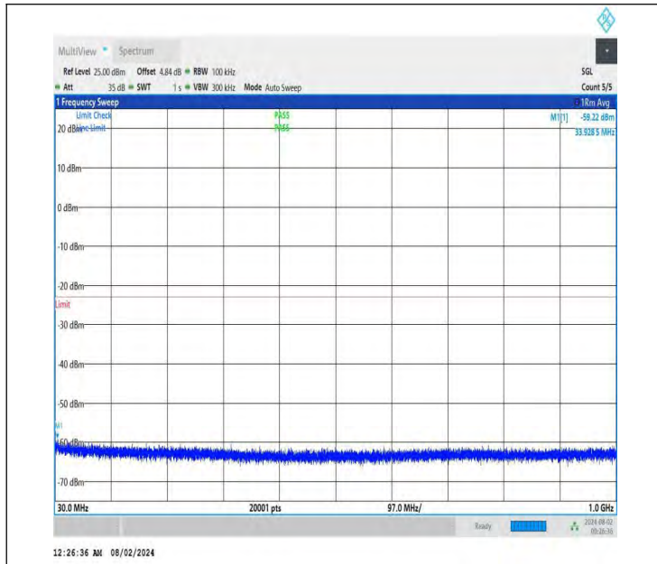
NTNV-DC_26A-n78A(3700-3800)-PC3-30-5+90-M+M-QPSK-IDL E-DFT-QPSK-Edge_1RB_Left-30-1000-PASS
