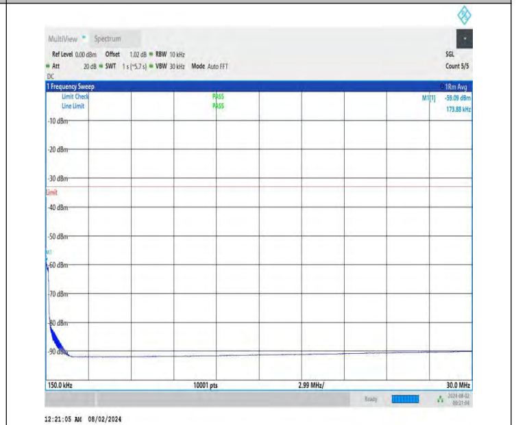
NTNV-DC_26A-n78A(3700-3800)-PC3-30-5+90-M+L-QPSK-IDLE -DFT-QPSK-Edge_1RB_Left-0.15-30-PASS
