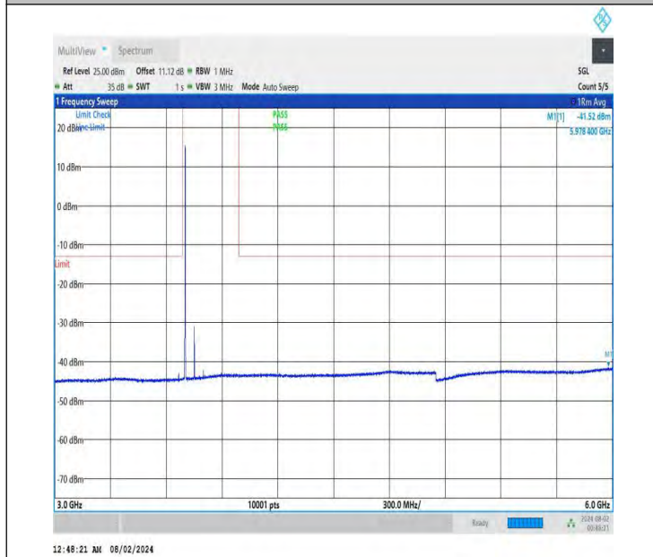
NTNV-DC_26A-n78A(3700-3800)-PC3-30-5+100-M+H-QPSK-ID LE-DFT-QPSK-Edge_1RB_Left-3000-6000-PASS
