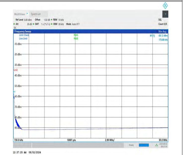
NTNV-DC_26A-n78A(3700-3800)-PC3-30-5+100-M+L-QPSK-IDL E-DFT-QPSK-Edge_1RB_Left-0.15-30-PASS
