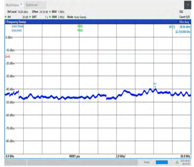
NTNV-DC_26A-n78A(3700-3800)-PC3-30-5+90-M+H-QPSK-IDLE -DFT-BPSK-Edge_1RB_Left-6000-26000-PASS
