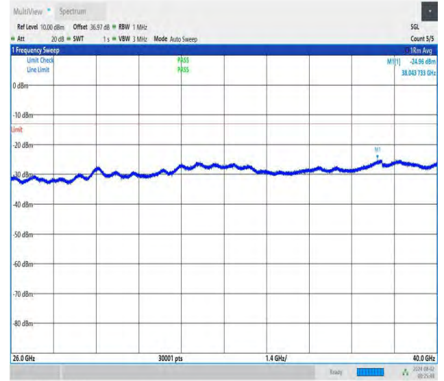
NTNV-DC_26A-n78A(3700-3800)-PC3-30-5+90-M+M-QPSK-IDLE -DFT-BPSK-Edge_1RB_Right-26000-40000-PASS
