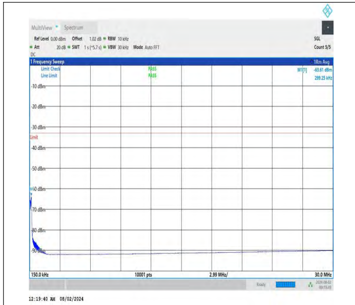
NTNV-DC_26A-n78A(3700-3800)-PC3-30-5+90-M+L-QPSK-IDL E-DFT-BPSK-Edge_1RB_Right-0.15-30-PASS
