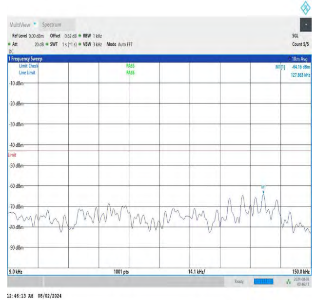
NTNV-DC_26A-n78A(3700-3800)-PC3-30-5+100-M+H-QPSK-IDL E-DFT-BPSK-Edge_1RB_Right-0.009-0.15-PASS
