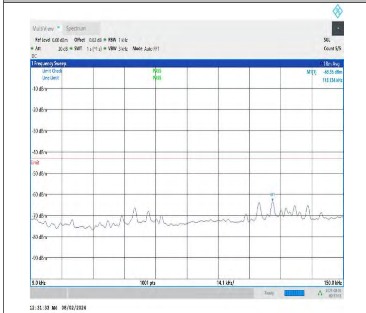
NTNV-DC_26A-n78A(3700-3800)-PC3-30-5+90-M+H-QPSK-IDL E-DFT-QPSK-Edge_1RB_Left-0.009-0.15-PASS
