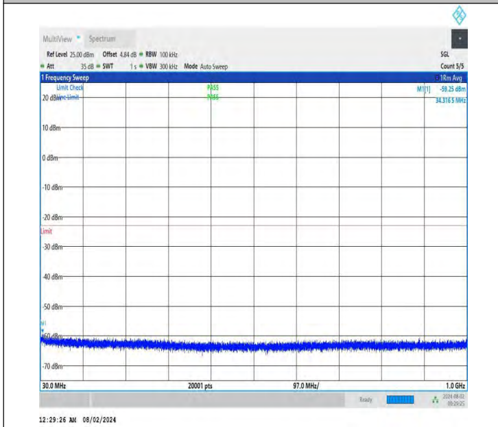
NTNV-DC_26A-n78A(3700-3800)-PC3-30-5+90-M+H-QPSK-IDL E-DFT-BPSK-Edge_1RB_Left-30-1000-PASS
