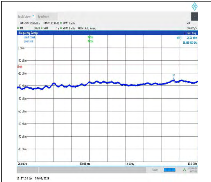
NTNV-DC_26A-n78A(3700-3800)-PC3-30-5+90-M+M-QPSK-IDL E-DFT-QPSK-Edge_1RB_Left-26000-40000-PASS
