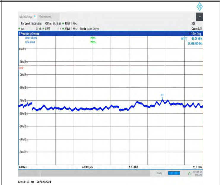
NTNV-DC_26A-n78A(3700-3800)-PC3-30-5+100-M+M-QPSK-IDL E-DFT-QPSK-Edge_1RB_Left-6000-26000-PASS
