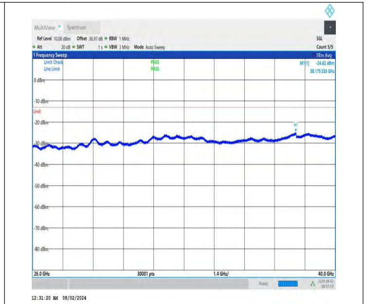
NTNV-DC_26A-n78A(3700-3800)-PC3-30-5+90-M+H-QPSK-IDLE -DFT-BPSK-Edge_1RB_Right-26000-40000-PASS
