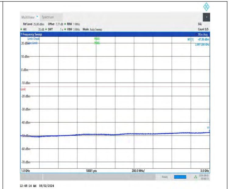
NTNV-DC_26A-n78A(3700-3800)-PC3-30-5+100-M+H-QPSK-IDL E-DFT-QPSK-Edge_1RB_Left-1000-3000-PASS
