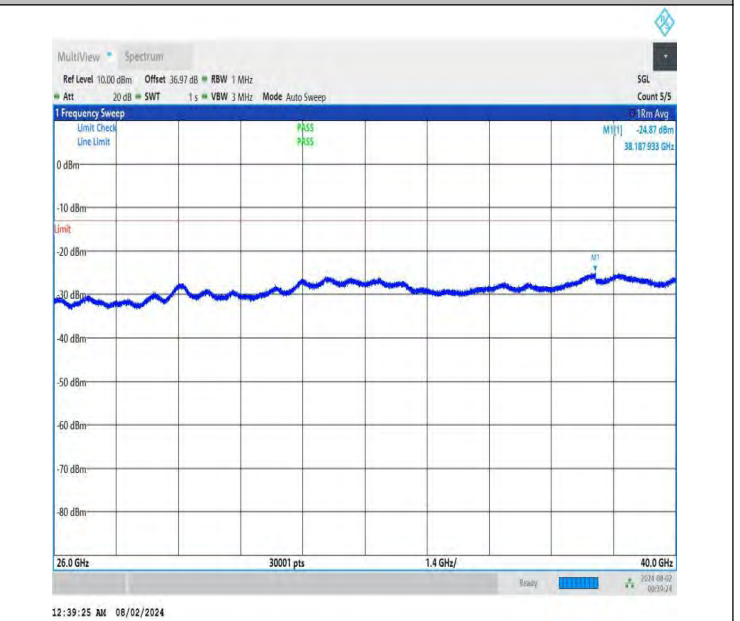
NTNV-DC_26A-n78A(3700-3800)-PC3-30-5+100-M+L-QPSK-IDL E-DFT-QPSK-Edge_1RB_Right-26000-40000-PASS
