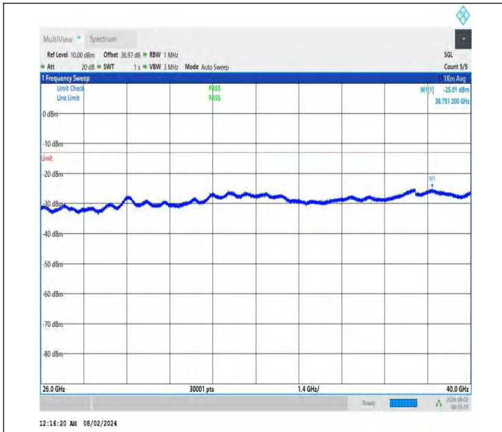
NTNV-DC_26A-n78A(3700-3800)-PC3-30-5+80-M+H-QPSK-IDL E-DFT-QPSK-Edge_1RB_Left-26000-40000-PASS
