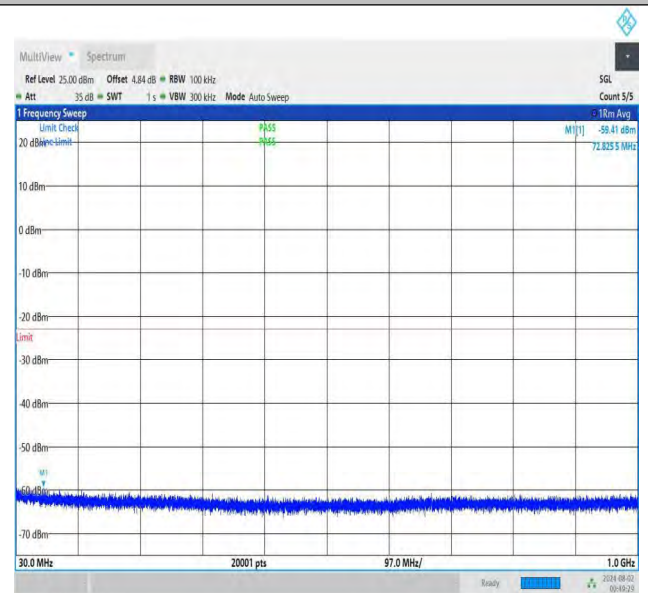
NTNV-DC_26A-n78A(3700-3800)-PC3-30-5+100-M+H-QPSK-IDL E-DFT-QPSK-Edge_1RB_Right-0.009-0.15-PASS
