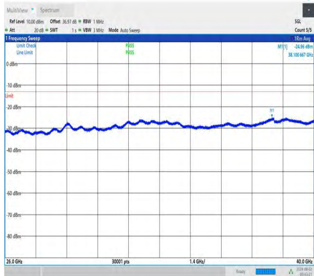
NTNV-DC_26A-n78A(3700-3800)-PC3-30-5+100-M+M-QPSK-ID LE-DFT-QPSK-Edge 1RB Left-26000-40000-PASS
