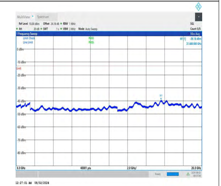
NTNV-DC_26A-n78A(3700-3800)-PC3-30-5+90-M+M-QPSK-IDLE -DFT-QPSK-Edge_1RB_Left-6000-26000-PASS
