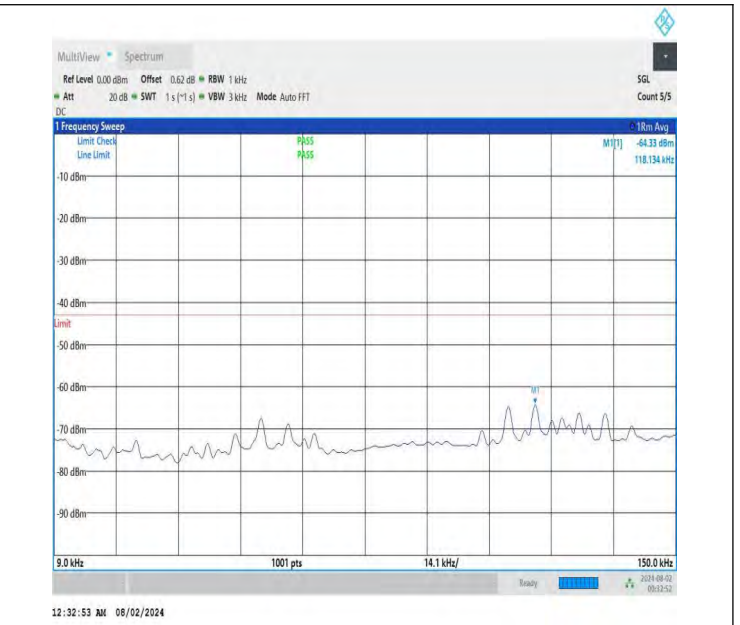
NTNV-DC_26A-n78A(3700-3800)-PC3-30-5+90-M+H-QPSK-IDLE -DFT-QPSK-Edge_1RB_Right-0.009-0.15-PASS
