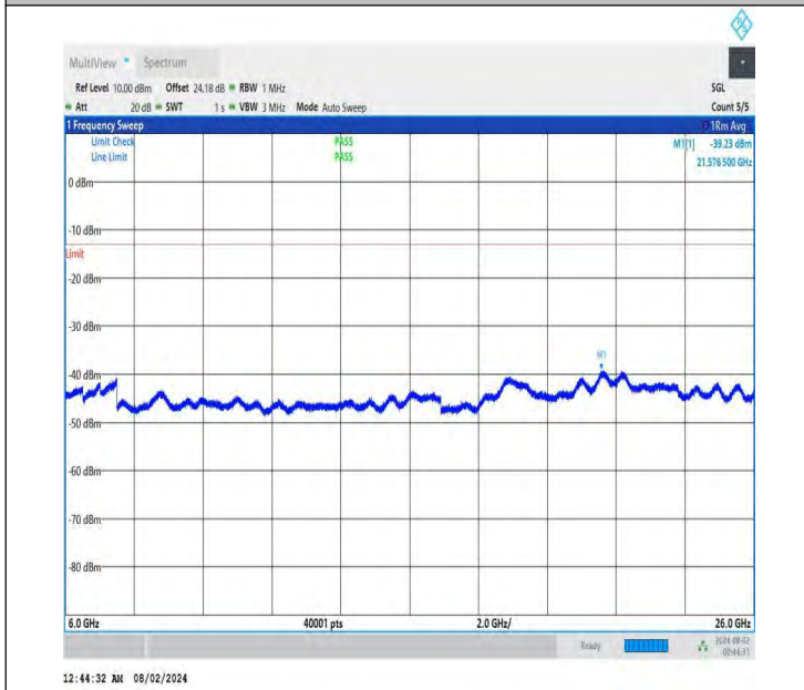
NTNV-DC_26A-n78A(3700-3800)-PC3-30-5+100-M+M-QPSK-ID LE-DFT-QPSK-Edge_1RB_Right-6000-26000-PASS
