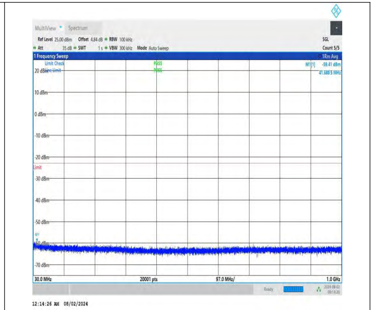
NTNV-DC_26A-n78A(3700-3800)-PC3-30-5+80-M+H-QPSK-IDLE -DFT-BPSK-Edge_1RB_Right-30-1000-PASS
