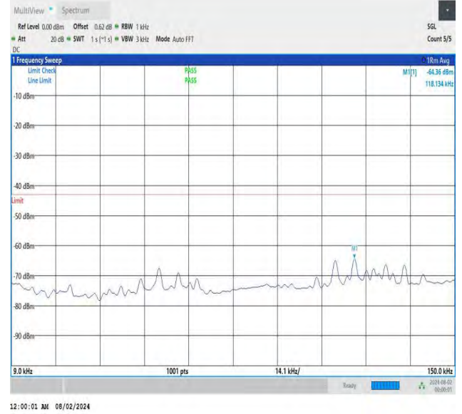
NTNV-DC_26A-n78A(3700-3800)-PC3-30-5+70-M+H-QPSK-IDLE -DFT-QPSK-Edge_1RB_Right-0.009-0.15-PASS
