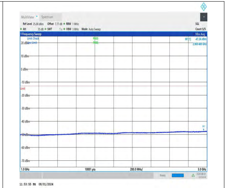
NTNV-DC_26A-n78A(3700-3800)-PC3-30-5+70-M+M-QPSK-IDLE -DFT-QPSK-Edge_1RB_Left-1000-3000-PASS
