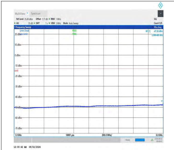
NTNV-DC_26A-n78A(3700-3800)-PC3-30-5+70-M+H-QPSK-IDL E-DFT-QPSK-Edge_1RB_Right-1000-3000-PASS
