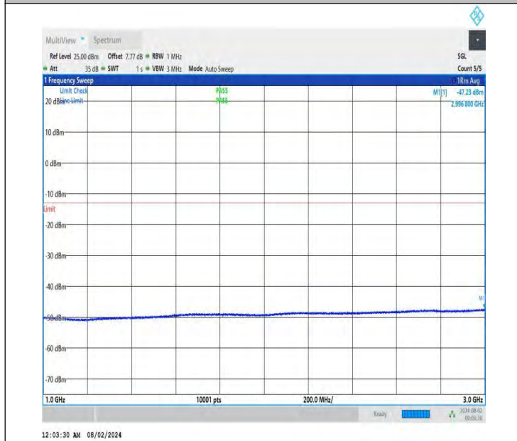
NTNV-DC_26A-n78A(3700-3800)-PC3-30-5+80-M+L-QPSK-IDL E-DFT-BPSK-Edge_1RB_Right-1000-3000-PASS
