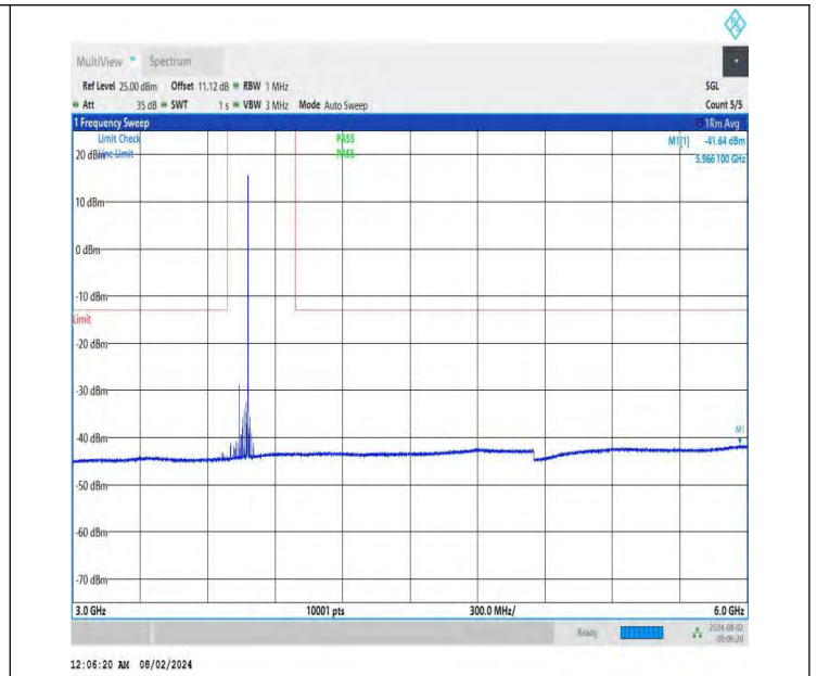
NTNV-DC_26A-n78A(3700-3800)-PC3-30-5+80-M+L-QPSK-IDLE -DFT-QPSK-Edge_1RB_Right-3000-6000-PASS
