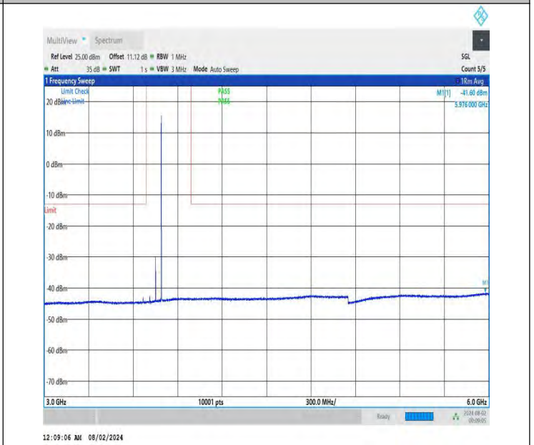
NTNV-DC_26A-n78A(3700-3800)-PC3-30-5+80-M+M-QPSK-IDLE -DFT-BPSK-Edge_1RB_Right-3000-6000-PASS
