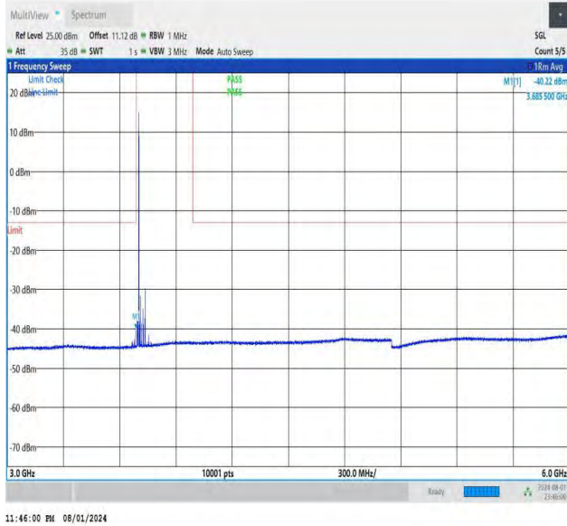
NTNV-DC_26A-n78A(3700-3800)-PC3-30-5+70-M+L-QPSK-IDL E-DFT-BPSK-Edge_1RB_Left-3000-6000-PASS
