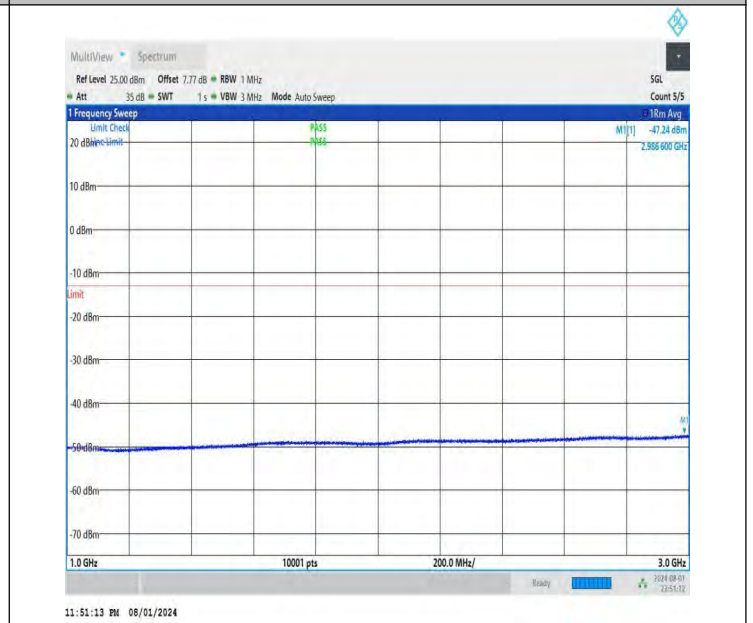
NTNV-DC_26A-n78A(3700-3800)-PC3-30-5+70-M+M-QPSK-IDLE -DFT-BPSK-Edge_1RB_Left-1000-3000-PASS
