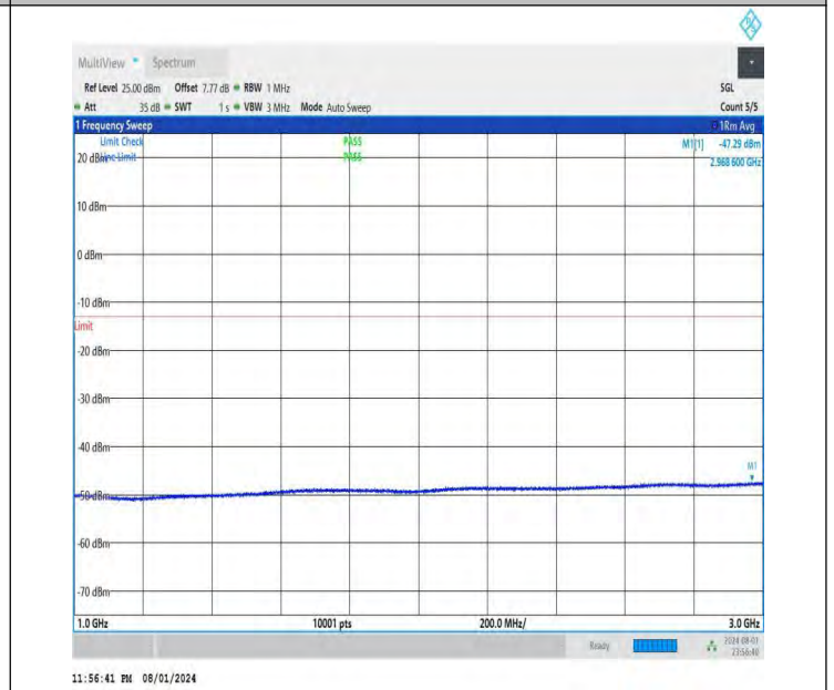
NTNV-DC_26A-n78A(3700-3800)-PC3-30-5+70-M+H-QPSK-IDLE -DFT-BPSK-Edge_1RB_Left-1000-3000-PASS
