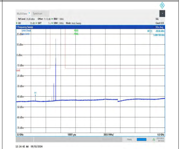
NTNV-DC_26A-n78A(3700-3800)-PC3-30-5+80-M+H-QPSK-IDLE -DFT-BPSK-Edge_1RB_Right-3000-6000-PASS
