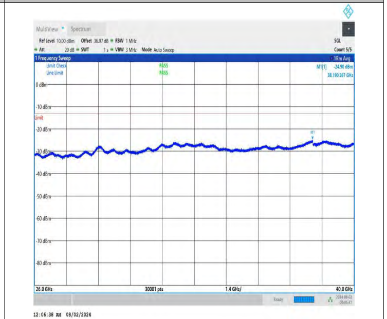
NTNV-DC_26A-n78A(3700-3800)-PC3-30-5+80-M+L-QPSK-IDLE -DFT-QPSK-Edge_1RB_Right-26000-40000-PASS
