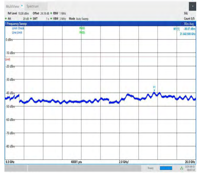
NTNV-DC_26A-n78A(3700-3800)-PC3-30-5+80-M+M-QPSK-IDLE -DFT-BPSK-Edge_1RB_Left-6000-26000-PASS
