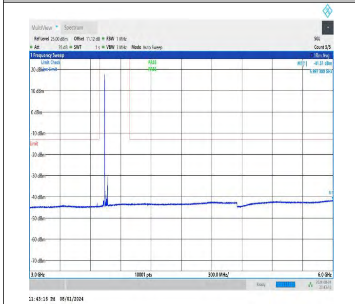
NTNV-DC_26A-n78A(3700-3800)-PC3-30-5+60-M+H-QPSK-IDL E-DFT-QPSK-Edge_1RB_Left-3000-6000-PASS
