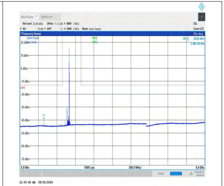
NTNV-DC_26A-n78A(3700-3800)-PC3-30-5+70-M+H-QPSK-IDLE -DFT-QPSK-Edge_1RB_Right-3000-6000-PASS
