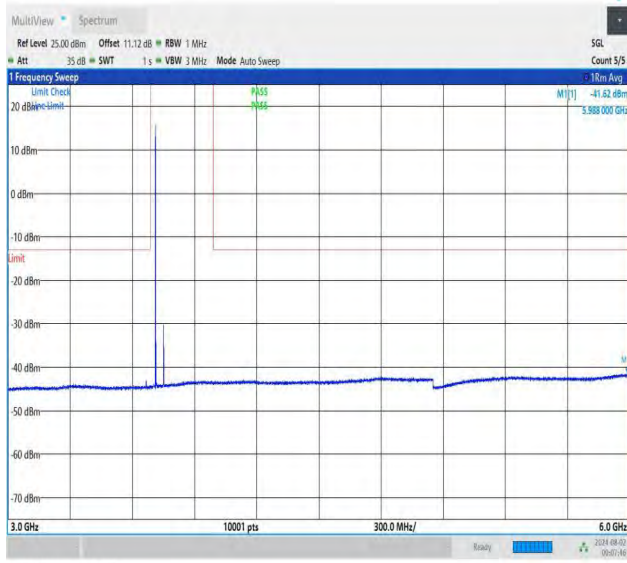
NTNV-DC_26A-n78A(3700-3800)-PC3-30-5+80-M+M-QPSK-IDL E-DFT-BPSK-Edge_1RB_Left-3000-6000-PASS
