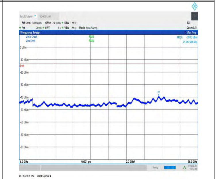
NTNV-DC_26A-n78A(3700-3800)-PC3-30-5+70-M+M-QPSK-IDLE -DFT-QPSK-Edge_1RB_Left-6000-26000-PASS
