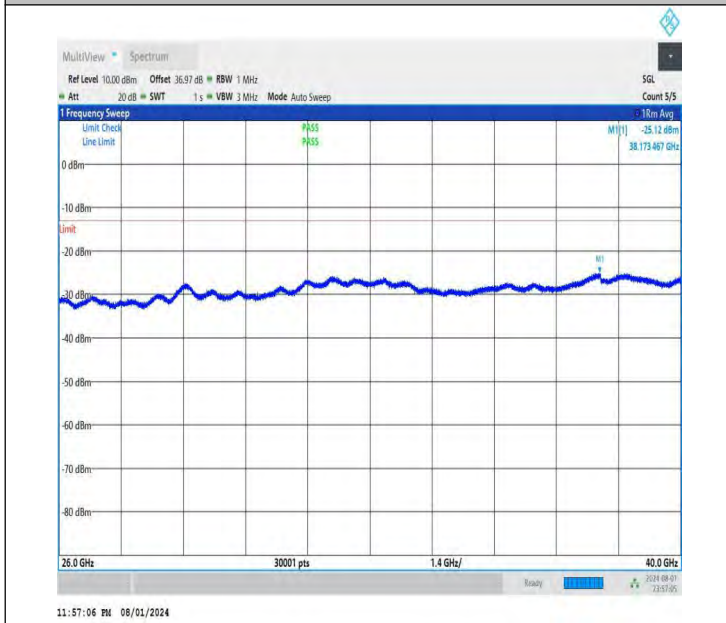
NTNV-DC_26A-n78A(3700-3800)-PC3-30-5+70-M+H-QPSK-IDL E-DFT-BPSK-Edge_1RB_Left-26000-40000-PASS
