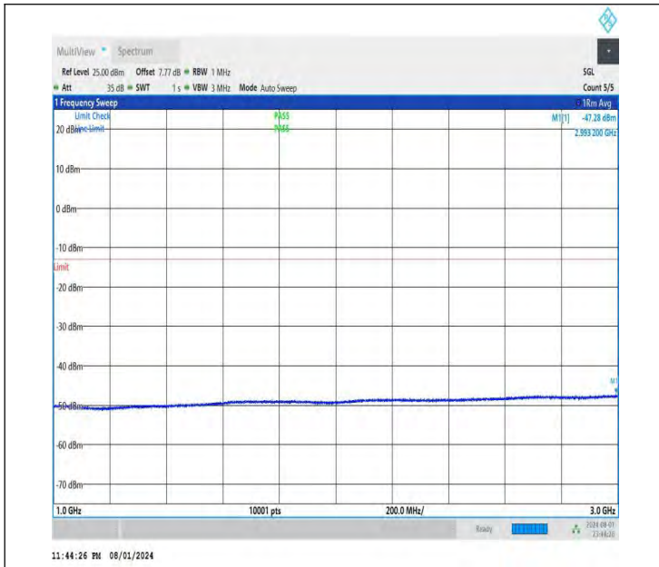
NTNV-DC_26A-n78A(3700-3800)-PC3-30-5+60-M+H-QPSK-IDL E-DFT-QPSK-Edge_1RB_Right-1000-3000-PASS
