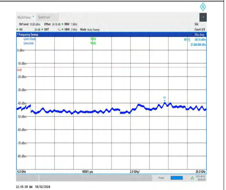
NTNV-DC_26A-n78A(3700-3800)-PC3-30-5+80-M+L-QPSK-IDLE -DFT-QPSK-Edge_1RB_Left-6000-26000-PASS
