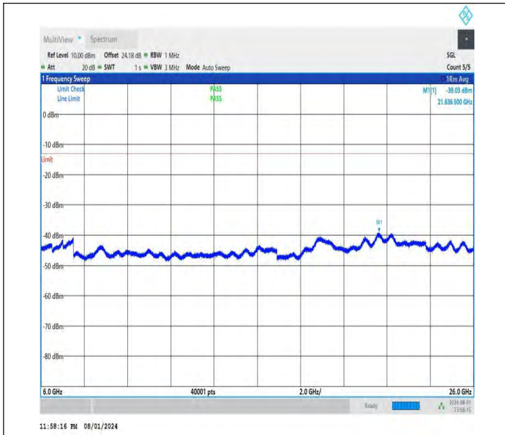
NTNV-DC_26A-n78A(3700-3800)-PC3-30-5+70-M+H-QPSK-IDL E-DFT-BPSK-Edge_1RB_Right-6000-26000-PASS
