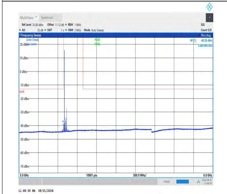
NTNV-DC_26A-n78A(3700-3800)-PC3-30-5+70-M+L-QPSK-IDL E-DFT-QPSK-Edge_1RB_Left-3000-6000-PASS
