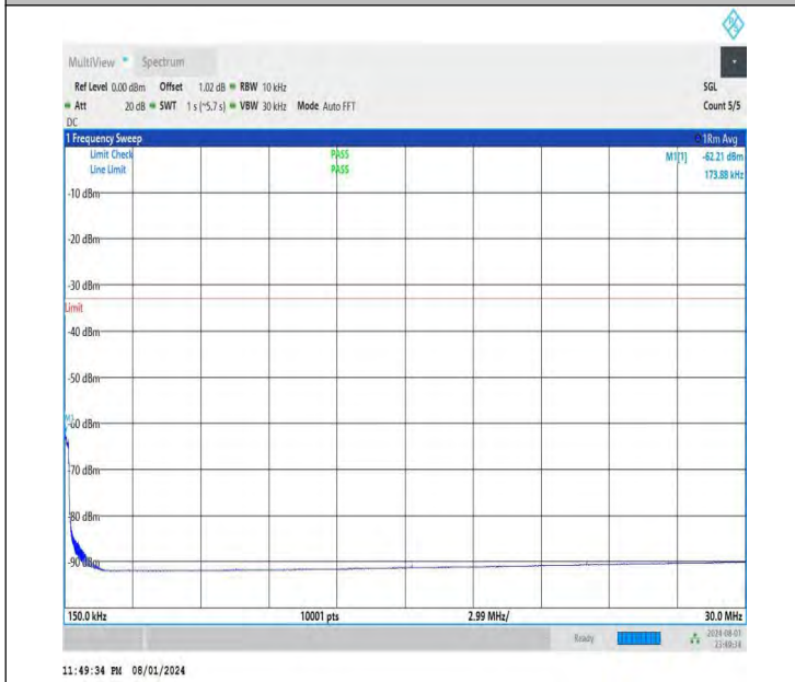
NTNV-DC_26A-n78A(3700-3800)-PC3-30-5+70-M+L-QPSK-IDL E-DFT-QPSK-Edge_1RB_Right-0.15-30-PASS
