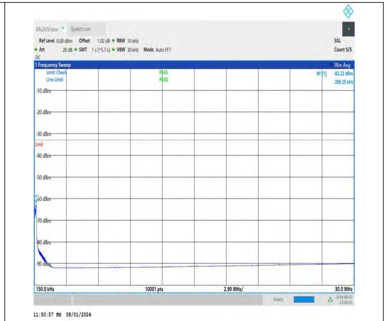
NTNV-DC_26A-n78A(3700-3800)-PC3-30-5+70-M+M-QPSK-IDLE -DFT-BPSK-Edge_1RB_Left-0.15-30-PASS
