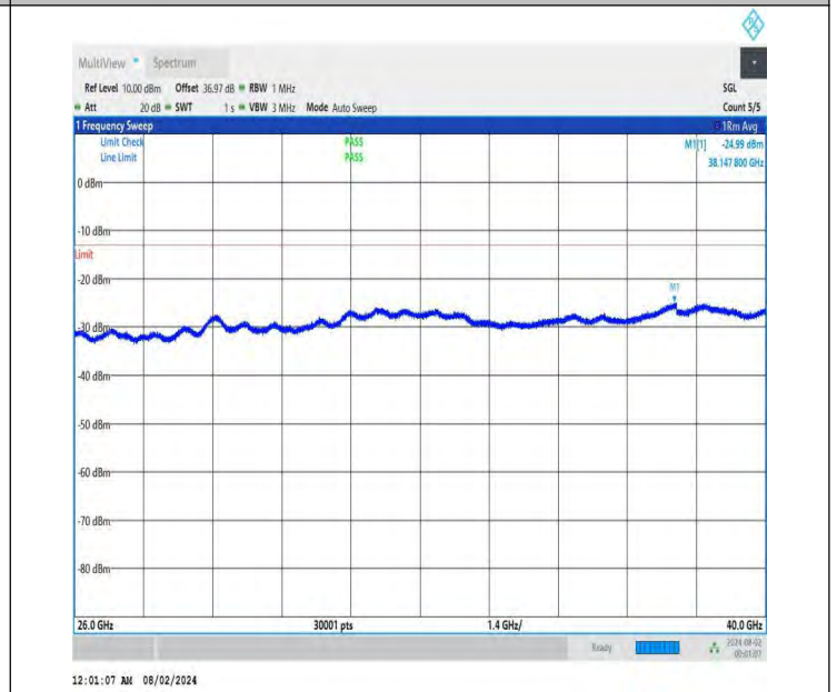
NTNV-DC_26A-n78A(3700-3800)-PC3-30-5+70-M+H-QPSK-IDLE -DFT-QPSK-Edge_1RB_Right-26000-40000-PASS
