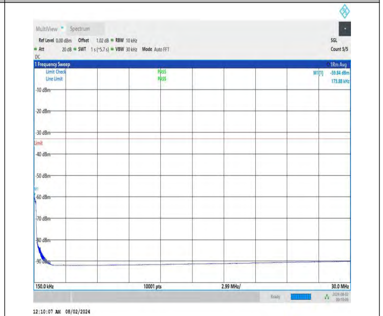
NTNV-DC_26A-n78A(3700-3800)-PC3-30-5+80-M+M-QPSK-IDLE -DFT-QPSK-Edge_1RB_Left-0.15-30-PASS
