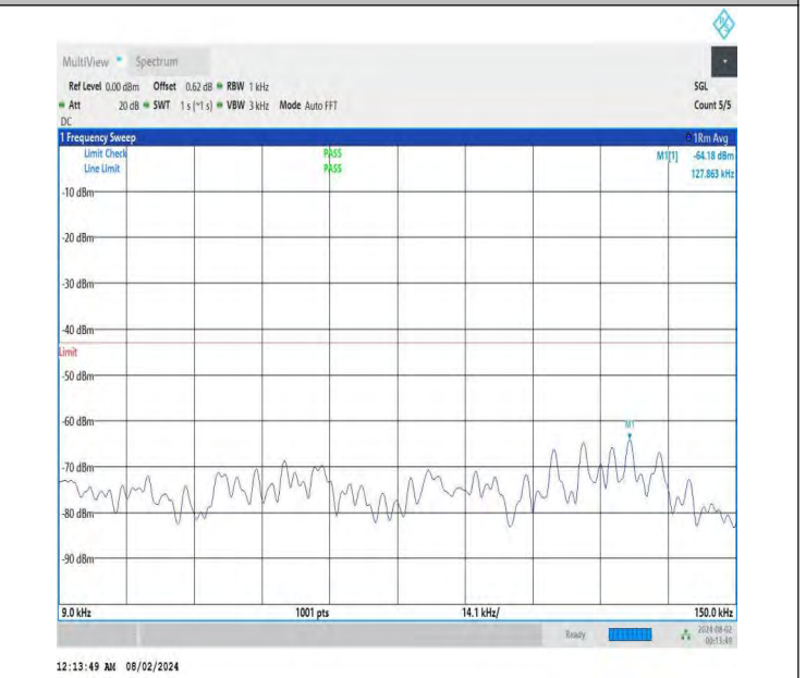
NTNV-DC_26A-n78A(3700-3800)-PC3-30-5+80-M+H-QPSK-IDLE -DFT-BPSK-Edge_1RB_Right-0.009-0.15-PASS
