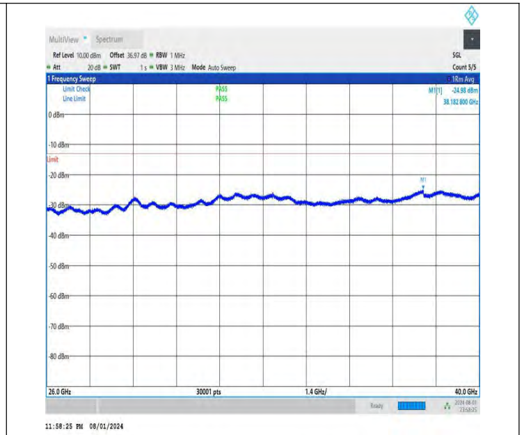
NTNV-DC_26A-n78A(3700-3800)-PC3-30-5+70-M+H-QPSK-IDLE -DFT-BPSK-Edge_1RB_Right-26000-40000-PASS
