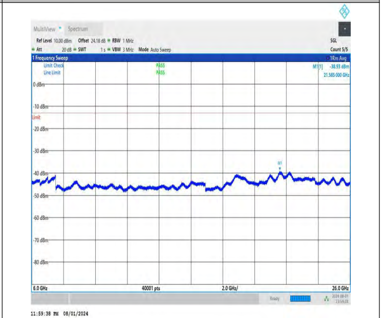
NTNV-DC_26A-n78A(3700-3800)-PC3-30-5+70-M+H-QPSK-IDLE -DFT-QPSK-Edge_1RB_Left-6000-26000-PASS
