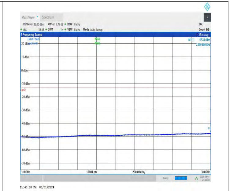
NTNV-DC_26A-n78A(3700-3800)-PC3-30-5+60-M+H-QPSK-IDLE -DFT-QPSK-Edge_1RB_Left-1000-3000-PASS
