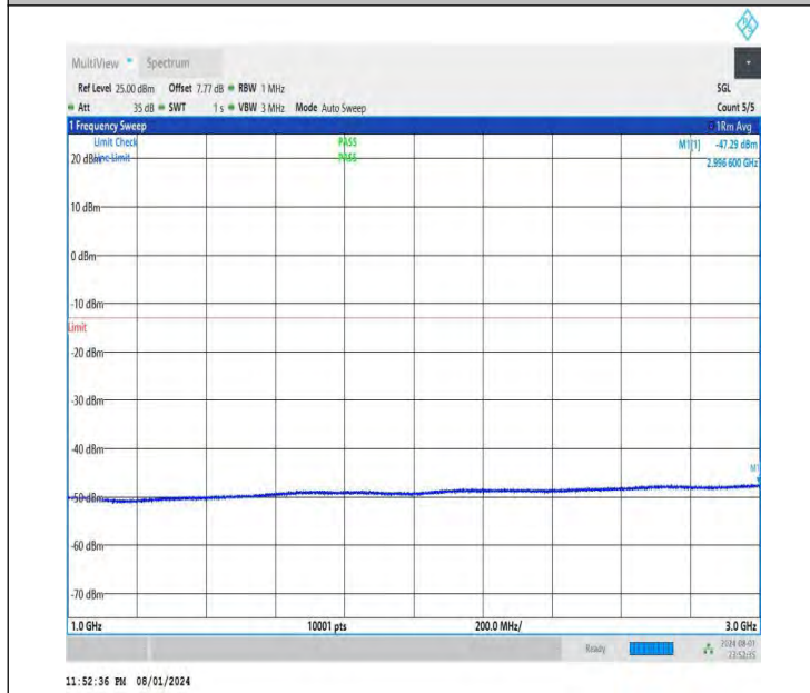
NTNV-DC_26A-n78A(3700-3800)-PC3-30-5+70-M+M-QPSK-IDL E-DFT-BPSK-Edge_1RB_Right-1000-3000-PASS
