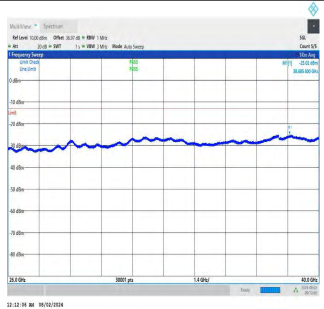
NTNV-DC_26A-n78A(3700-3800)-PC3-30-5+80-M+M-QPSK-IDLE -DFT-QPSK-Edge_1RB_Right-26000-40000-PASS
