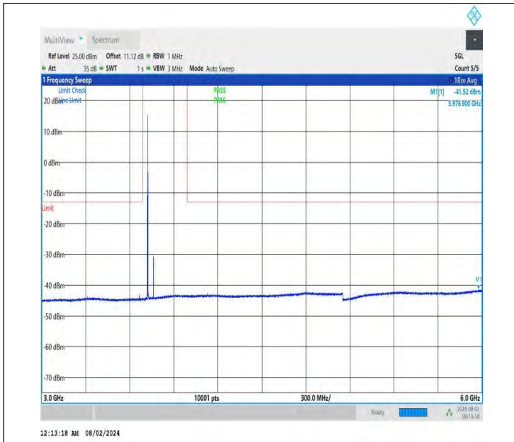
NTNV-DC_26A-n78A(3700-3800)-PC3-30-5+80-M+H-QPSK-IDL E-DFT-BPSK-Edge_1RB_Left-3000-6000-PASS
