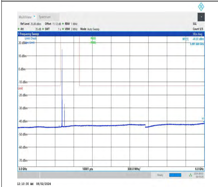
NTNV-DC_26A-n78A(3700-3800)-PC3-30-5+80-M+M-QPSK-IDL E-DFT-QPSK-Edge_1RB_Left-3000-6000-PASS
