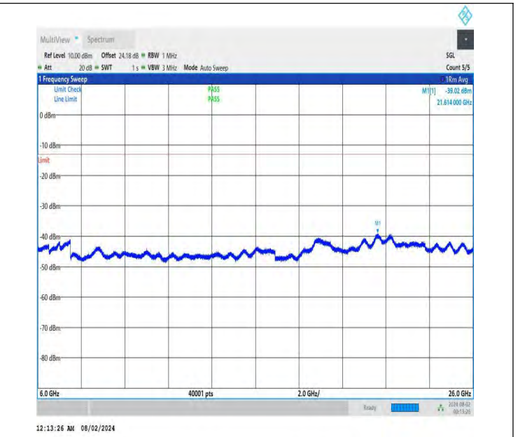
NTNV-DC_26A-n78A(3700-3800)-PC3-30-5+80-M+H-QPSK-IDLE -DFT-BPSK-Edge_1RB_Left-6000-26000-PASS
