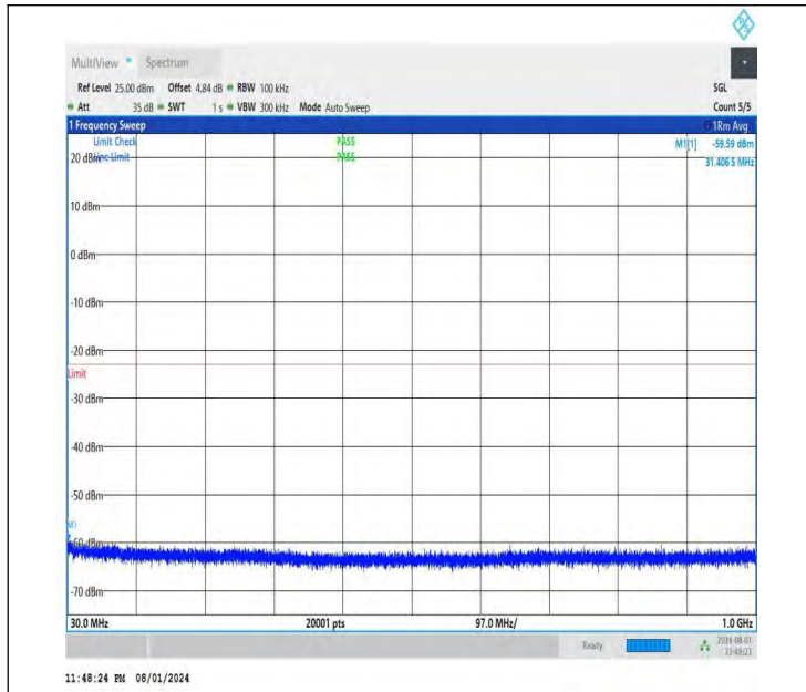
NTNV-DC_26A-n78A(3700-3800)-PC3-30-5+70-M+L-QPSK-IDL E-DFT-QPSK-Edge_1RB_Left-30-1000-PASS
