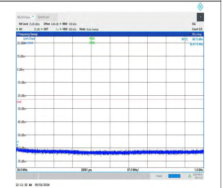
NTNV-DC_26A-n78A(3700-3800)-PC3-30-5+80-M+M-QPSK-IDLE -DFT-QPSK-Edge_1RB_Right-30-1000-PASS
