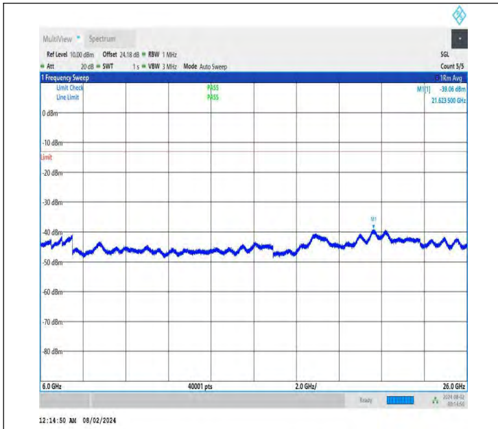
NTNV-DC_26A-n78A(3700-3800)-PC3-30-5+80-M+H-QPSK-IDL E-DFT-BPSK-Edge_1RB_Right-6000-26000-PASS
