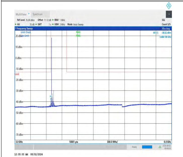
NTNV-DC_26A-n78A(3700-3800)-PC3-30-5+80-M+L-QPSK-IDL E-DFT-QPSK-Edge_1RB_Left-3000-6000-PASS
