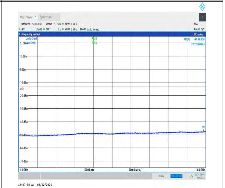
NTNV-DC_26A-n78A(3700-3800)-PC3-30-5+80-M+M-QPSK-IDLE -DFT-BPSK-Edge_1RB_Left-1000-3000-PASS
