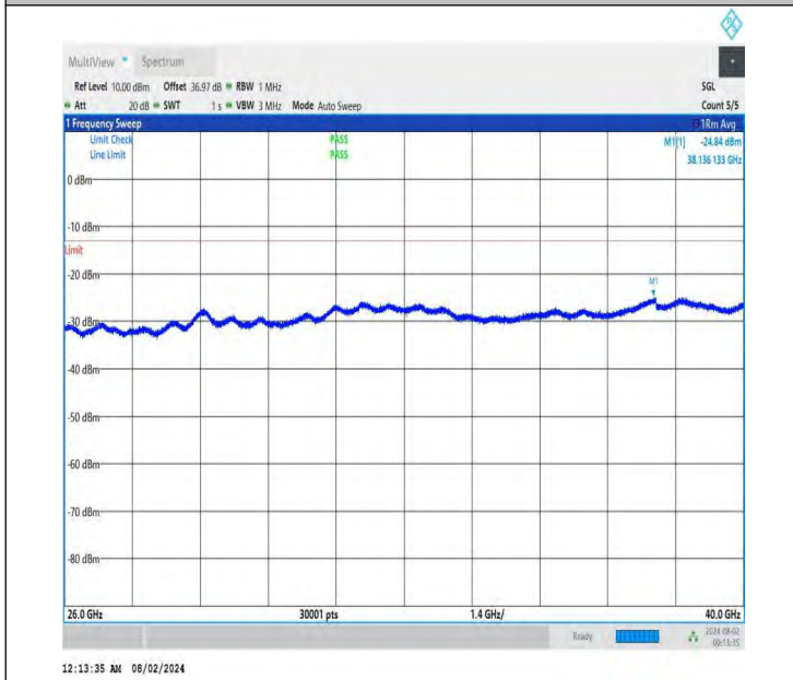
NTNV-DC_26A-n78A(3700-3800)-PC3-30-5+80-M+H-QPSK-IDL E-DFT-BPSK-Edge_1RB_Left-26000-40000-PASS
