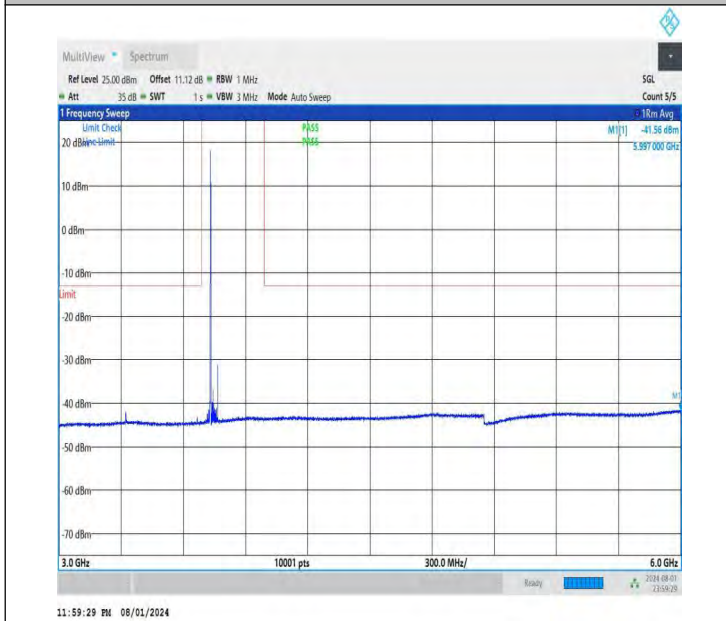
NTNV-DC_26A-n78A(3700-3800)-PC3-30-5+70-M+H-QPSK-IDL E-DFT-QPSK-Edge_1RB_Left-3000-6000-PASS
