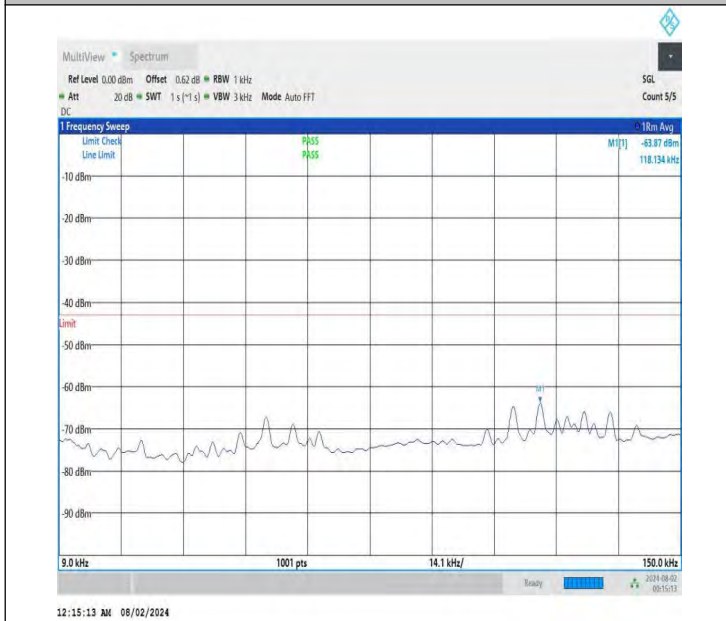
NTNV-DC_26A-n78A(3700-3800)-PC3-30-5+80-M+H-QPSK-IDL E-DFT-QPSK-Edge_1RB_Left-0.009-0.15-PASS
