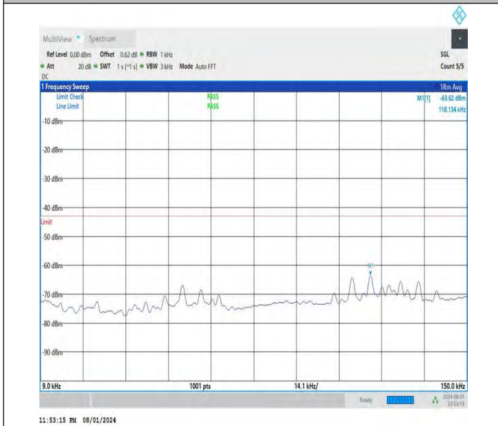
NTNV-DC_26A-n78A(3700-3800)-PC3-30-5+70-M+M-QPSK-IDL E-DFT-QPSK-Edge_1RB_Left-0.009-0.15-PASS
