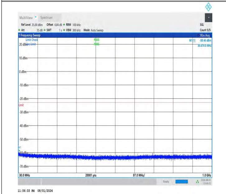
NTNV-DC_26A-n78A(3700-3800)-PC3-30-5+70-M+H-QPSK-IDL E-DFT-BPSK-Edge_1RB_Left-30-1000-PASS
