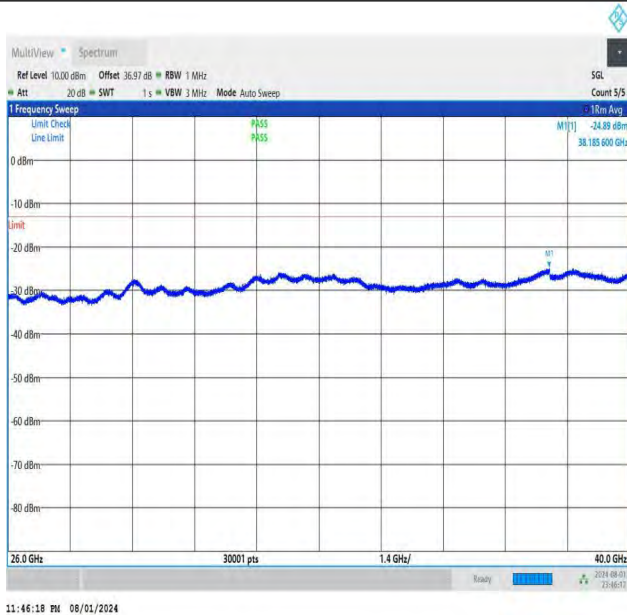
NTNV-DC_26A-n78A(3700-3800)-PC3-30-5+70-M+L-QPSK-IDL E-DFT-BPSK-Edge_1RB_Left-26000-40000-PASS
