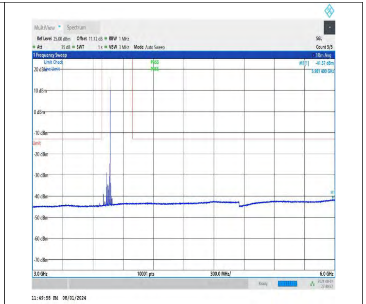
NTNV-DC_26A-n78A(3700-3800)-PC3-30-5+70-M+L-QPSK-IDLE -DFT-QPSK-Edge_1RB_Right-3000-6000-PASS
