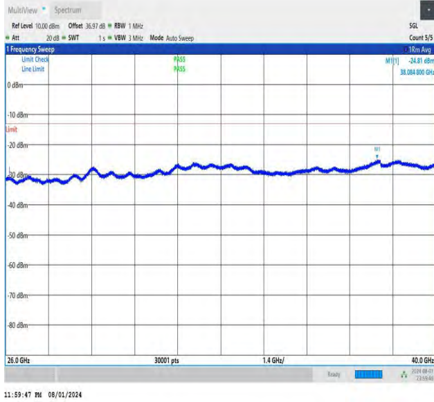
NTNV-DC_26A-n78A(3700-3800)-PC3-30-5+70-M+H-QPSK-IDL E-DFT-QPSK-Edge_1RB_Left-26000-40000-PASS
