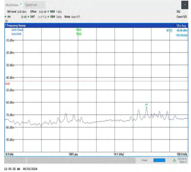
NTNV-DC_26A-n78A(3700-3800)-PC3-30-5+80-M+L-QPSK-IDLE -DFT-QPSK-Edge_1RB_Right-0.009-0.15-PASS
