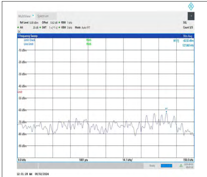
NTNV-DC_26A-n78A(3700-3800)-PC3-30-5+80-M+L-QPSK-IDL E-DFT-BPSK-Edge_1RB_Left-0.009-0.15-PASS
