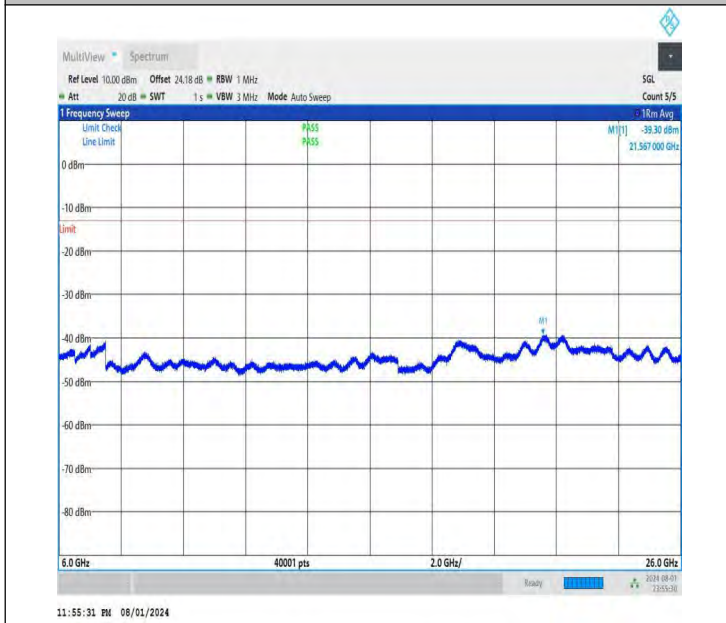
NTNV-DC_26A-n78A(3700-3800)-PC3-30-5+70-M+M-QPSK-IDL E-DFT-QPSK-Edge_1RB_Right-6000-26000-PASS
