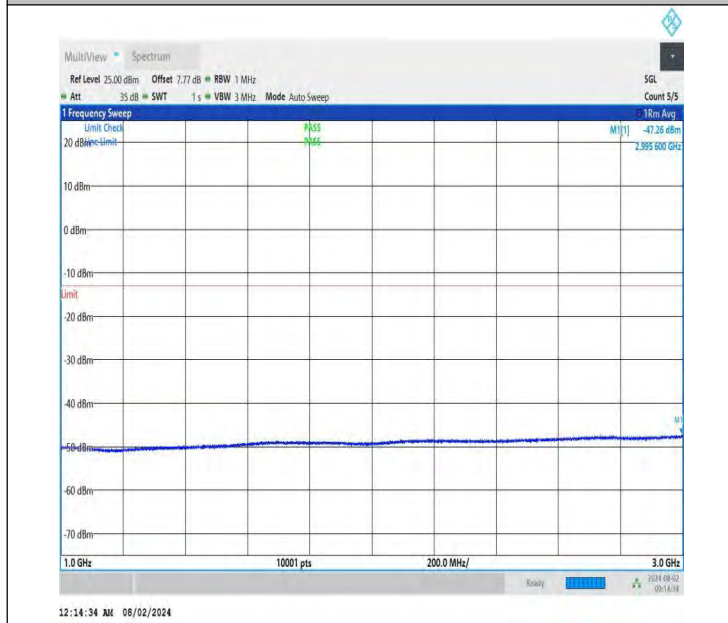
NTNV-DC_26A-n78A(3700-3800)-PC3-30-5+80-M+H-QPSK-IDL E-DFT-BPSK-Edge_1RB_Right-1000-3000-PASS
