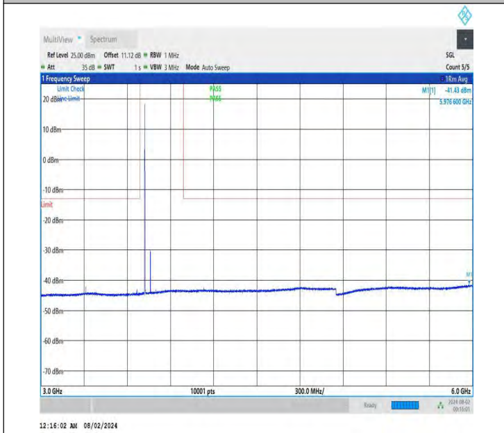
NTNV-DC_26A-n78A(3700-3800)-PC3-30-5+80-M+H-QPSK-IDL E-DFT-QPSK-Edge_1RB_Left-3000-6000-PASS
