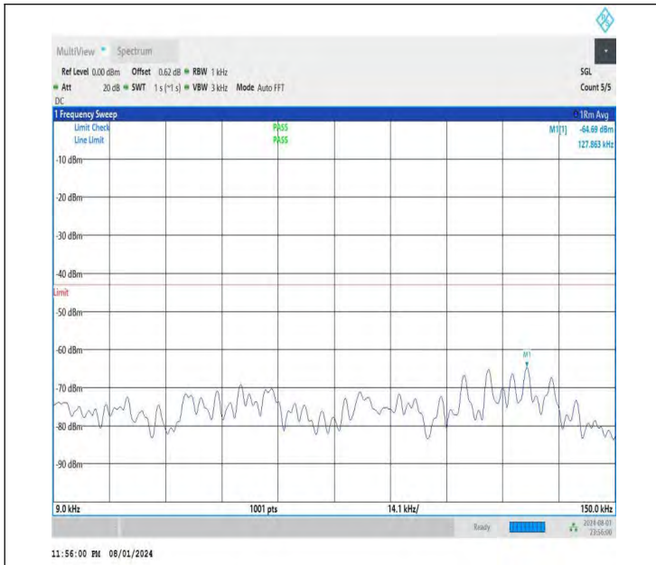
NTNV-DC_26A-n78A(3700-3800)-PC3-30-5+70-M+H-QPSK-IDL E-DFT-BPSK-Edge_1RB_Left-0.009-0.15-PASS
