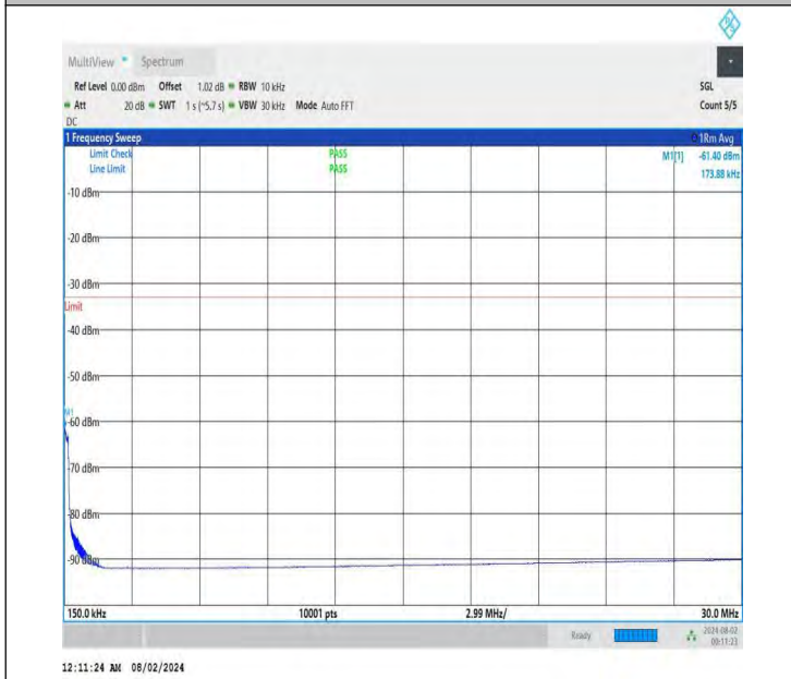
NTNV-DC_26A-n78A(3700-3800)-PC3-30-5+80-M+M-QPSK-IDL E-DFT-QPSK-Edge_1RB_Right-0.15-30-PASS
