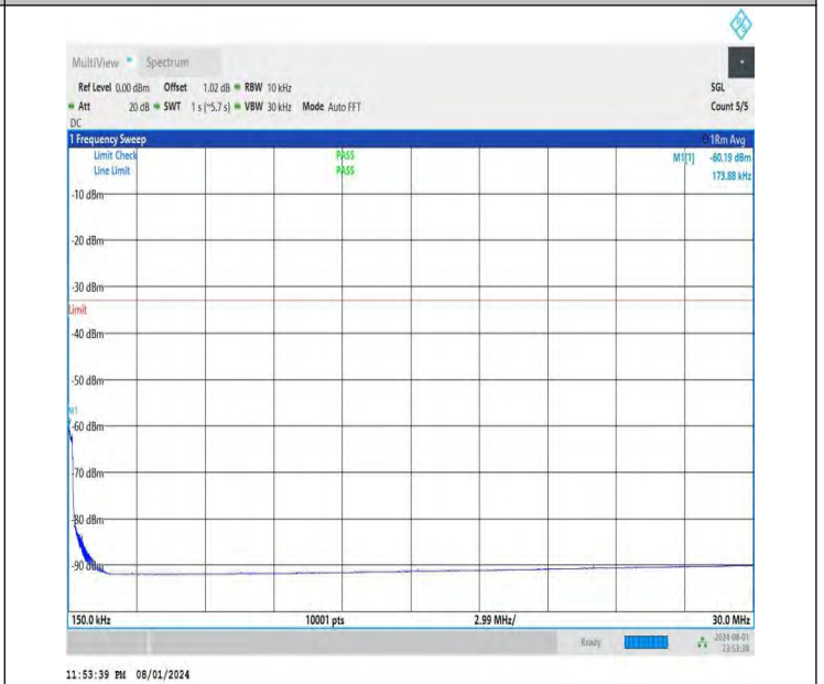
NTNV-DC_26A-n78A(3700-3800)-PC3-30-5+70-M+M-QPSK-IDLE -DFT-QPSK-Edge_1RB_Left-0.15-30-PASS
