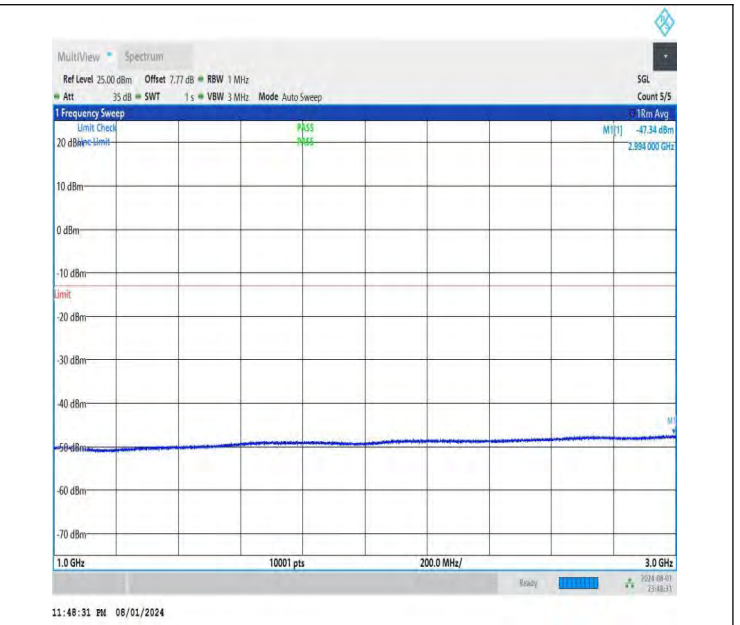
NTNV-DC_26A-n78A(3700-3800)-PC3-30-5+70-M+L-QPSK-IDLE -DFT-QPSK-Edge_1RB_Left-1000-3000-PASS
