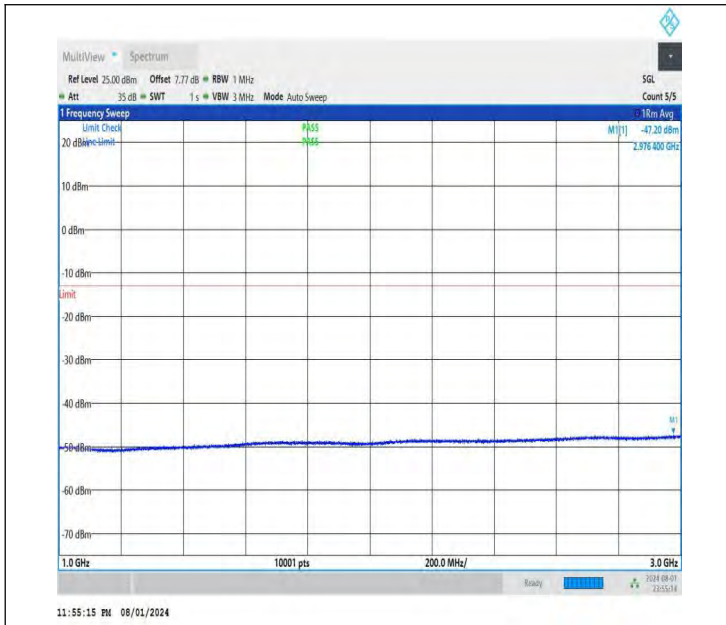
NTNV-DC_26A-n78A(3700-3800)-PC3-30-5+70-M+M-QPSK-IDL E-DFT-QPSK-Edge_1RB_Right-1000-3000-PASS
