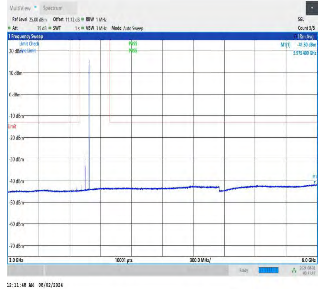
NTNV-DC_26A-n78A(3700-3800)-PC3-30-5+80-M+M-QPSK-IDLE -DFT-QPSK-Edge_1RB_Right-3000-6000-PASS
