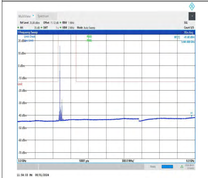
NTNV-DC_26A-n78A(3700-3800)-PC3-30-5+70-M+M-QPSK-IDL E-DFT-QPSK-Edge_1RB_Left-3000-6000-PASS
