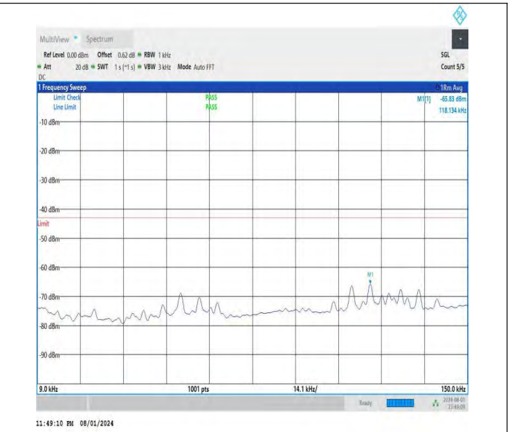
NTNV-DC_26A-n78A(3700-3800)-PC3-30-5+70-M+L-QPSK-IDLE -DFT-QPSK-Edge_1RB_Right-0.009-0.15-PASS
