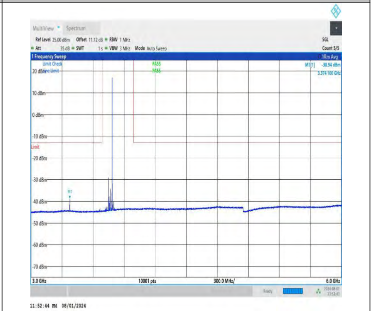
NTNV-DC_26A-n78A(3700-3800)-PC3-30-5+70-M+M-QPSK-IDLE -DFT-BPSK-Edge_1RB_Right-3000-6000-PASS
