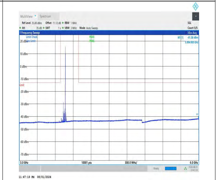
NTNV-DC_26A-n78A(3700-3800)-PC3-30-5+70-M+L-QPSK-IDLE -DFT-BPSK-Edge_1RB_Right-3000-6000-PASS
