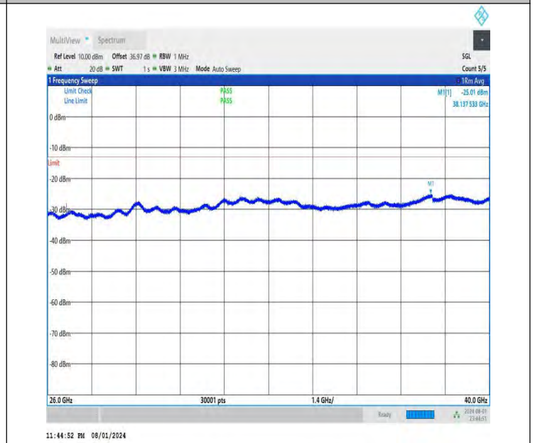
NTNV-DC_26A-n78A(3700-3800)-PC3-30-5+60-M+H-QPSK-IDLE -DFT-QPSK-Edge_1RB_Right-26000-40000-PASS
