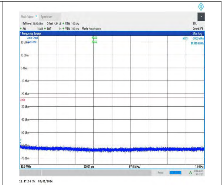
NTNV-DC_26A-n78A(3700-3800)-PC3-30-5+70-M+L-QPSK-IDLE -DFT-BPSK-Edge_1RB_Right-30-1000-PASS
