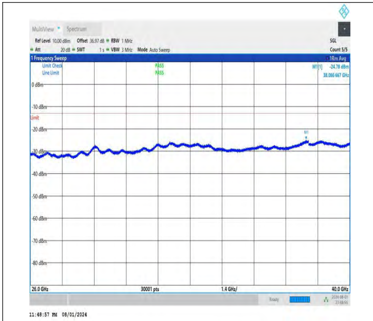
NTNV-DC_26A-n78A(3700-3800)-PC3-30-5+70-M+L-QPSK-IDL E-DFT-QPSK-Edge_1RB_Left-26000-40000-PASS
