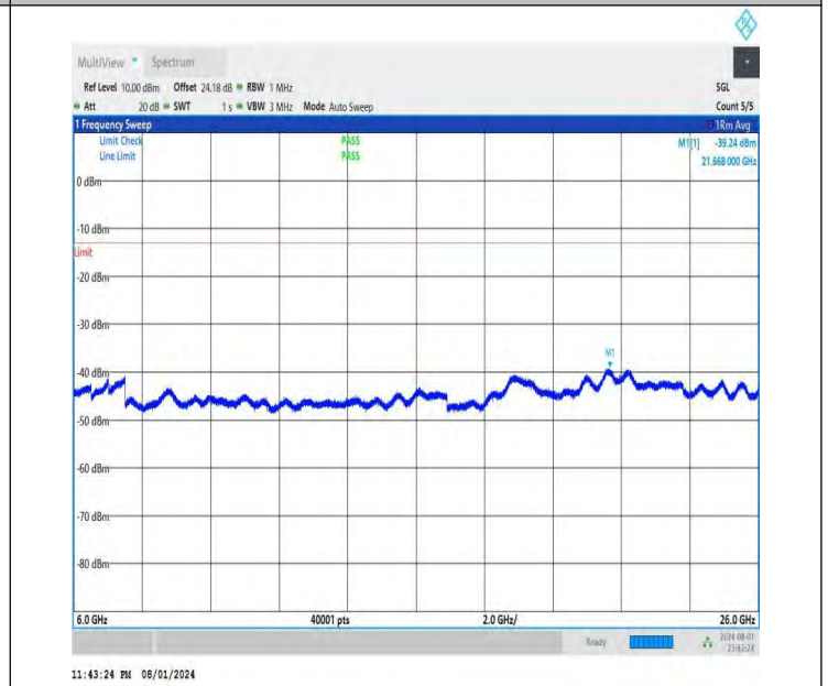
NTNV-DC_26A-n78A(3700-3800)-PC3-30-5+60-M+H-QPSK-IDLE -DFT-QPSK-Edge_1RB_Left-6000-26000-PASS
