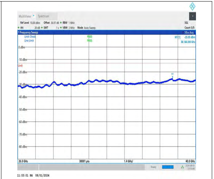
NTNV-DC_26A-n78A(3700-3800)-PC3-30-5+70-M+M-QPSK-IDLE -DFT-BPSK-Edge_1RB_Right-26000-40000-PASS
