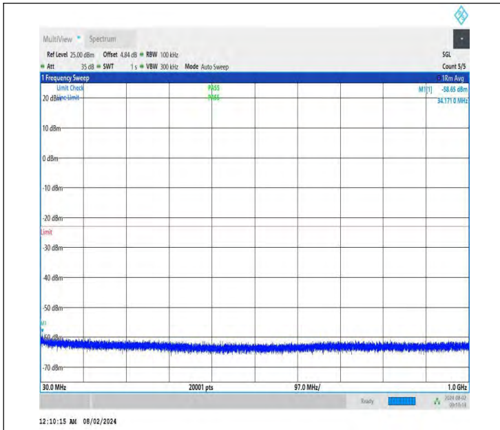
NTNV-DC_26A-n78A(3700-3800)-PC3-30-5+80-M+M-QPSK-IDL E-DFT-QPSK-Edge_1RB_Left-30-1000-PASS
