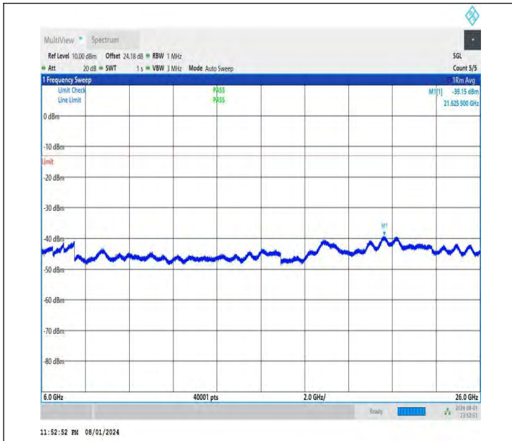
NTNV-DC_26A-n78A(3700-3800)-PC3-30-5+70-M+M-QPSK-IDL E-DFT-BPSK-Edge_1RB_Right-6000-26000-PASS
