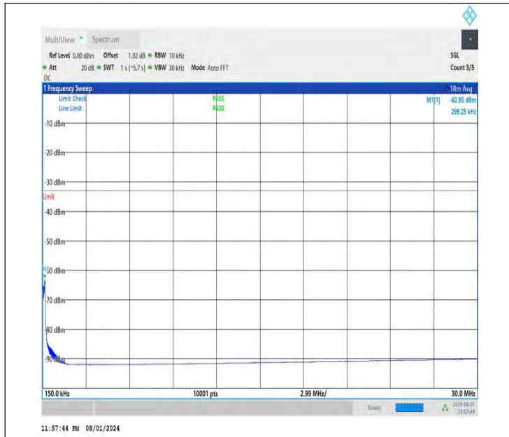
NTNV-DC_26A-n78A(3700-3800)-PC3-30-5+70-M+H-QPSK-IDL E-DFT-BPSK-Edge_1RB_Right-0.15-30-PASS
