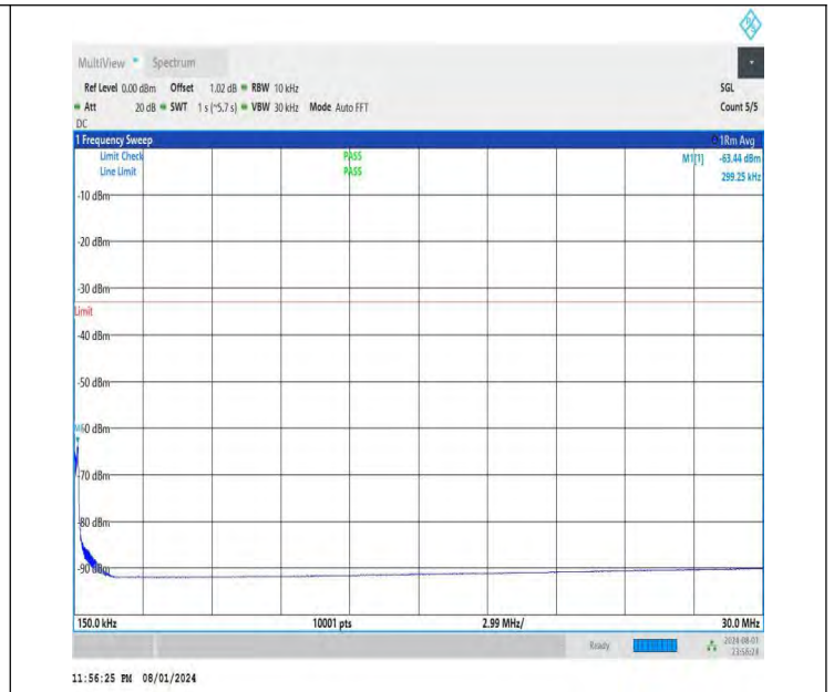
NTNV-DC_26A-n78A(3700-3800)-PC3-30-5+70-M+H-QPSK-IDLE -DFT-BPSK-Edge_1RB_Left-0.15-30-PASS
