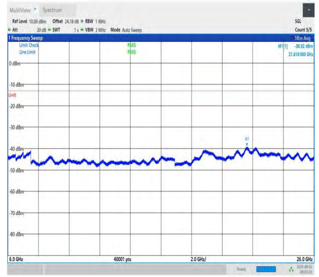
NTNV-DC_26A-n78A(3700-3800)-PC3-30-5+80-M+L-QPSK-IDLE -DFT-BPSK-Edge_1RB_Left-6000-26000-PASS
