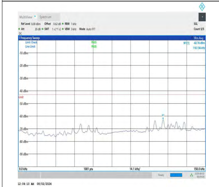
NTNV-DC_26A-n78A(3700-3800)-PC3-30-5+80-M+L-QPSK-IDL E-DFT-QPSK-Edge_1RB_Left-0.009-0.15-PASS
