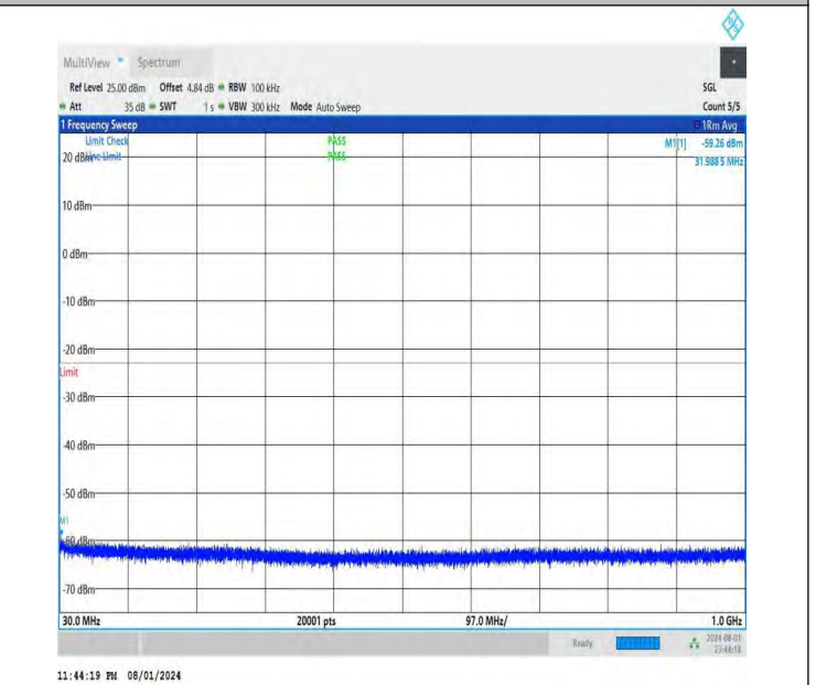
NTNV-DC_26A-n78A(3700-3800)-PC3-30-5+60-M+H-QPSK-IDLE -DFT-QPSK-Edge_1RB_Right-30-1000-PASS
