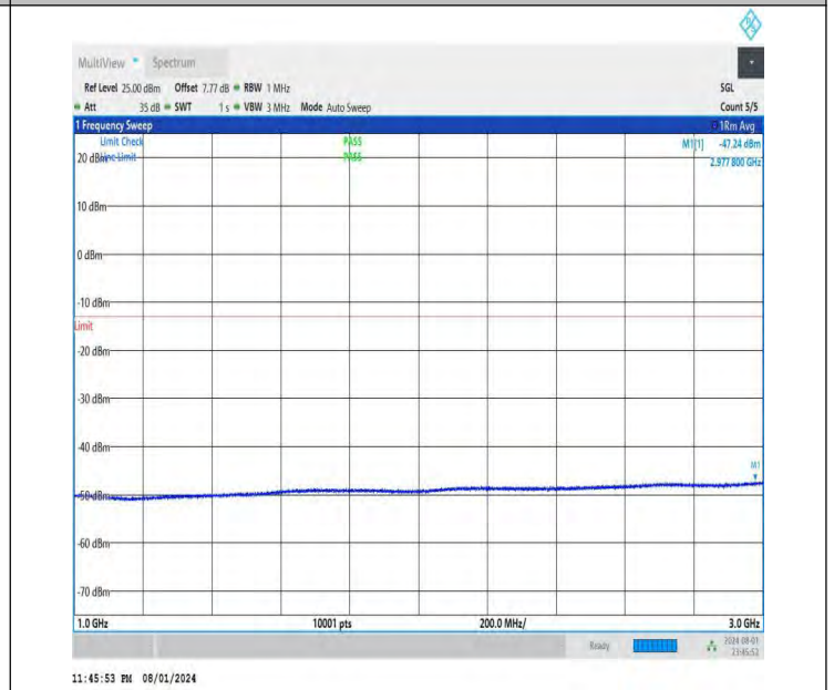
NTNV-DC_26A-n78A(3700-3800)-PC3-30-5+70-M+L-QPSK-IDLE -DFT-BPSK-Edge_1RB_Left-1000-3000-PASS
