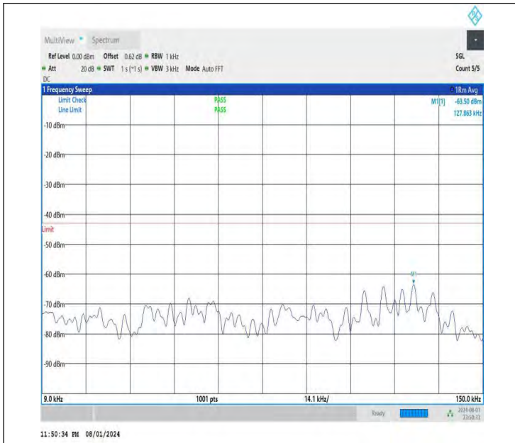
NTNV-DC_26A-n78A(3700-3800)-PC3-30-5+70-M+M-QPSK-IDL E-DFT-BPSK-Edge_1RB_Left-0.009-0.15-PASS
