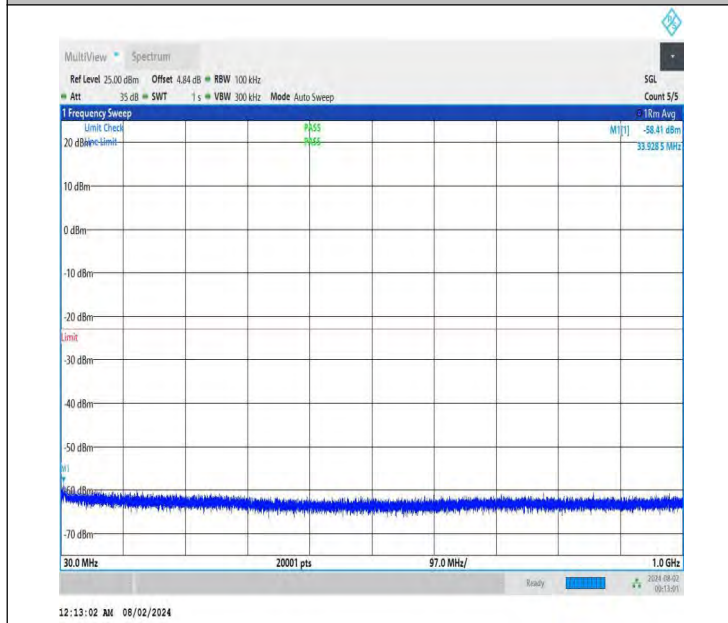
NTNV-DC_26A-n78A(3700-3800)-PC3-30-5+80-M+H-QPSK-IDL E-DFT-BPSK-Edge_1RB_Left-30-1000-PASS
