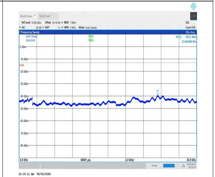
NTNV-DC_26A-n78A(3700-3800)-PC3-30-5+80-M+H-QPSK-IDLE -DFT-QPSK-Edge_1RB_Left-6000-26000-PASS
