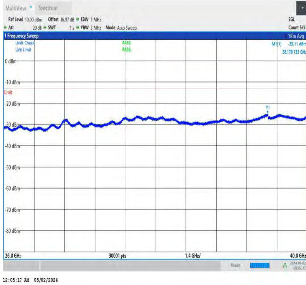
NTNV-DC_26A-n78A(3700-3800)-PC3-30-5+80-M+L-QPSK-IDL E-DFT-QPSK-Edge_1RB_Left-26000-40000-PASS
