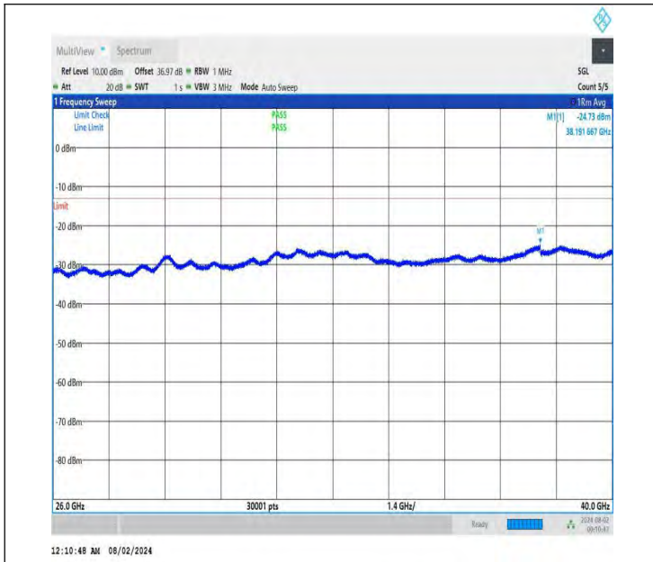
NTNV-DC_26A-n78A(3700-3800)-PC3-30-5+80-M+M-QPSK-IDL E-DFT-QPSK-Edge_1RB_Left-26000-40000-PASS
