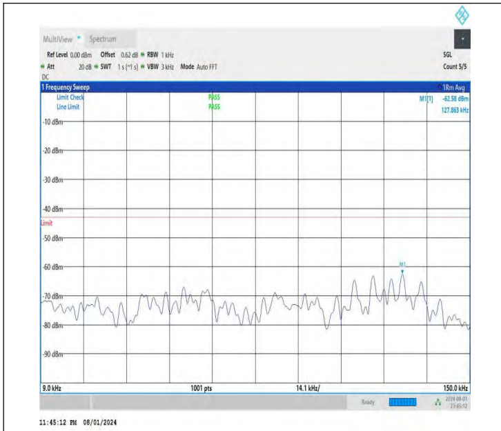
NTNV-DC_26A-n78A(3700-3800)-PC3-30-5+70-M+L-QPSK-IDL E-DFT-BPSK-Edge_1RB_Left-0.009-0.15-PASS
