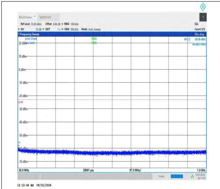
NTNV-DC_26A-n78A(3700-3800)-PC3-30-5+80-M+H-QPSK-IDL E-DFT-QPSK-Edge_1RB_Left-30-1000-PASS
