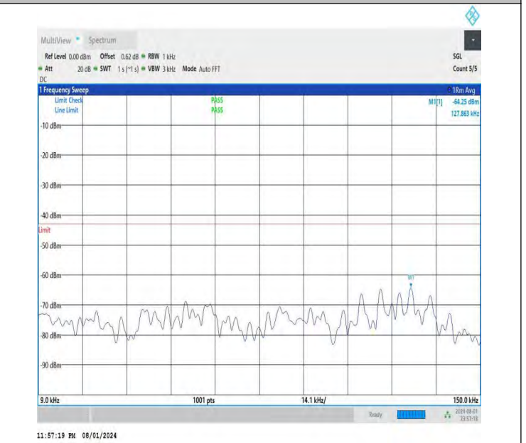
NTNV-DC_26A-n78A(3700-3800)-PC3-30-5+70-M+H-QPSK-IDLE -DFT-BPSK-Edge_1RB_Right-0.009-0.15-PASS
