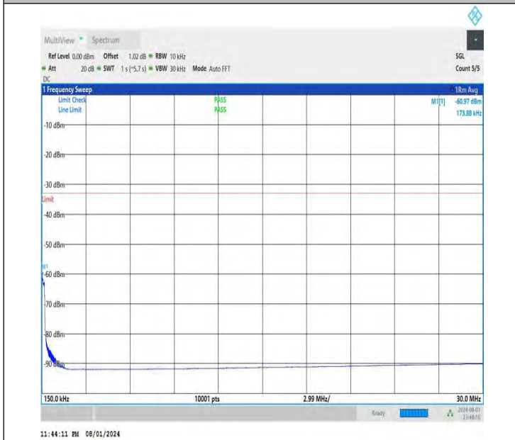
NTNV-DC_26A-n78A(3700-3800)-PC3-30-5+60-M+H-QPSK-IDL E-DFT-QPSK-Edge_1RB_Right-0.15-30-PASS
