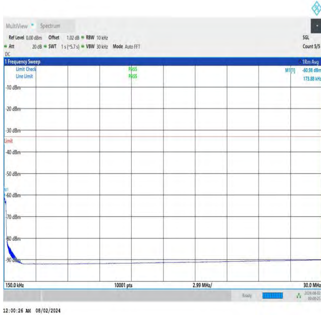
NTNV-DC_26A-n78A(3700-3800)-PC3-30-5+70-M+H-QPSK-IDL E-DFT-QPSK-Edge_1RB_Right-0.15-30-PASS
