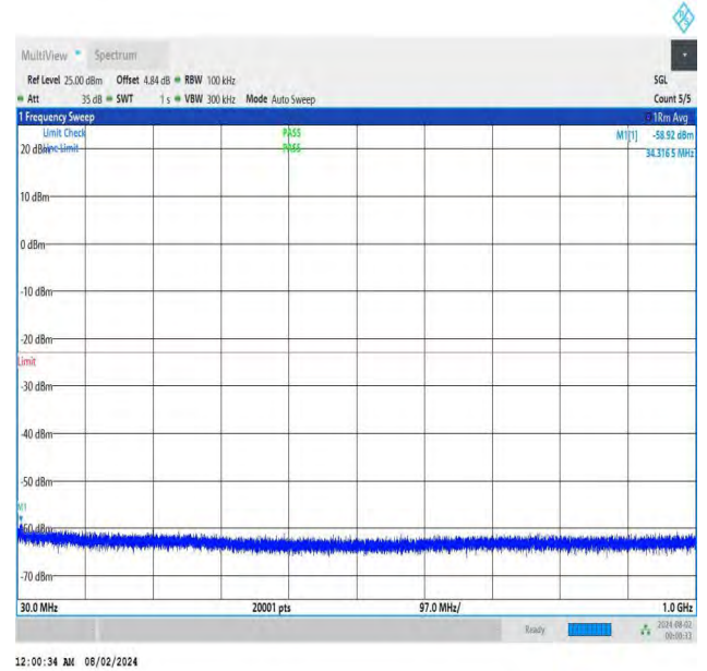
NTNV-DC_26A-n78A(3700-3800)-PC3-30-5+70-M+H-QPSK-IDLE -DFT-QPSK-Edge_1RB_Right-30-1000-PASS
