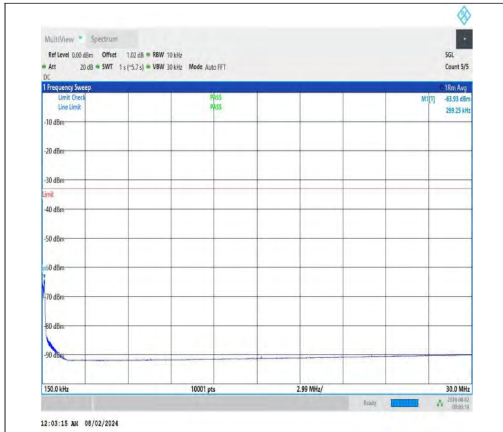
NTNV-DC_26A-n78A(3700-3800)-PC3-30-5+80-M+L-QPSK-IDL E-DFT-BPSK-Edge_1RB_Right-0.15-30-PASS
