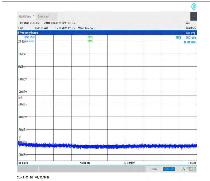
NTNV-DC_26A-n78A(3700-3800)-PC3-30-5+60-M+H-QPSK-IDL E-DFT-QPSK-Edge_1RB_Left-30-1000-PASS
