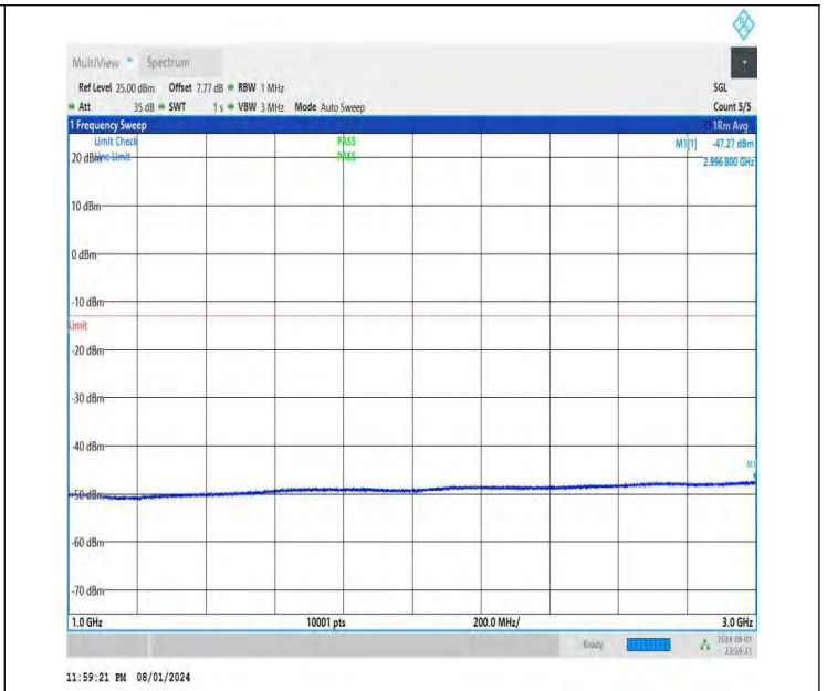
NTNV-DC_26A-n78A(3700-3800)-PC3-30-5+70-M+H-QPSK-IDLE -DFT-QPSK-Edge_1RB_Left-1000-3000-PASS
