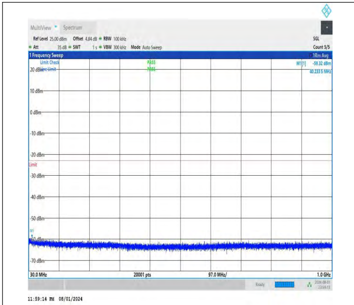
NTNV-DC_26A-n78A(3700-3800)-PC3-30-5+70-M+H-QPSK-IDL E-DFT-QPSK-Edge_1RB_Left-30-1000-PASS
