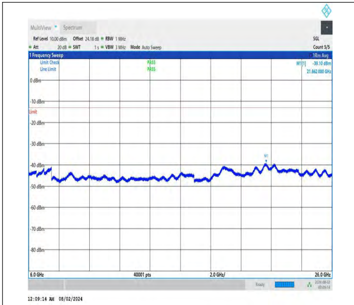
NTNV-DC_26A-n78A(3700-3800)-PC3-30-5+80-M+M-QPSK-IDL E-DFT-BPSK-Edge_1RB_Right-6000-26000-PASS
