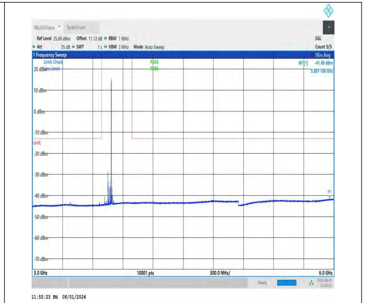
NTNV-DC_26A-n78A(3700-3800)-PC3-30-5+70-M+M-QPSK-IDLE -DFT-QPSK-Edge_1RB_Right-3000-6000-PASS
