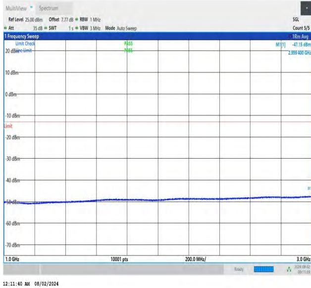
NTNV-DC_26A-n78A(3700-3800)-PC3-30-5+80-M+M-QPSK-IDL E-DFT-QPSK-Edge_1RB_Right-1000-3000-PASS
