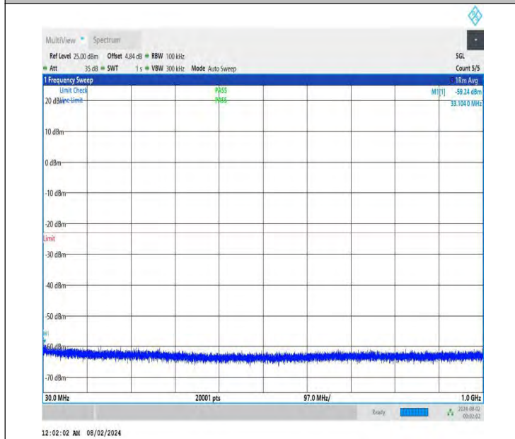
NTNV-DC_26A-n78A(3700-3800)-PC3-30-5+80-M+L-QPSK-IDL E-DFT-BPSK-Edge_1RB_Left-30-1000-PASS
