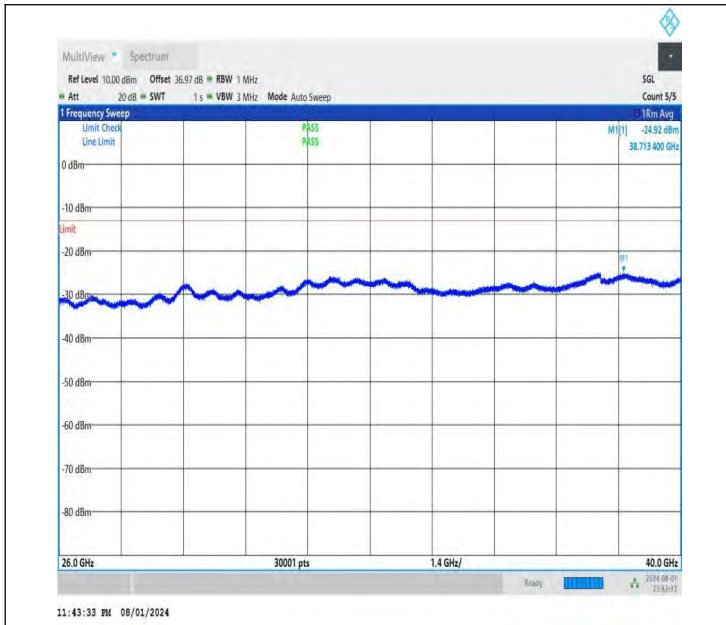
NTNV-DC_26A-n78A(3700-3800)-PC3-30-5+60-M+H-QPSK-IDL E-DFT-QPSK-Edge_1RB_Left-26000-40000-PASS
