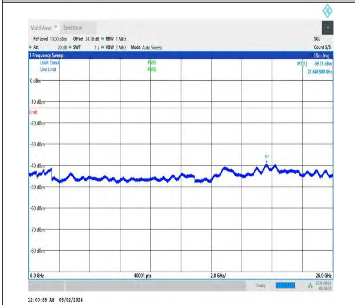
NTNV-DC_26A-n78A(3700-3800)-PC3-30-5+70-M+H-QPSK-IDL E-DFT-QPSK-Edge_1RB_Right-6000-26000-PASS
