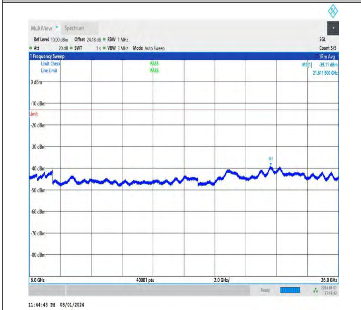
NTNV-DC_26A-n78A(3700-3800)-PC3-30-5+60-M+H-QPSK-IDL E-DFT-QPSK-Edge_1RB_Right-6000-26000-PASS
