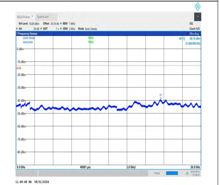
NTNV-DC_26A-n78A(3700-3800)-PC3-30-5+70-M+L-QPSK-IDLE -DFT-QPSK-Edge_1RB_Left-6000-26000-PASS
