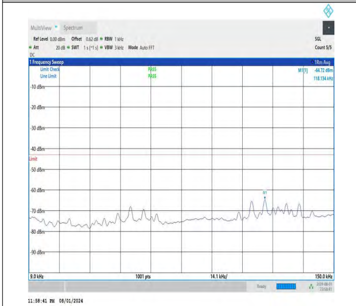
NTNV-DC_26A-n78A(3700-3800)-PC3-30-5+70-M+H-QPSK-IDL E-DFT-QPSK-Edge_1RB_Left-0.009-0.15-PASS
