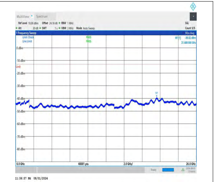
NTNV-DC_26A-n78A(3700-3800)-PC3-30-5+70-M+H-QPSK-IDLE -DFT-BPSK-Edge_1RB_Left-6000-26000-PASS
