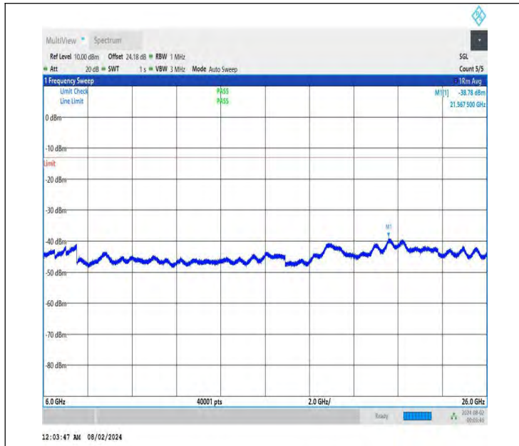
NTNV-DC_26A-n78A(3700-3800)-PC3-30-5+80-M+L-QPSK-IDL E-DFT-BPSK-Edge_1RB_Right-6000-26000-PASS
