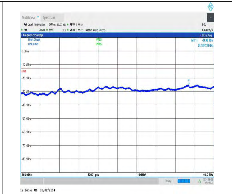
NTNV-DC_26A-n78A(3700-3800)-PC3-30-5+80-M+H-QPSK-IDLE -DFT-BPSK-Edge_1RB_Right-26000-40000-PASS
