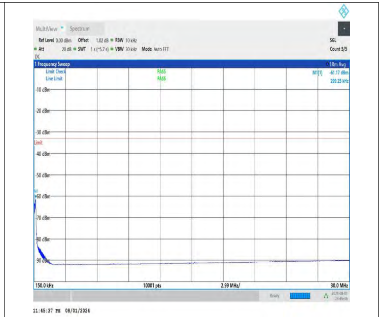
NTNV-DC_26A-n78A(3700-3800)-PC3-30-5+70-M+L-QPSK-IDLE -DFT-BPSK-Edge_1RB_Left-0.15-30-PASS
