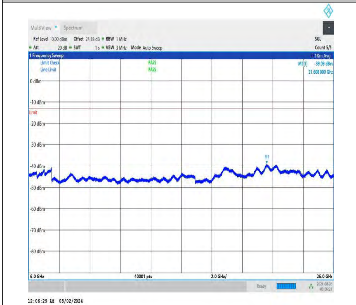
NTNV-DC_26A-n78A(3700-3800)-PC3-30-5+80-M+L-QPSK-IDL E-DFT-QPSK-Edge_1RB_Right-6000-26000-PASS
