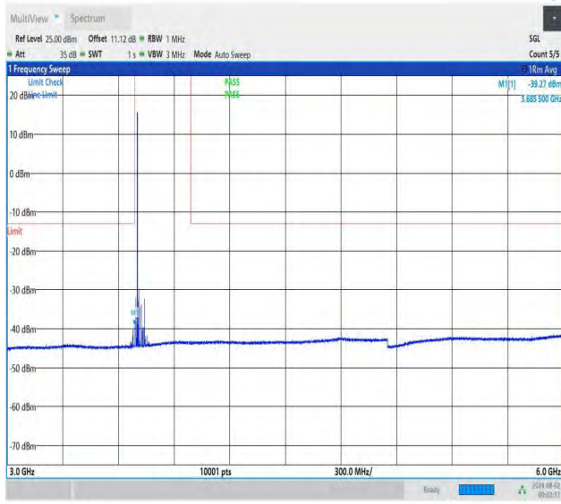
NTNV-DC_26A-n78A(3700-3800)-PC3-30-5+80-M+L-QPSK-IDL E-DFT-BPSK-Edge_1RB_Left-3000-6000-PASS
