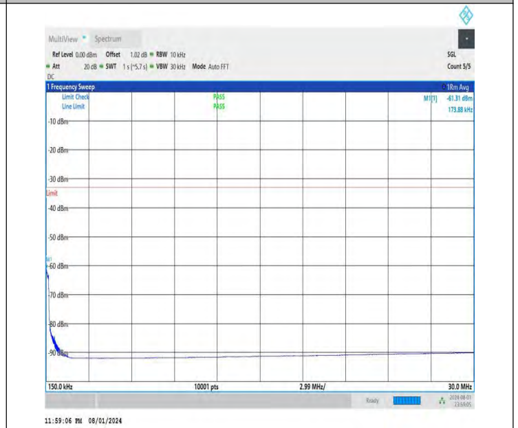
NTNV-DC_26A-n78A(3700-3800)-PC3-30-5+70-M+H-QPSK-IDLE -DFT-QPSK-Edge_1RB_Left-0.15-30-PASS
