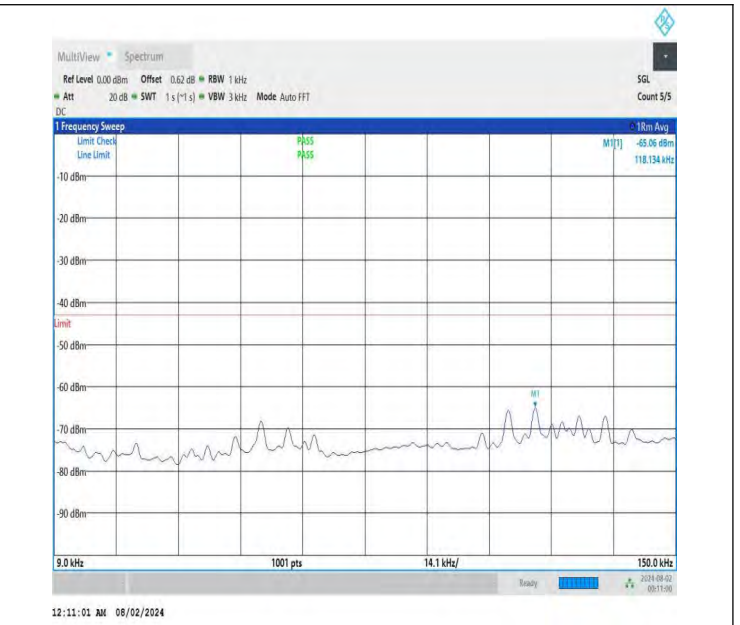
NTNV-DC_26A-n78A(3700-3800)-PC3-30-5+80-M+M-QPSK-IDLE -DFT-QPSK-Edge_1RB_Right-0.009-0.15-PASS
