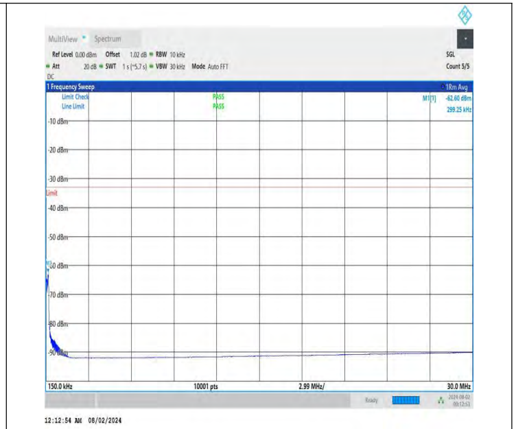
NTNV-DC_26A-n78A(3700-3800)-PC3-30-5+80-M+H-QPSK-IDLE -DFT-BPSK-Edge_1RB_Left-0.15-30-PASS
