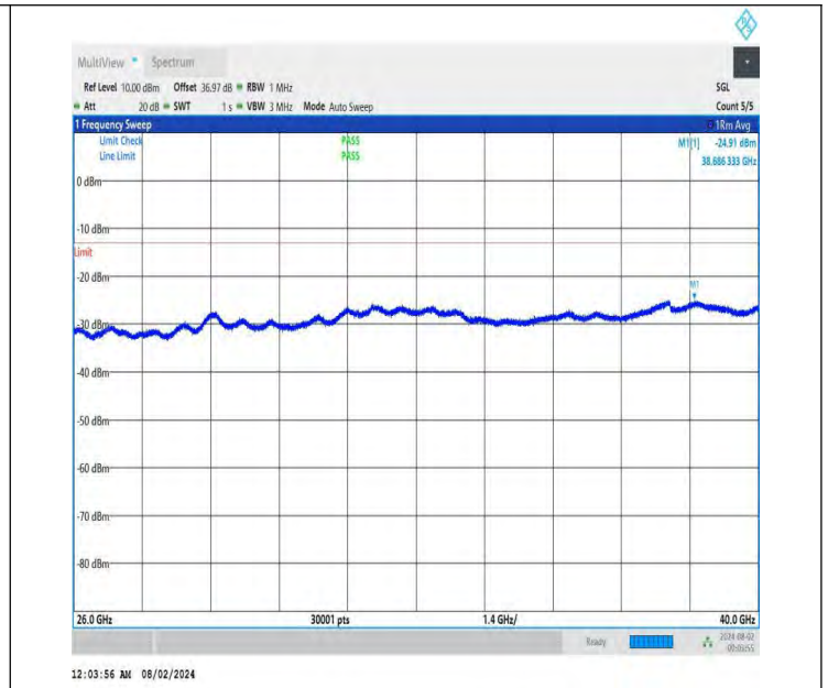
NTNV-DC_26A-n78A(3700-3800)-PC3-30-5+80-M+L-QPSK-IDLE -DFT-BPSK-Edge_1RB_Right-26000-40000-PASS
