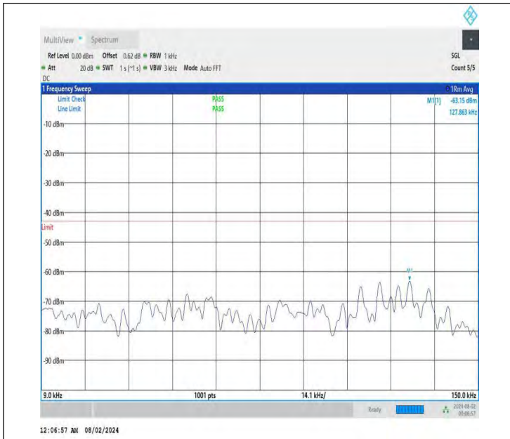
NTNV-DC_26A-n78A(3700-3800)-PC3-30-5+80-M+M-QPSK-IDL E-DFT-BPSK-Edge_1RB_Left-0.009-0.15-PASS
