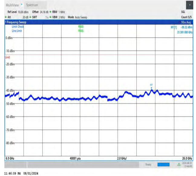
NTNV-DC_26A-n78A(3700-3800)-PC3-30-5+70-M+L-QPSK-IDLE -DFT-BPSK-Edge_1RB_Left-6000-26000-PASS
