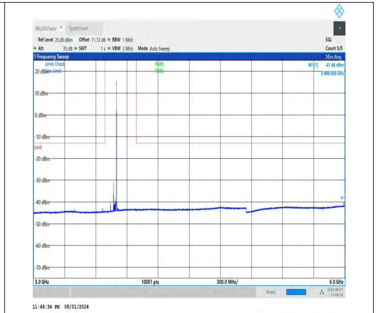
NTNV-DC_26A-n78A(3700-3800)-PC3-30-5+60-M+H-QPSK-IDLE -DFT-QPSK-Edge_1RB_Right-3000-6000-PASS
