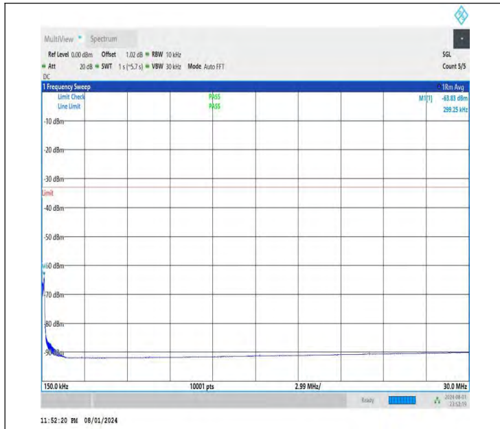
NTNV-DC_26A-n78A(3700-3800)-PC3-30-5+70-M+M-QPSK-IDL E-DFT-BPSK-Edge_1RB_Right-0.15-30-PASS
