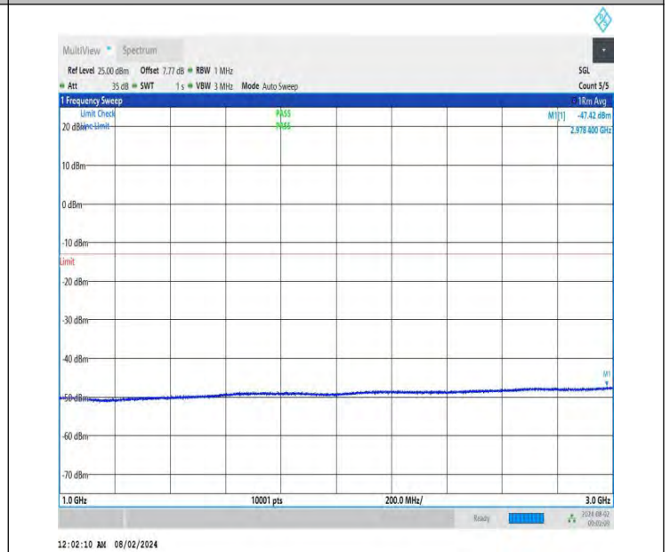
NTNV-DC_26A-n78A(3700-3800)-PC3-30-5+80-M+L-QPSK-IDLE -DFT-BPSK-Edge_1RB_Left-1000-3000-PASS
