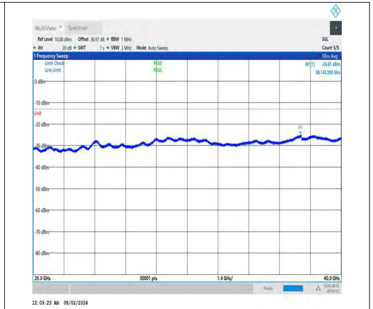
NTNV-DC_26A-n78A(3700-3800)-PC3-30-5+80-M+M-QPSK-IDLE -DFT-BPSK-Edge_1RB_Right-26000-40000-PASS
