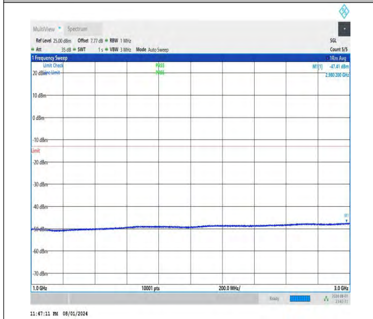
NTNV-DC_26A-n78A(3700-3800)-PC3-30-5+70-M+L-QPSK-IDL E-DFT-BPSK-Edge_1RB_Right-1000-3000-PASS
