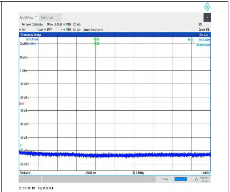
NTNV-DC_26A-n78A(3700-3800)-PC3-30-5+70-M+M-QPSK-IDLE -DFT-BPSK-Edge_1RB_Right-30-1000-PASS
