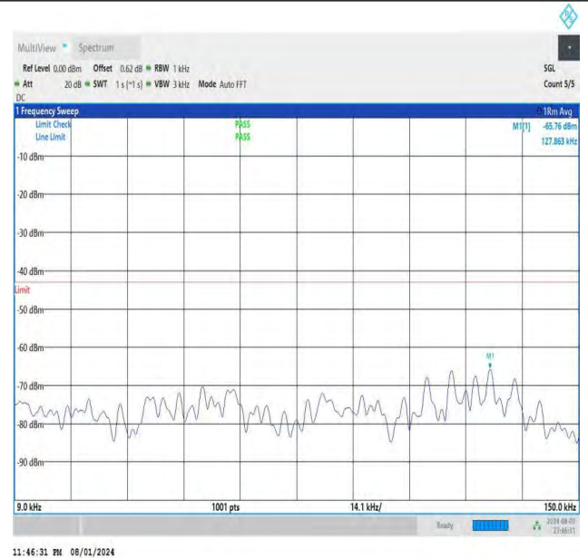
NTNV-DC_26A-n78A(3700-3800)-PC3-30-5+70-M+L-QPSK-IDLE -DFT-BPSK-Edge_1RB_Right-0.009-0.15-PASS
