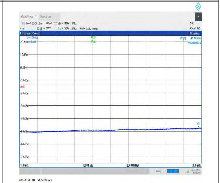
NTNV-DC_26A-n78A(3700-3800)-PC3-30-5+80-M+H-QPSK-IDLE -DFT-BPSK-Edge_1RB_Left-1000-3000-PASS
