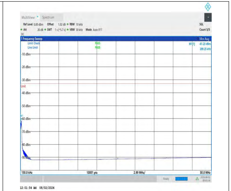
NTNV-DC_26A-n78A(3700-3800)-PC3-30-5+80-M+L-QPSK-IDLE -DFT-BPSK-Edge_1RB_Left-0.15-30-PASS
