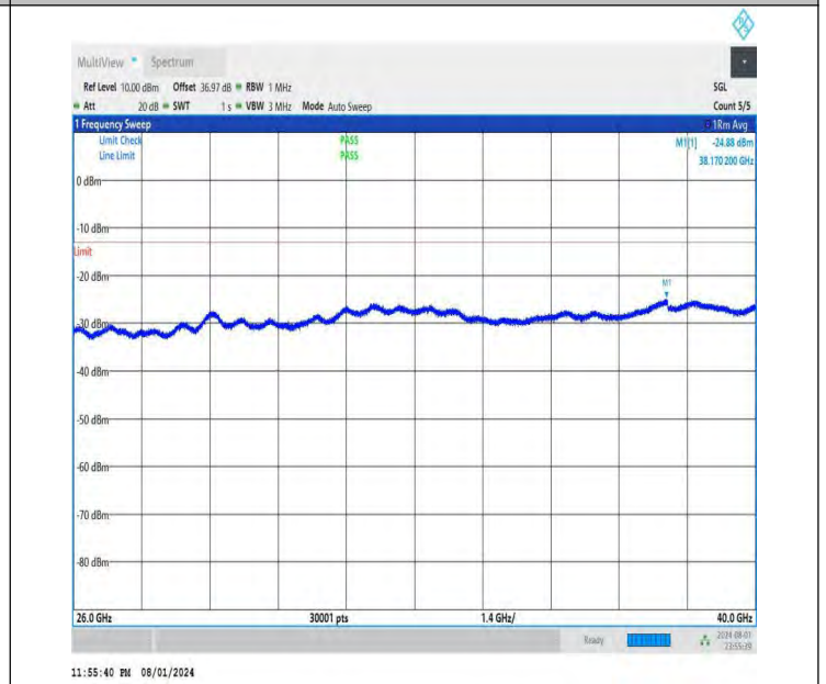
NTNV-DC_26A-n78A(3700-3800)-PC3-30-5+70-M+M-QPSK-IDLE -DFT-QPSK-Edge_1RB_Right-26000-40000-PASS
