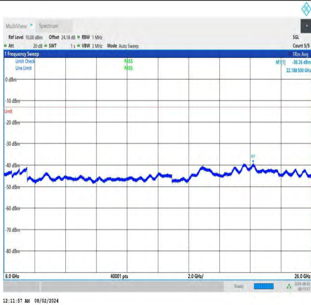
NTNV-DC_26A-n78A(3700-3800)-PC3-30-5+80-M+M-QPSK-IDL E-DFT-QPSK-Edge_1RB_Right-6000-26000-PASS
