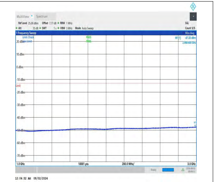
NTNV-DC_26A-n78A(3700-3800)-PC3-30-5+80-M+L-QPSK-IDLE -DFT-QPSK-Edge_1RB_Left-1000-3000-PASS
