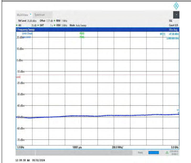
NTNV-DC_26A-n78A(3700-3800)-PC3-30-5+80-M+M-QPSK-IDL E-DFT-BPSK-Edge_1RB_Right-1000-3000-PASS
