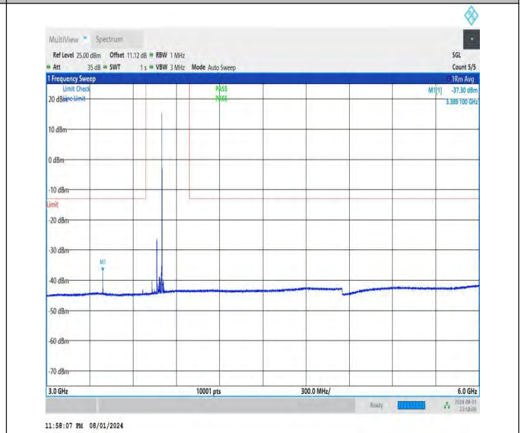
NTNV-DC_26A-n78A(3700-3800)-PC3-30-5+70-M+H-QPSK-IDLE -DFT-BPSK-Edge_1RB_Right-3000-6000-PASS
