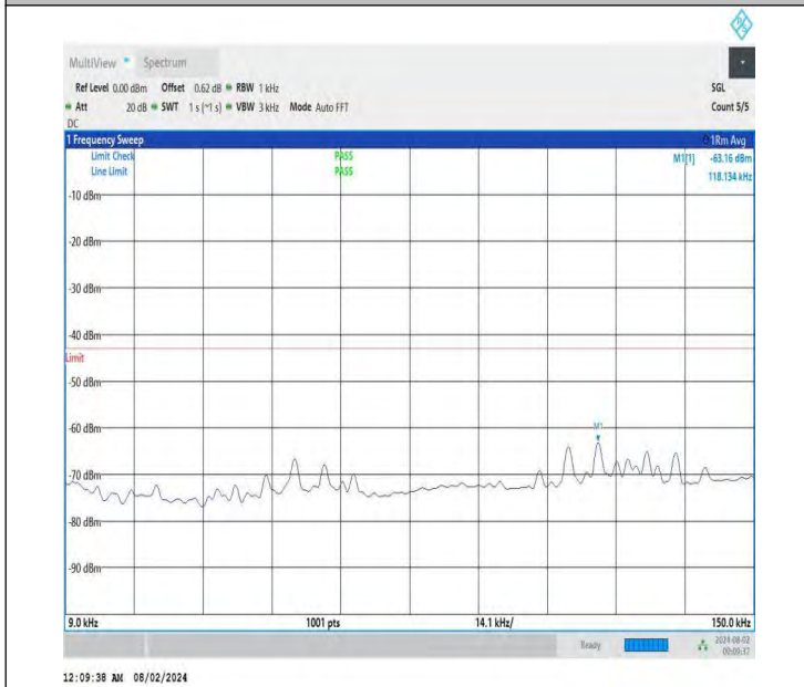
NTNV-DC_26A-n78A(3700-3800)-PC3-30-5+80-M+M-QPSK-IDL E-DFT-QPSK-Edge_1RB_Left-0.009-0.15-PASS
