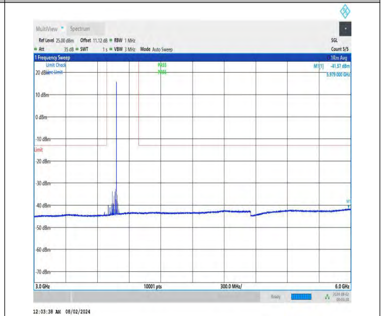
NTNV-DC_26A-n78A(3700-3800)-PC3-30-5+80-M+L-QPSK-IDLE -DFT-BPSK-Edge_1RB_Right-3000-6000-PASS
