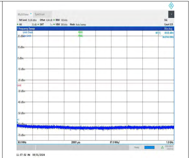
NTNV-DC_26A-n78A(3700-3800)-PC3-30-5+70-M+H-QPSK-IDLE -DFT-BPSK-Edge_1RB_Right-30-1000-PASS
