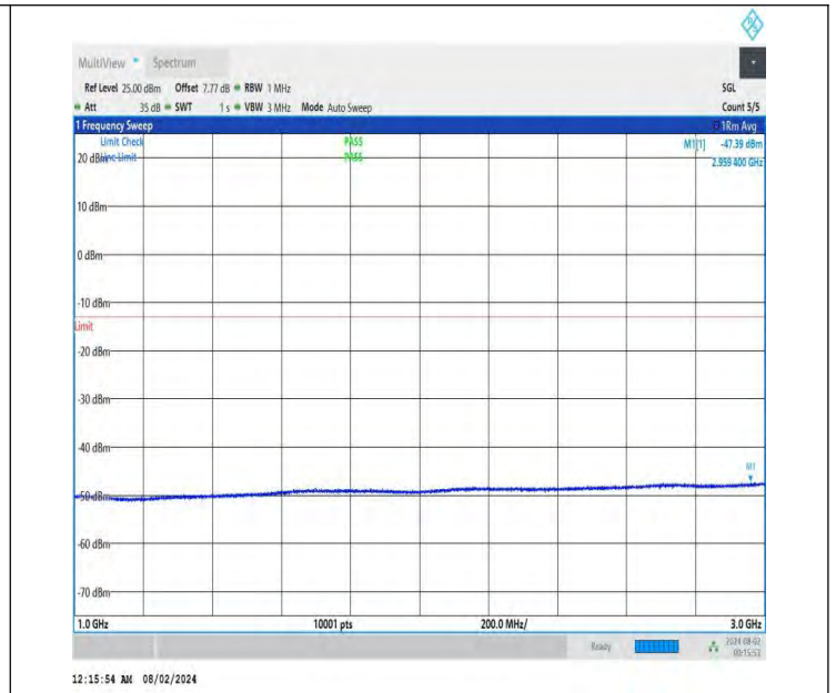
NTNV-DC_26A-n78A(3700-3800)-PC3-30-5+80-M+H-QPSK-IDLE -DFT-QPSK-Edge_1RB_Left-1000-3000-PASS
