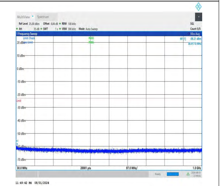
NTNV-DC_26A-n78A(3700-3800)-PC3-30-5+70-M+L-QPSK-IDLE -DFT-QPSK-Edge_1RB_Right-30-1000-PASS
