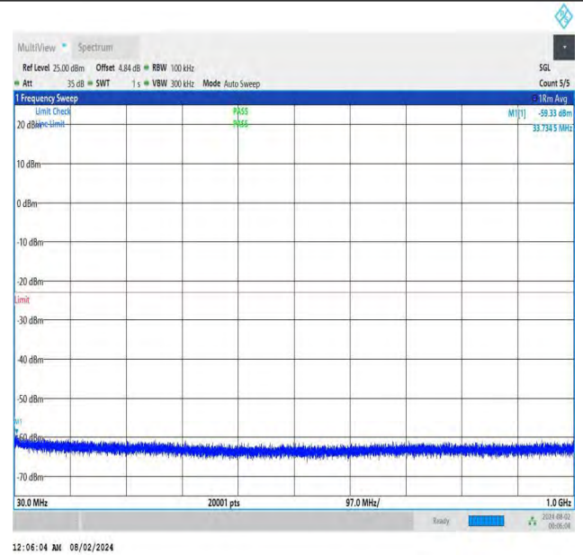
NTNV-DC_26A-n78A(3700-3800)-PC3-30-5+80-M+L-QPSK-IDLE -DFT-QPSK-Edge_1RB_Right-30-1000-PASS
