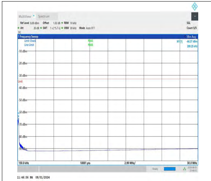
NTNV-DC_26A-n78A(3700-3800)-PC3-30-5+70-M+L-QPSK-IDL E-DFT-BPSK-Edge_1RB_Right-0.15-30-PASS
