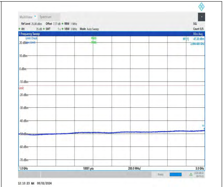
NTNV-DC_26A-n78A(3700-3800)-PC3-30-5+80-M+M-QPSK-IDLE -DFT-QPSK-Edge_1RB_Left-1000-3000-PASS
