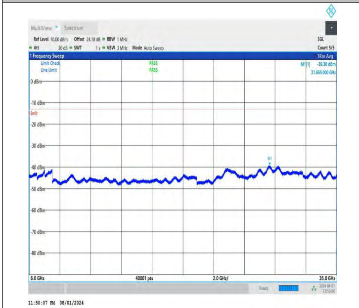
NTNV-DC_26A-n78A(3700-3800)-PC3-30-5+70-M+L-QPSK-IDL E-DFT-QPSK-Edge_1RB_Right-6000-26000-PASS
