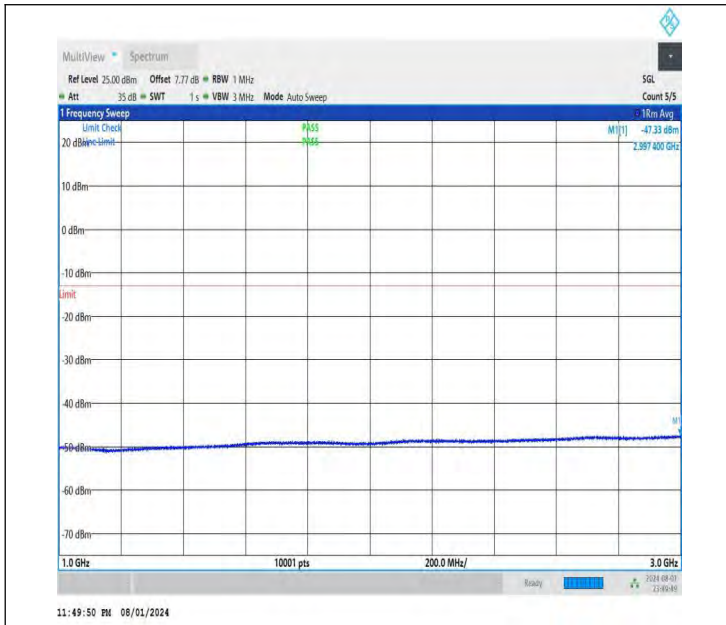
NTNV-DC_26A-n78A(3700-3800)-PC3-30-5+70-M+L-QPSK-IDL E-DFT-QPSK-Edge_1RB_Right-1000-3000-PASS
