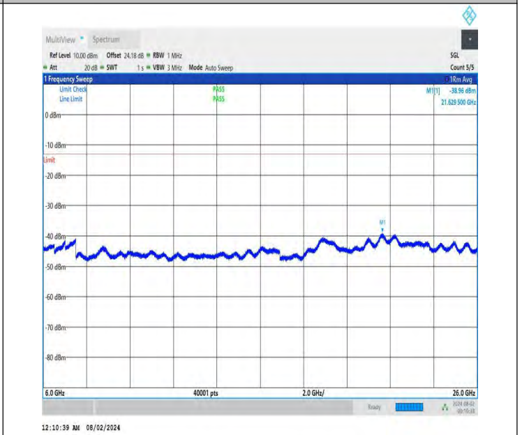
NTNV-DC_26A-n78A(3700-3800)-PC3-30-5+80-M+M-QPSK-IDLE -DFT-QPSK-Edge_1RB_Left-6000-26000-PASS
