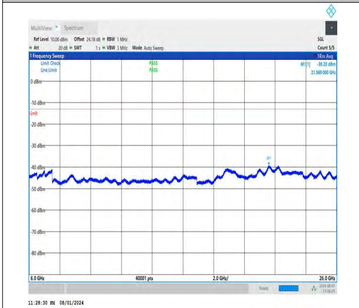
NTNV-DC_26A-n78A(3700-3800)-PC3-30-5+50-M+H-QPSK-IDL E-DFT-QPSK-Edge_1RB_Right-6000-26000-PASS
