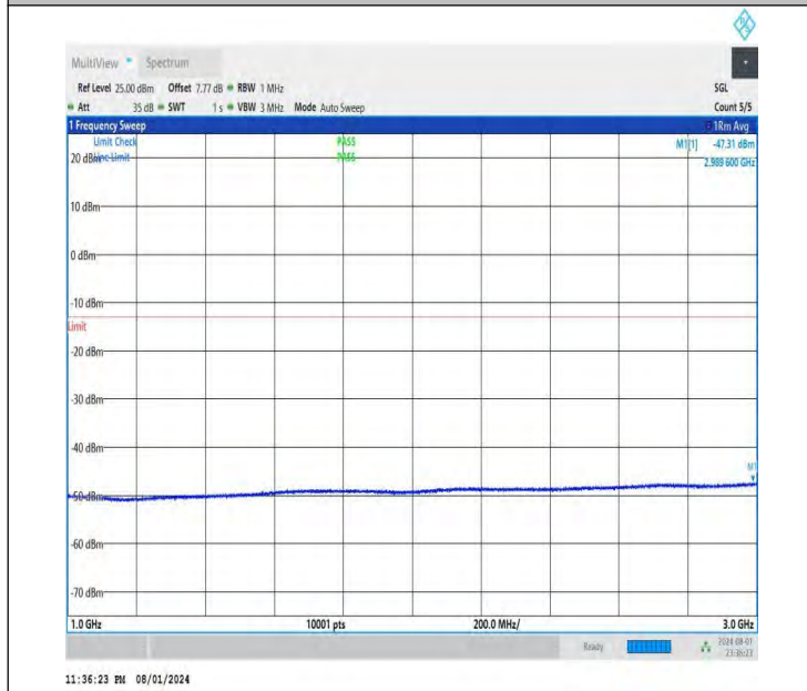
NTNV-DC_26A-n78A(3700-3800)-PC3-30-5+60-M+M-QPSK-IDL E-DFT-BPSK-Edge_1RB_Right-1000-3000-PASS
