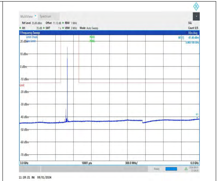
NTNV-DC_26A-n78A(3700-3800)-PC3-30-5+50-M+H-QPSK-IDLE -DFT-QPSK-Edge_1RB_Right-3000-6000-PASS
