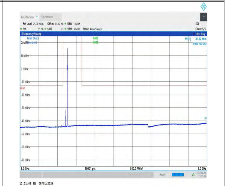
NTNV-DC_26A-n78A(3700-3800)-PC3-30-5+60-M+L-QPSK-IDLE -DFT-BPSK-Edge_1RB_Right-3000-6000-PASS
