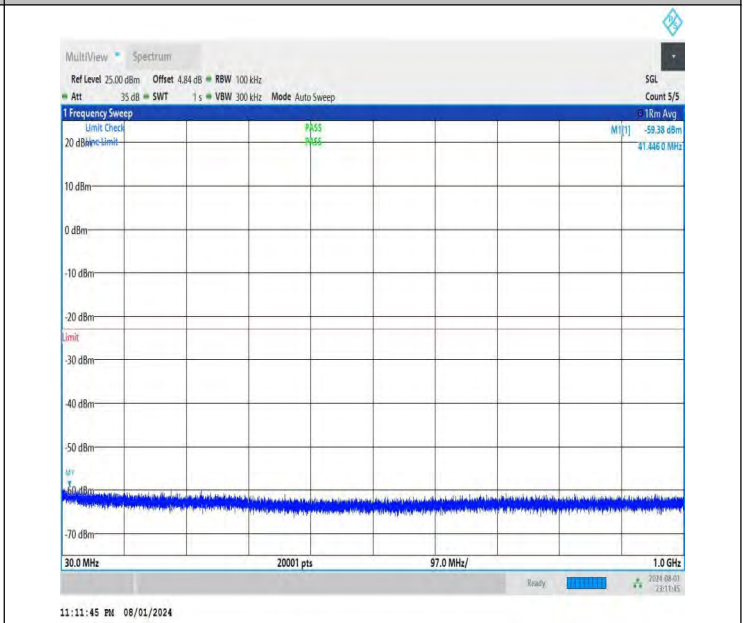
NTNV-DC_26A-n78A(3700-3800)-PC3-30-5+40-M+H-QPSK-IDLE -DFT-QPSK-Edge_1RB_Right-30-1000-PASS
