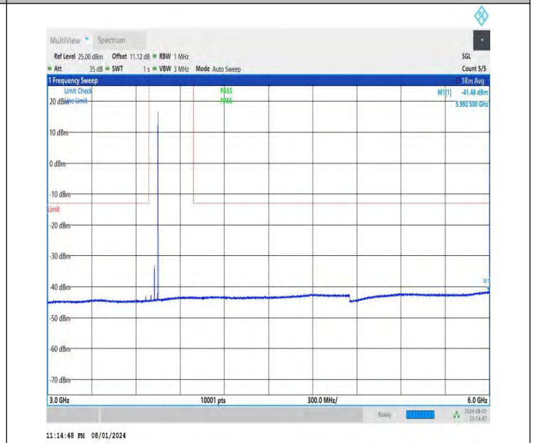
NTNV-DC_26A-n78A(3700-3800)-PC3-30-5+50-M+L-QPSK-IDLE -DFT-BPSK-Edge_1RB_Right-3000-6000-PASS
