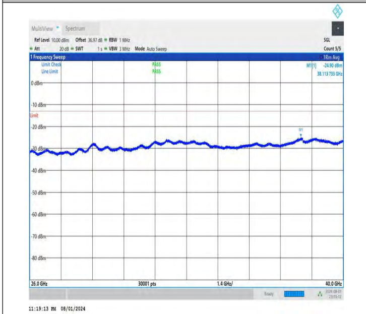
NTNV-DC_26A-n78A(3700-3800)-PC3-30-5+50-M+M-QPSK-IDL E-DFT-BPSK-Edge_1RB_Left-26000-40000-PASS
