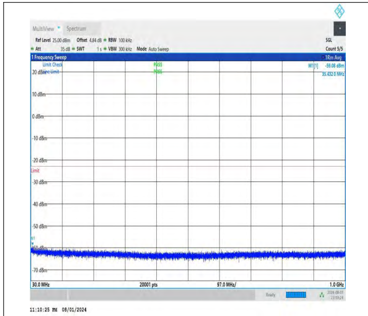
NTNV-DC_26A-n78A(3700-3800)-PC3-30-5+40-M+H-QPSK-IDL E-DFT-QPSK-Edge_1RB_Left-30-1000-PASS
