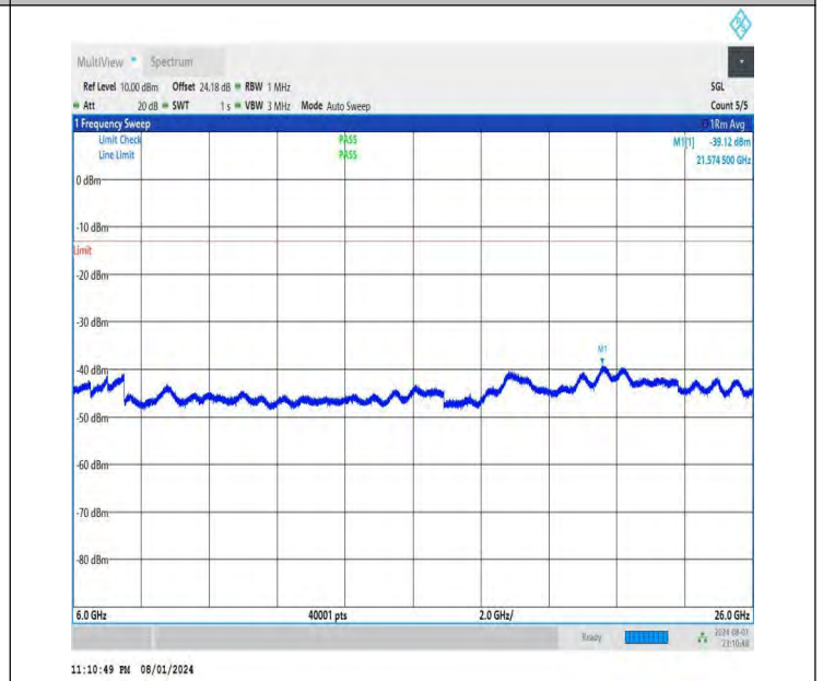
NTNV-DC_26A-n78A(3700-3800)-PC3-30-5+40-M+H-QPSK-IDLE -DFT-QPSK-Edge_1RB_Left-6000-26000-PASS
