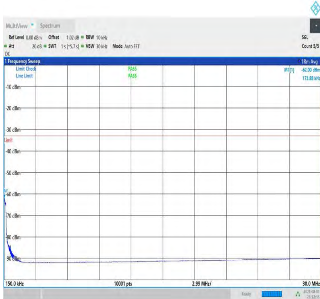
NTNV-DC_26A-n78A(3700-3800)-PC3-30-5+50-M+M-QPSK-IDL E-DFT-QPSK-Edge_1RB_Left-26000-40000-PASS
