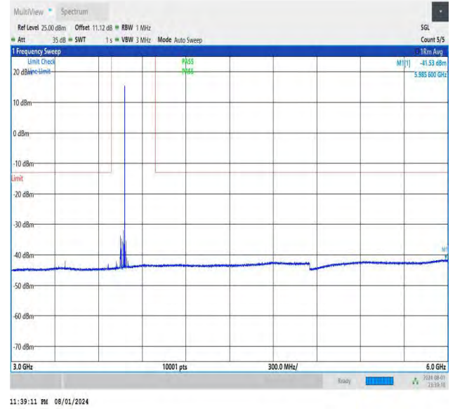
NTNV-DC_26A-n78A(3700-3800)-PC3-30-5+60-M+M-QPSK-IDLE -DFT-QPSK-Edge_1RB_Right-3000-6000-PASS
