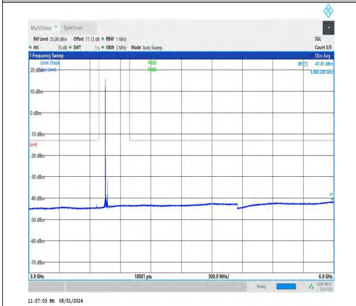
NTNV-DC_26A-n78A(3700-3800)-PC3-30-5+50-M+H-QPSK-IDL E-DFT-QPSK-Edge_1RB_Left-3000-6000-PASS
