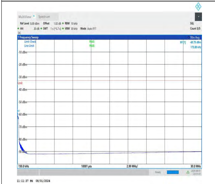
NTNV-DC_26A-n78A(3700-3800)-PC3-30-5+40-M+H-QPSK-IDL E-DFT-QPSK-Edge_1RB_Right-0.15-30-PASS
