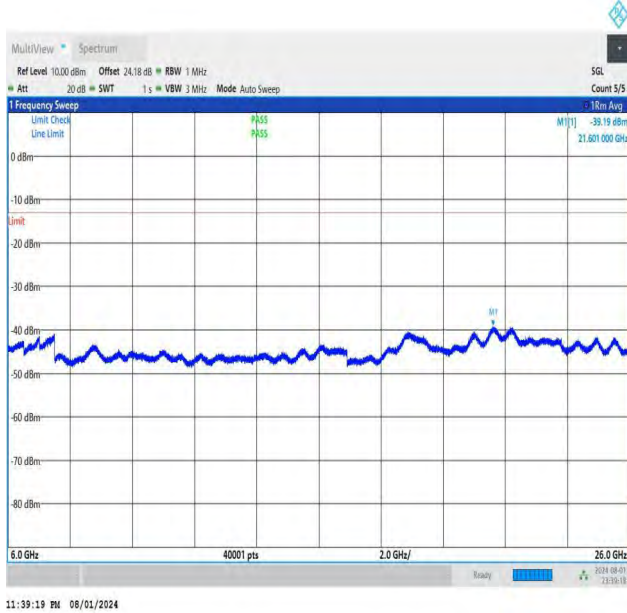
NTNV-DC_26A-n78A(3700-3800)-PC3-30-5+60-M+M-QPSK-IDL E-DFT-QPSK-Edge_1RB_Right-6000-26000-PASS
