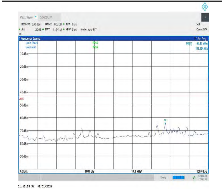
NTNV-DC_26A-n78A(3700-3800)-PC3-30-5+60-M+H-QPSK-IDL E-DFT-QPSK-Edge_1RB_Left-0.009-0.15-PASS
