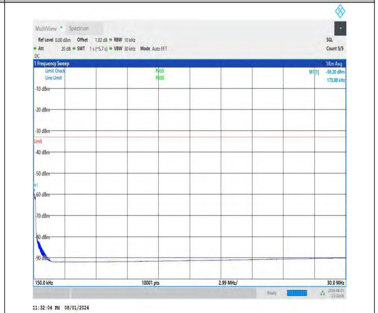
NTNV-DC_26A-n78A(3700-3800)-PC3-30-5+60-M+L-QPSK-IDLE -DFT-QPSK-Edge_1RB_Left-0.15-30-PASS
