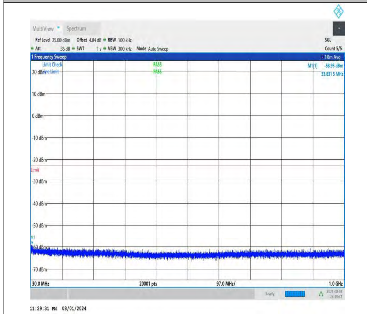
NTNV-DC_26A-n78A(3700-3800)-PC3-30-5+60-M+L-QPSK-IDL E-DFT-BPSK-Edge_1RB_Left-30-1000-PASS
