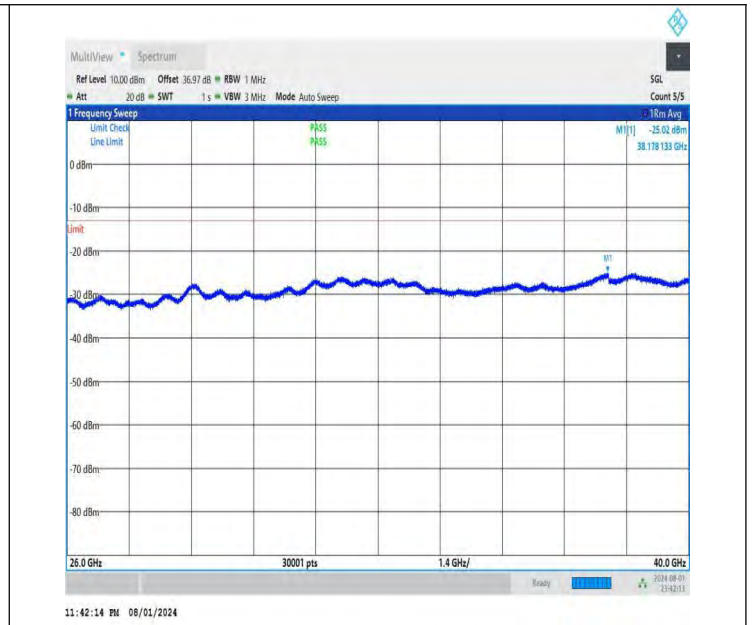
NTNV-DC_26A-n78A(3700-3800)-PC3-30-5+60-M+H-QPSK-IDLE -DFT-BPSK-Edge_1RB_Right-26000-40000-PASS
