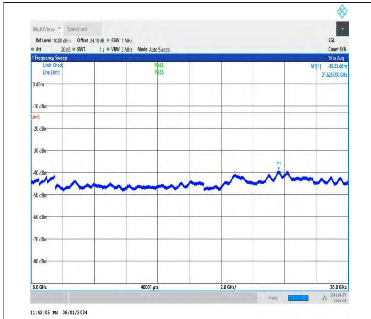
NTNV-DC_26A-n78A(3700-3800)-PC3-30-5+60-M+H-QPSK-IDL E-DFT-BPSK-Edge_1RB_Right-6000-26000-PASS
