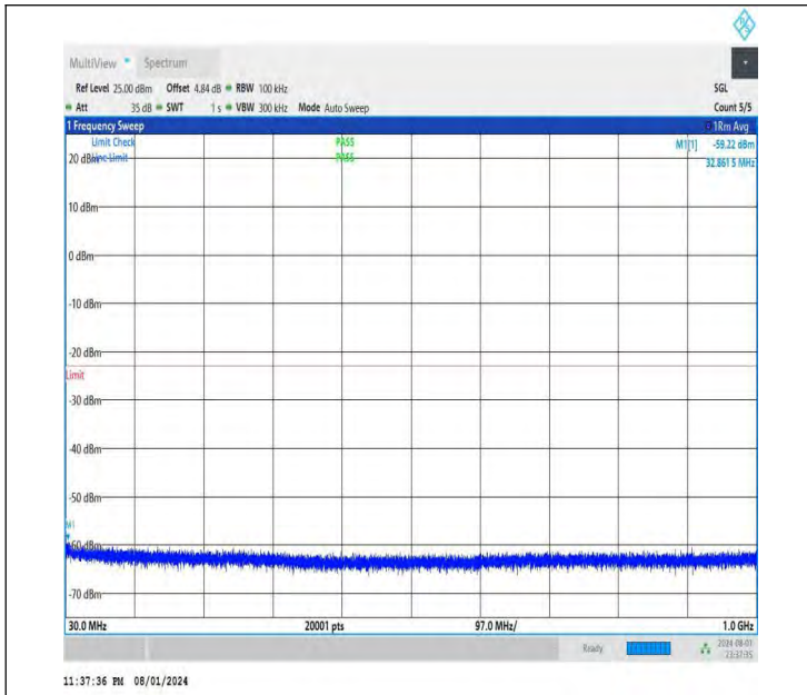
NTNV-DC_26A-n78A(3700-3800)-PC3-30-5+60-M+M-QPSK-IDL E-DFT-QPSK-Edge_1RB_Left-30-1000-PASS
