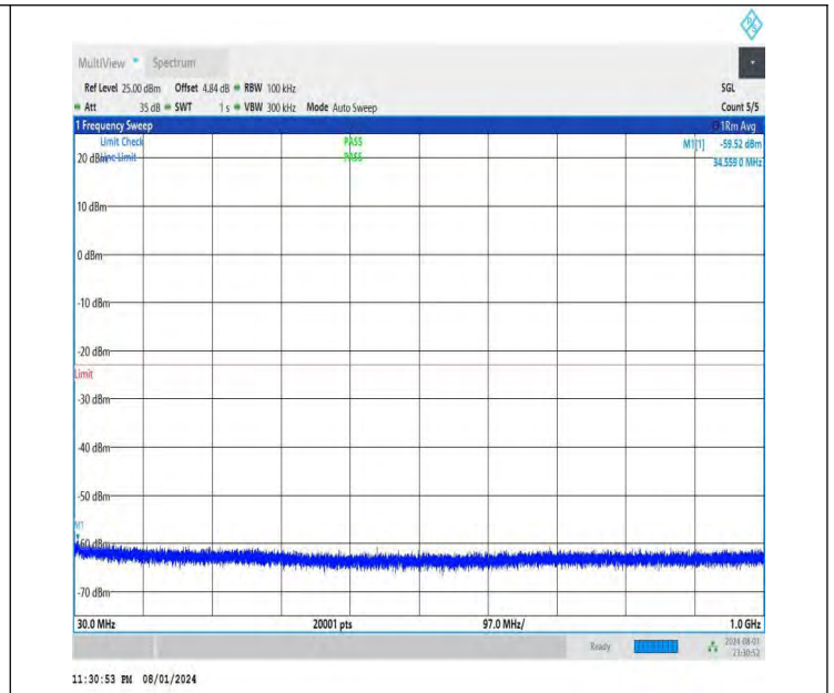
NTNV-DC_26A-n78A(3700-3800)-PC3-30-5+60-M+L-QPSK-IDLE -DFT-BPSK-Edge_1RB_Right-30-1000-PASS
