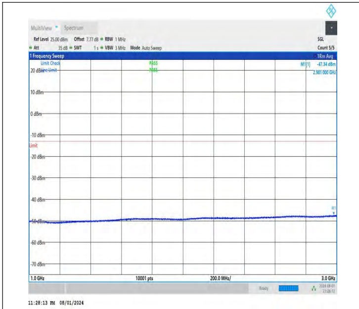
NTNV-DC_26A-n78A(3700-3800)-PC3-30-5+50-M+H-QPSK-IDL E-DFT-QPSK-Edge_1RB_Right-1000-3000-PASS
