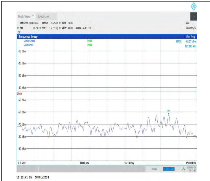
NTNV-DC_26A-n78A(3700-3800)-PC3-30-5+50-M+L-QPSK-IDL E-DFT-BPSK-Edge_1RB_Left-0.009-0.15-PASS
