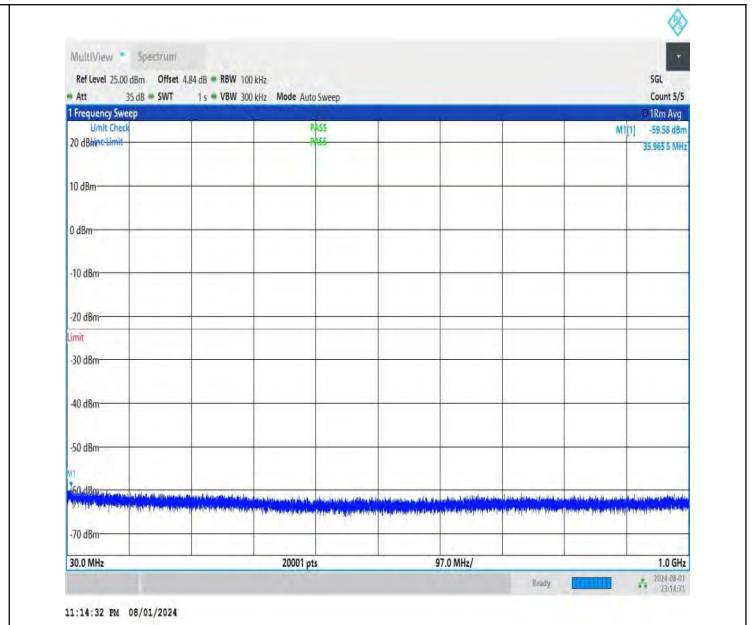
NTNV-DC_26A-n78A(3700-3800)-PC3-30-5+50-M+L-QPSK-IDLE -DFT-BPSK-Edge_1RB_Right-30-1000-PASS
