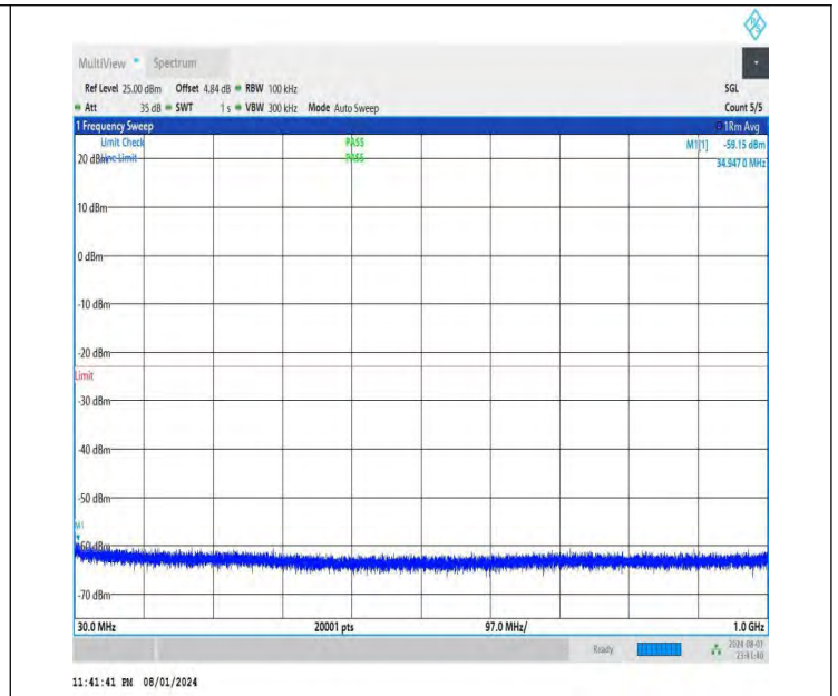
NTNV-DC_26A-n78A(3700-3800)-PC3-30-5+60-M+H-QPSK-IDLE -DFT-BPSK-Edge_1RB_Right-30-1000-PASS
