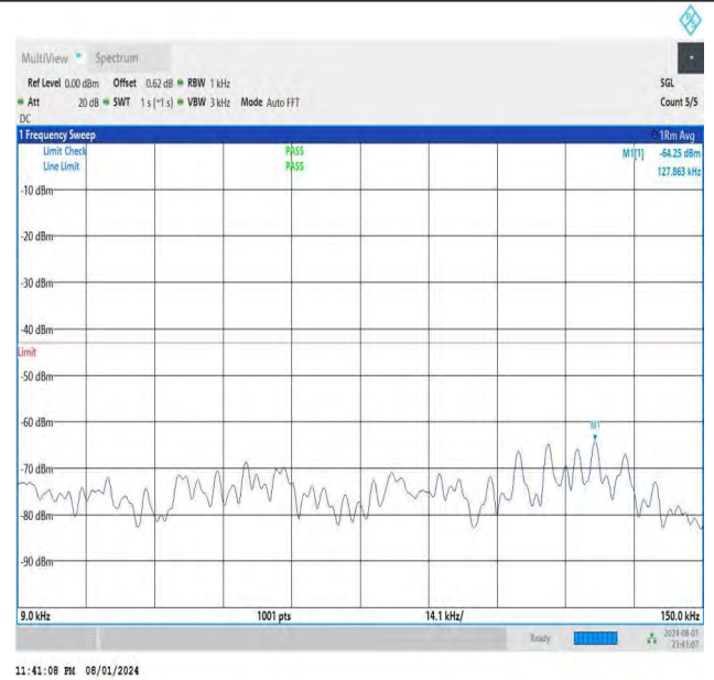
NTNV-DC_26A-n78A(3700-3800)-PC3-30-5+60-M+H-QPSK-IDLE -DFT-BPSK-Edge_1RB_Right-0.009-0.15-PASS
