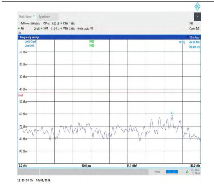
NTNV-DC_26A-n78A(3700-3800)-PC3-30-5+60-M+L-QPSK-IDL E-DFT-BPSK-Edge_1RB_Left-0.009-0.15-PASS
