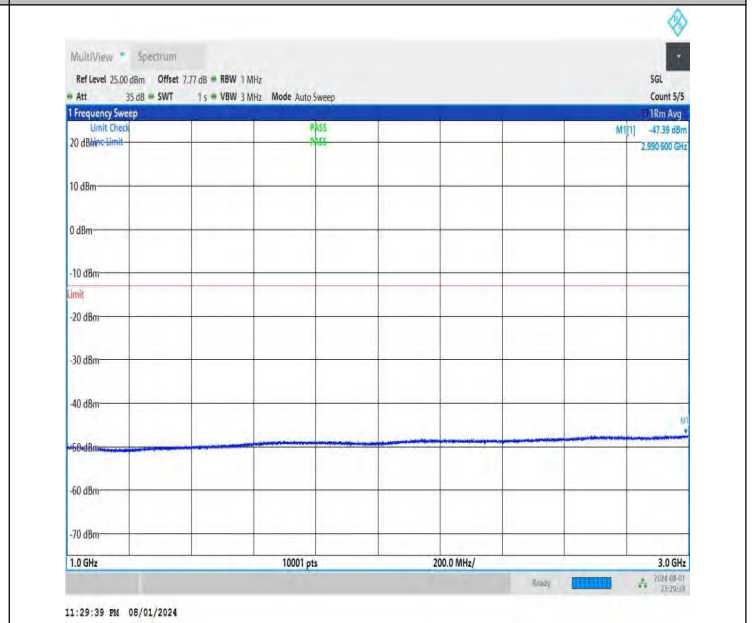
NTNV-DC_26A-n78A(3700-3800)-PC3-30-5+60-M+L-QPSK-IDLE -DFT-BPSK-Edge_1RB_Left-1000-3000-PASS
