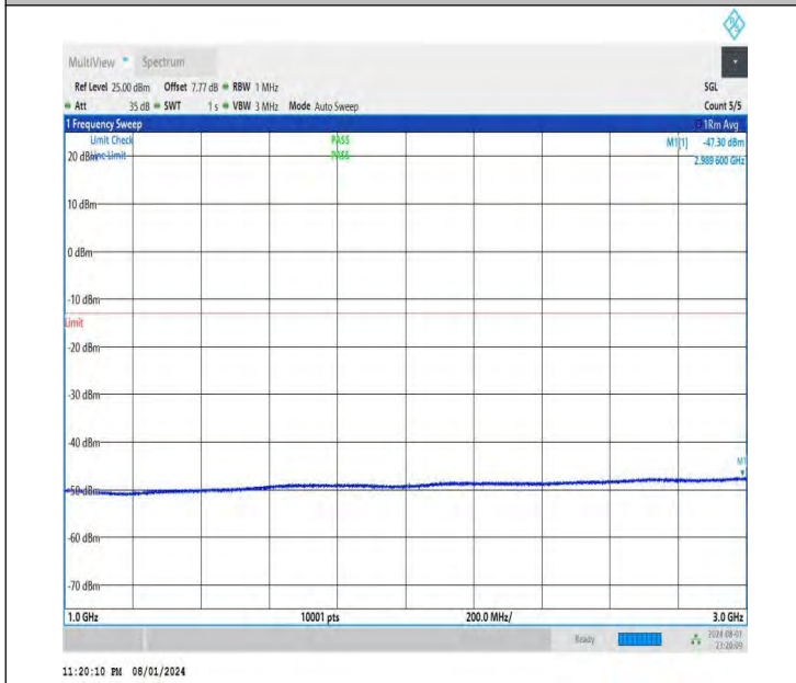
NTNV-DC_26A-n78A(3700-3800)-PC3-30-5+50-M+M-QPSK-IDL E-DFT-BPSK-Edge_1RB_Right-1000-3000-PASS
