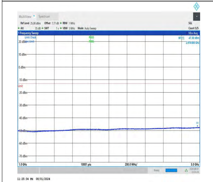
NTNV-DC_26A-n78A(3700-3800)-PC3-30-5+50-M+H-QPSK-IDL E-DFT-BPSK-Edge_1RB_Right-1000-3000-PASS
