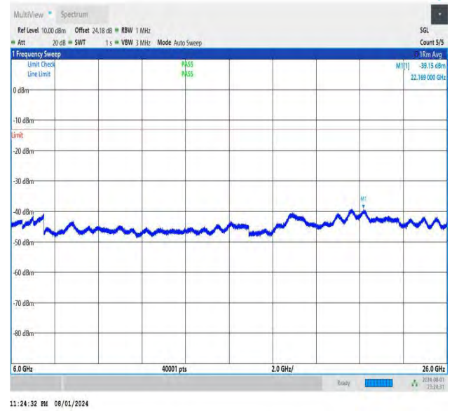
NTNV-DC_26A-n78A(3700-3800)-PC3-30-5+50-M+H-QPSK-IDLE -DFT-BPSK-Edge_1RB_Left-6000-26000-PASS
