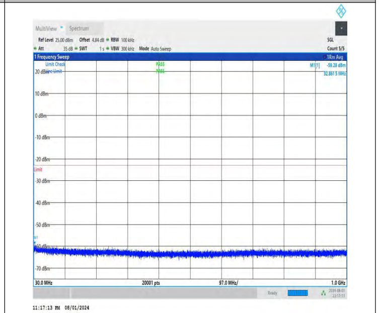
NTNV-DC_26A-n78A(3700-3800)-PC3-30-5+50-M+L-QPSK-IDLE -DFT-QPSK-Edge_1RB_Right-30-1000-PASS
