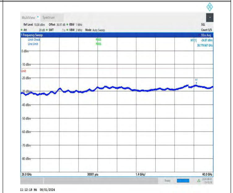
NTNV-DC_26A-n78A(3700-3800)-PC3-30-5+40-M+H-QPSK-IDLE -DFT-QPSK-Edge_1RB_Right-26000-40000-PASS
