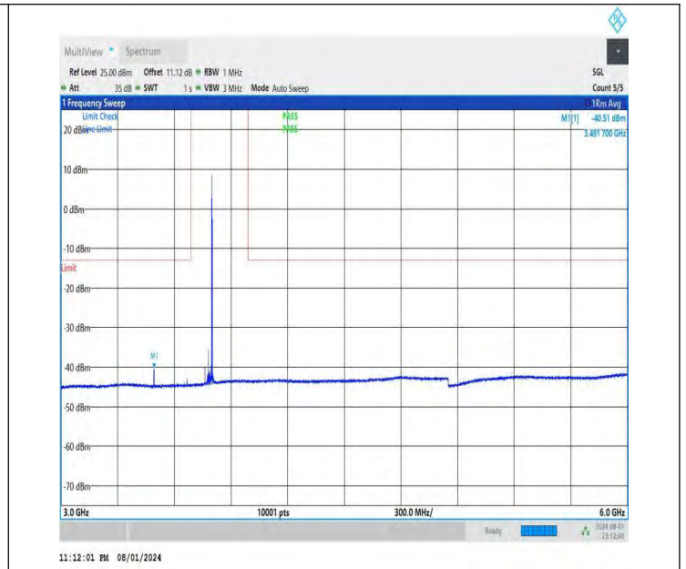
NTNV-DC_26A-n78A(3700-3800)-PC3-30-5+40-M+H-QPSK-IDLE -DFT-QPSK-Edge_1RB_Right-3000-6000-PASS
