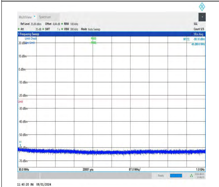
NTNV-DC_26A-n78A(3700-3800)-PC3-30-5+60-M+H-QPSK-IDL E-DFT-BPSK-Edge_1RB_Left-30-1000-PASS
