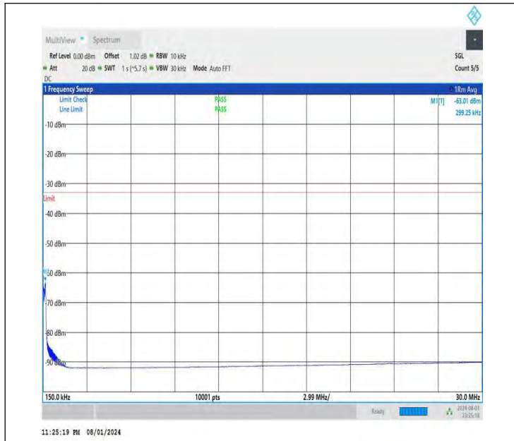
NTNV-DC_26A-n78A(3700-3800)-PC3-30-5+50-M+H-QPSK-IDL E-DFT-BPSK-Edge_1RB_Right-0.15-30-PASS
