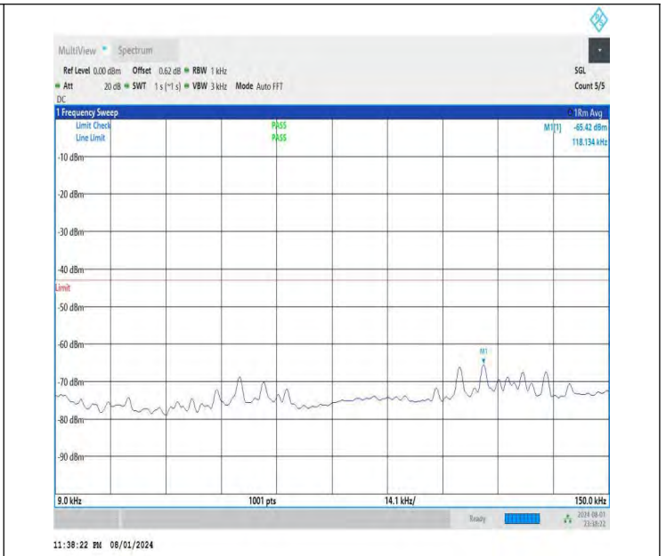
NTNV-DC_26A-n78A(3700-3800)-PC3-30-5+60-M+M-QPSK-IDLE -DFT-QPSK-Edge_1RB_Right-0.009-0.15-PASS
