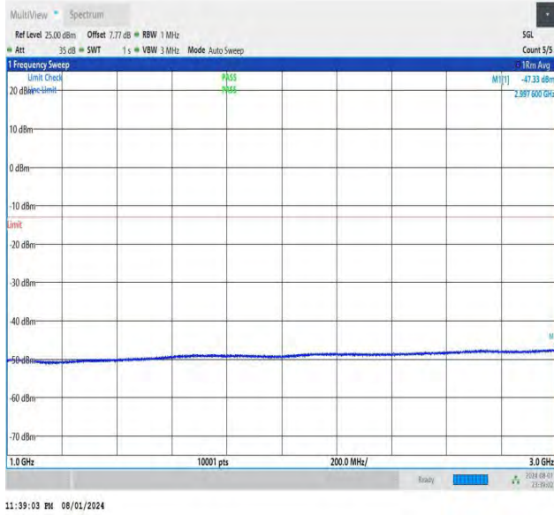
NTNV-DC_26A-n78A(3700-3800)-PC3-30-5+60-M+M-QPSK-IDL E-DFT-QPSK-Edge_1RB_Right-1000-3000-PASS
