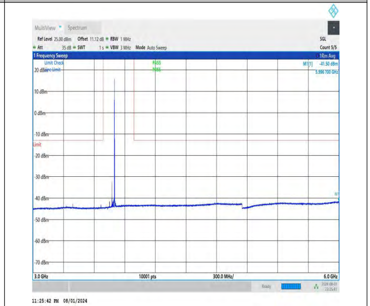
NTNV-DC_26A-n78A(3700-3800)-PC3-30-5+50-M+H-QPSK-IDLE -DFT-BPSK-Edge_1RB_Right-3000-6000-PASS
