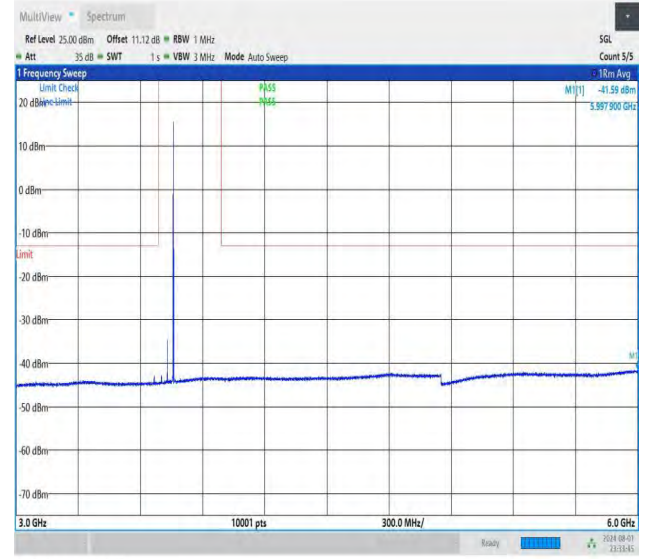
NTNV-DC_26A-n78A(3700-3800)-PC3-30-5+60-M+L-QPSK-IDLE -DFT-QPSK-Edge_1RB_Right-3000-6000-PASS
