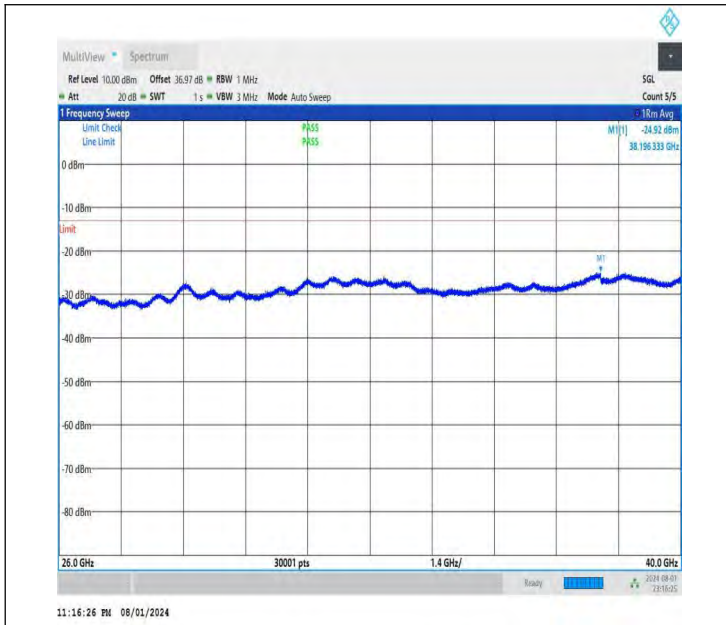
NTNV-DC_26A-n78A(3700-3800)-PC3-30-5+50-M+L-QPSK-IDL E-DFT-QPSK-Edge_1RB_Left-26000-40000-PASS
