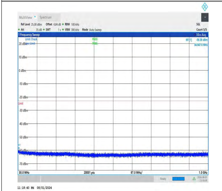
NTNV-DC_26A-n78A(3700-3800)-PC3-30-5+50-M+M-QPSK-IDL E-DFT-BPSK-Edge_1RB_Left-30-1000-PASS
