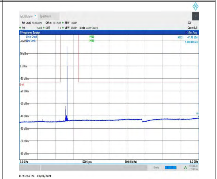
NTNV-DC_26A-n78A(3700-3800)-PC3-30-5+60-M+H-QPSK-IDLE -DFT-BPSK-Edge_1RB_Right-3000-6000-PASS
