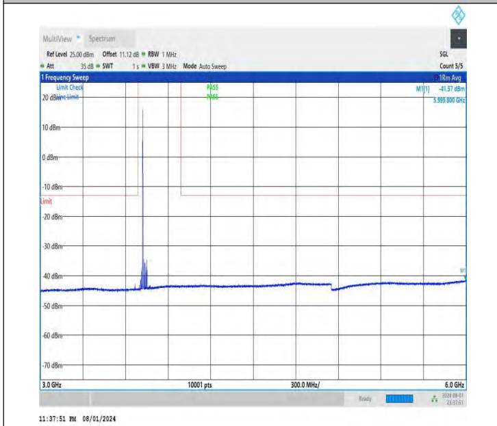
NTNV-DC_26A-n78A(3700-3800)-PC3-30-5+60-M+M-QPSK-IDL E-DFT-QPSK-Edge_1RB_Left-3000-6000-PASS
