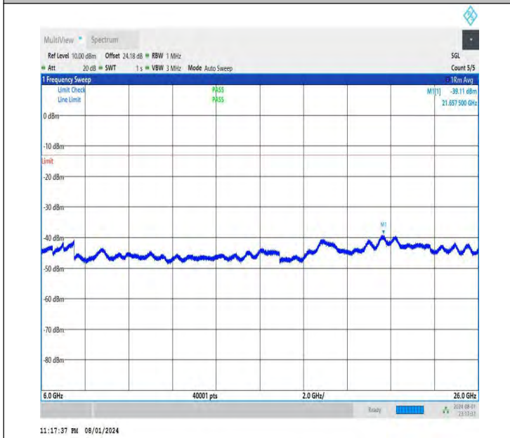
NTNV-DC_26A-n78A(3700-3800)-PC3-30-5+50-M+L-QPSK-IDL E-DFT-QPSK-Edge_1RB_Right-6000-26000-PASS
