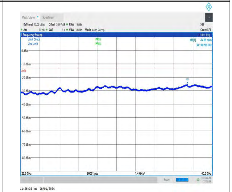
NTNV-DC_26A-n78A(3700-3800)-PC3-30-5+50-M+H-QPSK-IDLE -DFT-QPSK-Edge_1RB_Right-26000-40000-PASS
