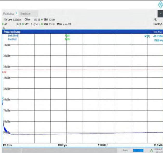
NTNV-DC_26A-n78A(3700-3800)-PC3-30-5+60-M+L-QPSK-IDL E-DFT-QPSK-Edge_1RB_Left-26000-40000-PASS
