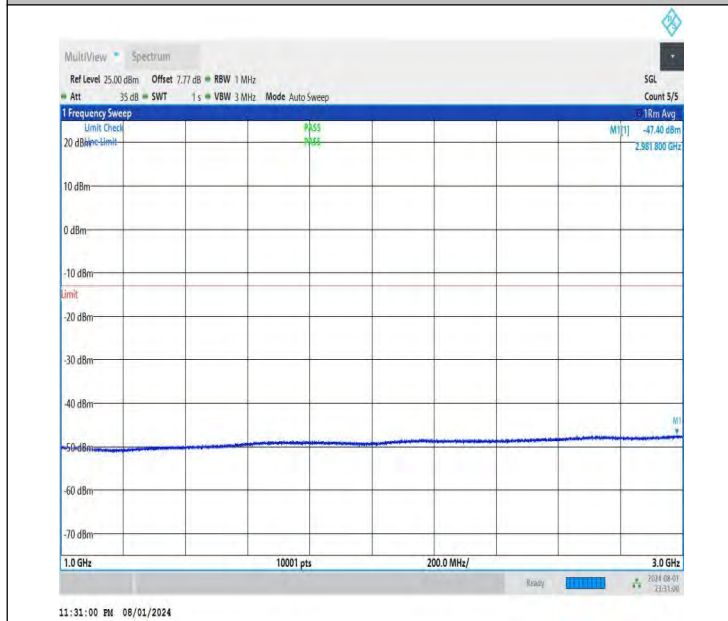
NTNV-DC_26A-n78A(3700-3800)-PC3-30-5+60-M+L-QPSK-IDL E-DFT-BPSK-Edge_1RB_Right-1000-3000-PASS
