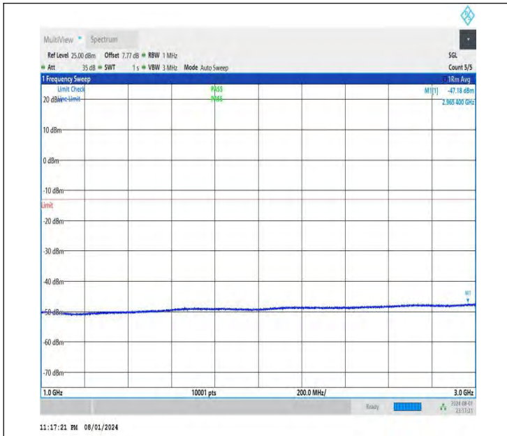
NTNV-DC_26A-n78A(3700-3800)-PC3-30-5+50-M+L-QPSK-IDL E-DFT-QPSK-Edge_1RB_Right-1000-3000-PASS
