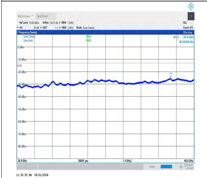
NTNV-DC_26A-n78A(3700-3800)-PC3-30-5+60-M+M-QPSK-IDL E-DFT-BPSK-Edge_1RB_Left-26000-40000-PASS
