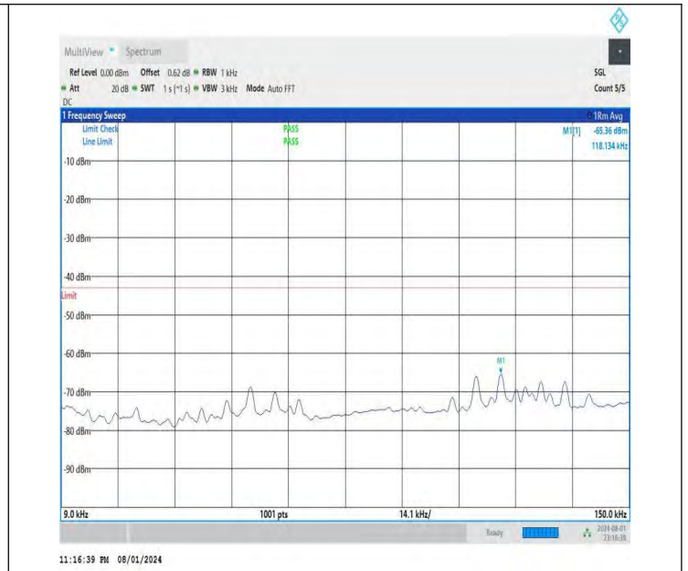
NTNV-DC_26A-n78A(3700-3800)-PC3-30-5+50-M+L-QPSK-IDLE -DFT-QPSK-Edge_1RB_Right-0.009-0.15-PASS
