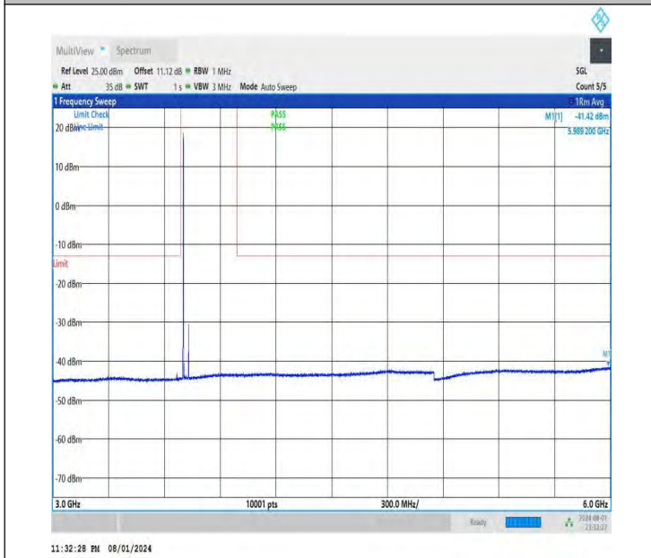
NTNV-DC_26A-n78A(3700-3800)-PC3-30-5+60-M+L-QPSK-IDL E-DFT-QPSK-Edge_1RB_Left-3000-6000-PASS
