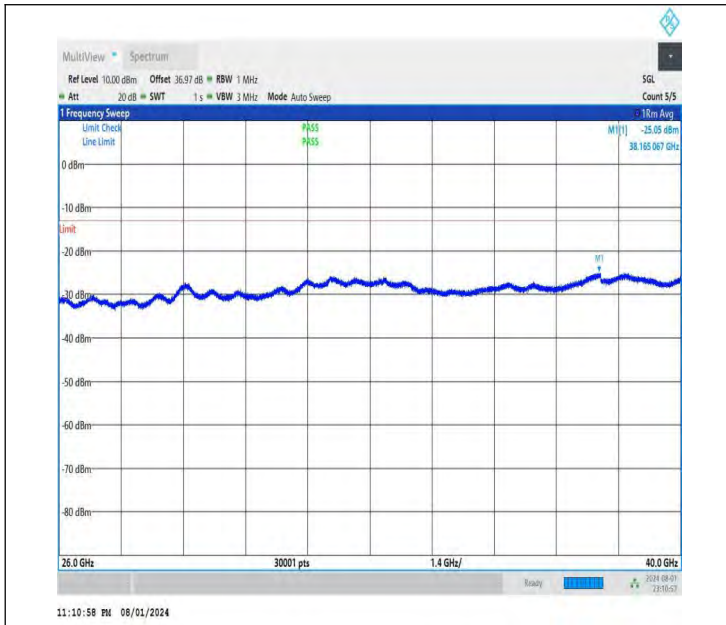
NTNV-DC_26A-n78A(3700-3800)-PC3-30-5+40-M+H-QPSK-IDL E-DFT-QPSK-Edge_1RB_Left-26000-40000-PASS
