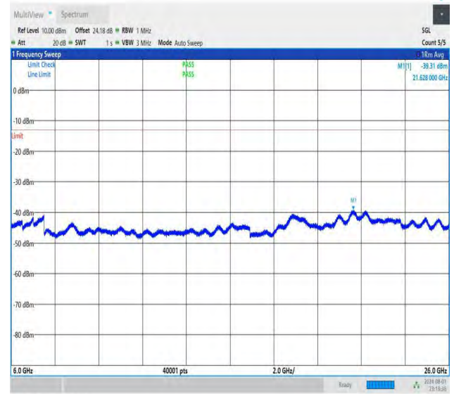
NTNV-DC_26A-n78A(3700-3800)-PC3-30-5+50-M+L-QPSK-IDLE -DFT-BPSK-Edge_1RB_Left-6000-26000-PASS
