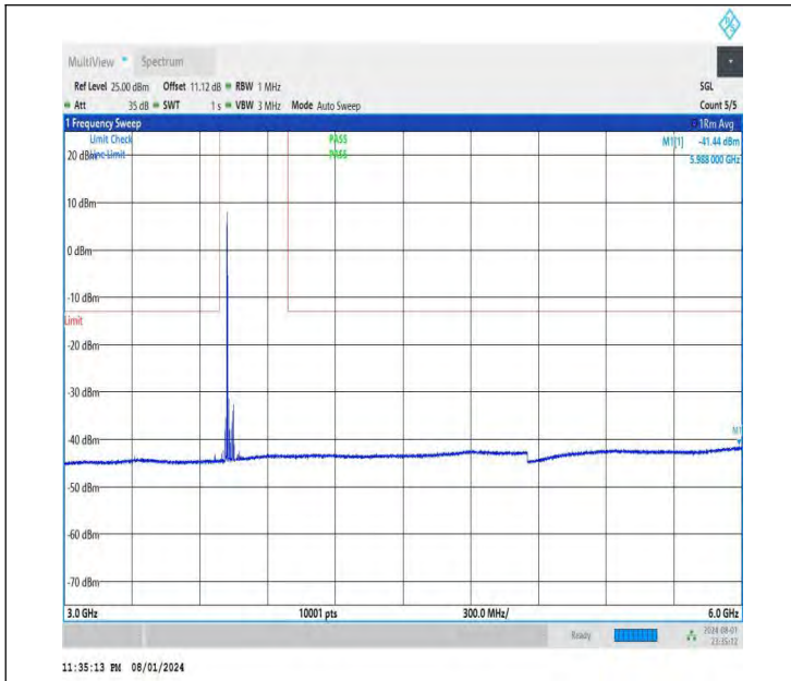
NTNV-DC_26A-n78A(3700-3800)-PC3-30-5+60-M+M-QPSK-IDL E-DFT-BPSK-Edge_1RB_Left-3000-6000-PASS
