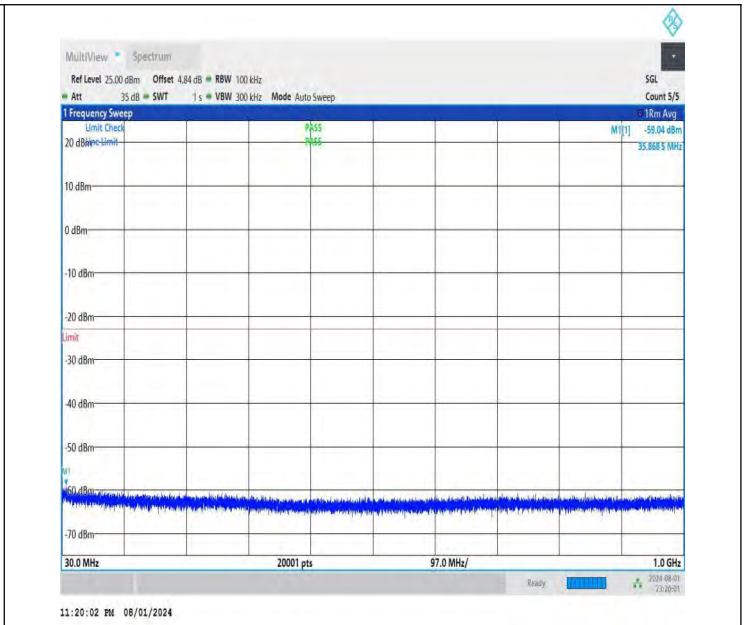
NTNV-DC_26A-n78A(3700-3800)-PC3-30-5+50-M+M-QPSK-IDLE -DFT-BPSK-Edge_1RB_Right-30-1000-PASS
