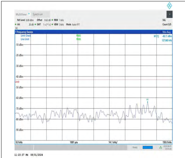
NTNV-DC_26A-n78A(3700-3800)-PC3-30-5+50-M+H-QPSK-IDL E-DFT-BPSK-Edge_1RB_Left-0.009-0.15-PASS
