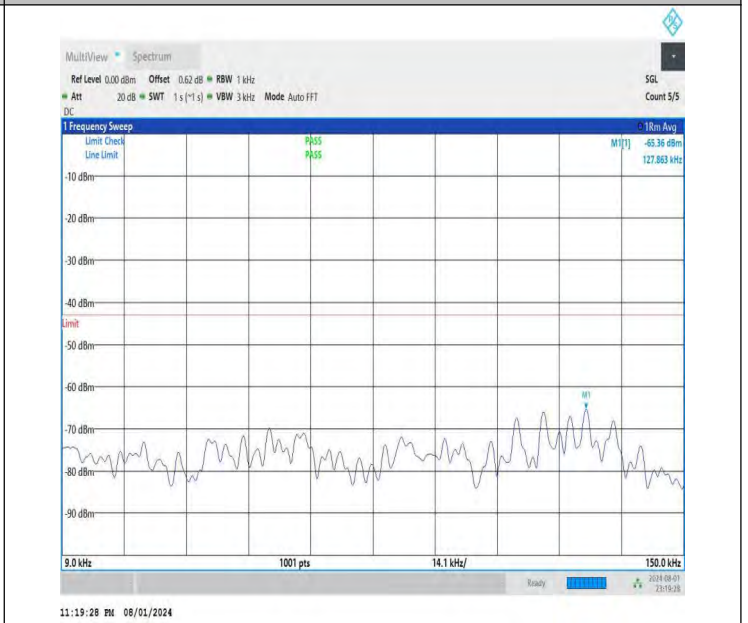
NTNV-DC_26A-n78A(3700-3800)-PC3-30-5+50-M+M-QPSK-IDLE -DFT-BPSK-Edge_1RB_Right-0.009-0.15-PASS
