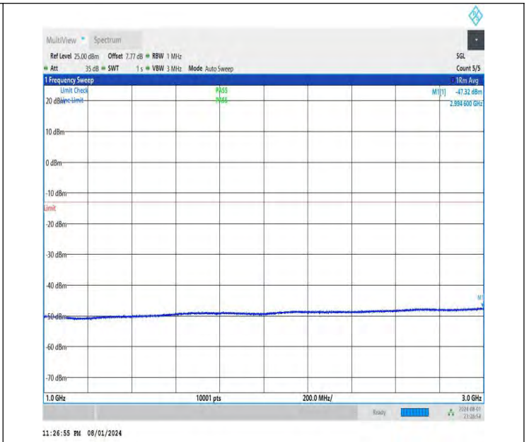
NTNV-DC_26A-n78A(3700-3800)-PC3-30-5+50-M+H-QPSK-IDLE -DFT-QPSK-Edge_1RB_Left-1000-3000-PASS
