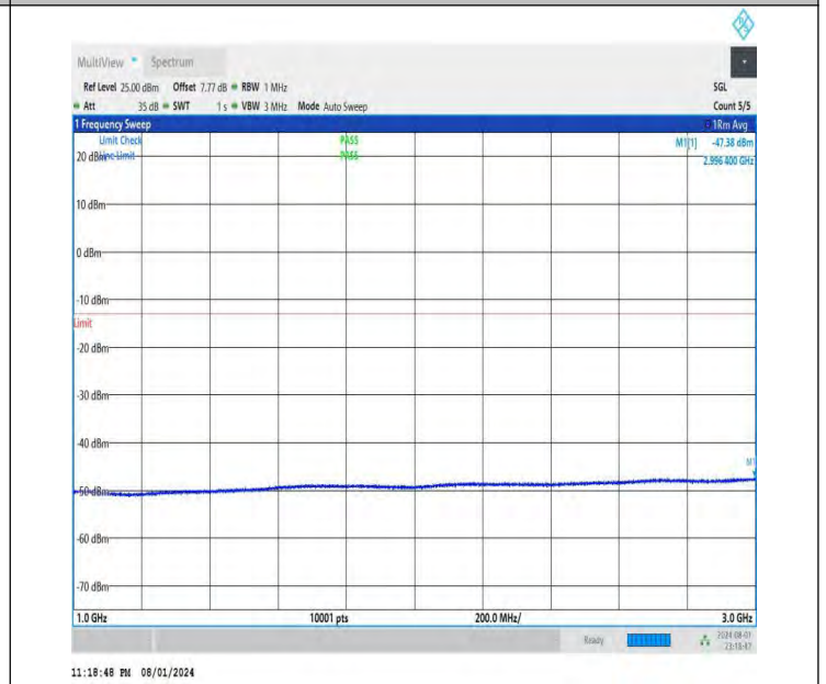
NTNV-DC_26A-n78A(3700-3800)-PC3-30-5+50-M+M-QPSK-IDLE -DFT-BPSK-Edge_1RB_Left-1000-3000-PASS
