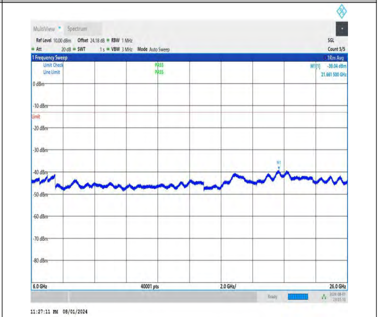
NTNV-DC_26A-n78A(3700-3800)-PC3-30-5+50-M+H-QPSK-IDLE -DFT-QPSK-Edge_1RB_Left-6000-26000-PASS
