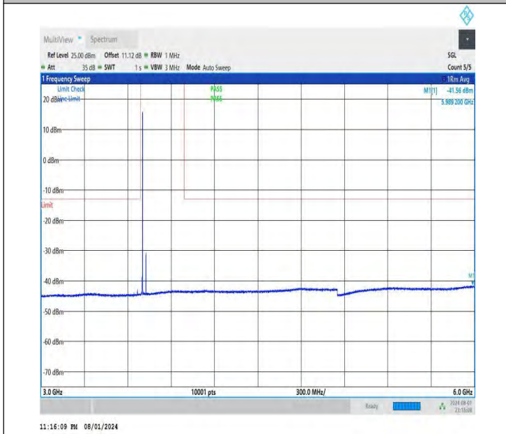
NTNV-DC_26A-n78A(3700-3800)-PC3-30-5+50-M+L-QPSK-IDL E-DFT-QPSK-Edge_1RB_Left-3000-6000-PASS
