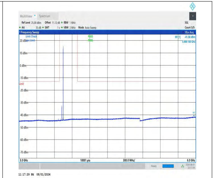
NTNV-DC_26A-n78A(3700-3800)-PC3-30-5+50-M+L-QPSK-IDLE -DFT-QPSK-Edge_1RB_Right-3000-6000-PASS
