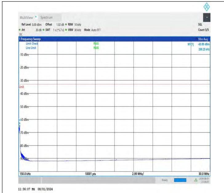
NTNV-DC_26A-n78A(3700-3800)-PC3-30-5+60-M+M-QPSK-IDL E-DFT-BPSK-Edge_1RB_Right-0.15-30-PASS
