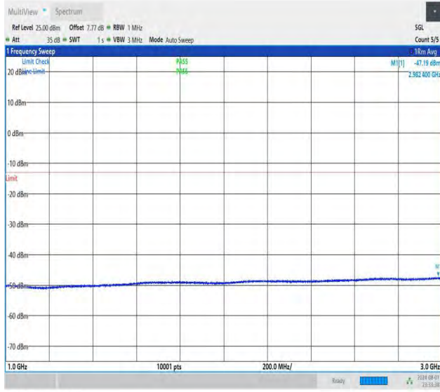
NTNV-DC_26A-n78A(3700-3800)-PC3-30-5+60-M+L-QPSK-IDL E-DFT-QPSK-Edge_1RB_Right-1000-3000-PASS
