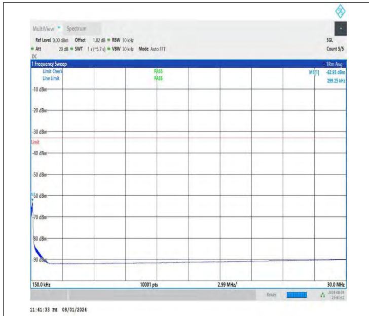
NTNV-DC_26A-n78A(3700-3800)-PC3-30-5+60-M+H-QPSK-IDL E-DFT-BPSK-Edge_1RB_Right-0.15-30-PASS
