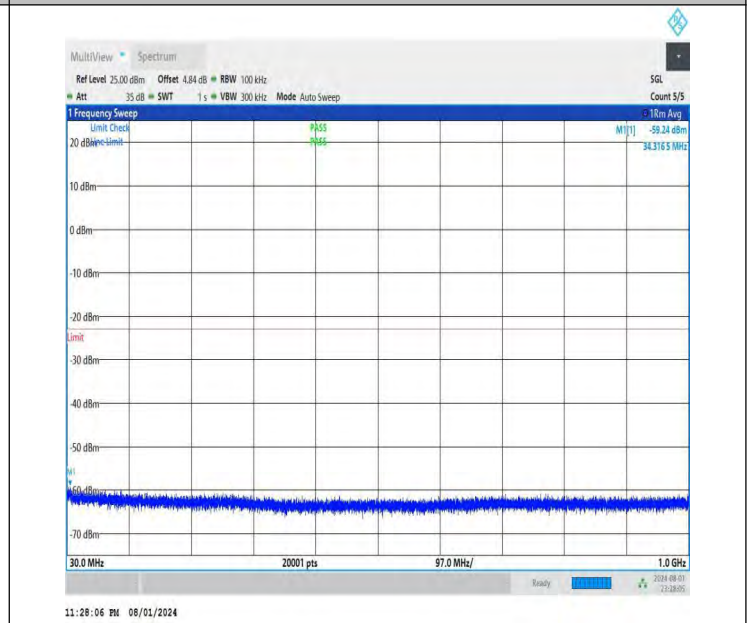
NTNV-DC_26A-n78A(3700-3800)-PC3-30-5+50-M+H-QPSK-IDLE -DFT-QPSK-Edge_1RB_Right-30-1000-PASS
