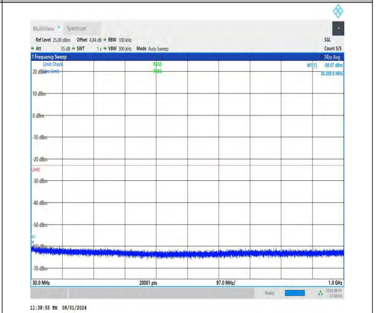
NTNV-DC_26A-n78A(3700-3800)-PC3-30-5+60-M+M-QPSK-IDLE -DFT-QPSK-Edge_1RB_Right-30-1000-PASS
