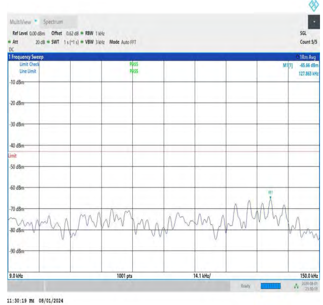
NTNV-DC_26A-n78A(3700-3800)-PC3-30-5+60-M+L-QPSK-IDLE -DFT-BPSK-Edge_1RB_Right-0.009-0.15-PASS
