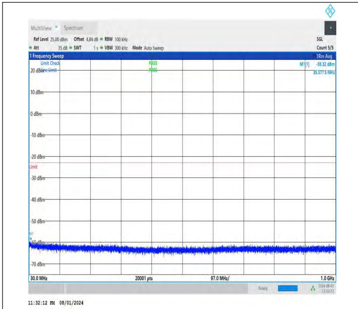
NTNV-DC_26A-n78A(3700-3800)-PC3-30-5+60-M+L-QPSK-IDL E-DFT-QPSK-Edge_1RB_Left-30-1000-PASS
