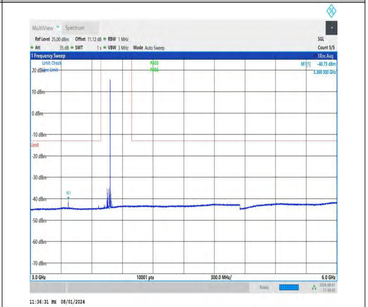
NTNV-DC_26A-n78A(3700-3800)-PC3-30-5+60-M+M-QPSK-IDLE -DFT-BPSK-Edge_1RB_Right-3000-6000-PASS
