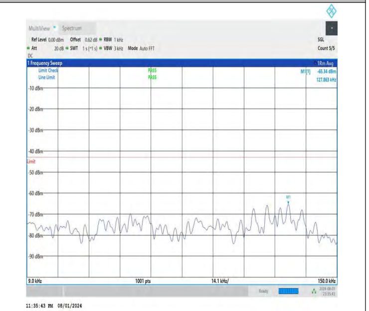
NTNV-DC_26A-n78A(3700-3800)-PC3-30-5+60-M+M-QPSK-IDLE -DFT-BPSK-Edge_1RB_Right-0.009-0.15-PASS
