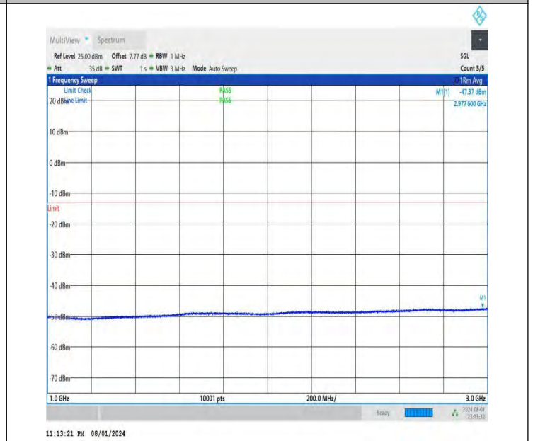
NTNV-DC_26A-n78A(3700-3800)-PC3-30-5+50-M+L-QPSK-IDLE -DFT-BPSK-Edge_1RB_Left-1000-3000-PASS
