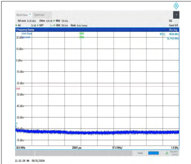
NTNV-DC_26A-n78A(3700-3800)-PC3-30-5+50-M+M-QPSK-IDL E-DFT-QPSK-Edge_1RB_Left-30-1000-PASS
