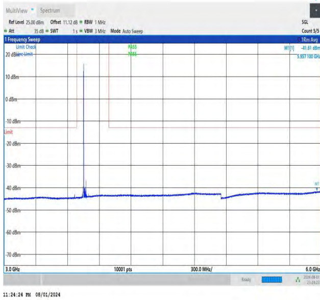
NTNV-DC_26A-n78A(3700-3800)-PC3-30-5+50-M+H-QPSK-IDL E-DFT-BPSK-Edge_1RB_Left-3000-6000-PASS
