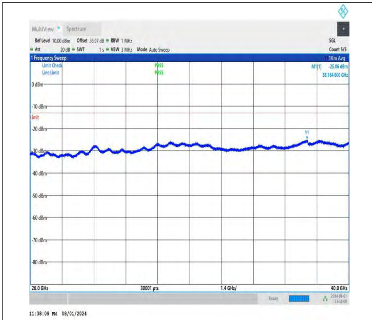
NTNV-DC_26A-n78A(3700-3800)-PC3-30-5+60-M+M-QPSK-IDL E-DFT-QPSK-Edge_1RB_Left-26000-40000-PASS
