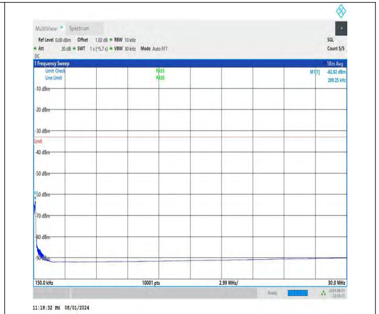
NTNV-DC_26A-n78A(3700-3800)-PC3-30-5+50-M+M-QPSK-IDLE -DFT-BPSK-Edge_1RB_Left-0.15-30-PASS
