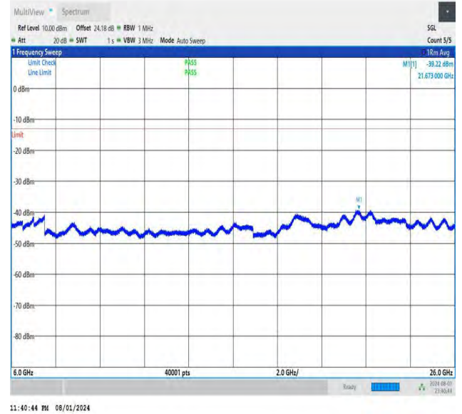
NTNV-DC_26A-n78A(3700-3800)-PC3-30-5+60-M+H-QPSK-IDLE -DFT-BPSK-Edge_1RB_Left-6000-26000-PASS
