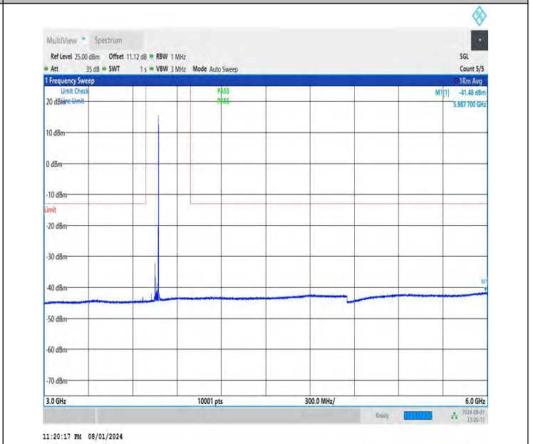
NTNV-DC_26A-n78A(3700-3800)-PC3-30-5+50-M+M-QPSK-IDLE -DFT-BPSK-Edge_1RB_Right-3000-6000-PASS
