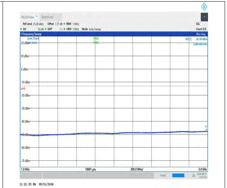
NTNV-DC_26A-n78A(3700-3800)-PC3-30-5+50-M+M-QPSK-IDLE -DFT-QPSK-Edge_1RB_Left-1000-3000-PASS
