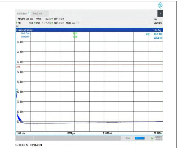
NTNV-DC_26A-n78A(3700-3800)-PC3-30-5+60-M+L-QPSK-IDLE -DFT-BPSK-Edge_1RB_Left-0.15-30-PASS
