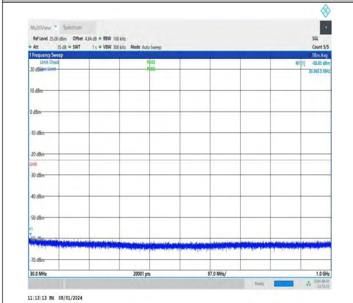
NTNV-DC_26A-n78A(3700-3800)-PC3-30-5+50-M+L-QPSK-IDL E-DFT-BPSK-Edge_1RB_Left-30-1000-PASS
