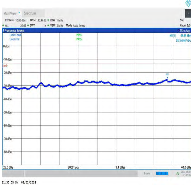
NTNV-DC_26A-n78A(3700-3800)-PC3-30-5+60-M+L-QPSK-IDL E-DFT-BPSK-Edge_1RB_Left-26000-40000-PASS
