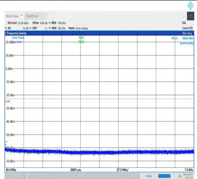
NTNV-DC_26A-n78A(3700-3800)-PC3-30-5+60-M+L-QPSK-IDLE -DFT-QPSK-Edge_1RB_Right-0.009-0.15-PASS
