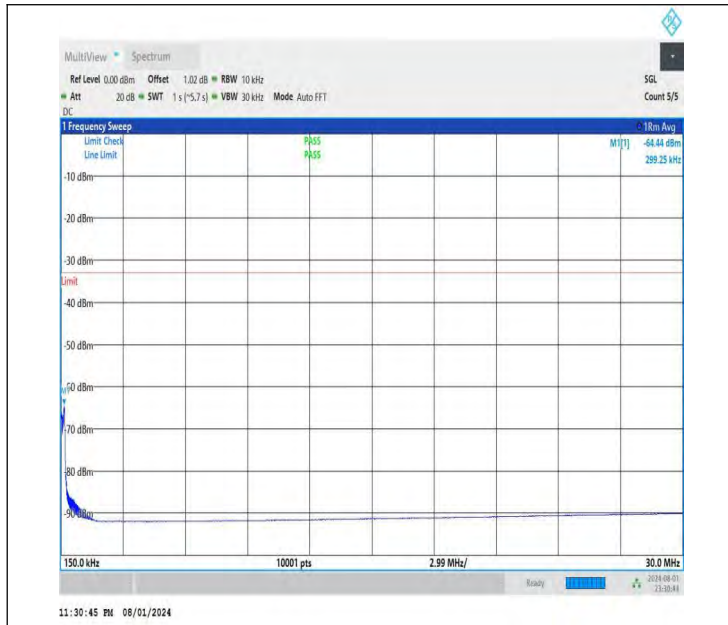
NTNV-DC_26A-n78A(3700-3800)-PC3-30-5+60-M+L-QPSK-IDL E-DFT-BPSK-Edge_1RB_Right-0.15-30-PASS
