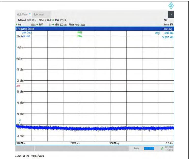
NTNV-DC_26A-n78A(3700-3800)-PC3-30-5+60-M+M-QPSK-IDLE -DFT-BPSK-Edge_1RB_Right-30-1000-PASS
