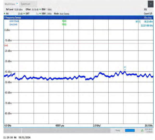
NTNV-DC_26A-n78A(3700-3800)-PC3-30-5+60-M+L-QPSK-IDLE -DFT-BPSK-Edge_1RB_Left-6000-26000-PASS
