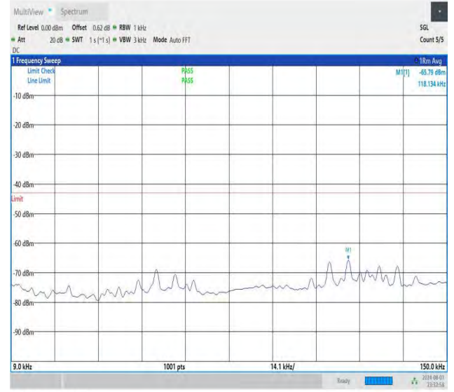
NTNV-DC_26A-n78A(3700-3800)-PC3-30-5+60-M+L-QPSK-IDLE -DFT-QPSK-Edge_1RB_Right-0.009-0.15-PASS
