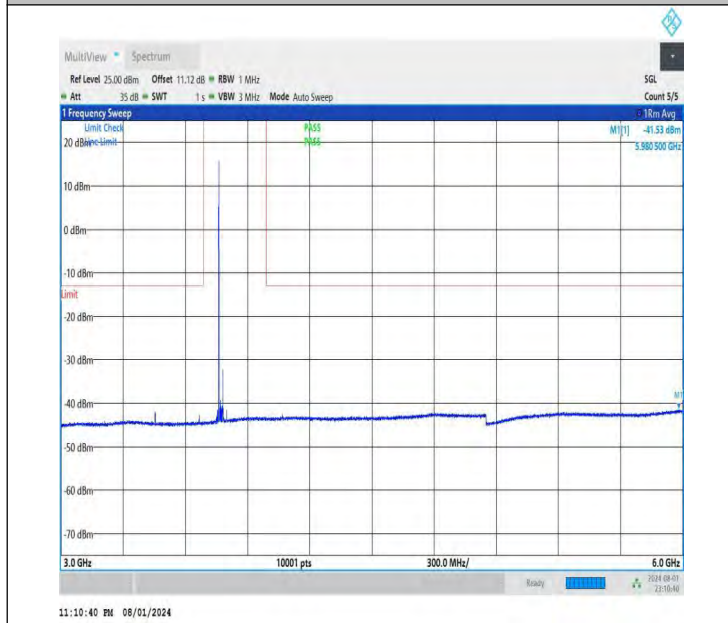
NTNV-DC_26A-n78A(3700-3800)-PC3-30-5+40-M+H-QPSK-IDL E-DFT-QPSK-Edge_1RB_Left-3000-6000-PASS
