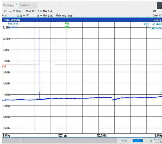
NTNV-DC_26A-n78A(3700-3800)-PC3-30-5+50-M+L-QPSK-IDL E-DFT-BPSK-Edge_1RB_Left-3000-6000-PASS
