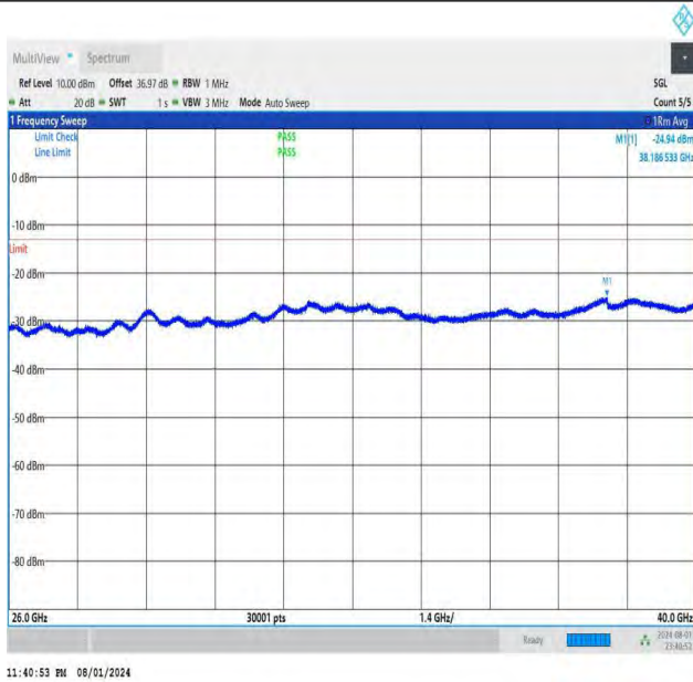
NTNV-DC_26A-n78A(3700-3800)-PC3-30-5+60-M+H-QPSK-IDL E-DFT-BPSK-Edge_1RB_Left-26000-40000-PASS
