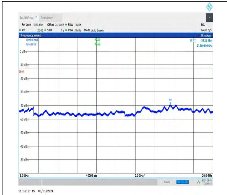
NTNV-DC_26A-n78A(3700-3800)-PC3-30-5+60-M+L-QPSK-IDL E-DFT-BPSK-Edge_1RB_Right-6000-26000-PASS
