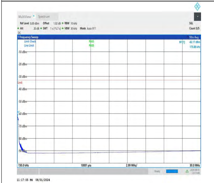
NTNV-DC_26A-n78A(3700-3800)-PC3-30-5+50-M+L-QPSK-IDL E-DFT-QPSK-Edge_1RB_Right-0.15-30-PASS
