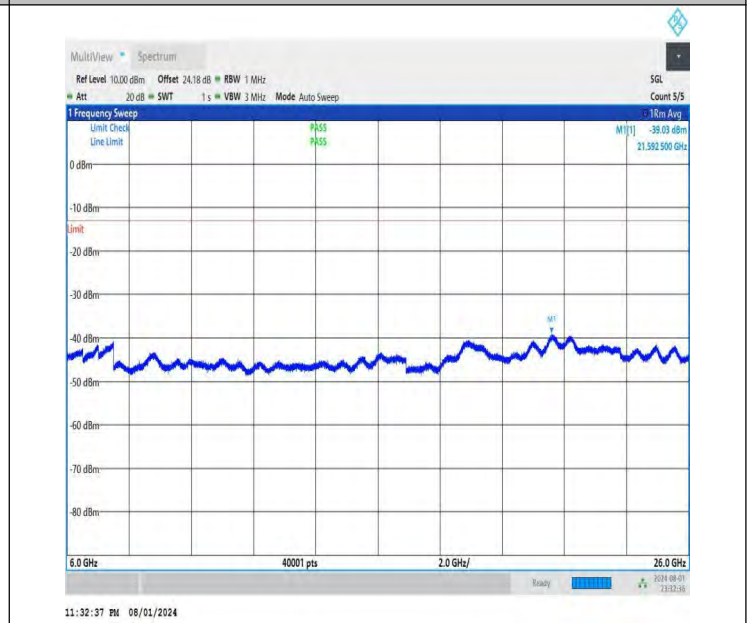
NTNV-DC_26A-n78A(3700-3800)-PC3-30-5+60-M+L-QPSK-IDLE -DFT-QPSK-Edge_1RB_Left-6000-26000-PASS
