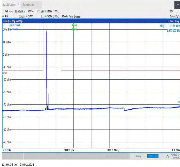
NTNV-DC_26A-n78A(3700-3800)-PC3-30-5+60-M+H-QPSK-IDL E-DFT-BPSK-Edge_1RB_Left-3000-6000-PASS
