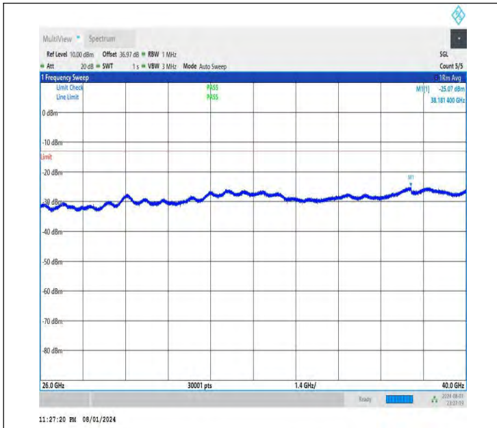
NTNV-DC_26A-n78A(3700-3800)-PC3-30-5+50-M+H-QPSK-IDL E-DFT-QPSK-Edge_1RB_Left-26000-40000-PASS
