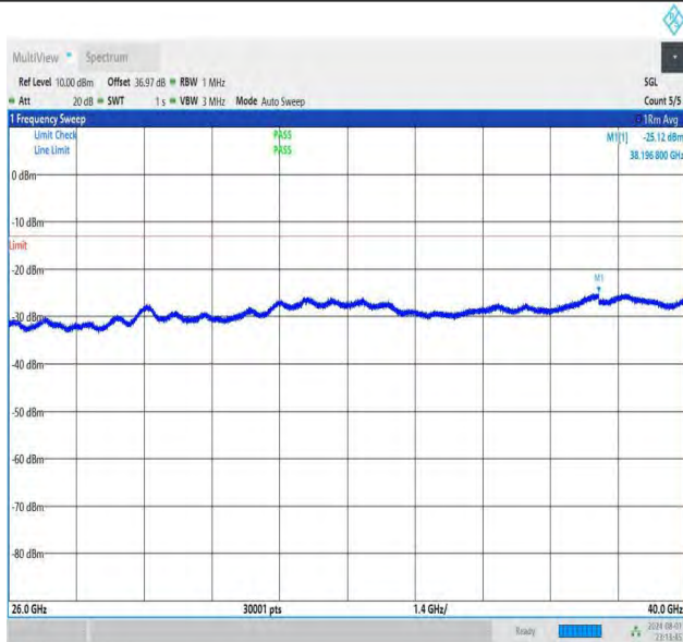
NTNV-DC_26A-n78A(3700-3800)-PC3-30-5+50-M+L-QPSK-IDL E-DFT-BPSK-Edge_1RB_Left-3000-6000-PASS
