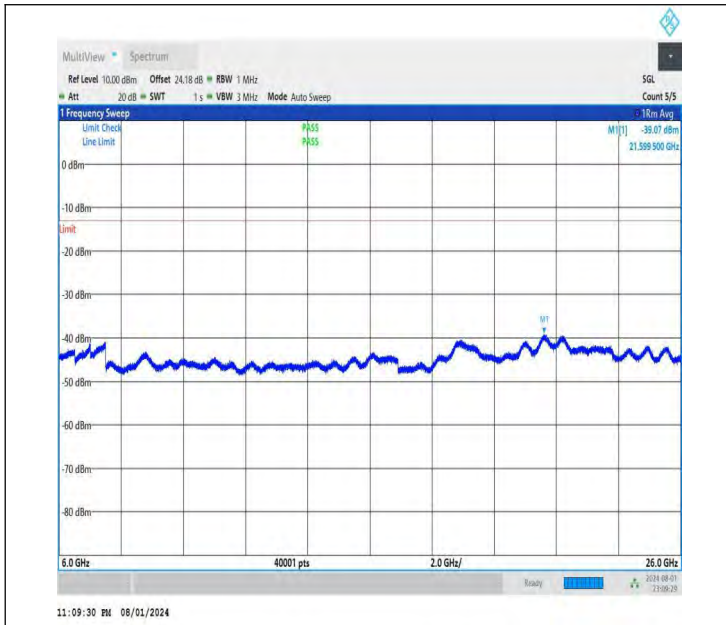
NTNV-DC_26A-n78A(3700-3800)-PC3-30-5+40-M+H-QPSK-IDL E-DFT-BPSK-Edge_1RB_Right-6000-26000-PASS
