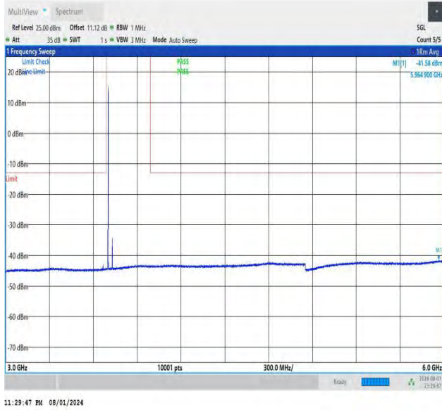
NTNV-DC_26A-n78A(3700-3800)-PC3-30-5+60-M+L-QPSK-IDL E-DFT-BPSK-Edge_1RB_Left-3000-6000-PASS
