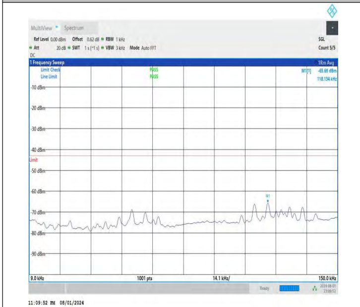
NTNV-DC_26A-n78A(3700-3800)-PC3-30-5+40-M+H-QPSK-IDL E-DFT-QPSK-Edge_1RB_Left-0.009-0.15-PASS
