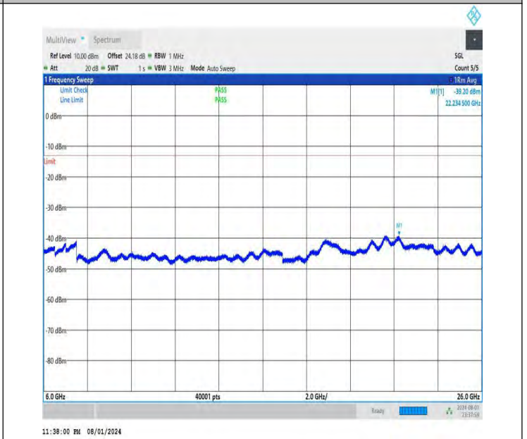
NTNV-DC_26A-n78A(3700-3800)-PC3-30-5+60-M+M-QPSK-IDLE -DFT-QPSK-Edge_1RB_Left-6000-26000-PASS
