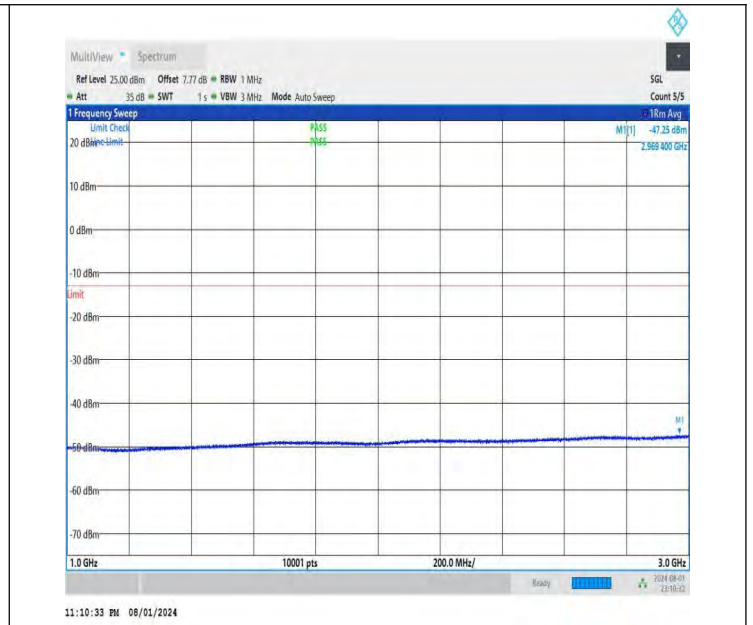
NTNV-DC_26A-n78A(3700-3800)-PC3-30-5+40-M+H-QPSK-IDLE -DFT-QPSK-Edge_1RB_Left-1000-3000-PASS
