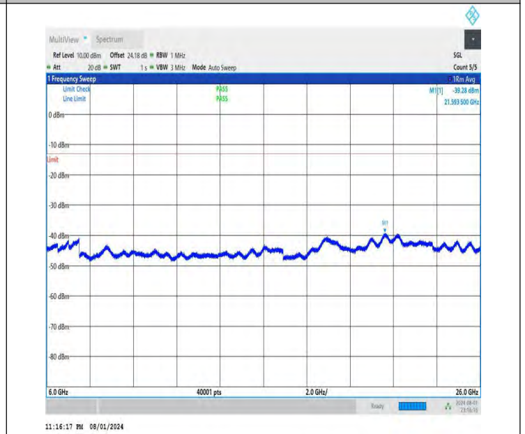
NTNV-DC_26A-n78A(3700-3800)-PC3-30-5+50-M+L-QPSK-IDLE -DFT-QPSK-Edge_1RB_Left-6000-26000-PASS
