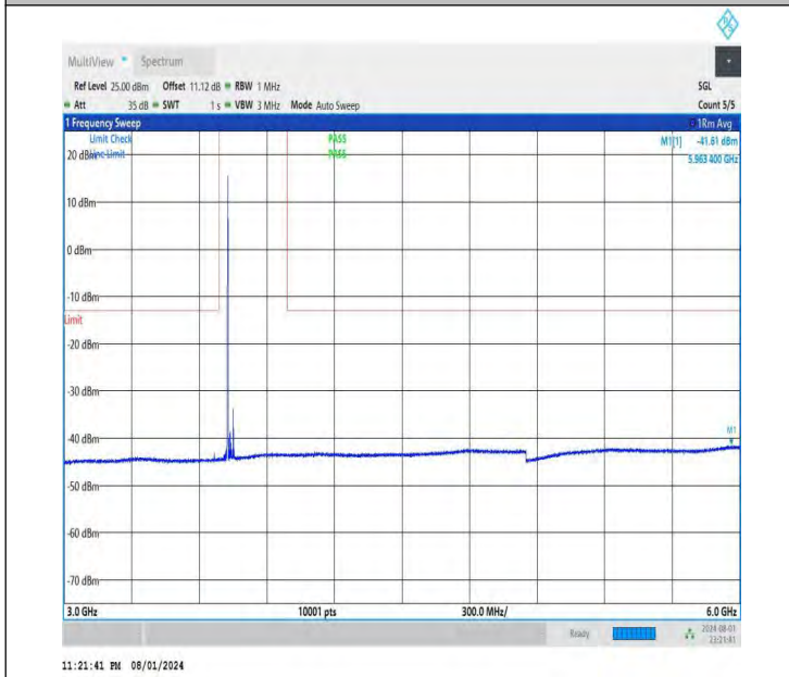
NTNV-DC_26A-n78A(3700-3800)-PC3-30-5+50-M+M-QPSK-IDL E-DFT-QPSK-Edge_1RB_Left-3000-6000-PASS
