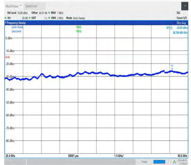
NTNV-DC_26A-n78A(3700-3800)-PC3-30-5+50-M+M-QPSK-IDLE -DFT-BPSK-Edge_1RB_Right-26000-40000-PASS
