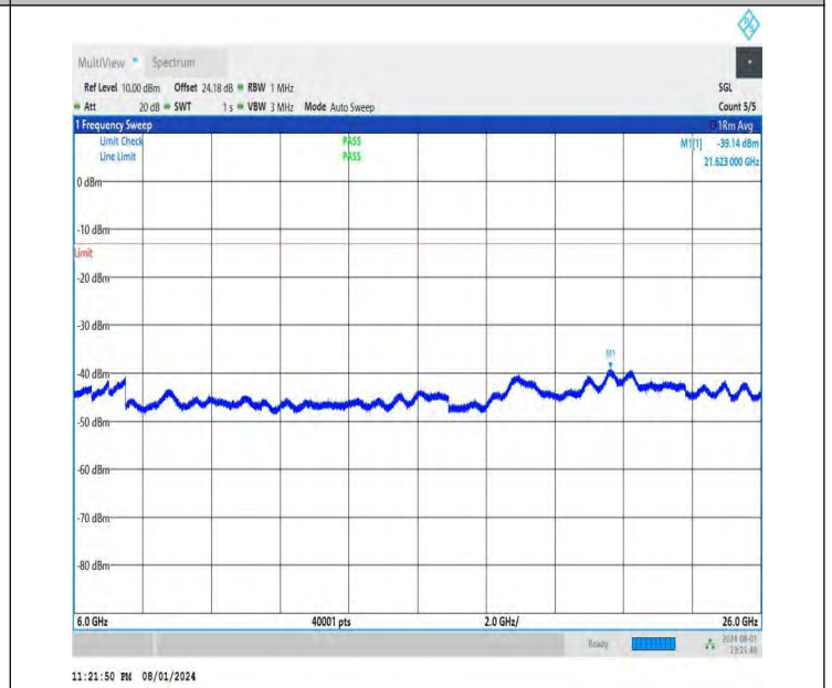
NTNV-DC_26A-n78A(3700-3800)-PC3-30-5+50-M+M-QPSK-IDLE -DFT-QPSK-Edge_1RB_Left-6000-26000-PASS
