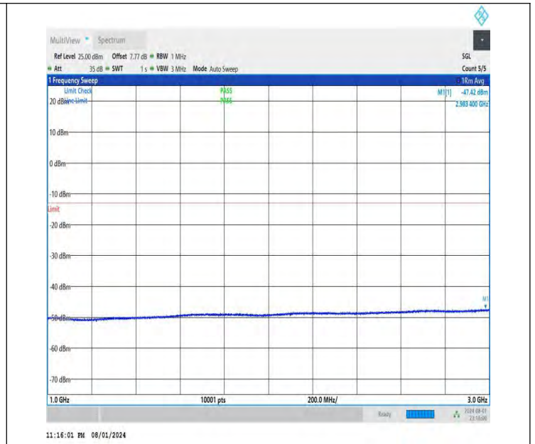
NTNV-DC_26A-n78A(3700-3800)-PC3-30-5+50-M+L-QPSK-IDLE -DFT-QPSK-Edge_1RB_Left-1000-3000-PASS
