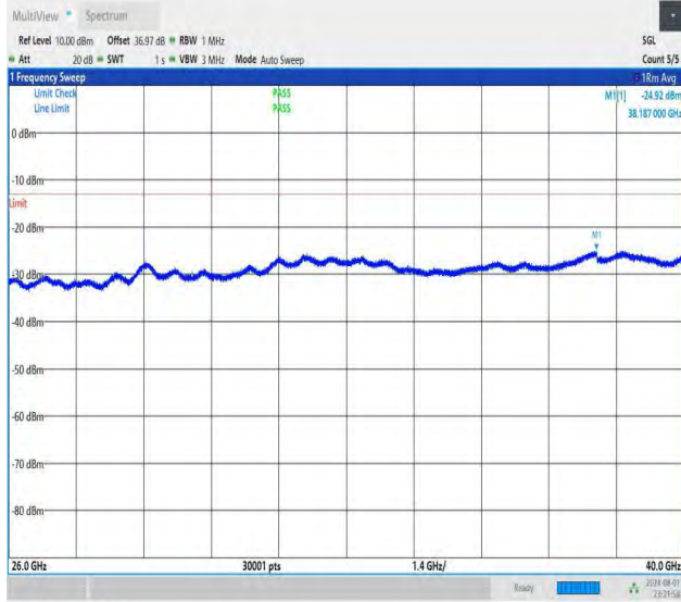
NTNV-DC_26A-n78A(3700-3800)-PC3-30-5+50-M+M-QPSK-IDL E-DFT-QPSK-Edge_1RB_Left-26000-40000-PASS
