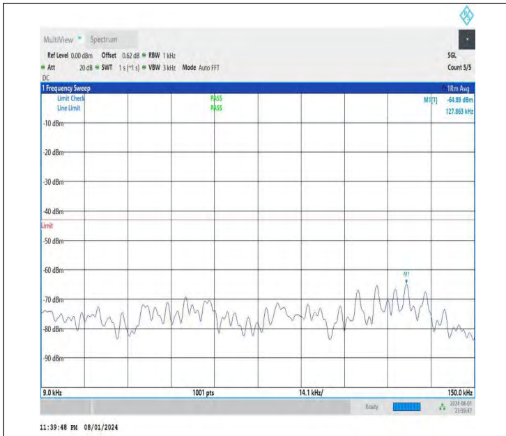
NTNV-DC_26A-n78A(3700-3800)-PC3-30-5+60-M+H-QPSK-IDL E-DFT-BPSK-Edge_1RB_Left-0.009-0.15-PASS
