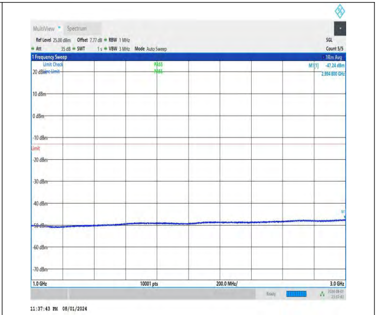
NTNV-DC_26A-n78A(3700-3800)-PC3-30-5+60-M+M-QPSK-IDLE -DFT-QPSK-Edge_1RB_Left-1000-3000-PASS
