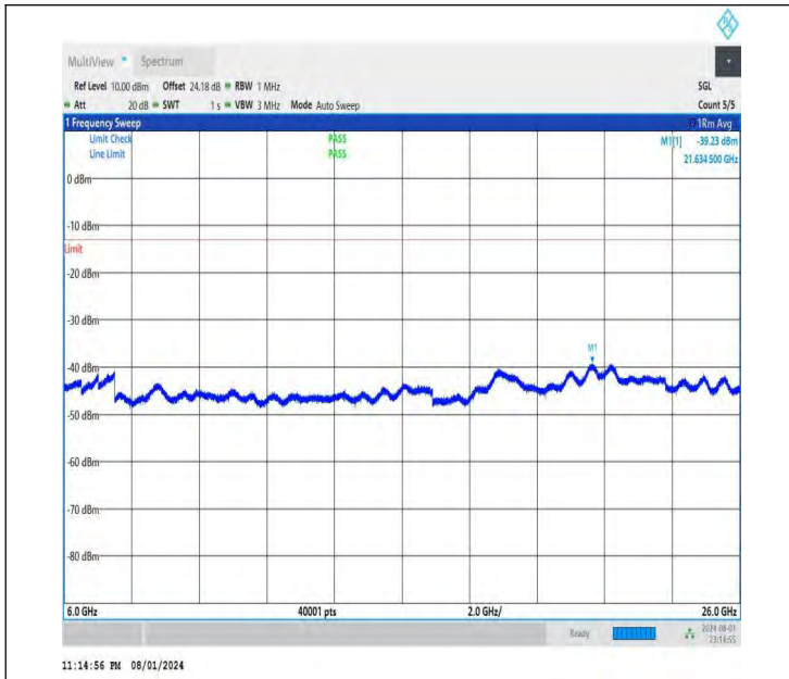
NTNV-DC_26A-n78A(3700-3800)-PC3-30-5+50-M+L-QPSK-IDL E-DFT-BPSK-Edge_1RB_Right-6000-26000-PASS
