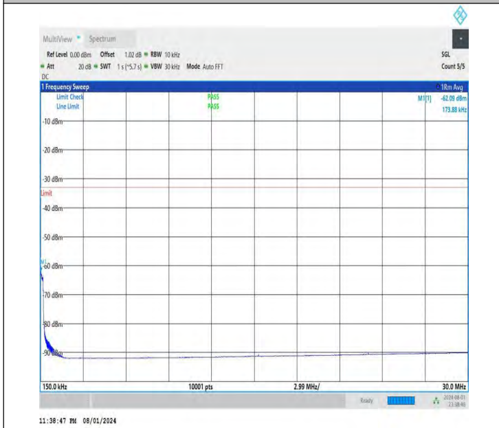
NTNV-DC_26A-n78A(3700-3800)-PC3-30-5+60-M+M-QPSK-IDL E-DFT-QPSK-Edge_1RB_Right-0.15-30-PASS
