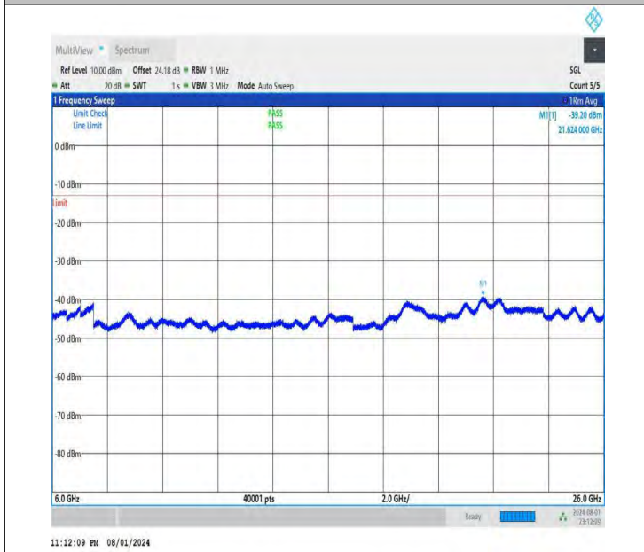
NTNV-DC_26A-n78A(3700-3800)-PC3-30-5+40-M+H-QPSK-IDL E-DFT-QPSK-Edge_1RB_Right-6000-26000-PASS
