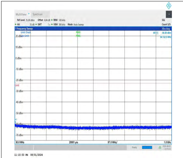
NTNV-DC_26A-n78A(3700-3800)-PC3-30-5+50-M+L-QPSK-IDL E-DFT-QPSK-Edge_1RB_Left-30-1000-PASS
