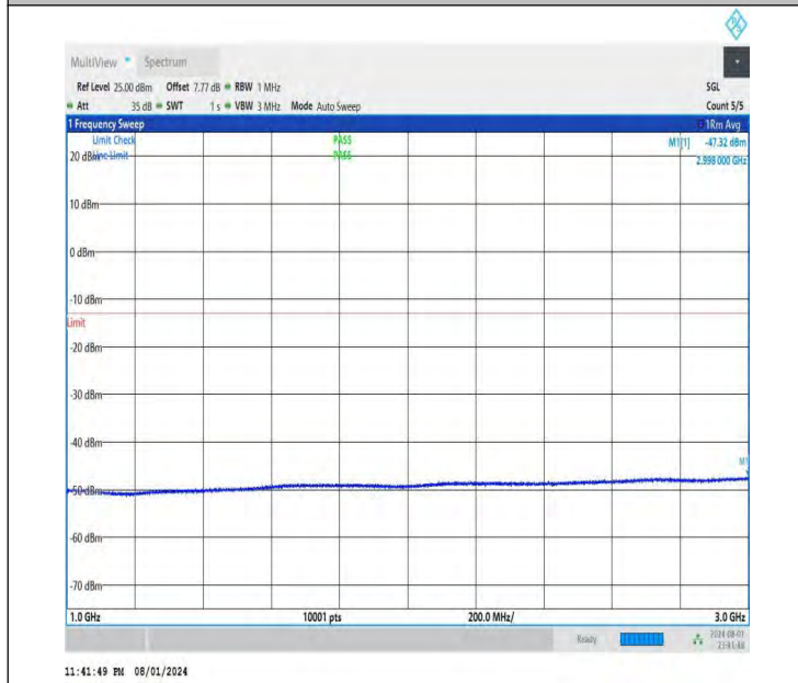
NTNV-DC_26A-n78A(3700-3800)-PC3-30-5+60-M+H-QPSK-IDL E-DFT-BPSK-Edge_1RB_Right-1000-3000-PASS
