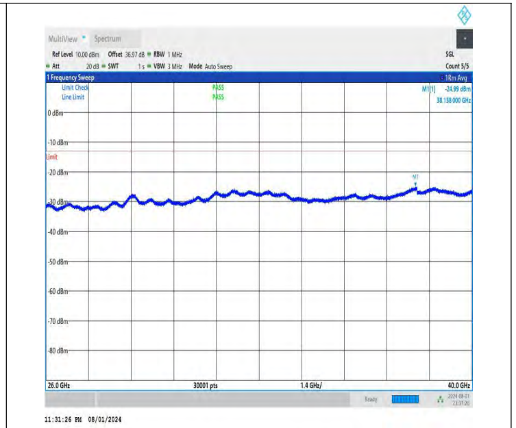
NTNV-DC_26A-n78A(3700-3800)-PC3-30-5+60-M+L-QPSK-IDLE -DFT-BPSK-Edge_1RB_Right-26000-40000-PASS
