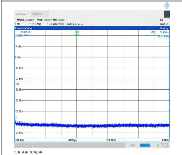
NTNV-DC_26A-n78A(3700-3800)-PC3-30-5+50-M+H-QPSK-IDL E-DFT-BPSK-Edge_1RB_Left-30-1000-PASS
