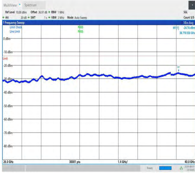
NTNV-DC_26A-n78A(3700-3800)-PC3-30-5+60-M+L-QPSK-IDL E-DFT-QPSK-Edge_1RB_Left-26000-40000-PASS
