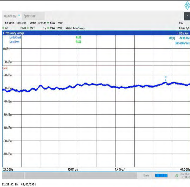
NTNV-DC_26A-n78A(3700-3800)-PC3-30-5+50-M+H-QPSK-IDL E-DFT-BPSK-Edge_1RB_Left-26000-40000-PASS
