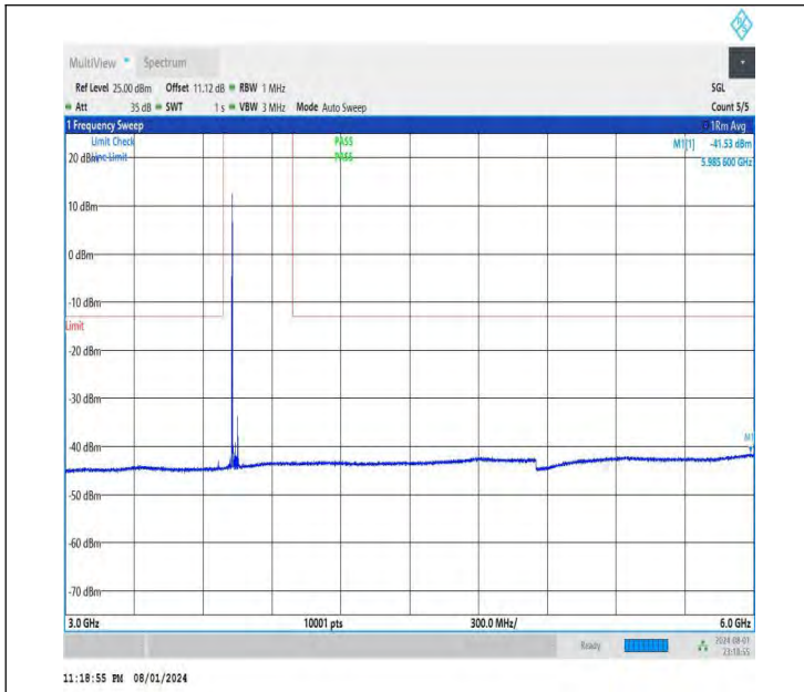
NTNV-DC_26A-n78A(3700-3800)-PC3-30-5+50-M+M-QPSK-IDL E-DFT-BPSK-Edge_1RB_Left-3000-6000-PASS
