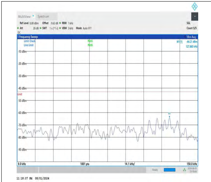
NTNV-DC_26A-n78A(3700-3800)-PC3-30-5+50-M+M-QPSK-IDL E-DFT-BPSK-Edge_1RB_Left-0.009-0.15-PASS
