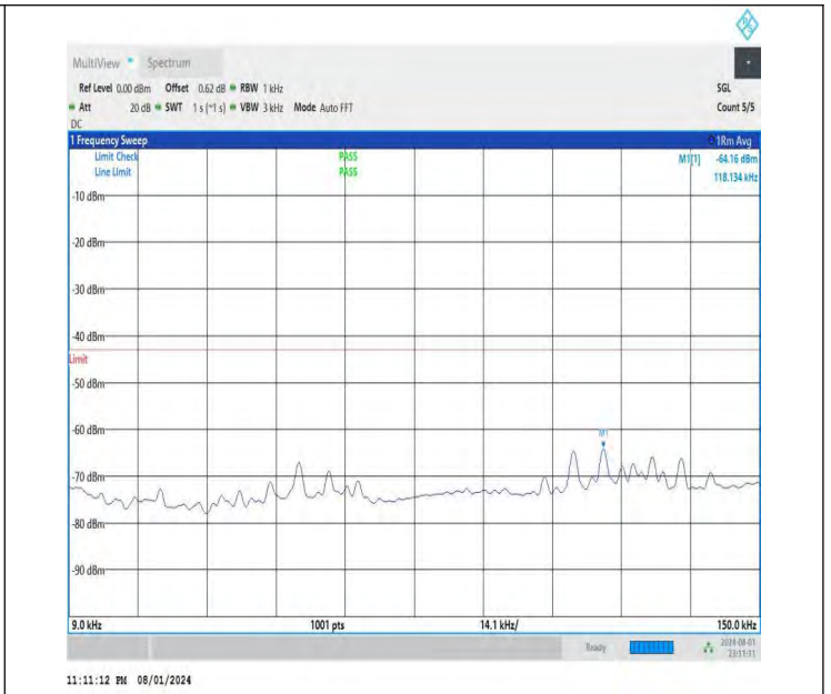
NTNV-DC_26A-n78A(3700-3800)-PC3-30-5+40-M+H-QPSK-IDLE -DFT-QPSK-Edge_1RB_Right-0.009-0.15-PASS
