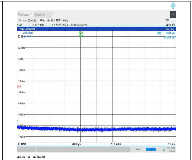
NTNV-DC_26A-n78A(3700-3800)-PC3-30-5+50-M+H-QPSK-IDLE -DFT-BPSK-Edge_1RB_Right-30-1000-PASS
