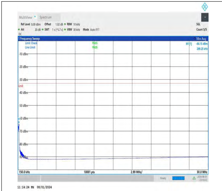
NTNV-DC_26A-n78A(3700-3800)-PC3-30-5+50-M+L-QPSK-IDL E-DFT-BPSK-Edge_1RB_Right-0.15-30-PASS
