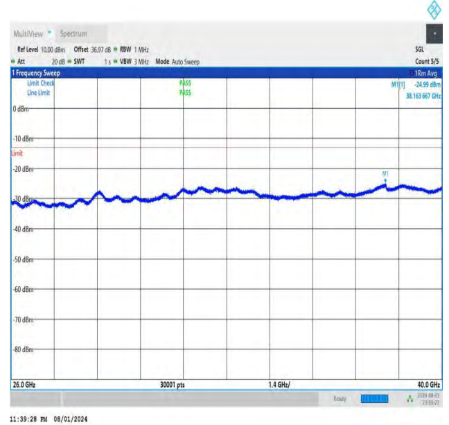
NTNV-DC_26A-n78A(3700-3800)-PC3-30-5+60-M+M-QPSK-IDLE -DFT-QPSK-Edge_1RB_Right-26000-40000-PASS
