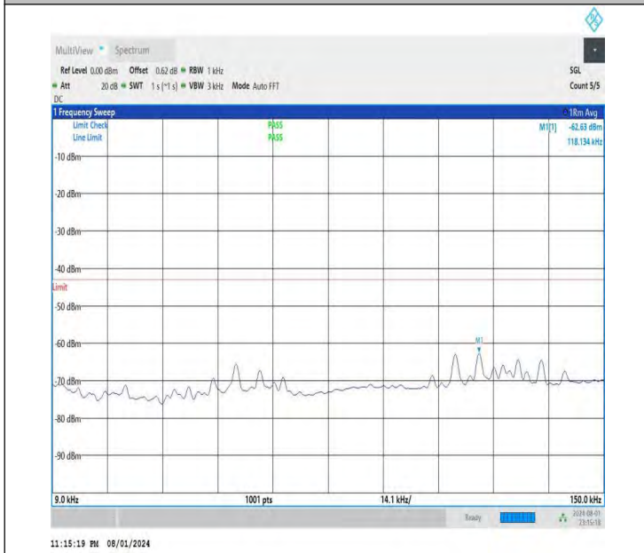
NTNV-DC_26A-n78A(3700-3800)-PC3-30-5+50-M+L-QPSK-IDL E-DFT-QPSK-Edge_1RB_Left-0.009-0.15-PASS
