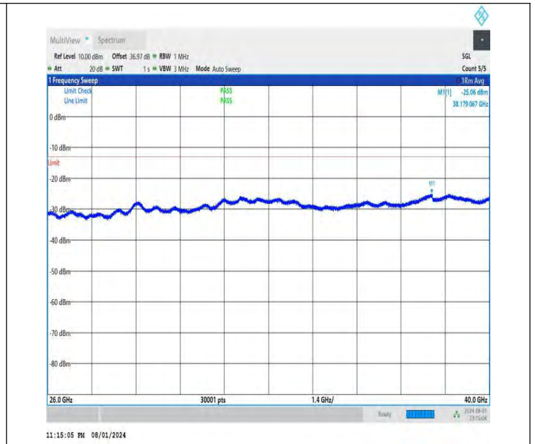
NTNV-DC_26A-n78A(3700-3800)-PC3-30-5+50-M+L-QPSK-IDLE -DFT-BPSK-Edge_1RB_Right-26000-40000-PASS
