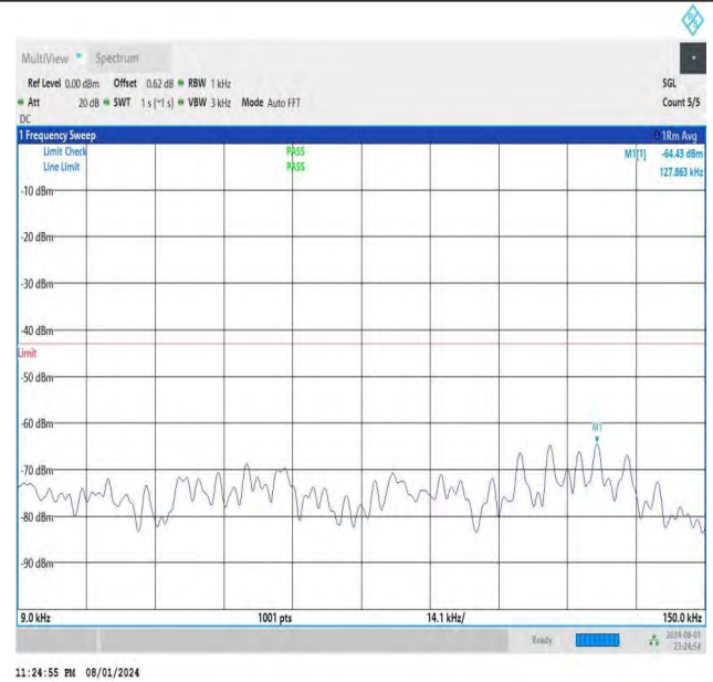
NTNV-DC_26A-n78A(3700-3800)-PC3-30-5+50-M+H-QPSK-IDLE -DFT-BPSK-Edge_1RB_Right-0.009-0.15-PASS
