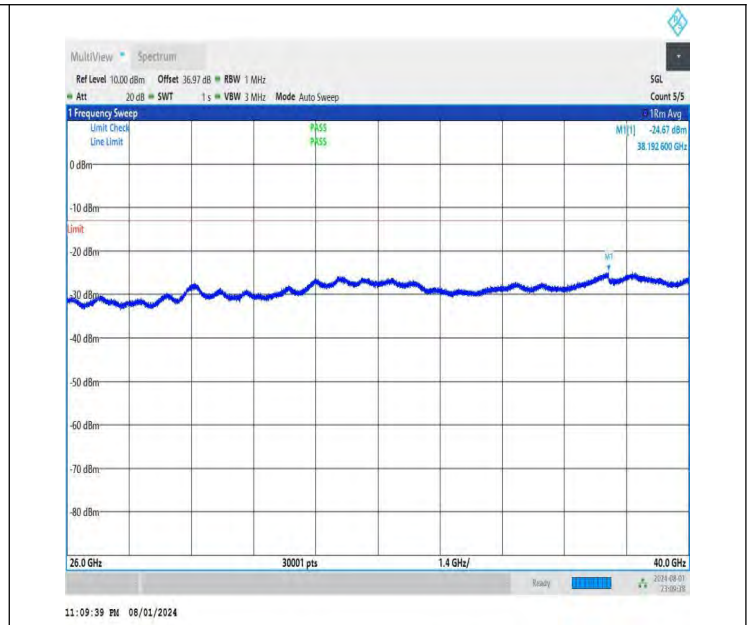
NTNV-DC_26A-n78A(3700-3800)-PC3-30-5+40-M+H-QPSK-IDLE -DFT-BPSK-Edge_1RB_Right-26000-40000-PASS
