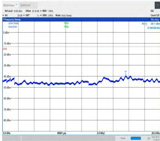
NTNV-DC_26A-n78A(3700-3800)-PC3-30-5+50-M+M-QPSK-IDL E-DFT-BPSK-Edge_1RB_Right-6000-26000-PASS
