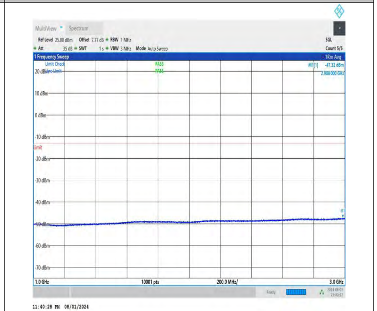
NTNV-DC_26A-n78A(3700-3800)-PC3-30-5+60-M+H-QPSK-IDLE -DFT-BPSK-Edge_1RB_Left-1000-3000-PASS
