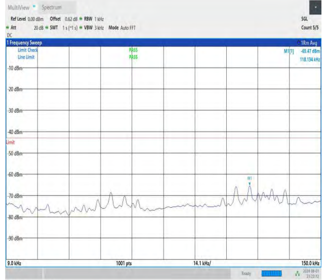
NTNV-DC_26A-n78A(3700-3800)-PC3-30-5+50-M+M-QPSK-IDLE -DFT-QPSK-Edge_1RB_Right-0.009-0.15-PASS
