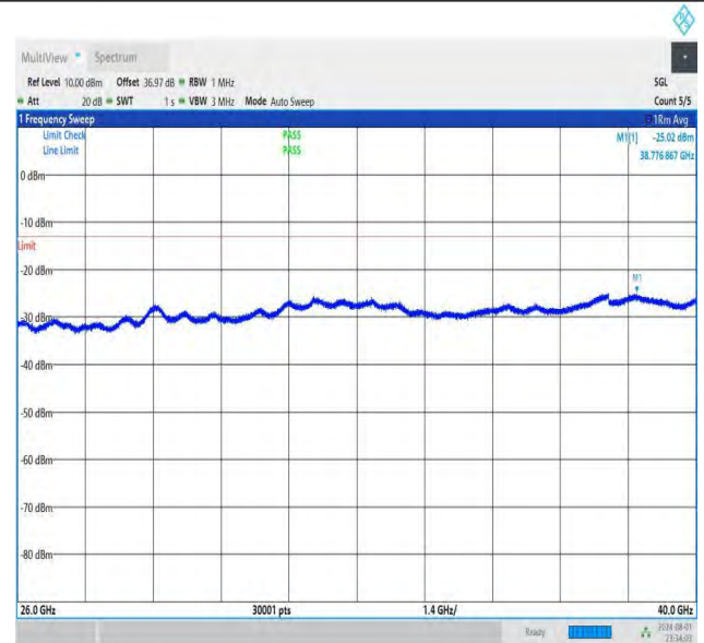
NTNV-DC_26A-n78A(3700-3800)-PC3-30-5+60-M+L-QPSK-IDLE -DFT-QPSK-Edge_1RB_Right-3000-6000-PASS
