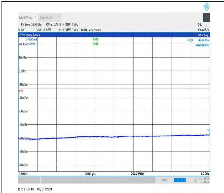
NTNV-DC_26A-n78A(3700-3800)-PC3-30-5+40-M+H-QPSK-IDL E-DFT-QPSK-Edge_1RB_Right-1000-3000-PASS
