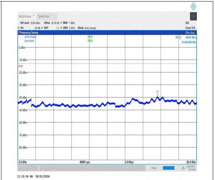
NTNV-DC_26A-n78A(3700-3800)-PC3-30-5+50-M+M-QPSK-IDLE -DFT-BPSK-Edge_1RB_Left-6000-26000-PASS
