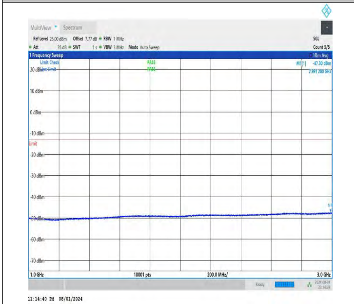
NTNV-DC_26A-n78A(3700-3800)-PC3-30-5+50-M+L-QPSK-IDL E-DFT-BPSK-Edge_1RB_Right-1000-3000-PASS
