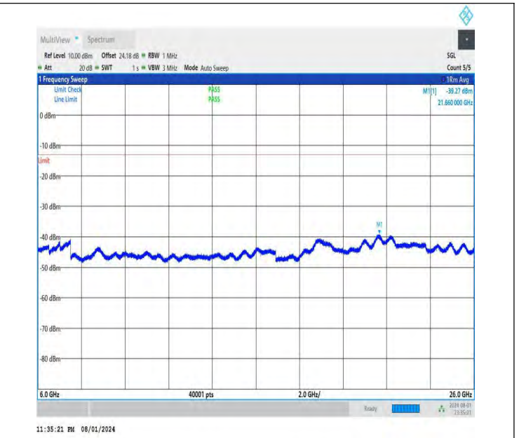
NTNV-DC_26A-n78A(3700-3800)-PC3-30-5+60-M+M-QPSK-IDLE -DFT-BPSK-Edge_1RB_Left-6000-26000-PASS
