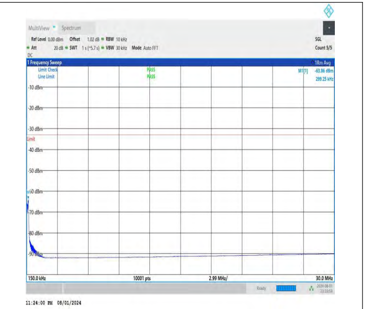
NTNV-DC_26A-n78A(3700-3800)-PC3-30-5+50-M+H-QPSK-IDLE -DFT-BPSK-Edge_1RB_Left-0.15-30-PASS
