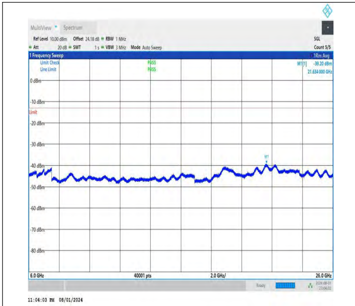
NTNV-DC_26A-n78A(3700-3800)-PC3-30-5+40-M+M-QPSK-IDL E-DFT-BPSK-Edge_1RB_Right-6000-26000-PASS
