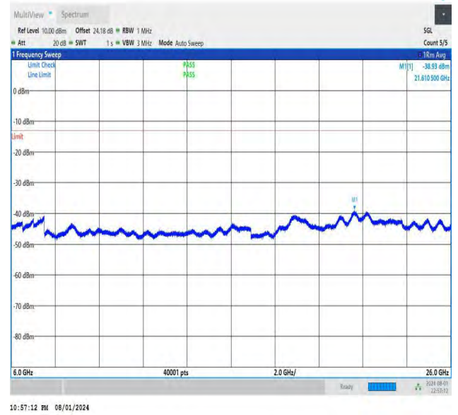
NTNV-DC_26A-n78A(3700-3800)-PC3-30-5+40-M+L-QPSK-IDLE -DFT-BPSK-Edge_1RB_Left-6000-26000-PASS
