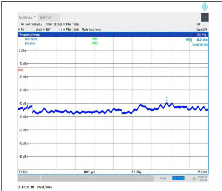
NTNV-DC_26A-n78A(3700-3800)-PC3-30-5+30-M+L-QPSK-IDL E-DFT-BPSK-Edge_1RB_Right-6000-26000-PASS
