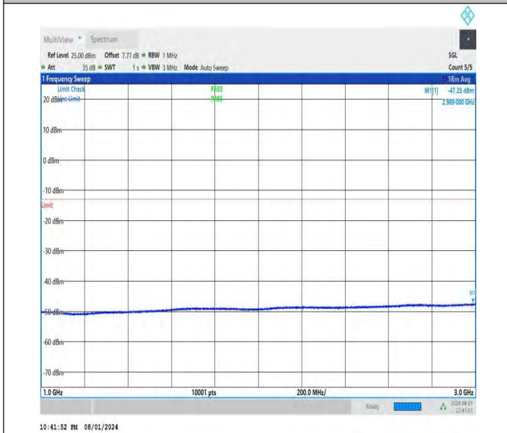
NTNV-DC_26A-n78A(3700-3800)-PC3-30-5+30-M+L-QPSK-IDL E-DFT-BPSK-Edge_1RB_Right-1000-3000-PASS
