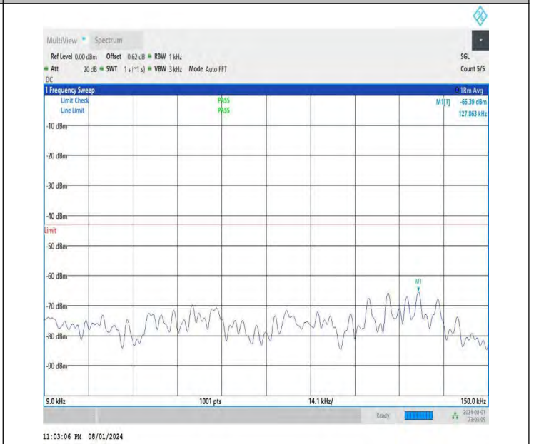
NTNV-DC_26A-n78A(3700-3800)-PC3-30-5+40-M+M-QPSK-IDLE -DFT-BPSK-Edge_1RB_Right-0.009-0.15-PASS
