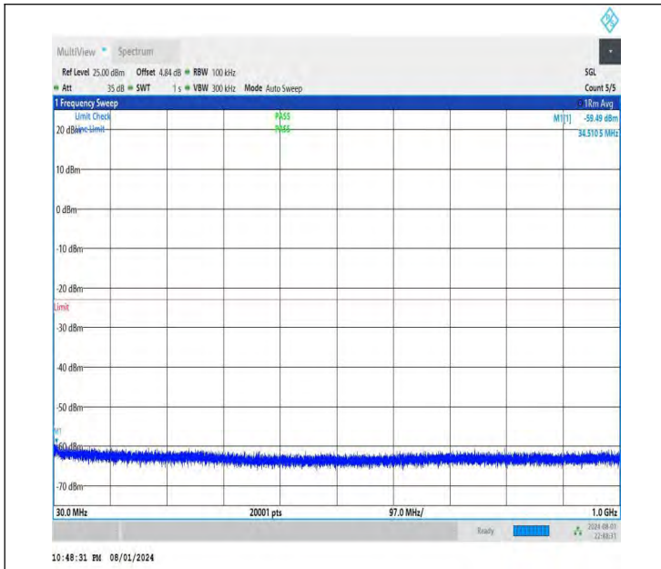
NTNV-DC_26A-n78A(3700-3800)-PC3-30-5+30-M+M-QPSK-IDL E-DFT-QPSK-Edge_1RB_Left-30-1000-PASS
