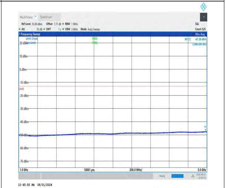
NTNV-DC_26A-n78A(3700-3800)-PC3-30-5+30-M+M-QPSK-IDLE -DFT-BPSK-Edge_1RB_Left-1000-3000-PASS
