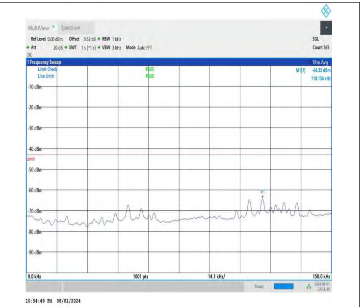
NTNV-DC_26A-n78A(3700-3800)-PC3-30-5+30-M+H-QPSK-IDLE -DFT-QPSK-Edge_1RB_Right-0.009-0.15-PASS
