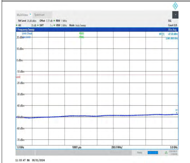
NTNV-DC_26A-n78A(3700-3800)-PC3-30-5+40-M+M-QPSK-IDL E-DFT-BPSK-Edge_1RB_Right-1000-3000-PASS
