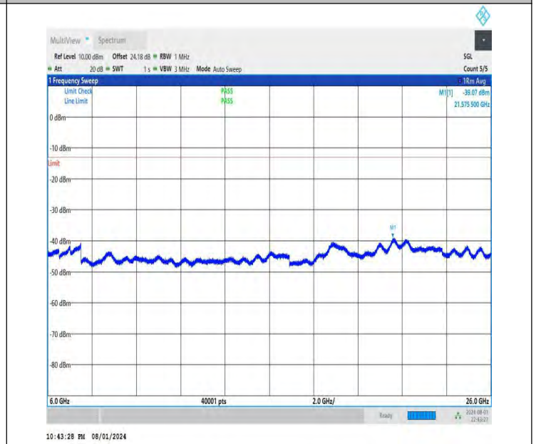
NTNV-DC_26A-n78A(3700-3800)-PC3-30-5+30-M+L-QPSK-IDLE -DFT-QPSK-Edge_1RB_Left-6000-26000-PASS
