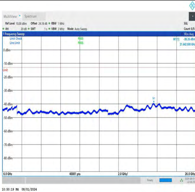
NTNV-DC_26A-n78A(3700-3800)-PC3-30-5+30-M+M-QPSK-IDL E-DFT-QPSK-Edge_1RB_Right-6000-26000-PASS
