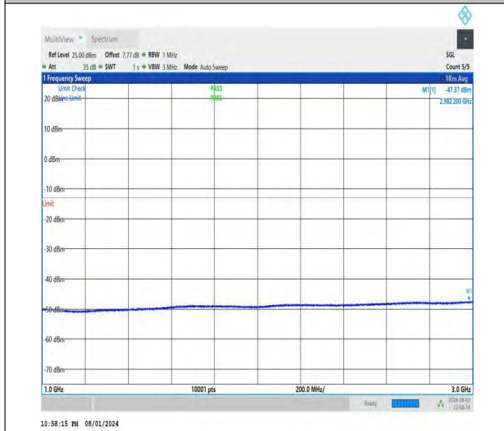
NTNV-DC_26A-n78A(3700-3800)-PC3-30-5+40-M+L-QPSK-IDL E-DFT-BPSK-Edge_1RB_Right-1000-3000-PASS
