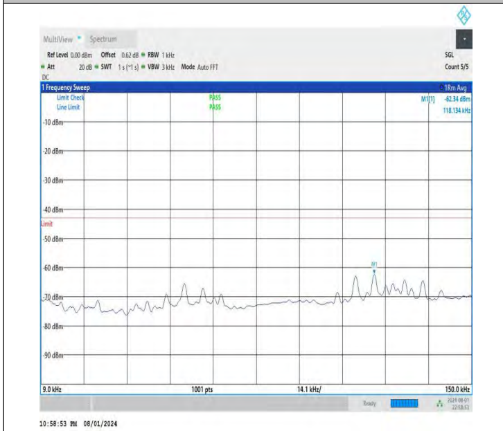
NTNV-DC_26A-n78A(3700-3800)-PC3-30-5+40-M+L-QPSK-IDL E-DFT-QPSK-Edge_1RB_Left-0.009-0.15-PASS
