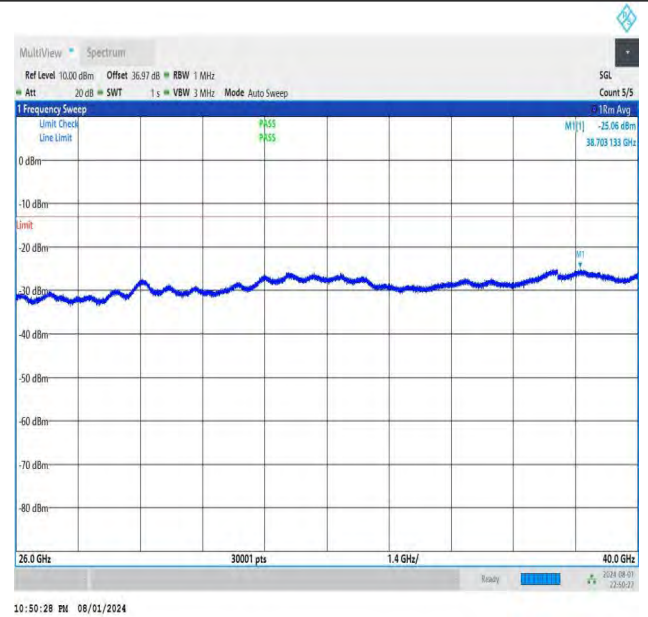
NTNV-DC_26A-n78A(3700-3800)-PC3-30-5+30-M+M-QPSK-IDLE -DFT-QPSK-Edge_1RB_Right-26000-40000-PASS
