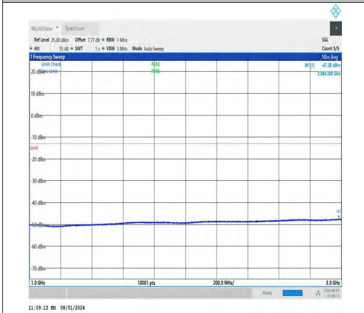
NTNV-DC_26A-n78A(3700-3800)-PC3-30-5+40-M+H-QPSK-IDL E-DFT-BPSK-Edge_1RB_Right-1000-3000-PASS
