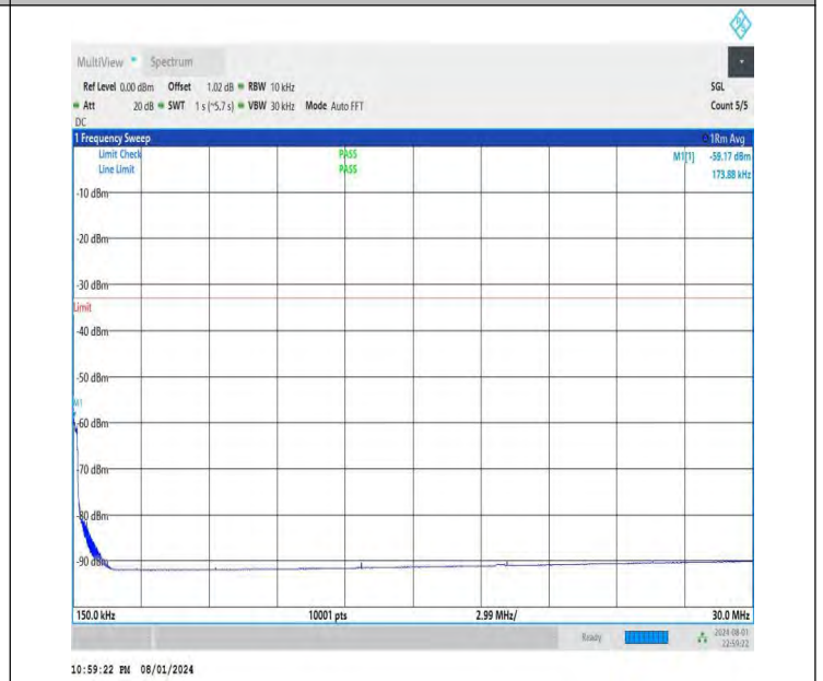
NTNV-DC_26A-n78A(3700-3800)-PC3-30-5+40-M+L-QPSK-IDLE -DFT-QPSK-Edge_1RB_Left-0.15-30-PASS
