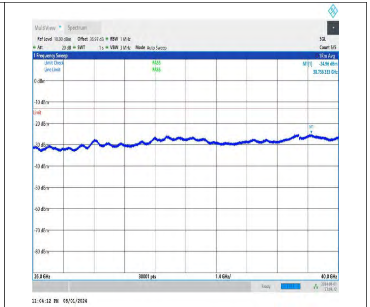
NTNV-DC_26A-n78A(3700-3800)-PC3-30-5+40-M+M-QPSK-IDLE -DFT-BPSK-Edge_1RB_Right-26000-40000-PASS
