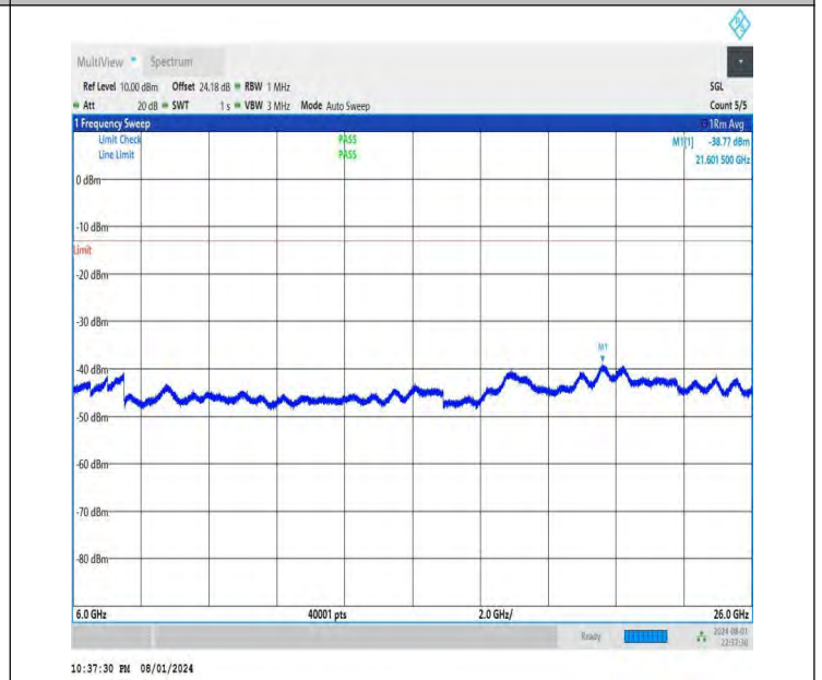
NTNV-DC_26A-n78A(3700-3800)-PC3-30-5+20-M+H-QPSK-IDLE -DFT-QPSK-Edge_1RB_Left-6000-26000-PASS
