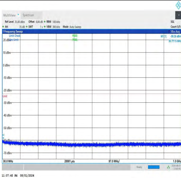
NTNV-DC_26A-n78A(3700-3800)-PC3-30-5+40-M+H-QPSK-IDL E-DFT-BPSK-Edge_1RB_Left-30-1000-PASS
