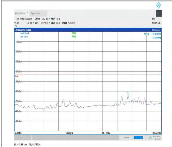
NTNV-DC_26A-n78A(3700-3800)-PC3-30-5+30-M+M-QPSK-IDL E-DFT-QPSK-Edge_1RB_Left-0.009-0.15-PASS
