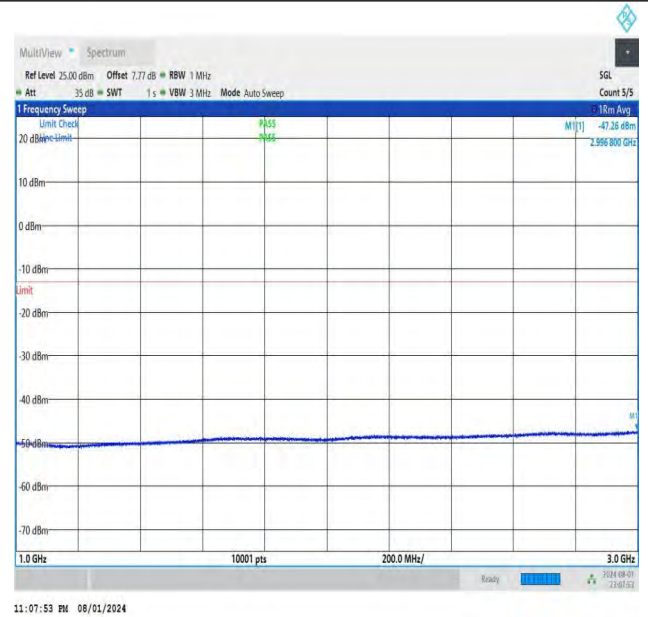
NTNV-DC_26A-n78A(3700-3800)-PC3-30-5+40-M+H-QPSK-IDLE -DFT-BPSK-Edge_1RB_Left-1000-3000-PASS
