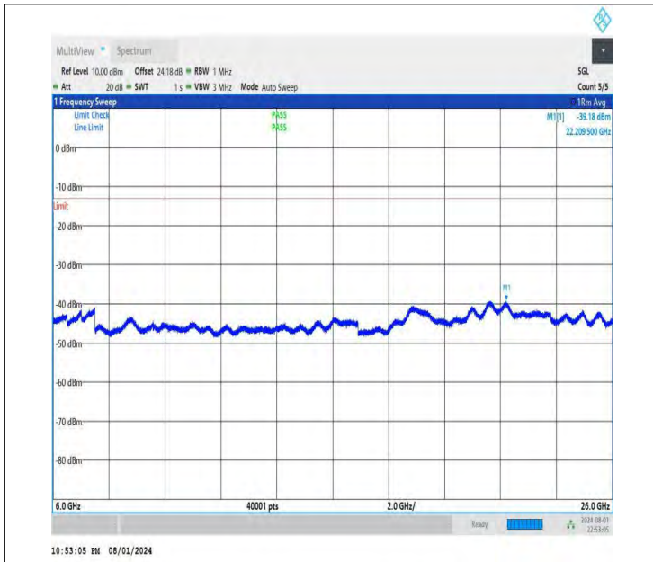
NTNV-DC_26A-n78A(3700-3800)-PC3-30-5+30-M+H-QPSK-IDL E-DFT-BPSK-Edge_1RB_Right-6000-26000-PASS
