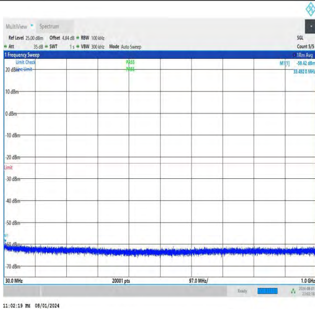
NTNV-DC_26A-n78A(3700-3800)-PC3-30-5+40-M+M-QPSK-IDL E-DFT-BPSK-Edge_1RB_Left-30-1000-PASS
