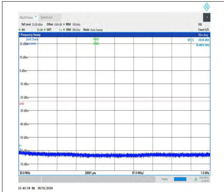
NTNV-DC_26A-n78A(3700-3800)-PC3-30-5+30-M+L-QPSK-IDL E-DFT-QPSK-Edge_1RB_Left-30-1000-PASS
