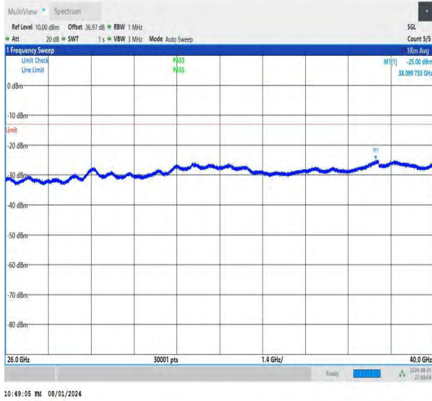
NTNV-DC_26A-n78A(3700-3800)-PC3-30-5+30-M+M-QPSK-IDL E-DFT-QPSK-Edge_1RB_Left-26000-40000-PASS
