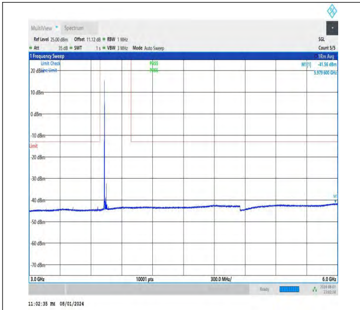
NTNV-DC_26A-n78A(3700-3800)-PC3-30-5+40-M+M-QPSK-IDL E-DFT-BPSK-Edge_1RB_Left-3000-6000-PASS
