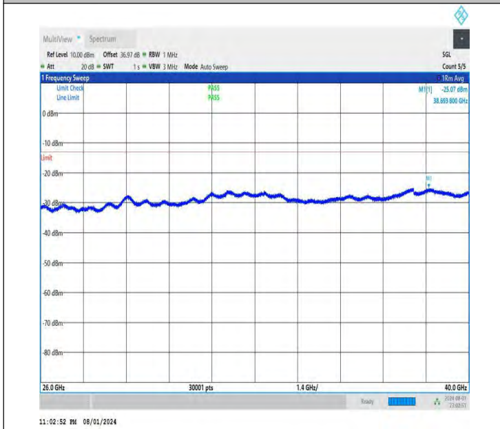
NTNV-DC_26A-n78A(3700-3800)-PC3-30-5+40-M+M-QPSK-IDL E-DFT-BPSK-Edge_1RB_Left-26000-40000-PASS
