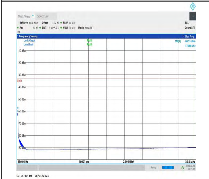
NTNV-DC_26A-n78A(3700-3800)-PC3-30-5+30-M+H-QPSK-IDL E-DFT-QPSK-Edge_1RB_Right-0.15-30-PASS
