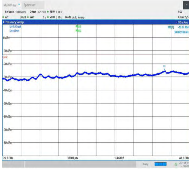
NTNV-DC_26A-n78A(3700-3800)-PC3-30-5+40-M+L-QPSK-IDL E-DFT-QPSK-Edge_1RB_Left-26000-40000-PASS
