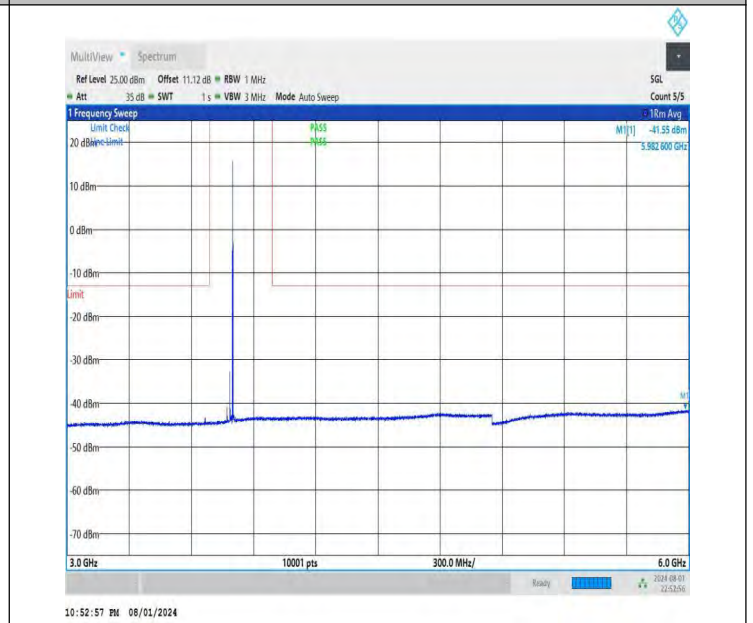
NTNV-DC_26A-n78A(3700-3800)-PC3-30-5+30-M+H-QPSK-IDLE -DFT-BPSK-Edge_1RB_Right-3000-6000-PASS
