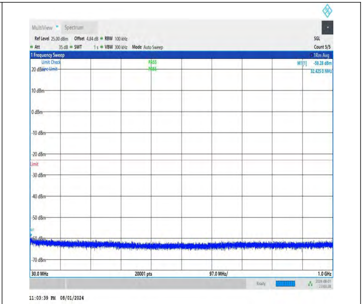
NTNV-DC_26A-n78A(3700-3800)-PC3-30-5+40-M+M-QPSK-IDLE -DFT-BPSK-Edge_1RB_Right-30-1000-PASS
