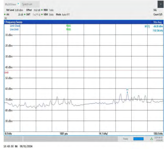
NTNV-DC_26A-n78A(3700-3800)-PC3-30-5+30-M+L-QPSK-IDLE -DFT-QPSK-Edge_1RB_Right-0.009-0.15-PASS
