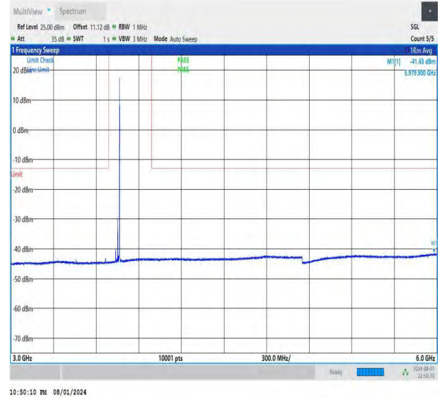
NTNV-DC_26A-n78A(3700-3800)-PC3-30-5+30-M+M-QPSK-IDLE -DFT-QPSK-Edge_1RB_Right-3000-6000-PASS
