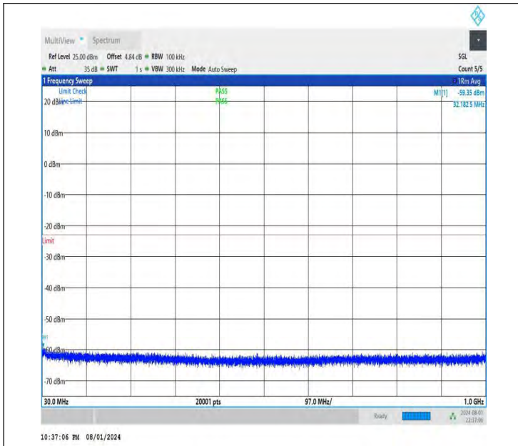
NTNV-DC_26A-n78A(3700-3800)-PC3-30-5+20-M+H-QPSK-IDL E-DFT-QPSK-Edge_1RB_Left-30-1000-PASS
