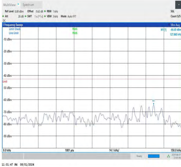
NTNV-DC_26A-n78A(3700-3800)-PC3-30-5+40-M+M-QPSK-IDL E-DFT-BPSK-Edge_1RB_Left-0.009-0.15-PASS
