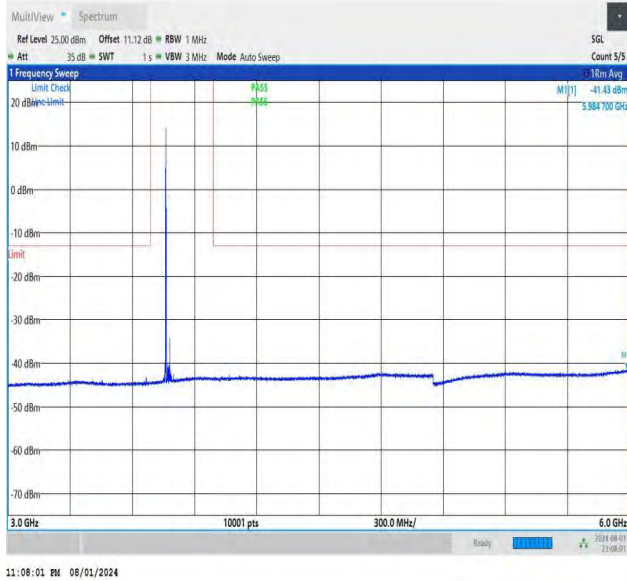
NTNV-DC_26A-n78A(3700-3800)-PC3-30-5+40-M+H-QPSK-IDL E-DFT-BPSK-Edge_1RB_Left-3000-6000-PASS
