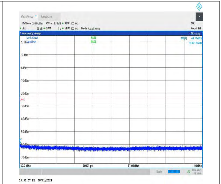
NTNV-DC_26A-n78A(3700-3800)-PC3-30-5+40-M+L-QPSK-IDLE -DFT-BPSK-Edge_1RB_Right-30-1000-PASS
