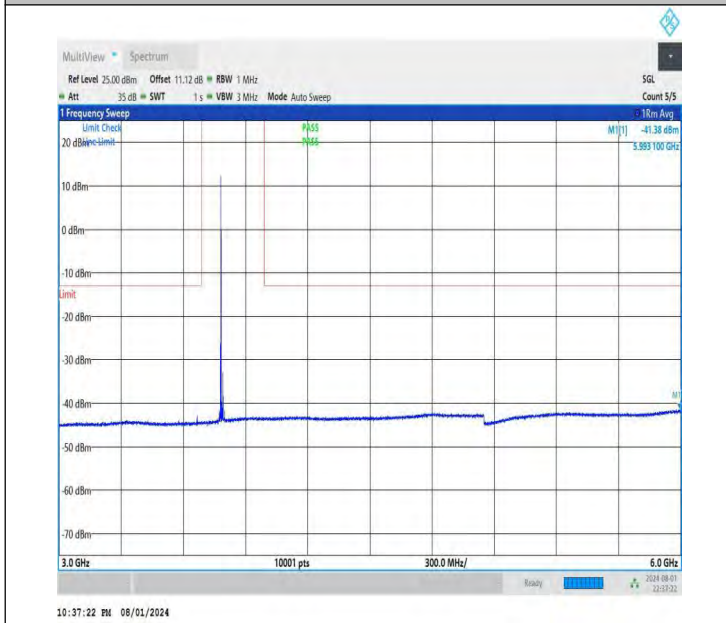
NTNV-DC_26A-n78A(3700-3800)-PC3-30-5+20-M+H-QPSK-IDL E-DFT-QPSK-Edge_1RB_Left-3000-6000-PASS
