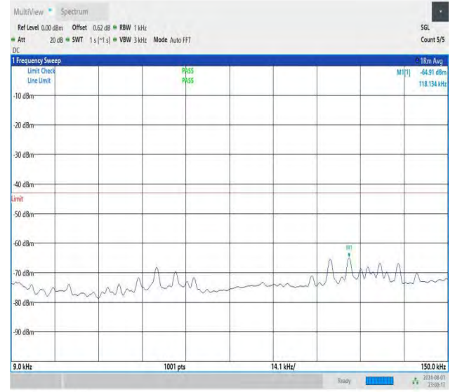
NTNV-DC_26A-n78A(3700-3800)-PC3-30-5+40-M+L-QPSK-IDLE -DFT-QPSK-Edge_1RB_Right-0.009-0.15-PASS
