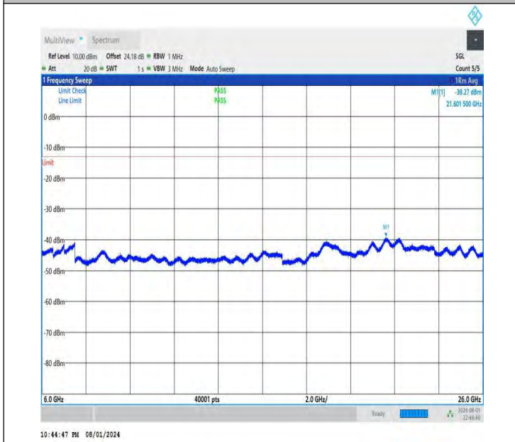
NTNV-DC_26A-n78A(3700-3800)-PC3-30-5+30-M+L-QPSK-IDL E-DFT-QPSK-Edge_1RB_Right-6000-26000-PASS
