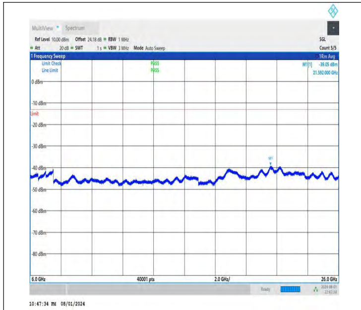
NTNV-DC_26A-n78A(3700-3800)-PC3-30-5+30-M+M-QPSK-IDL E-DFT-BPSK-Edge_1RB_Right-6000-26000-PASS
