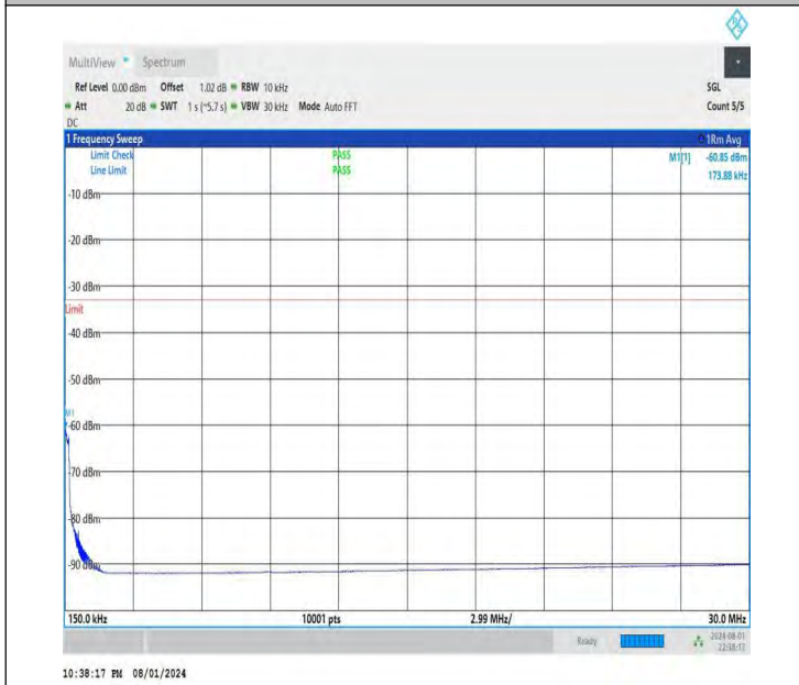
NTNV-DC_26A-n78A(3700-3800)-PC3-30-5+20-M+H-QPSK-IDL E-DFT-QPSK-Edge_1RB_Right-0.15-30-PASS
