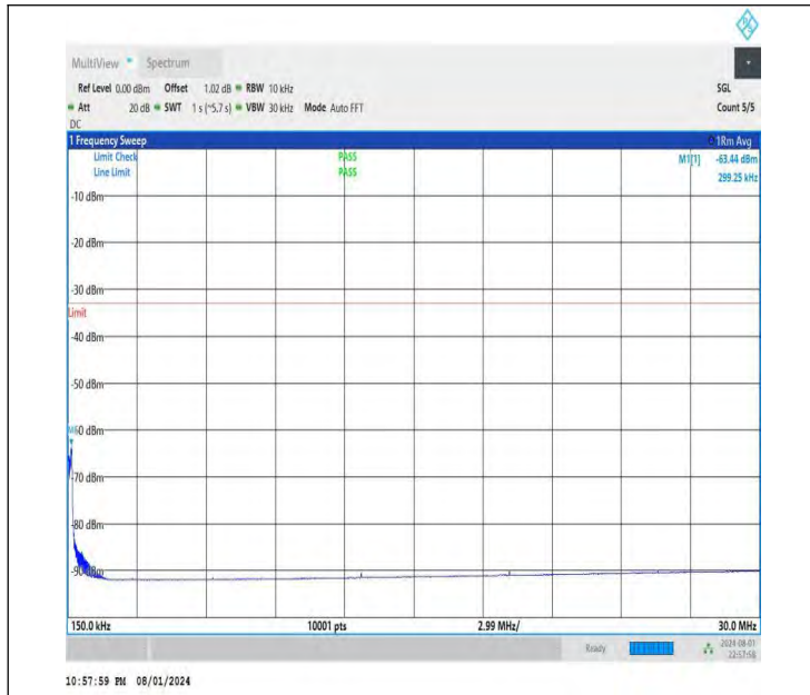
NTNV-DC_26A-n78A(3700-3800)-PC3-30-5+40-M+L-QPSK-IDL E-DFT-BPSK-Edge_1RB_Right-0.15-30-PASS
