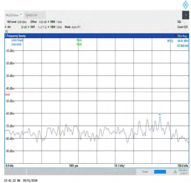
NTNV-DC_26A-n78A(3700-3800)-PC3-30-5+30-M+L-QPSK-IDLE -DFT-BPSK-Edge_1RB_Right-0.009-0.15-PASS
