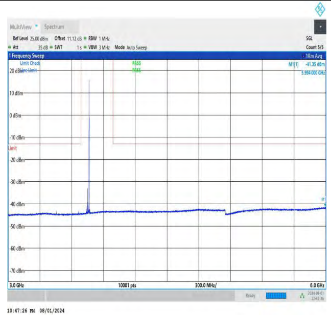
NTNV-DC_26A-n78A(3700-3800)-PC3-30-5+30-M+M-QPSK-IDLE -DFT-BPSK-Edge_1RB_Right-3000-6000-PASS
