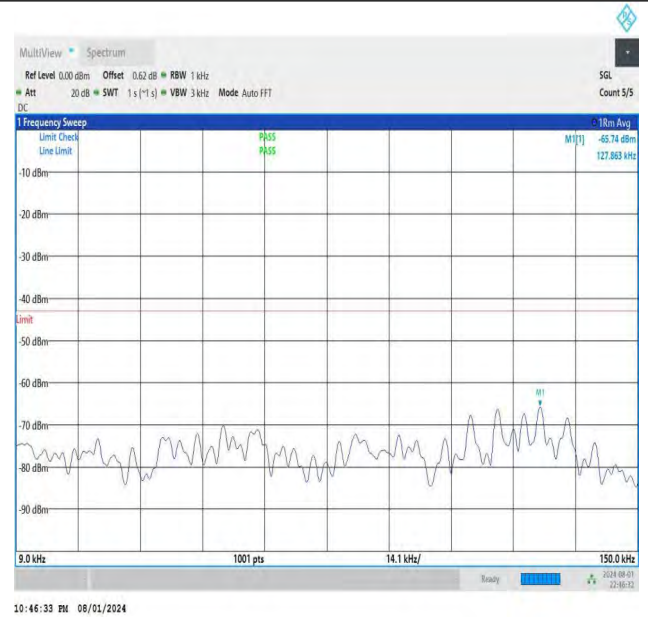
NTNV-DC_26A-n78A(3700-3800)-PC3-30-5+30-M+M-QPSK-IDLE -DFT-BPSK-Edge_1RB_Right-0.009-0.15-PASS
