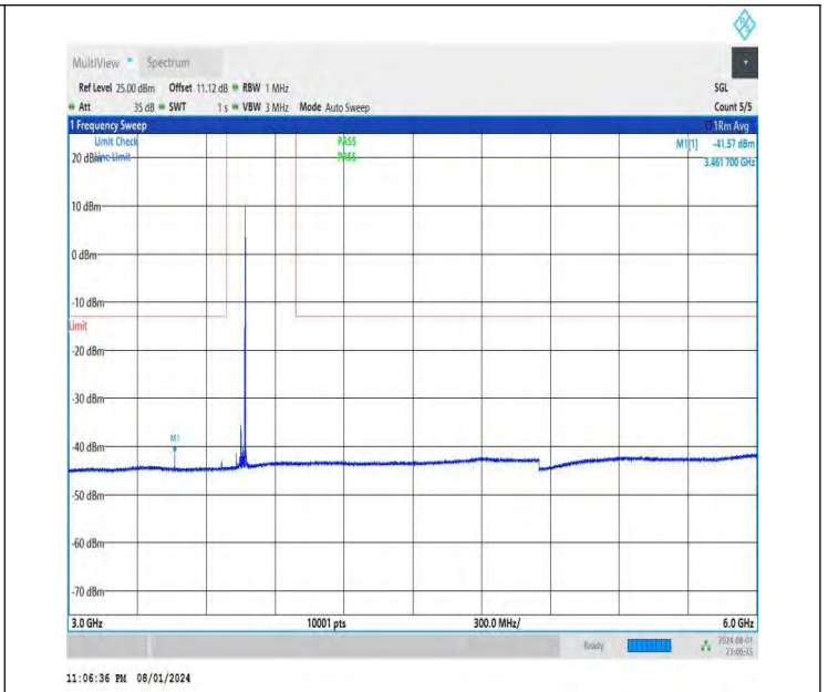
NTNV-DC_26A-n78A(3700-3800)-PC3-30-5+40-M+M-QPSK-IDLE -DFT-QPSK-Edge_1RB_Right-3000-6000-PASS
