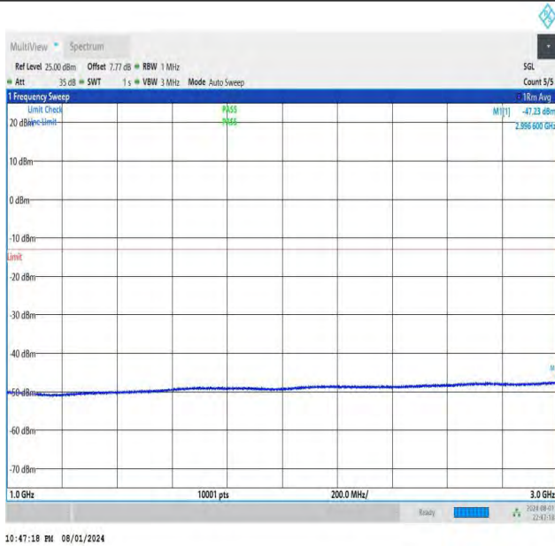
NTNV-DC_26A-n78A(3700-3800)-PC3-30-5+30-M+M-QPSK-IDL E-DFT-BPSK-Edge_1RB_Right-1000-3000-PASS
