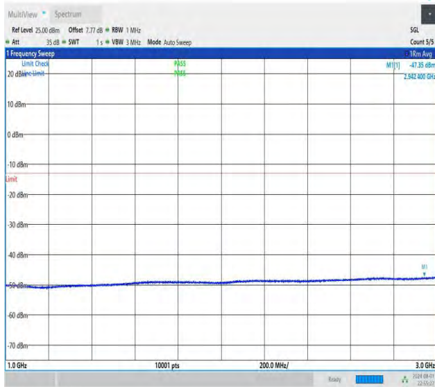
NTNV-DC_26A-n78A(3700-3800)-PC3-30-5+30-M+H-QPSK-IDL E-DFT-QPSK-Edge_1RB_Right-1000-3000-PASS
