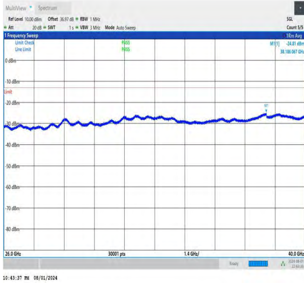
NTNV-DC_26A-n78A(3700-3800)-PC3-30-5+30-M+L-QPSK-IDL E-DFT-QPSK-Edge_1RB_Left-26000-40000-PASS
