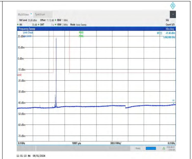
NTNV-DC_26A-n78A(3700-3800)-PC3-30-5+40-M+L-QPSK-IDLE -DFT-QPSK-Edge_1RB_Right-3000-6000-PASS
