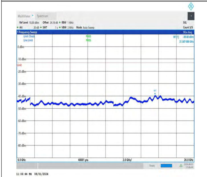
NTNV-DC_26A-n78A(3700-3800)-PC3-30-5+40-M+M-QPSK-IDL E-DFT-QPSK-Edge_1RB_Right-6000-26000-PASS
