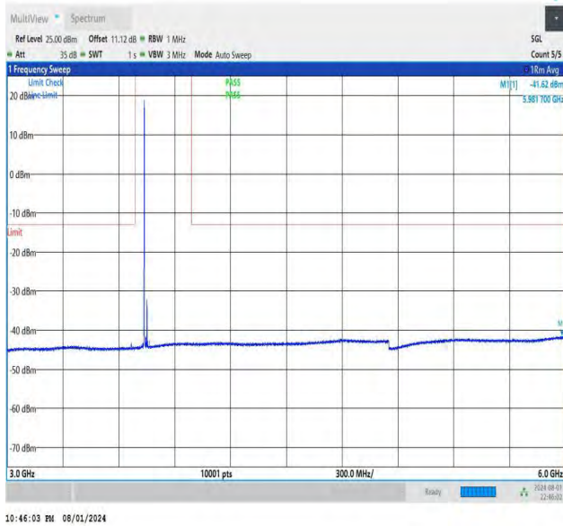
NTNV-DC_26A-n78A(3700-3800)-PC3-30-5+30-M+M-QPSK-IDL E-DFT-BPSK-Edge_1RB_Left-3000-6000-PASS
