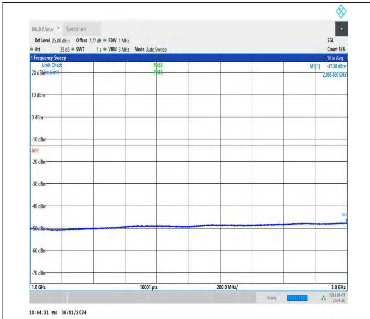
NTNV-DC_26A-n78A(3700-3800)-PC3-30-5+30-M+L-QPSK-IDL E-DFT-QPSK-Edge_1RB_Right-1000-3000-PASS
