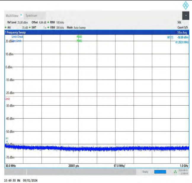
NTNV-DC_26A-n78A(3700-3800)-PC3-30-5+30-M+M-QPSK-IDLE -DFT-QPSK-Edge_1RB_Right-30-1000-PASS
