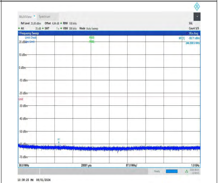
NTNV-DC_26A-n78A(3700-3800)-PC3-30-5+20-M+H-QPSK-IDLE -DFT-QPSK-Edge_1RB_Right-30-1000-PASS
