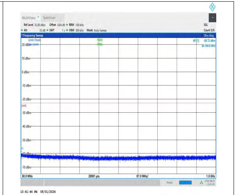
NTNV-DC_26A-n78A(3700-3800)-PC3-30-5+30-M+L-QPSK-IDLE -DFT-BPSK-Edge_1RB_Right-30-1000-PASS
