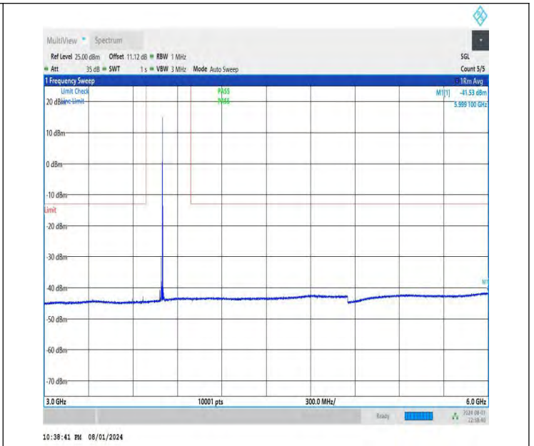
NTNV-DC_26A-n78A(3700-3800)-PC3-30-5+20-M+H-QPSK-IDLE -DFT-QPSK-Edge_1RB_Right-3000-6000-PASS
