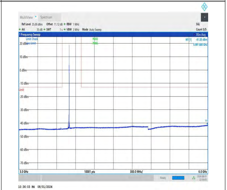
NTNV-DC_26A-n78A(3700-3800)-PC3-30-5+20-M+H-QPSK-IDLE -DFT-BPSK-Edge_1RB_Right-3000-6000-PASS
