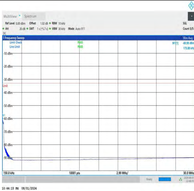
NTNV-DC_26A-n78A(3700-3800)-PC3-30-5+30-M+L-QPSK-IDL E-DFT-QPSK-Edge_1RB_Right-0.15-30-PASS
