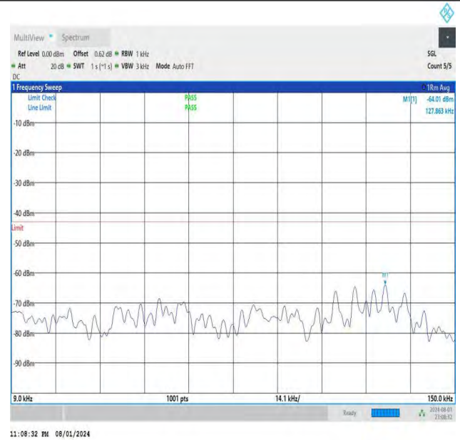
NTNV-DC_26A-n78A(3700-3800)-PC3-30-5+40-M+H-QPSK-IDLE -DFT-BPSK-Edge_1RB_Right-0.009-0.15-PASS
