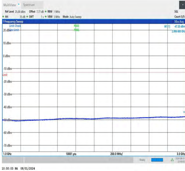
NTNV-DC_26A-n78A(3700-3800)-PC3-30-5+30-M+M-QPSK-IDL E-DFT-QPSK-Edge_1RB_Right-1000-3000-PASS
