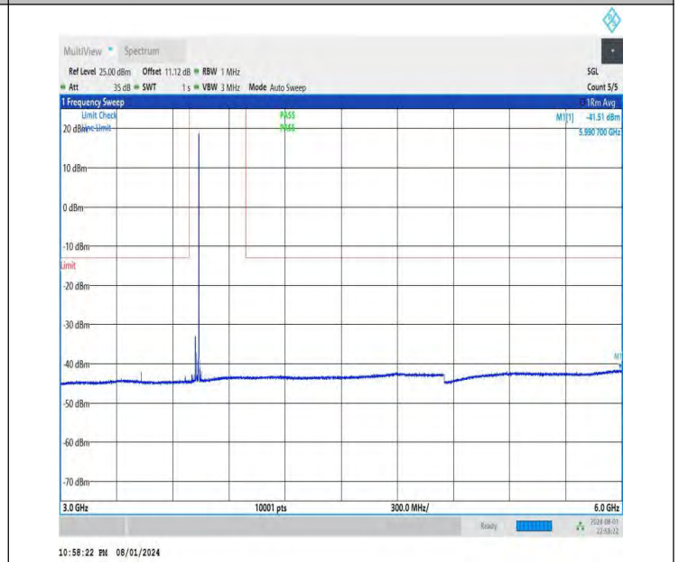
NTNV-DC_26A-n78A(3700-3800)-PC3-30-5+40-M+L-QPSK-IDLE -DFT-BPSK-Edge_1RB_Right-3000-6000-PASS
