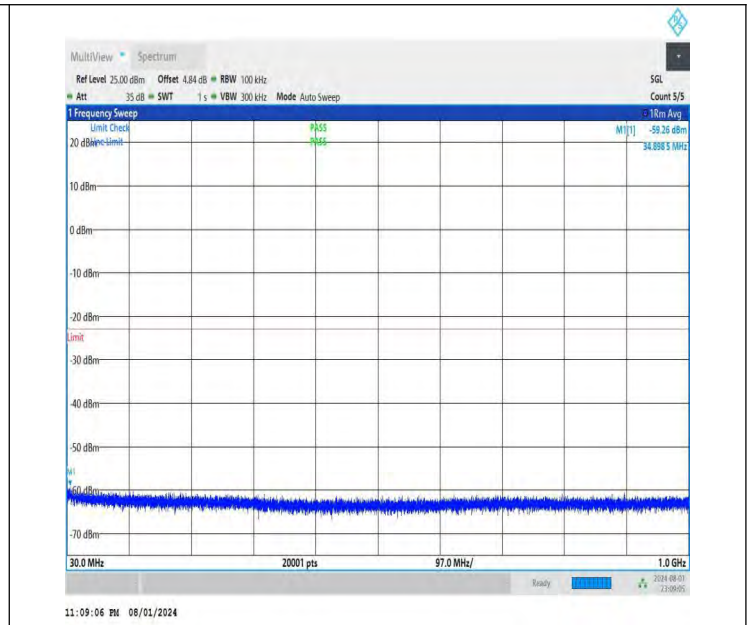
NTNV-DC_26A-n78A(3700-3800)-PC3-30-5+40-M+H-QPSK-IDLE -DFT-BPSK-Edge_1RB_Right-30-1000-PASS
