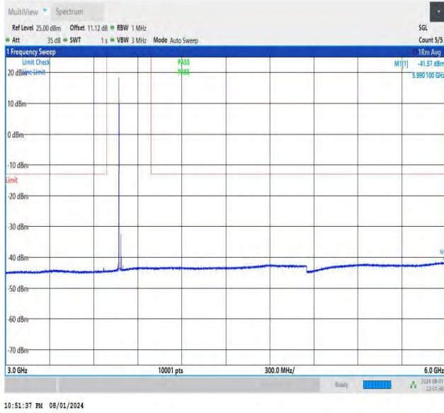
NTNV-DC_26A-n78A(3700-3800)-PC3-30-5+30-M+H-QPSK-IDL E-DFT-BPSK-Edge_1RB_Left-3000-6000-PASS
