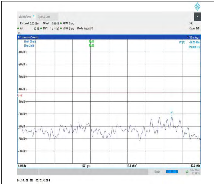
NTNV-DC_26A-n78A(3700-3800)-PC3-30-5+30-M+L-QPSK-IDL E-DFT-BPSK-Edge_1RB_Left-0.009-0.15-PASS
