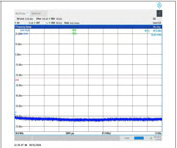
NTNV-DC_26A-n78A(3700-3800)-PC3-30-5+20-M+H-QPSK-IDLE -DFT-BPSK-Edge_1RB_Right-30-1000-PASS
