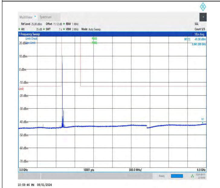
NTNV-DC_26A-n78A(3700-3800)-PC3-30-5+40-M+L-QPSK-IDL E-DFT-QPSK-Edge_1RB_Left-3000-6000-PASS
