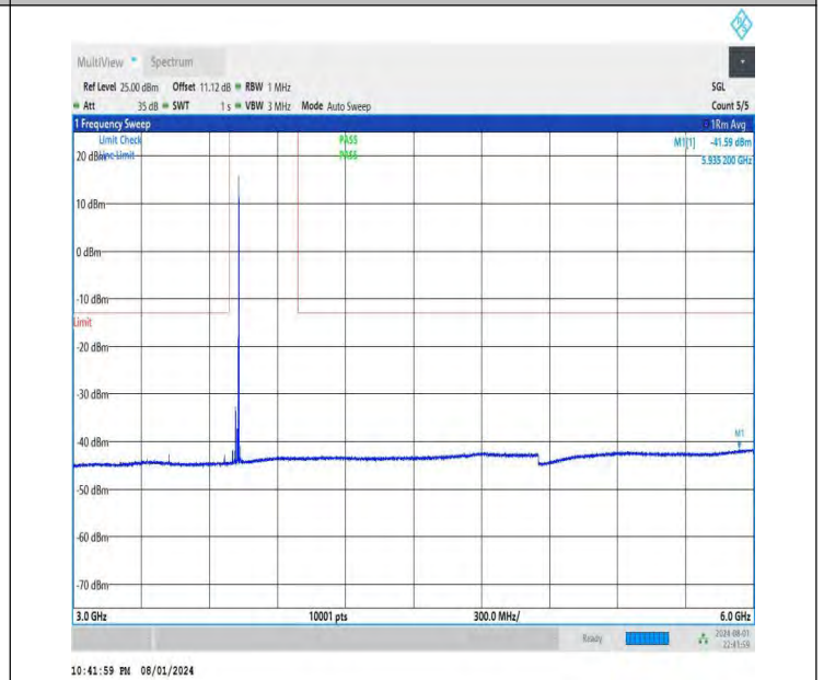
NTNV-DC_26A-n78A(3700-3800)-PC3-30-5+30-M+L-QPSK-IDLE -DFT-BPSK-Edge_1RB_Right-3000-6000-PASS
