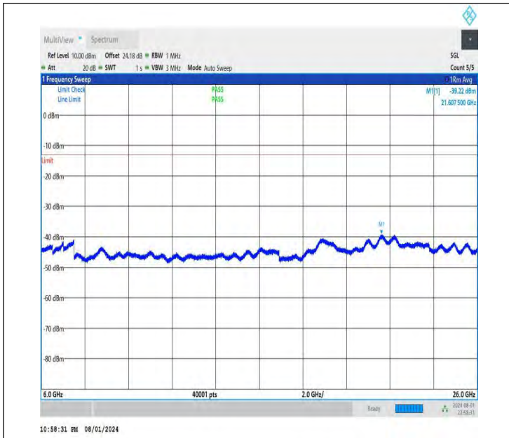
NTNV-DC_26A-n78A(3700-3800)-PC3-30-5+40-M+L-QPSK-IDL E-DFT-BPSK-Edge_1RB_Right-6000-26000-PASS
