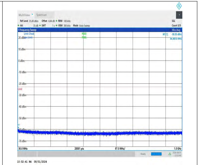
NTNV-DC_26A-n78A(3700-3800)-PC3-30-5+30-M+H-QPSK-IDLE -DFT-BPSK-Edge_1RB_Right-30-1000-PASS
