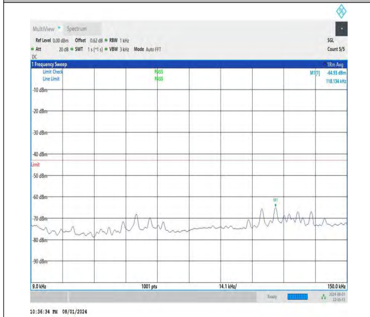
NTNV-DC_26A-n78A(3700-3800)-PC3-30-5+20-M+H-QPSK-IDL E-DFT-QPSK-Edge_1RB_Left-0.009-0.15-PASS
