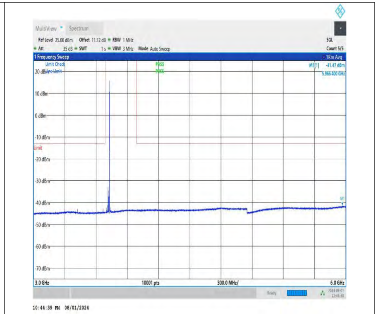
NTNV-DC_26A-n78A(3700-3800)-PC3-30-5+30-M+L-QPSK-IDLE -DFT-QPSK-Edge_1RB_Right-3000-6000-PASS
