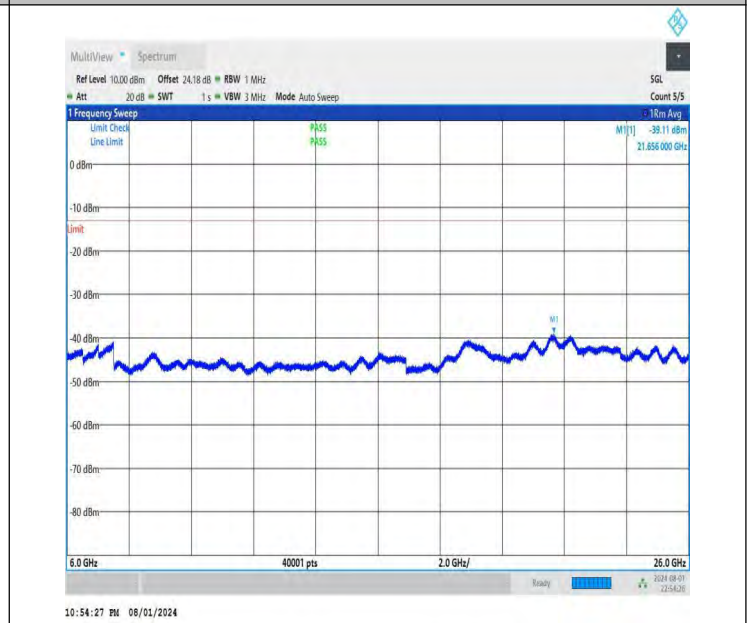
NTNV-DC_26A-n78A(3700-3800)-PC3-30-5+30-M+H-QPSK-IDLE -DFT-QPSK-Edge_1RB_Left-6000-26000-PASS
