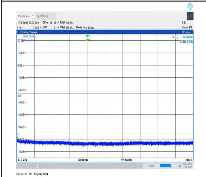
NTNV-DC_26A-n78A(3700-3800)-PC3-30-5+30-M+L-QPSK-IDL E-DFT-BPSK-Edge_1RB_Left-30-1000-PASS
