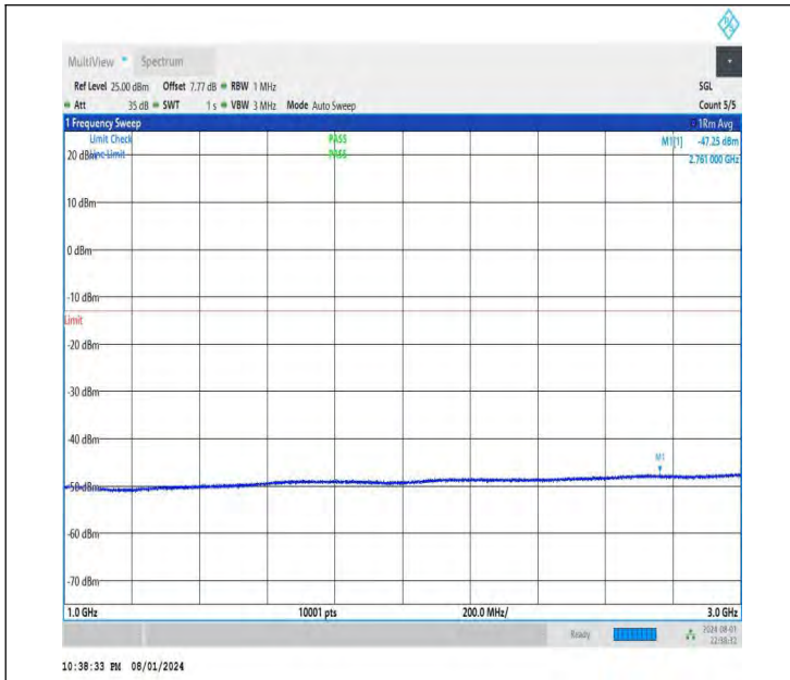
NTNV-DC_26A-n78A(3700-3800)-PC3-30-5+20-M+H-QPSK-IDL E-DFT-QPSK-Edge_1RB_Right-1000-3000-PASS
