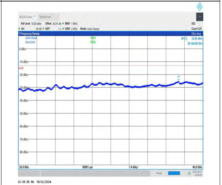
NTNV-DC_26A-n78A(3700-3800)-PC3-30-5+20-M+H-QPSK-IDLE -DFT-QPSK-Edge_1RB_Right-26000-40000-PASS
