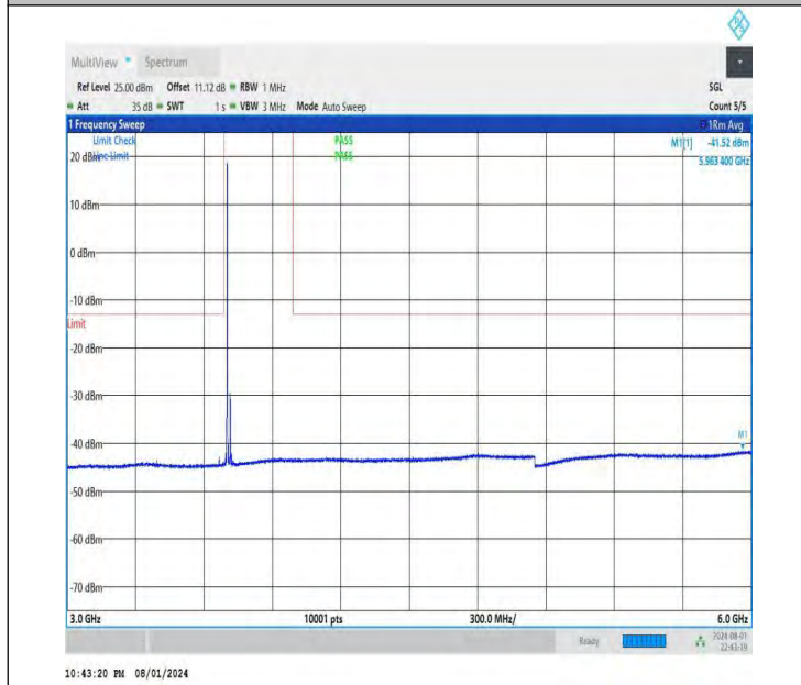
NTNV-DC_26A-n78A(3700-3800)-PC3-30-5+30-M+L-QPSK-IDL E-DFT-QPSK-Edge_1RB_Left-3000-6000-PASS
