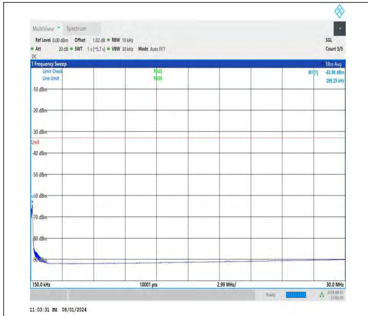
NTNV-DC_26A-n78A(3700-3800)-PC3-30-5+40-M+M-QPSK-IDL E-DFT-BPSK-Edge_1RB_Right-0.15-30-PASS
