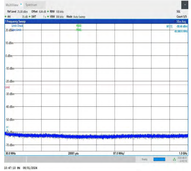
NTNV-DC_26A-n78A(3700-3800)-PC3-30-5+30-M+M-QPSK-IDLE -DFT-BPSK-Edge_1RB_Right-30-1000-PASS
