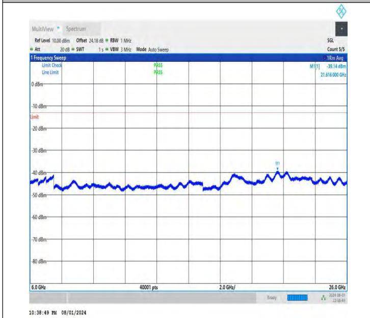
NTNV-DC_26A-n78A(3700-3800)-PC3-30-5+20-M+H-QPSK-IDL E-DFT-QPSK-Edge_1RB_Right-6000-26000-PASS
