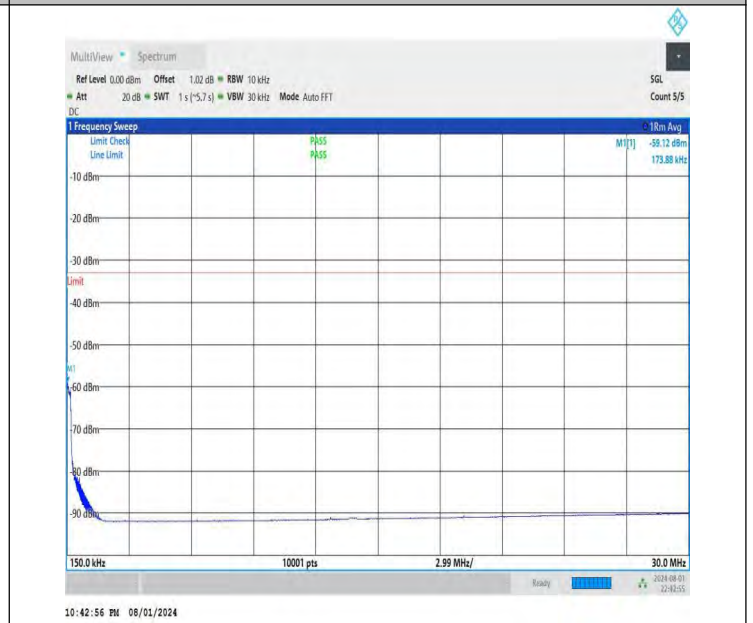
NTNV-DC_26A-n78A(3700-3800)-PC3-30-5+30-M+L-QPSK-IDLE -DFT-QPSK-Edge_1RB_Left-0.15-30-PASS
