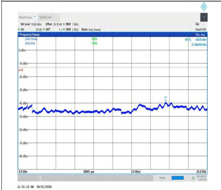
NTNV-DC_26A-n78A(3700-3800)-PC3-30-5+40-M+L-QPSK-IDL E-DFT-QPSK-Edge_1RB_Right-6000-26000-PASS
