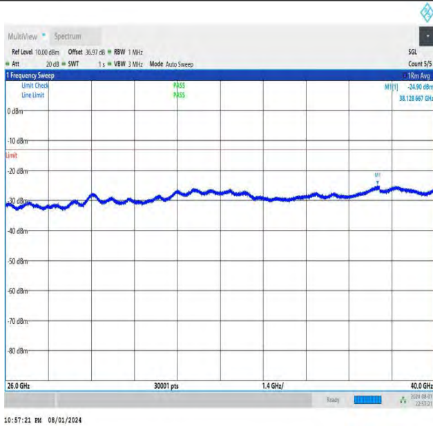
NTNV-DC_26A-n78A(3700-3800)-PC3-30-5+40-M+L-QPSK-IDL E-DFT-BPSK-Edge_1RB_Left-26000-40000-PASS
