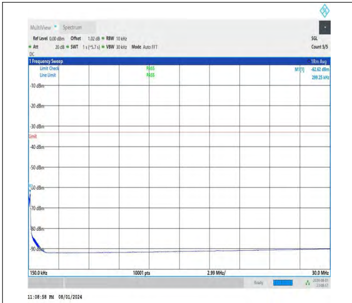
NTNV-DC_26A-n78A(3700-3800)-PC3-30-5+40-M+H-QPSK-IDL E-DFT-BPSK-Edge_1RB_Right-0.15-30-PASS
