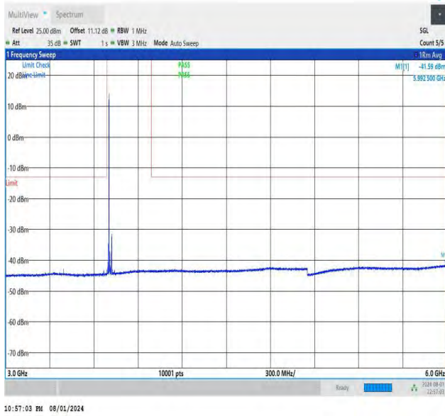
NTNV-DC_26A-n78A(3700-3800)-PC3-30-5+40-M+L-QPSK-IDL E-DFT-BPSK-Edge_1RB_Left-3000-6000-PASS
