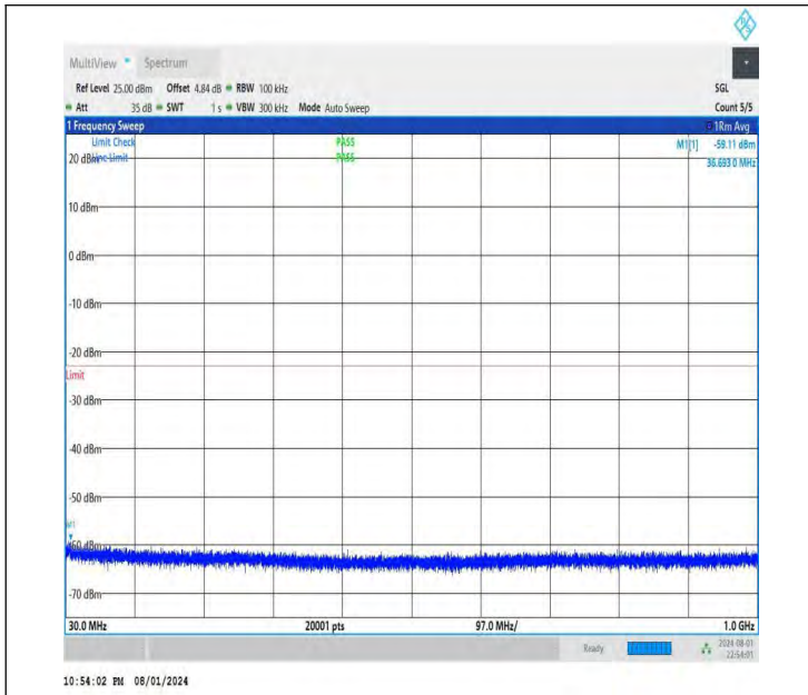
NTNV-DC_26A-n78A(3700-3800)-PC3-30-5+30-M+H-QPSK-IDL E-DFT-QPSK-Edge_1RB_Left-30-1000-PASS
