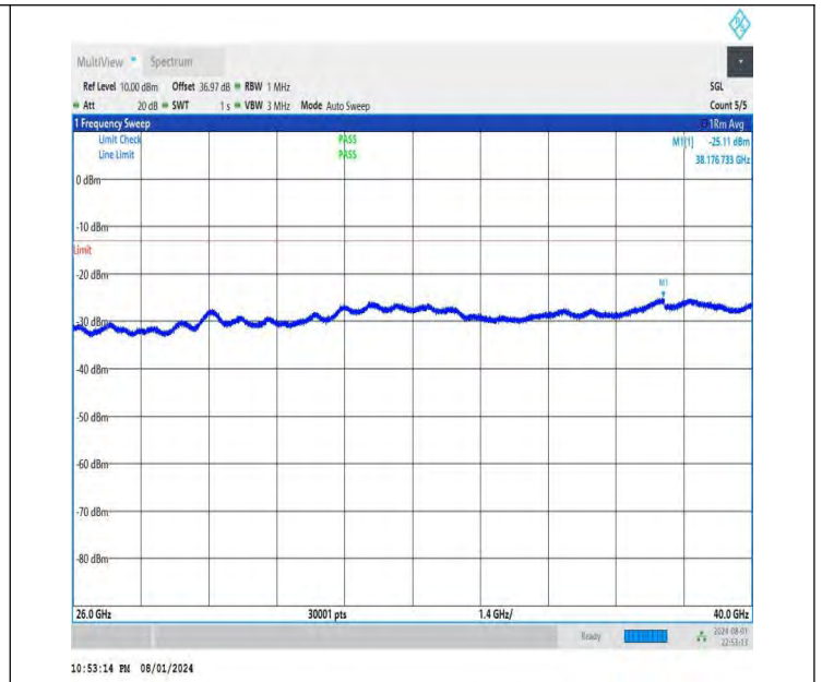
NTNV-DC_26A-n78A(3700-3800)-PC3-30-5+30-M+H-QPSK-IDLE -DFT-BPSK-Edge_1RB_Right-26000-40000-PASS
