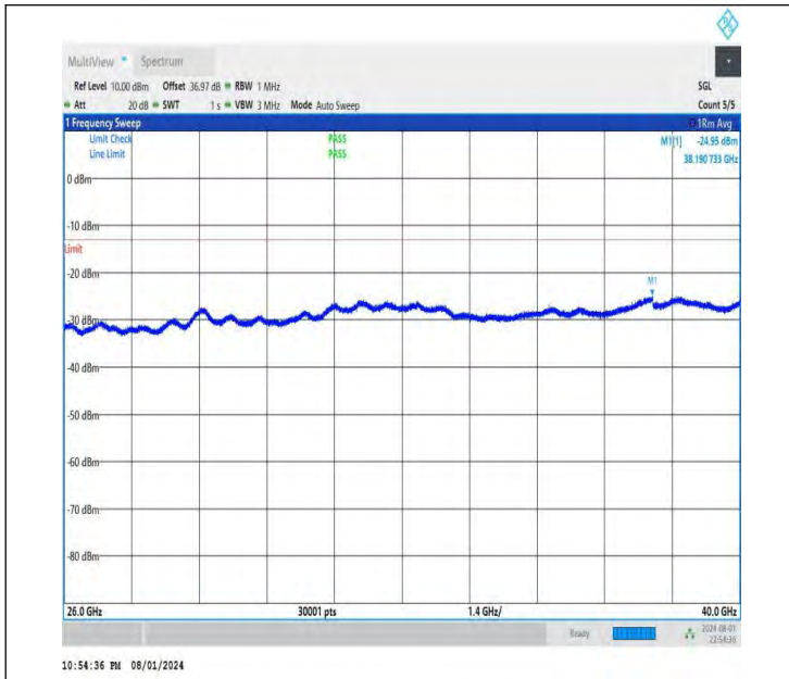
NTNV-DC_26A-n78A(3700-3800)-PC3-30-5+30-M+H-QPSK-IDL E-DFT-QPSK-Edge_1RB_Left-26000-40000-PASS
