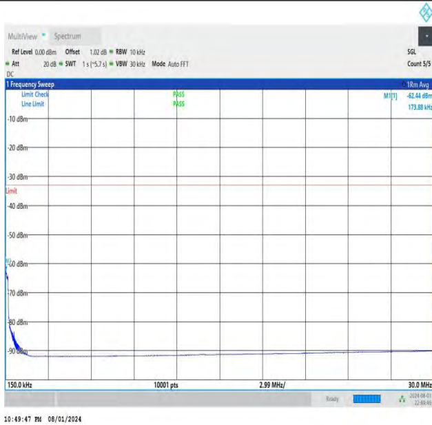
NTNV-DC_26A-n78A(3700-3800)-PC3-30-5+30-M+M-QPSK-IDL E-DFT-QPSK-Edge_1RB_Right-0.15-30-PASS
