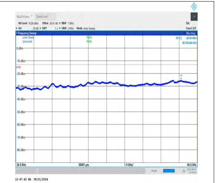
NTNV-DC_26A-n78A(3700-3800)-PC3-30-5+30-M+M-QPSK-IDLE -DFT-BPSK-Edge_1RB_Right-26000-40000-PASS
