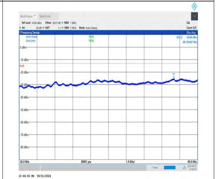
NTNV-DC_26A-n78A(3700-3800)-PC3-30-5+30-M+L-QPSK-IDLE -DFT-QPSK-Edge_1RB_Right-26000-40000-PASS
