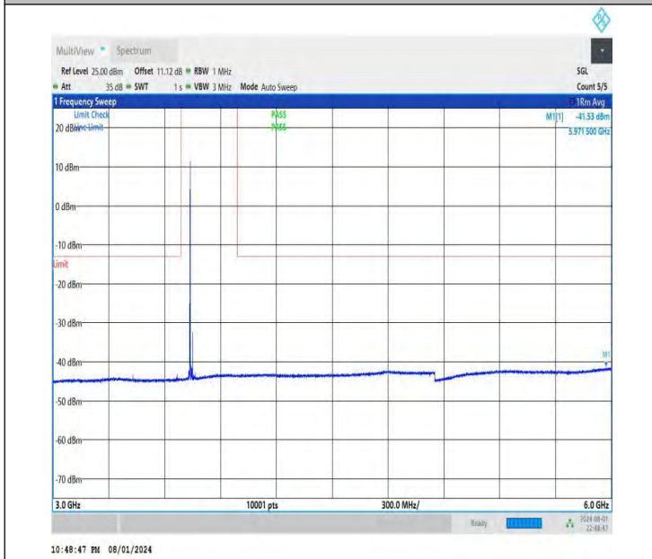
NTNV-DC_26A-n78A(3700-3800)-PC3-30-5+30-M+M-QPSK-IDL E-DFT-QPSK-Edge_1RB_Left-3000-6000-PASS
