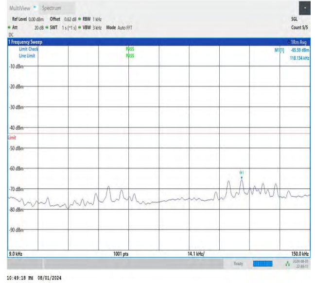
NTNV-DC_26A-n78A(3700-3800)-PC3-30-5+30-M+M-QPSK-IDLE -DFT-QPSK-Edge_1RB_Right-0.009-0.15-PASS
