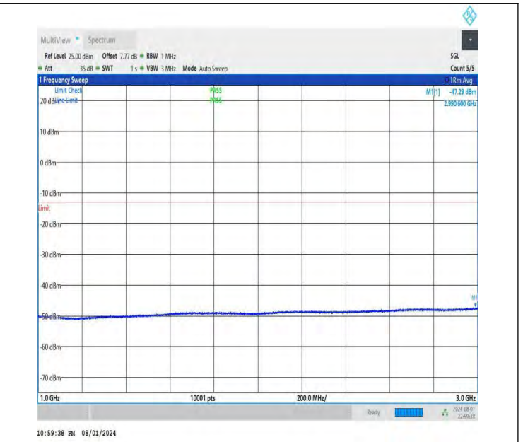
NTNV-DC_26A-n78A(3700-3800)-PC3-30-5+40-M+L-QPSK-IDLE -DFT-QPSK-Edge_1RB_Left-1000-3000-PASS
