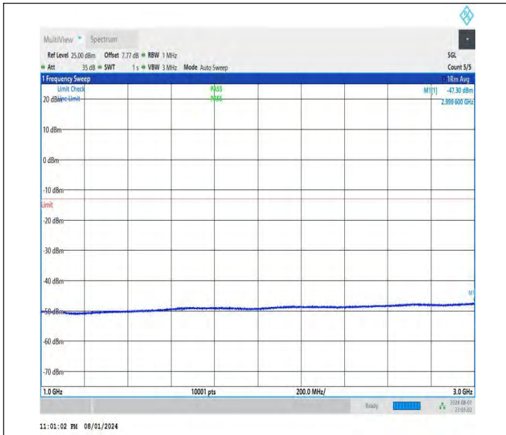
NTNV-DC_26A-n78A(3700-3800)-PC3-30-5+40-M+L-QPSK-IDL E-DFT-QPSK-Edge_1RB_Right-1000-3000-PASS
