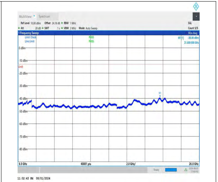
NTNV-DC_26A-n78A(3700-3800)-PC3-30-5+40-M+M-QPSK-IDLE -DFT-BPSK-Edge_1RB_Left-6000-26000-PASS
