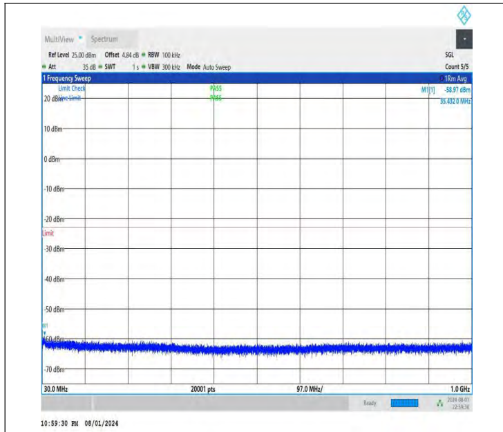
NTNV-DC_26A-n78A(3700-3800)-PC3-30-5+40-M+L-QPSK-IDL E-DFT-QPSK-Edge_1RB_Left-30-1000-PASS
