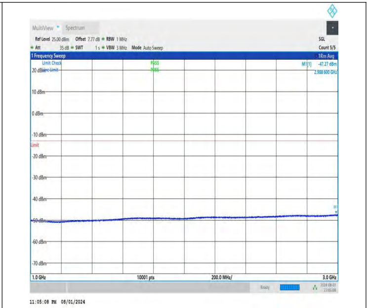
NTNV-DC_26A-n78A(3700-3800)-PC3-30-5+40-M+M-QPSK-IDLE -DFT-QPSK-Edge_1RB_Left-1000-3000-PASS
