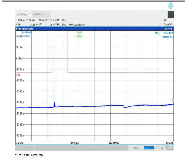
NTNV-DC_26A-n78A(3700-3800)-PC3-30-5+40-M+M-QPSK-IDL E-DFT-QPSK-Edge_1RB_Left-3000-6000-PASS
