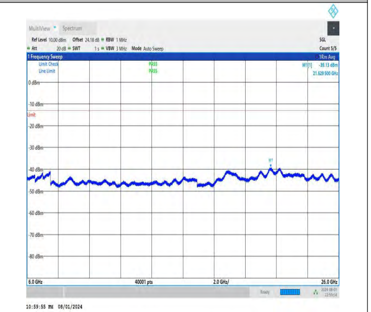
NTNV-DC_26A-n78A(3700-3800)-PC3-30-5+40-M+L-QPSK-IDLE -DFT-QPSK-Edge_1RB_Left-6000-26000-PASS
