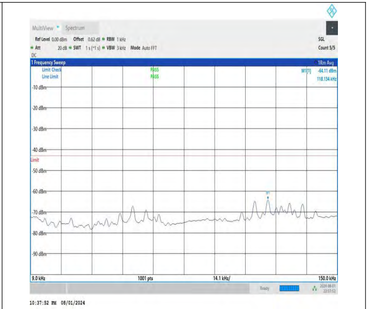
NTNV-DC_26A-n78A(3700-3800)-PC3-30-5+20-M+H-QPSK-IDLE -DFT-QPSK-Edge_1RB_Right-0.009-0.15-PASS
