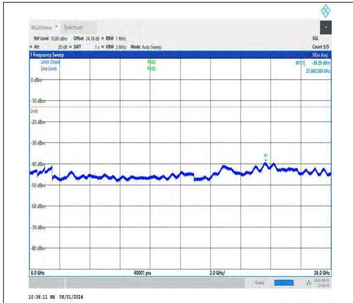
NTNV-DC_26A-n78A(3700-3800)-PC3-30-5+20-M+H-QPSK-IDL E-DFT-BPSK-Edge_1RB_Right-6000-26000-PASS
