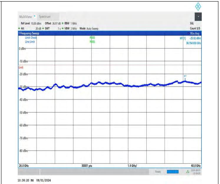
NTNV-DC_26A-n78A(3700-3800)-PC3-30-5+20-M+H-QPSK-IDLE -DFT-BPSK-Edge_1RB_Right-26000-40000-PASS
