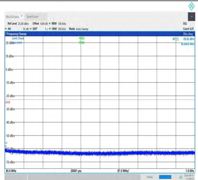
NTNV-DC_26A-n78A(3700-3800)-PC3-30-5+40-M+L-QPSK-IDLE -DFT-QPSK-Edge_1RB_Right-0.009-0.15-PASS
