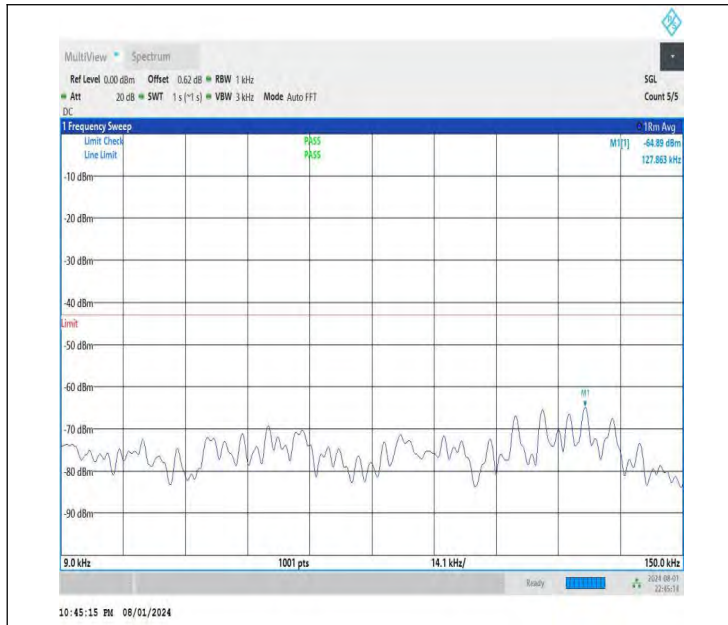
NTNV-DC_26A-n78A(3700-3800)-PC3-30-5+30-M+M-QPSK-IDL E-DFT-BPSK-Edge_1RB_Left-0.009-0.15-PASS
