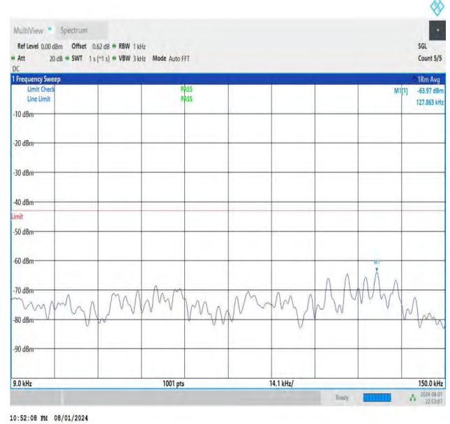
NTNV-DC_26A-n78A(3700-3800)-PC3-30-5+30-M+H-QPSK-IDLE -DFT-BPSK-Edge_1RB_Right-0.009-0.15-PASS
