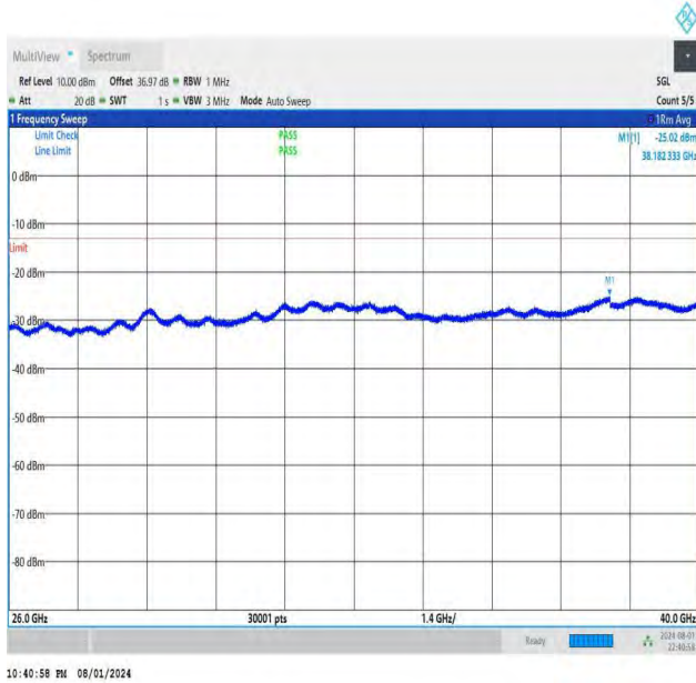
NTNV-DC_26A-n78A(3700-3800)-PC3-30-5+30-M+L-QPSK-IDL E-DFT-BPSK-Edge_1RB_Left-26000-40000-PASS
