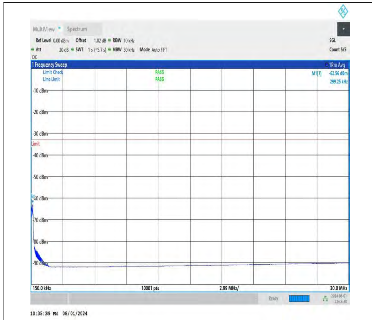
NTNV-DC_26A-n78A(3700-3800)-PC3-30-5+20-M+H-QPSK-IDL E-DFT-BPSK-Edge_1RB_Right-0.15-30-PASS
