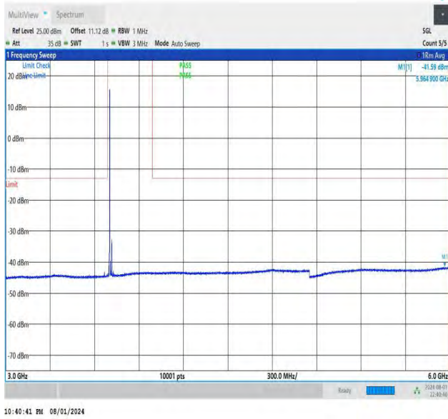
NTNV-DC_26A-n78A(3700-3800)-PC3-30-5+30-M+L-QPSK-IDL E-DFT-BPSK-Edge_1RB_Left-3000-6000-PASS
