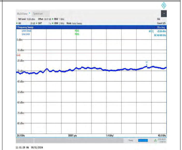
NTNV-DC_26A-n78A(3700-3800)-PC3-30-5+40-M+L-QPSK-IDLE -DFT-QPSK-Edge_1RB_Right-26000-40000-PASS
