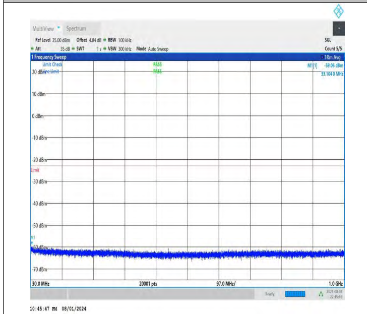
NTNV-DC_26A-n78A(3700-3800)-PC3-30-5+30-M+M-QPSK-IDL E-DFT-BPSK-Edge_1RB_Left-30-1000-PASS
