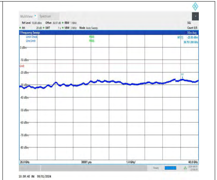
NTNV-DC_26A-n78A(3700-3800)-PC3-30-5+40-M+L-QPSK-IDLE -DFT-BPSK-Edge_1RB_Right-26000-40000-PASS
