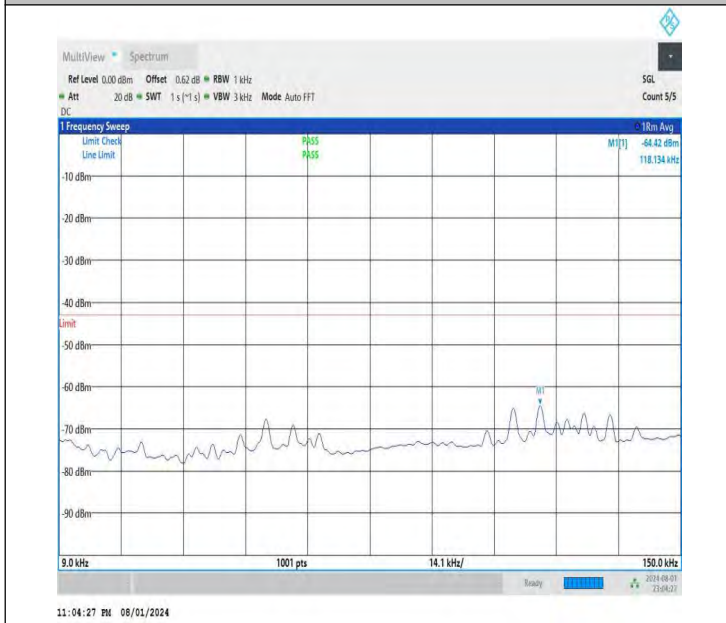
NTNV-DC_26A-n78A(3700-3800)-PC3-30-5+40-M+M-QPSK-IDL E-DFT-QPSK-Edge_1RB_Left-0.009-0.15-PASS
