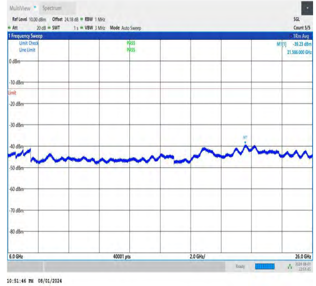
NTNV-DC_26A-n78A(3700-3800)-PC3-30-5+30-M+H-QPSK-IDLE -DFT-BPSK-Edge_1RB_Left-6000-26000-PASS
