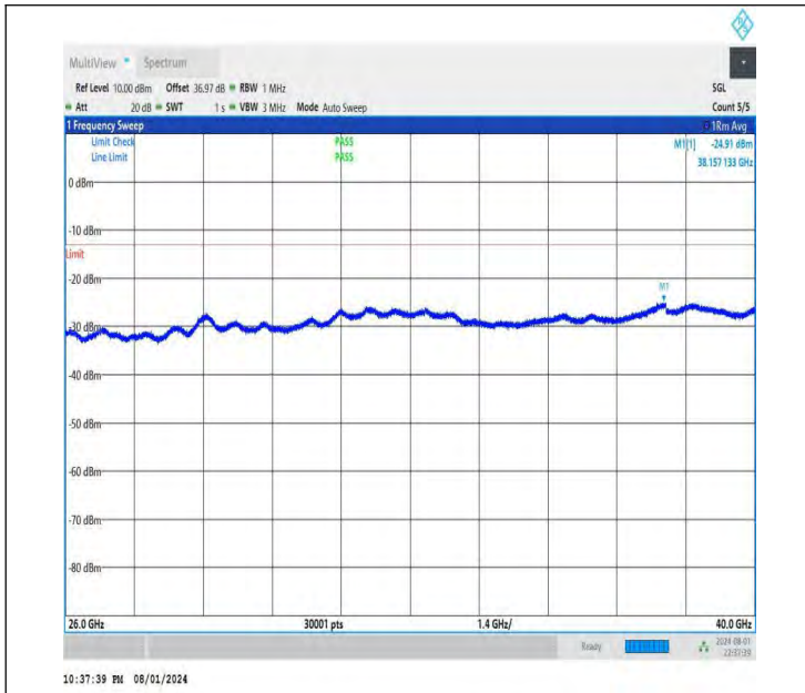
NTNV-DC_26A-n78A(3700-3800)-PC3-30-5+20-M+H-QPSK-IDL E-DFT-QPSK-Edge_1RB_Left-26000-40000-PASS
