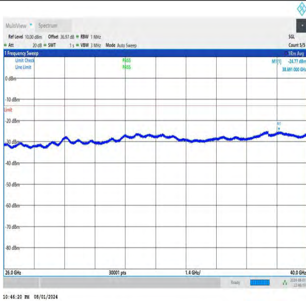
NTNV-DC_26A-n78A(3700-3800)-PC3-30-5+30-M+M-QPSK-IDL E-DFT-BPSK-Edge_1RB_Left-26000-40000-PASS
