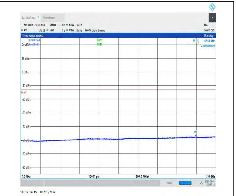
NTNV-DC_26A-n78A(3700-3800)-PC3-30-5+20-M+H-QPSK-IDLE -DFT-QPSK-Edge_1RB_Left-1000-3000-PASS
