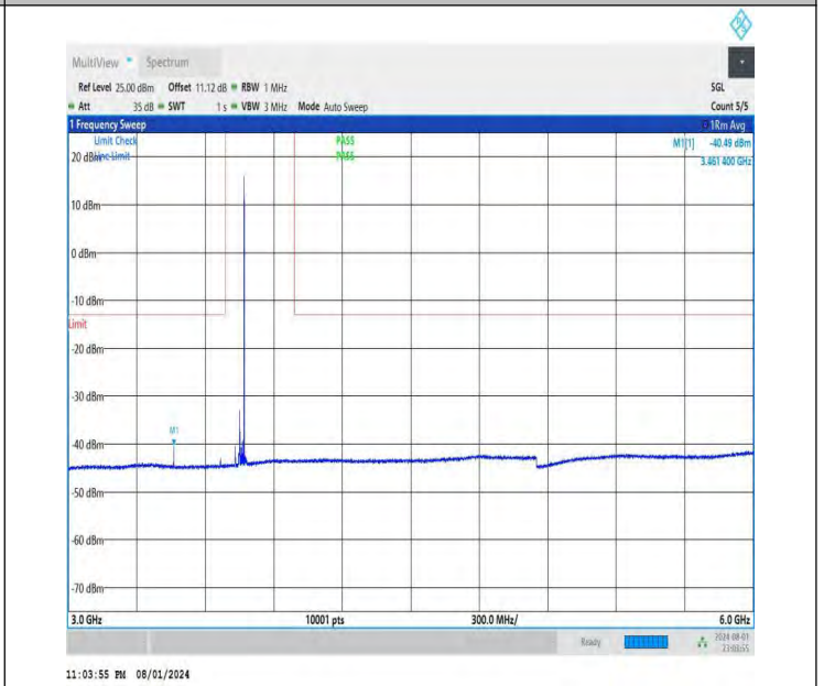
NTNV-DC_26A-n78A(3700-3800)-PC3-30-5+40-M+M-QPSK-IDLE -DFT-BPSK-Edge_1RB_Right-3000-6000-PASS
