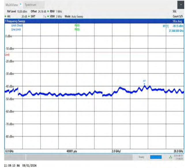
NTNV-DC_26A-n78A(3700-3800)-PC3-30-5+40-M+H-QPSK-IDLE -DFT-BPSK-Edge_1RB_Left-6000-26000-PASS
