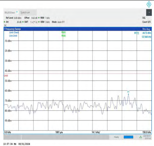
NTNV-DC_26A-n78A(3700-3800)-PC3-30-5+40-M+L-QPSK-IDLE -DFT-BPSK-Edge_1RB_Right-0.009-0.15-PASS
