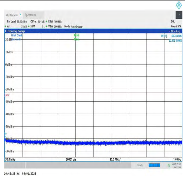
NTNV-DC_26A-n78A(3700-3800)-PC3-30-5+30-M+L-QPSK-IDLE -DFT-QPSK-Edge_1RB_Right-30-1000-PASS
