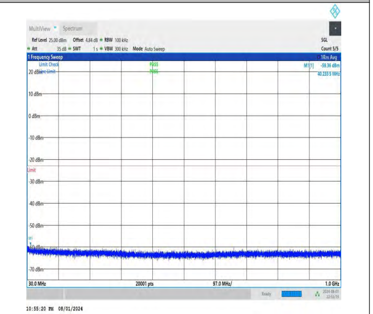
NTNV-DC_26A-n78A(3700-3800)-PC3-30-5+30-M+H-QPSK-IDLE -DFT-QPSK-Edge_1RB_Right-30-1000-PASS
