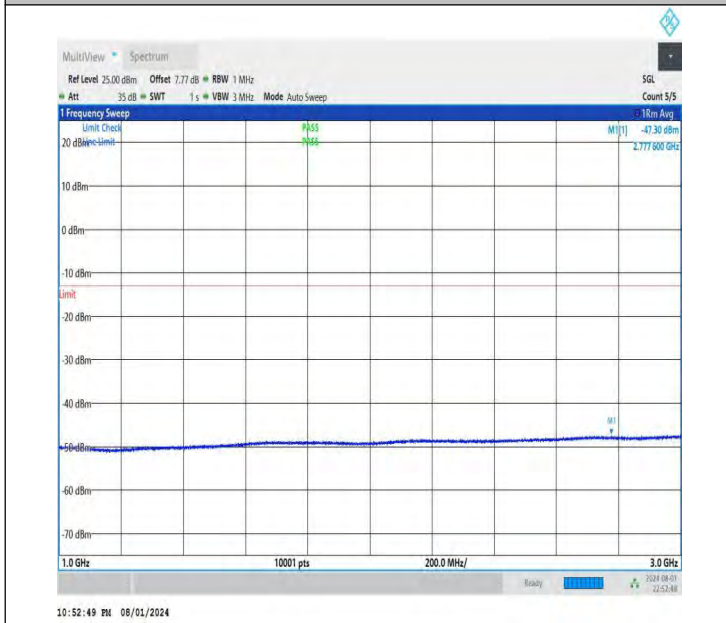
NTNV-DC_26A-n78A(3700-3800)-PC3-30-5+30-M+H-QPSK-IDL E-DFT-BPSK-Edge_1RB_Right-1000-3000-PASS
