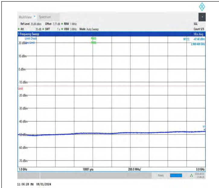
NTNV-DC_26A-n78A(3700-3800)-PC3-30-5+40-M+M-QPSK-IDL E-DFT-QPSK-Edge_1RB_Right-1000-3000-PASS
