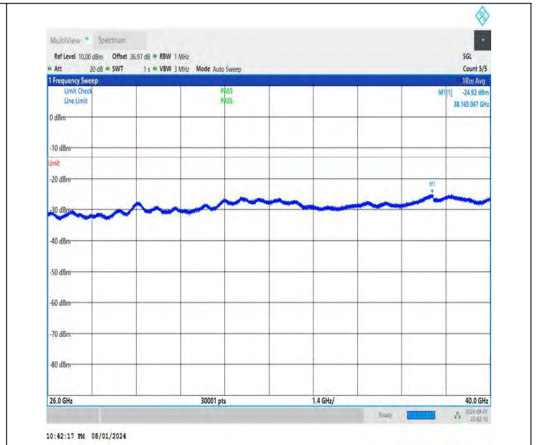
NTNV-DC_26A-n78A(3700-3800)-PC3-30-5+30-M+L-QPSK-IDLE -DFT-BPSK-Edge_1RB_Right-26000-40000-PASS
