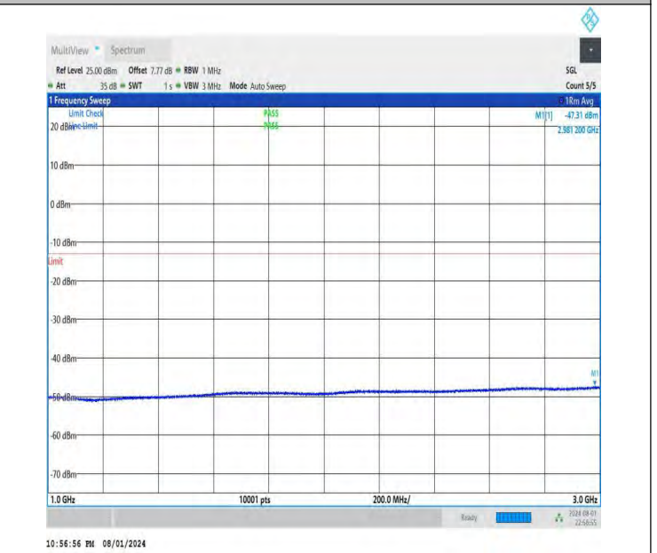
NTNV-DC_26A-n78A(3700-3800)-PC3-30-5+40-M+L-QPSK-IDLE -DFT-BPSK-Edge_1RB_Left-1000-3000-PASS
