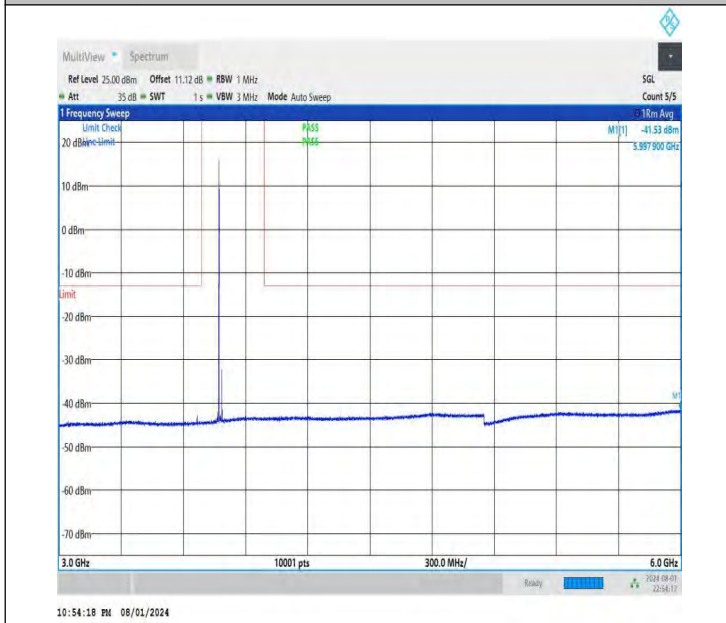
NTNV-DC_26A-n78A(3700-3800)-PC3-30-5+30-M+H-QPSK-IDL E-DFT-QPSK-Edge_1RB_Left-3000-6000-PASS
