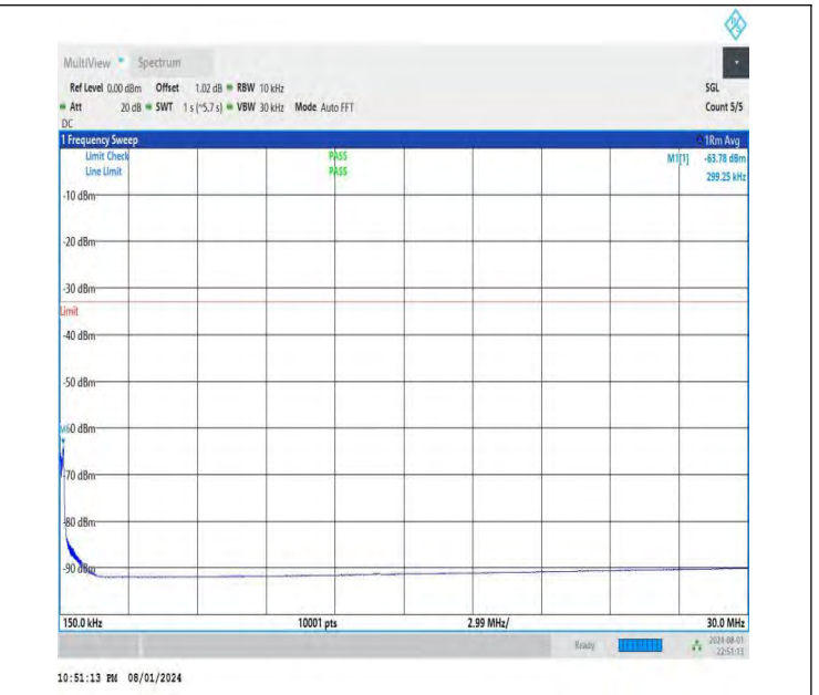
NTNV-DC_26A-n78A(3700-3800)-PC3-30-5+30-M+H-QPSK-IDLE -DFT-BPSK-Edge_1RB_Left-0.15-30-PASS
