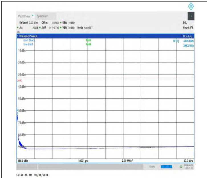
NTNV-DC_26A-n78A(3700-3800)-PC3-30-5+30-M+L-QPSK-IDL E-DFT-BPSK-Edge_1RB_Right-0.15-30-PASS
