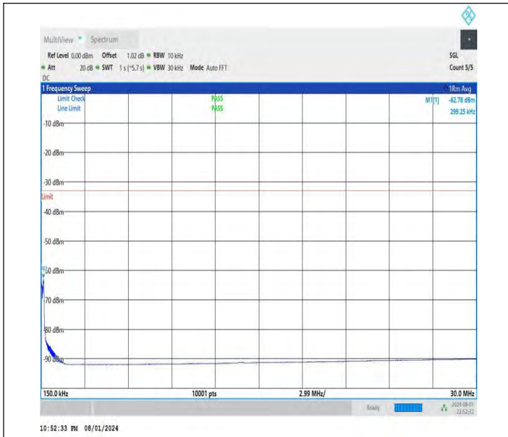
NTNV-DC_26A-n78A(3700-3800)-PC3-30-5+30-M+H-QPSK-IDL E-DFT-BPSK-Edge_1RB_Right-0.15-30-PASS
