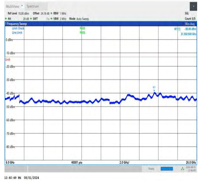
NTNV-DC_26A-n78A(3700-3800)-PC3-30-5+30-M+L-QPSK-IDLE -DFT-BPSK-Edge_1RB_Left-6000-26000-PASS
