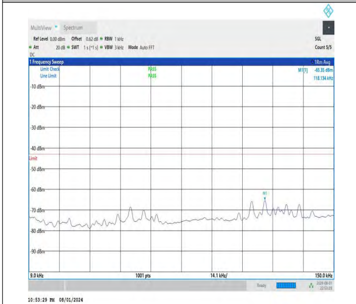
NTNV-DC_26A-n78A(3700-3800)-PC3-30-5+30-M+H-QPSK-IDL E-DFT-QPSK-Edge_1RB_Left-0.009-0.15-PASS
