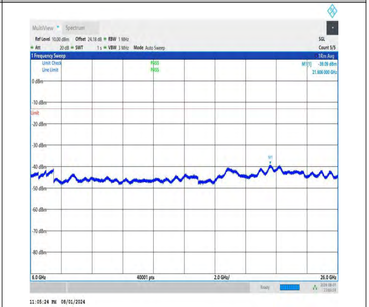
NTNV-DC_26A-n78A(3700-3800)-PC3-30-5+40-M+M-QPSK-IDLE -DFT-QPSK-Edge_1RB_Left-6000-26000-PASS
