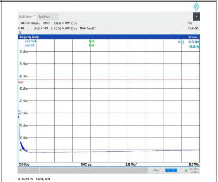
NTNV-DC_26A-n78A(3700-3800)-PC3-30-5+20-M+H-QPSK-IDLE -DFT-QPSK-Edge_1RB_Left-0.15-30-PASS
