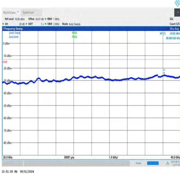
NTNV-DC_26A-n78A(3700-3800)-PC3-30-5+30-M+H-QPSK-IDL E-DFT-BPSK-Edge_1RB_Left-26000-40000-PASS
