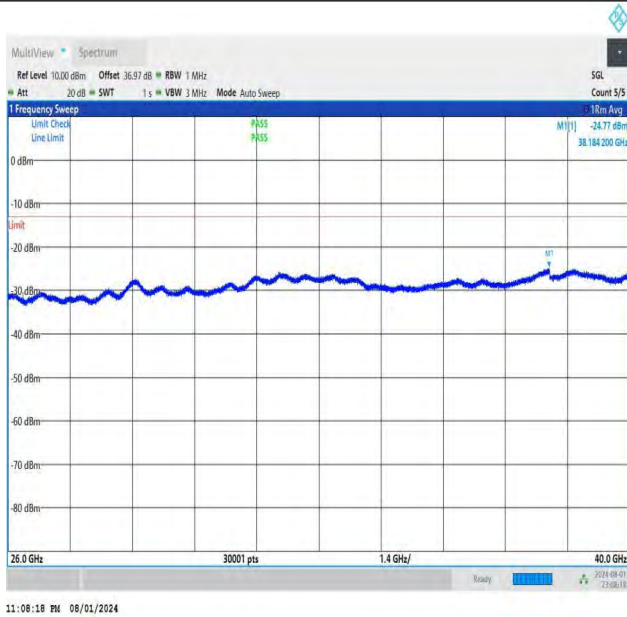
NTNV-DC_26A-n78A(3700-3800)-PC3-30-5+40-M+H-QPSK-IDL E-DFT-BPSK-Edge_1RB_Left-26000-40000-PASS
