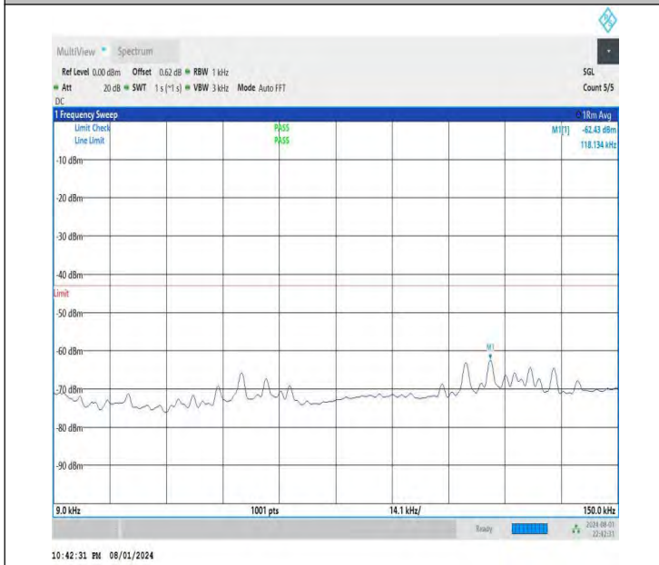
NTNV-DC_26A-n78A(3700-3800)-PC3-30-5+30-M+L-QPSK-IDL E-DFT-QPSK-Edge_1RB_Left-0.009-0.15-PASS
