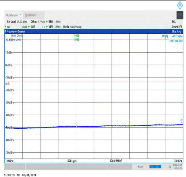
NTNV-DC_26A-n78A(3700-3800)-PC3-30-5+40-M+M-QPSK-IDLE -DFT-BPSK-Edge_1RB_Left-1000-3000-PASS
