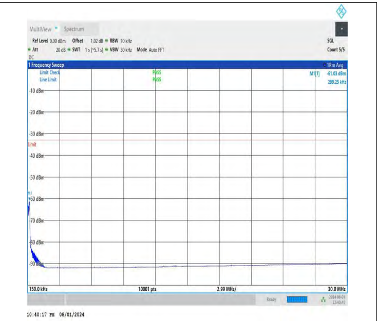
NTNV-DC_26A-n78A(3700-3800)-PC3-30-5+30-M+L-QPSK-IDLE -DFT-BPSK-Edge_1RB_Left-0.15-30-PASS
