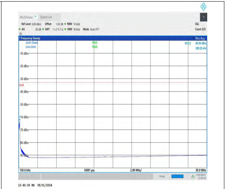
NTNV-DC_26A-n78A(3700-3800)-PC3-30-5+30-M+M-QPSK-IDLE -DFT-BPSK-Edge_1RB_Left-0.15-30-PASS
