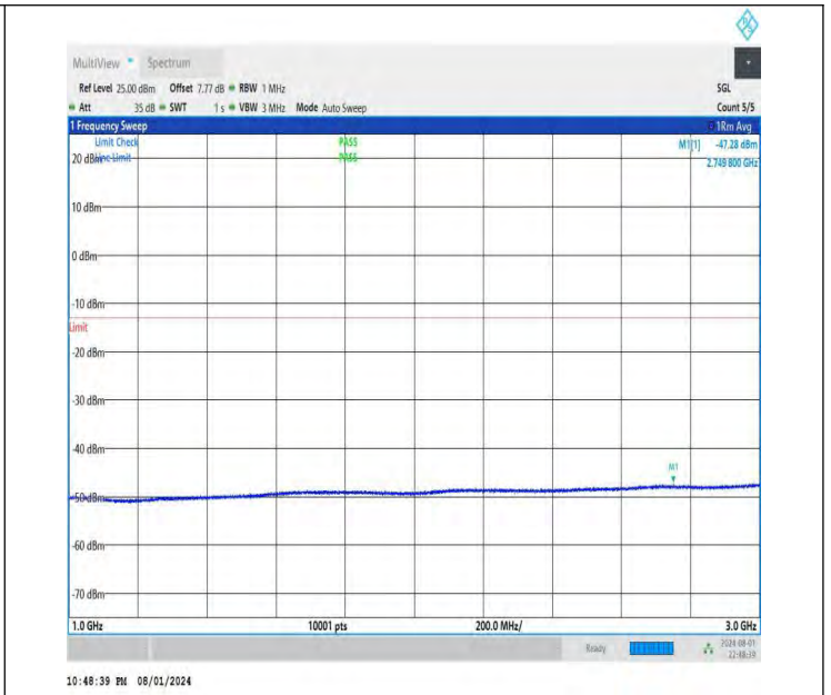
NTNV-DC_26A-n78A(3700-3800)-PC3-30-5+30-M+M-QPSK-IDLE -DFT-QPSK-Edge_1RB_Left-1000-3000-PASS
