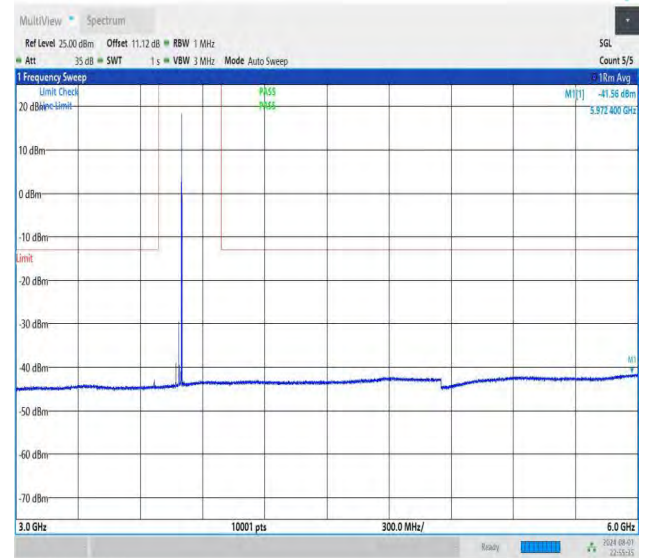
NTNV-DC_26A-n78A(3700-3800)-PC3-30-5+30-M+H-QPSK-IDLE -DFT-QPSK-Edge_1RB_Right-3000-6000-PASS
