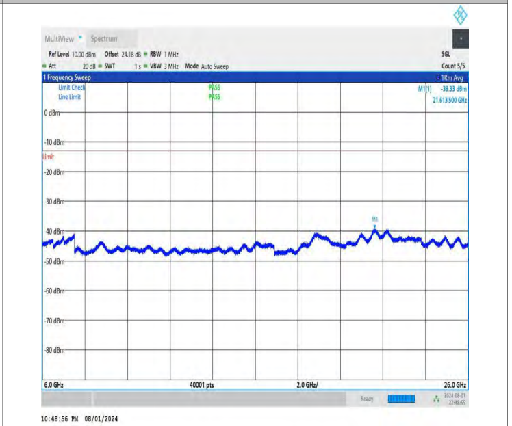
NTNV-DC_26A-n78A(3700-3800)-PC3-30-5+30-M+M-QPSK-IDLE -DFT-QPSK-Edge_1RB_Left-6000-26000-PASS
