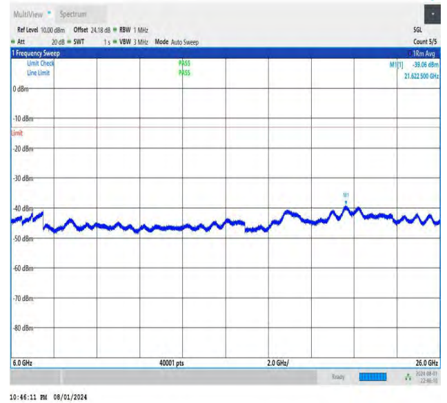
NTNV-DC_26A-n78A(3700-3800)-PC3-30-5+30-M+M-QPSK-IDLE -DFT-BPSK-Edge_1RB_Left-6000-26000-PASS
