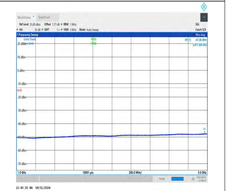
NTNV-DC_26A-n78A(3700-3800)-PC3-30-5+30-M+L-QPSK-IDLE -DFT-BPSK-Edge_1RB_Left-1000-3000-PASS
