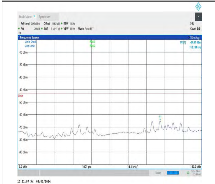
NTNV-DC_26A-n78A(3700-3800)-PC3-30-5+20-M+M-QPSK-IDL E-DFT-QPSK-Edge_1RB_Left-0.009-0.15-PASS
