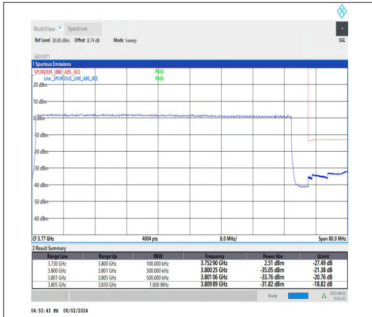
NTNV-DC_26A-n78A(3700-3800)-PC3-30-5+70-M+H-QPSK-IDLE -DFT-BPSK-Outer_Full-PASS
