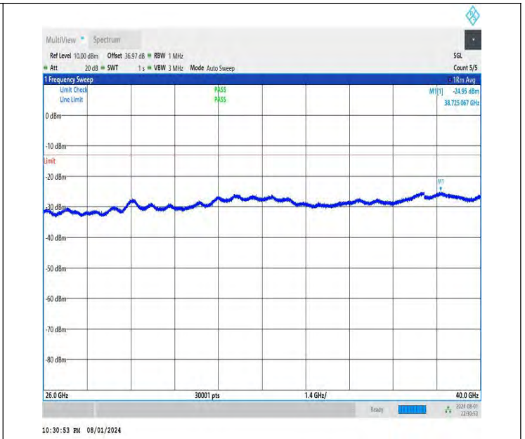
NTNV-DC_26A-n78A(3700-3800)-PC3-30-5+20-M+M-QPSK-IDLE -DFT-BPSK-Edge_1RB_Right-26000-40000-PASS
