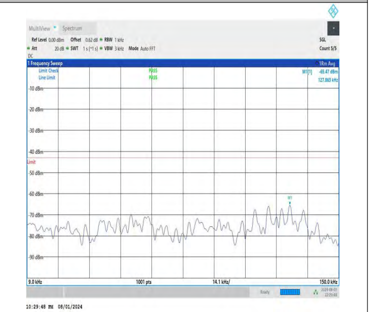
NTNV-DC_26A-n78A(3700-3800)-PC3-30-5+20-M+M-QPSK-IDLE -DFT-BPSK-Edge_1RB_Right-0.009-0.15-PASS
