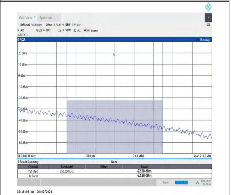
NTNV-DC_26A-n78A(3700-3800)-PC3-30-5+100-M+H-QPSK-IDL E-DFT-BPSK-Edge_1RB_Right-PASS_Final1
