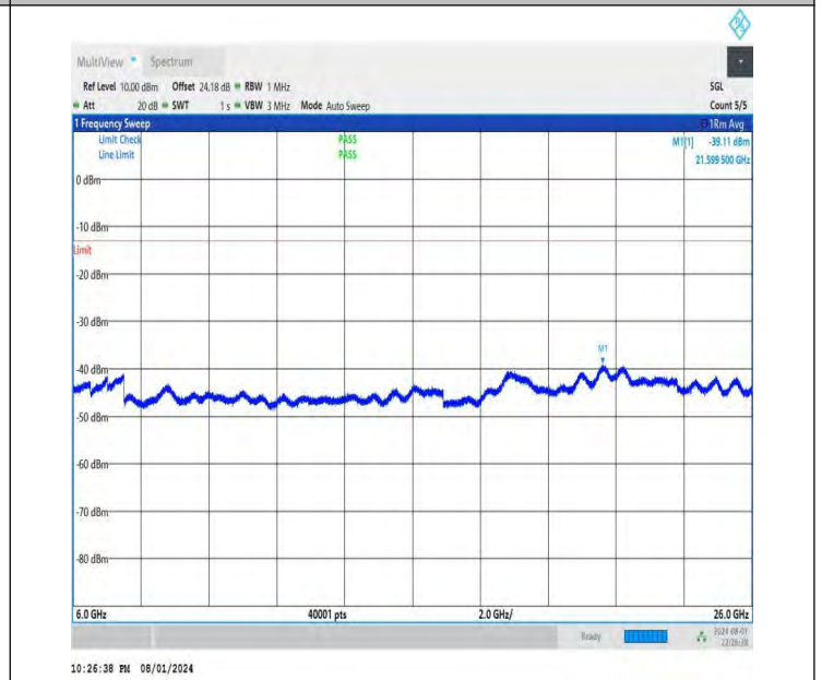
NTNV-DC_26A-n78A(3700-3800)-PC3-30-5+20-M+L-QPSK-IDLE -DFT-QPSK-Edge_1RB_Left-6000-26000-PASS
