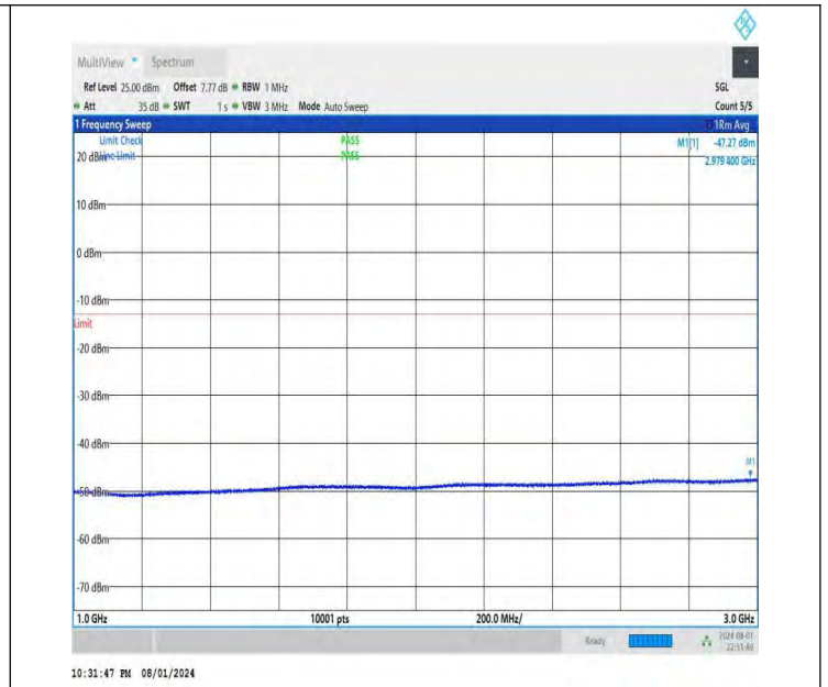
NTNV-DC_26A-n78A(3700-3800)-PC3-30-5+20-M+M-QPSK-IDLE -DFT-QPSK-Edge_1RB_Left-1000-3000-PASS
