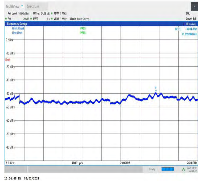
NTNV-DC_26A-n78A(3700-3800)-PC3-30-5+20-M+H-QPSK-IDLE -DFT-BPSK-Edge_1RB_Left-6000-26000-PASS
