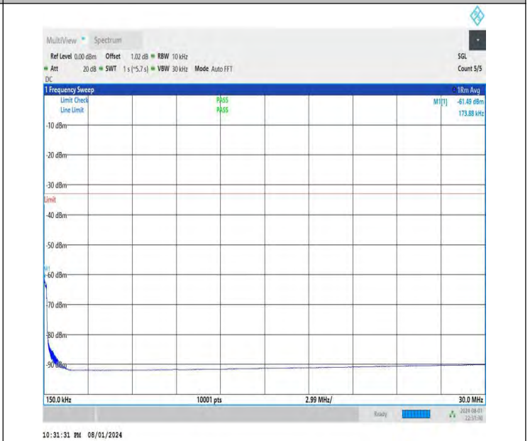
NTNV-DC_26A-n78A(3700-3800)-PC3-30-5+20-M+M-QPSK-IDLE -DFT-QPSK-Edge_1RB_Left-0.15-30-PASS
