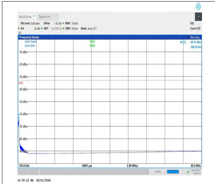
NTNV-DC_26A-n78A(3700-3800)-PC3-30-5+20-M+M-QPSK-IDL E-DFT-BPSK-Edge_1RB_Right-0.15-30-PASS
