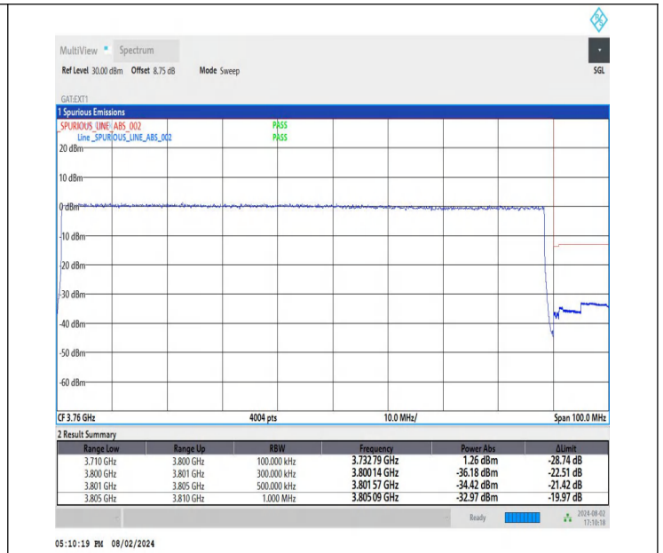
NTNV-DC_26A-n78A(3700-3800)-PC3-30-5+90-M+H-QPSK-IDLE E-DFT-BPSK-Outer_Full-PASS
