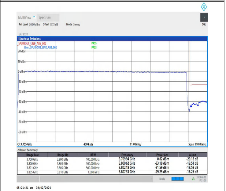
NTNV-DC_26A-n78A(3700-3800)-PC3-30-5+100-M+H-QPSK-IDL E-DFT-QPSK-Outer_Full-PASS
