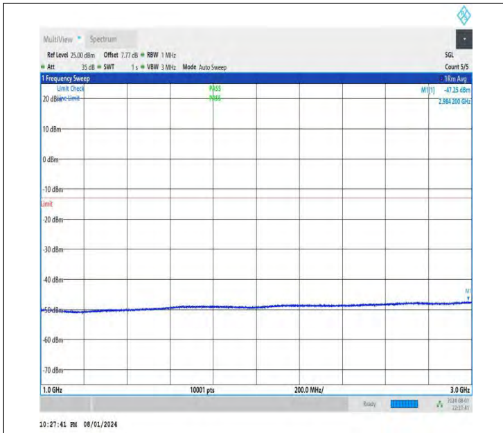
NTNV-DC_26A-n78A(3700-3800)-PC3-30-5+20-M+L-QPSK-IDL E-DFT-QPSK-Edge_1RB_Right-1000-3000-PASS
