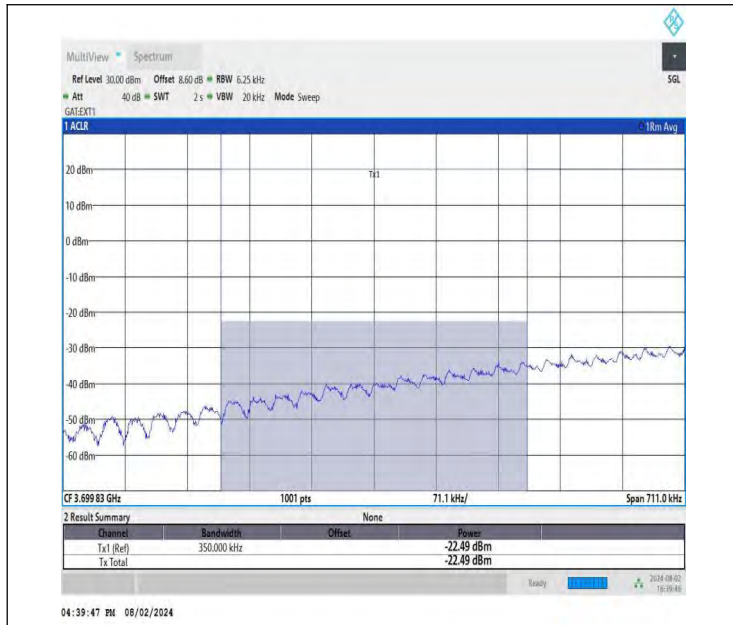
NTNV-DC_26A-n78A(3700-3800)-PC3-30-5+60-M+L-QPSK-IDLE -DFT-BPSK-Edge_1RB_Left-PASS_Final1
