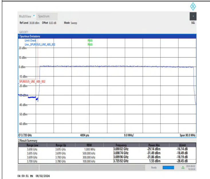
NTNV-DC_26A-n78A(3700-3800)-PC3-30-5+80-M+L-QPSK-IDLE -DFT-QPSK-Outer_Full-PASS
