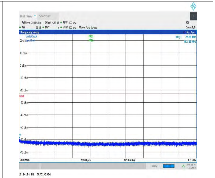
NTNV-DC_26A-n78A(3700-3800)-PC3-30-5+20-M+L-QPSK-IDLE -DFT-BPSK-Edge_1RB_Right-30-1000-PASS
