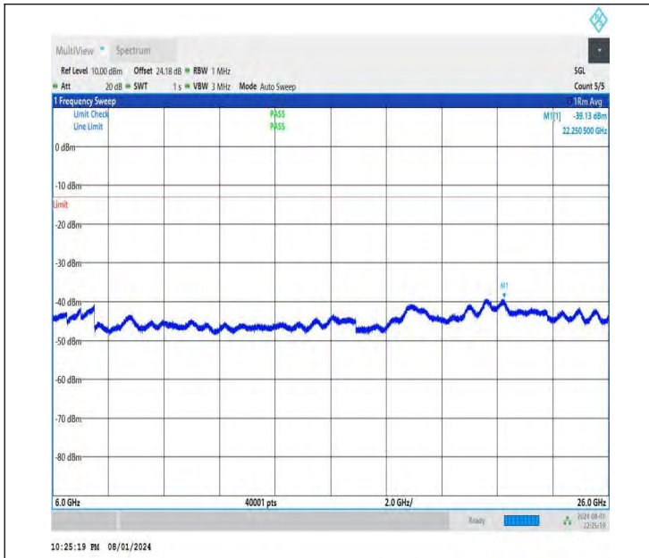
NTNV-DC_26A-n78A(3700-3800)-PC3-30-5+20-M+L-QPSK-IDL E-DFT-BPSK-Edge_1RB_Right-6000-26000-PASS
