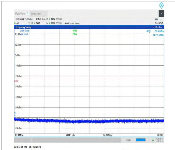
NTNV-DC_26A-n78A(3700-3800)-PC3-30-5+20-M+L-QPSK-IDL E-DFT-QPSK-Edge_1RB_Left-30-1000-PASS
