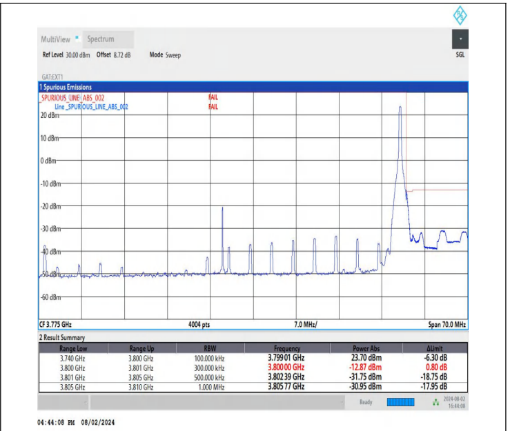
NTNV-DC_26A-n78A(3700-3800)-PC3-30-5+60-M+H-QPSK-IDL E-DFT-BPSK-Edge_1RB_Right-FAIL
