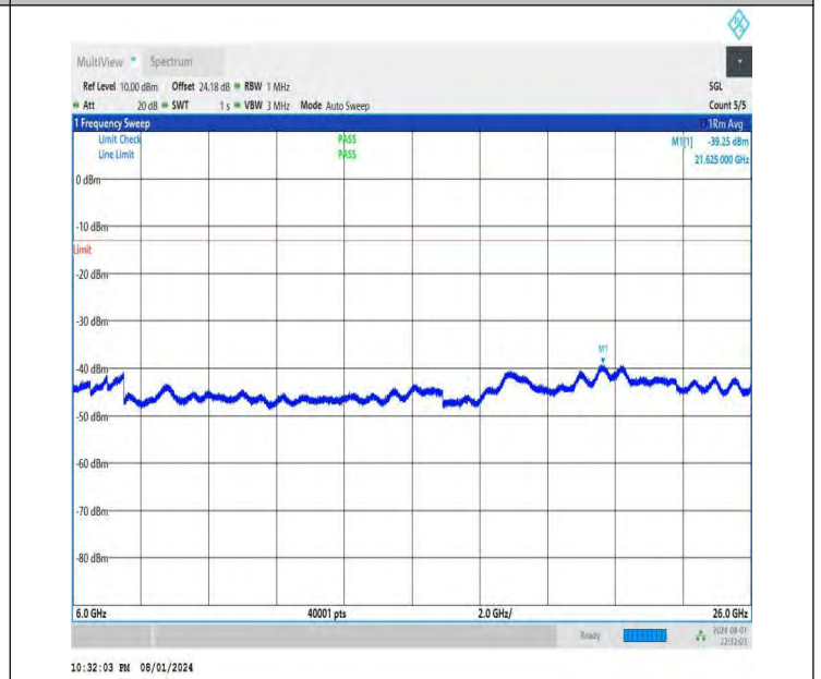
NTNV-DC_26A-n78A(3700-3800)-PC3-30-5+20-M+M-QPSK-IDLE -DFT-QPSK-Edge_1RB_Left-6000-26000-PASS
