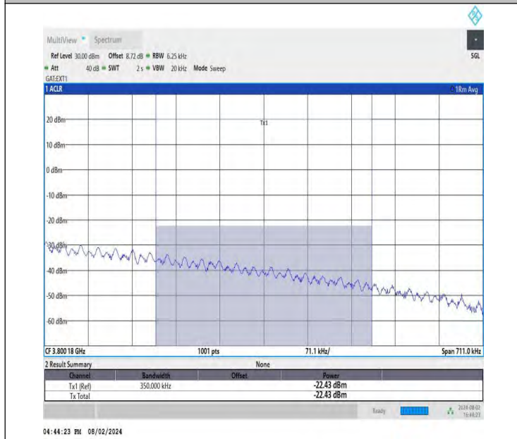
NTNV-DC_26A-n78A(3700-3800)-PC3-30-5+60-M+H-QPSK-IDLE -DFT-BPSK-Edge_1RB_Right-PASS_Final1
