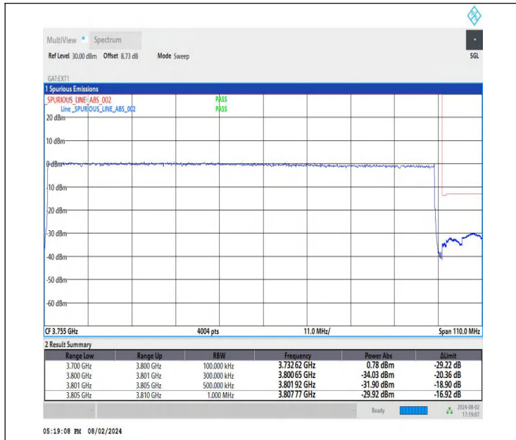
NTNV-DC_26A-n78A(3700-3800)-PC3-30-5+100-M+H-QPSK-IDL E-DFT-BPSK-Outer_Full-PASS
