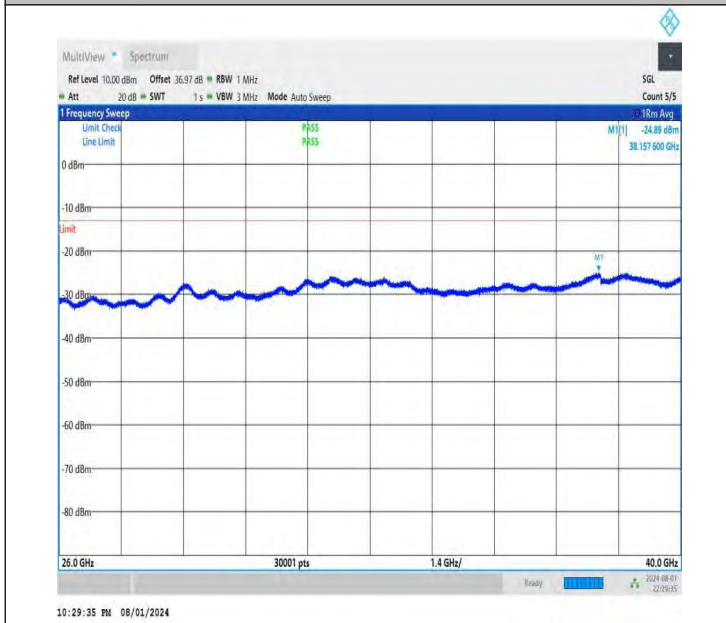
NTNV-DC_26A-n78A(3700-3800)-PC3-30-5+20-M+M-QPSK-IDL E-DFT-BPSK-Edge_1RB_Left-26000-40000-PASS
