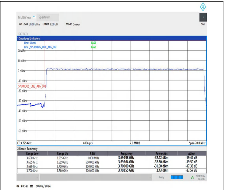
NTNV-DC_26A-n78A(3700-3800)-PC3-30-5+60-M+L-QPSK-IDLE -DFT-BPSK-Outer_Full-PASS
