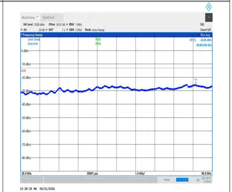
NTNV-DC_26A-n78A(3700-3800)-PC3-30-5+20-M+L-QPSK-IDLE -DFT-QPSK-Edge_1RB_Right-26000-40000-PASS
