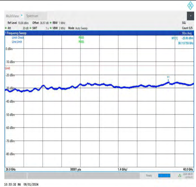
NTNV-DC_26A-n78A(3700-3800)-PC3-30-5+20-M+M-QPSK-IDLE -DFT-QPSK-Edge_1RB_Right-26000-40000-PASS
