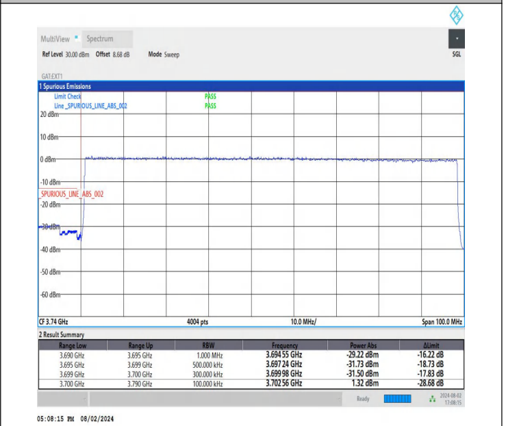
NTNV-DC_26A-n78A(3700-3800)-PC3-30-5+90-M+L-QPSK-IDLE -DFT-QPSK-Outer_Full-PASS
