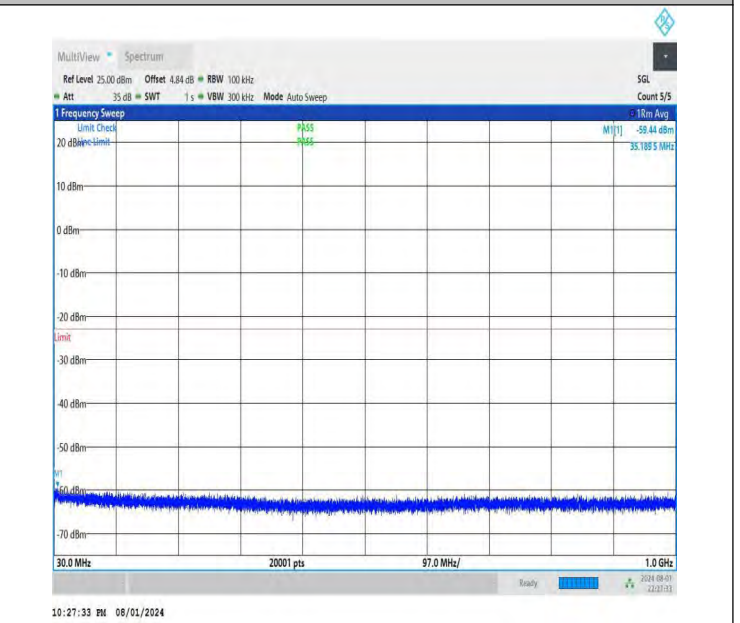
NTNV-DC_26A-n78A(3700-3800)-PC3-30-5+20-M+L-QPSK-IDLE -DFT-QPSK-Edge_1RB_Right-30-1000-PASS
