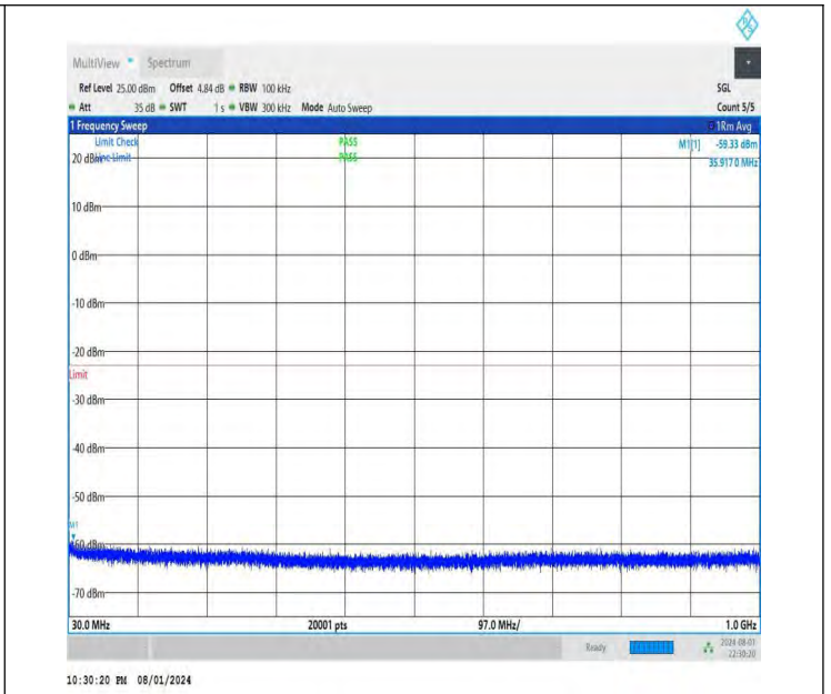
NTNV-DC_26A-n78A(3700-3800)-PC3-30-5+20-M+M-QPSK-IDLE -DFT-BPSK-Edge_1RB_Right-30-1000-PASS
