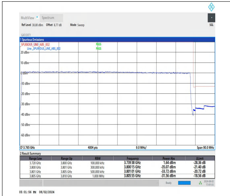
NTNV-DC_26A-n78A(3700-3800)-PC3-30-5+80-M+H-QPSK-IDLE -DFT-BPSK-Outer_Full-PASS
