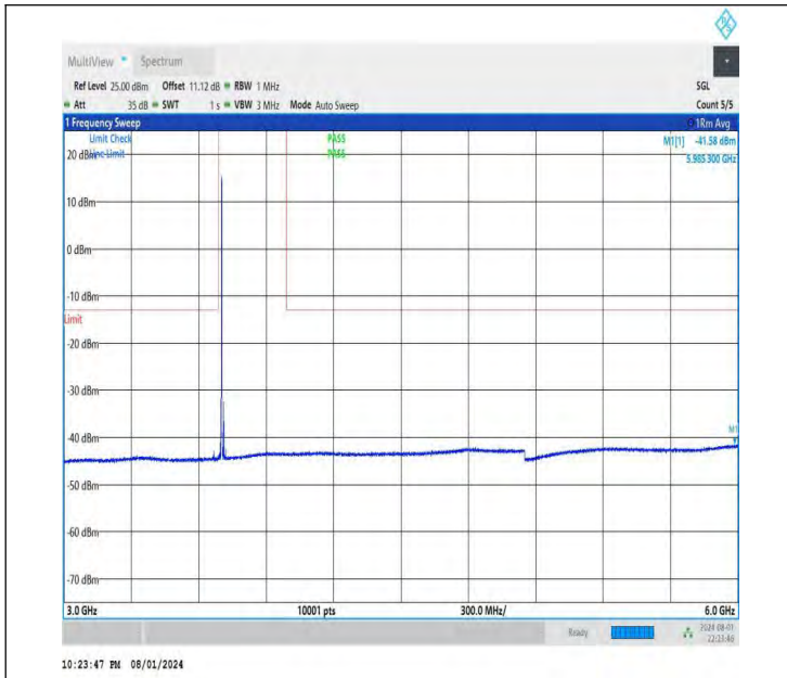
NTNV-DC_26A-n78A(3700-3800)-PC3-30-5+20-M+L-QPSK-IDL E-DFT-BPSK-Edge_1RB_Left-3000-6000-PASS
