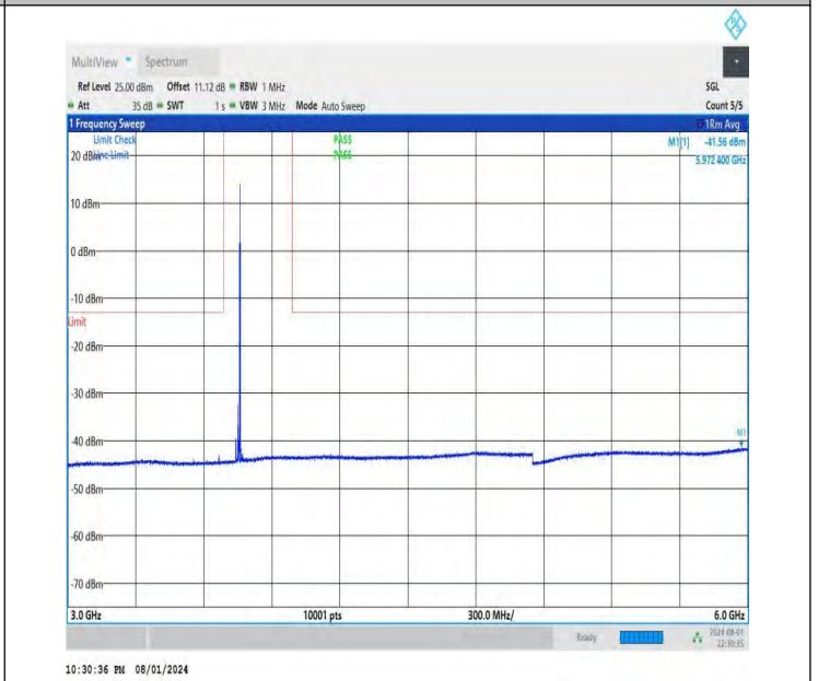
NTNV-DC_26A-n78A(3700-3800)-PC3-30-5+20-M+M-QPSK-IDLE -DFT-BPSK-Edge_1RB_Right-3000-6000-PASS
