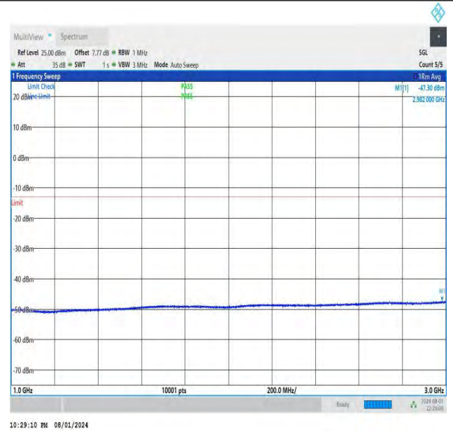
NTNV-DC_26A-n78A(3700-3800)-PC3-30-5+20-M+M-QPSK-IDLE -DFT-BPSK-Edge_1RB_Left-1000-3000-PASS
