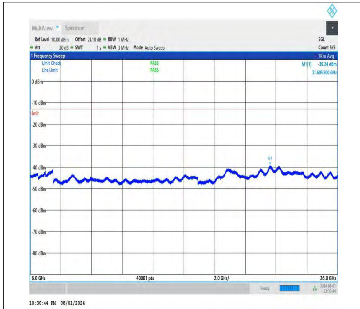
NTNV-DC_26A-n78A(3700-3800)-PC3-30-5+20-M+M-QPSK-IDL E-DFT-BPSK-Edge_1RB_Right-6000-26000-PASS
