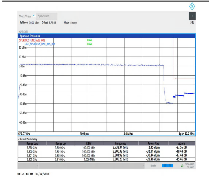
NTNV-DC_26A-n78A(3700-3800)-PC3-30-5+70-M+H-QPSK-IDLE -DFT-QPSK-Outer_Full-PASS
