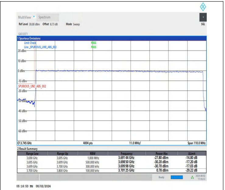
NTNV-DC_26A-n78A(3700-3800)-PC3-30-5+100-M+L-QPSK-IDL E-DFT-QPSK-Outer_Full-PASS
