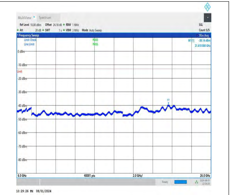
NTNV-DC_26A-n78A(3700-3800)-PC3-30-5+20-M+M-QPSK-IDLE -DFT-BPSK-Edge_1RB_Left-6000-26000-PASS
