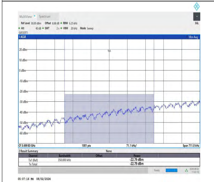
NTNV-DC_26A-n78A(3700-3800)-PC3-30-5+90-M+L-QPSK-IDLE -DFT-QPSK-Edge_1RB_Left-PASS_Final1
