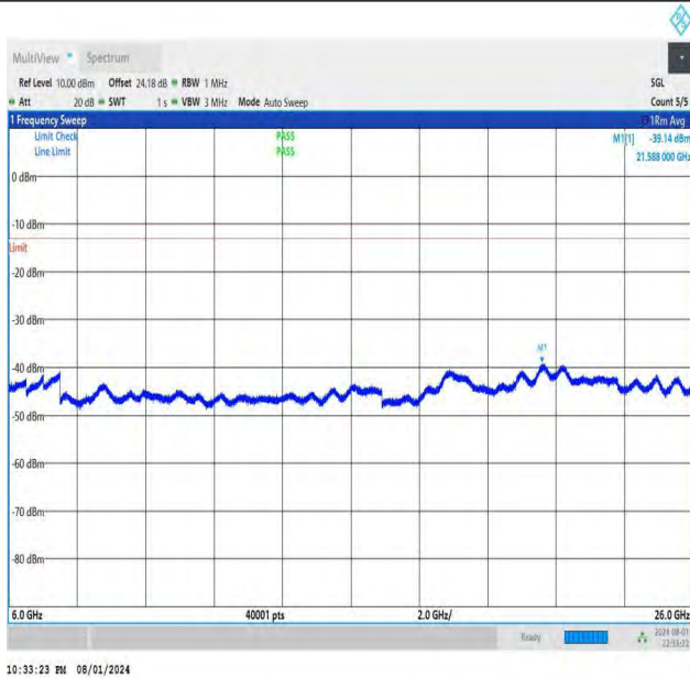
NTNV-DC_26A-n78A(3700-3800)-PC3-30-5+20-M+M-QPSK-IDL E-DFT-QPSK-Edge_1RB_Right-6000-26000-PASS
