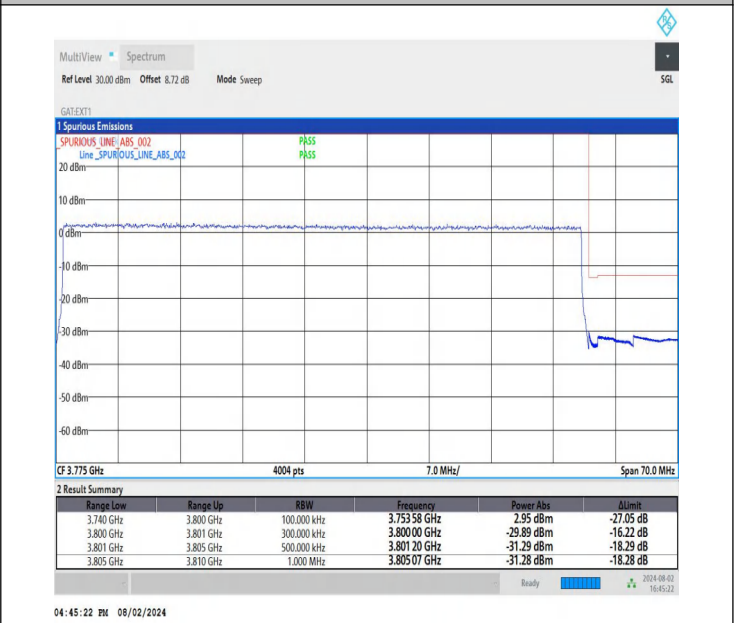
NTNV-DC_26A-n78A(3700-3800)-PC3-30-5+60-M+H-QPSK-IDL E-DFT-BPSK-Outer_Full-PASS
