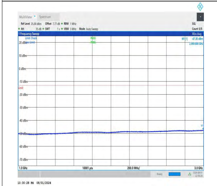
NTNV-DC_26A-n78A(3700-3800)-PC3-30-5+20-M+M-QPSK-IDL E-DFT-BPSK-Edge_1RB_Right-1000-3000-PASS
