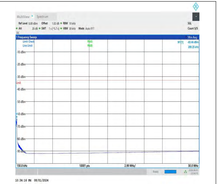
NTNV-DC_26A-n78A(3700-3800)-PC3-30-5+20-M+H-QPSK-IDLE -DFT-BPSK-Edge_1RB_Left-0.15-30-PASS
