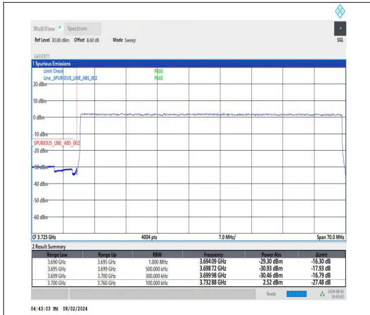
NTNV-DC_26A-n78A(3700-3800)-PC3-30-5+60-M+L-QPSK-IDLE -DFT-QPSK-Outer_Full-PASS
