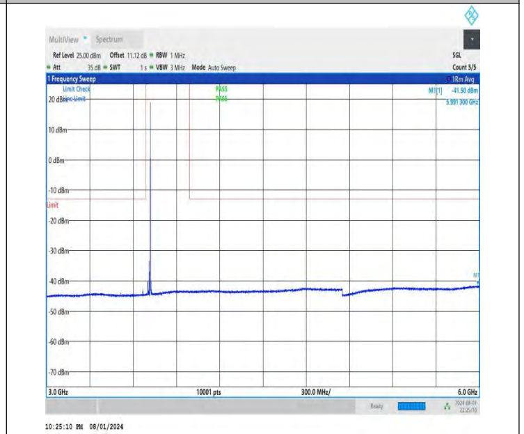
NTNV-DC_26A-n78A(3700-3800)-PC3-30-5+20-M+L-QPSK-IDLE -DFT-BPSK-Edge_1RB_Right-PASS
