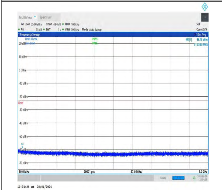
NTNV-DC_26A-n78A(3700-3800)-PC3-30-5+20-M+H-QPSK-IDL E-DFT-BPSK-Edge_1RB_Left-30-1000-PASS
