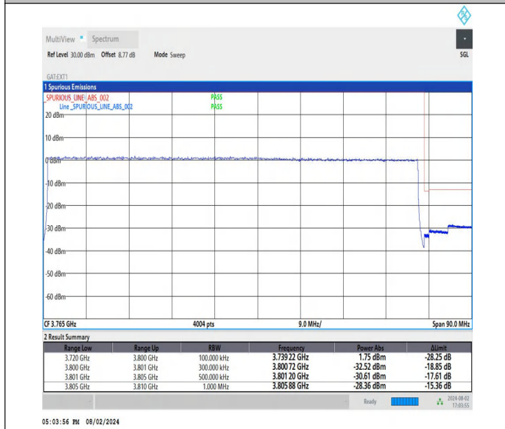
NTNV-DC_26A-n78A(3700-3800)-PC3-30-5+80-M+H-QPSK-IDLE -DFT-QPSK-Outer_Full-PASS
