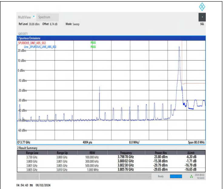
NTNV-DC_26A-n78A(3700-3800)-PC3-30-5+70-M+H-QPSK-IDLE E-DFT-QPSK-Edge_1RB_Right-PASS
