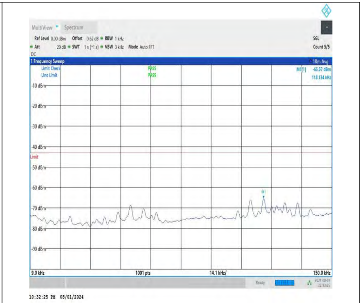
NTNV-DC_26A-n78A(3700-3800)-PC3-30-5+20-M+M-QPSK-IDLE -DFT-QPSK-Edge_1RB_Right-0.009-0.15-PASS
