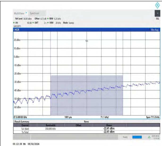
NTNV-DC_26A-n78A(3700-3800)-PC3-30-5+100-M+L-QPSK-IDL E-DFT-BPSK-Edge_1RB_Left-PASS_Final1
