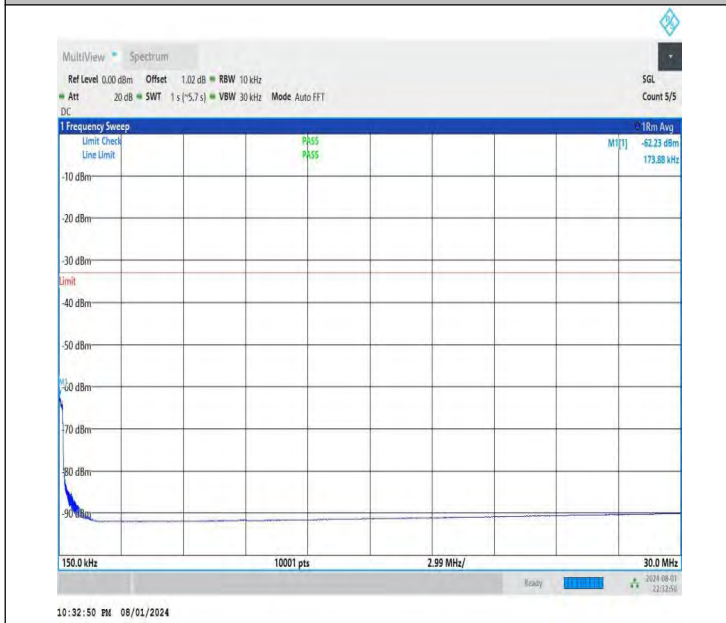
NTNV-DC_26A-n78A(3700-3800)-PC3-30-5+20-M+M-QPSK-IDL E-DFT-QPSK-Edge_1RB_Right-0.15-30-PASS
