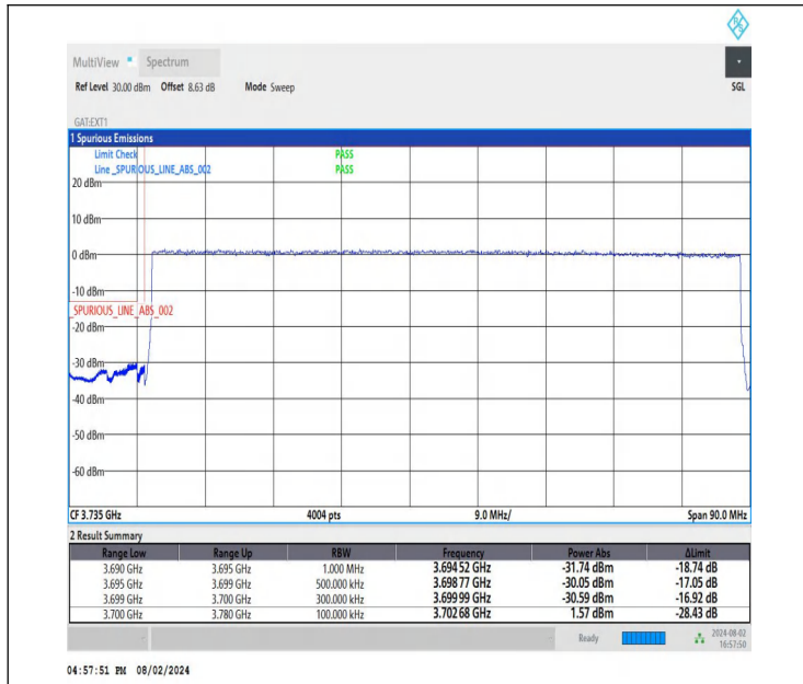
NTNV-DC_26A-n78A(3700-3800)-PC3-30-5+80-M+L-QPSK-IDLE -DFT-BPSK-Outer_Full-PASS
