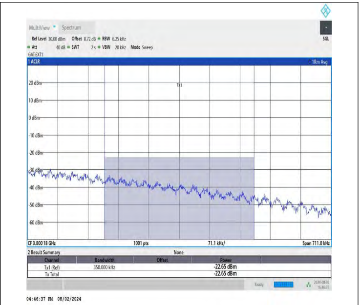
NTNV-DC_26A-n78A(3700-3800)-PC3-30-5+60-M+H-QPSK-IDLE E-DFT-QPSK-Edge_1RB_Right-PASS_Final1
