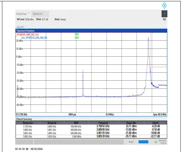
NTNV-DC_26A-n78A(3700-3800)-PC3-30-5+80-M+H-QPSK-IDLE E-DFT-QPSK-Edge_1RB_Right-PASS
