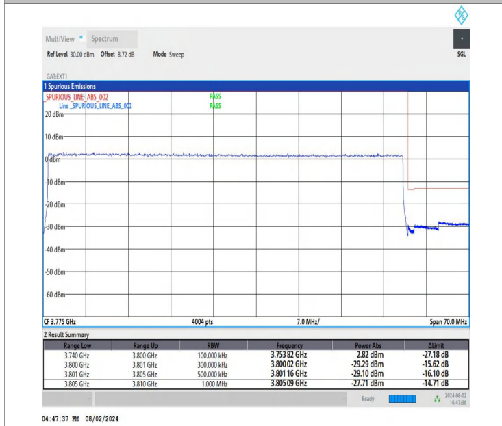
NTNV-DC_26A-n78A(3700-3800)-PC3-30-5+60-M+H-QPSK-IDLE -DFT-QPSK-Outer_Full-PASS
