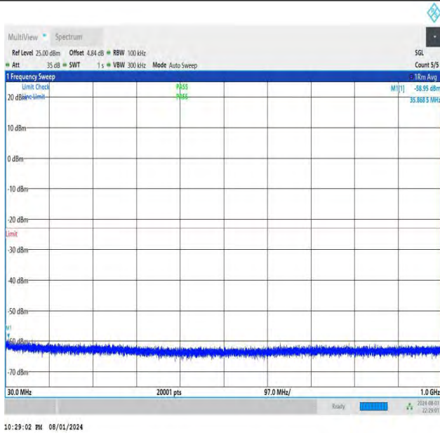
NTNV-DC_26A-n78A(3700-3800)-PC3-30-5+20-M+M-QPSK-IDL E-DFT-BPSK-Edge_1RB_Left-30-1000-PASS
