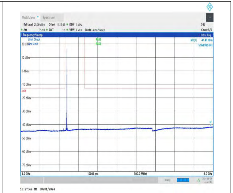
NTNV-DC_26A-n78A(3700-3800)-PC3-30-5+20-M+L-QPSK-IDLE -DFT-QPSK-Edge_1RB_Right-3000-6000-PASS
