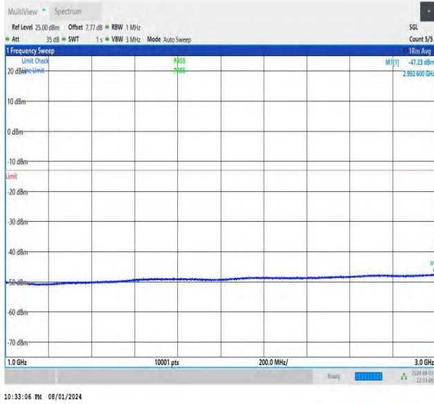
NTNV-DC_26A-n78A(3700-3800)-PC3-30-5+20-M+M-QPSK-IDL E-DFT-QPSK-Edge_1RB_Right-1000-3000-PASS
