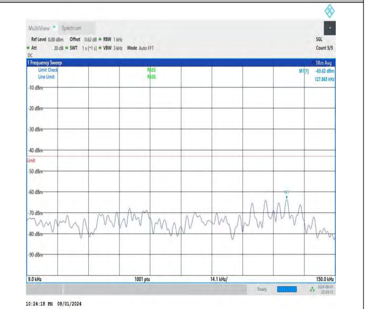
NTNV-DC_26A-n78A(3700-3800)-PC3-30-5+20-M+L-QPSK-IDLE -DFT-BPSK-Edge_1RB_Right-0.009-0.15-PASS
