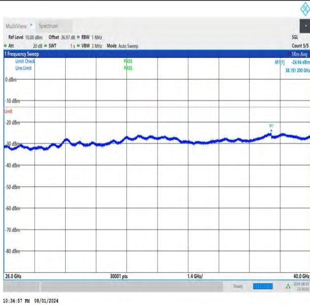
NTNV-DC_26A-n78A(3700-3800)-PC3-30-5+20-M+H-QPSK-IDL E-DFT-BPSK-Edge_1RB_Left-26000-40000-PASS
