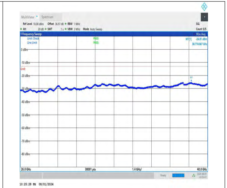
NTNV-DC_26A-n78A(3700-3800)-PC3-30-5+20-M+L-QPSK-IDLE -DFT-BPSK-Edge_1RB_Right-26000-40000-PASS
