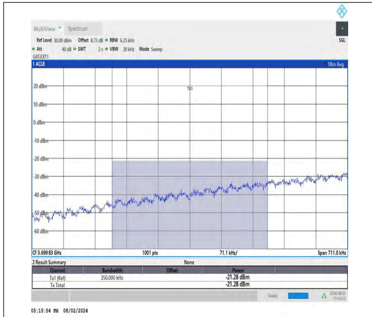
NTNV-DC_26A-n78A(3700-3800)-PC3-30-5+100-M+L-QPSK-IDL E-DFT-QPSK-Edge_1RB_Left-PASS_Final1
