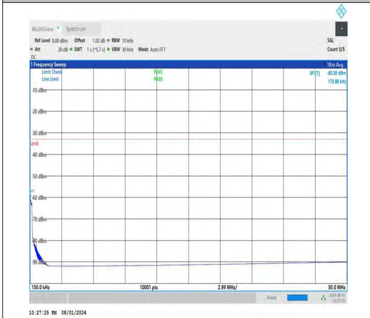
NTNV-DC_26A-n78A(3700-3800)-PC3-30-5+20-M+L-QPSK-IDL E-DFT-QPSK-Edge_1RB_Right-0.15-30-PASS
