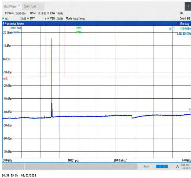
NTNV-DC_26A-n78A(3700-3800)-PC3-30-5+20-M+H-QPSK-IDL E-DFT-BPSK-Edge_1RB_Left-3000-6000-PASS
