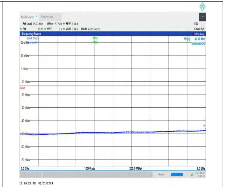
NTNV-DC_26A-n78A(3700-3800)-PC3-30-5+20-M+L-QPSK-IDLE -DFT-QPSK-Edge_1RB_Left-1000-3000-PASS
