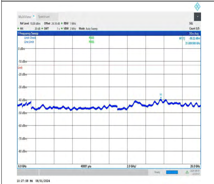
NTNV-DC_26A-n78A(3700-3800)-PC3-30-5+20-M+L-QPSK-IDL E-DFT-QPSK-Edge_1RB_Right-6000-26000-PASS
