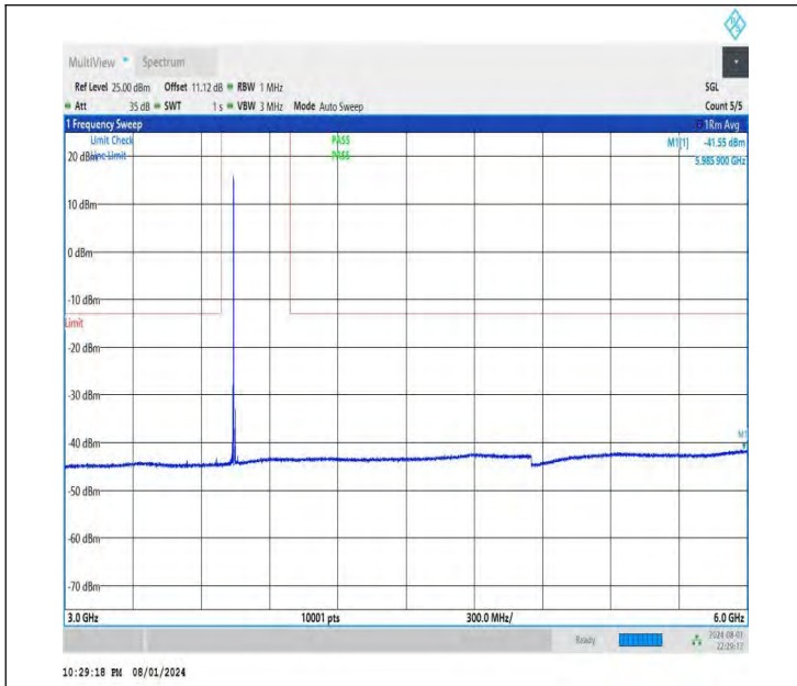
NTNV-DC_26A-n78A(3700-3800)-PC3-30-5+20-M+M-QPSK-IDL E-DFT-BPSK-Edge_1RB_Left-3000-6000-PASS
