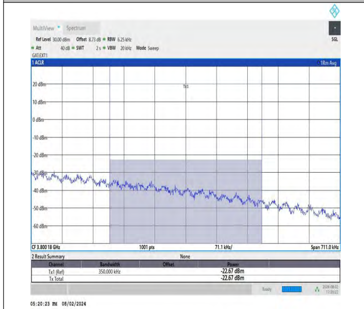
NTNV-DC_26A-n78A(3700-3800)-PC3-30-5+100-M+H-QPSK-IDL E-DFT-QPSK-Edge_1RB_Right-PASS_Final1
