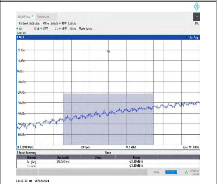
NTNV-DC_26A-n78A(3700-3800)-PC3-30-5+60-M+L-QPSK-IDLE -DFT-QPSK-Edge_1RB_Left-PASS_Final1
