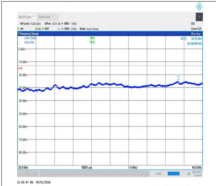
NTNV-DC_26A-n78A(3700-3800)-PC3-30-5+20-M+L-QPSK-IDL E-DFT-QPSK-Edge_1RB_Left-26000-40000-PASS
