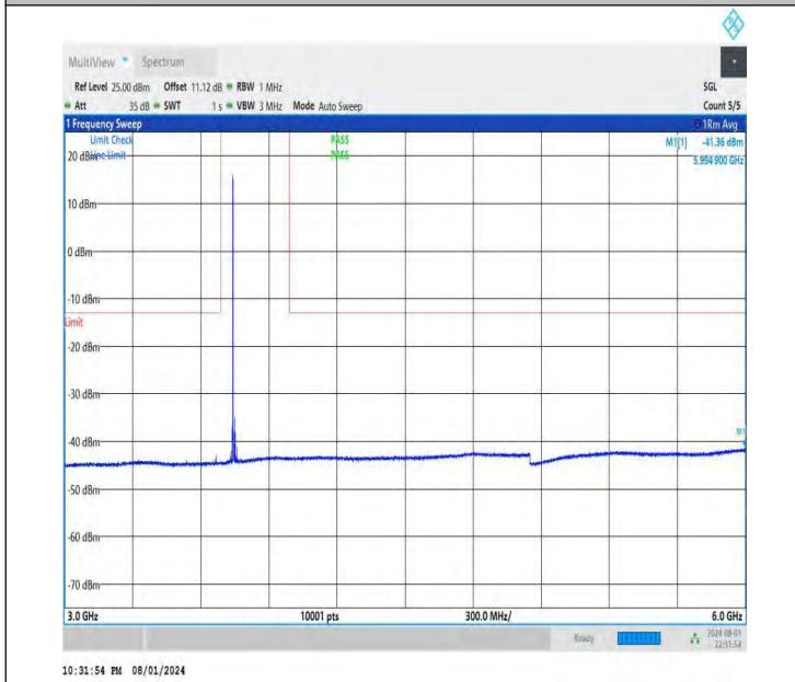
NTNV-DC_26A-n78A(3700-3800)-PC3-30-5+20-M+M-QPSK-IDL E-DFT-QPSK-Edge_1RB_Left-3000-6000-PASS
