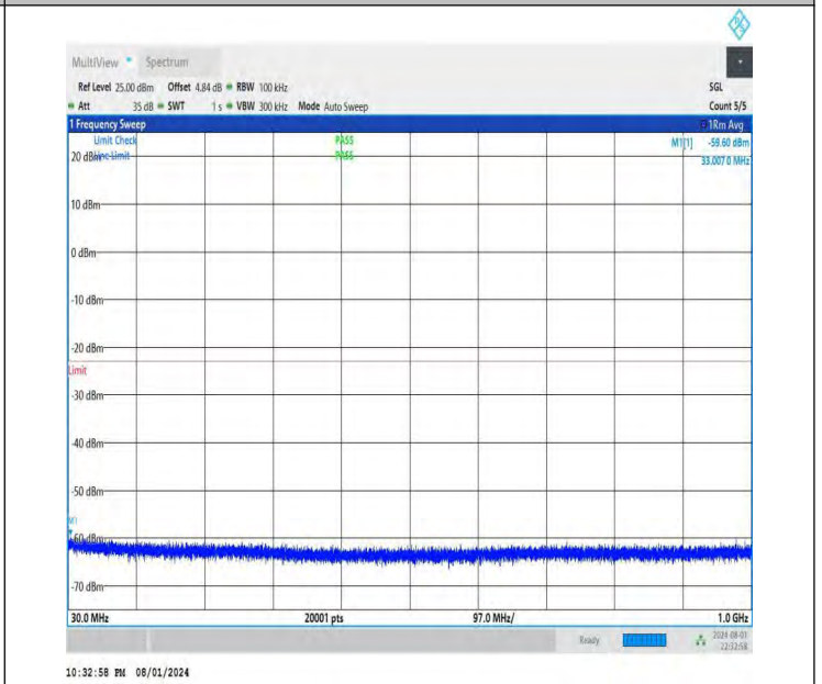
NTNV-DC_26A-n78A(3700-3800)-PC3-30-5+20-M+M-QPSK-IDLE -DFT-QPSK-Edge_1RB_Right-30-1000-PASS
