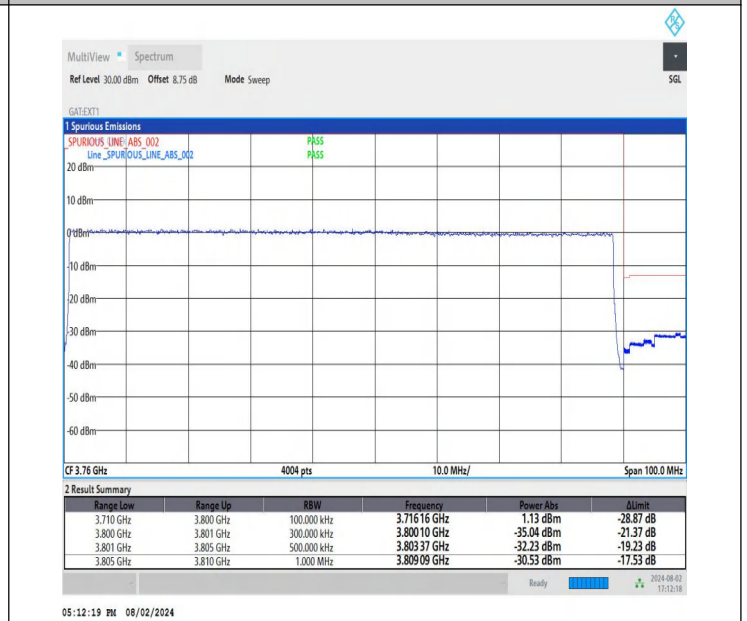
NTNV-DC_26A-n78A(3700-3800)-PC3-30-5+90-M+H-QPSK-IDLE E-DFT-QPSK-Outer_Full-PASS
