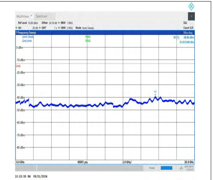
NTNV-DC_26A-n78A(3700-3800)-PC3-30-5+20-M+L-QPSK-IDLE -DFT-BPSK-Edge_1RB_Left-6000-26000-PASS
