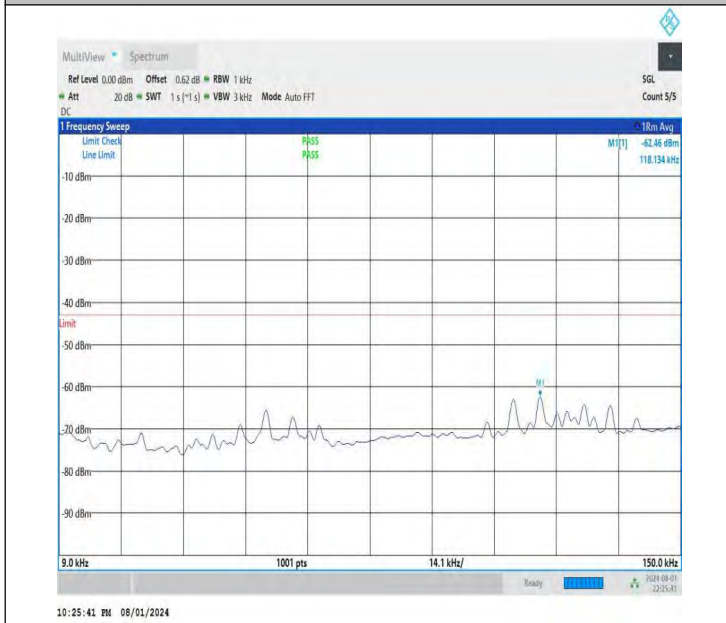
NTNV-DC_26A-n78A(3700-3800)-PC3-30-5+20-M+L-QPSK-IDL E-DFT-QPSK-Edge_1RB_Left-0.009-0.15-PASS
