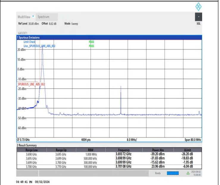
NTNV-DC_26A-n78A(3700-3800)-PC3-30-5+70-M+L-QPSK-IDLE -DFT-BPSK-Edge_1RB_Left-PASS
