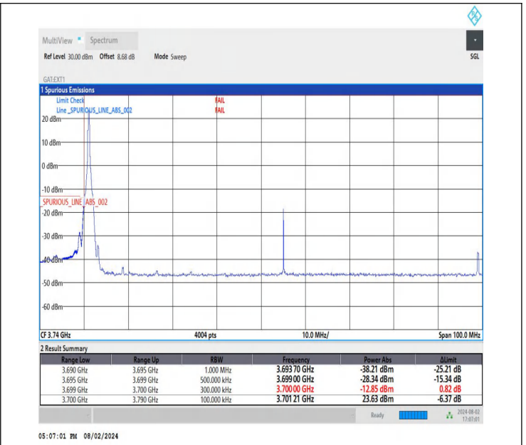
NTNV-DC_26A-n78A(3700-3800)-PC3-30-5+90-M+L-QPSK-IDLE -DFT-QPSK-Edge_1RB_Left-FAIL
