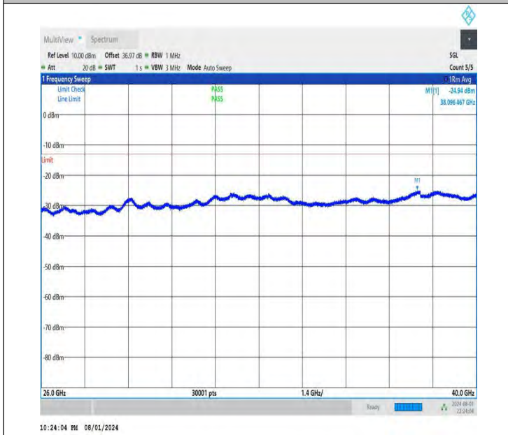
NTNV-DC_26A-n78A(3700-3800)-PC3-30-5+20-M+L-QPSK-IDL E-DFT-BPSK-Edge_1RB_Left-26000-40000-PASS
