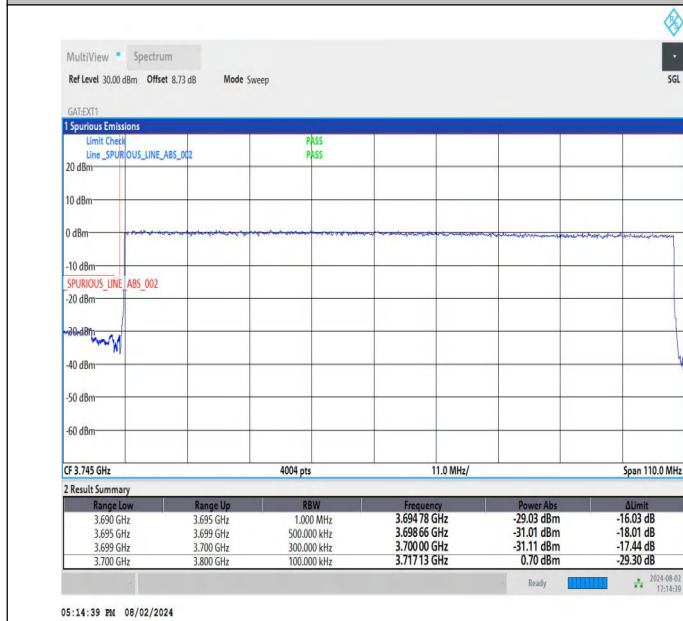
NTNV-DC_26A-n78A(3700-3800)-PC3-30-5+100-M+L-QPSK-IDL E-DFT-BPSK-Outer_Full-PASS
