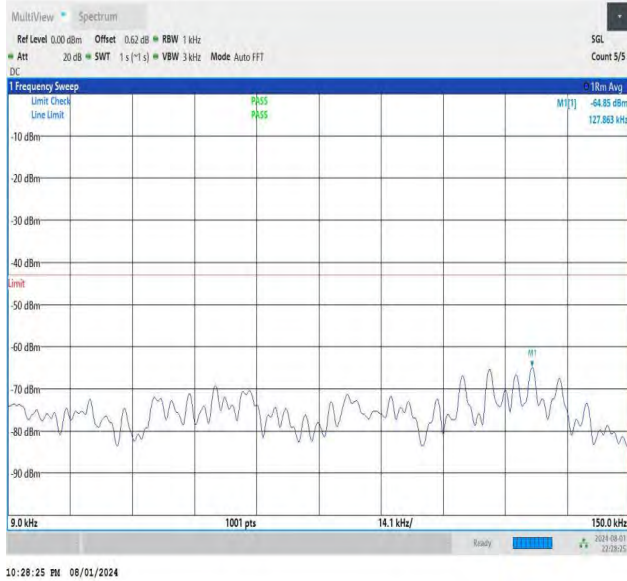
NTNV-DC_26A-n78A(3700-3800)-PC3-30-5+20-M+M-QPSK-IDL E-DFT-BPSK-Edge_1RB_Left-0.009-0.15-PASS
