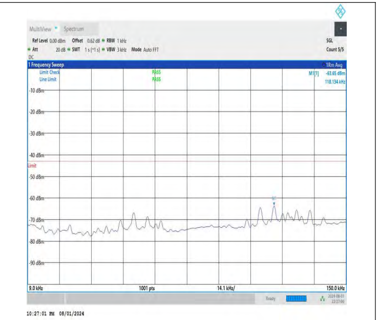
NTNV-DC_26A-n78A(3700-3800)-PC3-30-5+20-M+L-QPSK-IDLE -DFT-QPSK-Edge_1RB_Right-0.009-0.15-PASS
