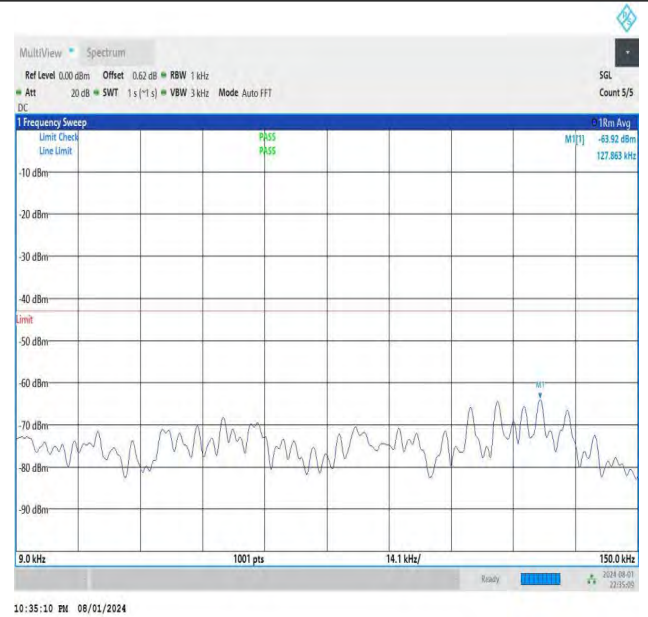
NTNV-DC_26A-n78A(3700-3800)-PC3-30-5+20-M+H-QPSK-IDLE -DFT-BPSK-Edge_1RB_Right-0.009-0.15-PASS
