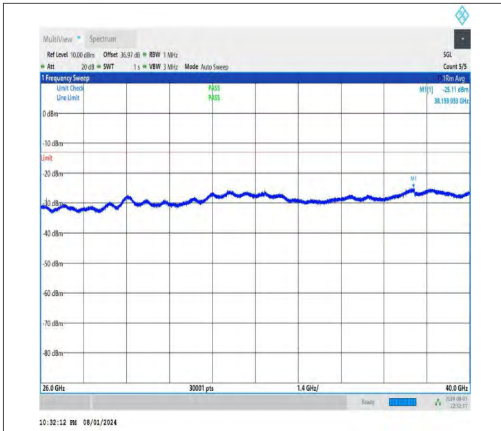
NTNV-DC_26A-n78A(3700-3800)-PC3-30-5+20-M+M-QPSK-IDL E-DFT-QPSK-Edge_1RB_Left-26000-40000-PASS
