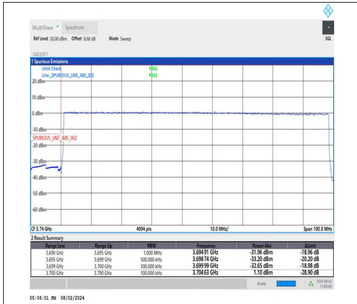
NTNV-DC_26A-n78A(3700-3800)-PC3-30-5+90-M+L-QPSK-IDLE -DFT-BPSK-Outer_Full-PASS
