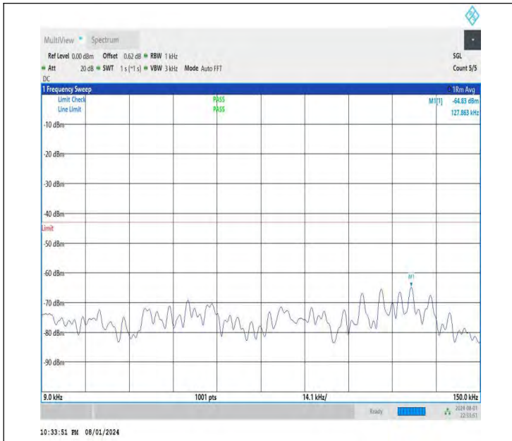
NTNV-DC_26A-n78A(3700-3800)-PC3-30-5+20-M+H-QPSK-IDL E-DFT-BPSK-Edge_1RB_Left-0.009-0.15-PASS
