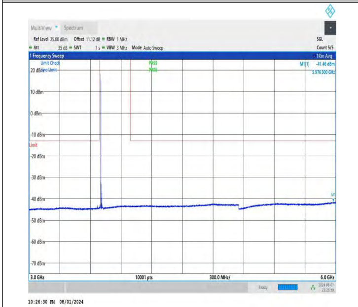
NTNV-DC_26A-n78A(3700-3800)-PC3-30-5+20-M+L-QPSK-IDL E-DFT-QPSK-Edge_1RB_Left-3000-6000-PASS
