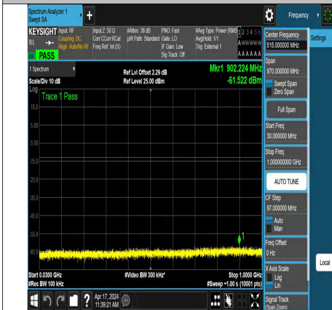
NTNV_N78-3700-3800_PC2_30_100_H_TID2_NS_01_30_1000
