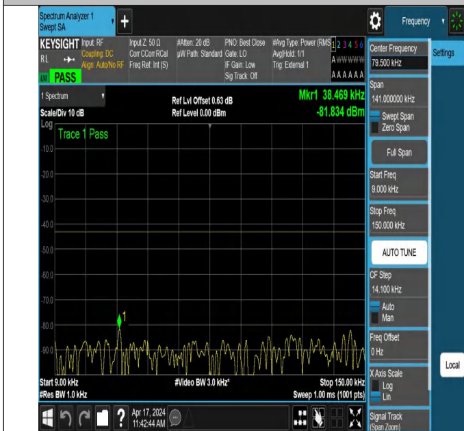
NTNV_N78-3700-3800_PC2_30_100_H_TID3_NS_01_0.009_0.
