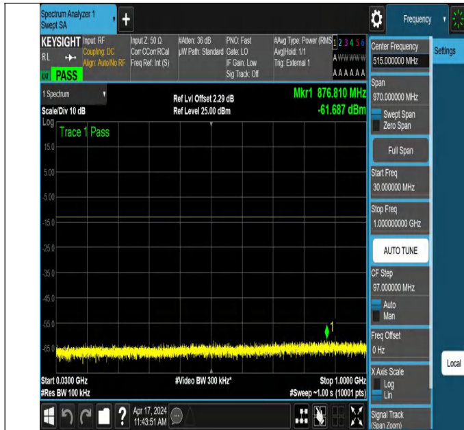
NTNV_N78-3700-3800_PC2_30_100_H_TID3_NS_01_30_1000
