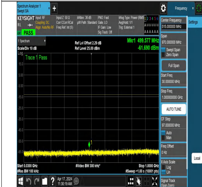
NTNV_N78-3700-3800_PC2_30_100_M_TID5_NS_01_30_1000
