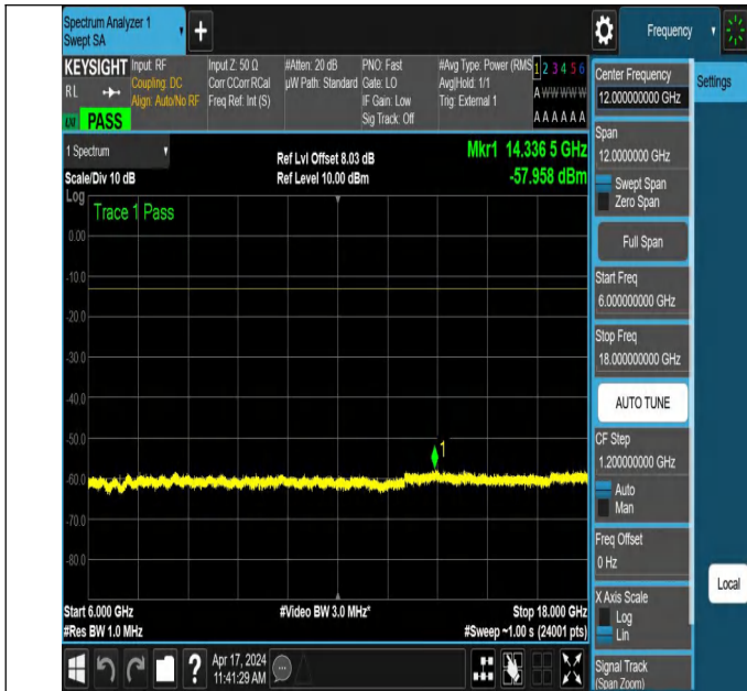
NTNV_N78-3700-3800_PC2_30_100_H_TID2_NS_01_6000_18
