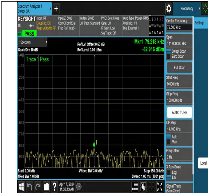
NTNV_N78-3700-3800_PC2_30_100_H_TID2_NS_01_0.009_0.
