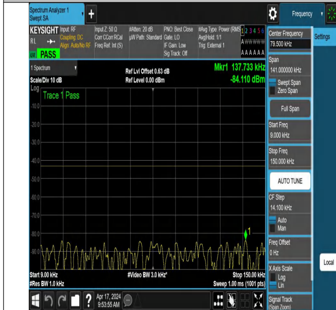
NTNV_N78-3700-3800_PC2_30_80_H_TID3_NS_01_0.009_0.15_#1
