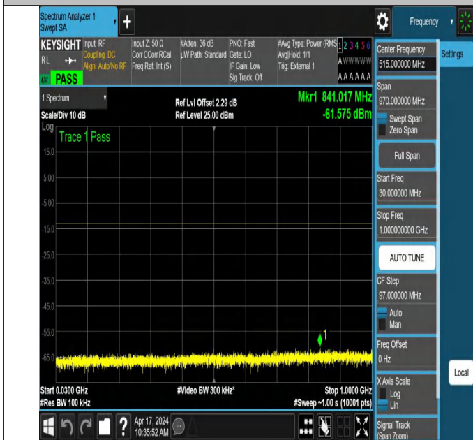
NTNV_N78-3700-3800_PC2_30_90_M_TID5_NS_01_30_1000_
