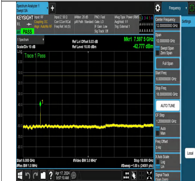
NTNV_N78-3700-3800_PC2_30_80_H_TID3_NS_01_6000_18000_#1
