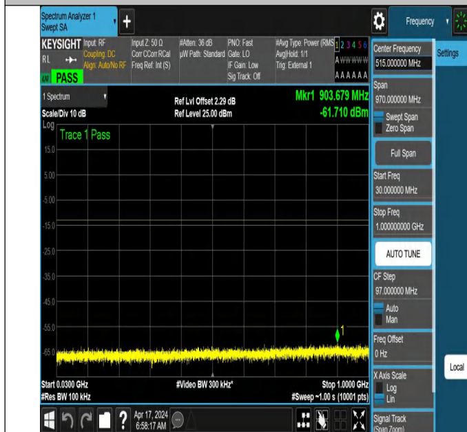
NTNV_N78-3700-3800_PC2_30_50_M_TID5_NS_01_30_1000_
