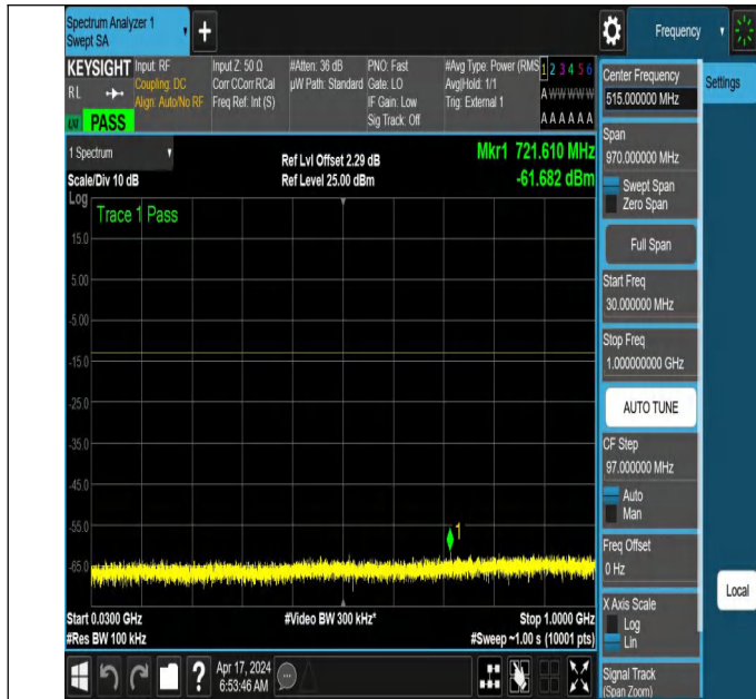
NTNV_N78-3700-3800_PC2_30_50_M_TID3_NS_01_30_1000_
