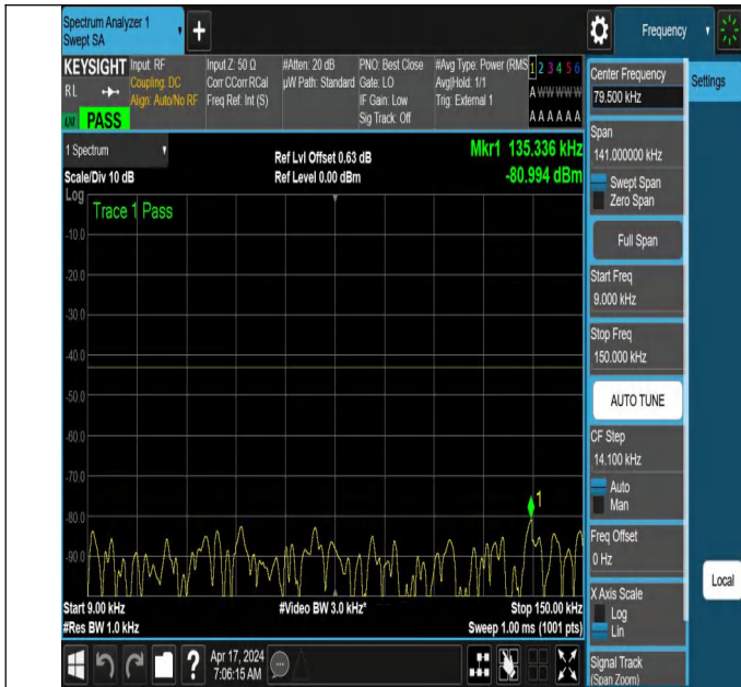
NTNV_N78-3700-3800_PC2_30_50_H_TID2_NS_01_0.009_0.1 5_#1
