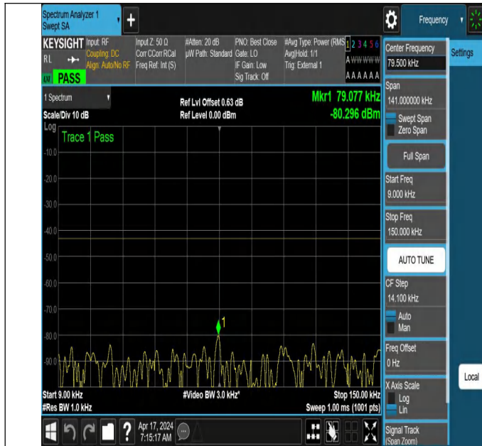
NTNV_N78-3700-3800_PC2_30_50_H_TID5_NS_01_0.009_0.1 5_#1
