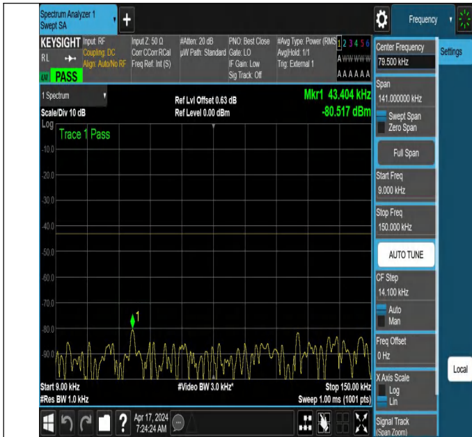
NTNV_N78-3700-3800_PC2_30_60_L_TID2_NS_01_0.009_0.1 5_#1
