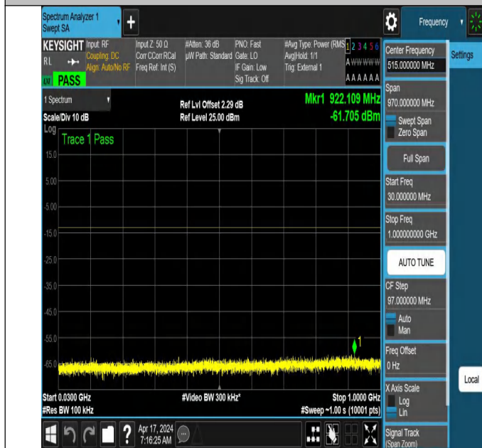
NTNV_N78-3700-3800_PC2_30_50_H_TID5_NS_01_30_1000_ #1
