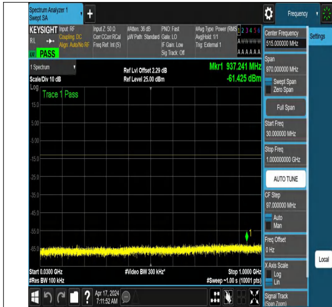
NTNV_N78-3700-3800_PC2_30_50_H_TID3_NS_01_30_1000_#1
