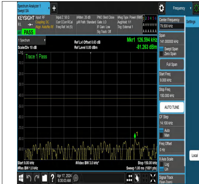
NTNV_N78-3700-3800_PC2_30_50_L_TID2_NS_01_0.009_0.1 5_#1
