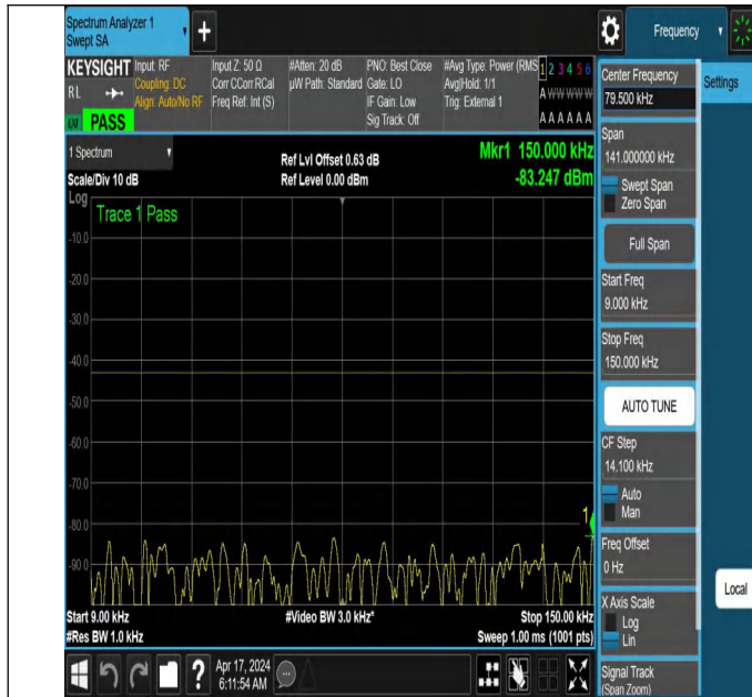
NTNV_N78-3700-3800_PC2_30_40_H_TID2_NS_01_0.009_0.1 5_#1
