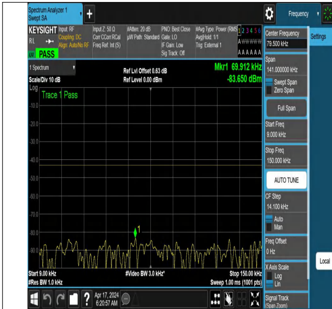
NTNV_N78-3700-3800_PC2_30_40_H_TID5_NS_01_0.009_0.1 5_#1
