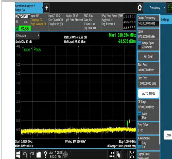
NTNV_N78-3700-3800_PC2_30_40_H_TID2_NS_01_30_1000_ #1
