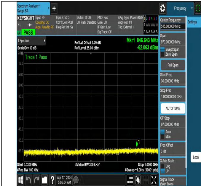
NTNV_N78-3700-3800_PC2_30_30_M_TID3_NS_01_30_1000_#1
