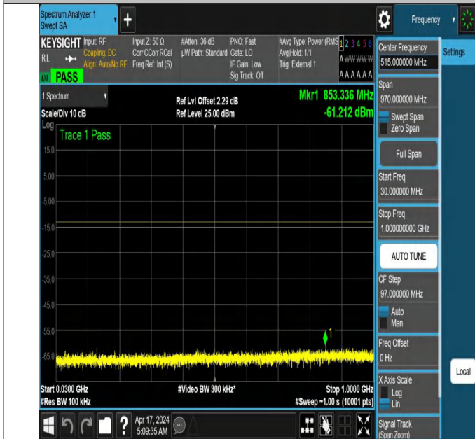
NTNV_N78-3700-3800_PC2_30_30_M_TID5_NS_01_30_1000_
