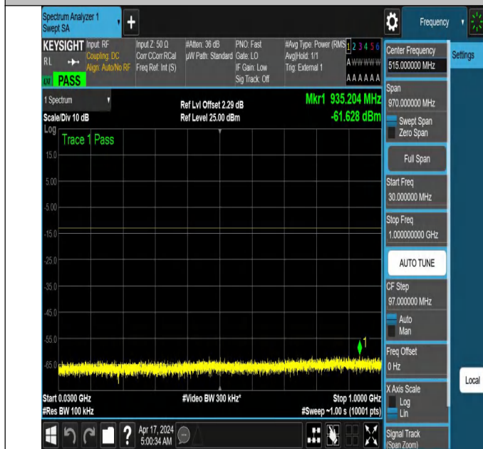
NTNV_N78-3700-3800_PC2_30_30_M_TID2_NS_01_30_1000_
