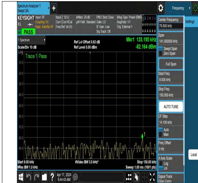
NTNV_N78-3700-3800_PC2_30_40_L_TID5_NS_01_0.009_0.1 5_#1
