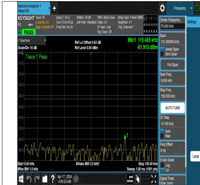
NTNV_N78-3700-3800_PC2_30_30_L_TID5_NS_01_0.009_0.1 5_#1
