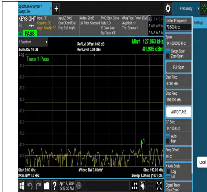
NTNV_N78-3700-3800_PC2_30_30_H_TID2_NS_01_0.009_0.1 5_#1
