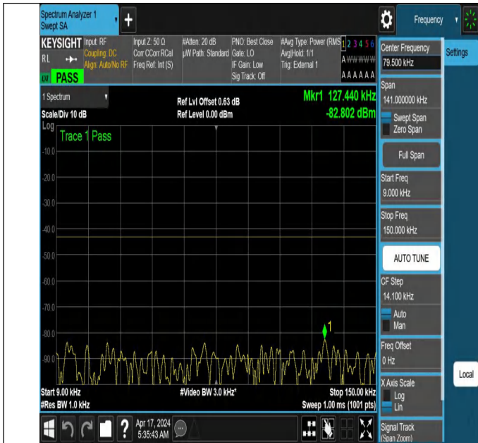
NTNV_N78-3700-3800_PC2_30_40_L_TID2_NS_01_0.009_0.1 5_#1
