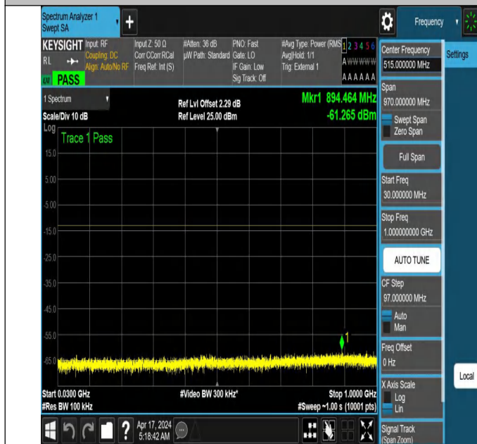
NTNV_N78-3700-3800_PC2_30_30_H_TID2_NS_01_30_1000_ #1
