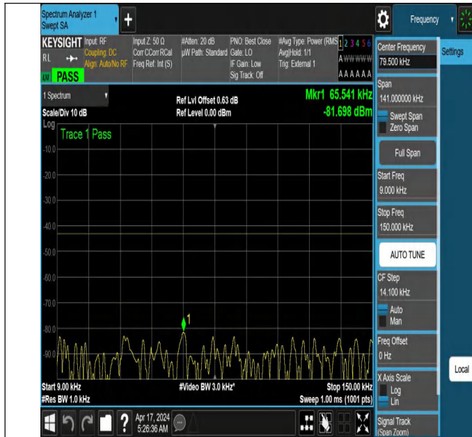
NTNV_N78-3700-3800_PC2_30_30_H_TID5_NS_01_0.009_0.1 5_#1
