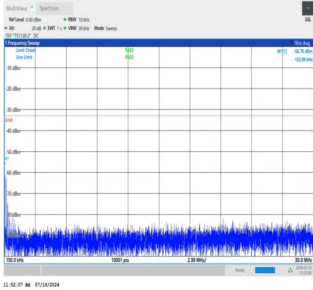
NTNV_N78-3450-3550_PC2_30_90_M_TID3_NS_01_0.15_30_#1
