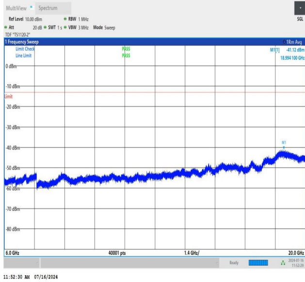
NTNV_N78-3450-3550_PC2_30_90_M_TID3_NS_01_6000_2000_0_#1
