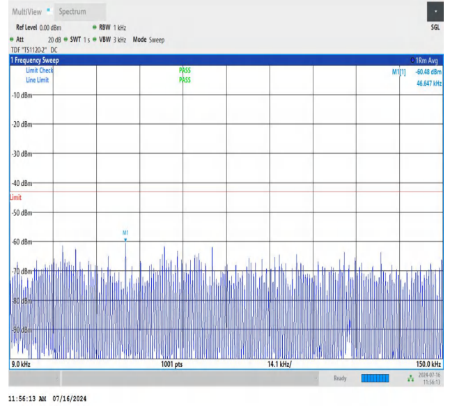
NTNV_N78-3450-3550_PC2_30_100_M_TID3_NS_01_0.009_0.15_#1
