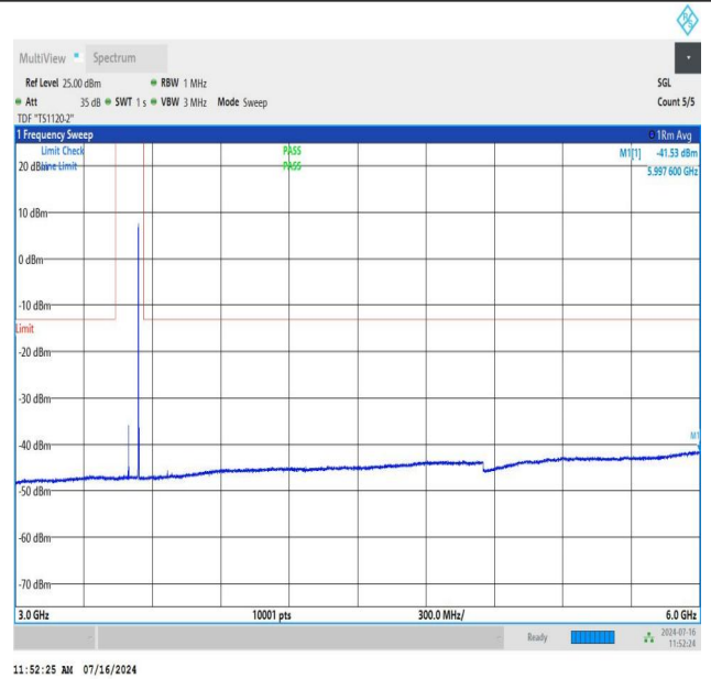
NTNV_N78-3450-3550_PC2_30_90_M_TID3_NS_01_3000_6000_#1
