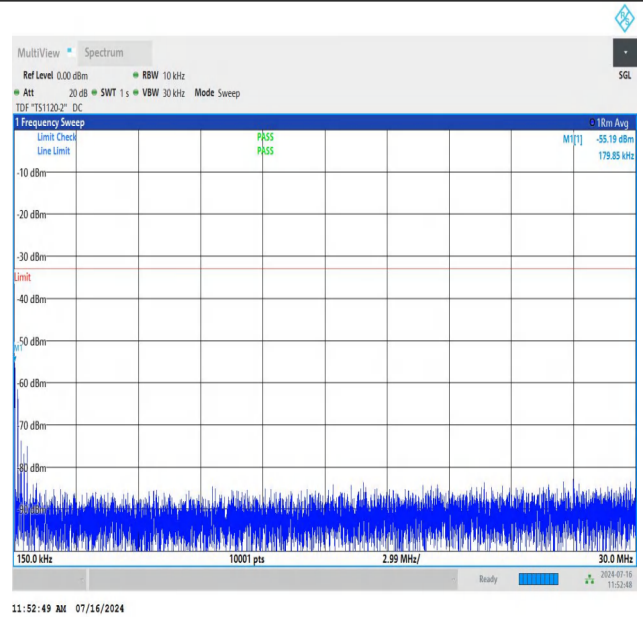
NTNV_N78-3450-3550_PC2_30_90_H_TID2_NS_01_0.15_30_#1
