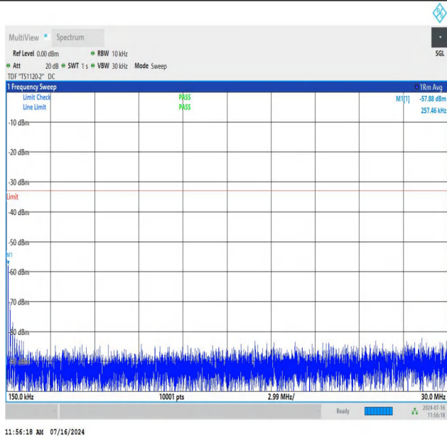
NTNV_N78-3450-3550_PC2_30_100_M_TID3_NS_01_0.15_30_#1
