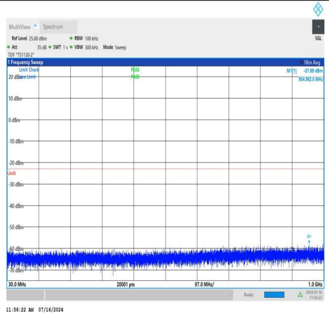
NTNV_N78-3450-3550_PC2_30_100_M_TID3_NS_01_30_1000_#1
