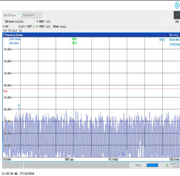
NTNV_N78-3450-3550_PC2_30_90_H_TID2_NS_01_0.009_0.15_#1
