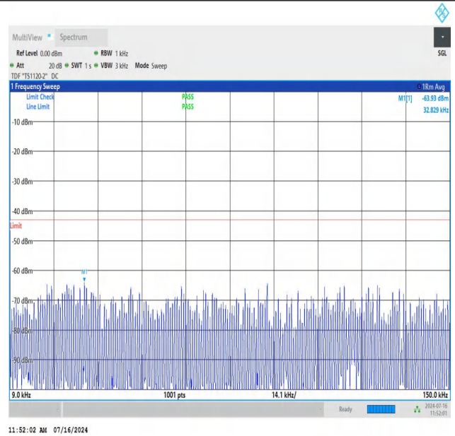
NTNV_N78-3450-3550_PC2_30_90_M_TID3_NS_01_0.009_0.15
