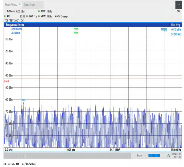
NTNV_N78-3450-3550_PC2_30_90_H_TID3_NS_01_0.009_0.15_#1
