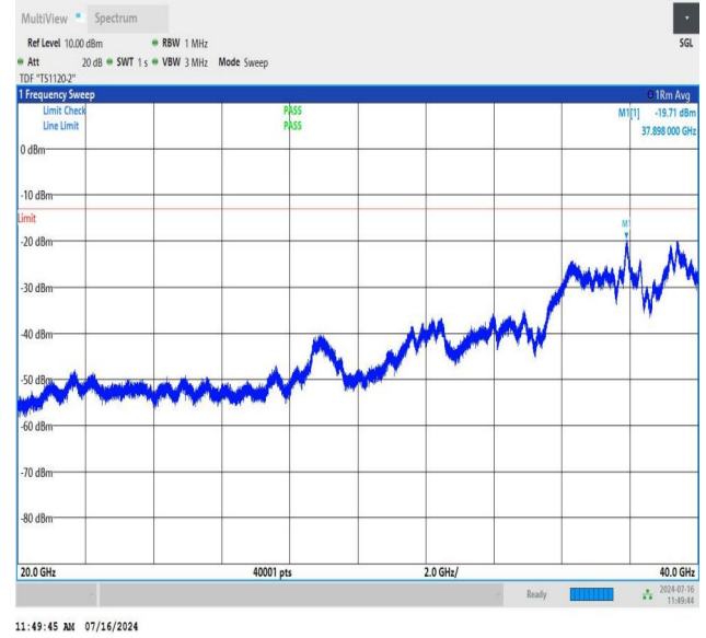
NTNV_N78-3450-3550_PC2_30_80_H_TID3_NS_01_20000_400_00_#1
