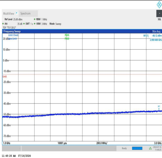
NTNV_N78-3450-3550_PC2_30_80_H_TID3_NS_01_1000_3000_#1
