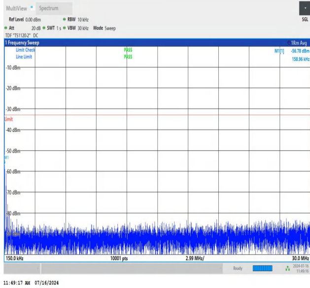
NTNV_N78-3450-3550_PC2_30_80_H_TID3_NS_01_0.15_30_#1
