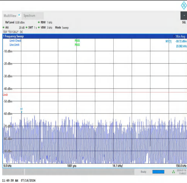
NTNV_N78-3450-3550_PC2_30_90_L_TID2_NS_01_0.009_0.15_#1
