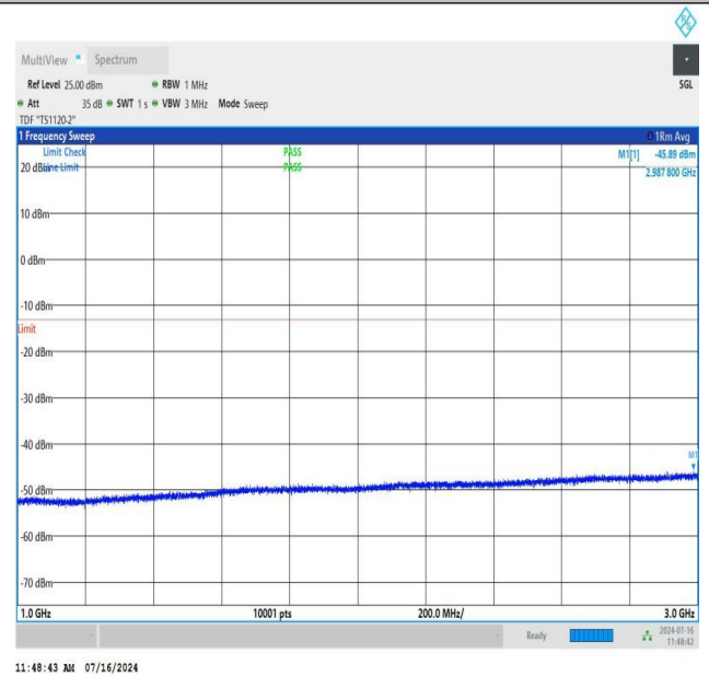
NTNV_N78-3450-3550_PC2_30_80_H_TID2_NS_01_1000_3000_#1
