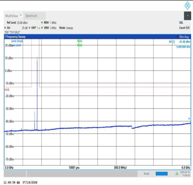
NTNV_N78-3450-3550_PC2_30_80_H_TID3_NS_01_3000_6000_#1
