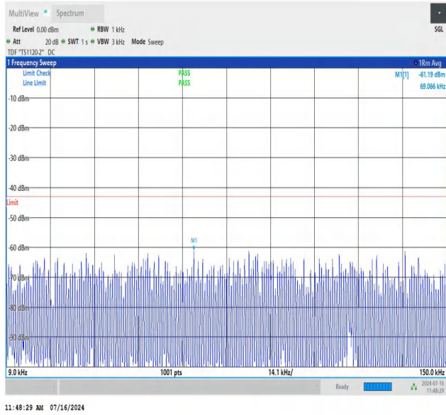
NTNV_N78-3450-3550_PC2_30_80_H_TID2_NS_01_0.009_0.15_#1
