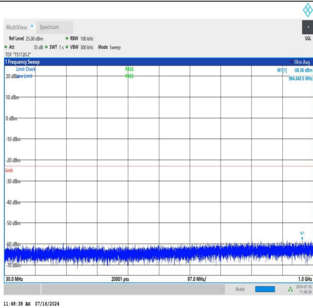
NTNV_N78-3450-3550_PC2_30_80_H_TID2_NS_01_30_1000_#1
