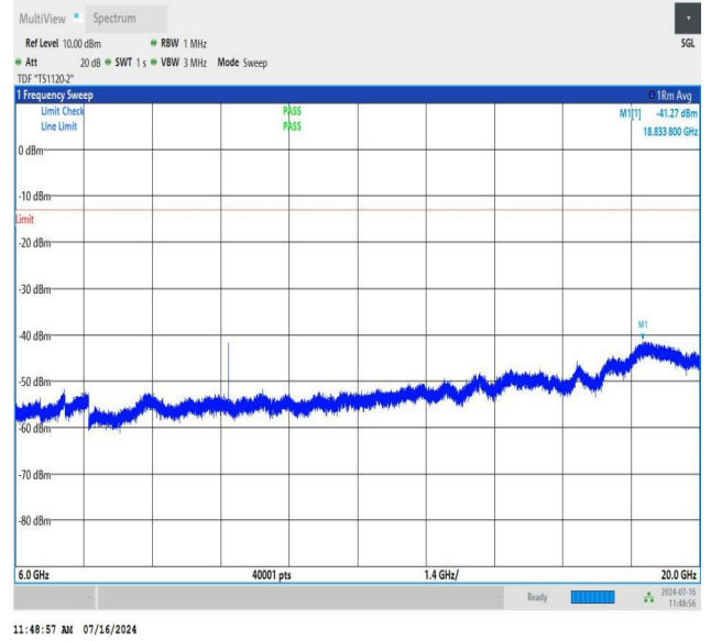
NTNV_N78-3450-3550_PC2_30_80_H_TID2_NS_01_6000_2000
