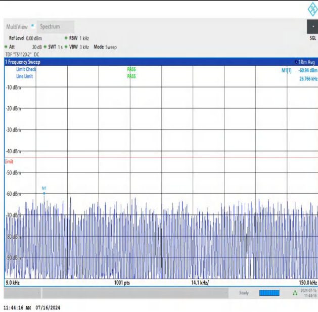
NTNV_N78-3450-3550_PC2_30_70_H_TID2_NS_01_0.009_0.15_#1
