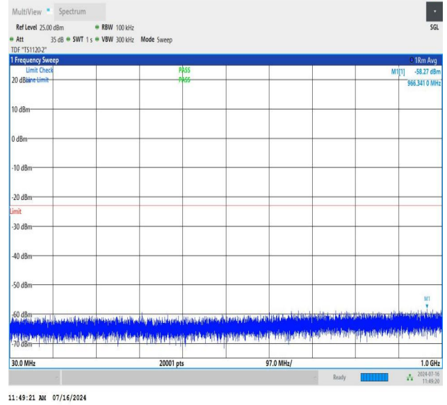
NTNV_N78-3450-3550_PC2_30_80_H_TID3_NS_01_30_1000_#
