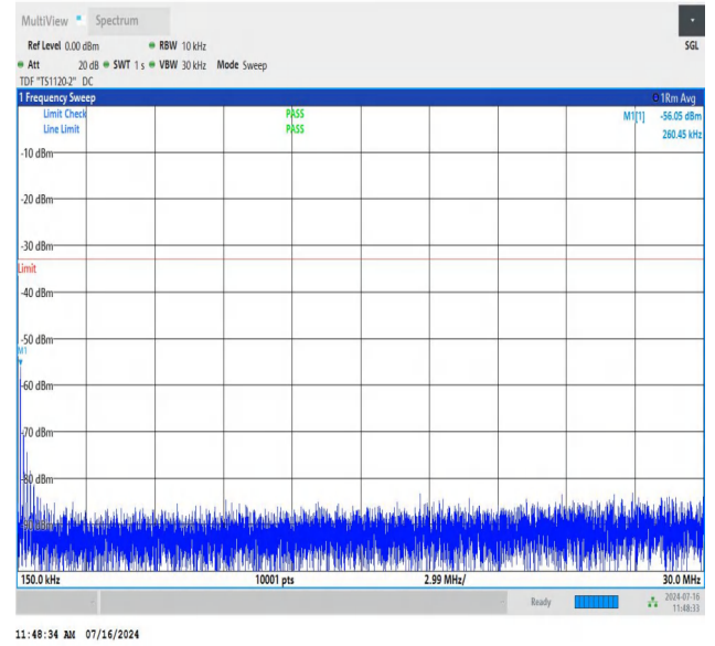
NTNV_N78-3450-3550_PC2_30_80_H_TID2_NS_01_0.15_30_#1
