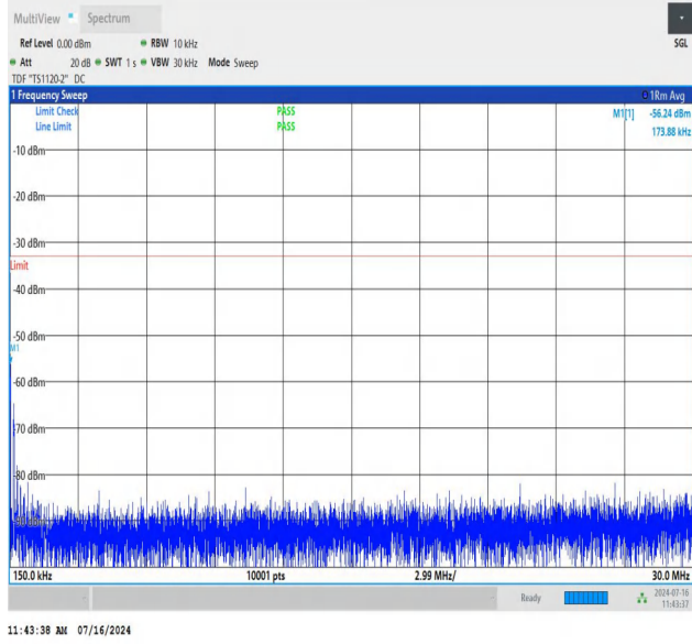
NTNV_N78-3450-3550_PC2_30_70_M_TID3_NS_01_0.15_30_#1
