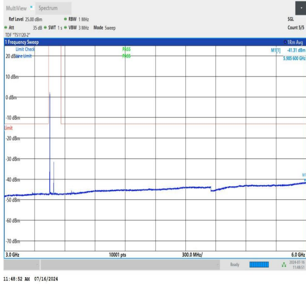
NTNV_N78-3450-3550_PC2_30_80_H_TID2_NS_01_3000_6000
