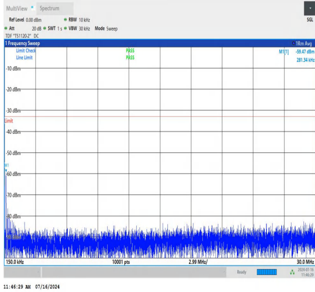
NTNV_N78-3450-3550_PC2_30_80_L_TID3_NS_01_0.15_30_#1
