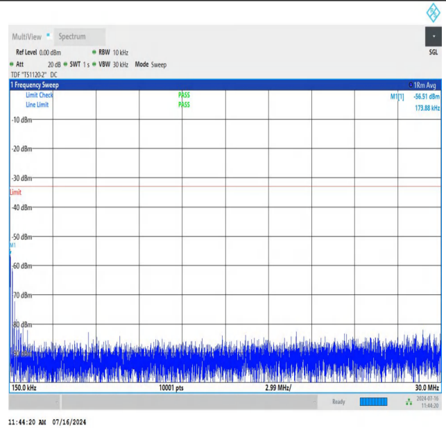
NTNV_N78-3450-3550_PC2_30_70_H_TID2_NS_01_0.15_30_#1
