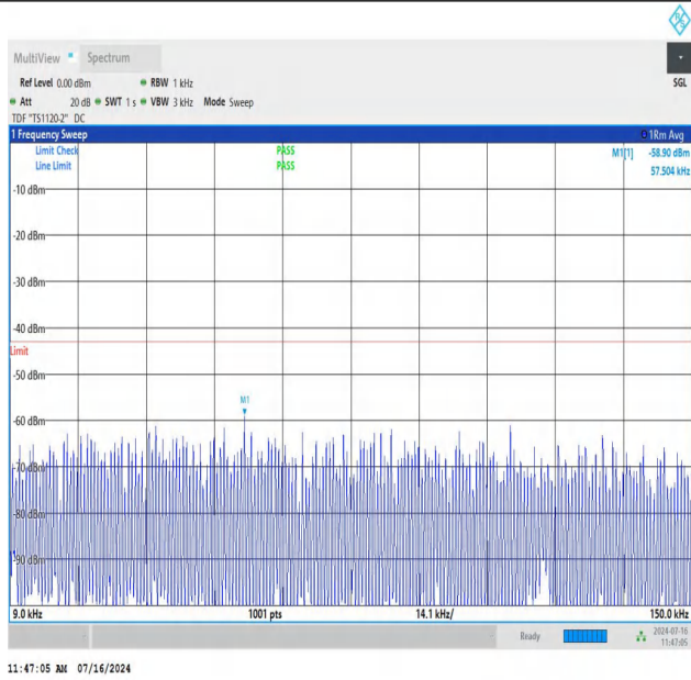
NTNV_N78-3450-3550_PC2_30_80_M_TID2_NS_01_0.009_0.15
