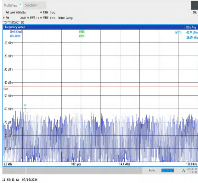
NTNV_N78-3450-3550_PC2_30_80_L_TID2_NS_01_0.009_0.15_#1
