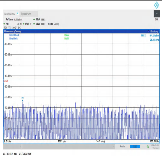
NTNV_N78-3450-3550_PC2_30_60_L_TID3_NS_01_0.009_0.15_#1
