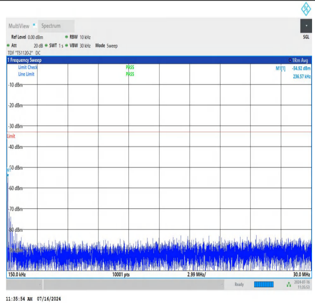
NTNV_N78-3450-3550_PC2_30_50_H_TID2_NS_01_0.15_30_#1
