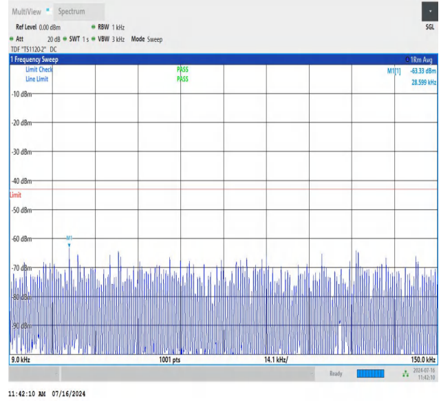
NTNV_N78-3450-3550_PC2_30_70_L_TID3_NS_01_0.009_0.15_#1
