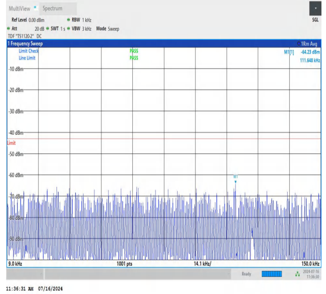
NTNV_N78-3450-3550_PC2_30_50_H_TID3_NS_01_0.009_0.15_#1
