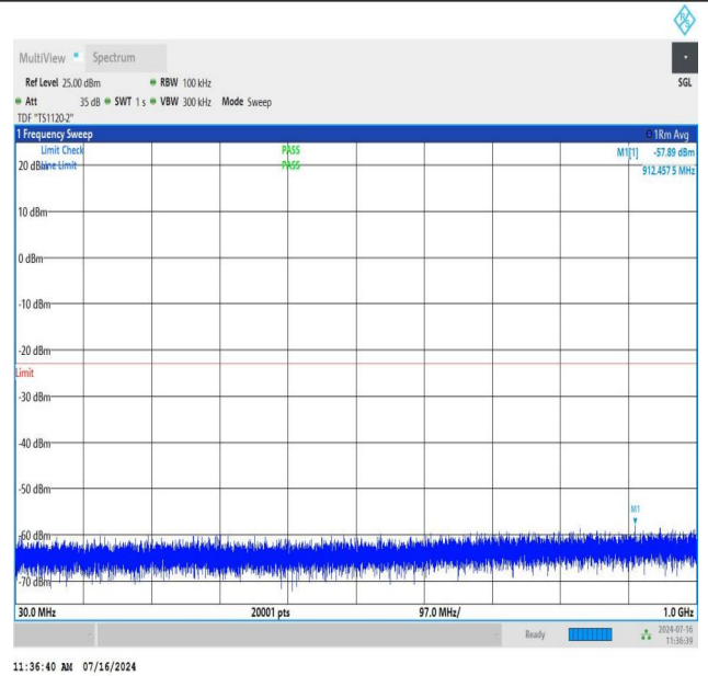
NTNV_N78-3450-3550_PC2_30_50_H_TID3_NS_01_30_1000_#1
