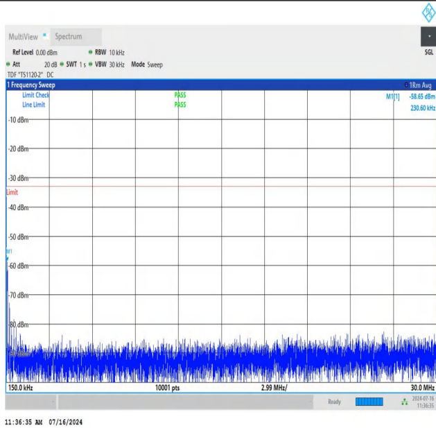
NTNV_N78-3450-3550_PC2_30_50_H_TID3_NS_01_0.15_30_#1
