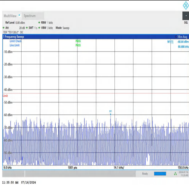
NTNV_N78-3450-3550_PC2_30_50_H_TID2_NS_01_0.009_0.15_#1
