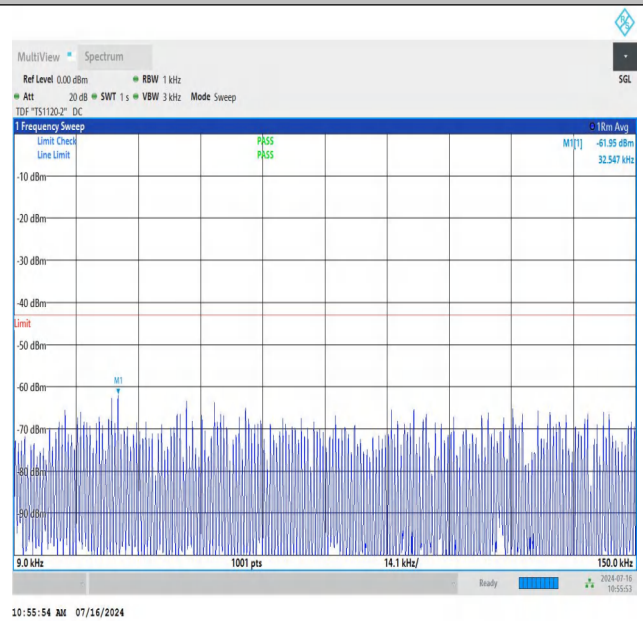
NTNV_N78-3450-3550_PC2_30_80_M_TID3_NS_01_0.009_0.15
