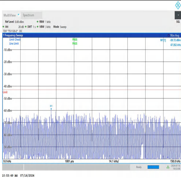
NTNV_N78-3450-3550_PC2_30_80_L_TID2_NS_01_0.009_0.15_#1
