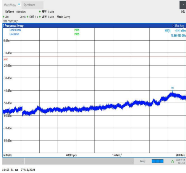
NTNV_N78-3450-3550_PC2_30_60_H_TID3_NS_01_6000_2000_0_#1
