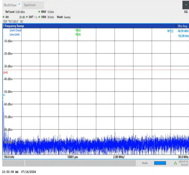
NTNV_N78-3450-3550_PC2_30_60_H_TID3_NS_01_0.15_30_#1
