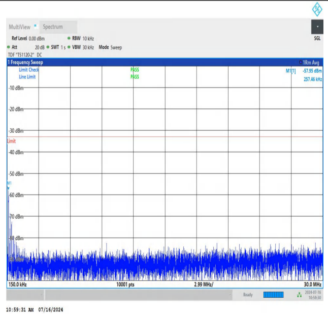
NTNV_N78-3450-3550_PC2_30_90_M_TID2_NS_01_0.15_30_#1
