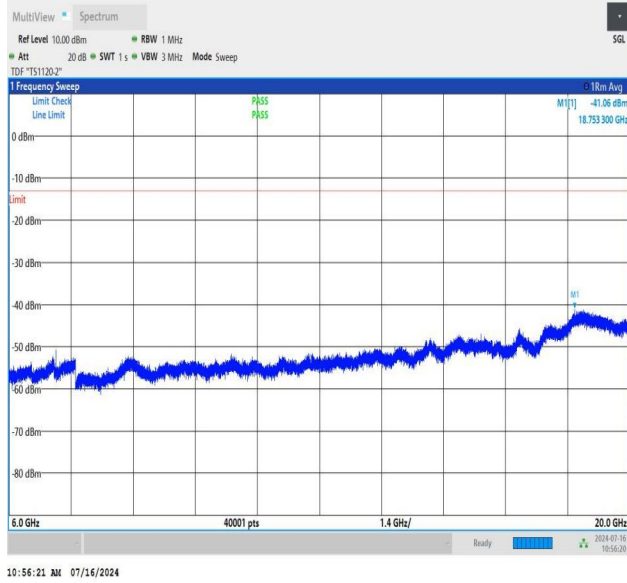
NTNV_N78-3450-3550_PC2_30_80_M_TID3_NS_01_6000_2000_0_#1
