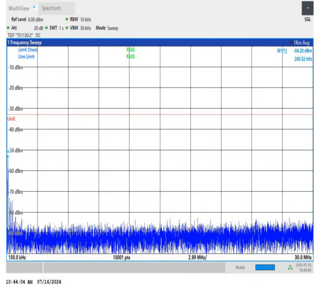
NTNV_N78-3450-3550_PC2_30_40_H_TID2_NS_01_0.15_30_#1
