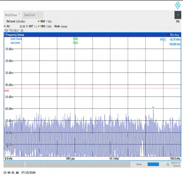
NTNV_N78-3450-3550_PC2_30_40_H_TID3_NS_01_0.009_0.15_#1
