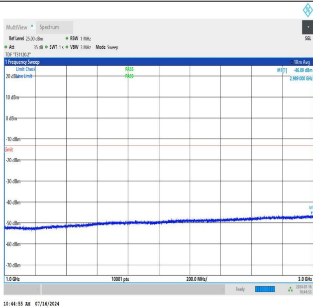
NTNV_N78-3450-3550_PC2_30_40_H_TID3_NS_01_1000_3000_#1
