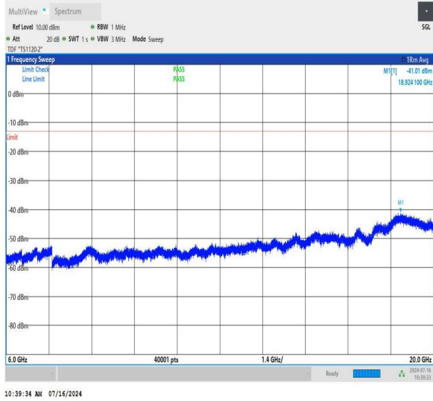
NTNV_N78-3450-3550_PC2_30_30_M_TID3_NS_01_6000_2000_0_#1
