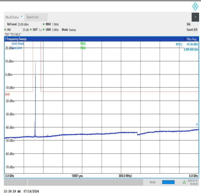
NTNV_N78-3450-3550_PC2_30_30_M_TID3_NS_01_3000_6000_#1
