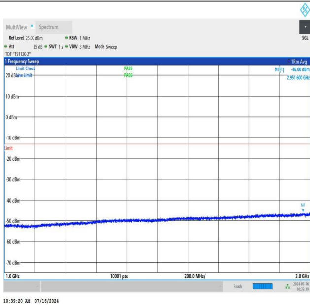
NTNV_N78-3450-3550_PC2_30_30_M_TID3_NS_01_1000_3000_#1
