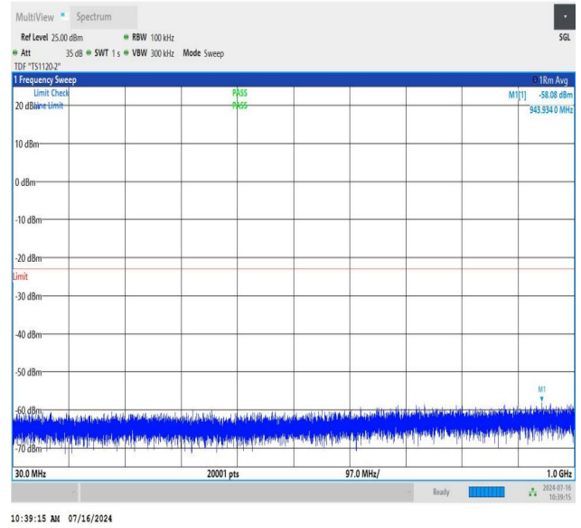
NTNV_N78-3450-3550_PC2_30_30_M_TID3_NS_01_30_1000_#
