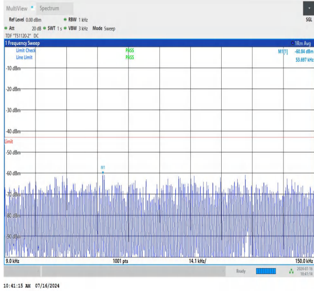
NTNV_N78-3450-3550_PC2_30_40_L_TID2_NS_01_0.009_0.15_#1
