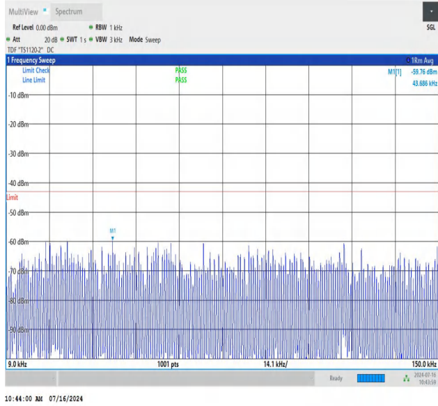
NTNV_N78-3450-3550_PC2_30_40_H_TID2_NS_01_0.009_0.15_#1
