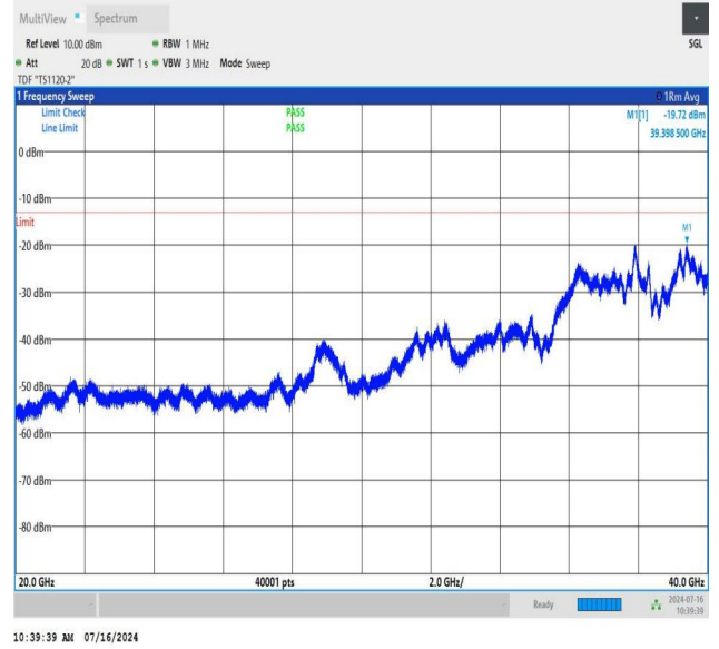
NTNV_N78-3450-3550_PC2_30_30_M_TID3_NS_01_20000_40000_#1
