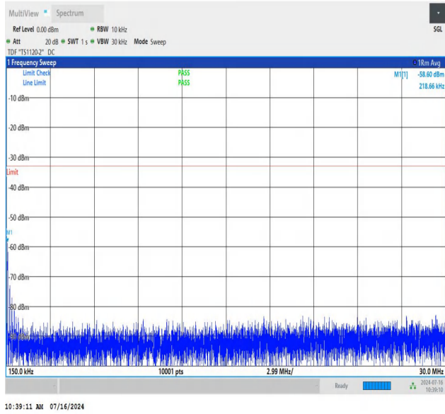
NTNV_N78-3450-3550_PC2_30_30_M_TID3_NS_01_0.15_30_#1
