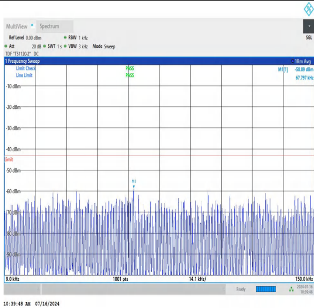
NTNV_N78-3450-3550_PC2_30_30_H_TID2_NS_01_0.009_0.15_#1
