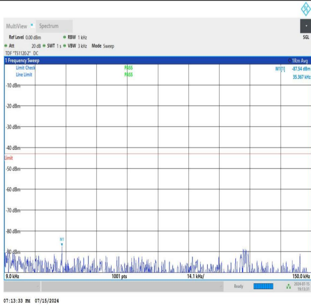
NTNV_N77-3700-3980_PC2_30_100_H_TID2_NS_01_0.009_0.15_5_#1
