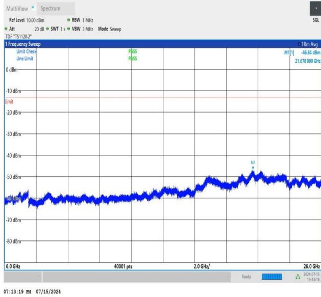
NTNV_N77-3700-3980_PC2_30_100_M_TID3_NS_01_6000_260_00_#1
