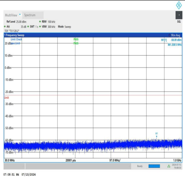
NTNV_N77-3700-3980_PC2_30_90_M_TID3_NS_01_30_1000_#1
