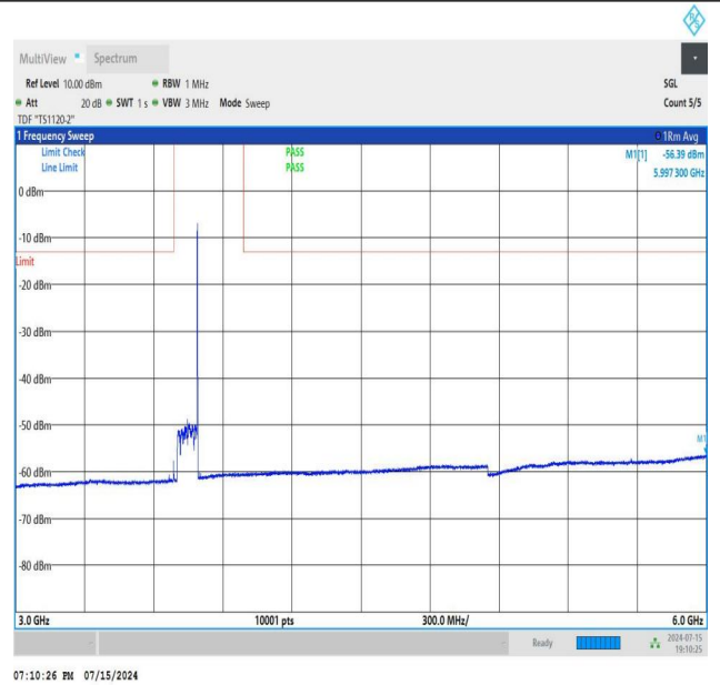
NTNV_N77-3700-3980_PC2_30_90_H_TID3_NS_01_3000_6000_#1
