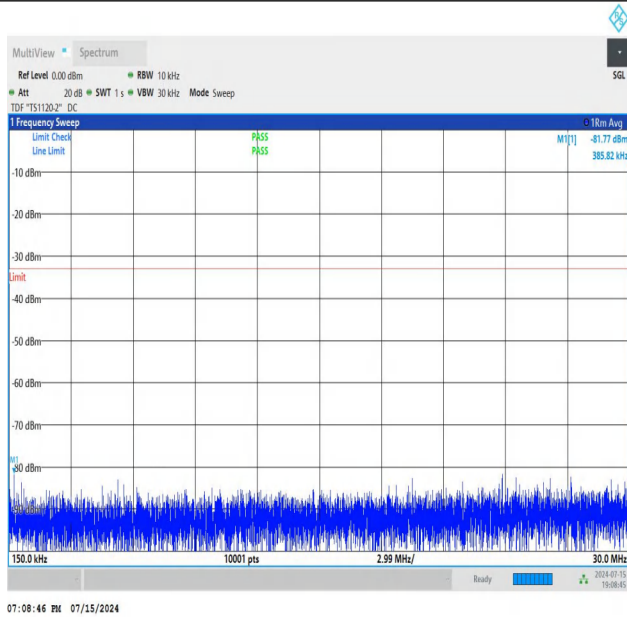
NTNV_N77-3700-3980_PC2_30_90_M_TID3_NS_01_0.15_30_#1
