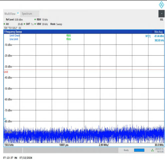
NTNV_N77-3700-3980_PC2_30_100_H_TID2_NS_01_0.15_30_#1
