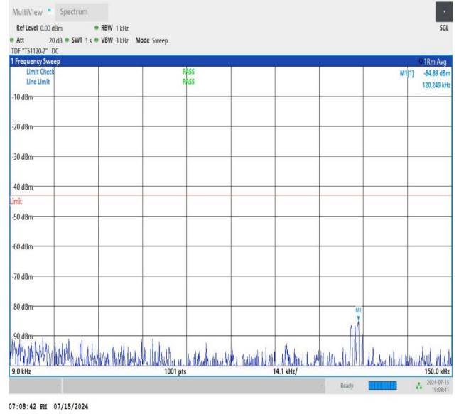
NTNV_N77-3700-3980_PC2_30_90_M_TID3_NS_01_0.009_0.15_#1
