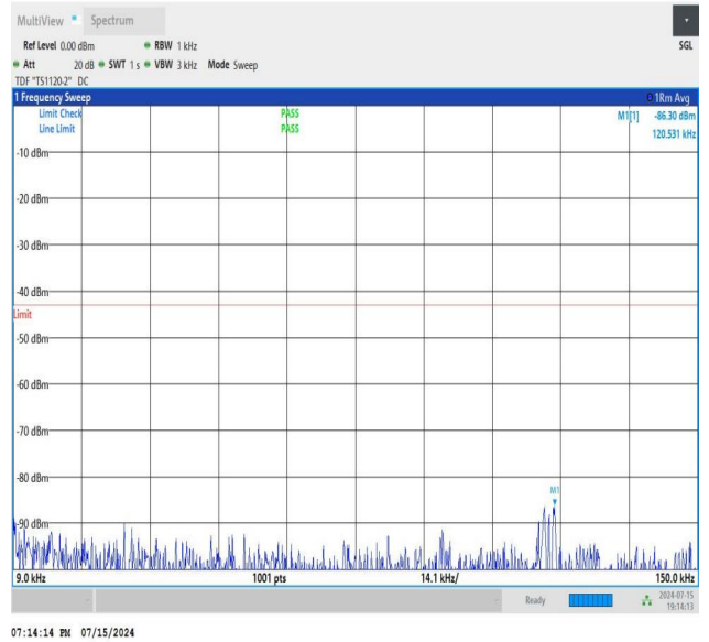
NTNV_N77-3700-3980_PC2_30_100_H_TID3_NS_01_0.009_0.15_#1
