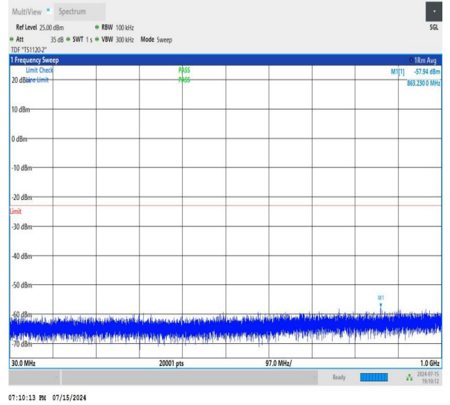
NTNV_N77-3700-3980_PC2_30_90_H_TID3_NS_01_30_1000_#1
