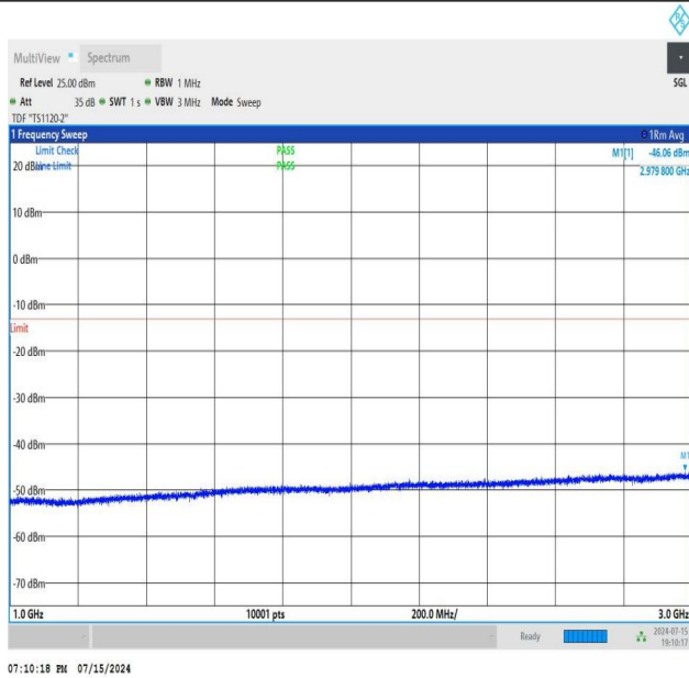
NTNV_N77-3700-3980_PC2_30_90_H_TID3_NS_01_1000_3000_#1
