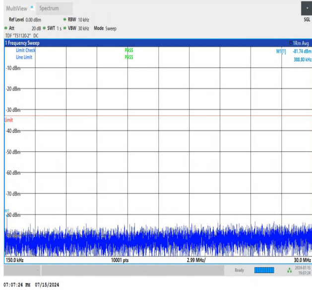
NTNV_N77-3700-3980_PC2_30_90_L_TID3_NS_01_0.15_30_#1
