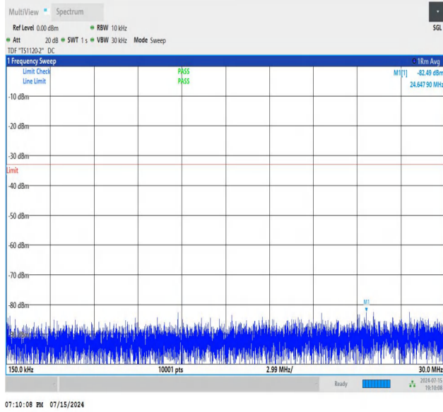
NTNV_N77-3700-3980_PC2_30_90_H_TID3_NS_01_0.15_30_#1
