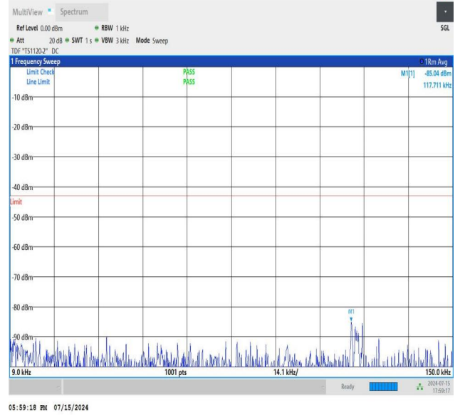
NTNV_N77-3450-3550_PC2_30_80_L_TID3_NS_01_0.009_0.15_#1
