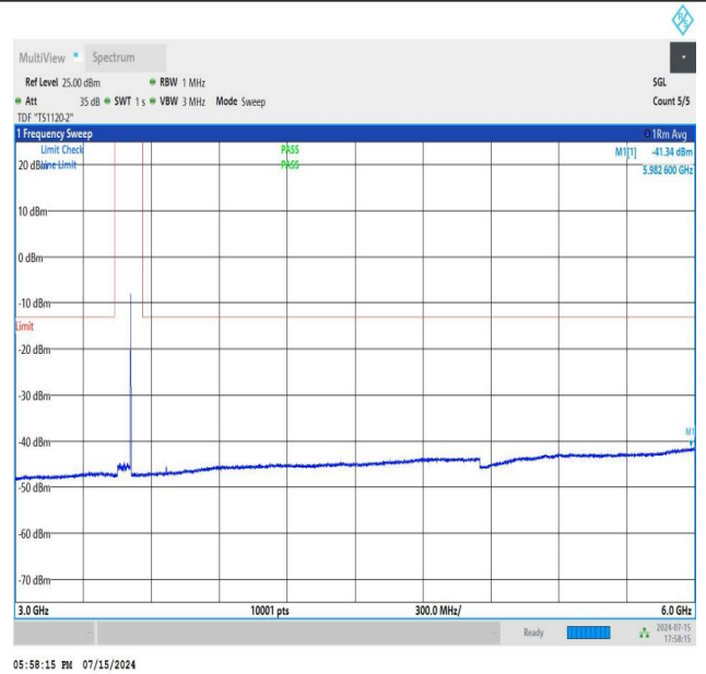
NTNV_N77-3450-3550_PC2_30_60_H_TID3_NS_01_3000_6000_#1
