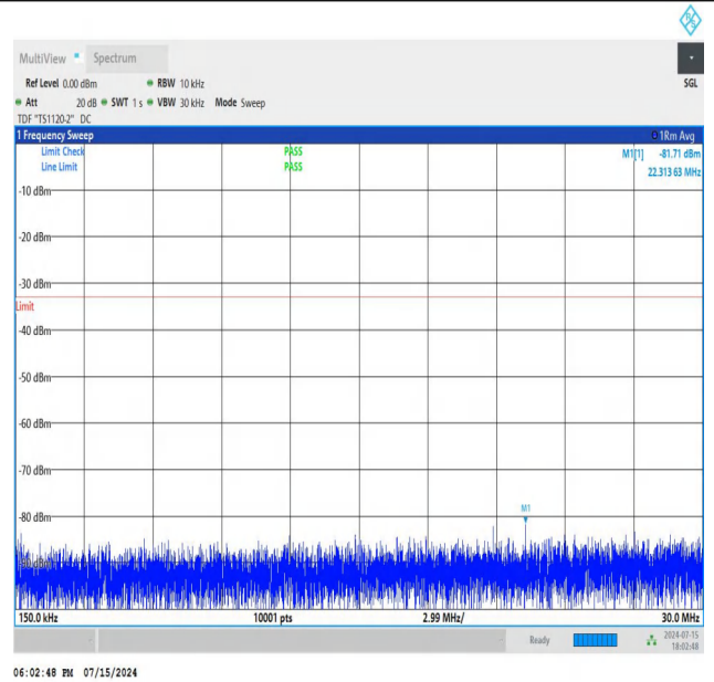
NTNV_N77-3450-3550_PC2_30_90_L_TID2_NS_01_0.15_30_#1
