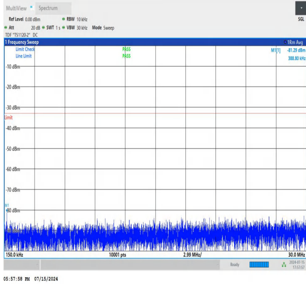
NTNV_N77-3450-3550_PC2_30_60_H_TID3_NS_01_0.15_30_#1
