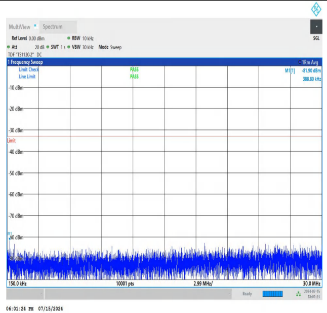
NTNV_N77-3450-3550_PC2_30_80_H_TID2_NS_01_0.15_30_#1
