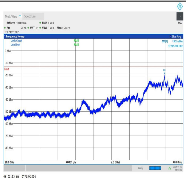
NTNV_N77-3450-3550_PC2_30_80_H_TID3_NS_01_20000_400 00_#1
