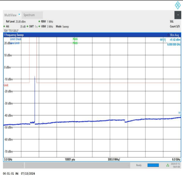
NTNV_N77-3450-3550_PC2_30_80_M_TID3_NS_01_3000_6000_#1
