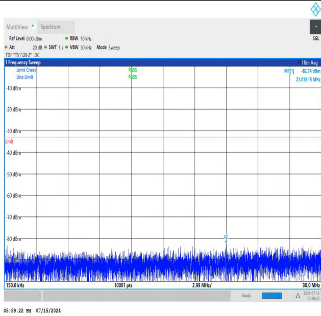
NTNV_N77-3450-3550_PC2_30_80_L_TID3_NS_01_0.15_30_#1
