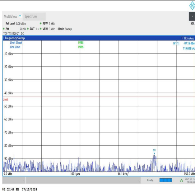
NTNV_N77-3450-3550_PC2_30_90_L_TID2_NS_01_0.009_0.15_#1
