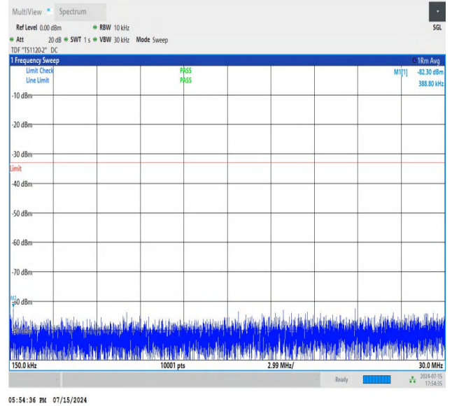
NTNV_N77-3450-3550_PC2_30_60_L_TID2_NS_01_0.15_30_#1
