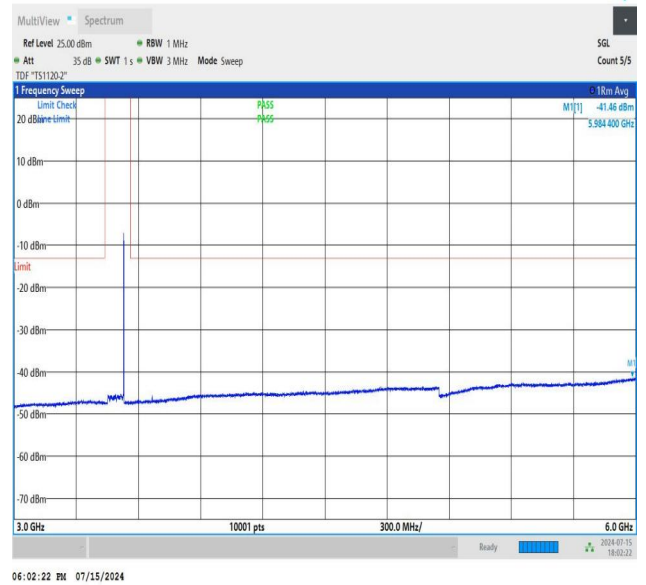
NTNV_N77-3450-3550_PC2_30_80_H_TID3_NS_01_3000_6000 _#1
