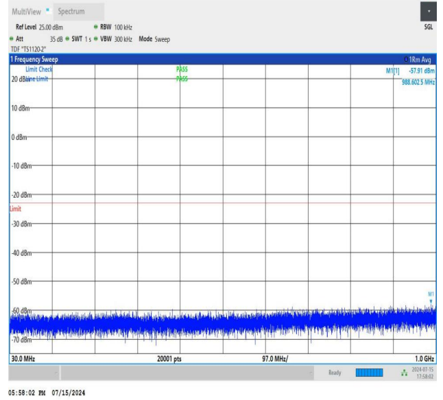
NTNV_N77-3450-3550_PC2_30_60_H_TID3_NS_01_30_1000_#
