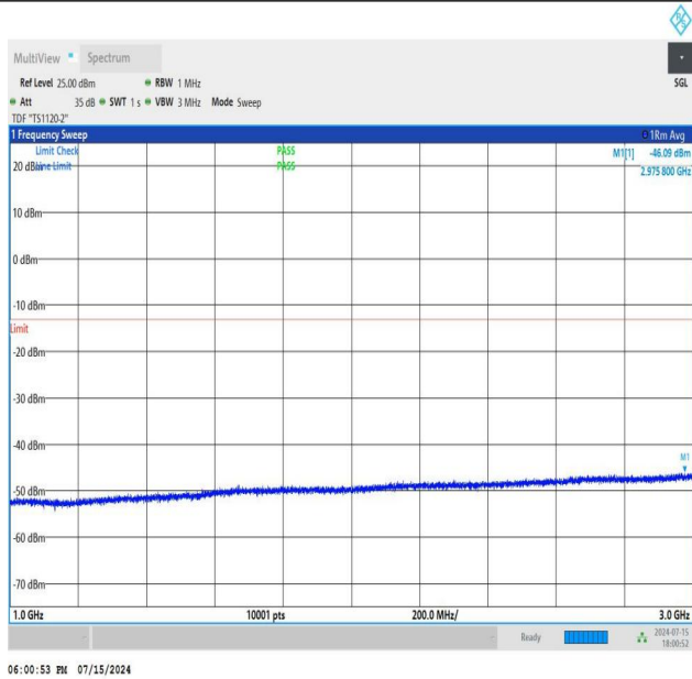
NTNV_N77-3450-3550_PC2_30_80_M_TID3_NS_01_1000_3000_#1
