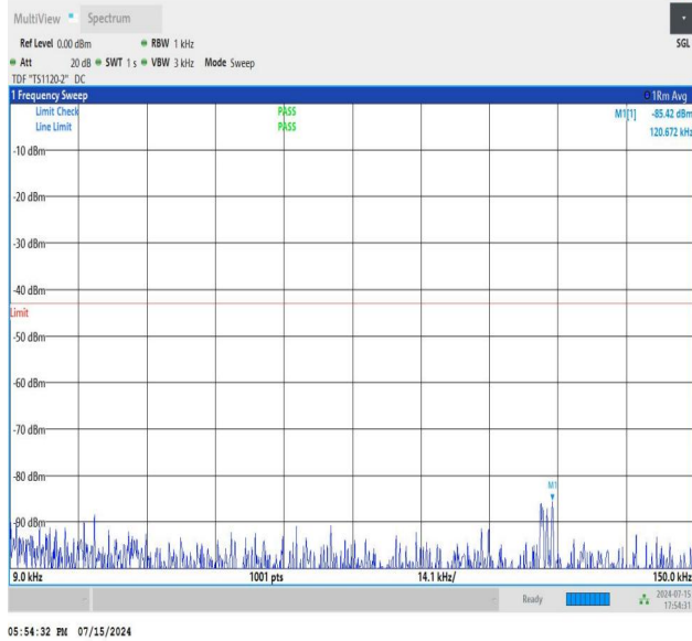
NTNV_N77-3450-3550_PC2_30_60_L_TID2_NS_01_0.009_0.15_#1
