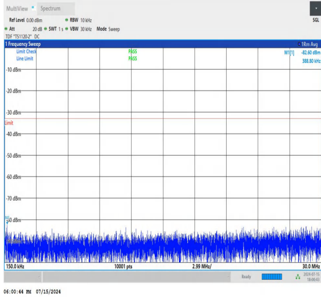
NTNV_N77-3450-3550_PC2_30_80_M_TID3_NS_01_0.15_30_#1
