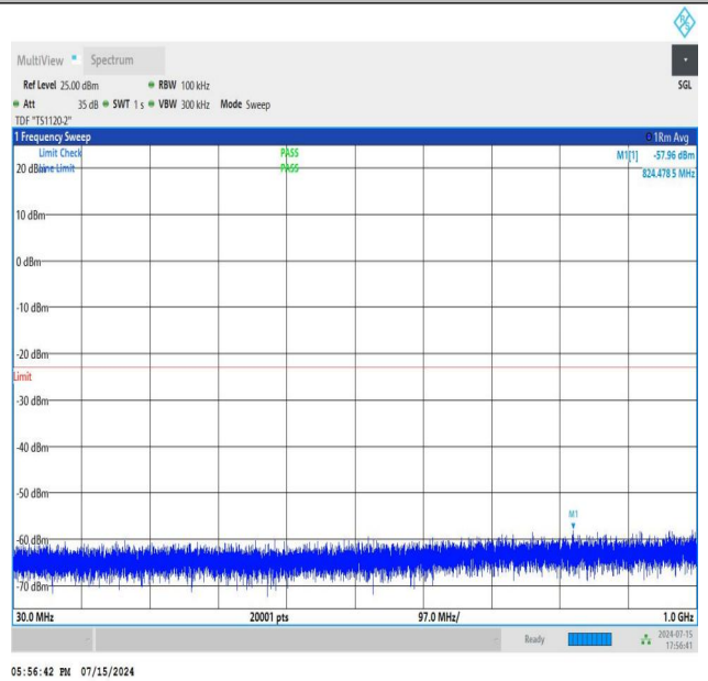
NTNV_N77-3450-3550_PC2_30_60_M_TID3_NS_01_30_1000_#1
