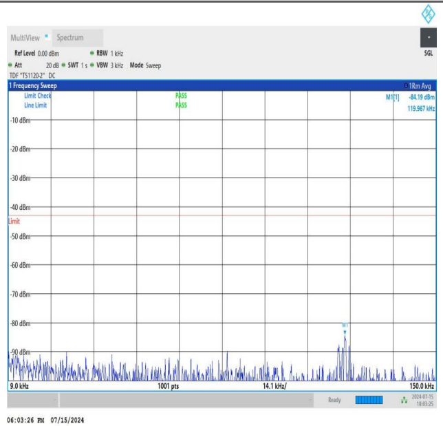
NTNV_N77-3450-3550_PC2_30_90_L_TID3_NS_01_0.009_0.15_#1
