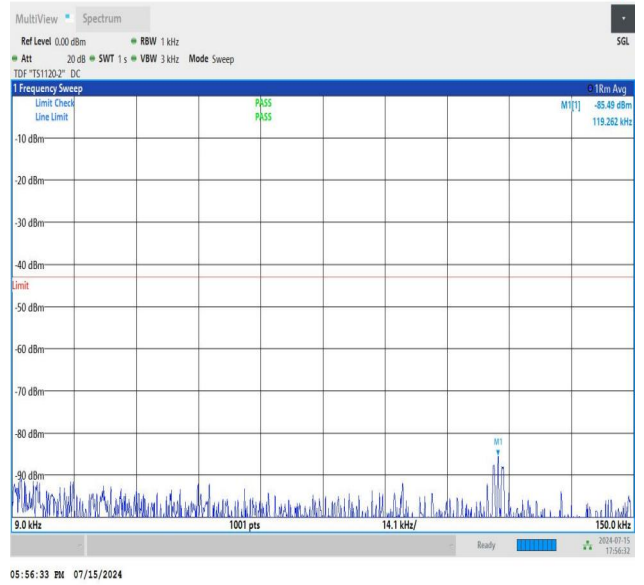
NTNV_N77-3450-3550_PC2_30_60_M_TID3_NS_01_0.009_0.15_#1
