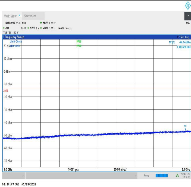
NTNV_N77-3450-3550_PC2_30_60_H_TID3_NS_01_1000_3000_#1
