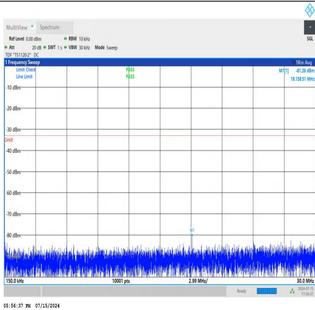
NTNV_N77-3450-3550_PC2_30_60_M_TID2_NS_01_20000_400_00_#1
