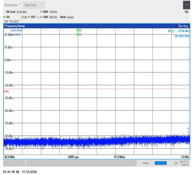
NTNV_N77-3450-3550_PC2_30_80_M_TID3_NS_01_30_1000_#
