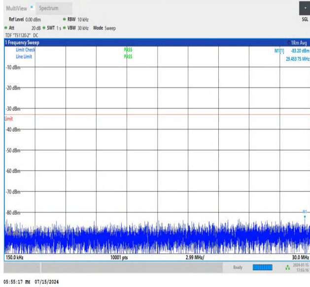
NTNV_N77-3450-3550_PC2_30_60_L_TID3_NS_01_0.15_30_#1
