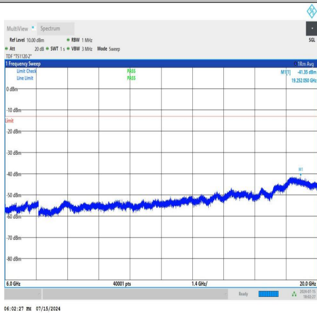
NTNV_N77-3450-3550_PC2_30_80_H_TID3_NS_01_6000_2000 0_#1
