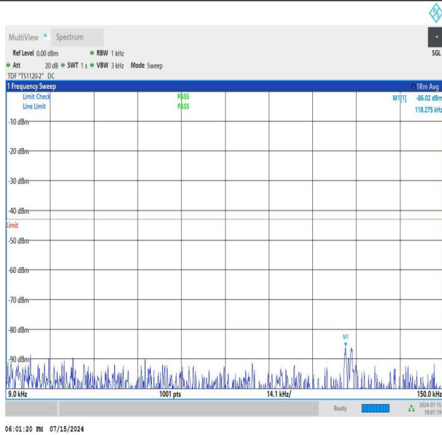
NTNV_N77-3450-3550_PC2_30_80_H_TID2_NS_01_0.009_0.15_#1
