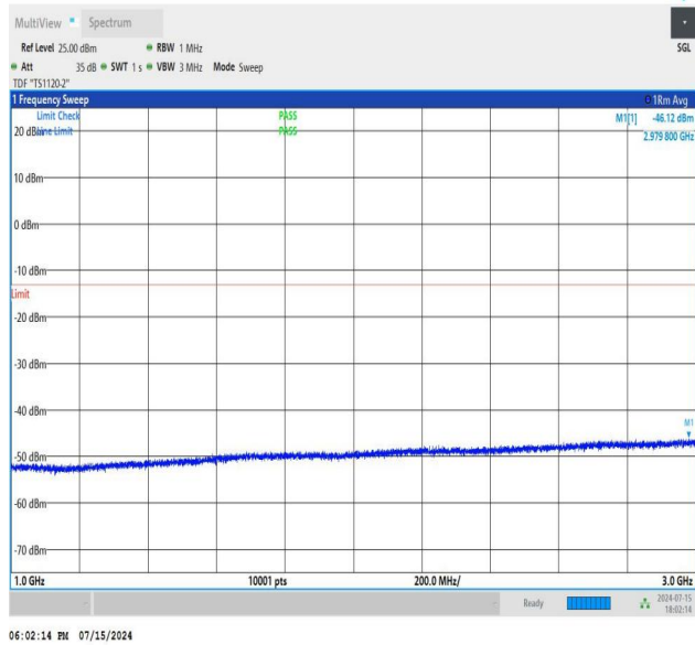
NTNV_N77-3450-3550_PC2_30_80_H_TID3_NS_01_1000_3000 #1
