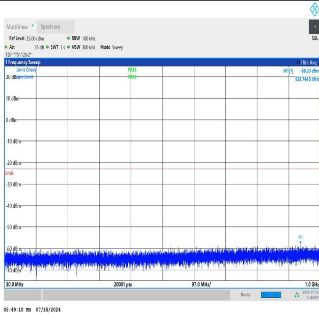
NTNV_N77-3450-3550_PC2_30_40_H_TID2_NS_01_30_1000_#1
