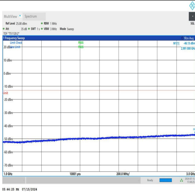
NTNV_N77-3450-3550_PC2_30_30_M_TID3_NS_01_1000_3000_#1
