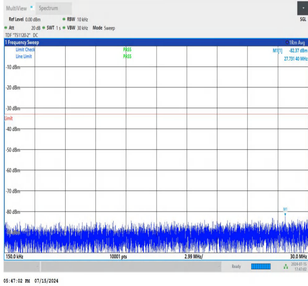
NTNV_N77-3450-3550_PC2_30_40_L_TID3_NS_01_0.15_30_#1
