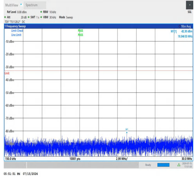
NTNV_N77-3450-3550_PC2_30_50_M_TID2_NS_01_0.15_30_#1
