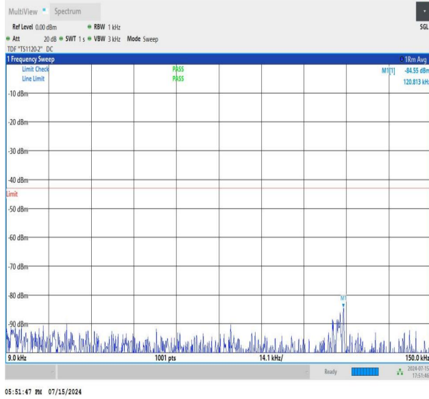
NTNV_N77-3450-3550_PC2_30_50_M_TID2_NS_01_0.009_0.15_#1
