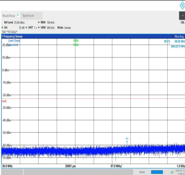
NTNV_N77-3450-3550_PC2_30_40_L_TID2_NS_01_0.009_0.15_#1
