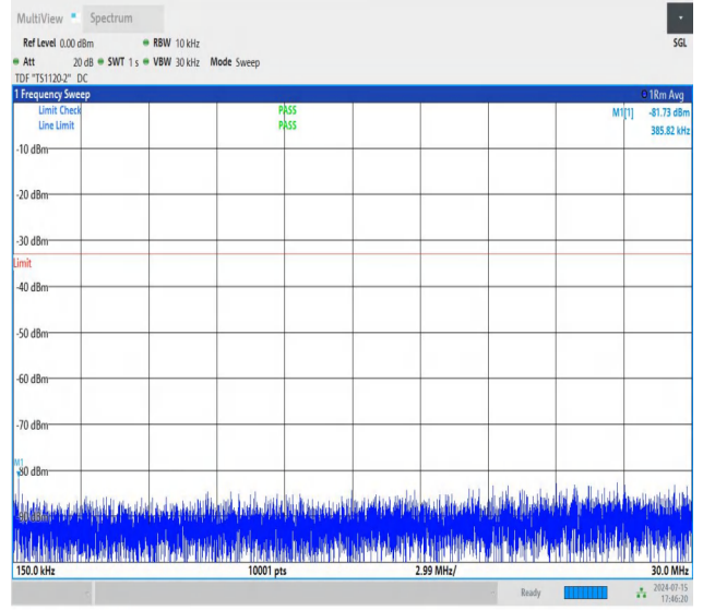
NTNV_N77-3450-3550_PC2_30_40_L_TID2_NS_01_0.15_30_#1
