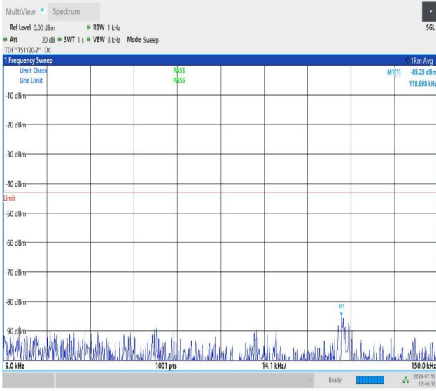
NTNV_N77-3450-3550_PC2_30_40_L_TID2_NS_01_0.009_0.15_#1
