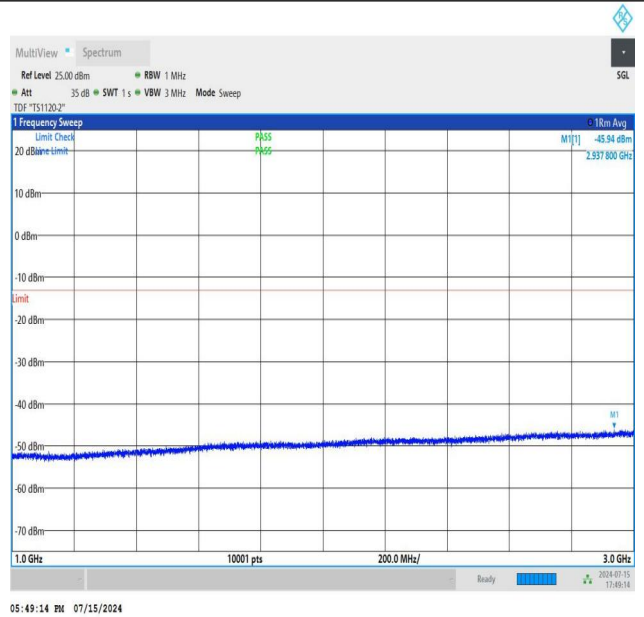
NTNV_N77-3450-3550_PC2_30_40_H_TID2_NS_01_1000_3000_#1
