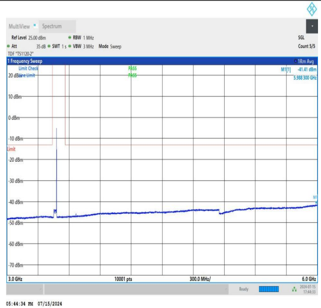
NTNV_N77-3450-3550_PC2_30_30_M_TID3_NS_01_3000_6000_#1
