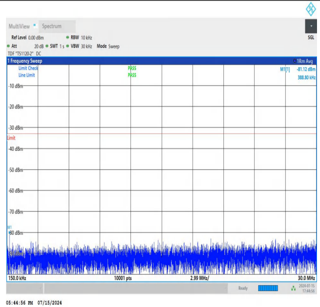
NTNV_N77-3450-3550_PC2_30_30_H_TID2_NS_01_0.15_30_#1
