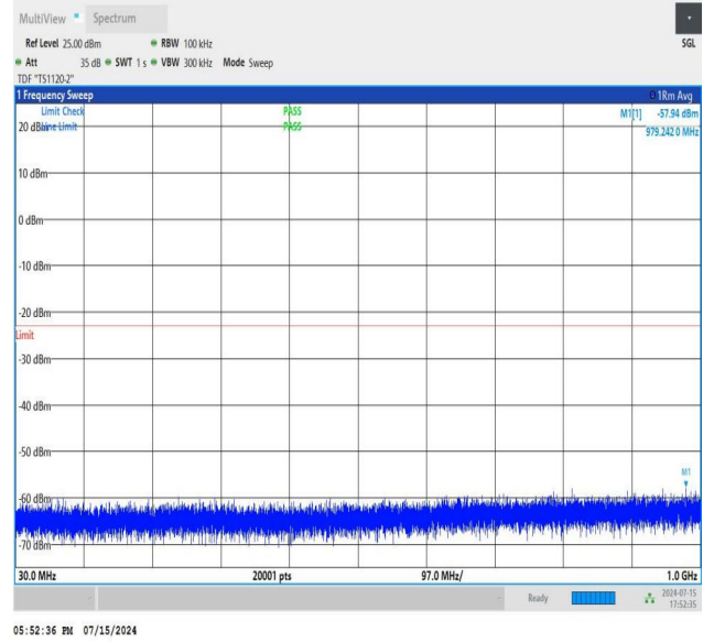
NTNV_N77-3450-3550_PC2_30_50_M_TID3_NS_01_30_1000_#
