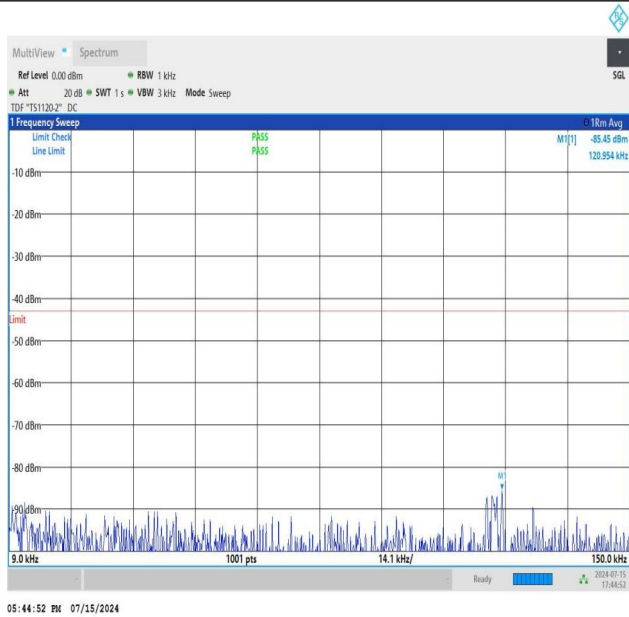
NTNV_N77-3450-3550_PC2_30_30_H_TID2_NS_01_0.009_0.15_#1
