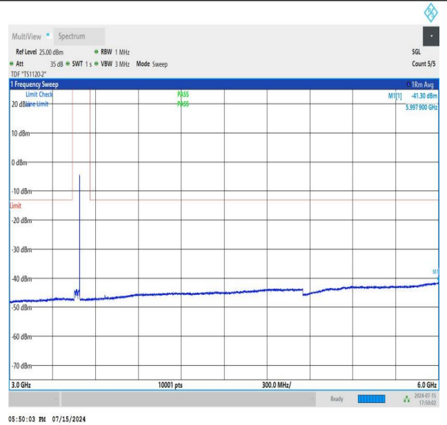
NTNV_N77-3450-3550_PC2_30_40_H_TID3_NS_01_3000_6000_#1
