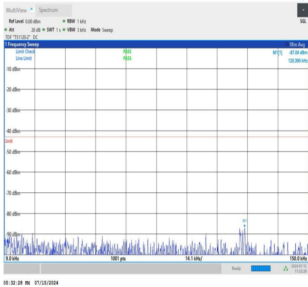
NTNV_N77-3450-3550_PC2_30_90_L_TID2_NS_01_0.009_0.15_#1
