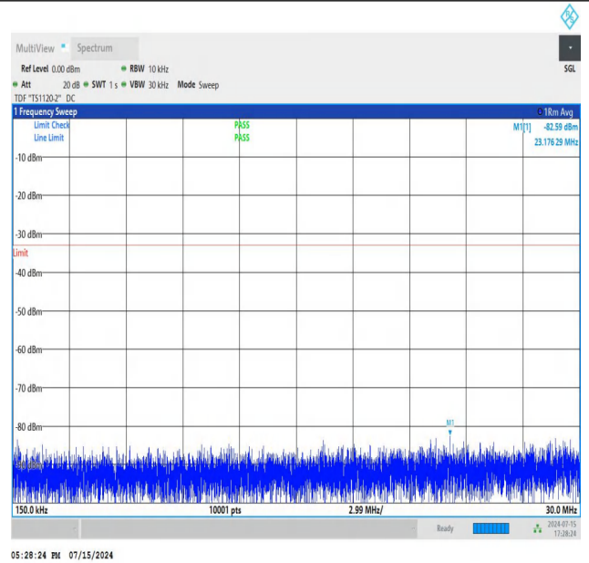
NTNV_N77-3450-3550_PC2_30_80_L_TID2_NS_01_0.15_30_#1
