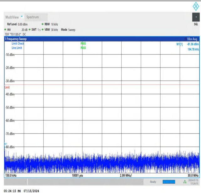
NTNV_N77-3450-3550_PC2_30_60_L_TID2_NS_01_0.15_30_#1
