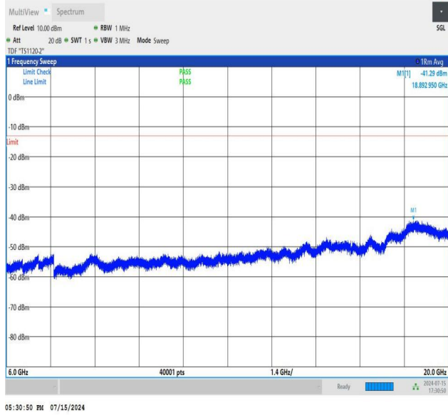
NTNV_N77-3450-3550_PC2_30_80_M_TID3_NS_01_6000_2000_0_#1
