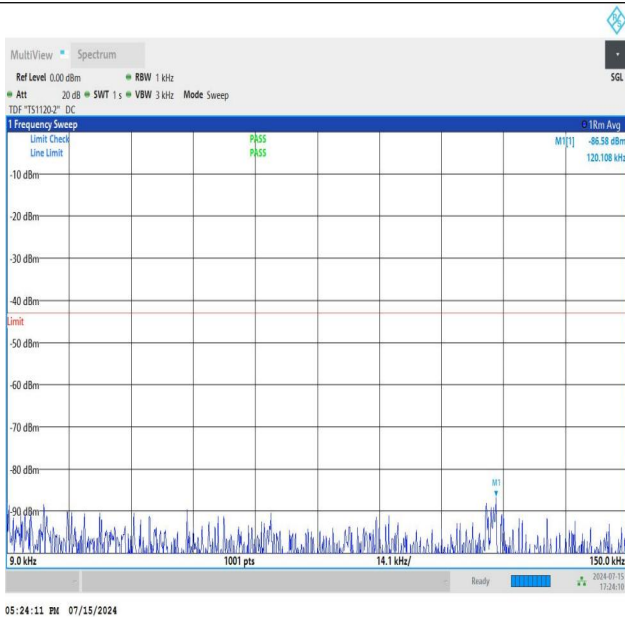
NTNV_N77-3450-3550_PC2_30_60_L_TID2_NS_01_0.009_0.15_#1
