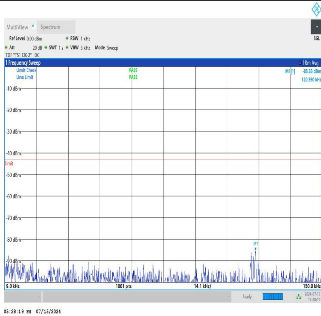
NTNV_N77-3450-3550_PC2_30_80_L_TID2_NS_01_0.009_0.15_#1
