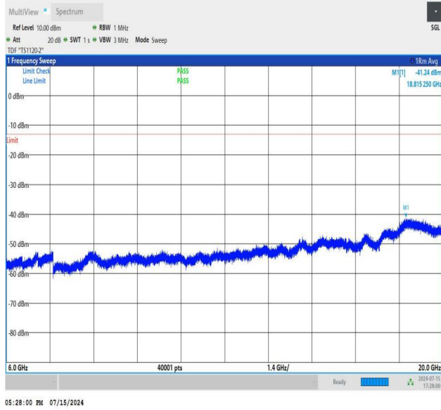
NTNV_N77-3450-3550_PC2_30_60_H_TID3_NS_01_6000_2000_0_#1
