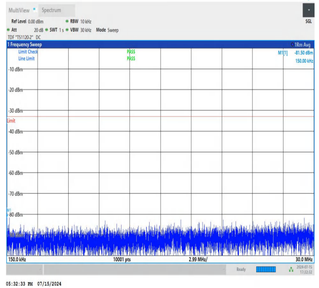
NTNV_N77-3450-3550_PC2_30_90_L_TID2_NS_01_0.15_30_#1
