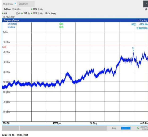
NTNV_N77-3450-3550_PC2_30_50_H_TID2_NS_01_20000_400_00_#1
