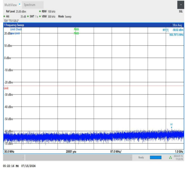
NTNV_N77-3450-3550_PC2_30_50_M_TID3_NS_01_30_1000_#
