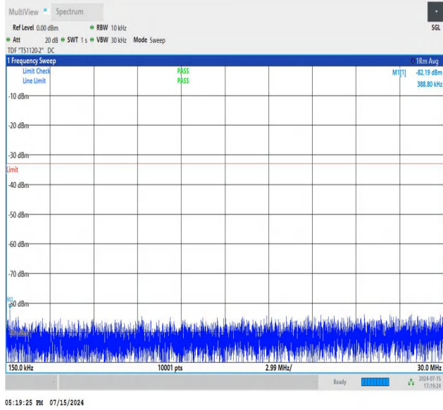
NTNV_N77-3450-3550_PC2_30_40_H_TID3_NS_01_0.15_30_#1
