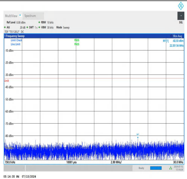
NTNV_N77-3450-3550_PC2_30_30_H_TID2_NS_01_0.15_30_#1
