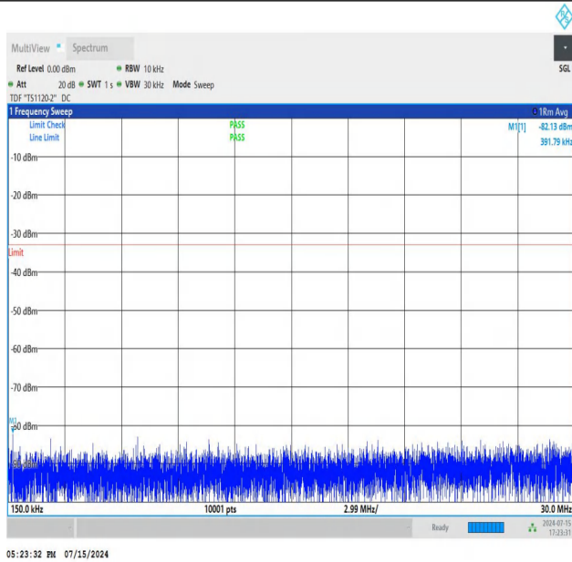
NTNV_N77-3450-3550_PC2_30_50_H_TID3_NS_01_0.15_30_#1
