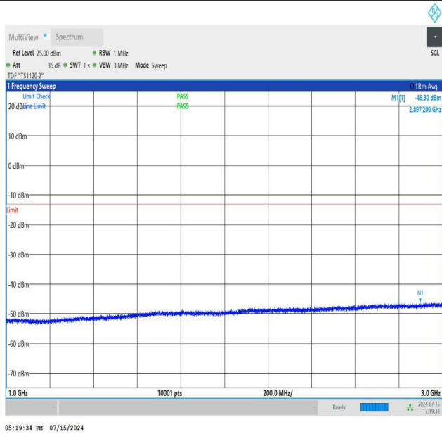
NTNV_N77-3450-3550_PC2_30_40_H_TID3_NS_01_1000_3000_#1
