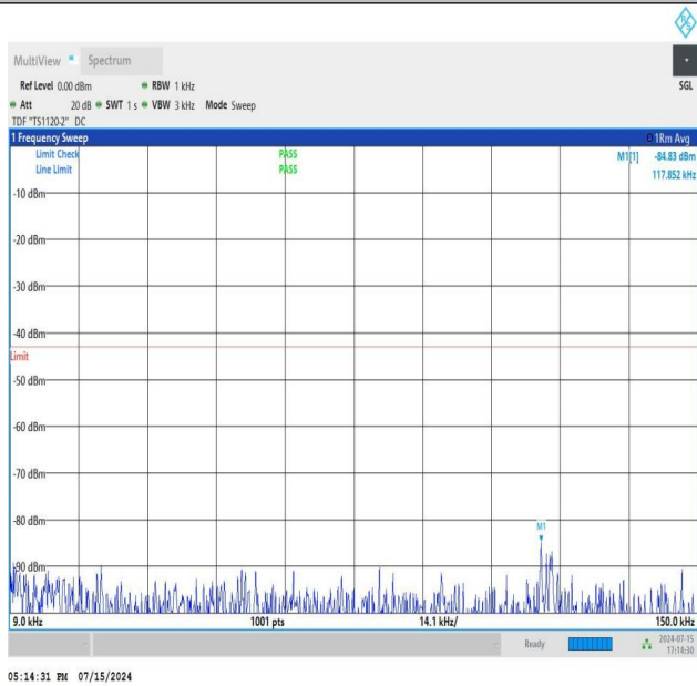
NTNV_N77-3450-3550_PC2_30_30_H_TID2_NS_01_0.009_0.15_#1
