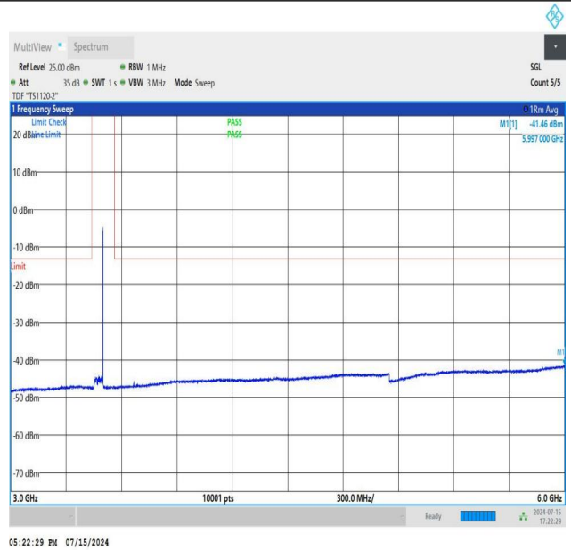
NTNV_N77-3450-3550_PC2_30_50_M_TID3_NS_01_3000_6000_#1
