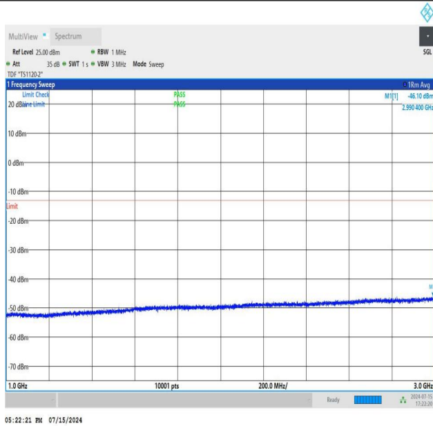
NTNV_N77-3450-3550_PC2_30_50_M_TID3_NS_01_1000_3000_#1
