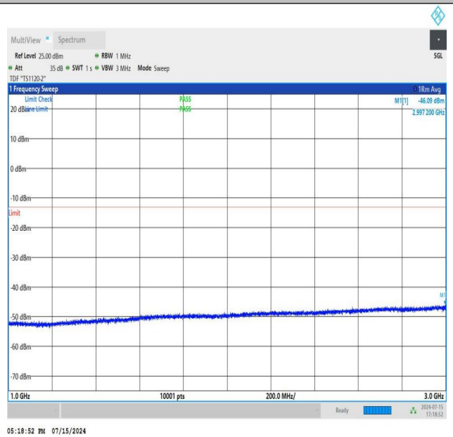
NTNV_N77-3450-3550_PC2_30_40_H_TID2_NS_01_1000_3000_#1
