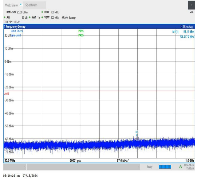
NTNV_N77-3450-3550_PC2_30_40_H_TID3_NS_01_30_1000_#
