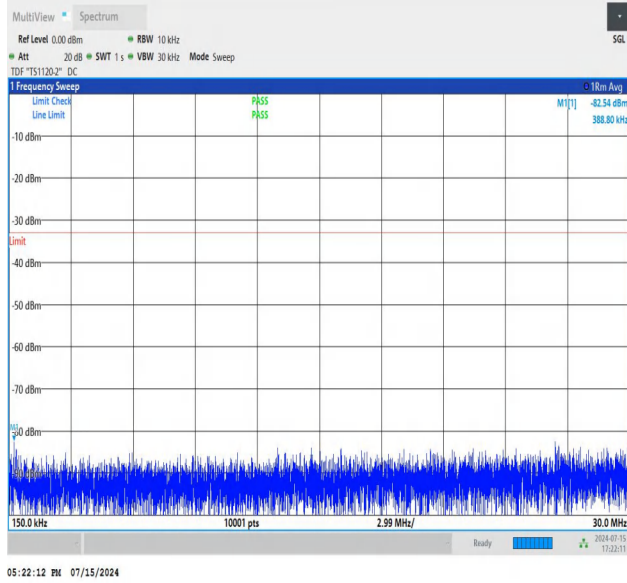
NTNV_N77-3450-3550_PC2_30_50_M_TID3_NS_01_0.15_30_#1
