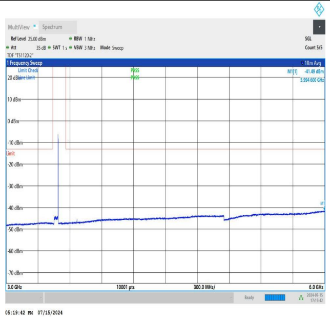
NTNV_N77-3450-3550_PC2_30_40_H_TID3_NS_01_3000_6000_#1
