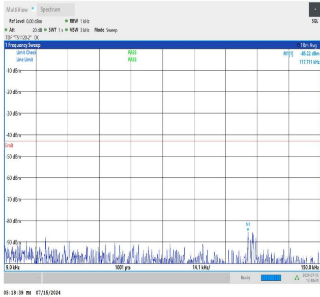
NTNV_N77-3450-3550_PC2_30_40_H_TID2_NS_01_0.009_0.15_#1
