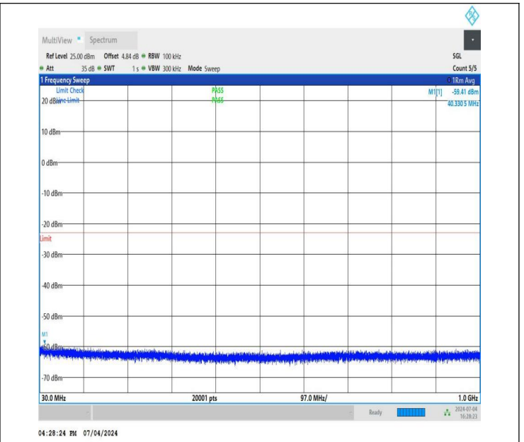
NTNV_DC_26A_n78A-3450-3550_PC3_30_5+90_M+M_TID2_N S_01_30_1000_#1
