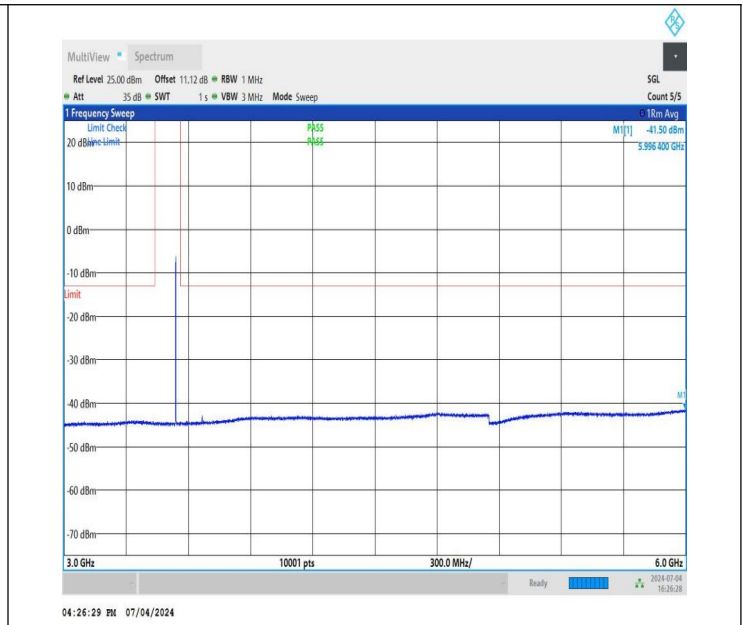
NTNV_DC_26A_n78A-3450-3550_PC3_30_5+90_M+L_TID5_NS_01_3000_6000_#1
