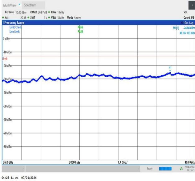
NTNV_DC_26A_n78A-3450-3550_PC3_30_5+90_M+L_TID4_NS_01_26000_40000_#1
