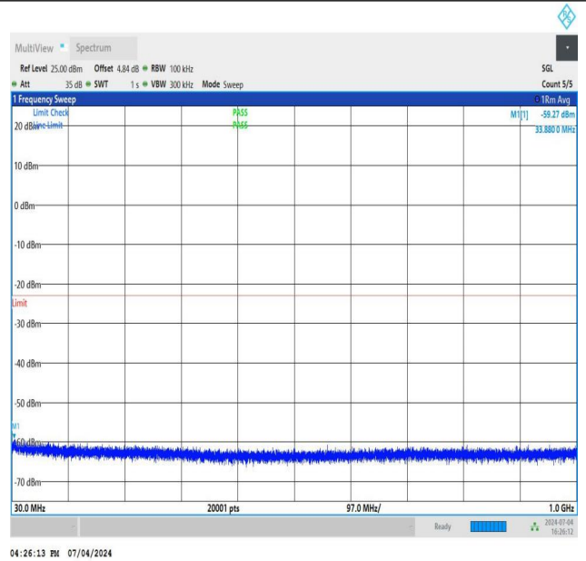
NTNV_DC_26A_n78A-3450-3550_PC3_30_5+90_M+L_TID5_NS_01_30_1000_#1
