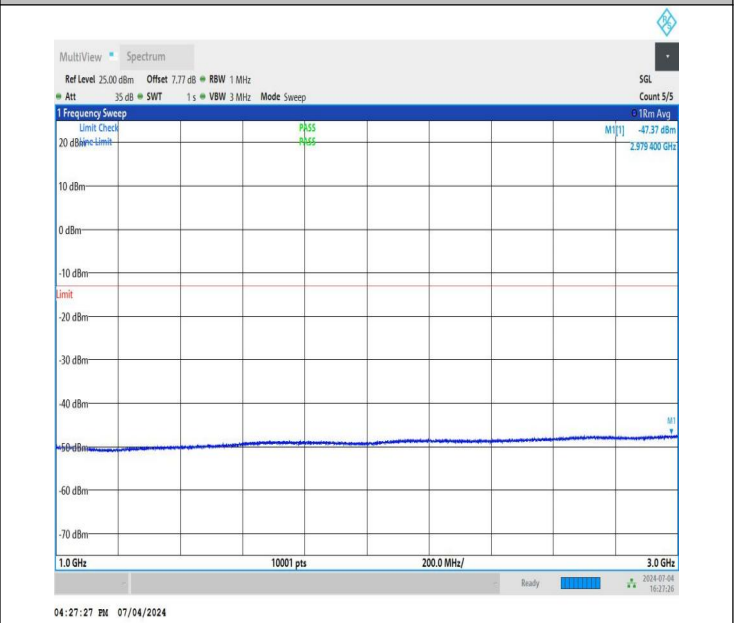
NTNV_DC_26A_n78A-3450-3550_PC3_30_5+90_M+M_TID1_N S_01_1000_3000_#1
