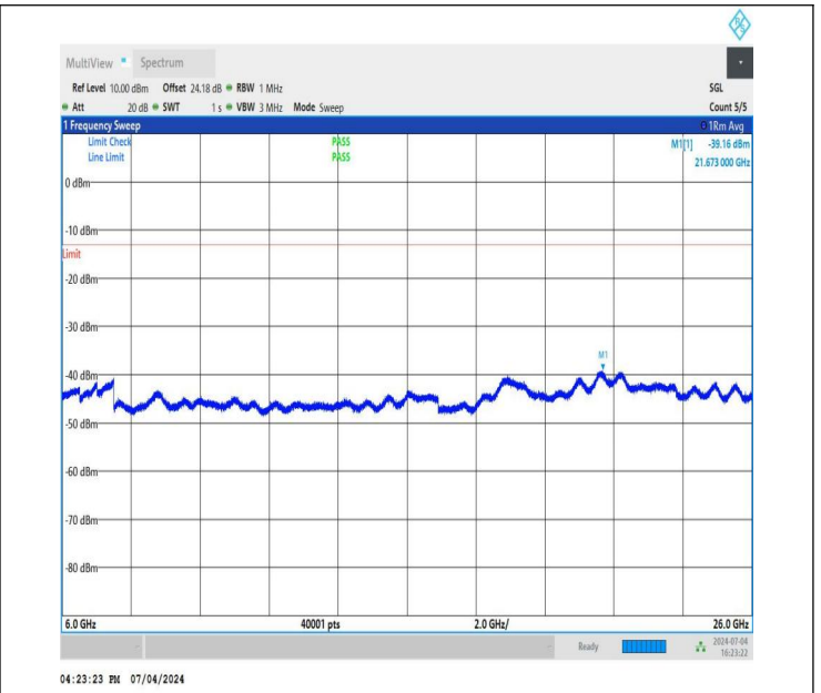
NTNV_DC_26A_n78A-3450-3550_PC3_30_5+90_M+L_TID1_NS_01_6000_26000_#1
