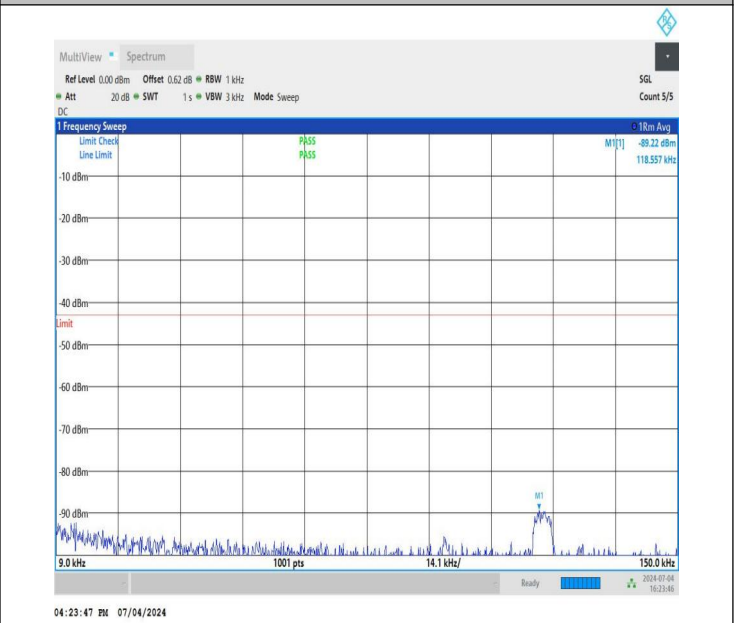
NTNV_DC_26A_n78A-3450-3550_PC3_30_5+90_M+L_TID2_NS_01_0.009_0.15_#1
