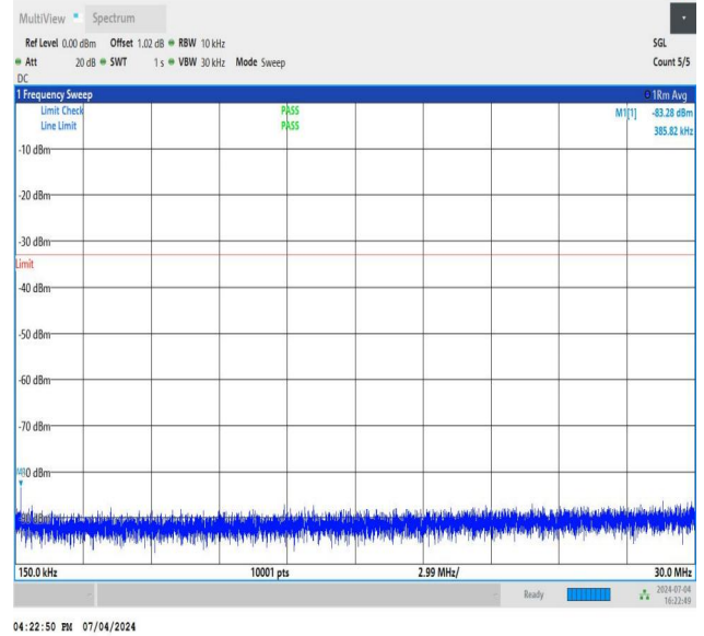
NTNV_DC_26A_n78A-3450-3550_PC3_30_5+90_M+L_TID1_NS_01_0.15_30_#1
