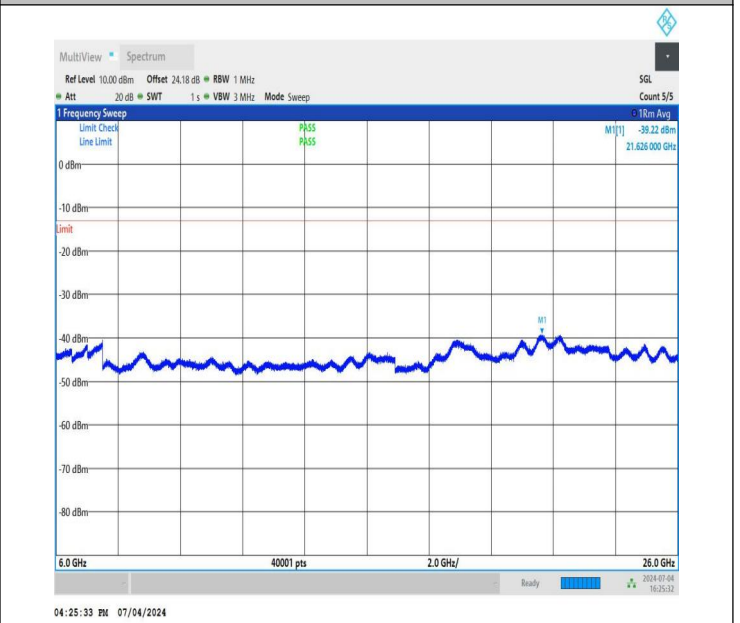
NTNV_DC_26A_n78A-3450-3550_PC3_30_5+90_M+L_TID4_NS_01_6000_26000_#1
