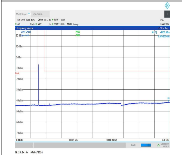
NTNV_DC_26A_n78A-3450-3550_PC3_30_5+90_M+L_TID4_NS_01_3000_6000_#1
