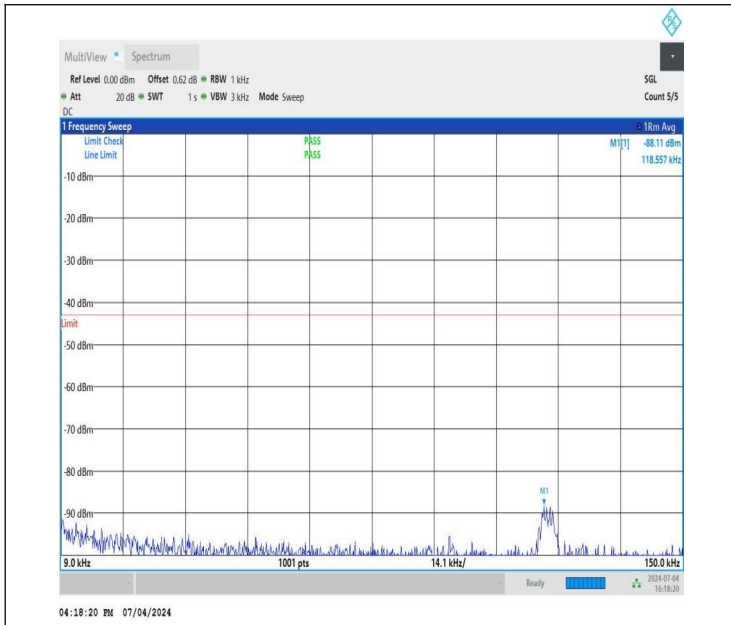
NTNV_DC_26A_n78A-3450-3550_PC3_30_5+80_M+H_TID1_N S_01_0.009_0.15_#1
