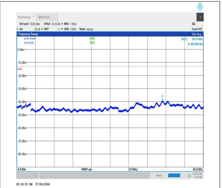
NTNV_DC_26A_n78A-3450-3550_PC3_30_5+80_M+H_TID1_N S_01_6000_26000_#1
