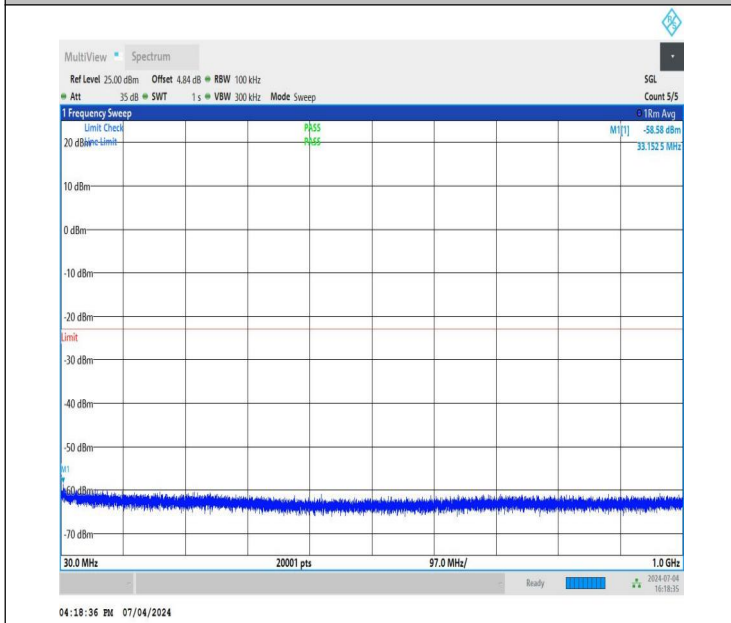
NTNV_DC_26A_n78A-3450-3550_PC3_30_5+80_M+H_TID1_N S_01_30_1000_#1
