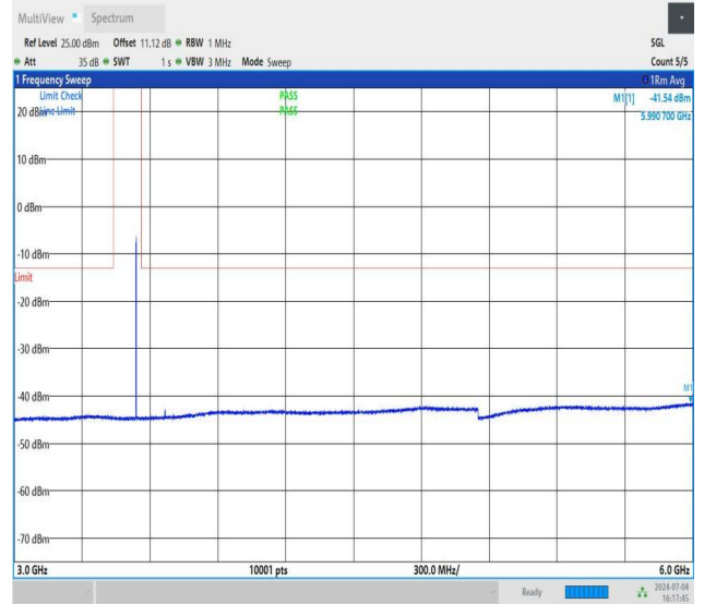
NTNV_DC_26A_n78A-3450-3550_PC3_30_5+80_M+M_TID5_N S_01_3000_6000_#1
