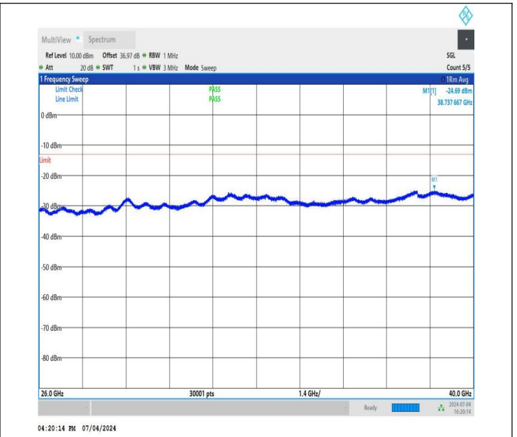
NTNV_DC_26A_n78A-3450-3550_PC3_30_5+80_M+H_TID2_N S_01_26000_40000_#1
