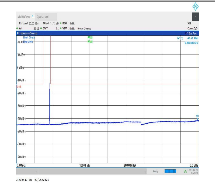
NTNV_DC_26A_n78A-3450-3550_PC3_30_5+90_M+M_TID2_N S_01_3000_6000_#1
