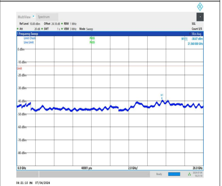
NTNV_DC_26A_n78A-3450-3550_PC3_30_5+80_M+H_TID4_N S_01_6000_26000_#1
