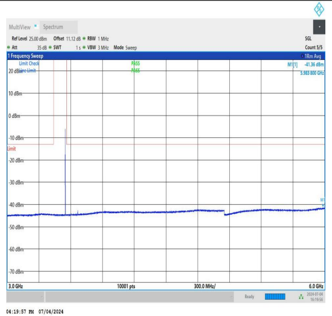
NTNV_DC_26A_n78A-3450-3550_PC3_30_5+80_M+H_TID2_N S_01_3000_6000_#1
