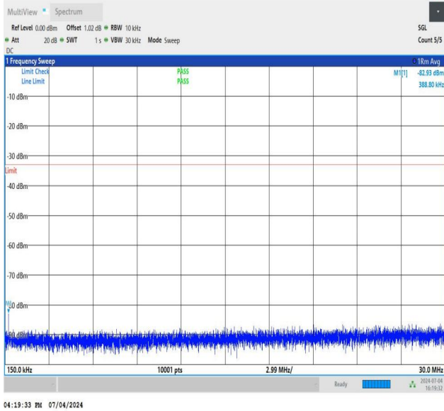
NTNV_DC_26A_n78A-3450-3550_PC3_30_5+80_M+H_TID2_N S_01_0.15_30_#1
