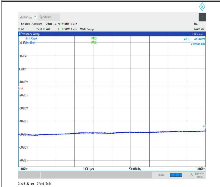
NTNV_DC_26A_n78A-3450-3550_PC3_30_5+90_M+M_TID2_N S_01_1000_3000_#1
