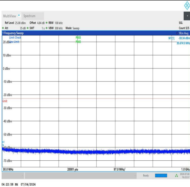
NTNV_DC_26A_n78A-3450-3550_PC3_30_5+90_M+L_TID1_NS_01_30_1000_#1
