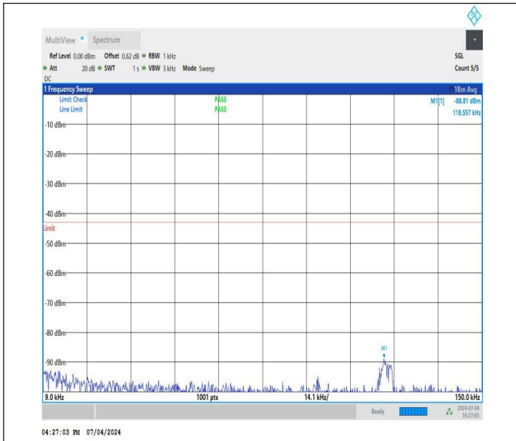
NTNV_DC_26A_n78A-3450-3550_PC3_30_5+90_M+M_TID1_N S_01_0.009_0.15_#1
