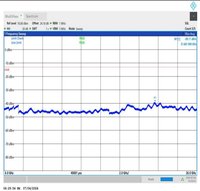
NTNV_DC_26A_n78A-3450-3550_PC3_30_5+90_M+M_TID4_N S_01_6000_26000_#1
