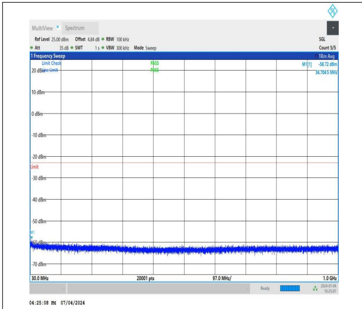
NTNV_DC_26A_n78A-3450-3550_PC3_30_5+90_M+L_TID4_NS_01_30_1000_#1
