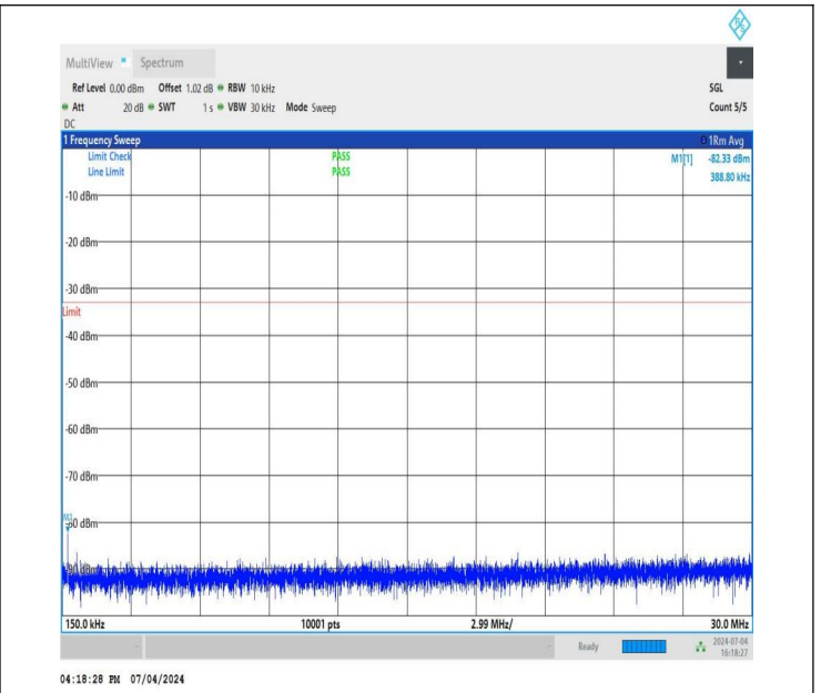
NTNV_DC_26A_n78A-3450-3550_PC3_30_5+80_M+H_TID1_N S_01_0.15_30_#1
