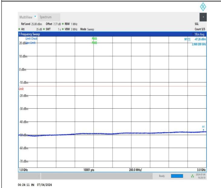
NTNV_DC_26A_n78A-3450-3550_PC3_30_5+90_M+L_TID2_NS_01_1000_3000_#1
