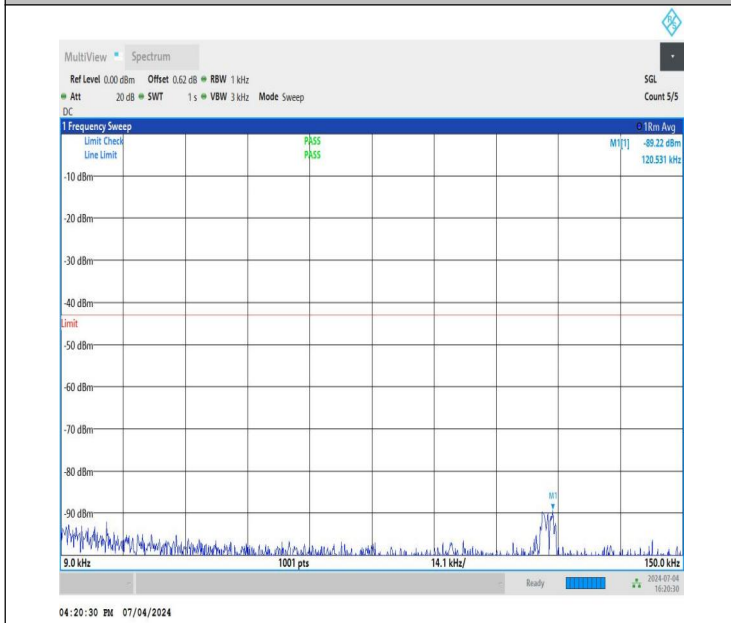
NTNV_DC_26A_n78A-3450-3550_PC3_30_5+80_M+H_TID4_N S_01_0.009_0.15_#1
