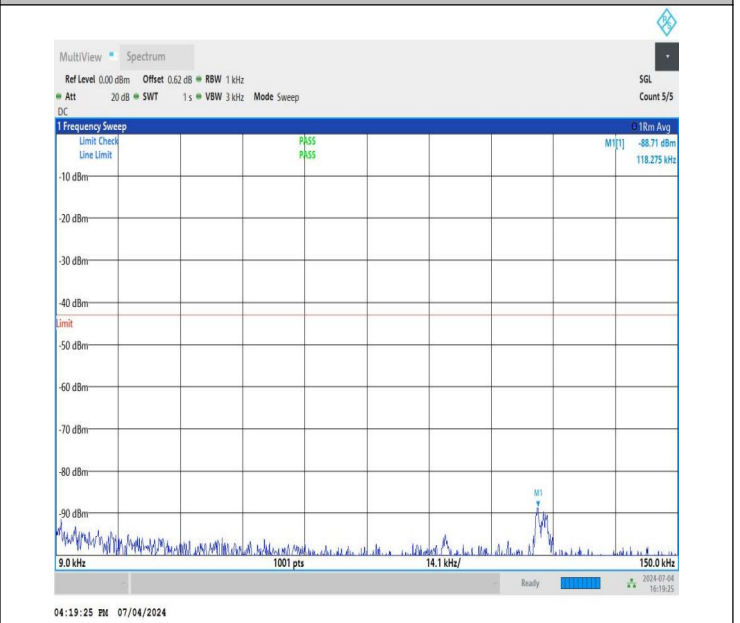
NTNV_DC_26A_n78A-3450-3550_PC3_30_5+80_M+H_TID2_N S_01_0.009_0.15_#1
