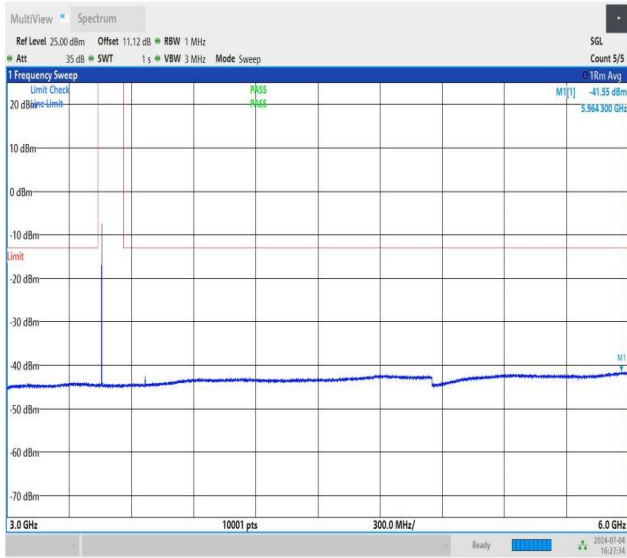
NTNV_DC_26A_n78A-3450-3550_PC3_30_5+90_M+M_TID1_N S_01_3000_6000_#1
