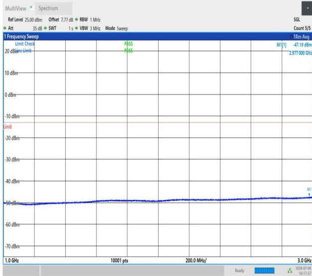
NTNV_DC_26A_n78A-3450-3550_PC3_30_5+80_M+M_TID5_N S_01_1000_3000_#1
