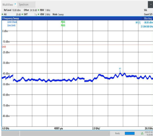
NTNV_DC_26A_n78A-3450-3550_PC3_30_5+90_M+M_TID2_N S_01_6000_26000_#1
