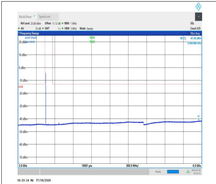
NTNV_DC_26A_n78A-3450-3550_PC3_30_5+90_M+L_TID1_NS_01_3000_6000_#1
