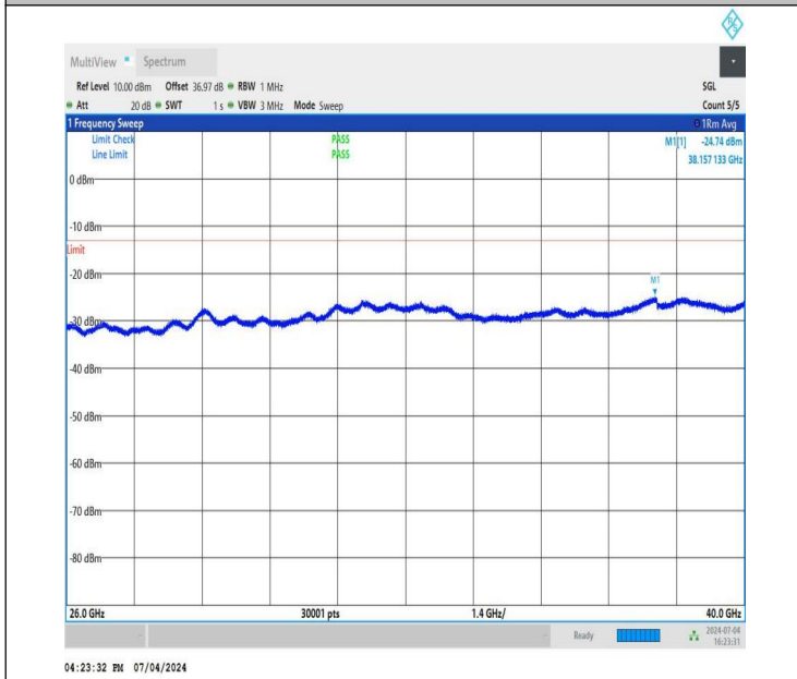
NTNV_DC_26A_n78A-3450-3550_PC3_30_5+90_M+L_TID1_NS_01_26000_40000_#1
