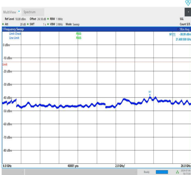
NTNV_DC_26A_n78A-3450-3550_PC3_30_5+80_M+M_TID5_N S_01_6000_26000_#1
