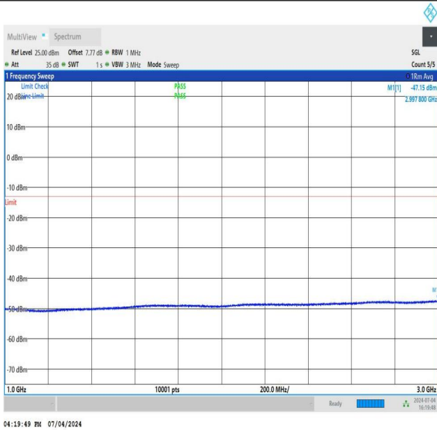
NTNV_DC_26A_n78A-3450-3550_PC3_30_5+80_M+H_TID2_N S_01_1000_3000_#1
