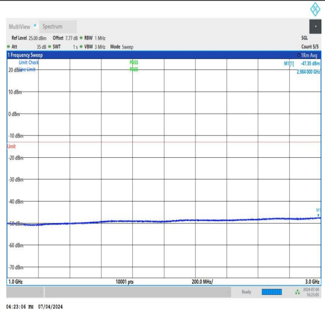
NTNV_DC_26A_n78A-3450-3550_PC3_30_5+90_M+L_TID1_NS_01_1000_3000_#1
