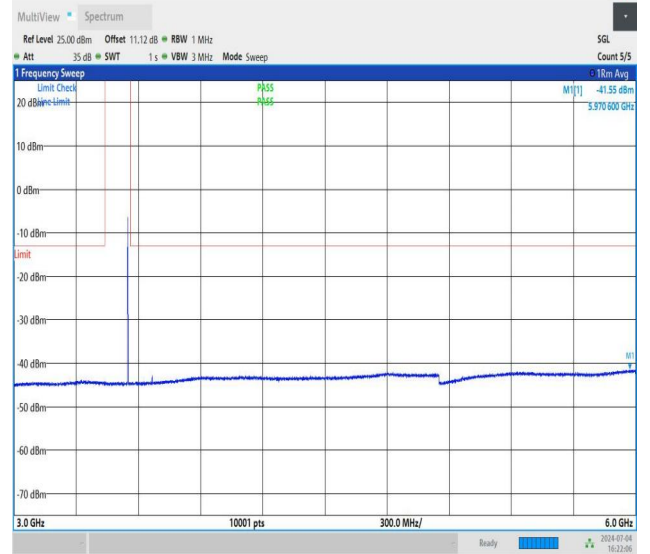
NTNV_DC_26A_n78A-3450-3550_PC3_30_5+80_M+H_TID5_N S_01_3000_6000_#1
