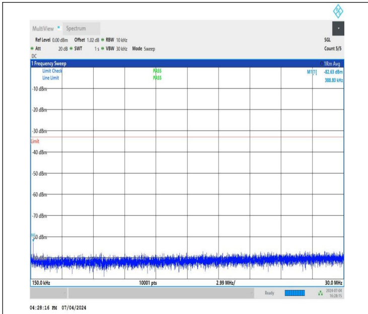
NTNV_DC_26A_n78A-3450-3550_PC3_30_5+90_M+M_TID2_N S_01_0.15_30_#1
