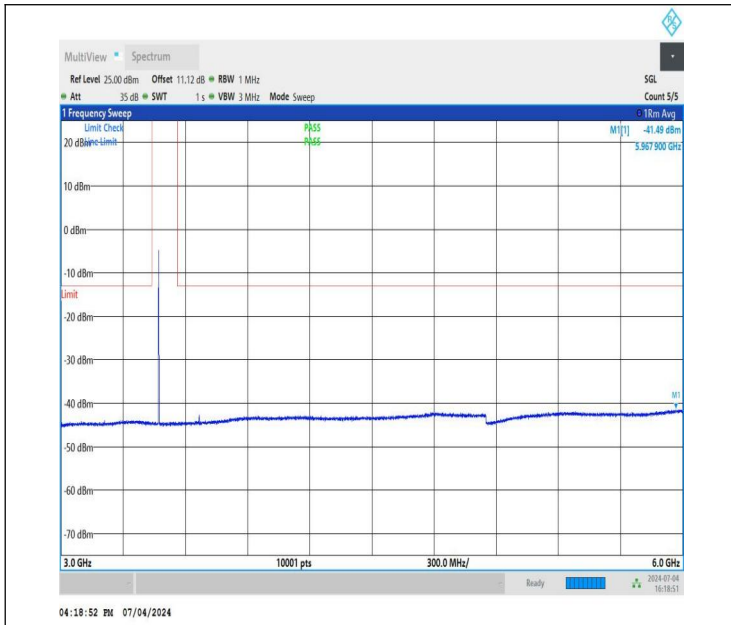
NTNV_DC_26A_n78A-3450-3550_PC3_30_5+80_M+H_TID1_N S_01_3000_6000_#1
