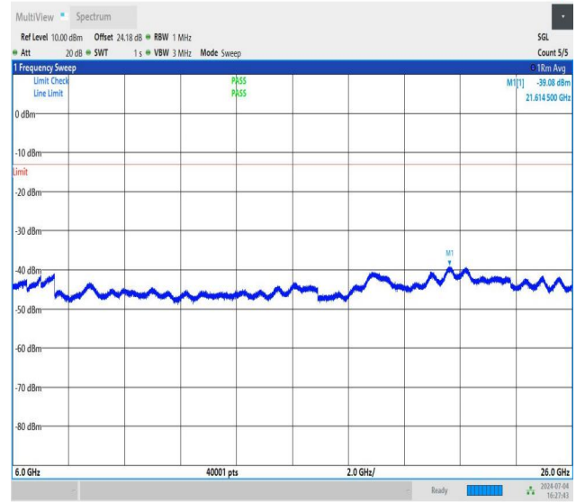
NTNV_DC_26A_n78A-3450-3550_PC3_30_5+90_M+M_TID1_N S_01_6000_26000_#1
