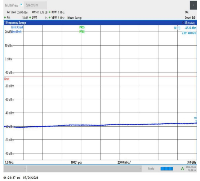
NTNV_DC_26A_n78A-3450-3550_PC3_30_5+90_M+M_TID4_N S_01_1000_3000_#1
