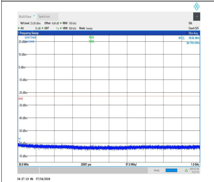
NTNV_DC_26A_n78A-3450-3550_PC3_30_5+90_M+M_TID1_N S_01_30_1000_#1
