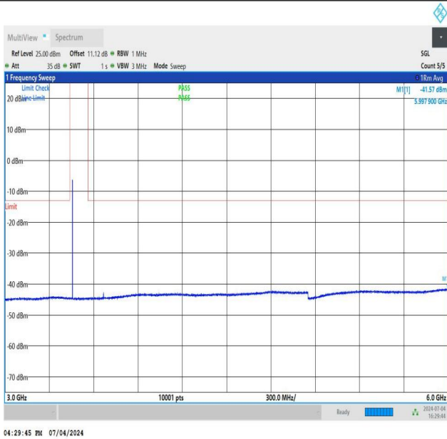
NTNV_DC_26A_n78A-3450-3550_PC3_30_5+90_M+M_TID4_N S_01_3000_6000_#1
