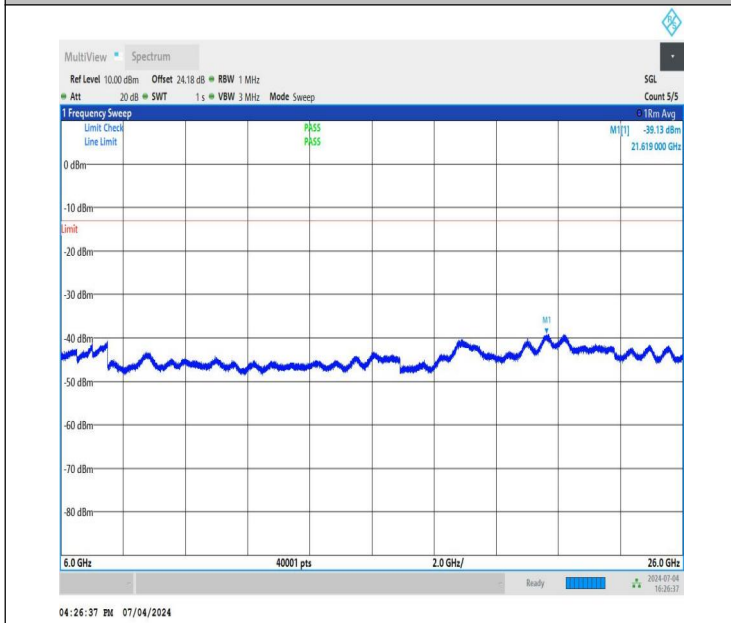
NTNV_DC_26A_n78A-3450-3550_PC3_30_5+90_M+L_TID5_NS_01_6000_26000_#1
