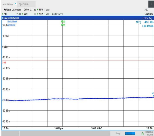
NTNV_DC_26A_n78A-3450-3550_PC3_30_5+80_M+H_TID5_N S_01_1000_3000_#1
