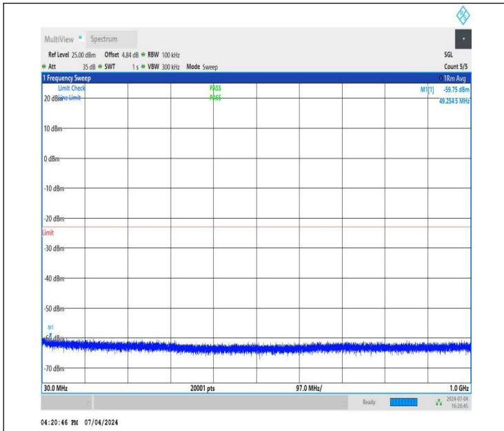
NTNV_DC_26A_n78A-3450-3550_PC3_30_5+80_M+H_TID4_N S_01_30_1000_#1
