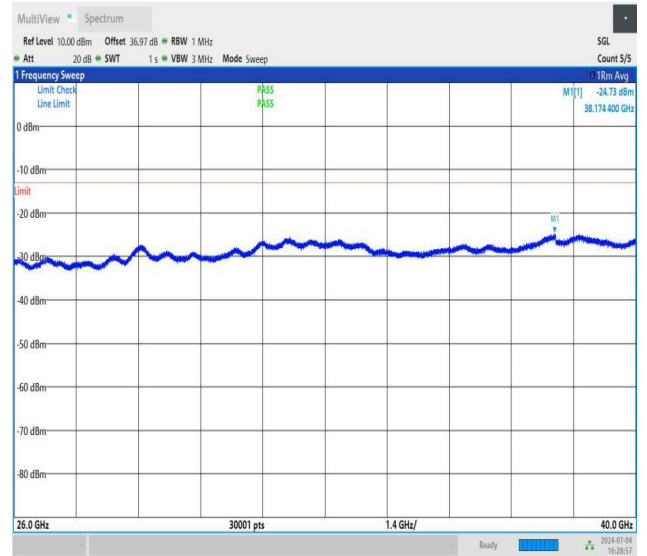
NTNV_DC_26A_n78A-3450-3550_PC3_30_5+90_M+M_TID2_N S_01_26000_40000_#1
