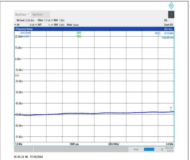
NTNV_DC_26A_n78A-3450-3550_PC3_30_5+90_M+L_TID4_NS_01_1000_3000_#1
