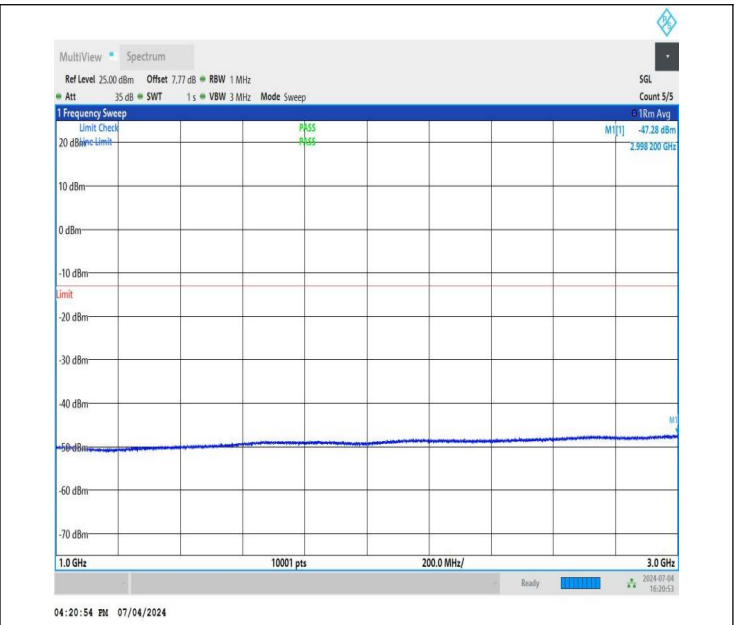
NTNV_DC_26A_n78A-3450-3550_PC3_30_5+80_M+H_TID4_N S_01_1000_3000_#1
