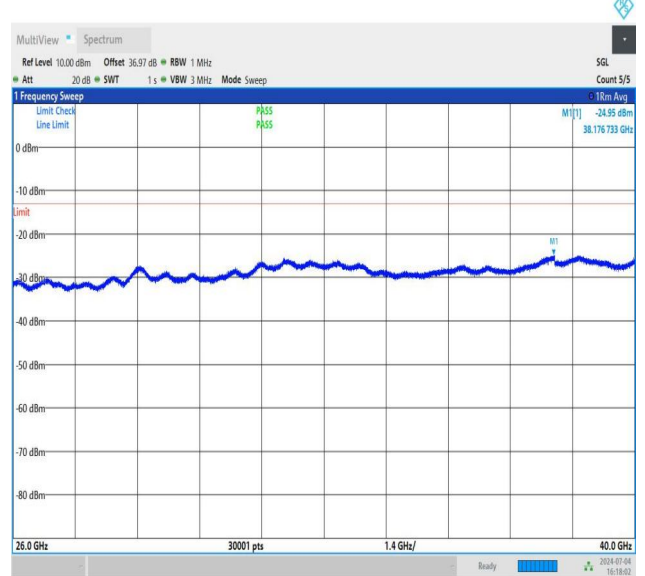
NTNV_DC_26A_n78A-3450-3550_PC3_30_5+80_M+M_TID5_N S_01_26000_40000_#1
