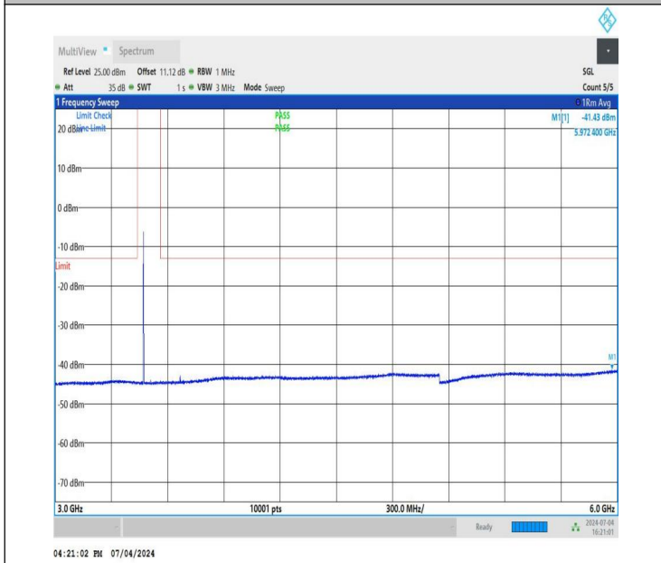
NTNV_DC_26A_n78A-3450-3550_PC3_30_5+80_M+H_TID4_N S_01_3000_6000_#1
