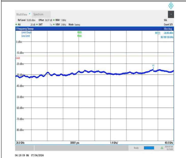
NTNV_DC_26A_n78A-3450-3550_PC3_30_5+80_M+H_TID1_N S_01_26000_40000_#1
