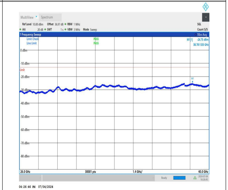
NTNV_DC_26A_n78A-3450-3550_PC3_30_5+90_M+L_TID5_NS_01_26000_40000_#1
