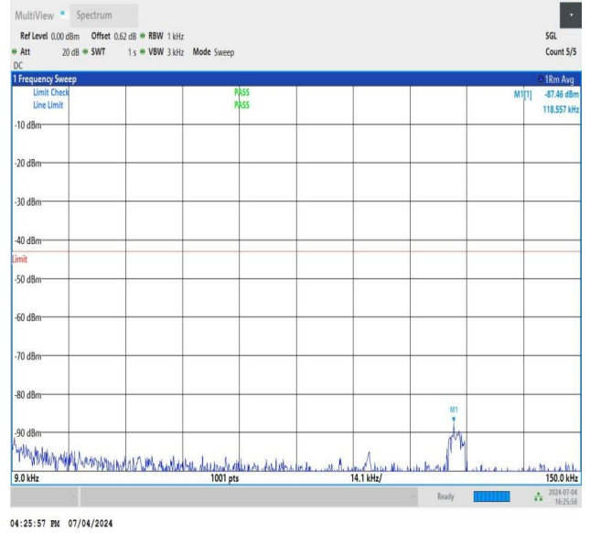
NTNV_DC_26A_n78A-3450-3550_PC3_30_5+90_M+L_TID5_NS_01_0.009_0.15_#1
