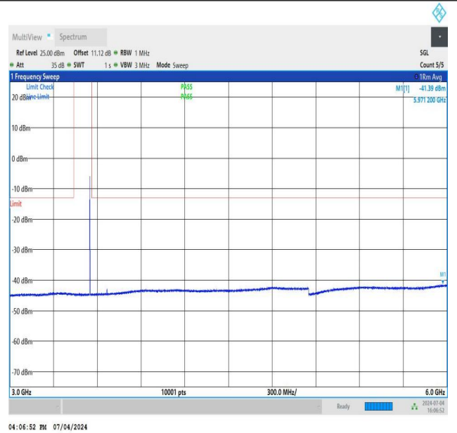
NTNV_DC_26A_n78A-3450-3550_PC3_30_5+70_M+H_TID2_N S_01_3000_6000_#1
