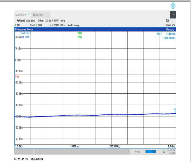
NTNV_DC_26A_n78A-3450-3550_PC3_30_5+70_M+H_TID1_N S_01_1000_3000_#1
