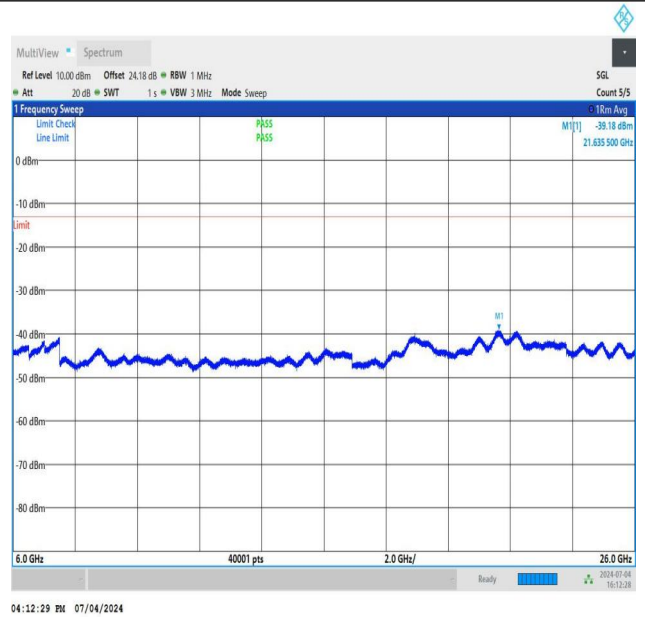
NTNV_DC_26A_n78A-3450-3550_PC3_30_5+80_M+L_TID4_NS_01_6000_26000_#1
