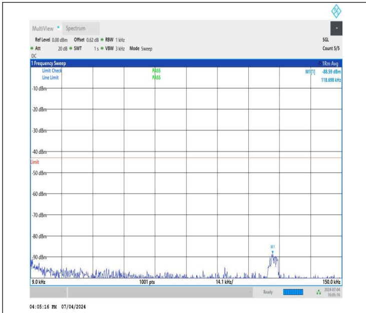
NTNV_DC_26A_n78A-3450-3550_PC3_30_5+70_M+H_TID1_N S_01_0.009_0.15_#1
