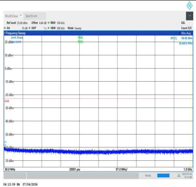
NTNV_DC_26A_n78A-3450-3550_PC3_30_5+80_M+L_TID5_NS_01_30_1000_#1
