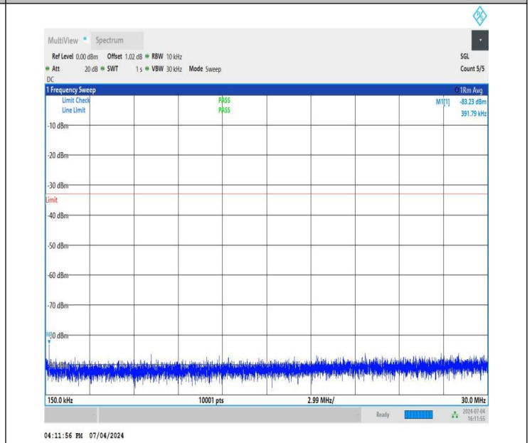
NTNV_DC_26A_n78A-3450-3550_PC3_30_5+80_M+L_TID4_NS_01_0.15_30_#1
