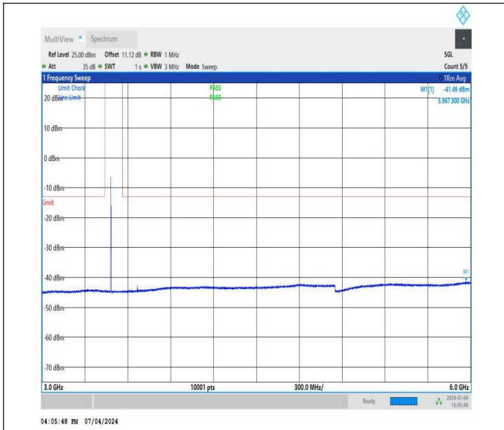
NTNV_DC_26A_n78A-3450-3550_PC3_30_5+70_M+H_TID1_N S_01_3000_6000_#1
