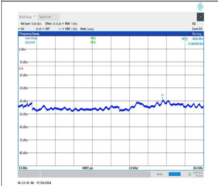
NTNV_DC_26A_n78A-3450-3550_PC3_30_5+80_M+L_TID5_NS_01_6000_26000_#1
