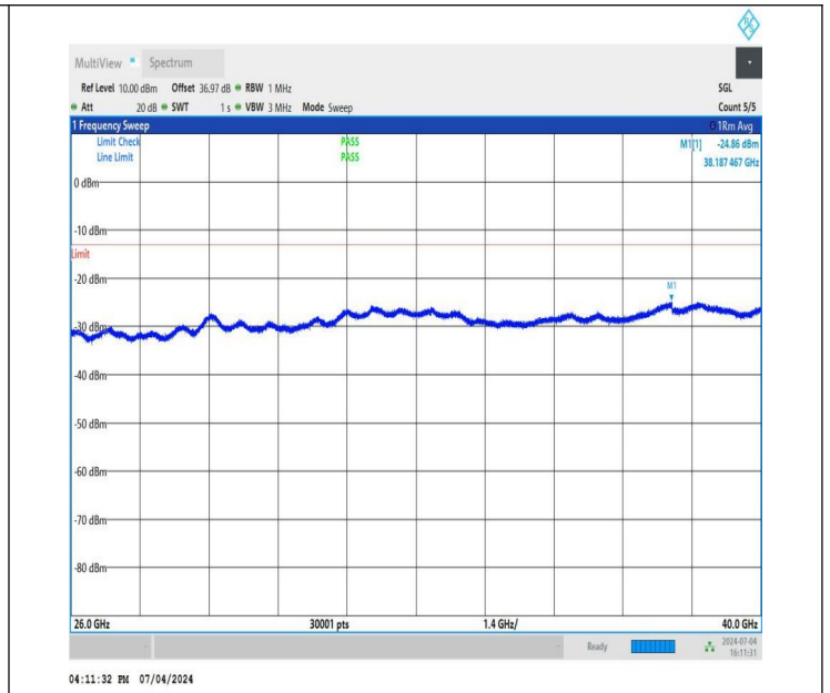
NTNV_DC_26A_n78A-3450-3550_PC3_30_5+80_M+L_TID2_NS_01_26000_40000_#1
