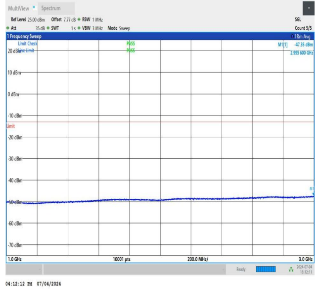
NTNV_DC_26A_n78A-3450-3550_PC3_30_5+80_M+L_TID4_NS_01_1000_3000_#1
