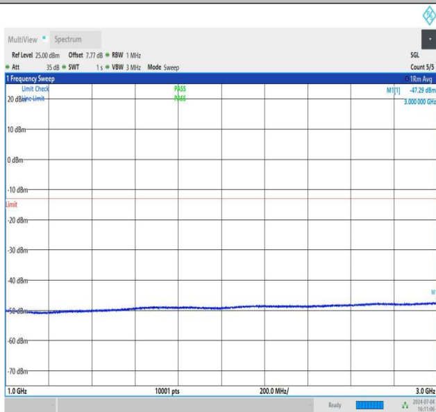
NTNV_DC_26A_n78A-3450-3550_PC3_30_5+80_M+L_TID2_NS _01_0.15_30_#1
