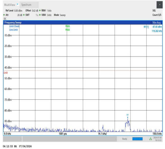
NTNV_DC_26A_n78A-3450-3550_PC3_30_5+80_M+L_TID5_NS_01_0.009_0.15_#1
