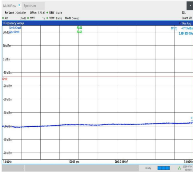
NTNV_DC_26A_n78A-3450-3550_PC3_30_5+70_M+H_TID5_N S_01_1000_3000_#1
