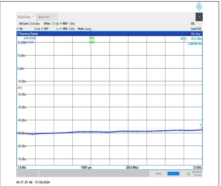
NTNV_DC_26A_n78A-3450-3550_PC3_30_5+70_M+H_TID4_N S_01_1000_3000_#1
