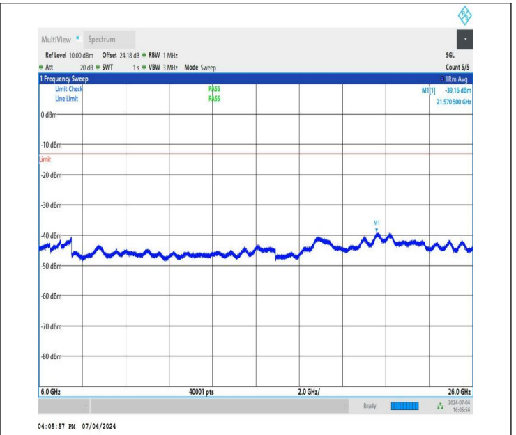
NTNV_DC_26A_n78A-3450-3550_PC3_30_5+70_M+H_TID1_N S_01_6000_26000_#1
