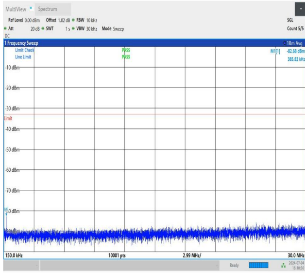
NTNV_DC_26A_n78A-3450-3550_PC3_30_5+80_M+L_TID2_NS _01_0.15_30_#1
