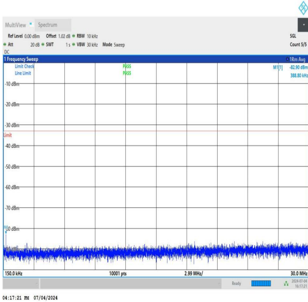
NTNV_DC_26A_n78A-3450-3550_PC3_30_5+80_M+M_TID5_N S_01_0.15_30_#1
