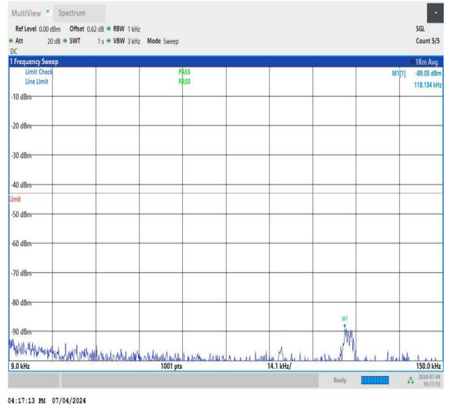
NTNV_DC_26A_n78A-3450-3550_PC3_30_5+80_M+M_TID5_N S_01_0.009_0.15_#1
