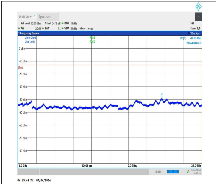
NTNV_DC_26A_n78A-3450-3550_PC3_30_5+80_M+M_TID2_N S_01_6000_26000_#1
