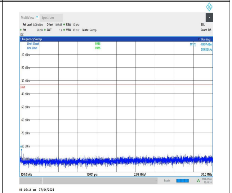
NTNV_DC_26A_n78A-3450-3550_PC3_30_5+80_M+M_TID4_N S_01_0.15_30_#1
