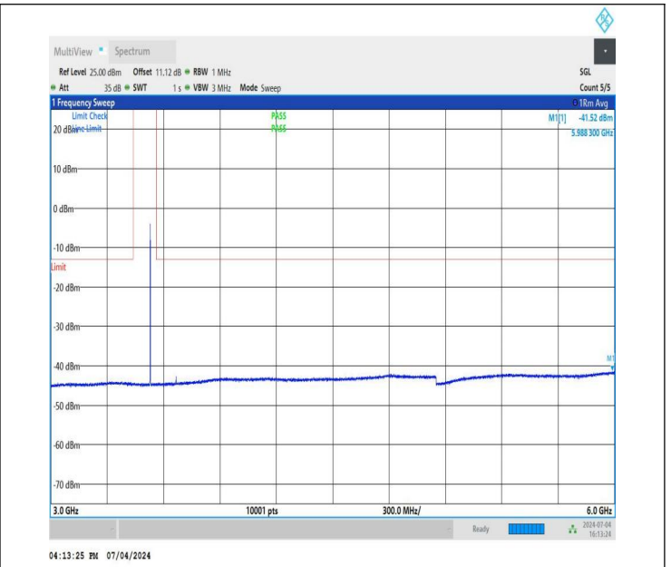
NTNV_DC_26A_n78A-3450-3550_PC3_30_5+80_M+L_TID5_NS_01_3000_6000_#1
