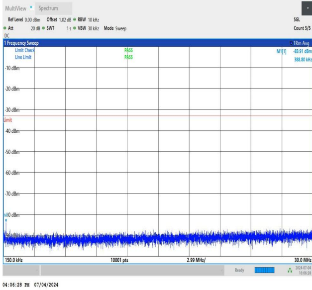
NTNV_DC_26A_n78A-3450-3550_PC3_30_5+70_M+H_TID2_N S_01_0.15_30_#1
