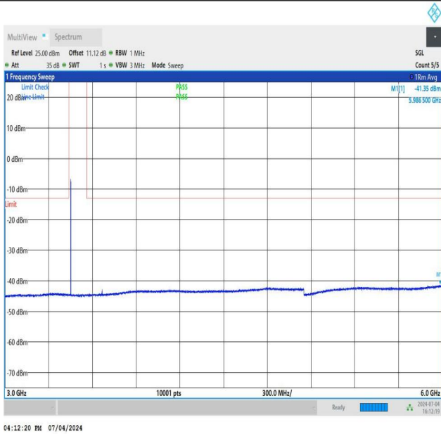
NTNV_DC_26A_n78A-3450-3550_PC3_30_5+80_M+L_TID4_NS_01_3000_6000_#1
