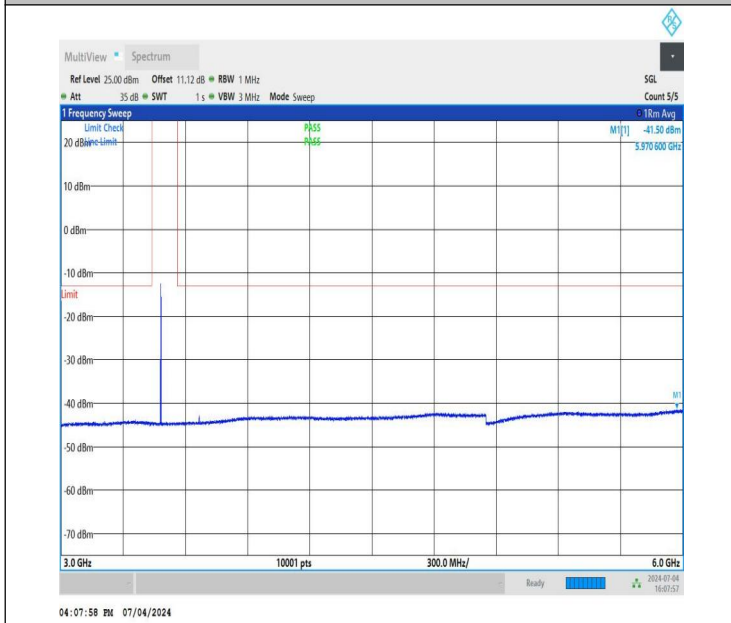
NTNV_DC_26A_n78A-3450-3550_PC3_30_5+70_M+H_TID4_N S_01_3000_6000_#1
