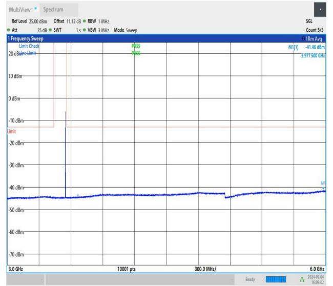
NTNV_DC_26A_n78A-3450-3550_PC3_30_5+70_M+H_TID5_N S_01_3000_6000_#1
