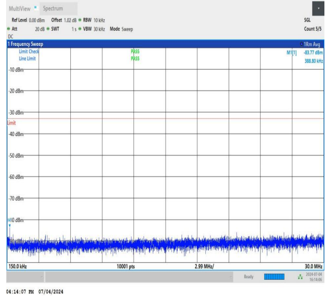
NTNV_DC_26A_n78A-3450-3550_PC3_30_5+80_M+M_TID1_N S_01_0.15_30_#1
