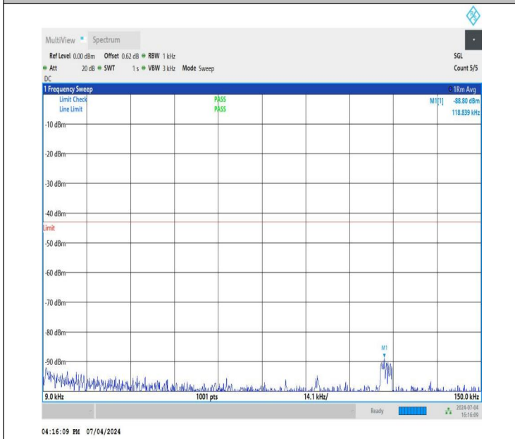
NTNV_DC_26A_n78A-3450-3550_PC3_30_5+80_M+M_TID4_N S_01_0.009_0.15_#1
