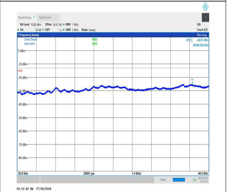
NTNV_DC_26A_n78A-3450-3550_PC3_30_5+80_M+L_TID5_NS_01_26000_40000_#1
