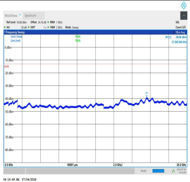
NTNV_DC_26A_n78A-3450-3550_PC3_30_5+80_M+M_TID4_N S_01_6000_26000_#1
