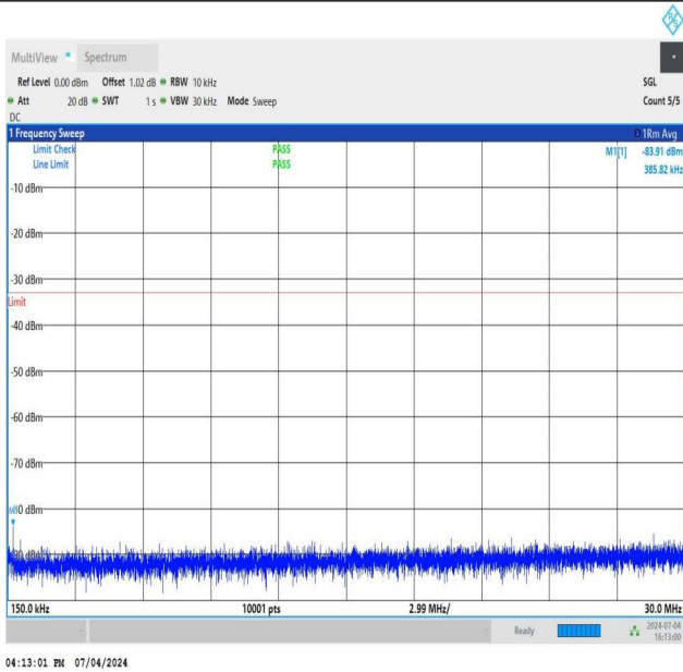
NTNV_DC_26A_n78A-3450-3550_PC3_30_5+80_M+L_TID5_NS_01_0.15_30_#1
