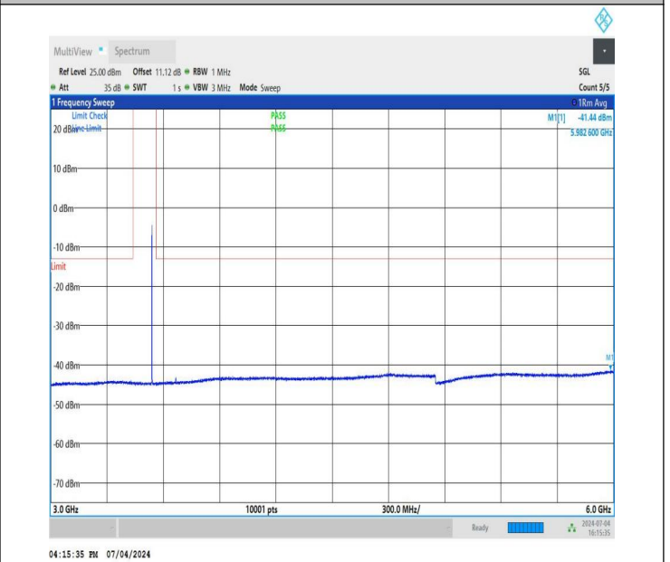
NTNV_DC_26A_n78A-3450-3550_PC3_30_5+80_M+M_TID2_N S_01_3000_6000_#1
