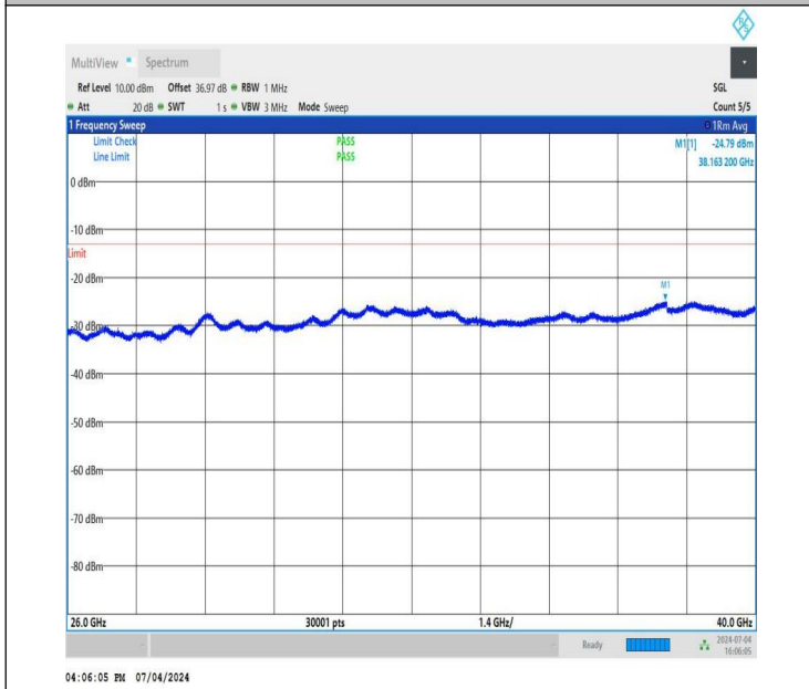
NTNV_DC_26A_n78A-3450-3550_PC3_30_5+70_M+H_TID1_N S_01_26000_40000_#1
