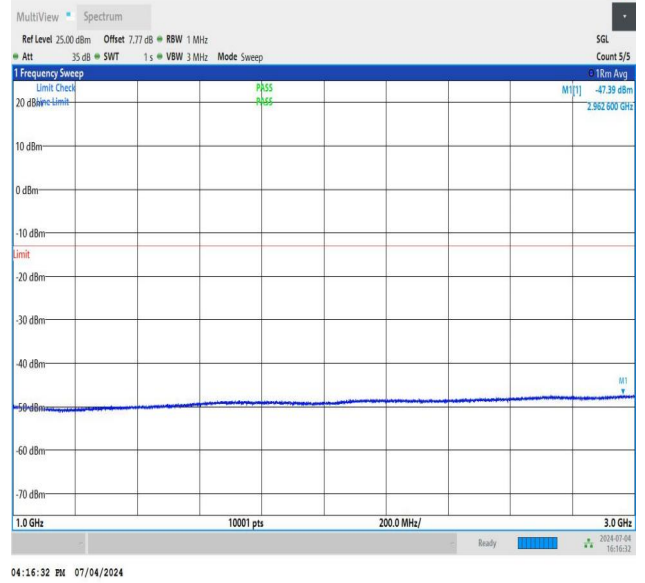
NTNV_DC_26A_n78A-3450-3550_PC3_30_5+80_M+M_TID4_N S_01_1000_3000_#1
