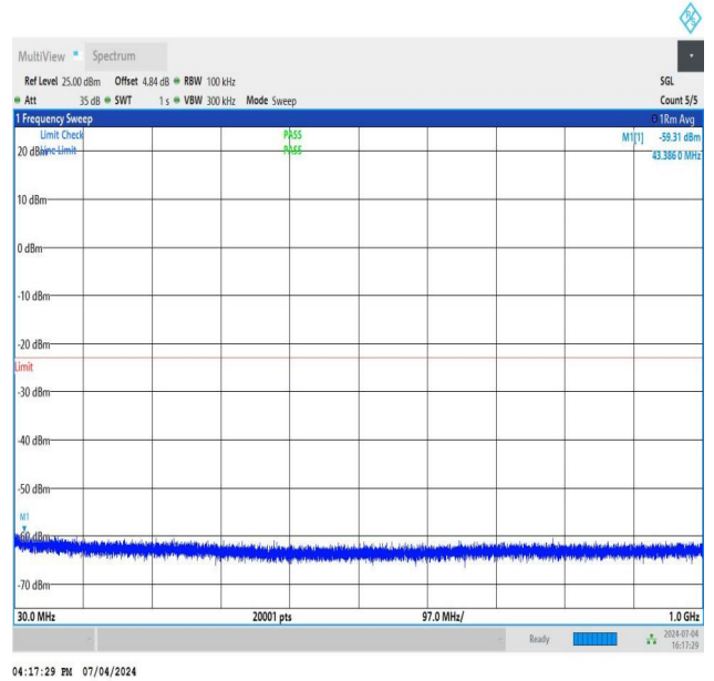
NTNV_DC_26A_n78A-3450-3550_PC3_30_5+80_M+M_TID5_N S_01_30_1000_#1
