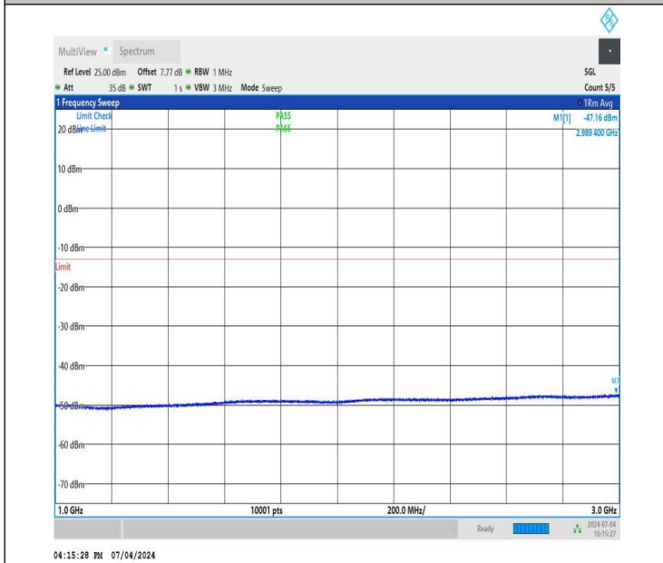
NTNV_DC_26A_n78A-3450-3550_PC3_30_5+80_M+M_TID2_N S_01_1000_3000_#1
