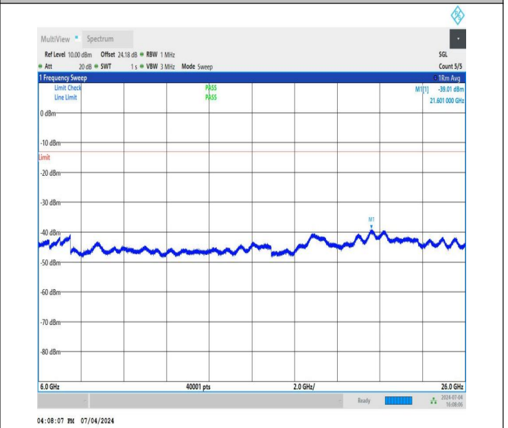
NTNV_DC_26A_n78A-3450-3550_PC3_30_5+70_M+H_TID4_N S_01_6000_26000_#1
