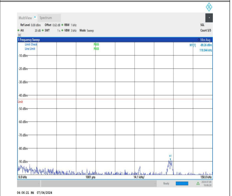
NTNV_DC_26A_n78A-3450-3550_PC3_30_5+70_M+H_TID2_N S_01_0.009_0.15_#1
