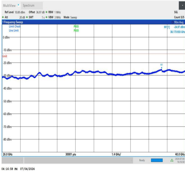
NTNV_DC_26A_n78A-3450-3550_PC3_30_5+80_M+M_TID4_N S_01_26000_40000_#1
