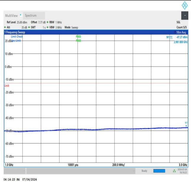
NTNV_DC_26A_n78A-3450-3550_PC3_30_5+80_M+M_TID1_N S_01_1000_3000_#1
