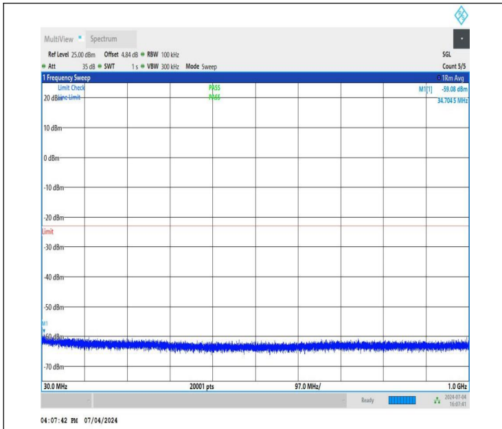
NTNV_DC_26A_n78A-3450-3550_PC3_30_5+70_M+H_TID4_N S_01_30_1000_#1
