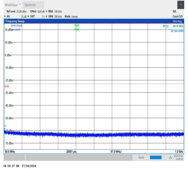
NTNV_DC_26A_n78A-3450-3550_PC3_30_5+70_M+H_TID2_N S_01_30_1000_#1
