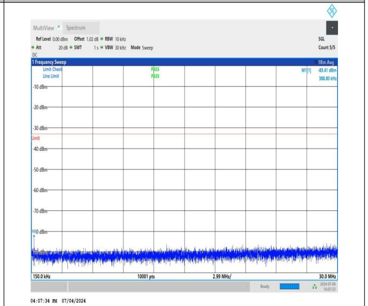
NTNV_DC_26A_n78A-3450-3550_PC3_30_5+70_M+H_TID4_N S_01_0.15_30_#1
