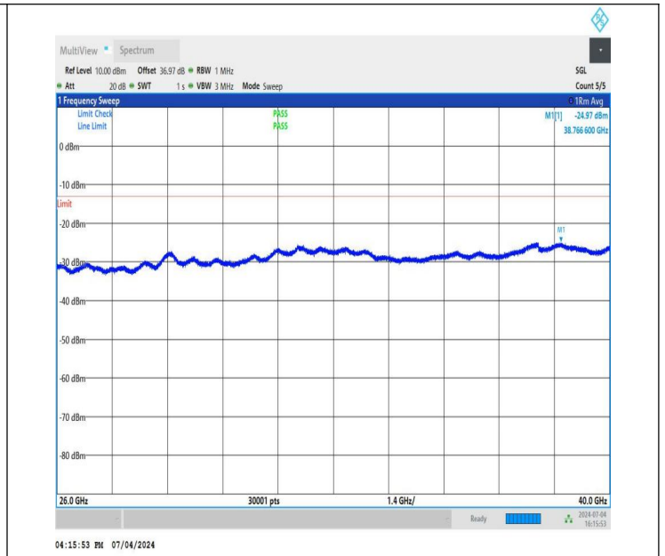
NTNV_DC_26A_n78A-3450-3550_PC3_30_5+80_M+M_TID2_N S_01_26000_40000_#1
