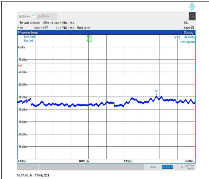
NTNV_DC_26A_n78A-3450-3550_PC3_30_5+70_M+H_TID2_N S_01_6000_26000_#1
