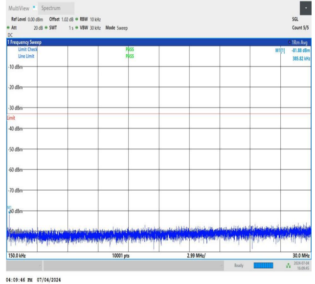
NTNV_DC_26A_n78A-3450-3550_PC3_30_5+80_M+L_TID1_NS_01_0.15_30_#1
