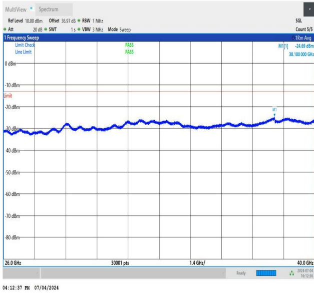
NTNV_DC_26A_n78A-3450-3550_PC3_30_5+80_M+L_TID4_NS_01_26000_40000_#1
