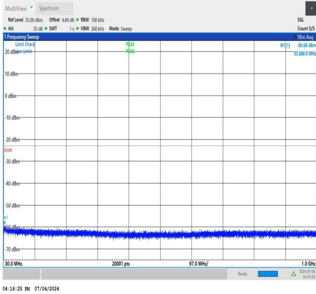
NTNV_DC_26A_n78A-3450-3550_PC3_30_5+80_M+M_TID4_N S_01_30_1000_#1
