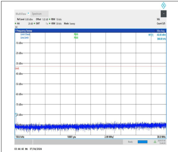
NTNV_DC_26A_n78A-3450-3550_PC3_30_5+60_M+L_TID2_NS_01_0.15_30_#1
