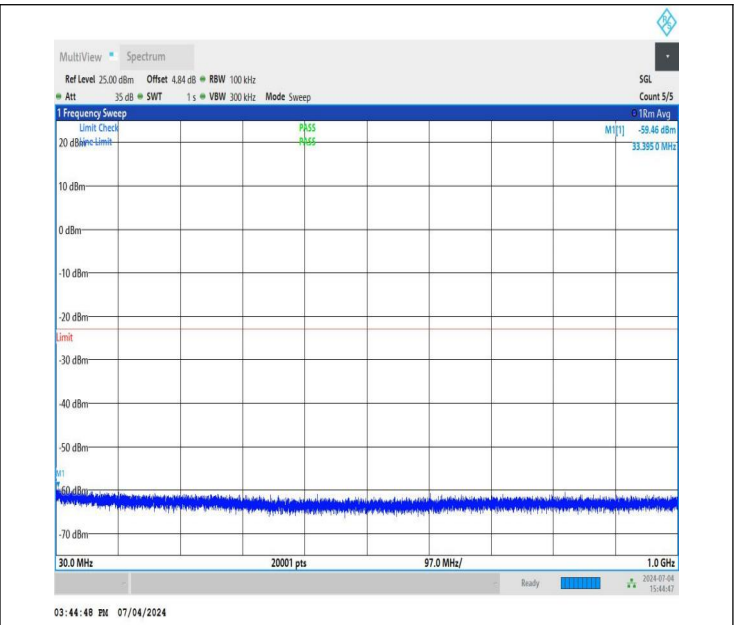
NTNV_DC_26A_n78A-3450-3550_PC3_30_5+60_M+L_TID2_NS_01_30_1000_#1
