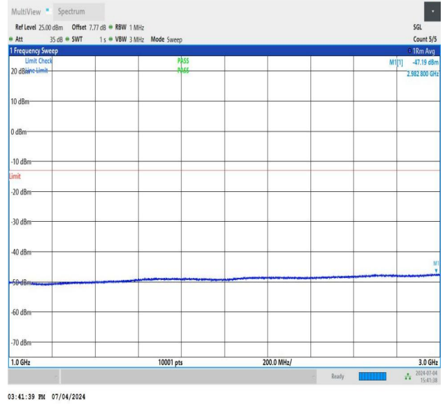
NTNV_DC_26A_n78A-3450-3550_PC3_30_5+50_M+H_TID4_N S_01_1000_3000_#1
