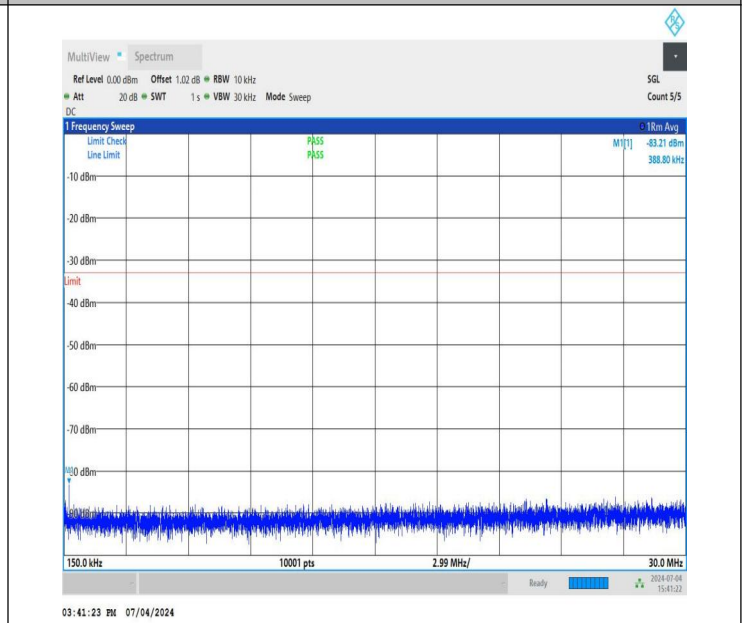
NTNV_DC_26A_n78A-3450-3550_PC3_30_5+50_M+H_TID4_N S_01_0.15_30_#1
