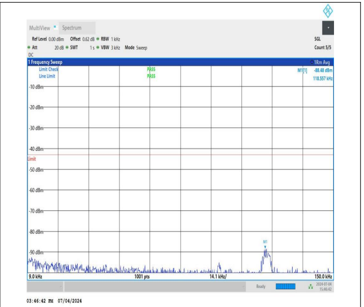
NTNV_DC_26A_n78A-3450-3550_PC3_30_5+60_M+L_TID5_NS_01_0.009_0.15_#1
