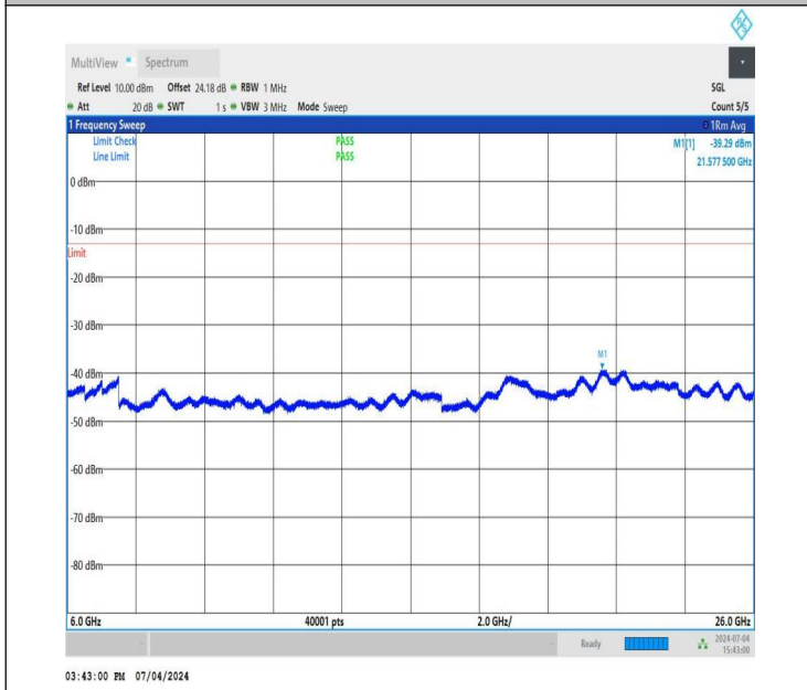
NTNV_DC_26A_n78A-3450-3550_PC3_30_5+50_M+H_TID5_N S_01_6000_26000_#1
