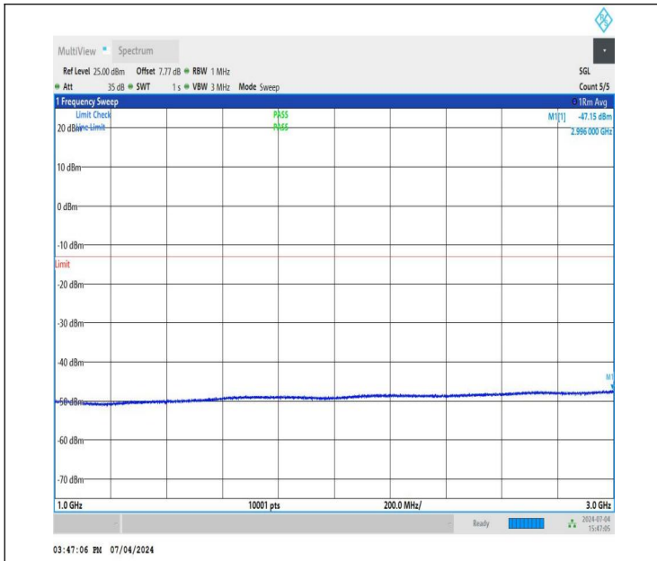
NTNV_DC_26A_n78A-3450-3550_PC3_30_5+60_M+L_TID5_NS_01_1000_3000_#1
