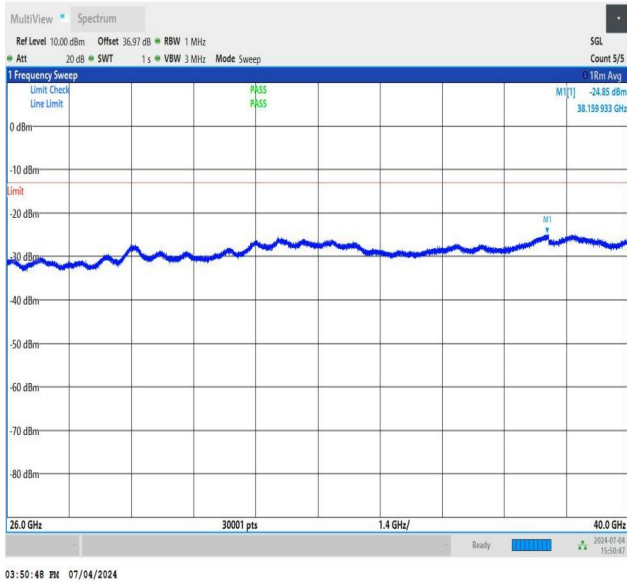
NTNV_DC_26A_n78A-3450-3550_PC3_30_5+60_M+M_TID4_N S_01_26000_40000_#1
