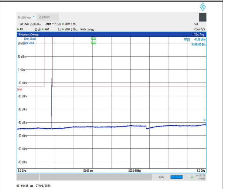
NTNV_DC_26A_n78A-3450-3550_PC3_30_5+50_M+H_TID2_N S_01_3000_6000_#1
