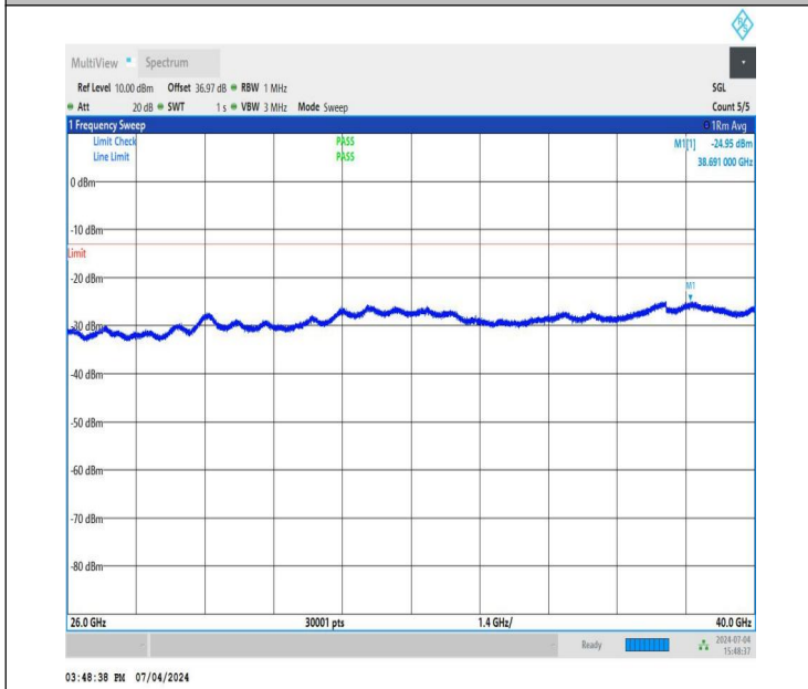
NTNV_DC_26A_n78A-3450-3550_PC3_30_5+60_M+M_TID1_N S_01_26000_40000_#1
