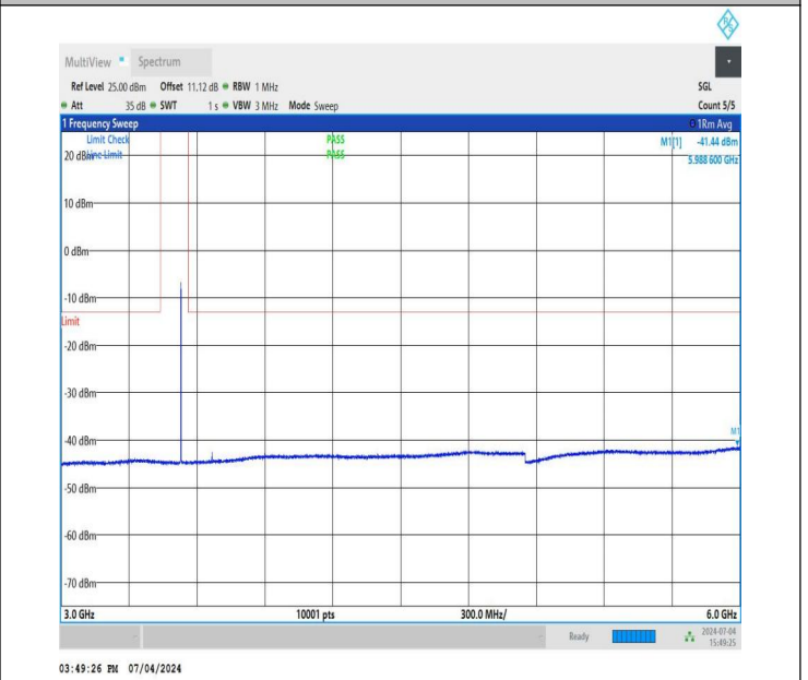
NTNV_DC_26A_n78A-3450-3550_PC3_30_5+60_M+M_TID2_N S_01_3000_6000_#1
