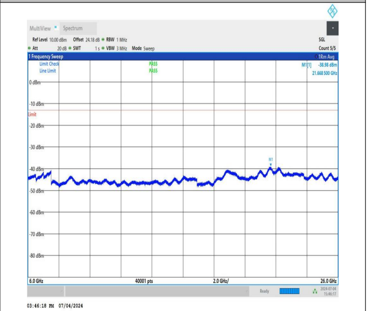
NTNV_DC_26A_n78A-3450-3550_PC3_30_5+60_M+L_TID4_NS_01_6000_26000_#1
