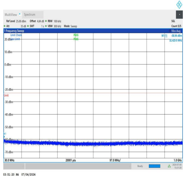
NTNV_DC_26A_n78A-3450-3550_PC3_30_5+60_M+M_TID5_N S_01_30_1000_#1
