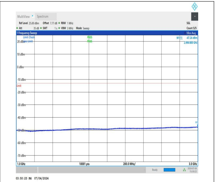
NTNV_DC_26A_n78A-3450-3550_PC3_30_5+60_M+M_TID4_N S_01_1000_3000_#1
