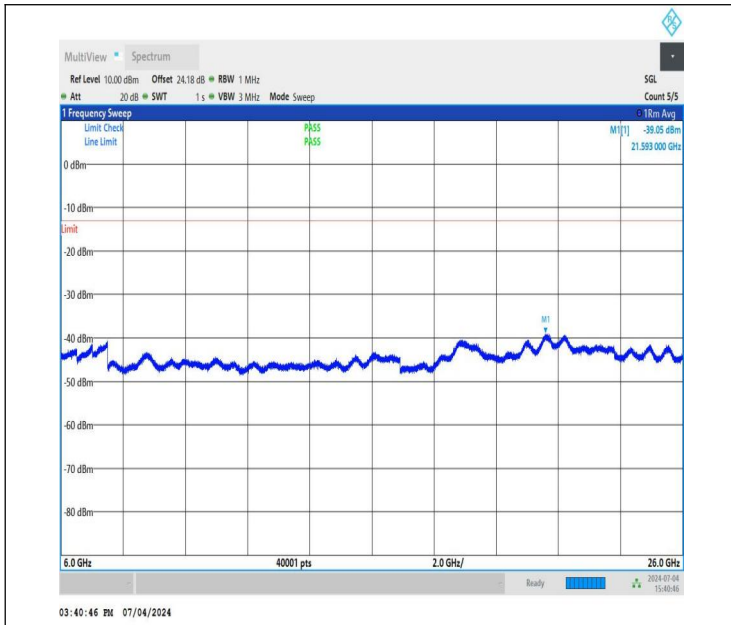
NTNV_DC_26A_n78A-3450-3550_PC3_30_5+50_M+H_TID2_N S_01_6000_26000_#1
