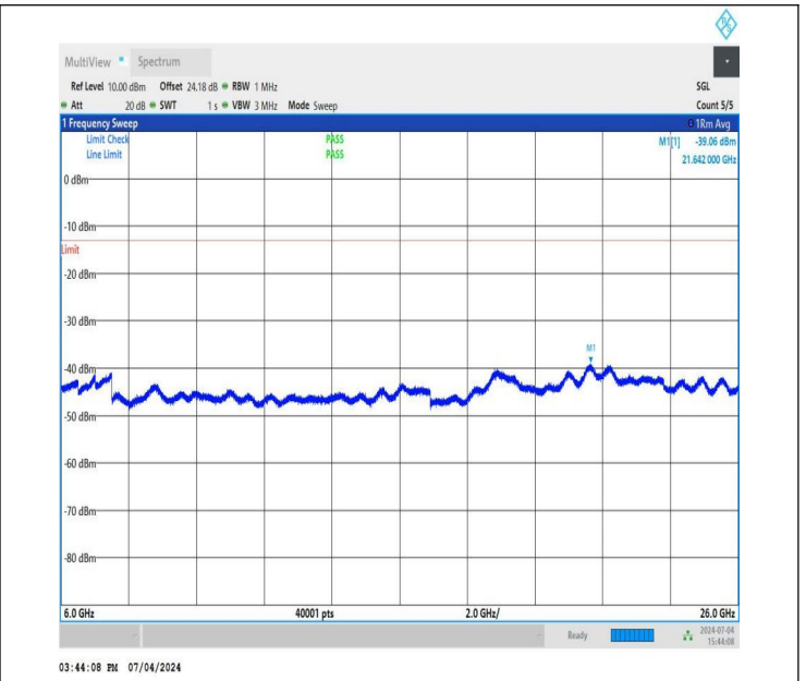
NTNV_DC_26A_n78A-3450-3550_PC3_30_5+60_M+L_TID1_NS_01_6000_26000_#1
