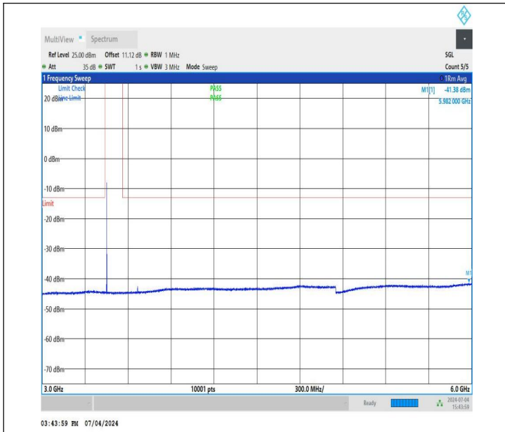
NTNV_DC_26A_n78A-3450-3550_PC3_30_5+60_M+L_TID1_NS_01_3000_6000_#1
