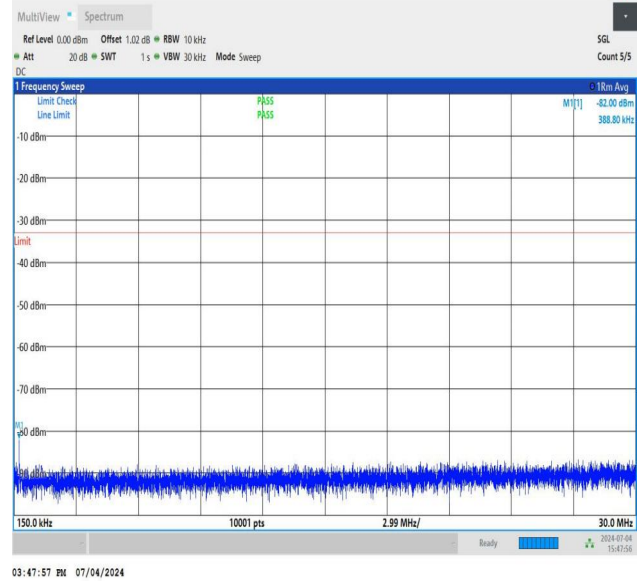
NTNV_DC_26A_n78A-3450-3550_PC3_30_5+60_M+M_TID1_N S_01_0.15_30_#1
