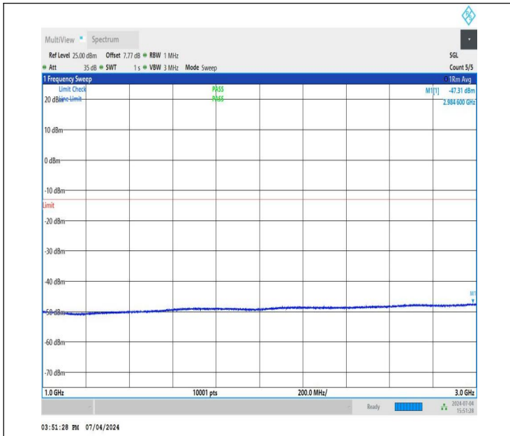
NTNV_DC_26A_n78A-3450-3550_PC3_30_5+60_M+M_TID5_N S_01_1000_3000_#1
