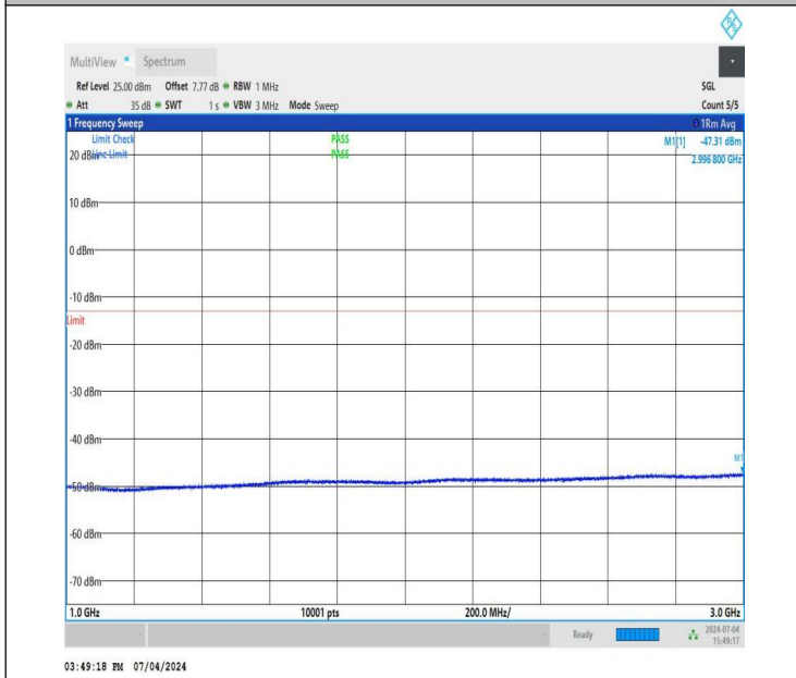
NTNV_DC_26A_n78A-3450-3550_PC3_30_5+60_M+M_TID2_N S_01_1000_3000_#1
