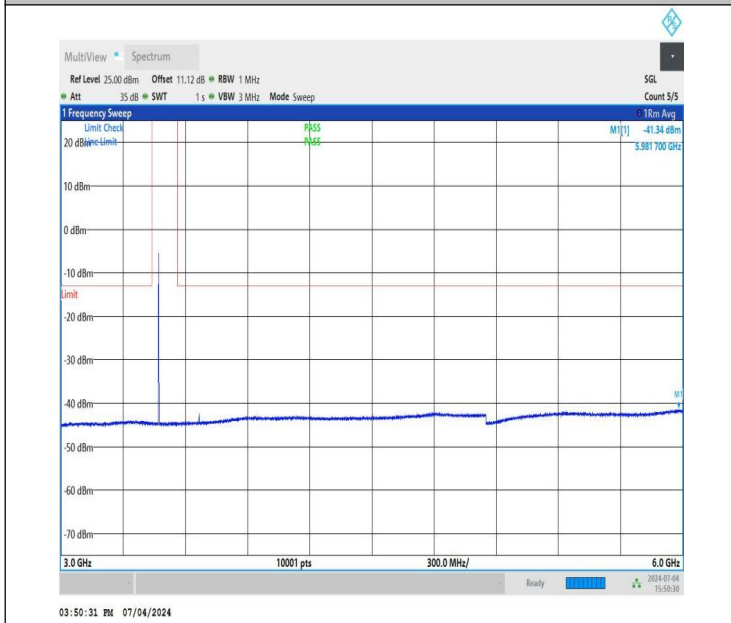
NTNV_DC_26A_n78A-3450-3550_PC3_30_5+60_M+M_TID4_N S_01_3000_6000_#1
