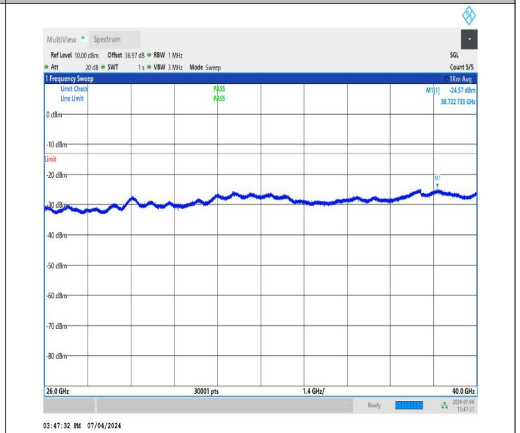
NTNV_DC_26A_n78A-3450-3550_PC3_30_5+60_M+L_TID5_NS_01_26000_40000_#1
