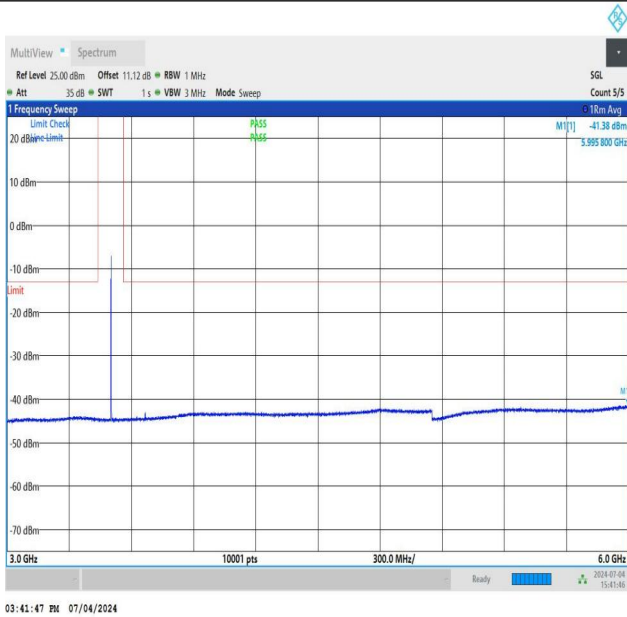
NTNV_DC_26A_n78A-3450-3550_PC3_30_5+50_M+H_TID4_N S_01_3000_6000_#1
