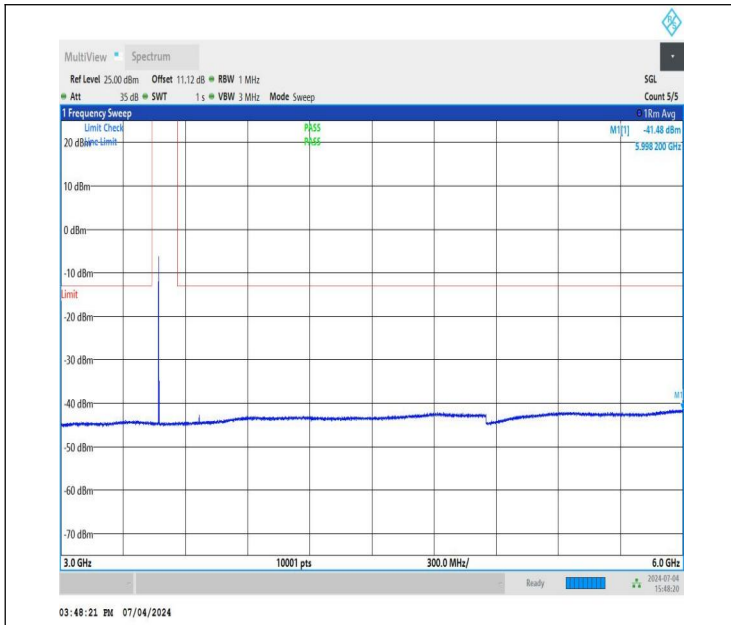
NTNV_DC_26A_n78A-3450-3550_PC3_30_5+60_M+M_TID1_N S_01_3000_6000_#1
