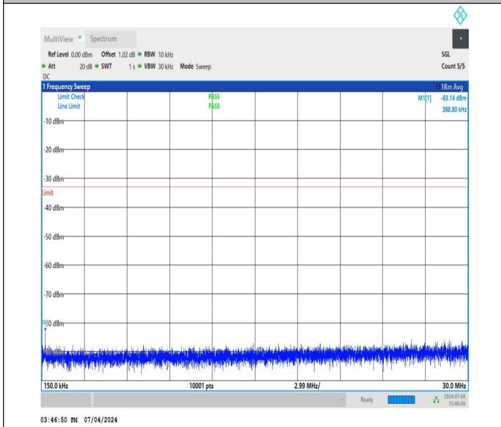
NTNV_DC_26A_n78A-3450-3550_PC3_30_5+60_M+L_TID5_NS_01_0.15_30_#1
