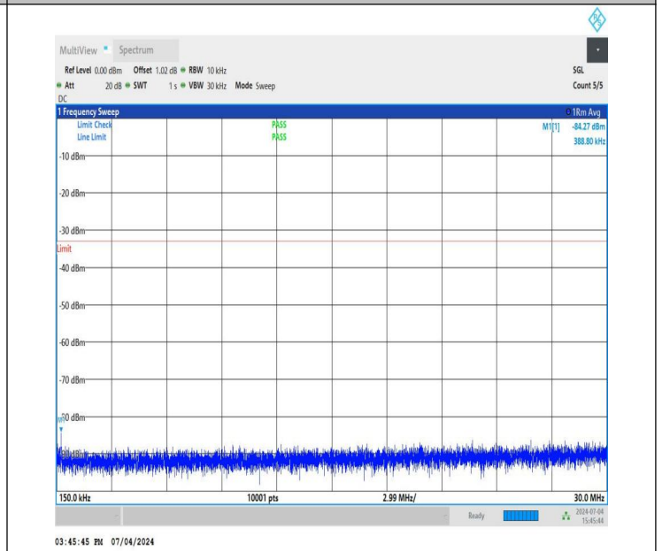
NTNV_DC_26A_n78A-3450-3550_PC3_30_5+60_M+L_TID4_NS_01_0.15_30_#1
