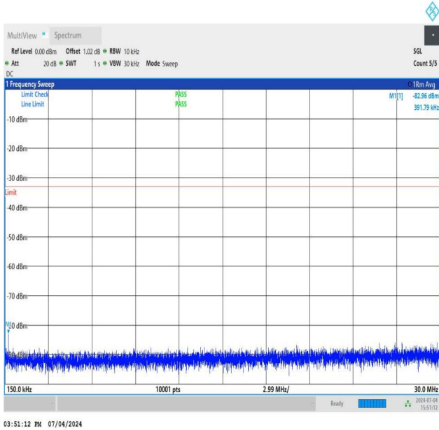
NTNV_DC_26A_n78A-3450-3550_PC3_30_5+60_M+M_TID5_N S_01_0.15_30_#1
