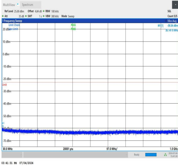
NTNV_DC_26A_n78A-3450-3550_PC3_30_5+50_M+H_TID4_N S_01_30_1000_#1
