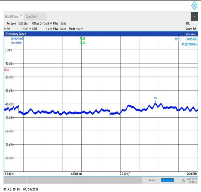
NTNV_DC_26A_n78A-3450-3550_PC3_30_5+50_M+H_TID4_N S_01_6000_26000_#1
