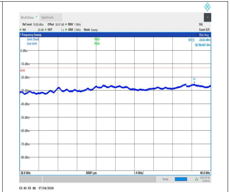
NTNV_DC_26A_n78A-3450-3550_PC3_30_5+50_M+H_TID2_N S_01_26000_40000_#1
