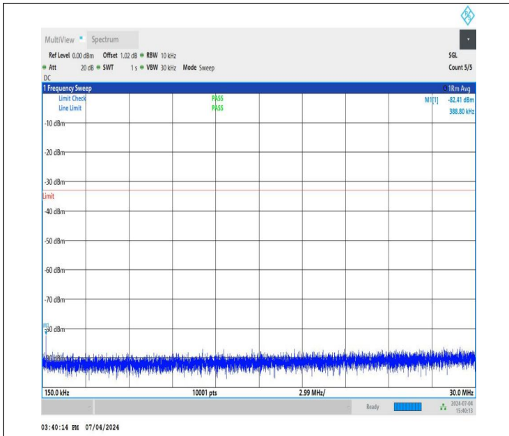
NTNV_DC_26A_n78A-3450-3550_PC3_30_5+50_M+H_TID2_N S_01_0.15_30_#1
