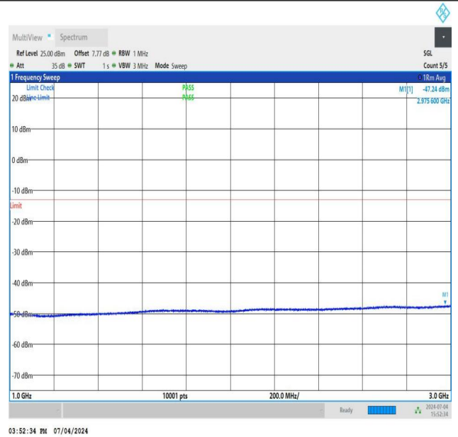
NTNV_DC_26A_n78A-3450-3550_PC3_30_5+60_M+H_TID1_N S_01_1000_3000_#1
