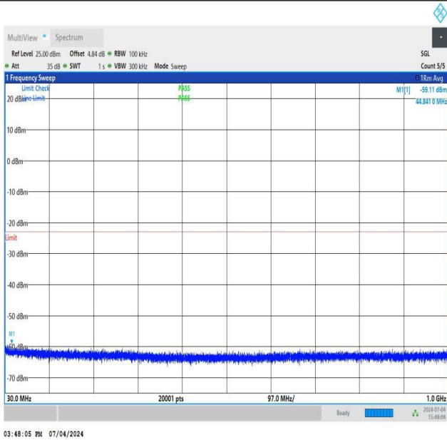
NTNV_DC_26A_n78A-3450-3550_PC3_30_5+60_M+M_TID1_N S_01_30_1000_#1
