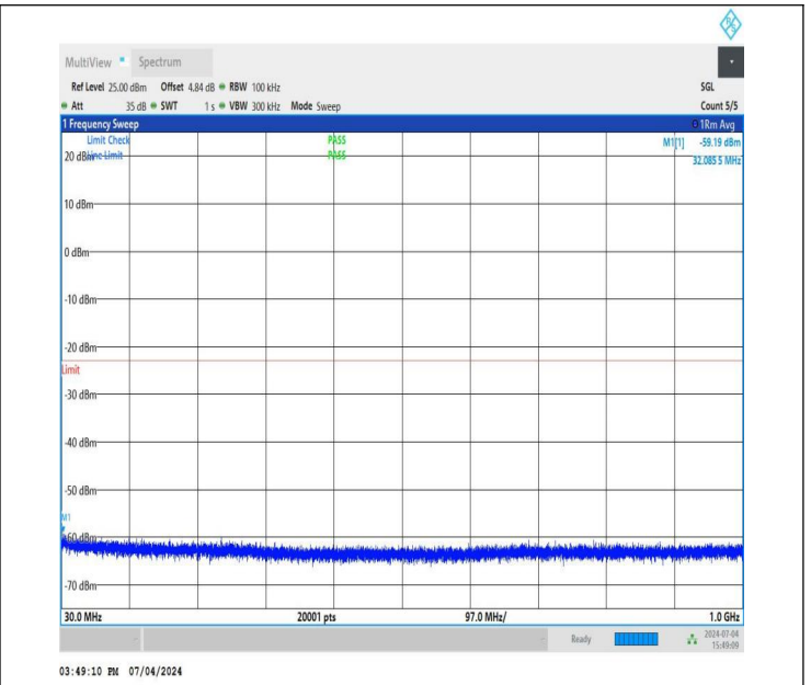
NTNV_DC_26A_n78A-3450-3550_PC3_30_5+60_M+M_TID2_N S_01_30_1000_#1
