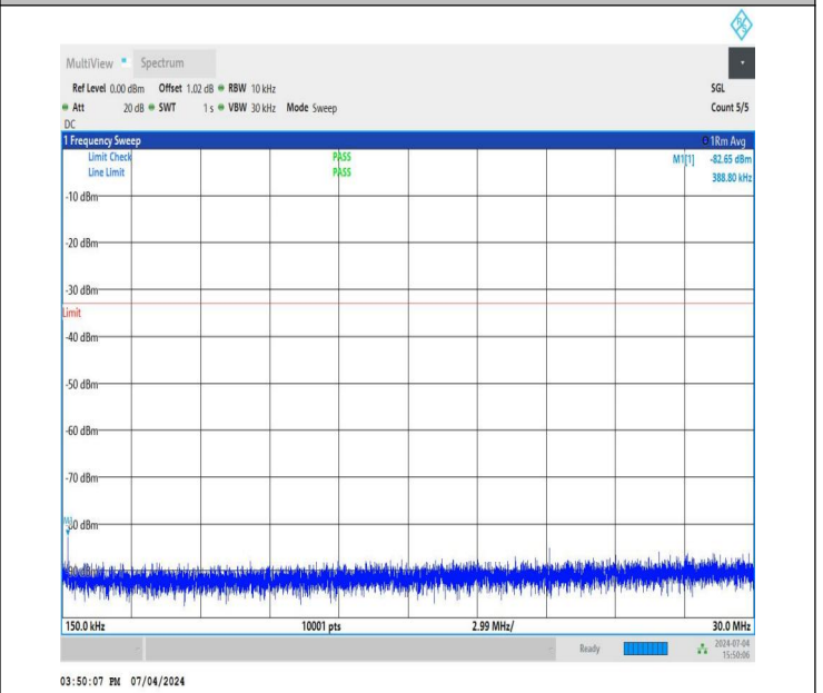
NTNV_DC_26A_n78A-3450-3550_PC3_30_5+60_M+M_TID4_N S_01_0.15_30_#1
