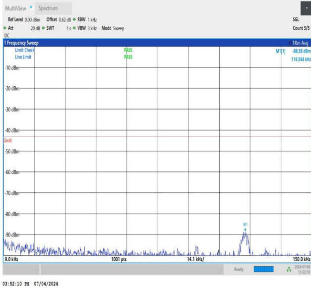
NTNV_DC_26A_n78A-3450-3550_PC3_30_5+60_M+H_TID1_N S_01_0.009_0.15_#1
