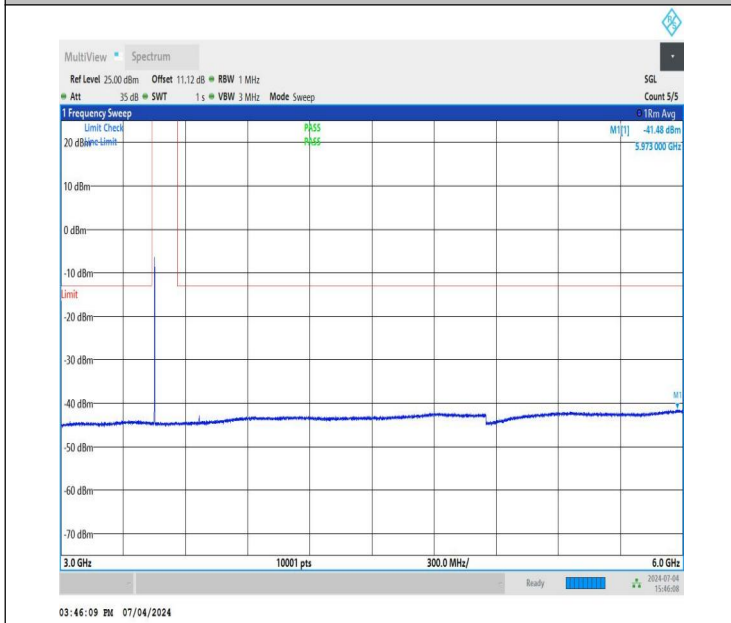
NTNV_DC_26A_n78A-3450-3550_PC3_30_5+60_M+L_TID4_NS_01_3000_6000_#1
