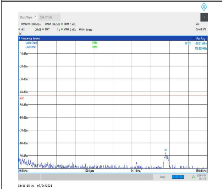
NTNV_DC_26A_n78A-3450-3550_PC3_30_5+50_M+H_TID4_N S_01_0.009_0.15_#1
