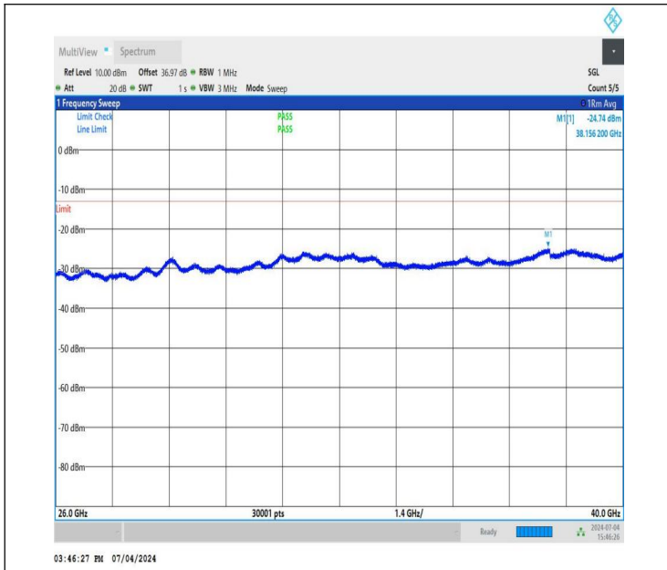
NTNV_DC_26A_n78A-3450-3550_PC3_30_5+60_M+L_TID4_NS_01_26000_40000_#1
