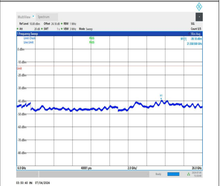
NTNV_DC_26A_n78A-3450-3550_PC3_30_5+60_M+M_TID4_N S_01_6000_26000_#1
