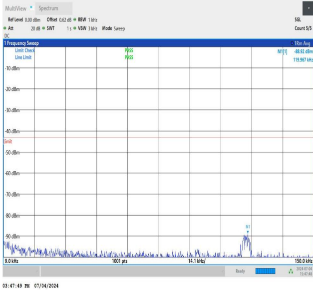
NTNV_DC_26A_n78A-3450-3550_PC3_30_5+60_M+M_TID1_N S_01_0.009_0.15_#1
