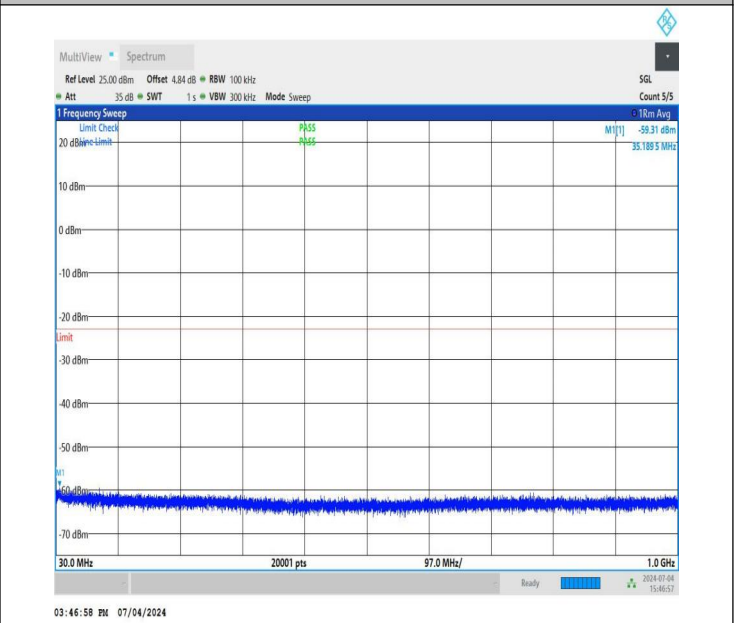
NTNV_DC_26A_n78A-3450-3550_PC3_30_5+60_M+L_TID5_NS_01_30_1000_#1
