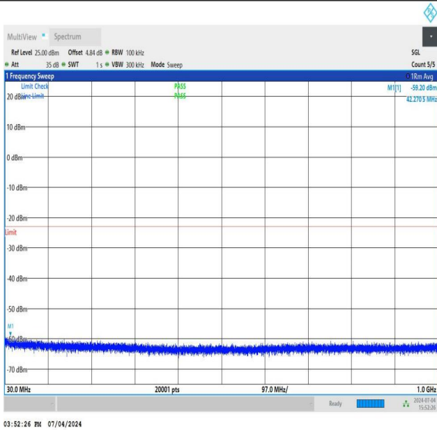
NTNV_DC_26A_n78A-3450-3550_PC3_30_5+60_M+H_TID1_N S_01_30_1000_#1
