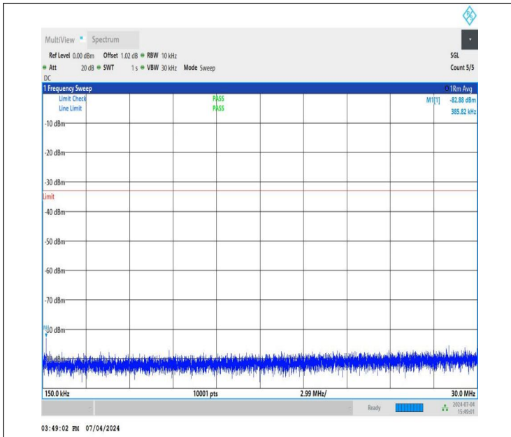
NTNV_DC_26A_n78A-3450-3550_PC3_30_5+60_M+M_TID2_N S_01_0.15_30_#1
