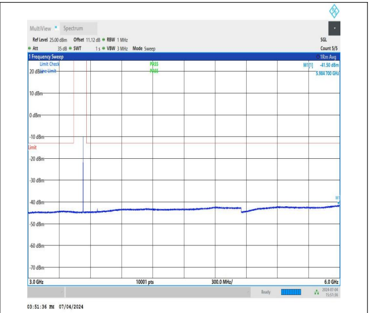
NTNV_DC_26A_n78A-3450-3550_PC3_30_5+60_M+M_TID5_N S_01_3000_6000_#1
