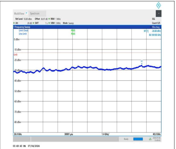
NTNV_DC_26A_n78A-3450-3550_PC3_30_5+60_M+M_TID2_N S_01_26000_40000_#1
