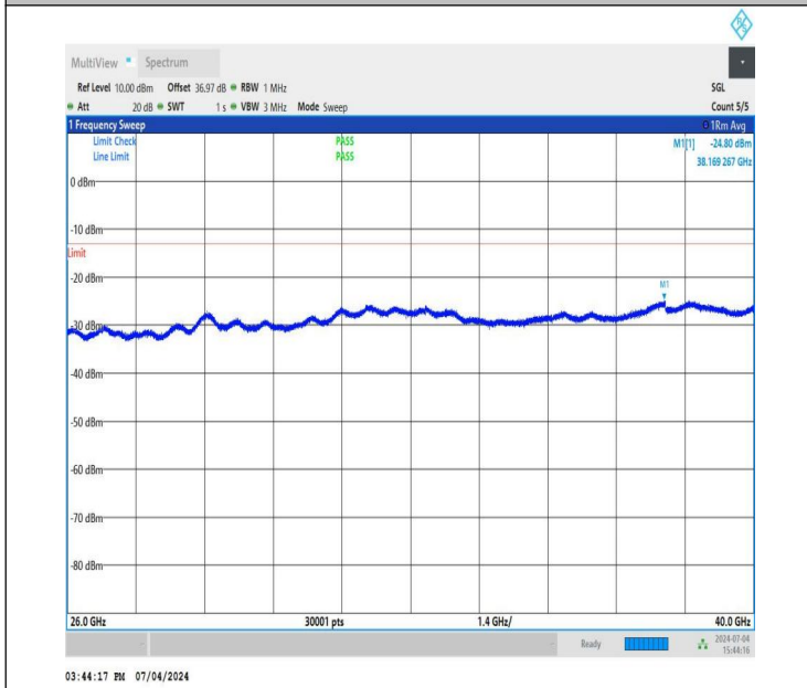
NTNV_DC_26A_n78A-3450-3550_PC3_30_5+60_M+L_TID1_NS_01_26000_40000_#1
