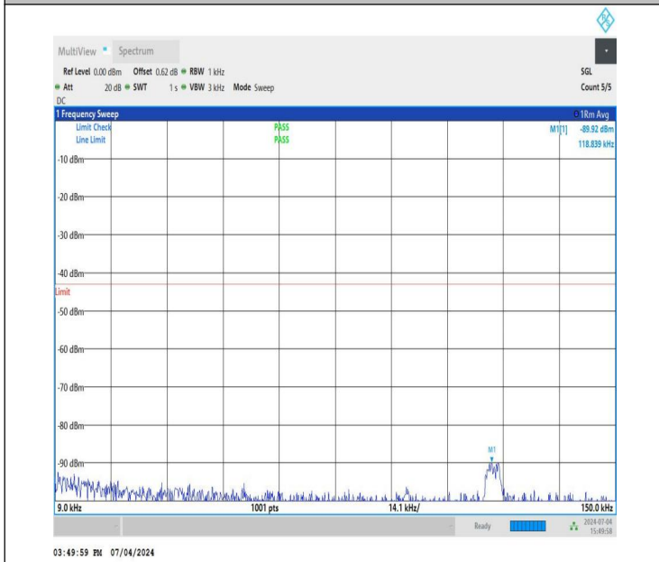
NTNV_DC_26A_n78A-3450-3550_PC3_30_5+60_M+M_TID4_N S_01_0.009_0.15_#1
