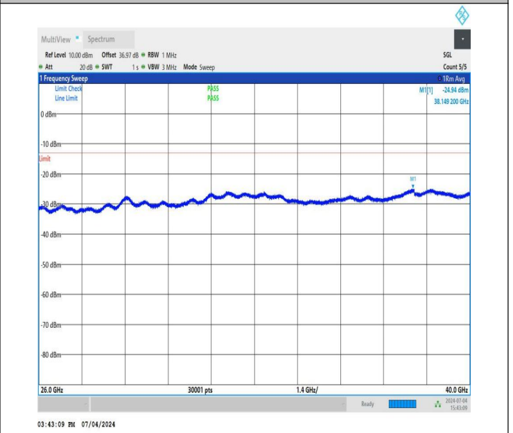
NTNV_DC_26A_n78A-3450-3550_PC3_30_5+50_M+H_TID5_N S_01_26000_40000_#1
