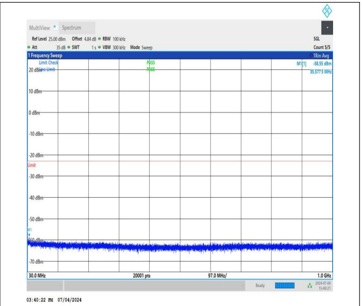
NTNV_DC_26A_n78A-3450-3550_PC3_30_5+50_M+H_TID2_N S_01_30_1000_#1
