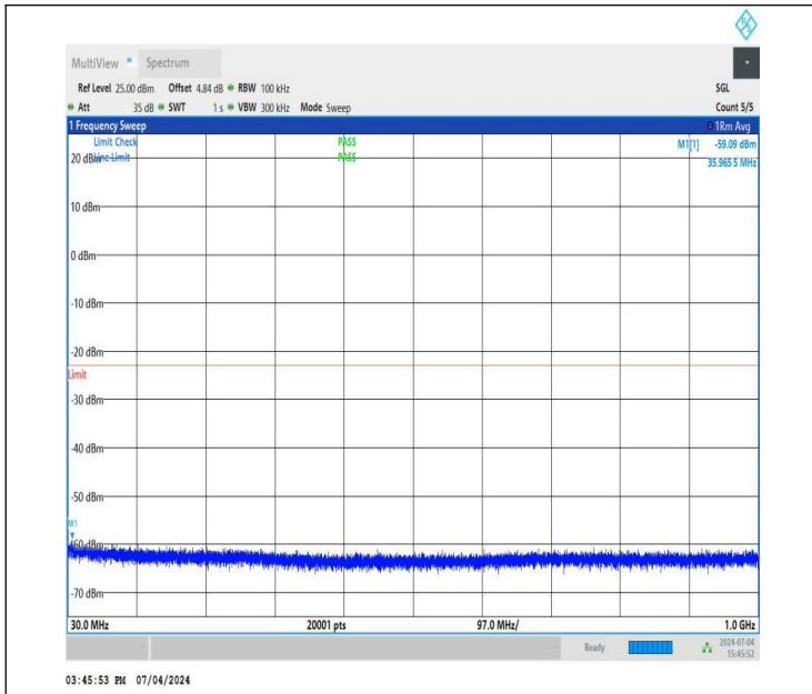
NTNV_DC_26A_n78A-3450-3550_PC3_30_5+60_M+L_TID4_NS_01_30_1000_#1
