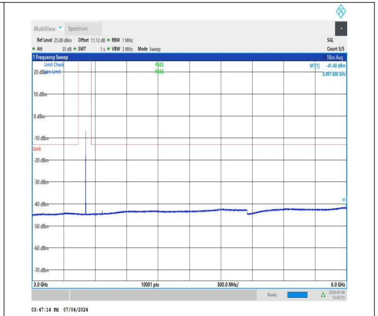
NTNV_DC_26A_n78A-3450-3550_PC3_30_5+60_M+L_TID5_NS_01_3000_6000_#1
