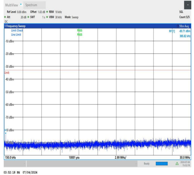
NTNV_DC_26A_n78A-3450-3550_PC3_30_5+60_M+H_TID1_N S_01_0.15_30_#1
