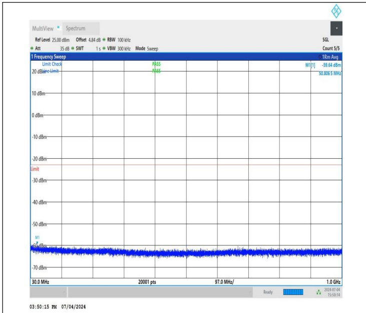
NTNV_DC_26A_n78A-3450-3550_PC3_30_5+60_M+M_TID4_N S_01_30_1000_#1
