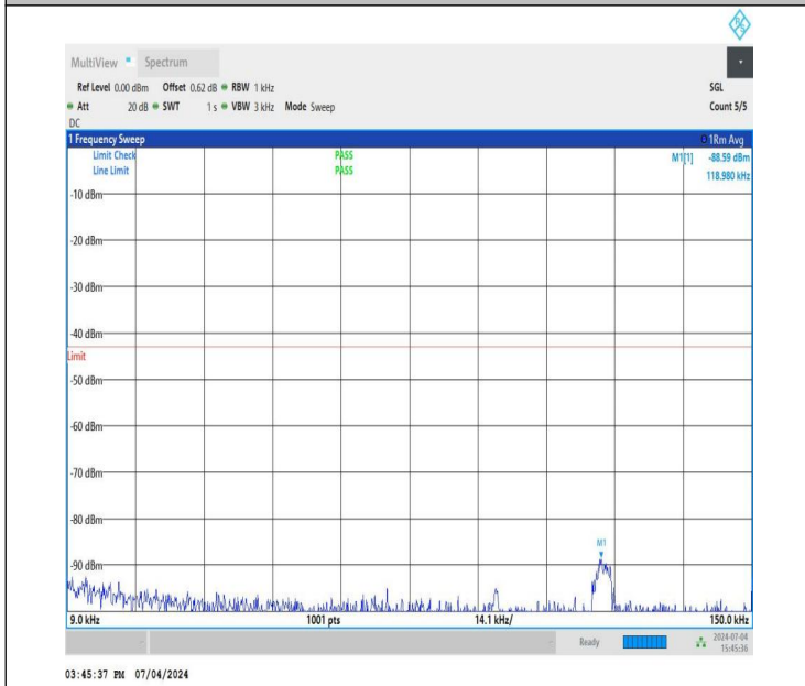
NTNV_DC_26A_n78A-3450-3550_PC3_30_5+60_M+L_TID4_NS_01_0.009_0.15_#1
