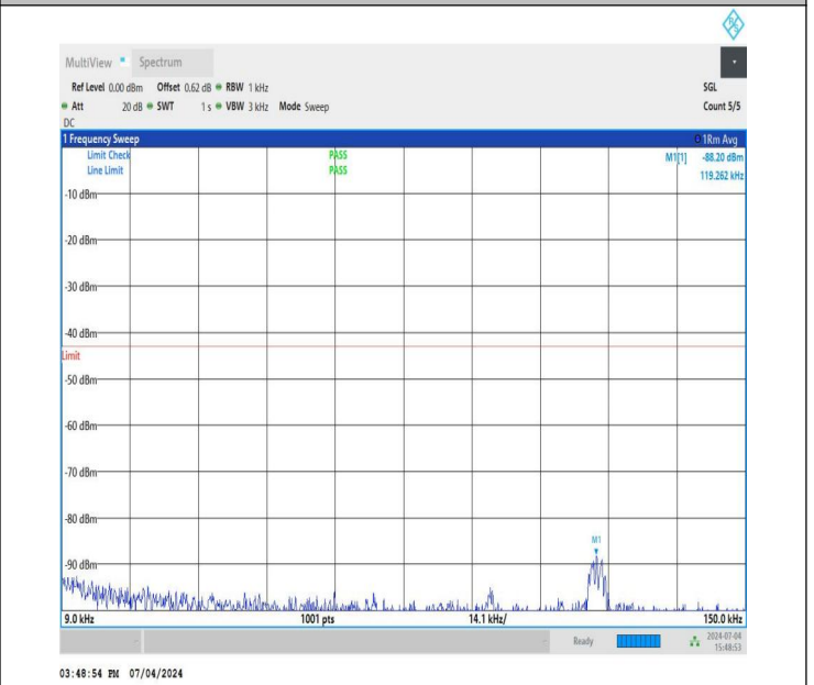
NTNV_DC_26A_n78A-3450-3550_PC3_30_5+60_M+M_TID2_N S_01_0.009_0.15_#1
