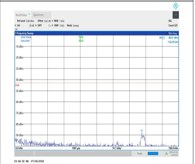
NTNV_DC_26A_n78A-3450-3550_PC3_30_5+60_M+L_TID2_NS_01_0.009_0.15_#1
