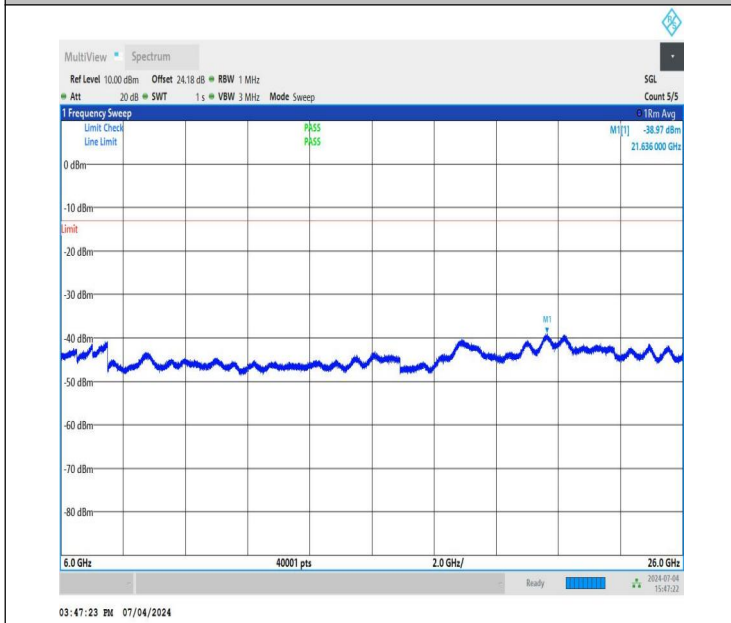
NTNV_DC_26A_n78A-3450-3550_PC3_30_5+60_M+L_TID5_NS_01_6000_26000_#1
