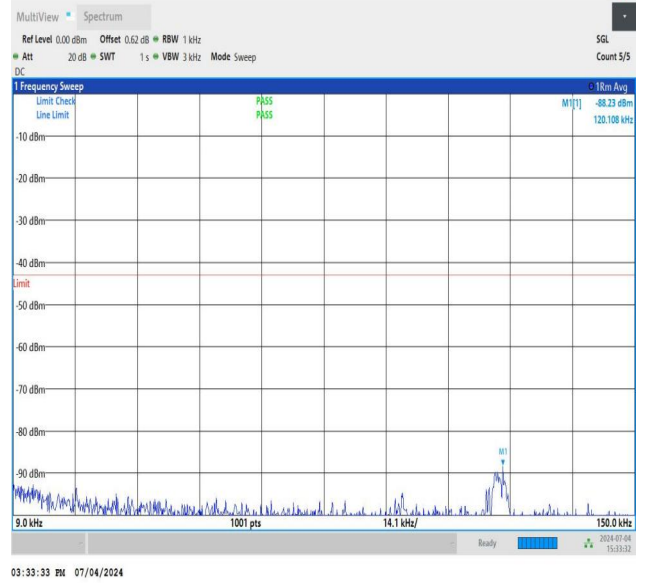
NTNV_DC_26A_n78A-3450-3550_PC3_30_5+50_M+L_TID5_NS_01_0.009_0.15_#1
