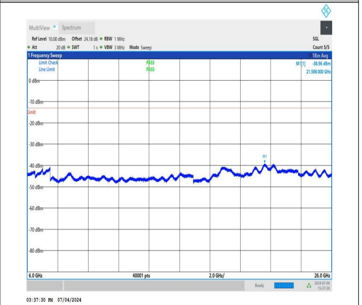
NTNV_DC_26A_n78A-3450-3550_PC3_30_5+50_M+M_TID4_N S_01_6000_26000_#1
