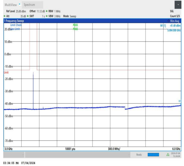
NTNV_DC_26A_n78A-3450-3550_PC3_30_5+50_M+L_TID5_NS_01_3000_6000_#1
