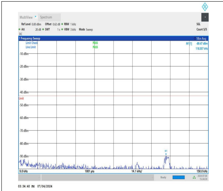
NTNV_DC_26A_n78A-3450-3550_PC3_30_5+50_M+M_TID1_N S_01_0.009_0.15_#1
