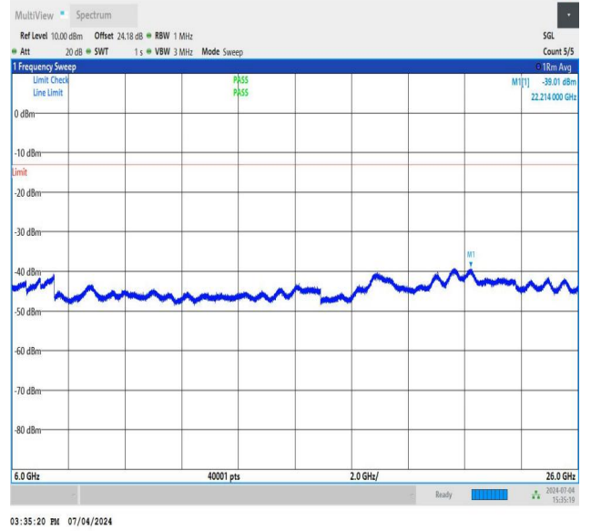
NTNV_DC_26A_n78A-3450-3550_PC3_30_5+50_M+M_TID1_N S_01_6000_26000_#1
