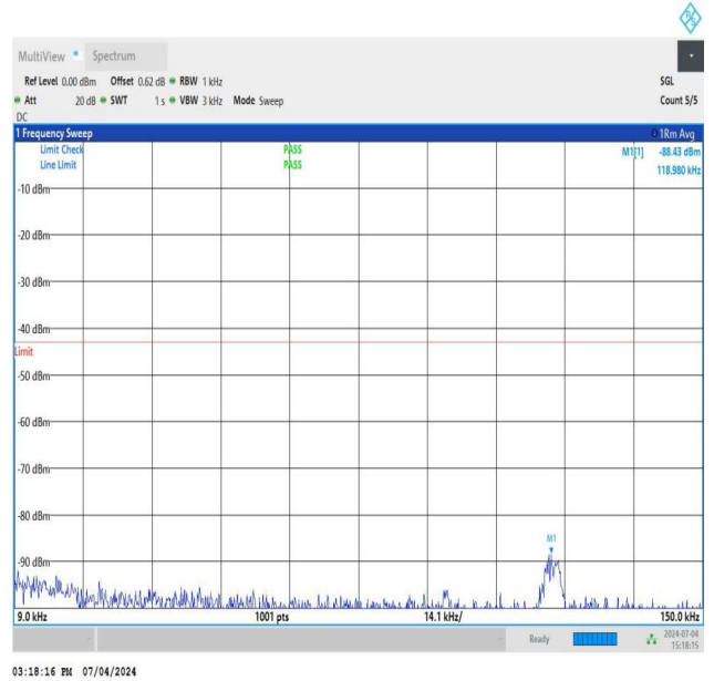
NTNV_DC_26A_n78A-3450-3550_PC3_30_5+40_M+L_TID2_NS_01_0.009_0.15_#1
