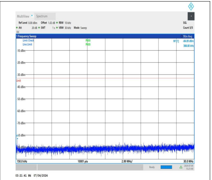
NTNV_DC_26A_n78A-3450-3550_PC3_30_5+40_M+M_TID1_N S_01_0.15_30_#1
