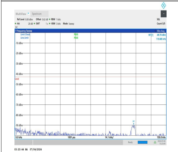
NTNV_DC_26A_n78A-3450-3550_PC3_30_5+40_M+M_TID4_N S_01_0.009_0.15_#1
