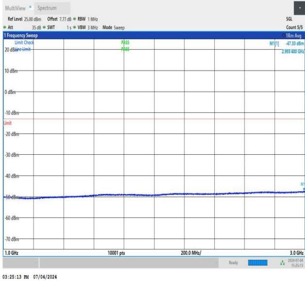
NTNV_DC_26A_n78A-3450-3550_PC3_30_5+40_M+M_TID5_N S_01_1000_3000_#1
