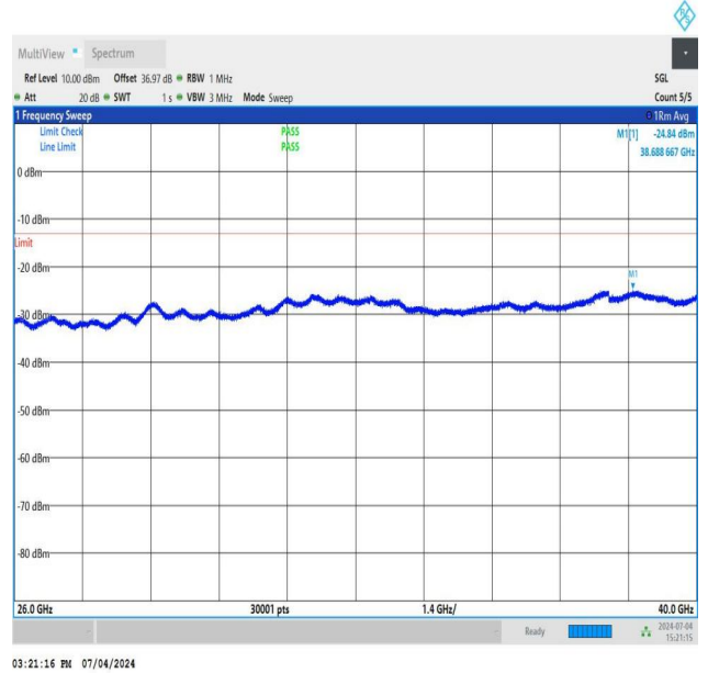
NTNV_DC_26A_n78A-3450-3550_PC3_30_5+40_M+L_TID5_NS_01_26000_40000_#1
