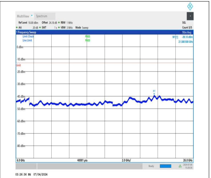
NTNV_DC_26A_n78A-3450-3550_PC3_30_5+40_M+H_TID1_N S_01_6000_26000_#1
