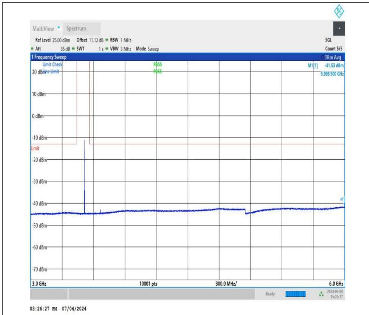
NTNV_DC_26A_n78A-3450-3550_PC3_30_5+40_M+H_TID1_N S_01_3000_6000_#1
