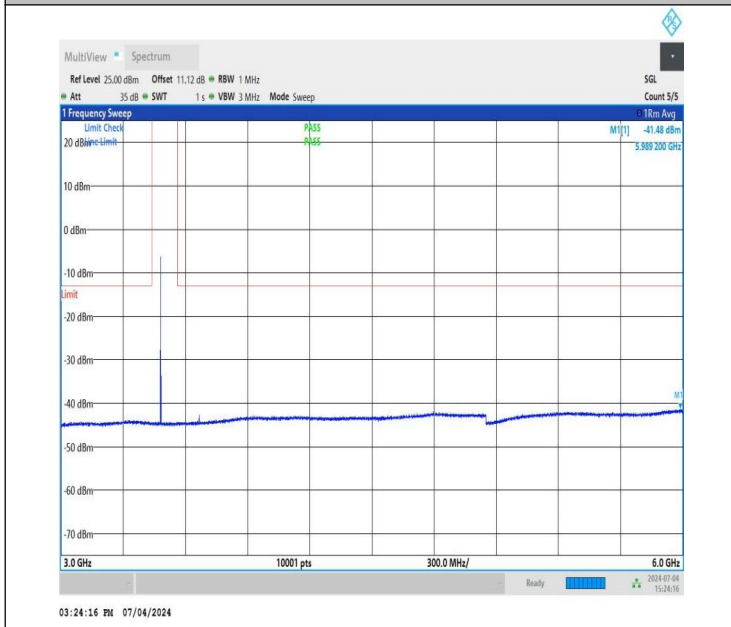
NTNV_DC_26A_n78A-3450-3550_PC3_30_5+40_M+M_TID4_N S_01_3000_6000_#1
