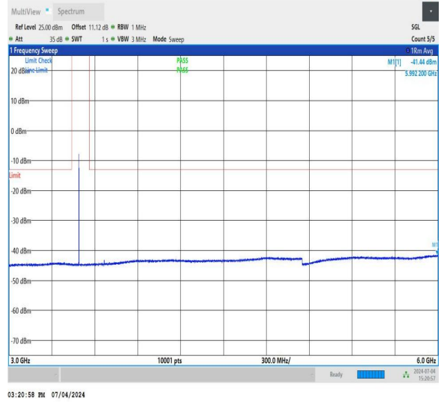
NTNV_DC_26A_n78A-3450-3550_PC3_30_5+40_M+L_TID5_NS_01_3000_6000_#1
