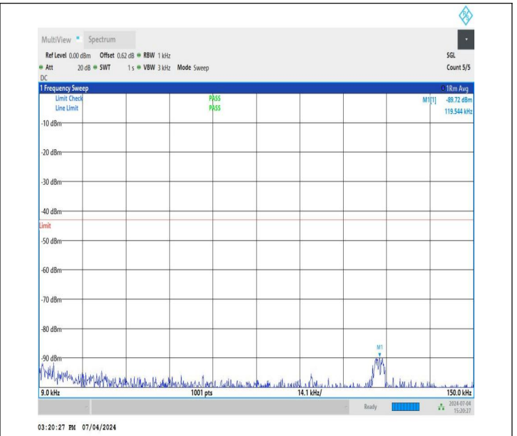
NTNV_DC_26A_n78A-3450-3550_PC3_30_5+40_M+L_TID5_NS_01_0.009_0.15_#1
