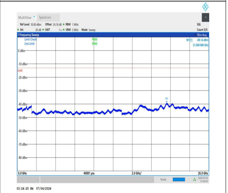
NTNV_DC_26A_n78A-3450-3550_PC3_30_5+40_M+M_TID4_N S_01_6000_26000_#1
