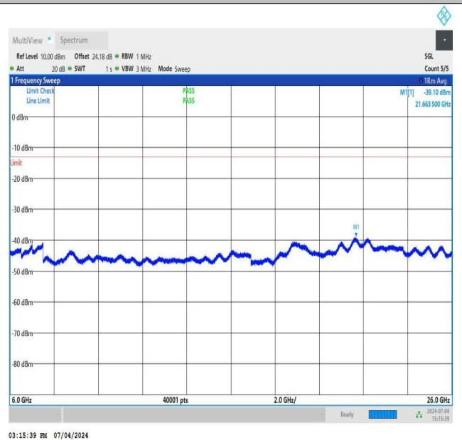
NTNV_DC_26A_n78A-3450-3550_PC3_30_5+30_M+H_TID4_N S_01_6000_26000_#1
