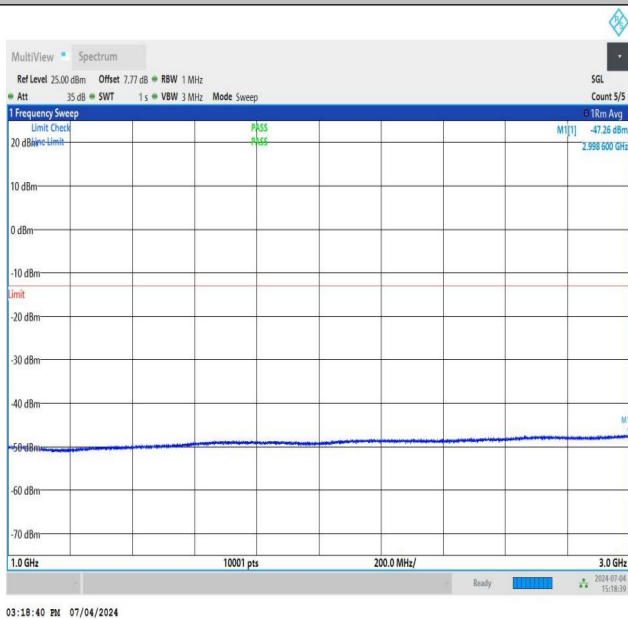
NTNV_DC_26A_n78A-3450-3550_PC3_30_5+40_M+L_TID2_NS _01_1000_3000_#1
