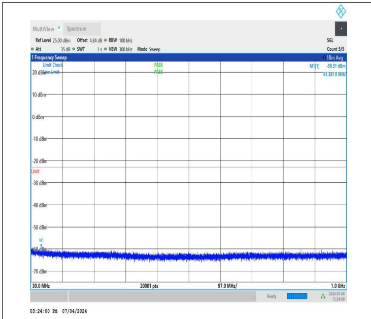
NTNV_DC_26A_n78A-3450-3550_PC3_30_5+40_M+M_TID4_N S_01_30_1000_#1
