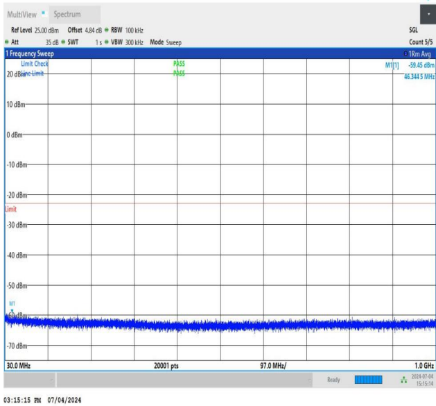
NTNV_DC_26A_n78A-3450-3550_PC3_30_5+30_M+H_TID4_N S_01_30_1000_#1
