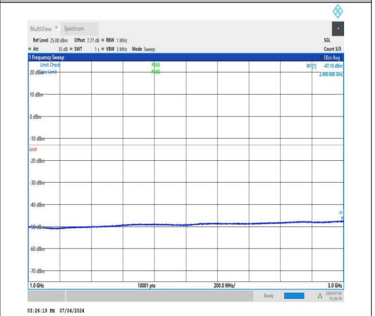
NTNV_DC_26A_n78A-3450-3550_PC3_30_5+40_M+H_TID1_N S_01_1000_3000_#1
