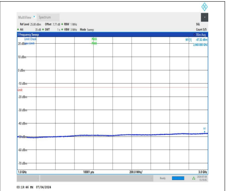
NTNV_DC_26A_n78A-3450-3550_PC3_30_5+40_M+L_TID4_NS_01_1000_3000_#1
