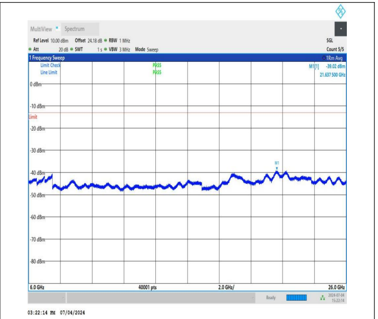
NTNV_DC_26A_n78A-3450-3550_PC3_30_5+40_M+M_TID1_N S_01_6000_26000_#1
