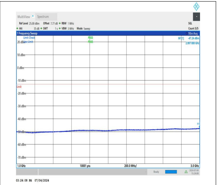
NTNV_DC_26A_n78A-3450-3550_PC3_30_5+40_M+M_TID4_N S_01_1000_3000_#1
