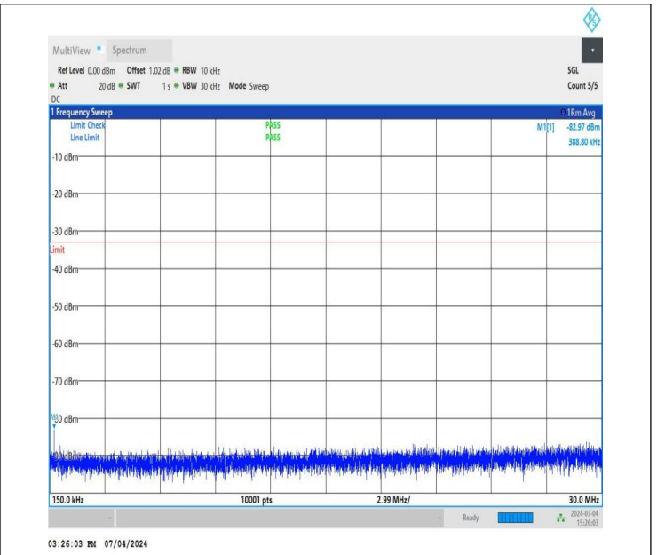
NTNV_DC_26A_n78A-3450-3550_PC3_30_5+40_M+H_TID1_N S_01_0.15_30_#1
