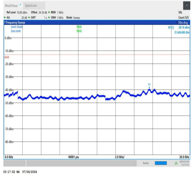
NTNV_DC_26A_n78A-3450-3550_PC3_30_5+40_M+L_TID1_NS_01_6000_26000_#1
