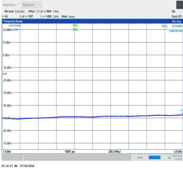
NTNV_DC_26A_n78A-3450-3550_PC3_30_5+30_M+H_TID5_N S_01_1000_3000_#1
