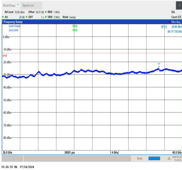
NTNV_DC_26A_n78A-3450-3550_PC3_30_5+40_M+M_TID4_N S_01_26000_40000_#1
