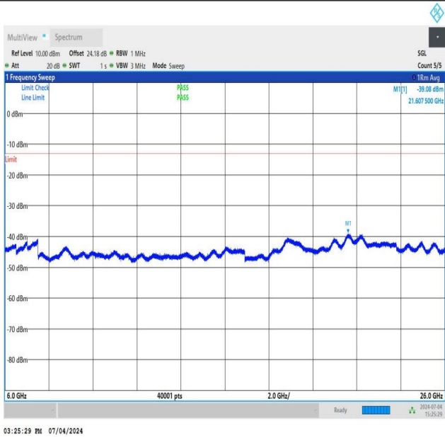
NTNV_DC_26A_n78A-3450-3550_PC3_30_5+40_M+M_TID5_N S_01_6000_26000_#1
