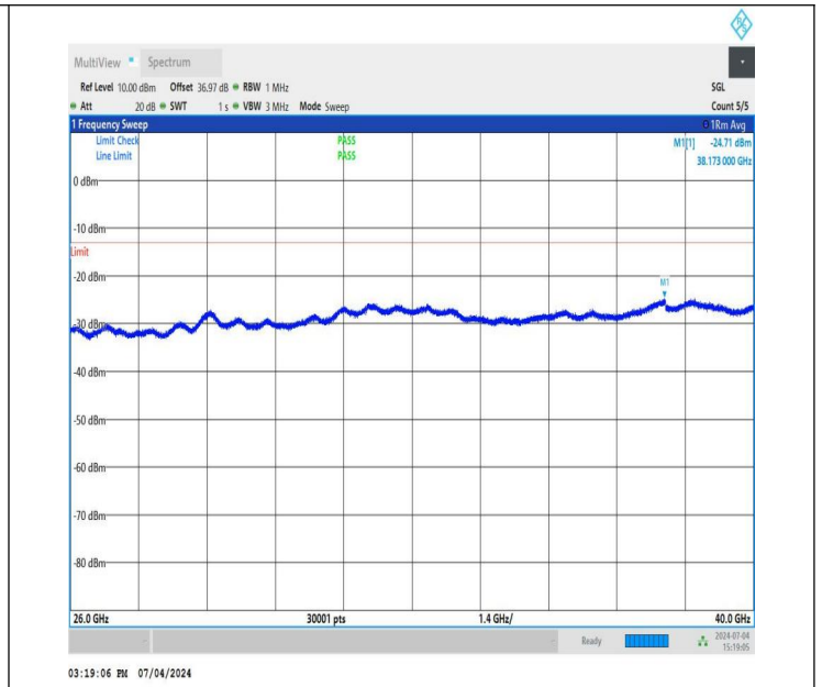
NTNV_DC_26A_n78A-3450-3550_PC3_30_5+40_M+L_TID2_NS_01_26000_40000_#1
