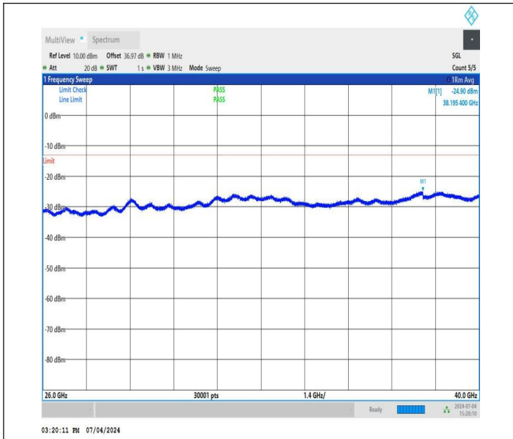
NTNV_DC_26A_n78A-3450-3550_PC3_30_5+40_M+L_TID4_NS_01_26000_40000_#1
