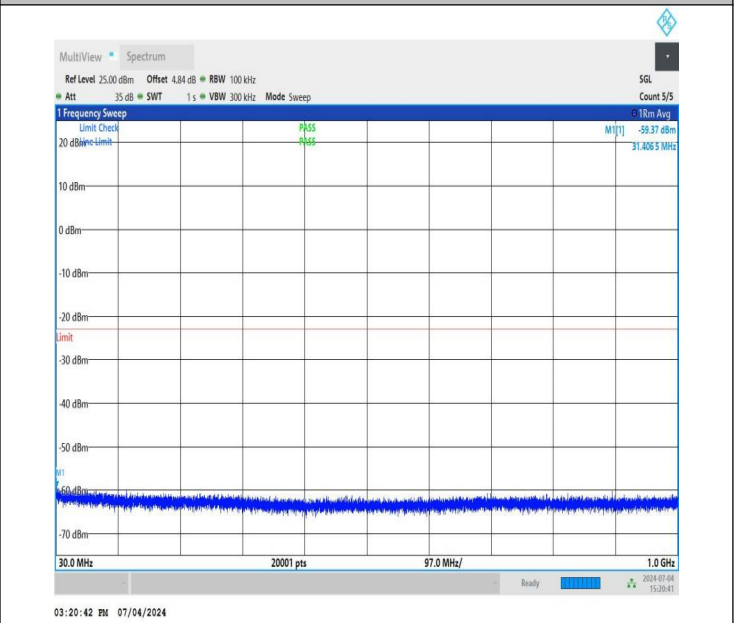
NTNV_DC_26A_n78A-3450-3550_PC3_30_5+40_M+L_TID5_NS_01_30_1000_#1
