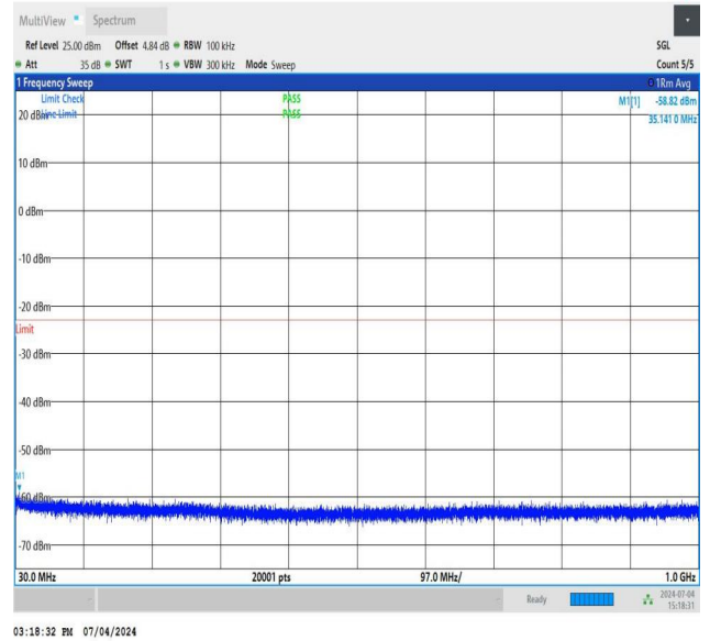
NTNV_DC_26A_n78A-3450-3550_PC3_30_5+40_M+L_TID2_NS _01_30_1000_#1
