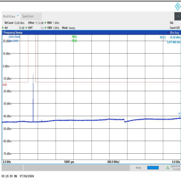
NTNV_DC_26A_n78A-3450-3550_PC3_30_5+30_M+H_TID4_N S_01_3000_6000_#1
