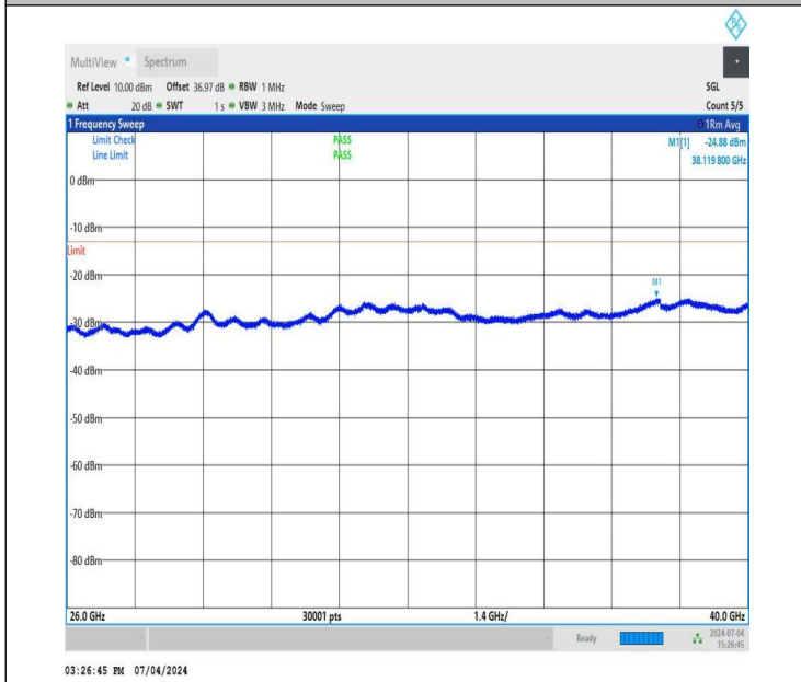
NTNV_DC_26A_n78A-3450-3550_PC3_30_5+40_M+H_TID1_N S_01_26000_40000_#1
