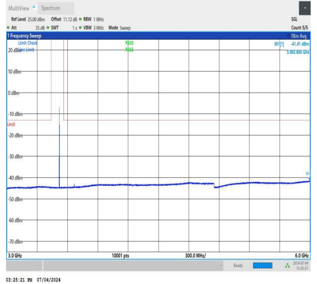
NTNV_DC_26A_n78A-3450-3550_PC3_30_5+40_M+M_TID5_N S_01_3000_6000_#1
