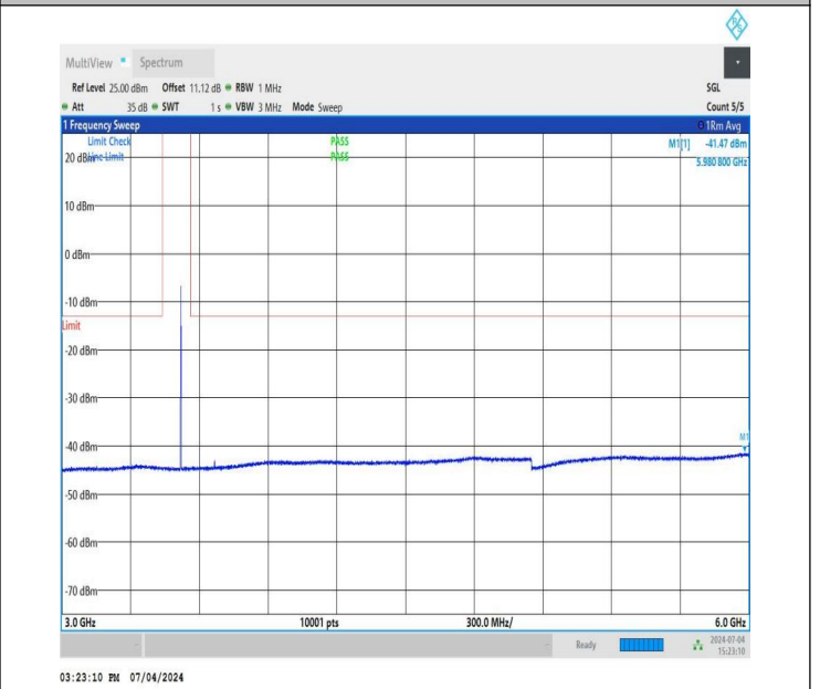
NTNV_DC_26A_n78A-3450-3550_PC3_30_5+40_M+M_TID2_N S_01_3000_6000_#1
