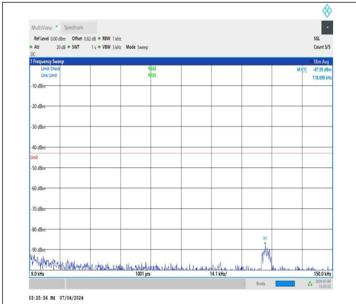
NTNV_DC_26A_n78A-3450-3550_PC3_30_5+40_M+H_TID1_N S_01_0.009_0.15_#1
