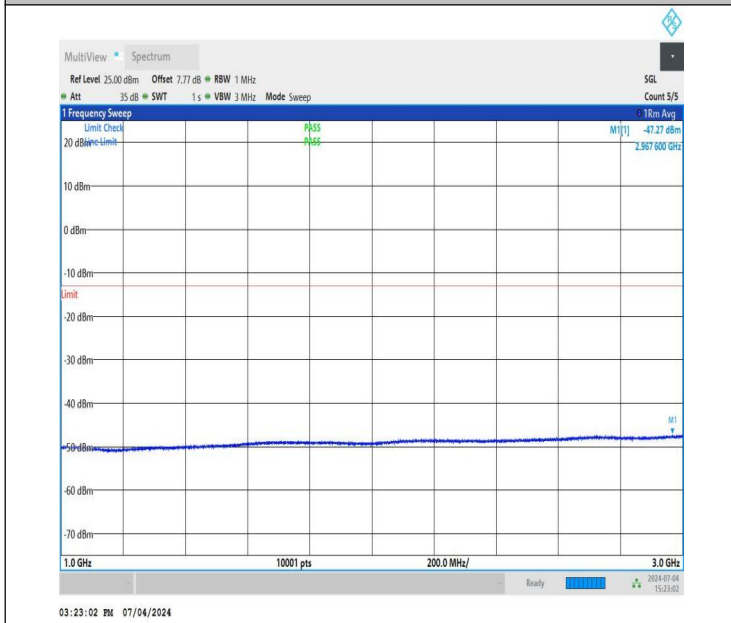
NTNV_DC_26A_n78A-3450-3550_PC3_30_5+40_M+M_TID2_N S_01_1000_3000_#1
