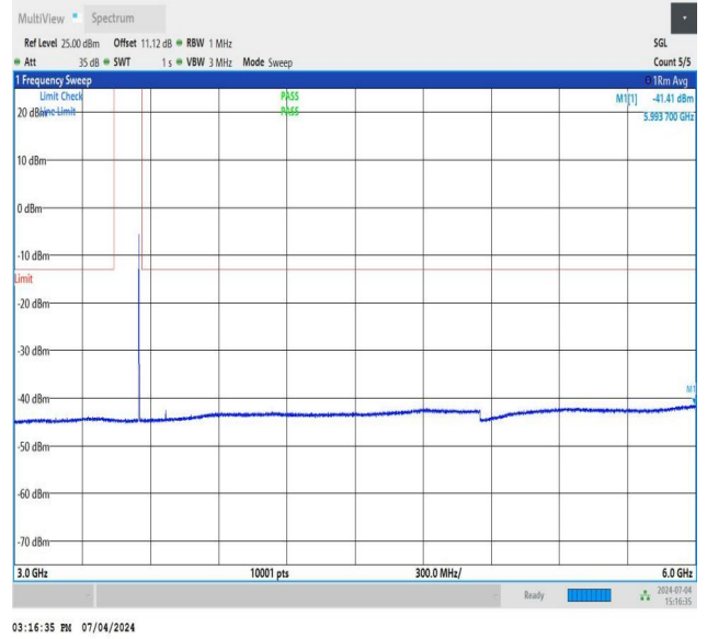
NTNV_DC_26A_n78A-3450-3550_PC3_30_5+30_M+H_TID5_N S_01_3000_6000_#1
