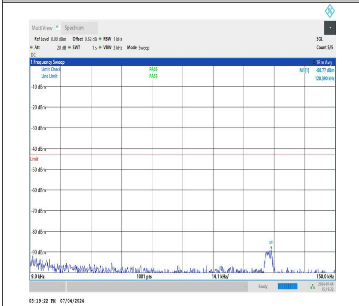
NTNV_DC_26A_n78A-3450-3550_PC3_30_5+40_M+L_TID4_NS_01_0.009_0.15_#1
