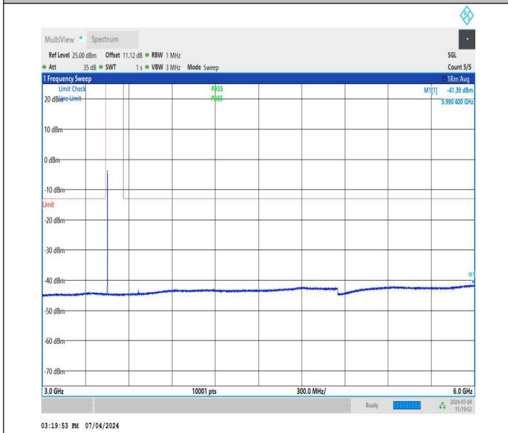
NTNV_DC_26A_n78A-3450-3550_PC3_30_5+40_M+L_TID4_NS_01_3000_6000_#1
