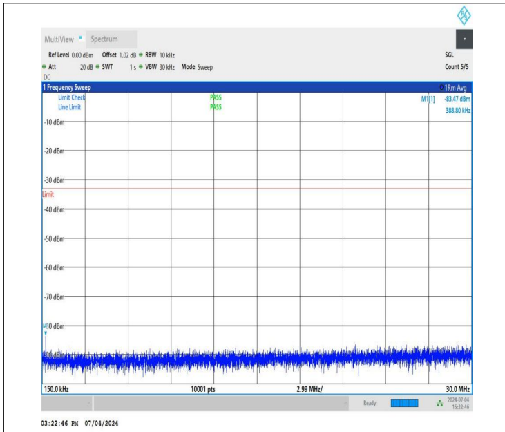
NTNV_DC_26A_n78A-3450-3550_PC3_30_5+40_M+M_TID2_N S_01_0.15_30_#1
