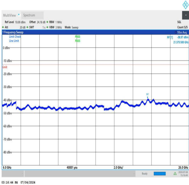
NTNV_DC_26A_n78A-3450-3550_PC3_30_5+30_M+H_TID5_N S_01_6000_26000_#1
