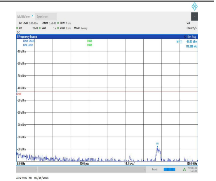
NTNV_DC_26A_n78A-3450-3550_PC3_30_5+40_M+H_TID2_N S_01_0.009_0.15_#1
