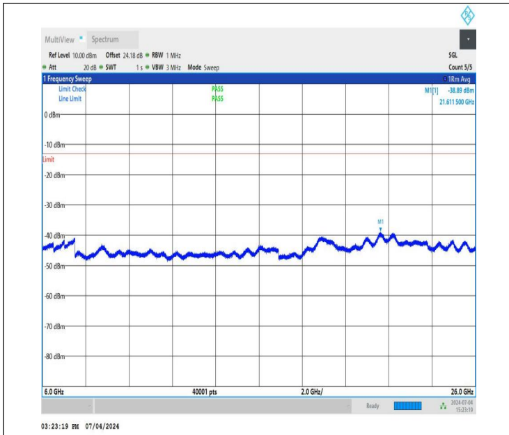
NTNV_DC_26A_n78A-3450-3550_PC3_30_5+40_M+M_TID2_N S_01_6000_26000_#1
