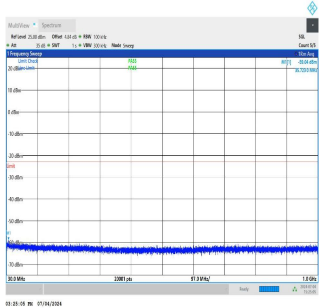
NTNV_DC_26A_n78A-3450-3550_PC3_30_5+40_M+M_TID5_N S_01_30_1000_#1
