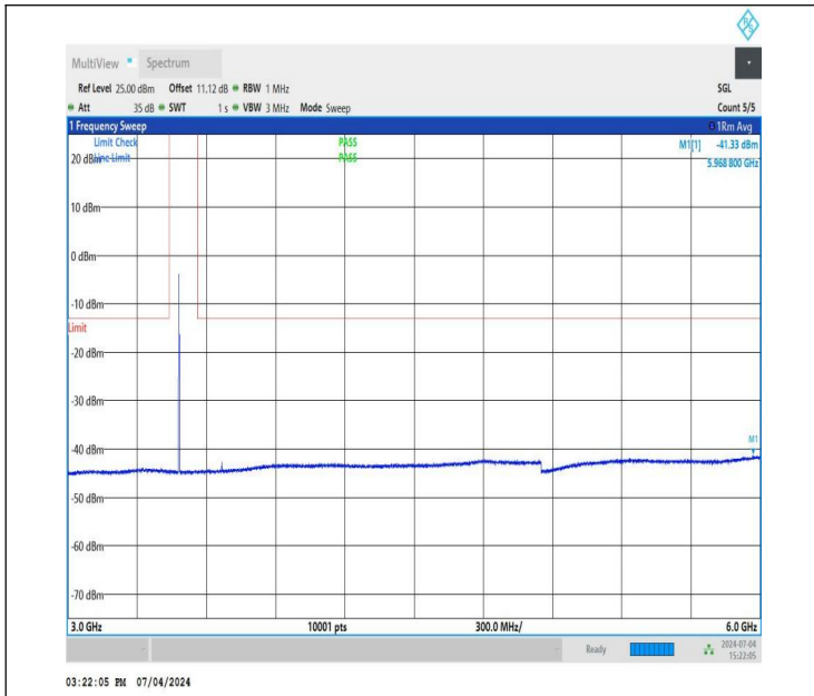
NTNV_DC_26A_n78A-3450-3550_PC3_30_5+40_M+M_TID1_N S_01_3000_6000_#1
