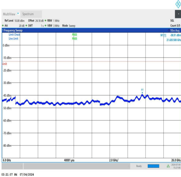
NTNV_DC_26A_n78A-3450-3550_PC3_30_5+40_M+L_TID5_NS_01_6000_26000_#1
