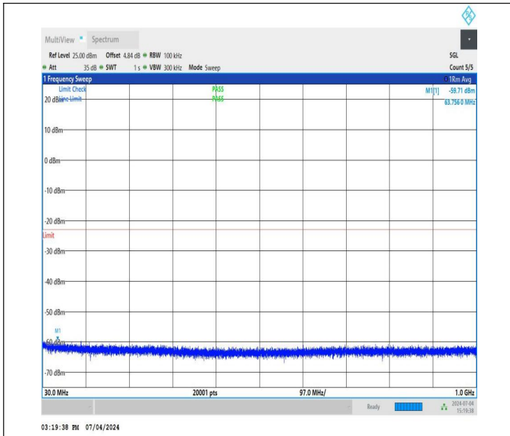
NTNV_DC_26A_n78A-3450-3550_PC3_30_5+40_M+L_TID4_NS_01_30_1000_#1
