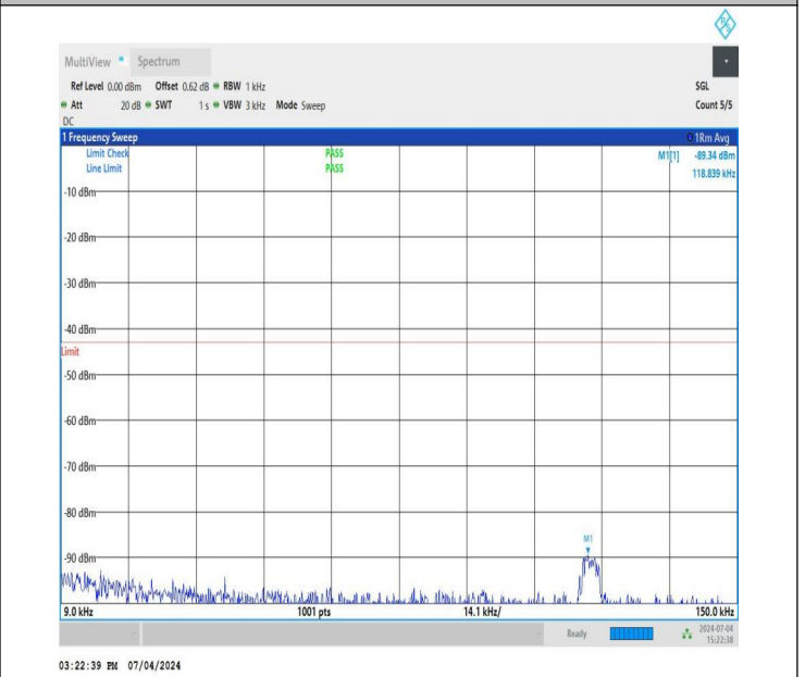
NTNV_DC_26A_n78A-3450-3550_PC3_30_5+40_M+M_TID2_N S_01_0.009_0.15_#1
