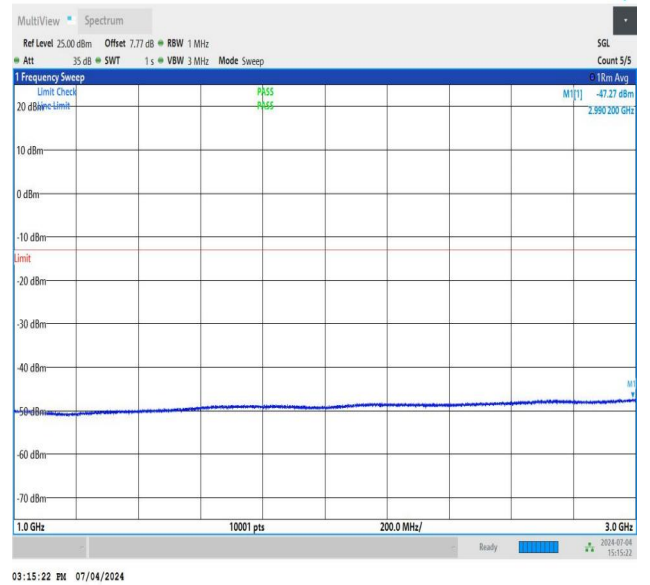
NTNV_DC_26A_n78A-3450-3550_PC3_30_5+30_M+H_TID4_N S_01_1000_3000_#1
