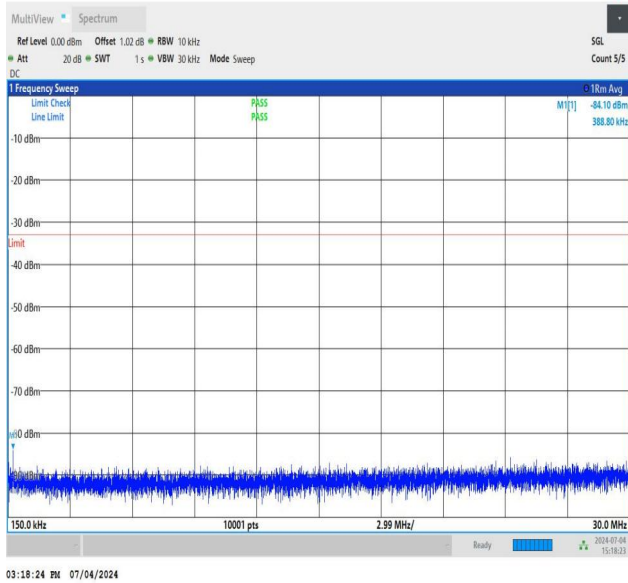
NTNV_DC_26A_n78A-3450-3550_PC3_30_5+40_M+L_TID2_NS _01_0.15_30_#1
