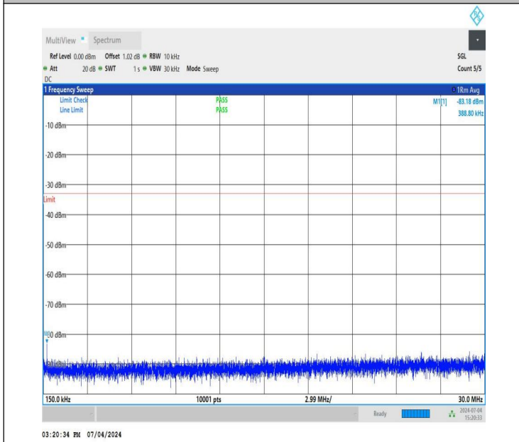
NTNV_DC_26A_n78A-3450-3550_PC3_30_5+40_M+L_TID5_NS_01_0.15_30_#1
