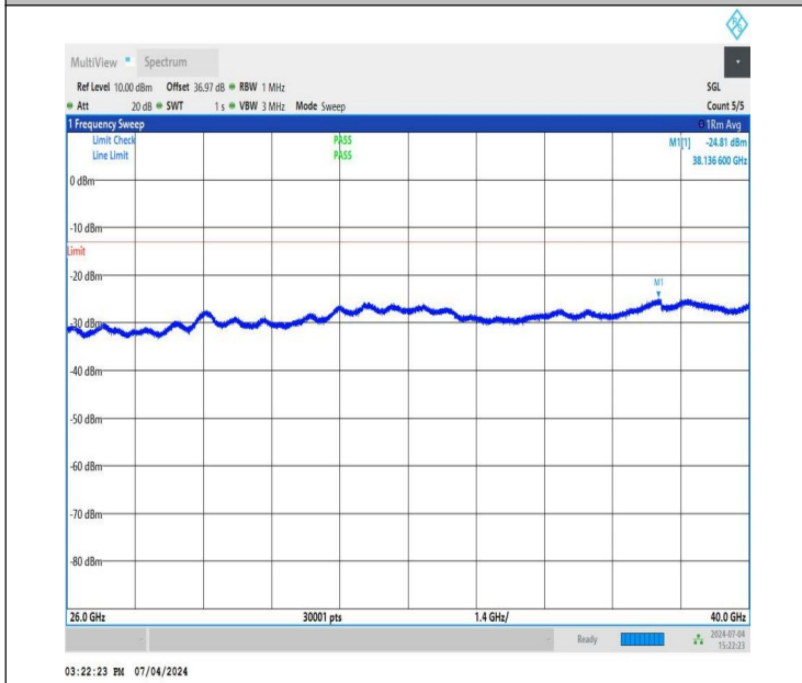
NTNV_DC_26A_n78A-3450-3550_PC3_30_5+40_M+M_TID1_N S_01_26000_40000_#1
