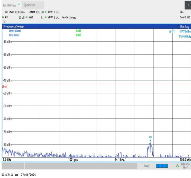
NTNV_DC_26A_n78A-3450-3550_PC3_30_5+40_M+L_TID1_NS_01_0.009_0.15_#1
