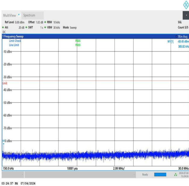
NTNV_DC_26A_n78A-3450-3550_PC3_30_5+40_M+M_TID5_N S_01_0.15_30_#1
