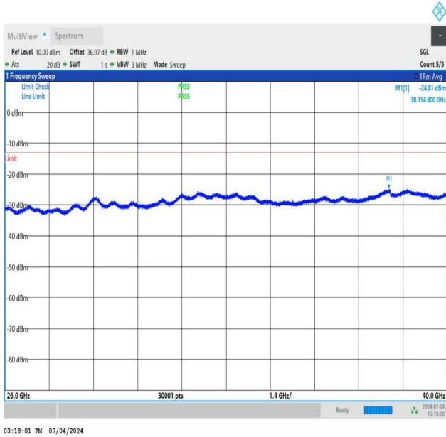
NTNV_DC_26A_n78A-3450-3550_PC3_30_5+40_M+L_TID1_NS_01_26000_40000_#1
