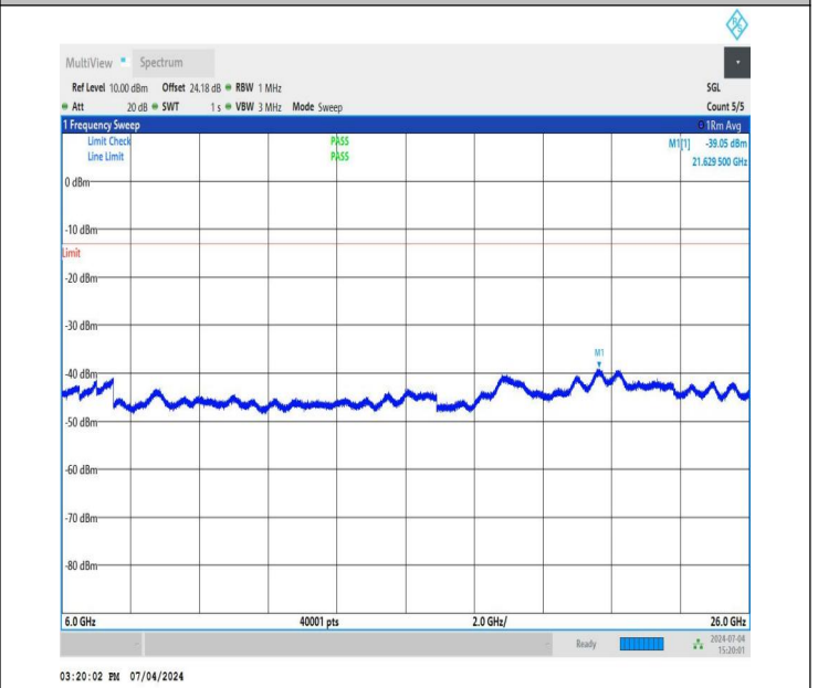
NTNV_DC_26A_n78A-3450-3550_PC3_30_5+40_M+L_TID4_NS_01_6000_26000_#1
