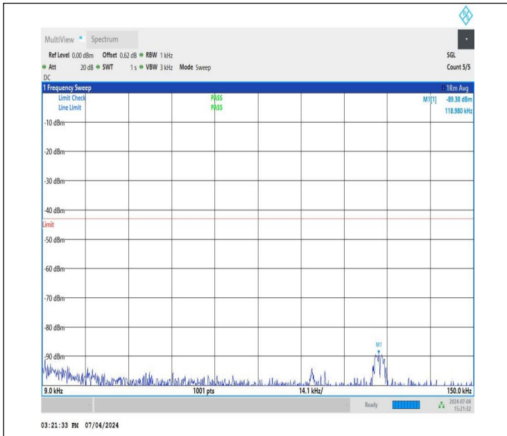
NTNV_DC_26A_n78A-3450-3550_PC3_30_5+40_M+M_TID1_N S_01_0.009_0.15_#1
