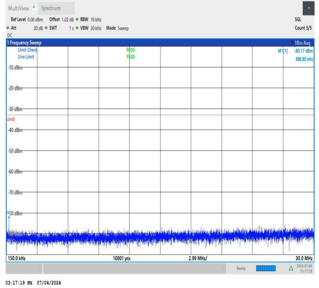
NTNV_DC_26A_n78A-3450-3550_PC3_30_5+40_M+L_TID1_NS_01_0.15_30_#1
