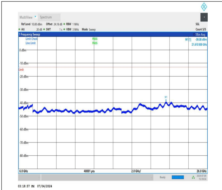
NTNV_DC_26A_n78A-3450-3550_PC3_30_5+40_M+L_TID2_NS_01_6000_26000_#1
