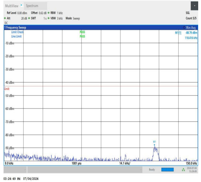
NTNV_DC_26A_n78A-3450-3550_PC3_30_5+40_M+M_TID5_N S_01_0.009_0.15_#1
