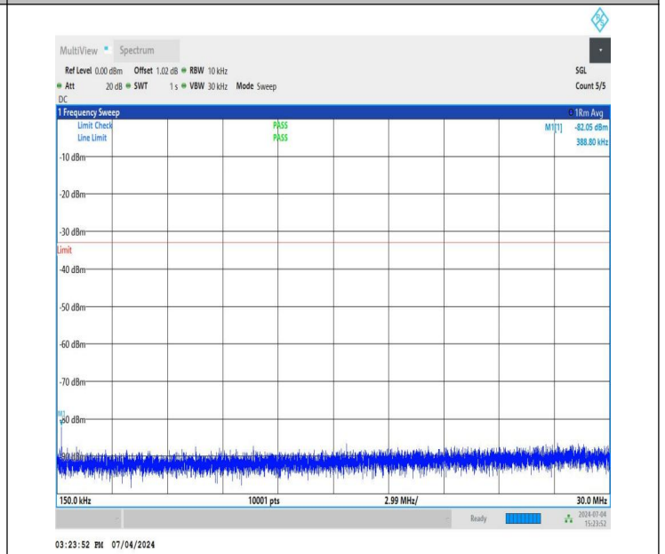
NTNV_DC_26A_n78A-3450-3550_PC3_30_5+40_M+M_TID4_N S_01_0.15_30_#1
