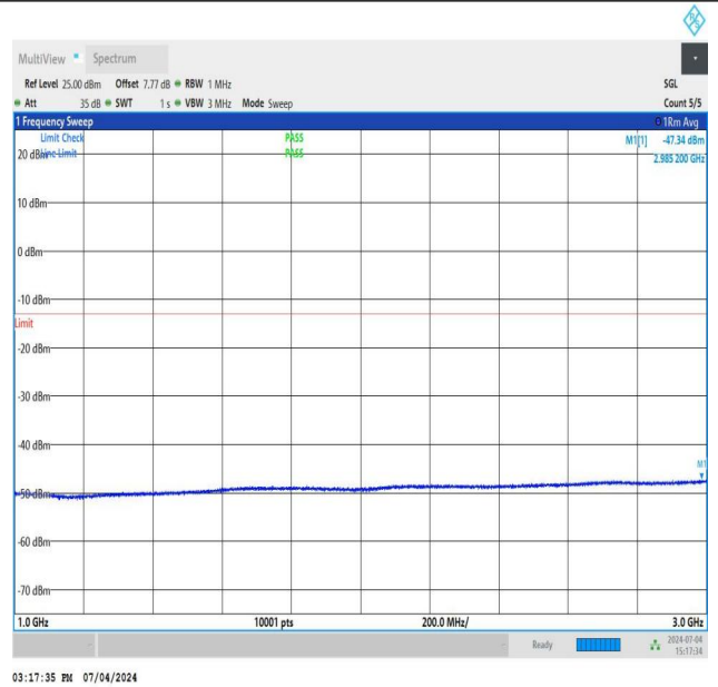
NTNV_DC_26A_n78A-3450-3550_PC3_30_5+40_M+L_TID1_NS_01_1000_3000_#1
