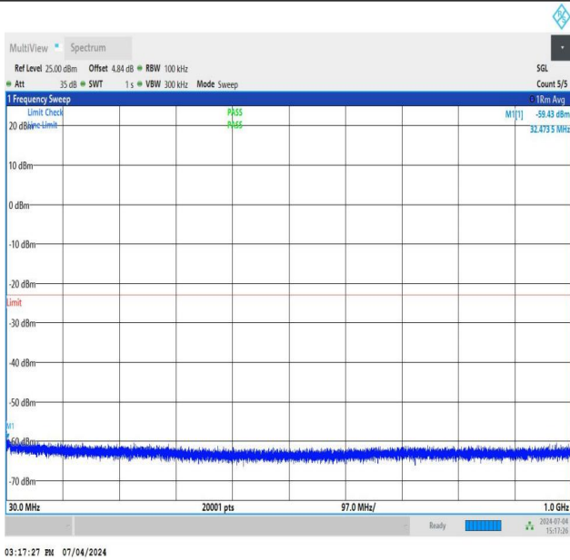
NTNV_DC_26A_n78A-3450-3550_PC3_30_5+40_M+L_TID1_NS_01_30_1000_#1
