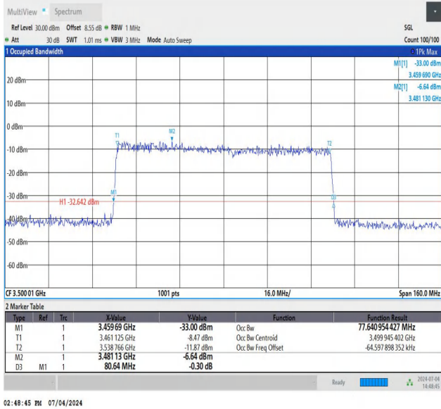
NTNV_DC_26A_n78A-3450-3550_PC3_30_5+80_M+M_TID6_A nt1#1
