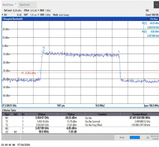
NTNV_DC_26A_n78A-3450-3550_PC3_30_5+90_M+M_TID8_A nt1#1
