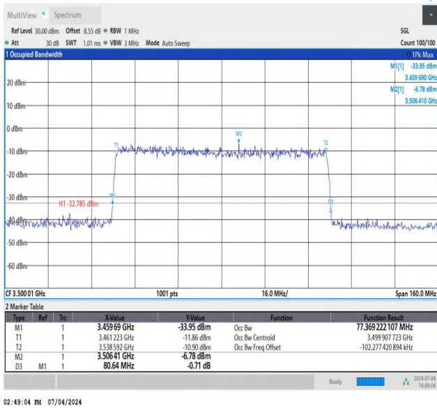
NTNV_DC_26A_n78A-3450-3550_PC3_30_5+80_M+M_TID8_A nt1#1
