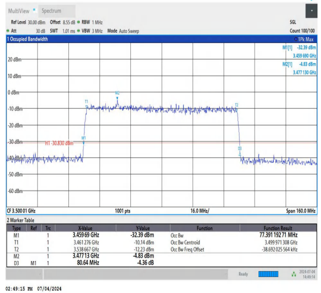
NTNV_DC_26A_n78A-3450-3550_PC3_30_5+80_M+M_TID9_A nt1#1
