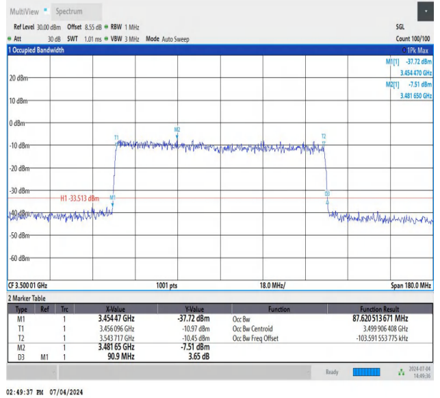
NTNV_DC_26A_n78A-3450-3550_PC3_30_5+90_M+M_TID7_A nt1#1
