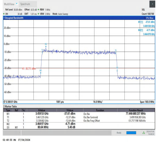
NTNV_DC_26A_n78A-3450-3550_PC3_30_5+80_M+M_TID7_A nt1#1
