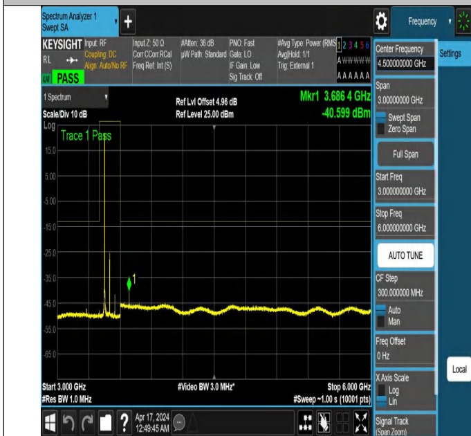
NTNV_N78-3450-3550_PC2_30_100_H_TID5_NS_01_3000_600_0_#1
