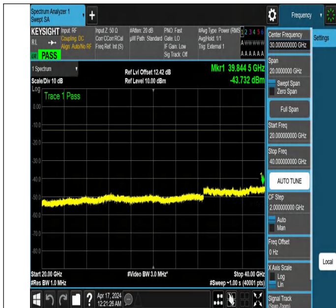
NTNV_N78-3450-3550_PC2_30_100_M_TID5_NS_01_20000_4 0000 #1
