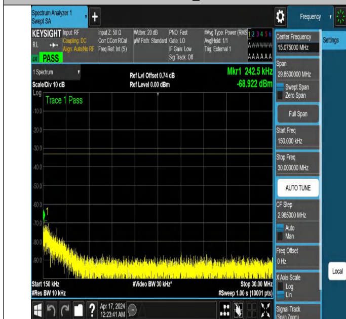
NTNV_N78-3450-3550_PC2_30_100_M_TID6_NS_01_0.15_30_#1
