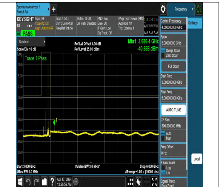
NTNV_N78-3450-3550_PC2_30_100_M_TID6_NS_01_3000_60 00 #1
