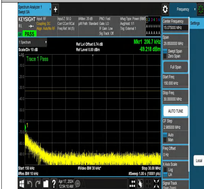
NTNV_N78-3450-3550_PC2_30_100_H_TID6_NS_01_0.15_30_#1
