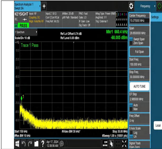
NTNV_N78-3450-3550_PC2_30_100_H_TID3_NS_01_0.15_30_
