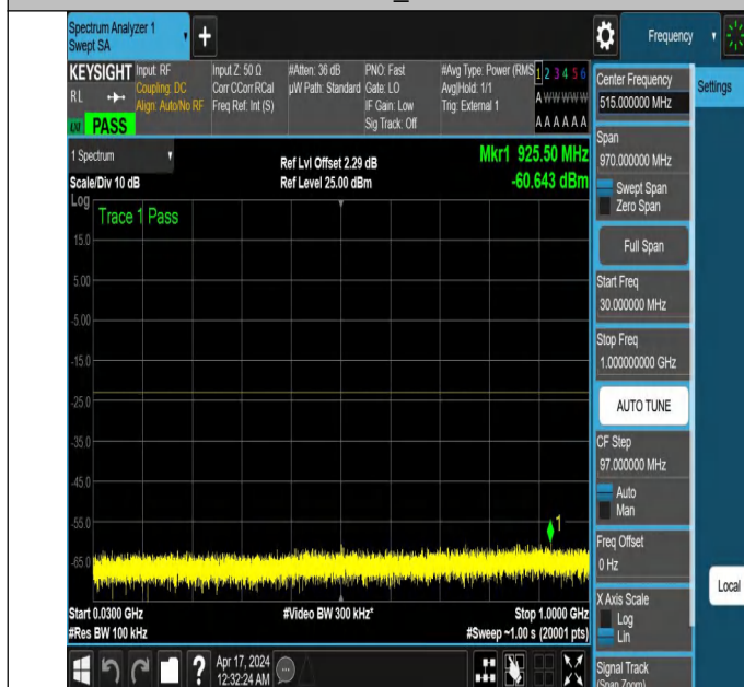
NTNV_N78-3450-3550_PC2_30_100_H_TID2_NS_01_30_1000
