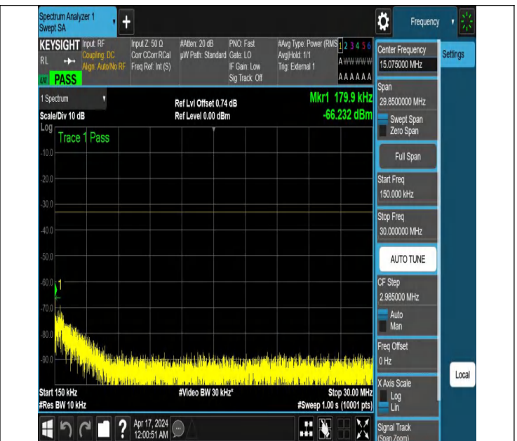
NTNV_N78-3450-3550_PC2_30_100_M_TID2_NS_01_0.15_30_
