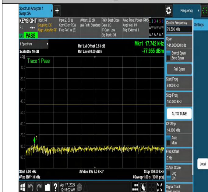
NTNV_N78-3450-3550_PC2_30_100_M_TID5_NS_01_0.009_0. 15 #1
